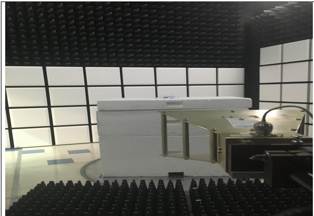
Radiated Measurement 1-18 GHz
