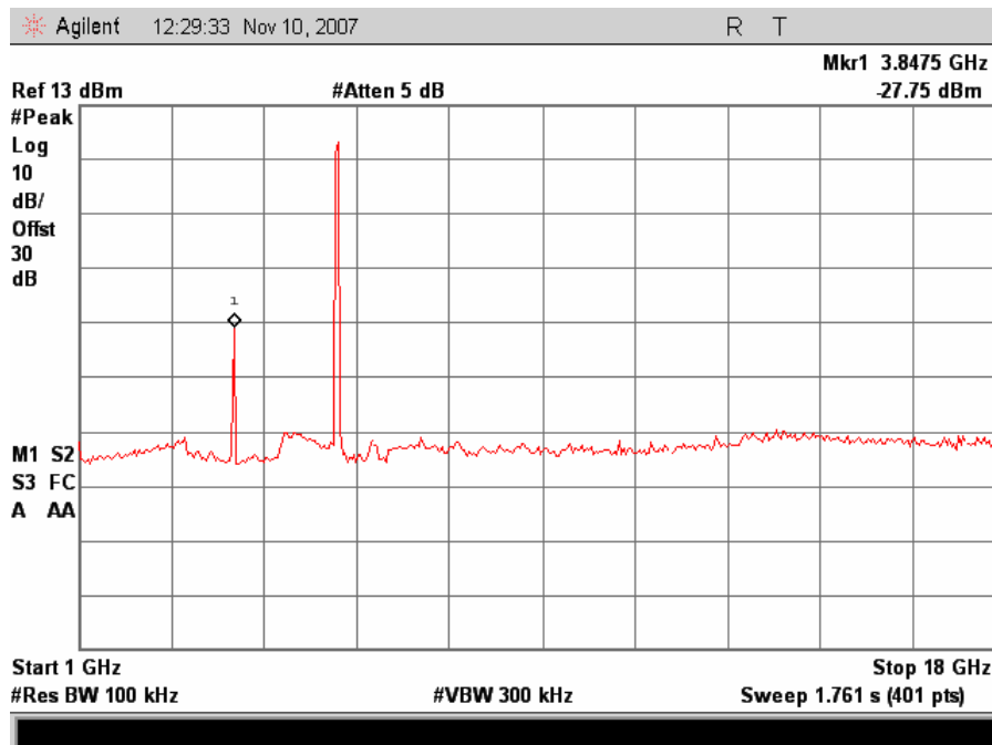
802.11/a – Low Channel Conducted Emissions 1-18GHz
