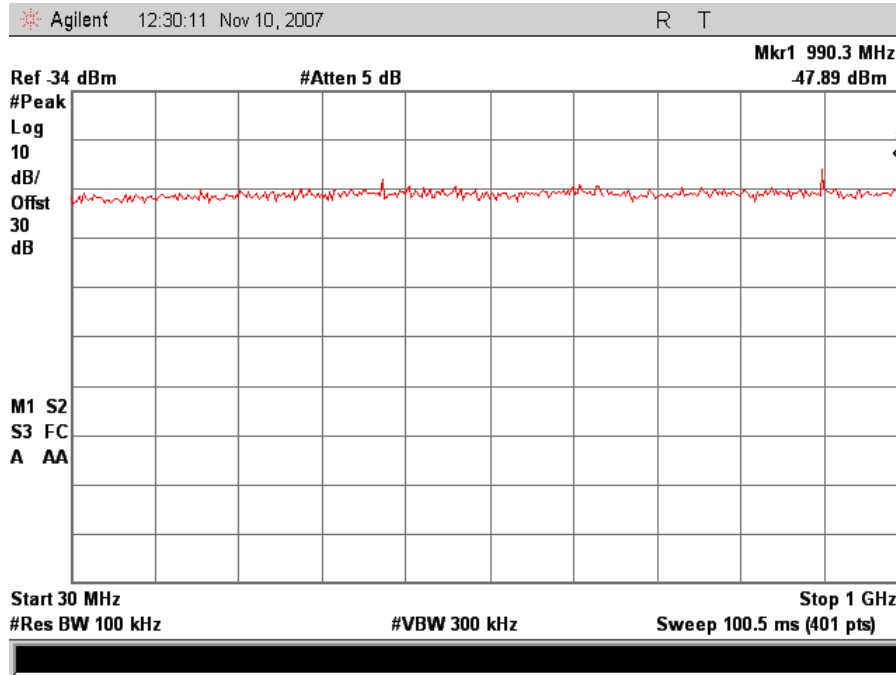
802.11/a – Low Channel Conducted Emissions 30MHz- 1GHz
