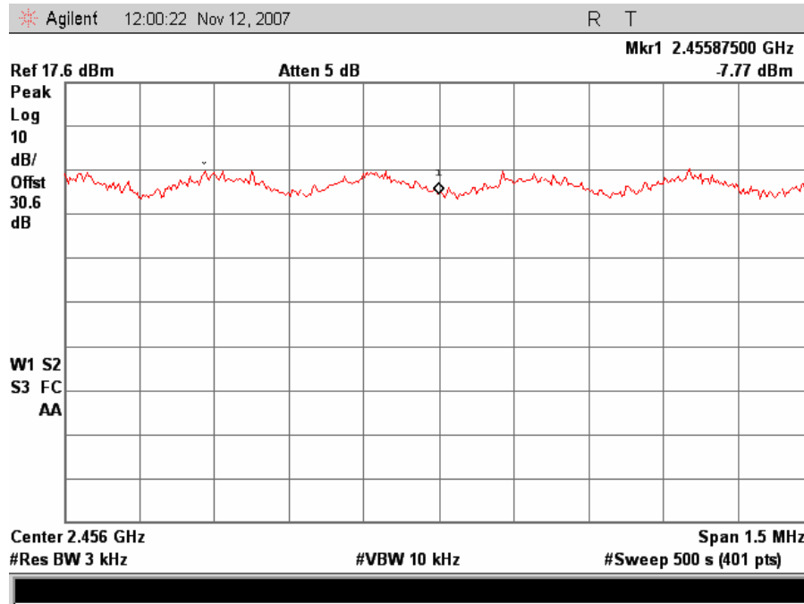
802.11/g – High Channel 10 Peak Power Spectral Density
