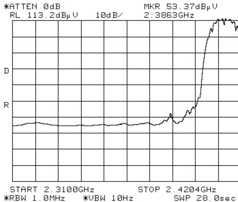
802.11/b radiated restricted band 2310- 2390 MHz Avg
