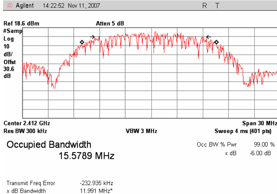
Plot 3. 802.11/b Low Ch Occupied Band Width.
