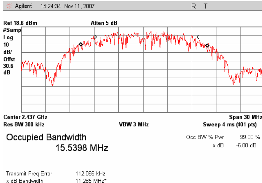
Plot 4. 802.11/b Mid Ch Occupied Band Width
