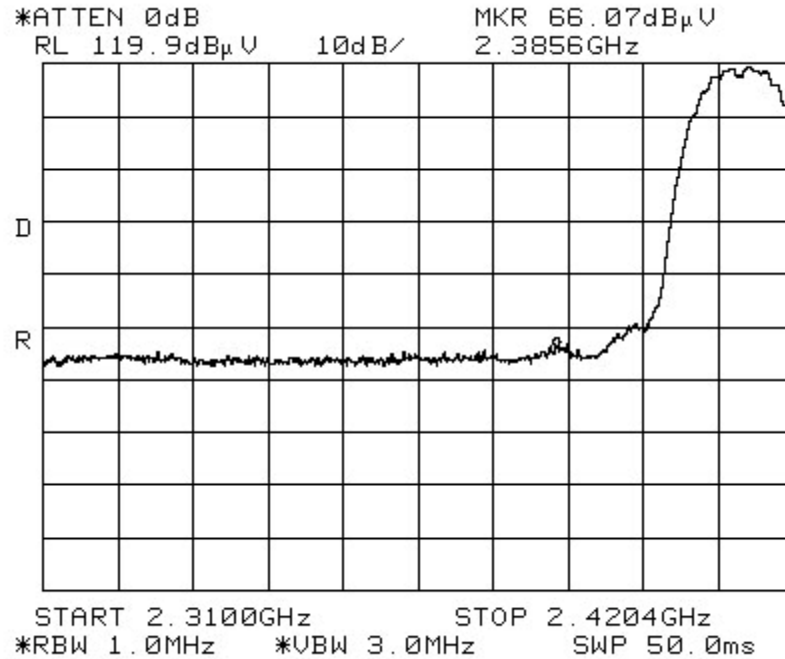
802.11/b radiated restricted band 2310- 2390 MHz Peak
