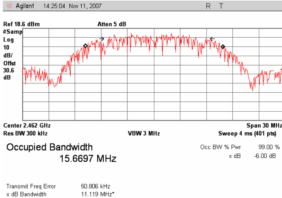
Plot 5. 802.11/b High Ch Occupied Band Width
