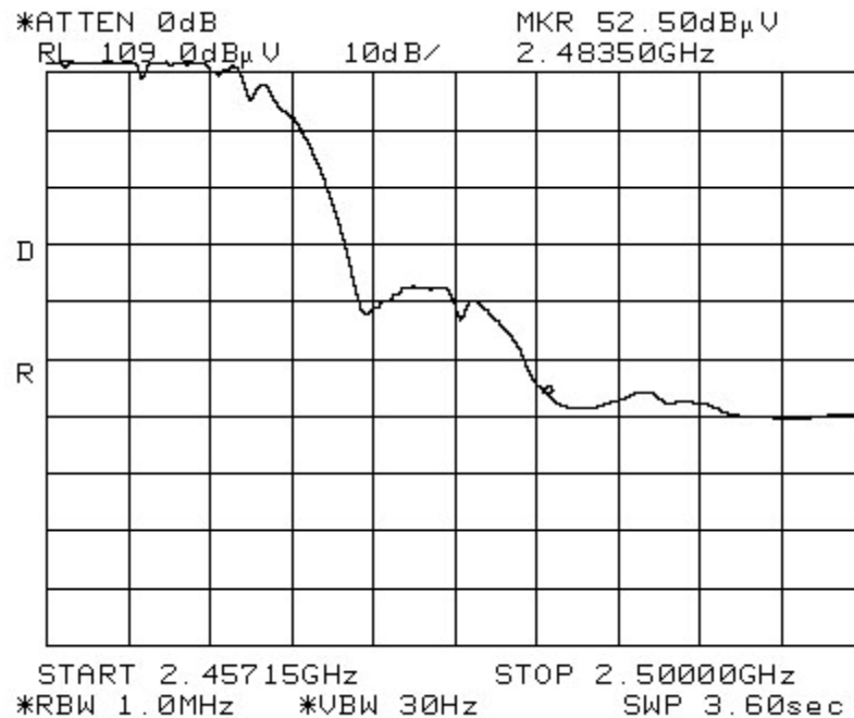
802.11/b radiated restricted band 2483.5 – 2500MHz Avg
