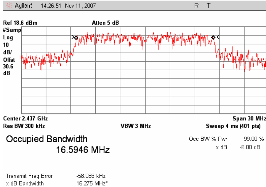
Plot 7. 802.11/g Mid Ch Occupied Band Width
