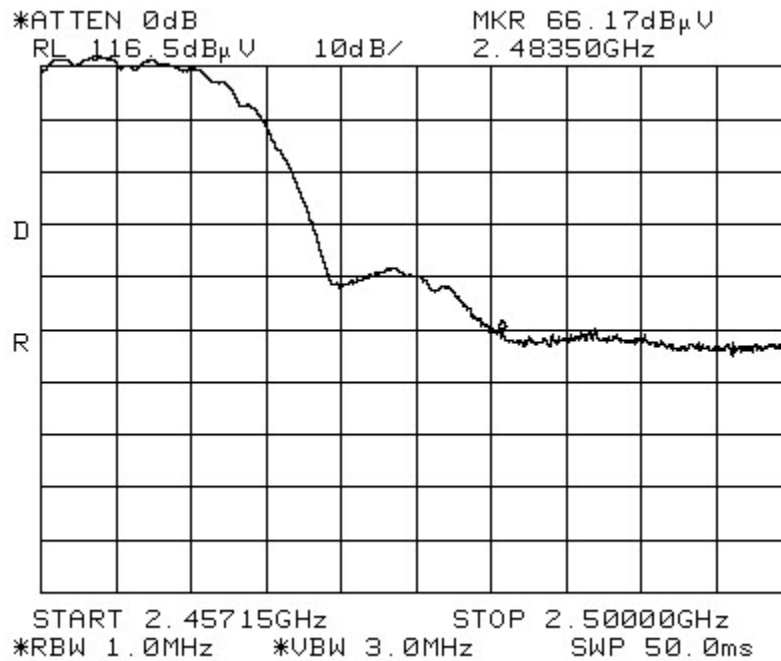
802.11/b radiated restricted band 2483.5 – 2500MHz Peak
