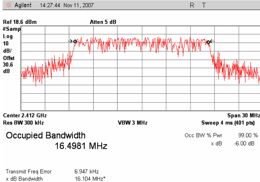
Plot 6. 802.11/g Low Ch Occupied Band Width
