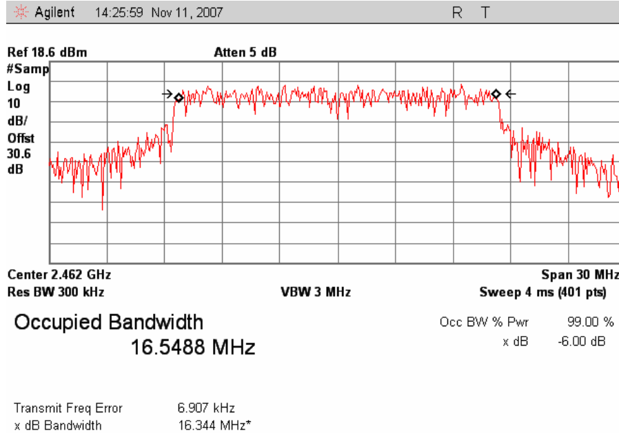
Plot 8. 802.11/g High Ch Occupied Band Width
