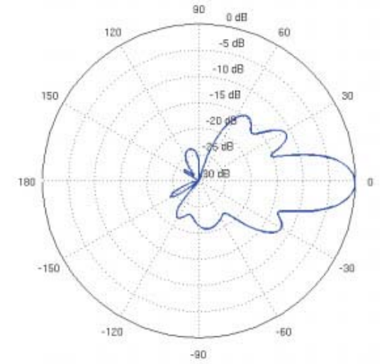
Vertical Elevation
