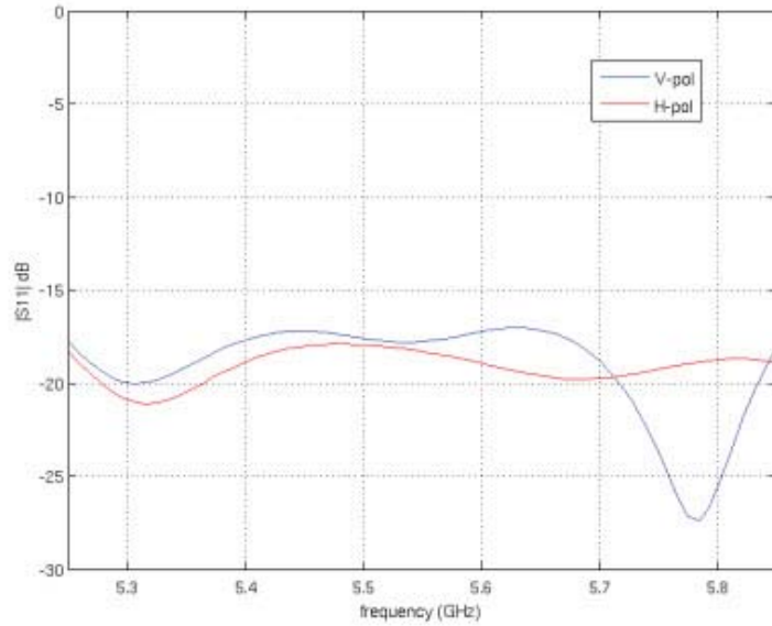
Return Loss
