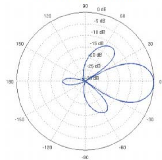
Horizontal Elevation
