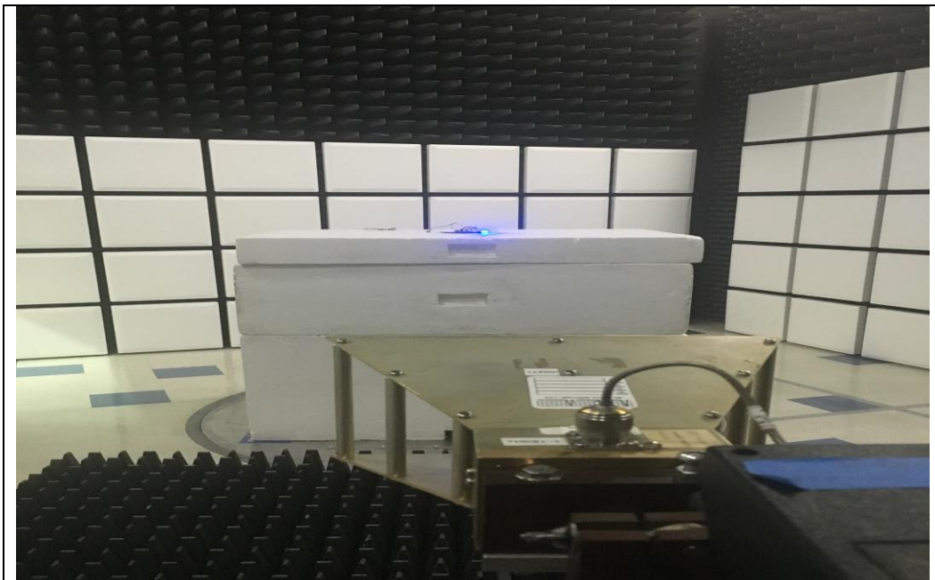
Radiated Measurement 1-18 GHz
