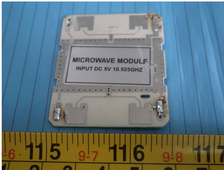
EUT – Antenna Top Shielding off View
