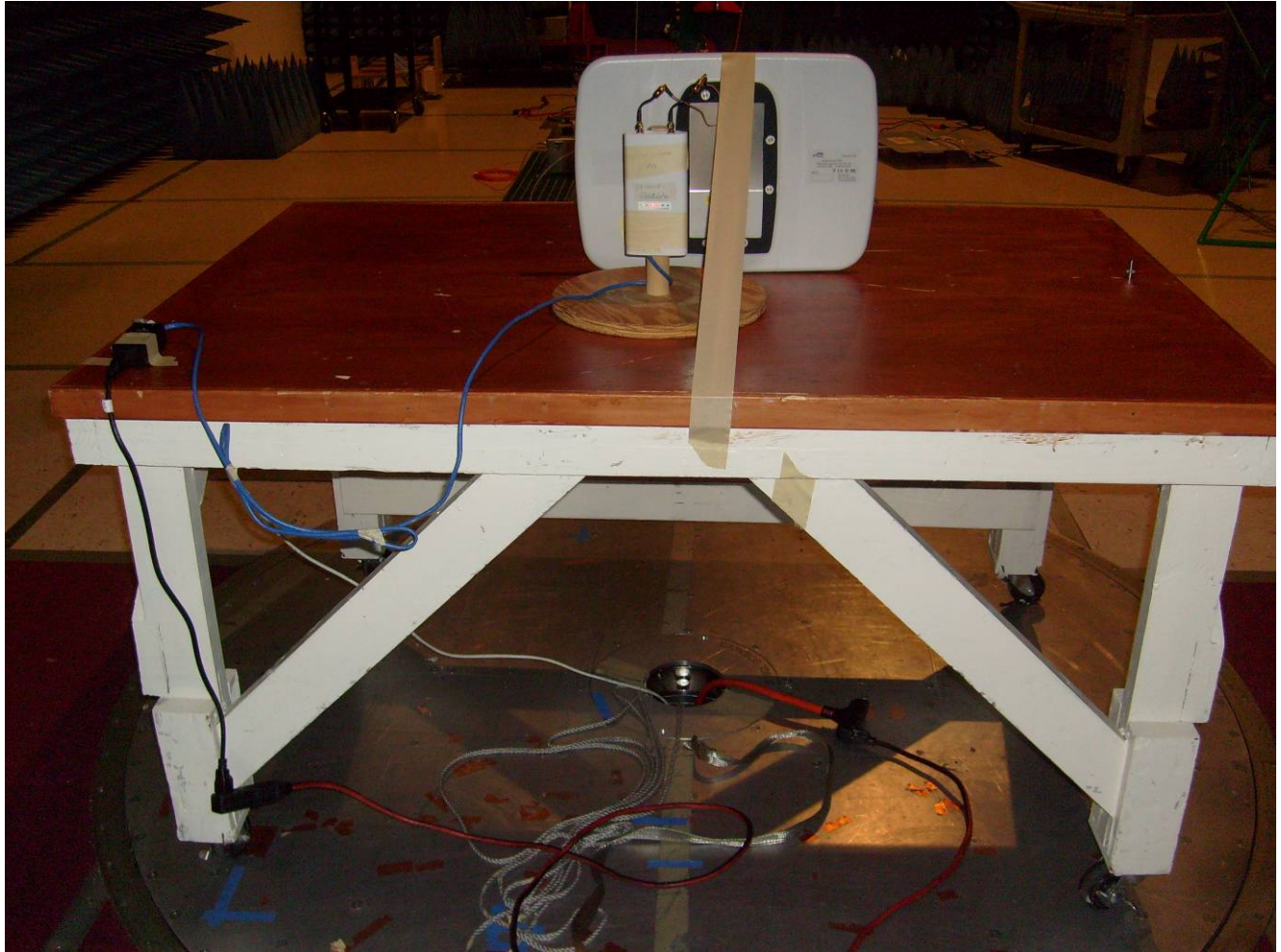
Photograph 4. Radiated Emission, Test Setup Back View
