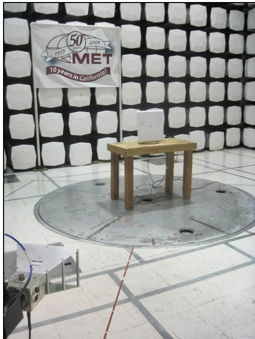
Photograph 3. Radiated Emissions, Test Setup, 1 GHz – 18 GHz
