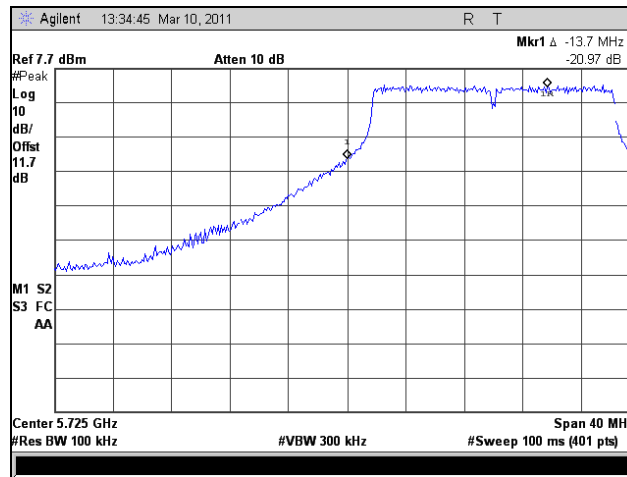
Plot 355. Conducted Band Edge, HT20, Low Channel, Port 2
