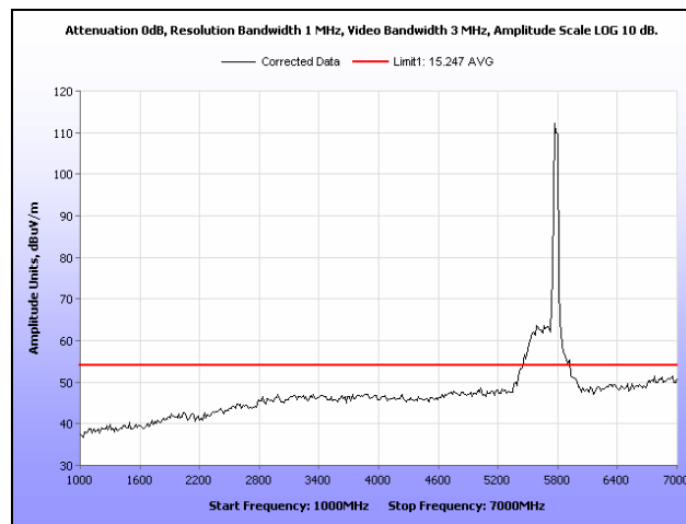
Plot 218. Radiated Spurious Emissions, HT40, Mid Channel, 1 GHz – 7 GHz, Average
