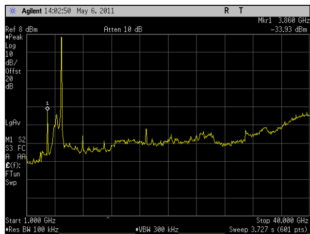
Plot 330. Conducted Spurious, High Channel, HT40, Port 1, 1 GHz - 40 GHz
