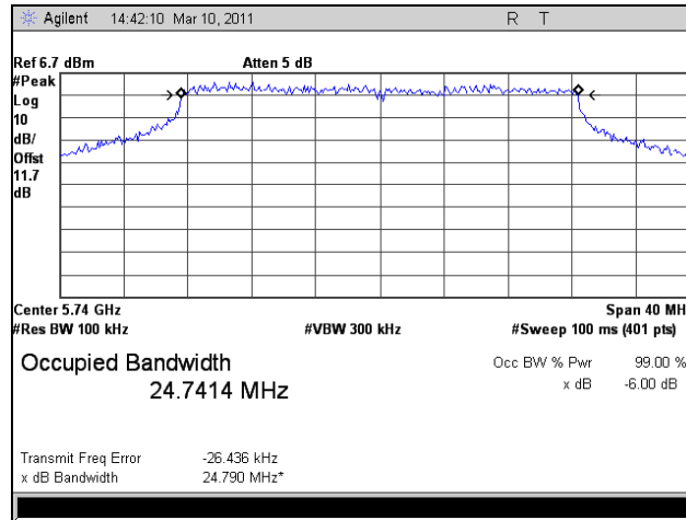
Plot 37. 6 dB Occupied Bandwidth, HT30, Port 1, Low Channel
