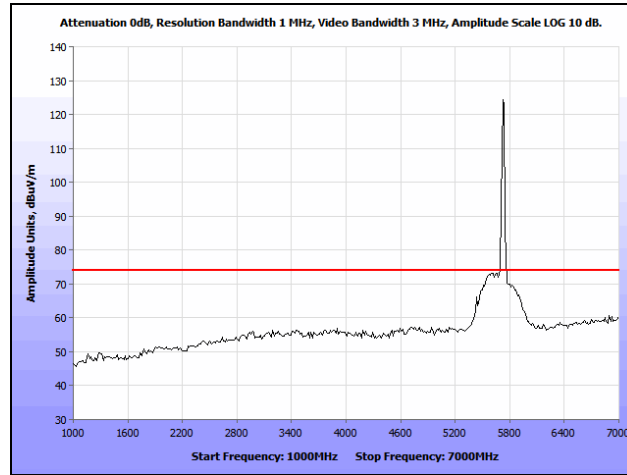
Plot 94. Radiated Spurious Emissions, Low Channel, 802.11a 20MHz, 1 GHz – 7 GHz, Peak
