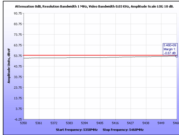
Plot 147. Restricted Band, HT8, Mid Channel
