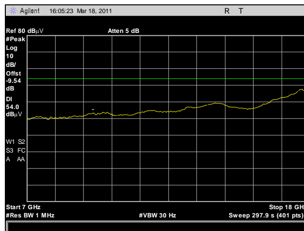
Plot 203. Radiated Spurious Emissions, HT30, Mid Channel, 7 GHz – 18 GHz, Average
