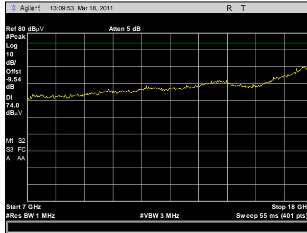
Plot 150. Radiated Spurious Emissions, HT8, Mid Channel, 7 GHz – 18 GHz, Peak
