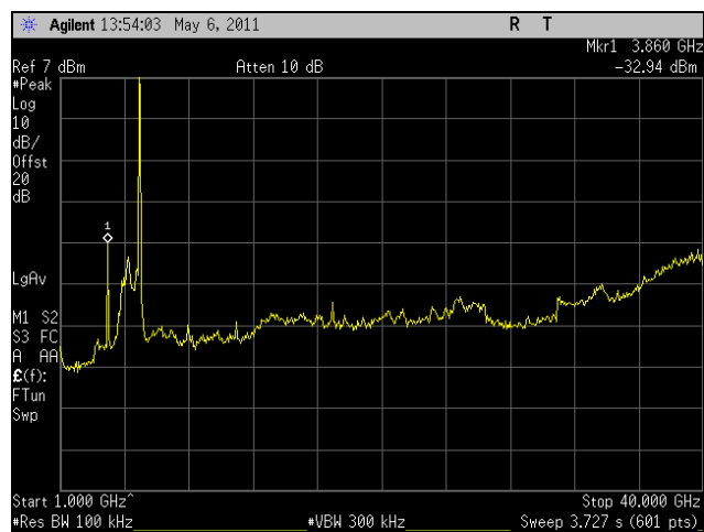
Plot 318. Conducted Spurious, High Channel, HT30, Port 1, 1 GHz - 40 GHz
