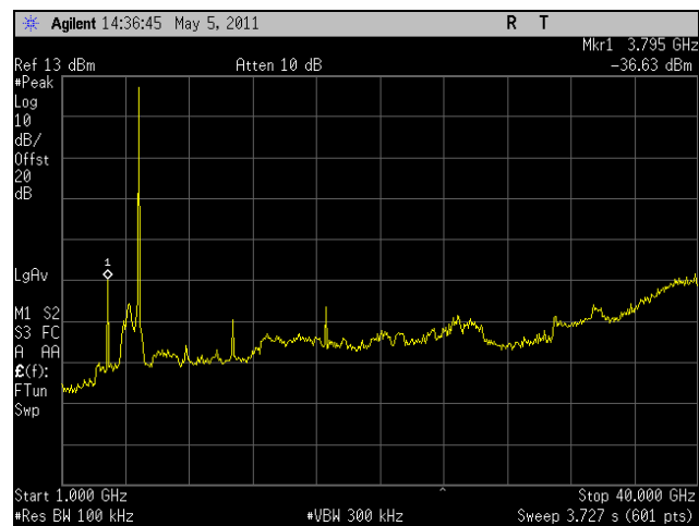
Plot 278. Conducted Spurious, Low Channel, HT8, Port 1, 1 GHz - 40 GHz
