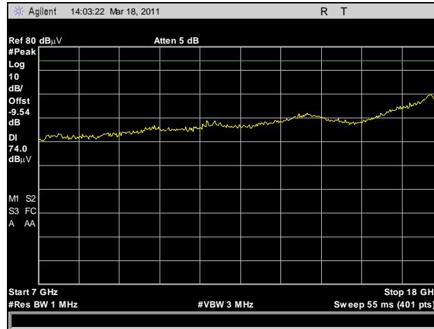
Plot 186. Radiated Spurious Emissions, HT20, Mid Channel, 7 GHz – 18 GHz, Peak
