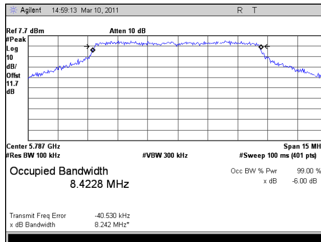
Plot 26. 6 dB Occupied Bandwidth, HT10, Port 1, Mid Channel
