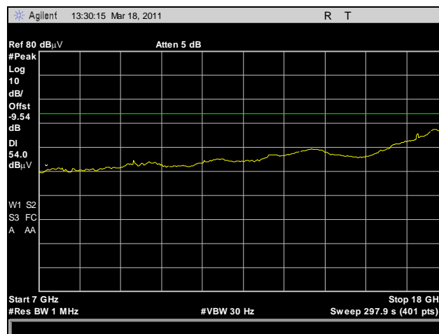
Plot 143. Radiated Spurious Emissions, HT8, Low Channel, 7 GHz – 18 GHz, Average
