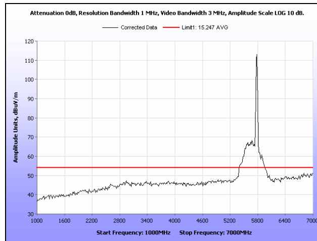
Plot 200. Radiated Spurious Emissions, HT30, Mid Channel, 1 GHz – 7 GHz, Average
