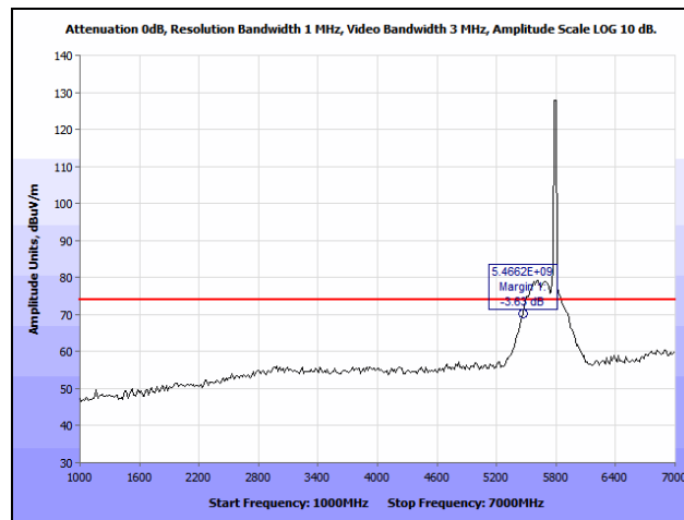
Plot 166. Radiated Spurious Emissions, HT10, Mid Channel, 1 GHz – 7 GHz, Peak
