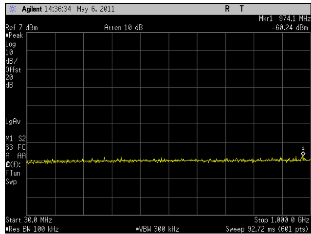
Plot 257. Conducted Spurious, High Channel, 802.11a 20 MHz, 30 MHz - 1 GHz
