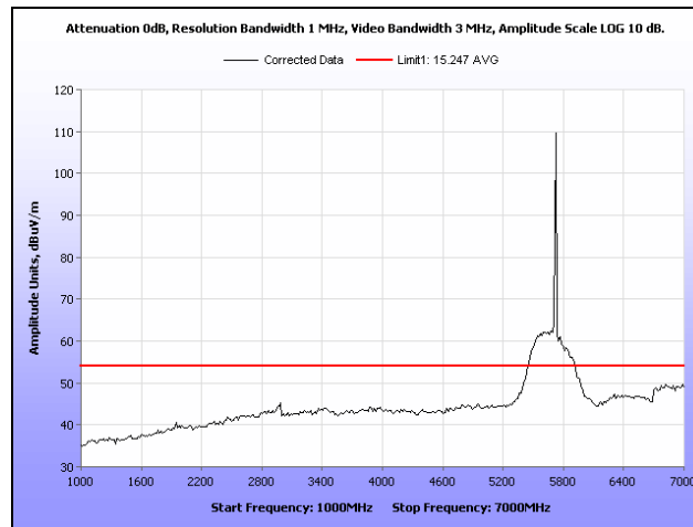
Plot 122. Radiated Spurious Emissions, HT5, Low Channel, 1 GHz – 7 GHz, Average
