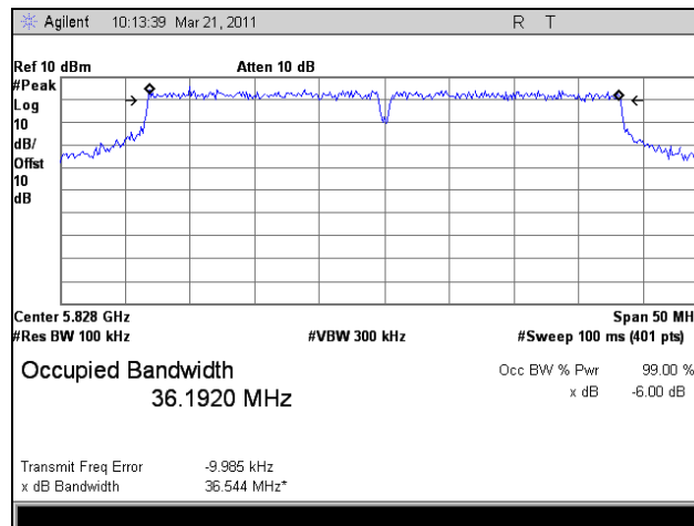
Plot 12. 6 dB Occupied Bandwidth, 802.11a 40 MHz, High Channel
