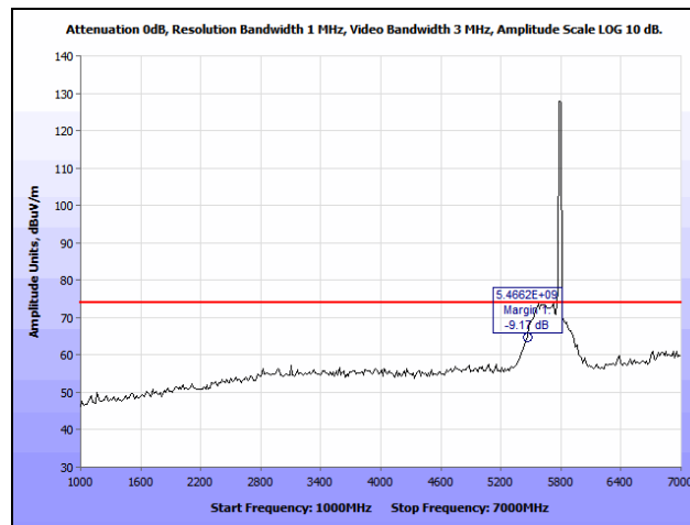
Plot 148. Radiated Spurious Emissions, HT8, Mid Channel, 1 GHz – 7 GHz, Peak
