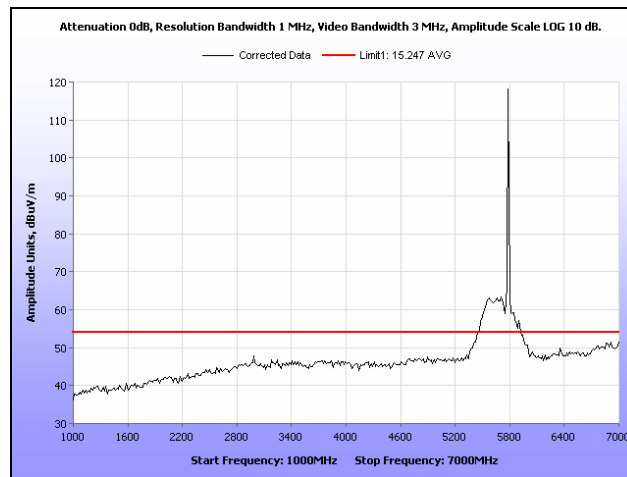
Plot 164. Radiated Spurious Emissions, HT10, Mid Channel, 1 GHz – 7 GHz, Average
