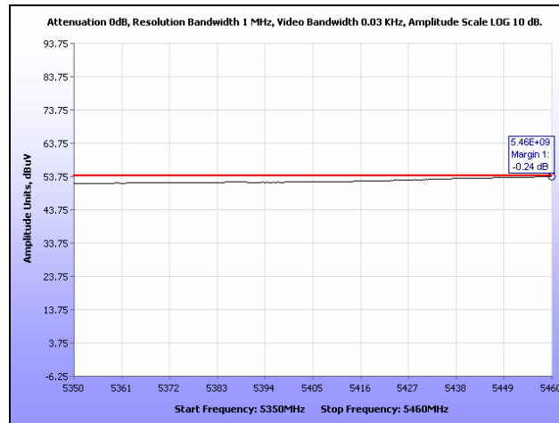
Plot 236. Restricted Band, HT5, Mid Channel
