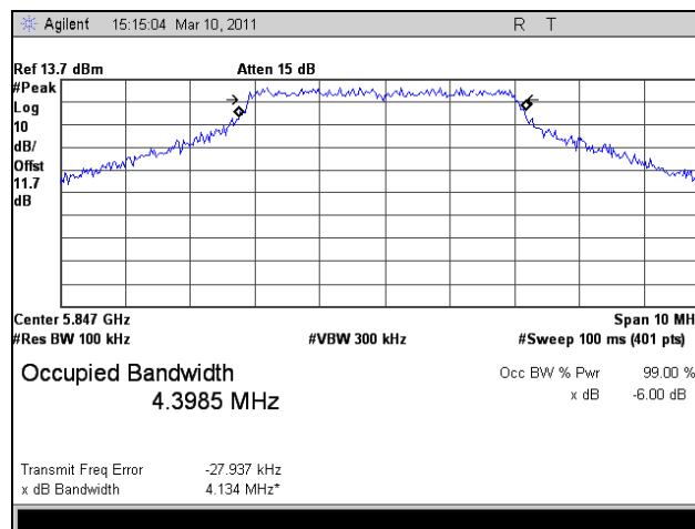
Plot 18. 6 dB Occupied Bandwidth, HT5, Port 2, High Channel
