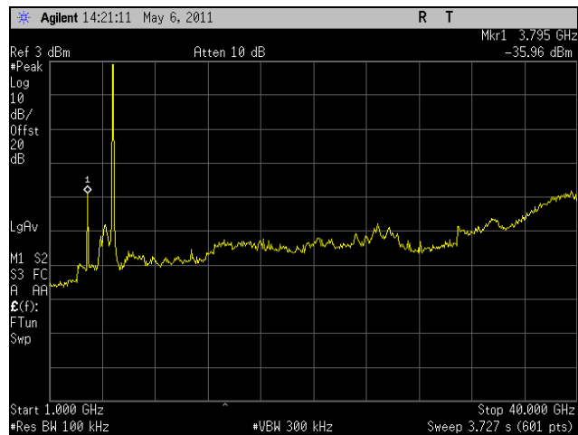
Plot 260. Conducted Spurious, Low Channel, 802.11a 40 MHz, 1 GHz - 40 GHz
