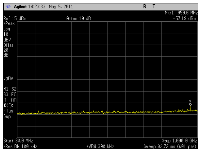
Plot 267. Conducted Spurious, Mid Channel, HT5, Port 1, 30 MHz - 1 GHz
