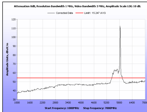
Plot 206. Radiated Spurious Emissions, HT30, High Channel, 1 GHz – 7 GHz, Average
