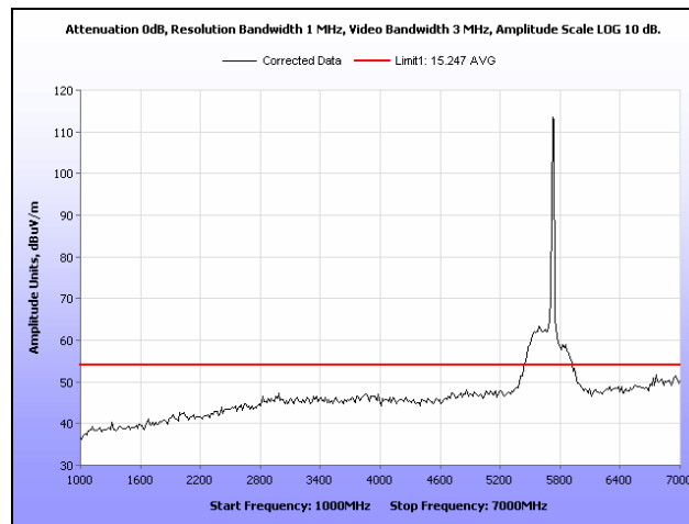
Plot 176. Radiated Spurious Emissions, HT20, Low Channel, 1 GHz – 7 GHz, Average
