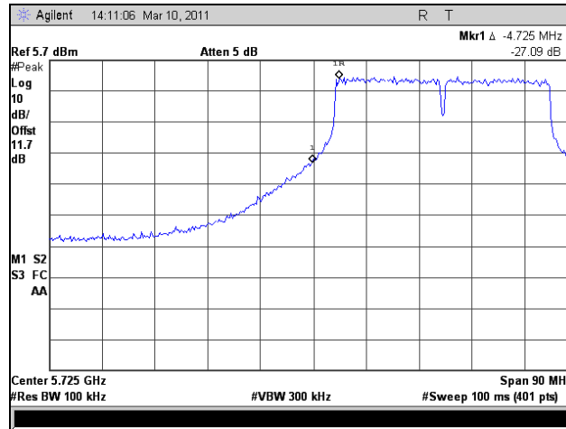
Plot 363. Conducted Band Edge, HT40, Low Channel, Port 2
