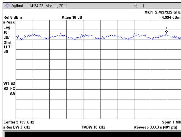
Plot 387. Peak Power Spectral Density, HT10, Port 2, Mid Channel
