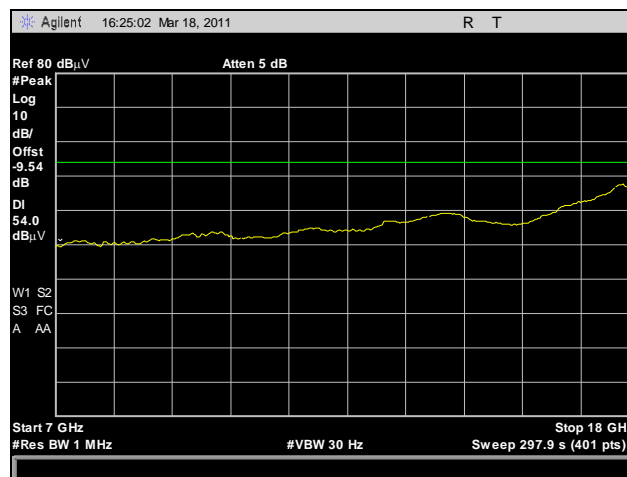
Plot 227. Radiated Spurious Emissions, HT40, High Channel, 7 GHz – 18 GHz, Average
