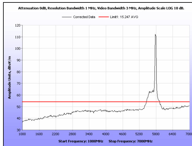
Plot 112. Radiated Spurious Emissions, Mid Channel, 802.11a 40MHz, 1 GHz – 7 GHz, Average
