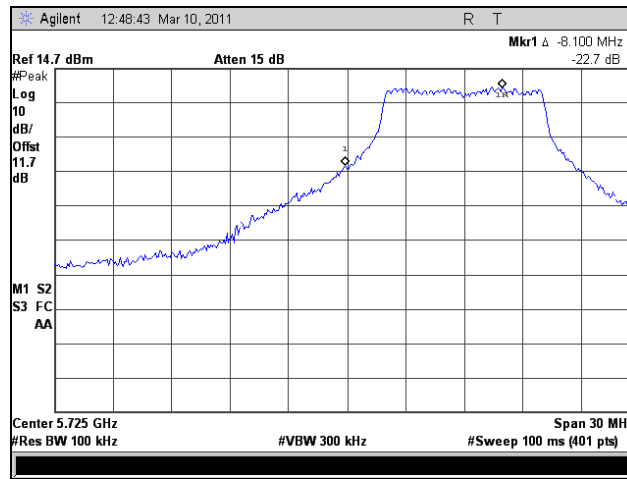
Plot 349. Conducted Band Edge, HT10, Low Channel, Port 1
