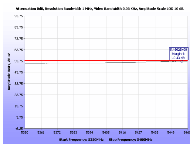
Plot 103. Restricted Band, 802.11a 20 MHz, High Channel
