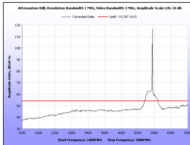
Plot 158. Radiated Spurious Emissions, HT10, Low Channel, 1 GHz – 7 GHz, Average
