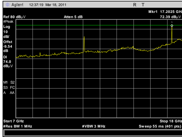
Plot 126. Radiated Spurious Emissions, HT5, Low Channel, 7 GHz – 18 GHz, Peak
