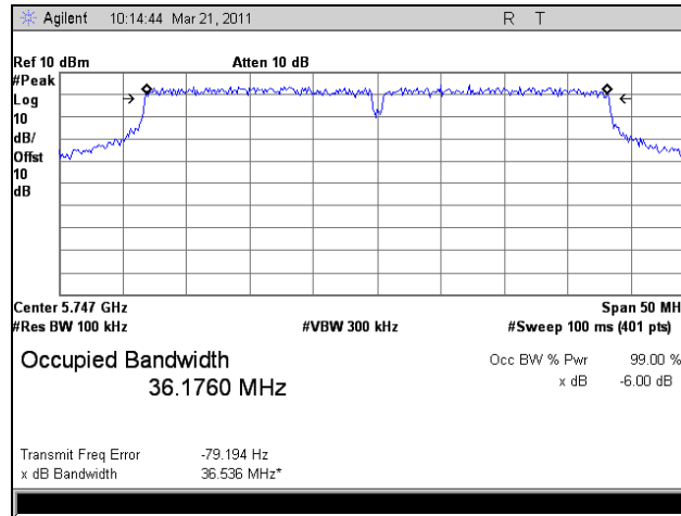
Plot 10. 6 dB Occupied Bandwidth, 802.11a 40 MHz, Low Channel
