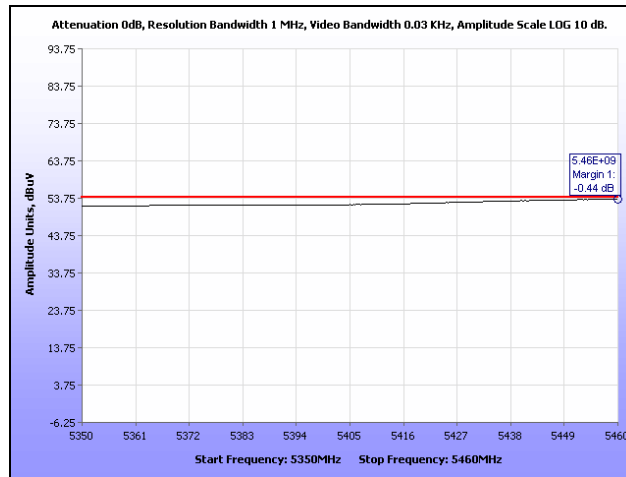
Plot 230. Restricted Band, 802.11a 20 MHz, Mid Channel
