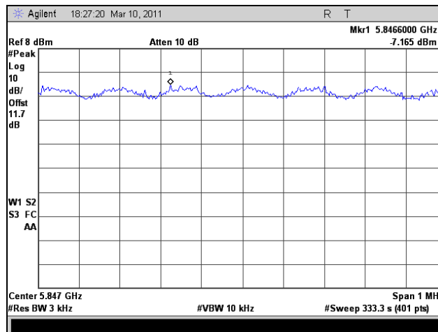
Plot 385. Peak Power Spectral Density, HT10, Port 1, High Channel
