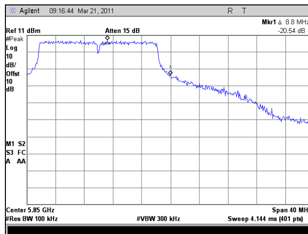
Plot 338. Conducted Band Edge, 802.11a 20 MHz, High Channel
