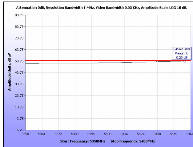
Plot 250. Restricted Band, HT40, Low Channel
