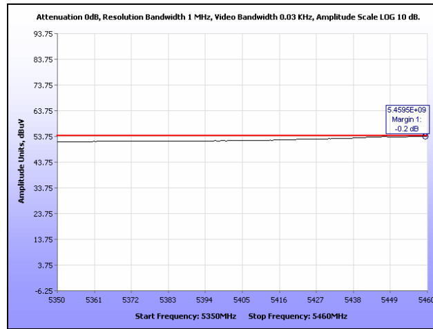
Plot 153. Restricted Band, HT8, High Channel
