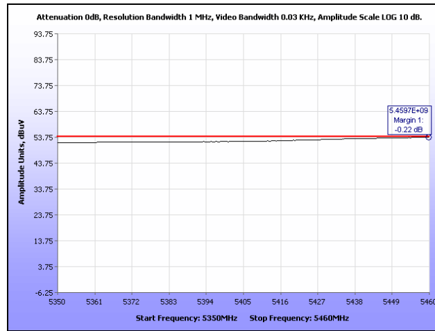
Plot 244. Restricted Band, HT20, Low Channel
