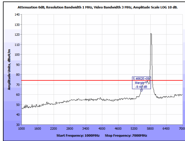
Plot 119. Radiated Spurious Emissions, High Channel, 802.11a 40MHz, 1 GHz – 7 GHz, Peak
