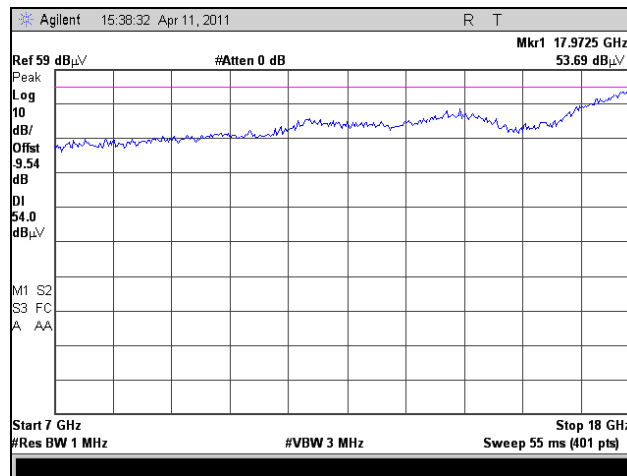
Plot 105. Radiated Spurious Emissions, High Channel, 802.11a 20 MHz, 7 GHz – 18 GHz
