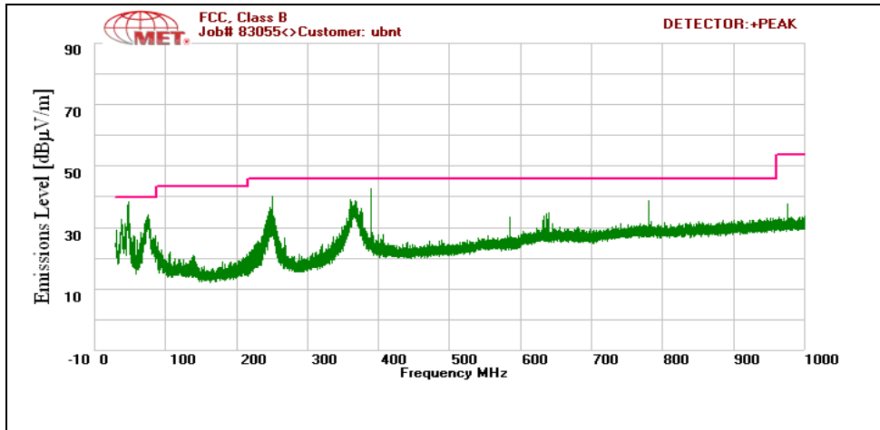
Plot 91. Radiated Spurious Emissions, 802.11a 20 MHz, Low Channel, 30 MHz – 1 GHz
