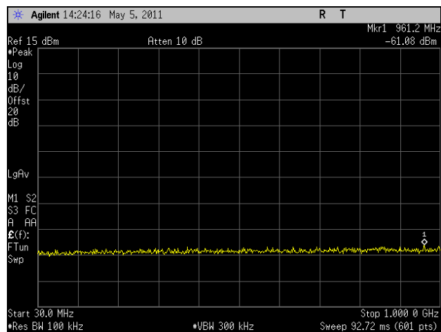
Plot 273. Conducted Spurious, Mid Channel, HT5, Port 2, 30 MHz - 1 GHz
