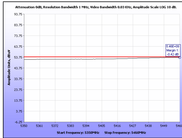
Plot 165. Restricted Band, HT10, Mid Channel
