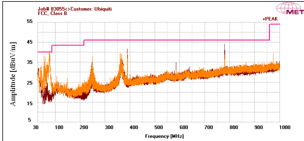
Plot 169. Radiated Spurious Emissions, HT10, High Channel, 30 MHz – 1 GHz
