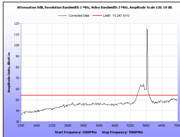
Plot 188. Radiated Spurious Emissions, HT20, High Channel, 1 GHz – 7 GHz, Average
