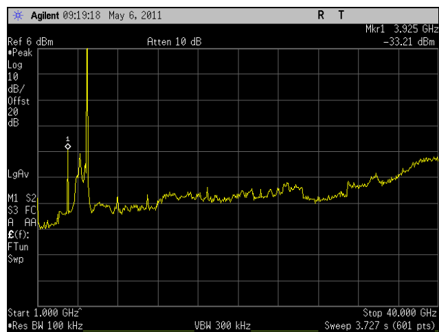
Plot 306. Conducted Spurious, High Channel, HT20, Port 1, 1 GHz - 40 GHz
