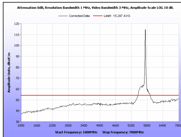
Plot 194. Radiated Spurious Emissions, HT30, Low Channel, 1 GHz – 7 GHz, Average
