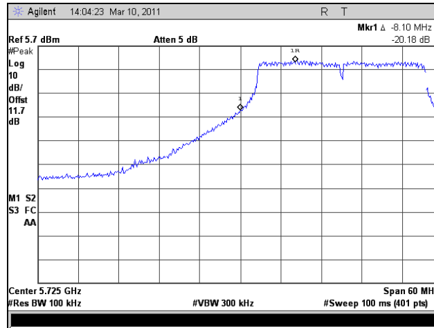
Plot 357. Conducted Band Edge, HT30, Low Channel, Port 1
