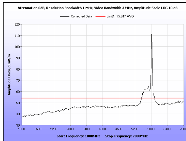
Plot 224. Radiated Spurious Emissions, HT40, High Channel, 1 GHz – 7 GHz, Average
