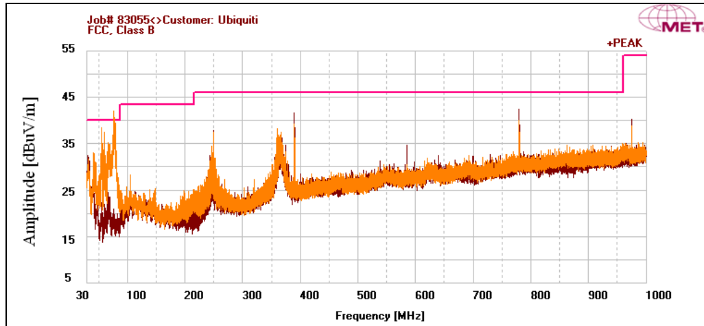
Plot 217. Radiated Spurious Emissions, HT40, Mid Channel, 30 MHz – 1 GHz
