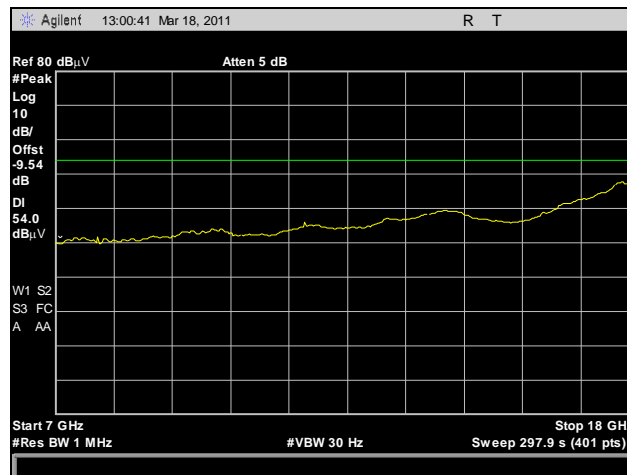
Plot 137. Radiated Spurious Emissions, HT5, High Channel, 7 GHz – 18 GHz, Average
