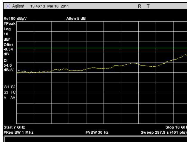
Plot 167. Radiated Spurious Emissions, HT10, Mid Channel, 7 GHz – 18 GHz, Average
