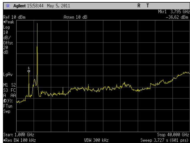
Plot 302. Conducted Spurious, Low Channel, HT20, Port 1, 1 GHz - 40 GHz
