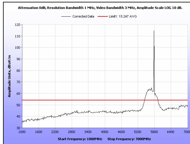
Plot 128. Radiated Spurious Emissions, HT5, Mid Channel, 1 GHz – 7 GHz, Average
