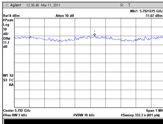
Plot 399. Peak Power Spectral Density, HT30, Port 2, Mid Channel
