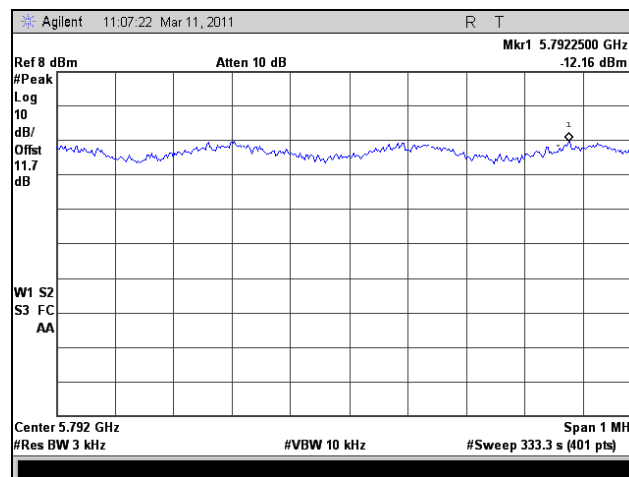
Plot 402. Peak Power Spectral Density, HT40, Port 1, Mid Channel
