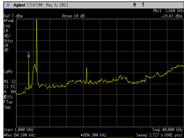
Plot 322. Conducted Spurious, Mid Channel, HT30, Port 2, 1 GHz - 40 GHz
