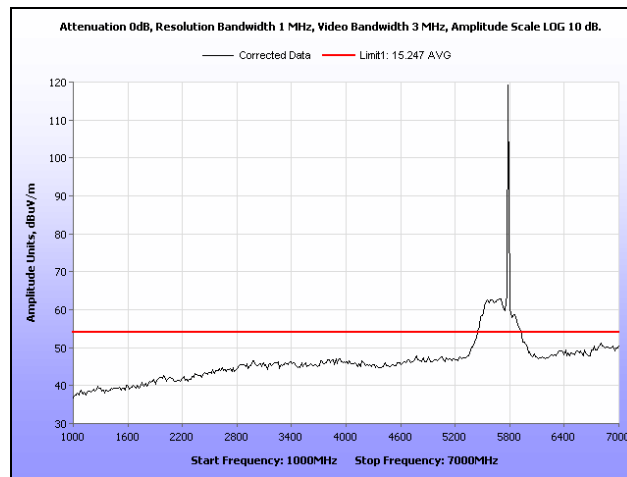
Plot 146. Radiated Spurious Emissions, HT8, Mid Channel, 1 GHz – 7 GHz, Average
