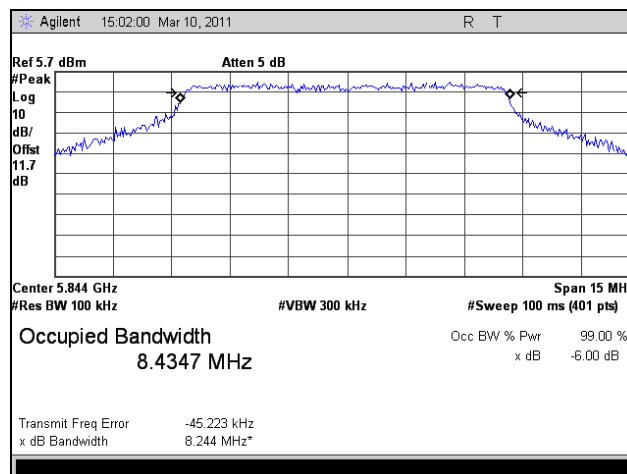
Plot 27. 6 dB Occupied Bandwidth, HT10, Port 1, High Channel
