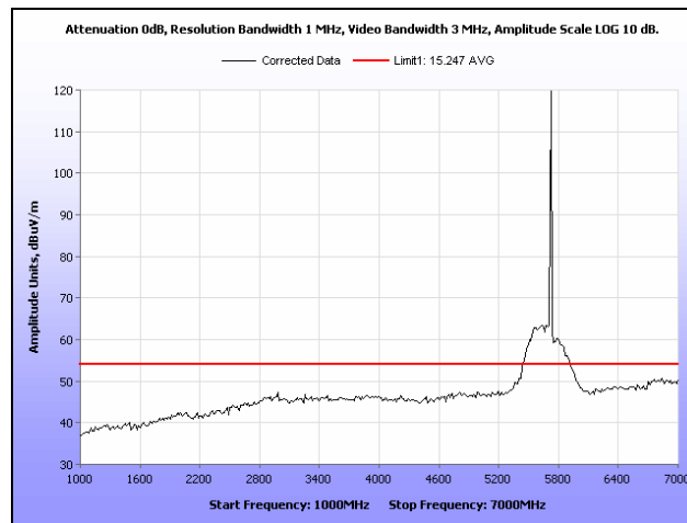
Plot 140. Radiated Spurious Emissions, HT8, Low Channel, 1 GHz – 7 GHz, Average
