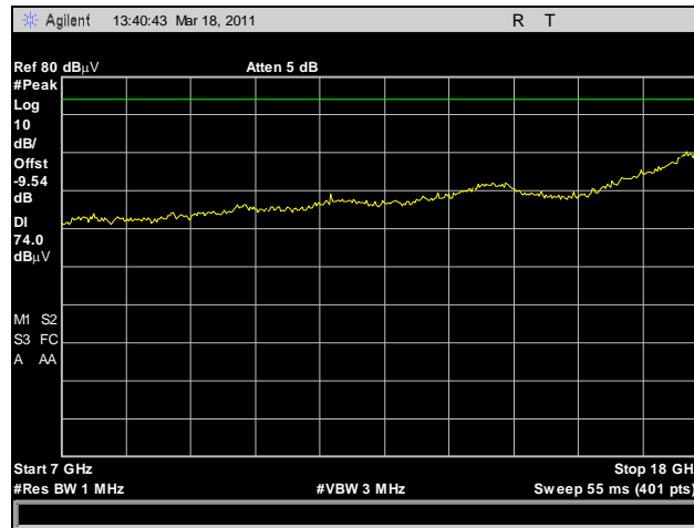
Plot 168. Radiated Spurious Emissions, HT10, Mid Channel, 7 GHz – 18 GHz, Peak
