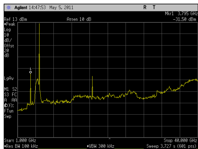
Plot 288. Conducted Spurious, High Channel, HT8, Port 2, 1 GHz - 40 GHz
