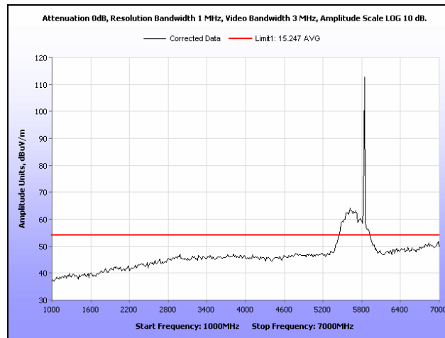
Plot 152. Radiated Spurious Emissions, HT8, High Channel, 1 GHz – 7 GHz, Average
