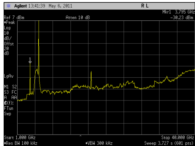
Plot 320. Conducted Spurious, Low Channel, HT30, Port 2, 1 GHz - 40 GHz
