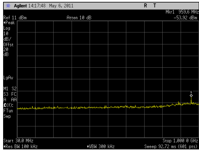
Plot 259. Conducted Spurious, Low Channel, 802.11a 40 MHz, 30 MHz - 1 GHz
