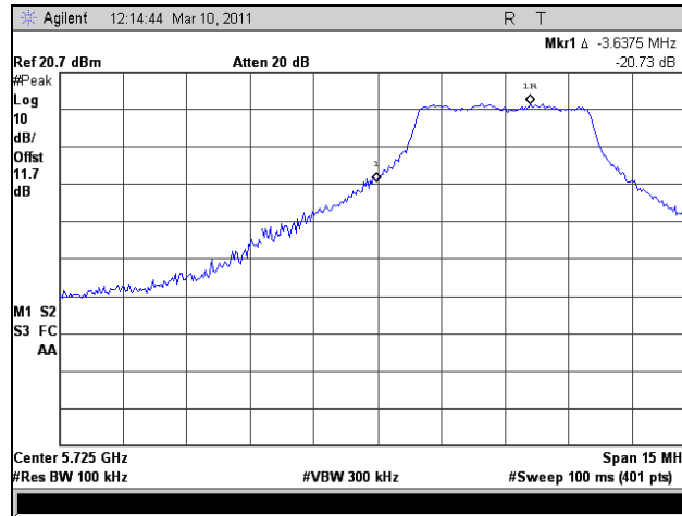
Plot 341. Conducted Band Edge, HT5, Low Channel, Port 1
