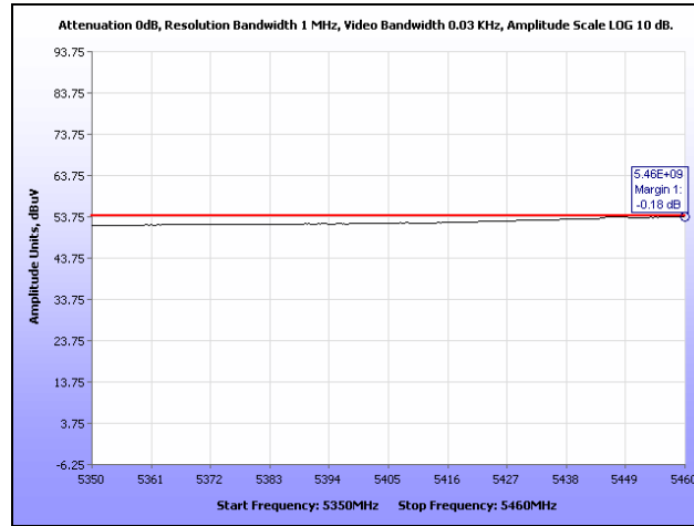
Plot 135. Restricted Band, HT5, High Channel
