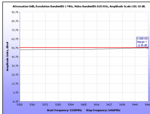
Plot 245. Restricted Band, HT20, Mid Channel
