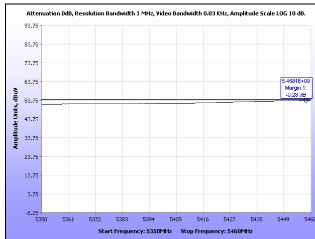
Plot 251. Restricted Band, HT40, Mid Channel
