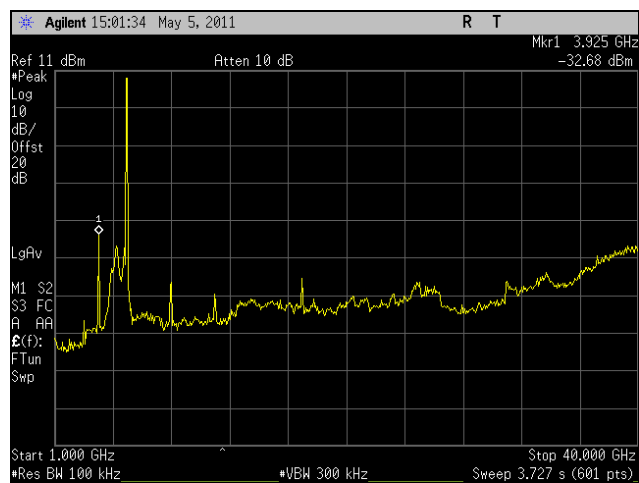
Plot 294. Conducted Spurious, High Channel, HT10, Port 1, 1 GHz - 40 GHz
