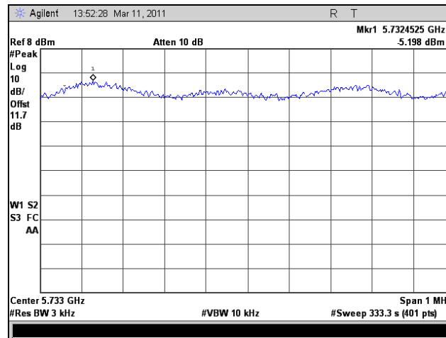
Plot 392. Peak Power Spectral Density, HT20, Port 2, Low Channel
