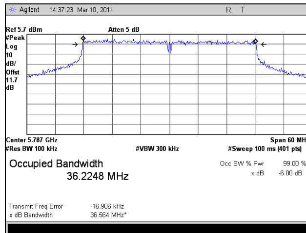
Plot 44. 6 dB Occupied Bandwidth, HT40, Port 1, Mid Channel
