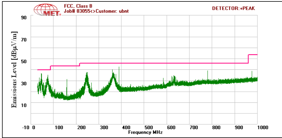
Plot 116. Radiated Spurious Emissions, 802.11a 40 MHz, High Channel, 30 MHz – 1 GHz
