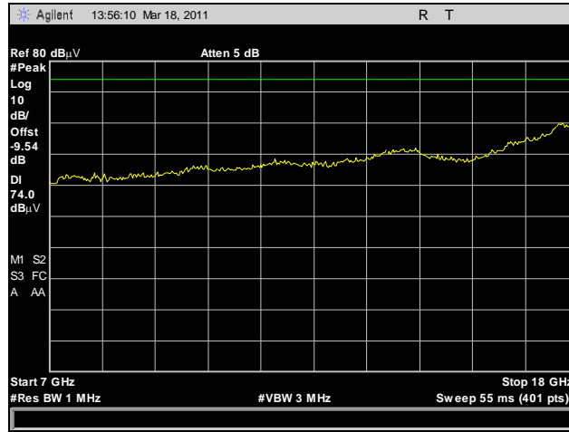
Plot 192. Radiated Spurious Emissions, HT20, High Channel, 7 GHz – 18 GHz, Peak
