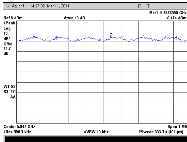
Plot 388. Peak Power Spectral Density, HT10, Port 2, High Channel
