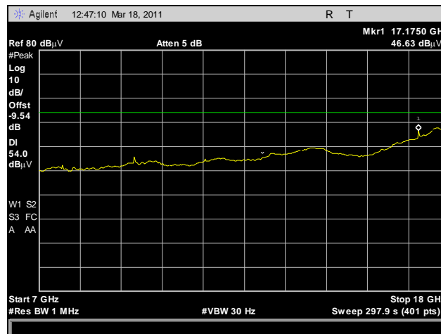
Plot 125. Radiated Spurious Emissions, HT5, Low Channel, 7 GHz – 18 GHz, Average
