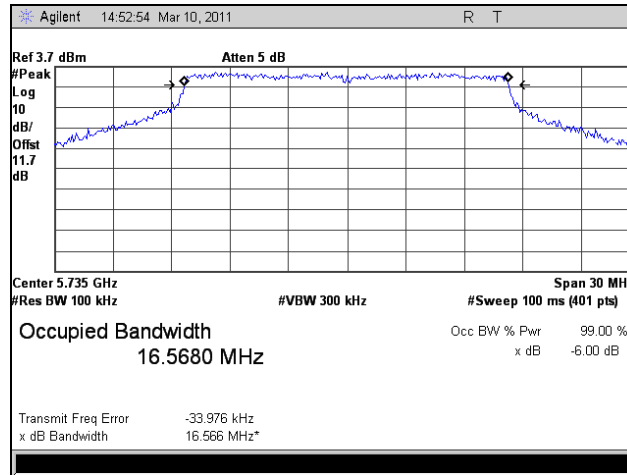
Plot 31. 6 dB Occupied Bandwidth, HT20, Port 1, Low Channel
