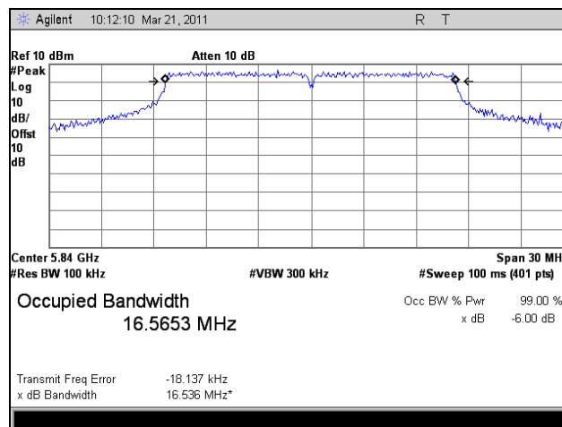
Plot 9. 6 dB Occupied Bandwidth, 802.11a 20 MHz, High Channel
