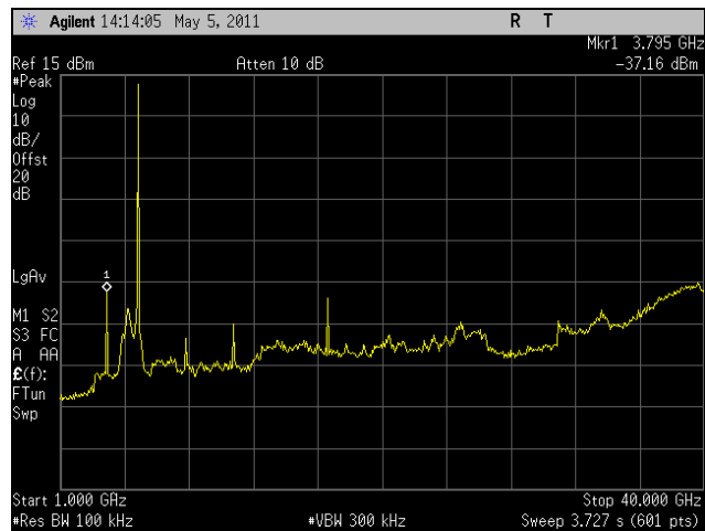
Plot 266. Conducted Spurious, Low Channel, HT5, Port 1, 1 GHz – 40 GHz
