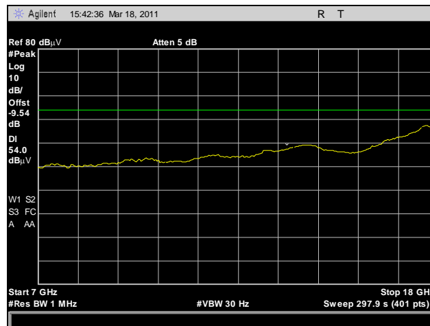
Plot 185. Radiated Spurious Emissions, HT20, Mid Channel, 7 GHz – 18 GHz, Average
