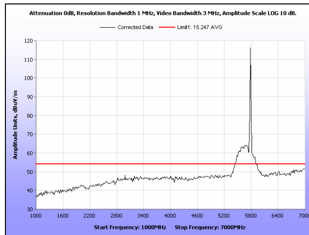
Plot 97. Radiated Spurious Emissions, Mid Channel, 802.11a 20MHz, 1 GHz – 7 GHz, Average
