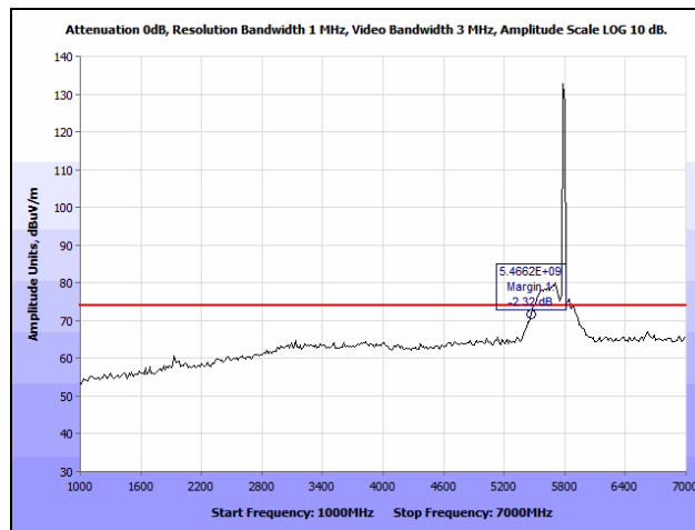
Plot 130. Radiated Spurious Emissions, HT5, Mid Channel, 1 GHz – 7 GHz, Peak
