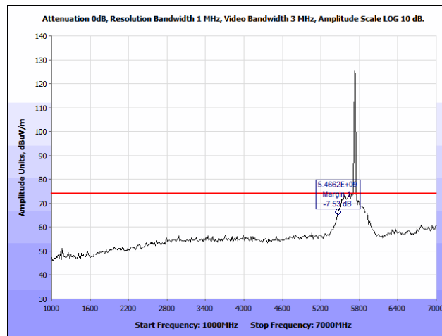
Plot 160. Radiated Spurious Emissions, HT10, Low Channel, 1 GHz – 7 GHz, Peak
