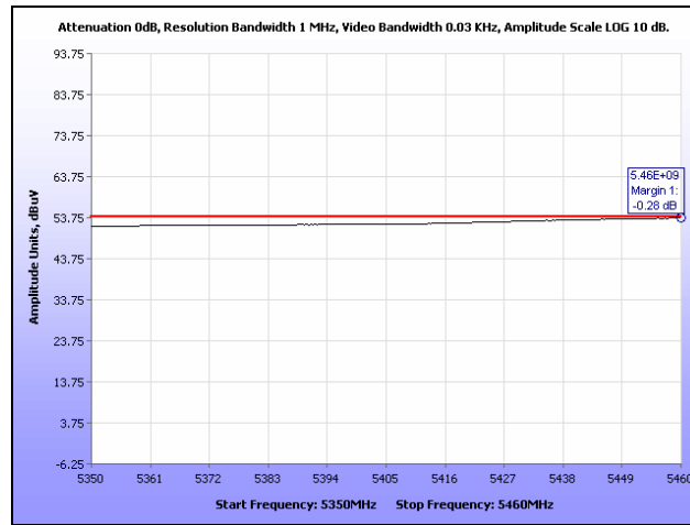
Plot 201. Restricted Band, HT30, Mid Channel
