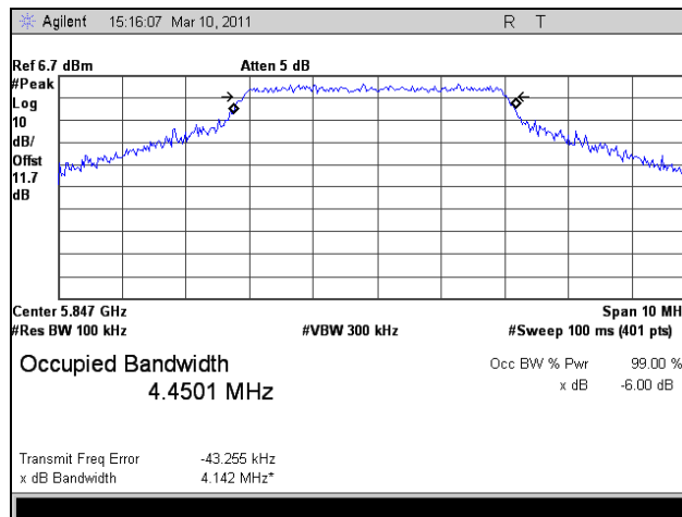
Plot 15. 6 dB Occupied Bandwidth, HT5, Port 1, High Channel
