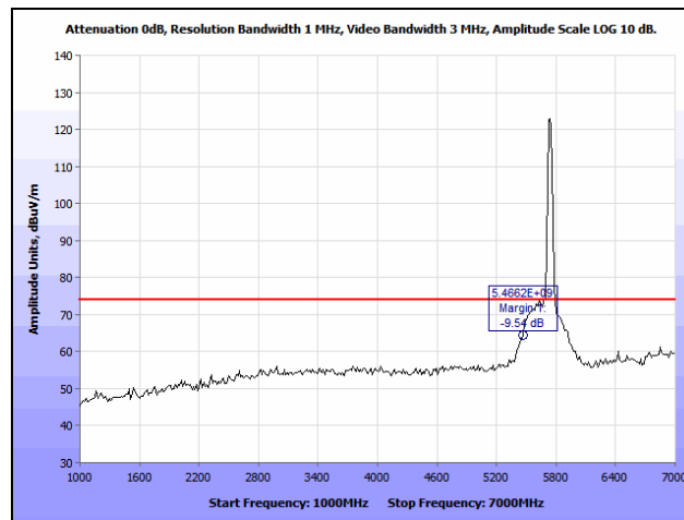
Plot 196. Radiated Spurious Emissions, HT30, Low Channel, 1 GHz – 7 GHz, Peak
