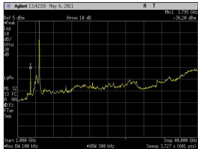
Plot 314. Conducted Spurious, Low Channel, HT30, Port 1, 1 GHz - 40 GHz
