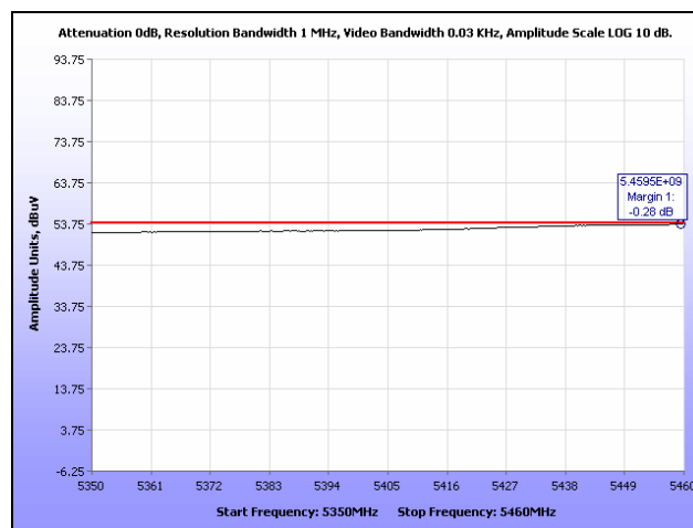
Plot 249. Restricted Band, HT30, High Channel
