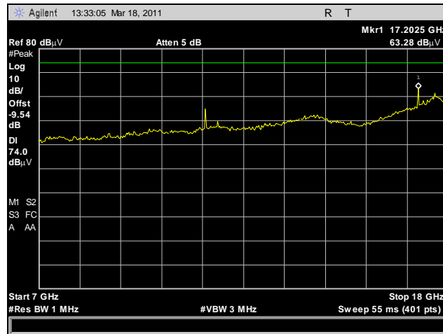
Plot 162. Radiated Spurious Emissions, HT10, Low Channel, 7 GHz – 18 GHz, Peak
