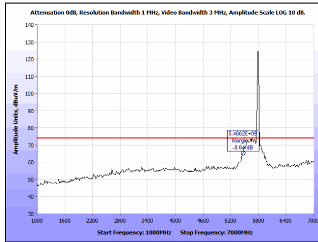
Plot 99. Radiated Spurious Emissions, Mid Channel, 802.11a 20MHz, 1 GHz – 7 GHz, Peak
