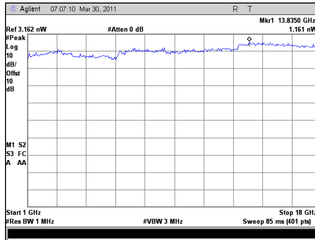
Plot 410. Receiver Spurious Emission, 1 GHz – 18 GHz, Port 2
