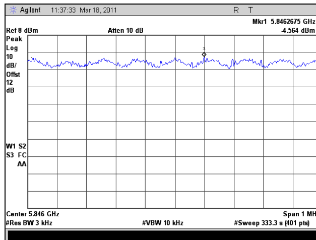
Plot 382. Peak Power Spectral Density, HT8, Port 2, High Channel
