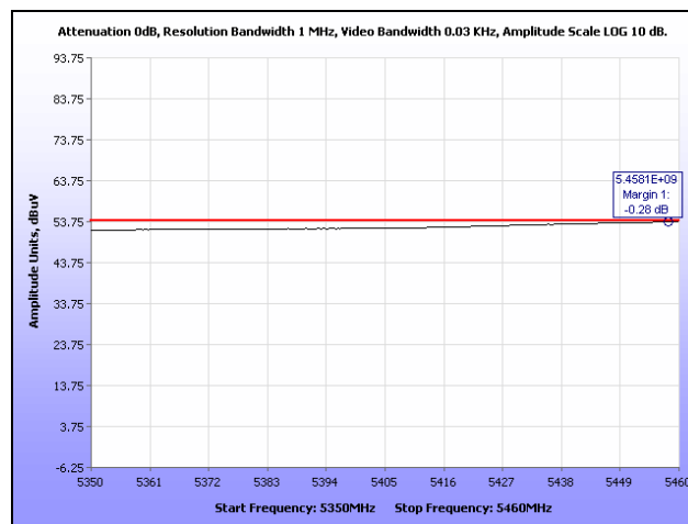
Plot 113. Restricted Band, 802.11a 40 MHz, Mid Channel
