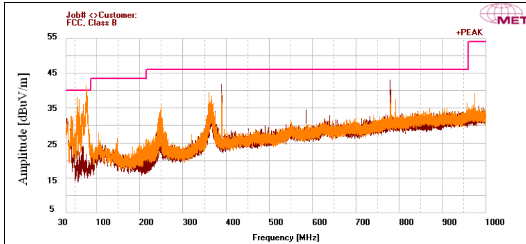
Plot 175. Radiated Spurious Emissions, HT20, Low Channel, 30 MHz – 1 GHz
