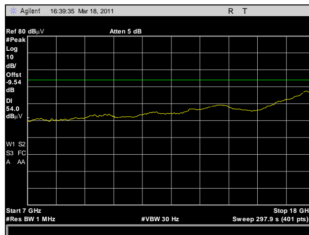
Plot 215. Radiated Spurious Emissions, HT40, Low Channel, 7 GHz – 18 GHz, Average
