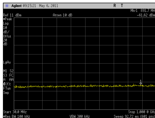
Plot 309. Conducted Spurious, Mid Channel, HT20, Port 2, 30 MHz - 1 GHz
