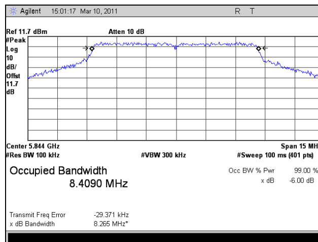
Plot 30. 6 dB Occupied Bandwidth, HT10, Port 2, High Channel
