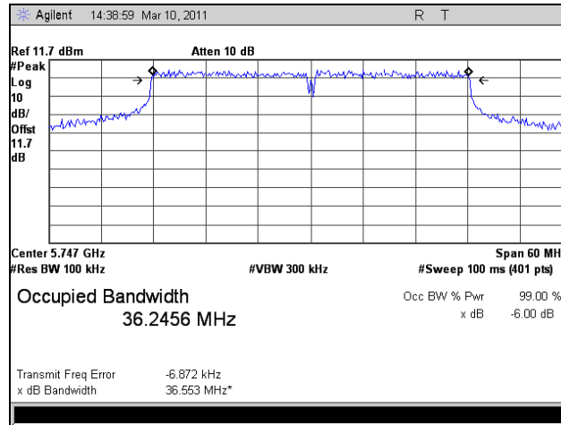
Plot 46. 6 dB Occupied Bandwidth, HT40, Port 2, Low Channel
