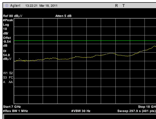
Plot 155. Radiated Spurious Emissions, HT8, High Channel, 7 GHz – 18 GHz, Average
