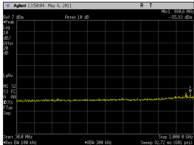
Plot 317. Conducted Spurious, High Channel, HT30, Port 1, 30 MHz - 1 GHz
