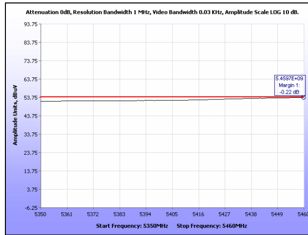
Plot 225. Restricted Band, HT40, High Channel
