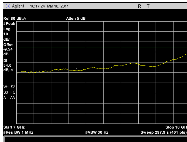
Plot 209. Radiated Spurious Emissions, HT30, High Channel, 7 GHz – 18 GHz, Peak
