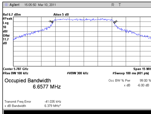
Plot 20. 6 dB Occupied Bandwidth, HT8, Port 1, Mid Channel
