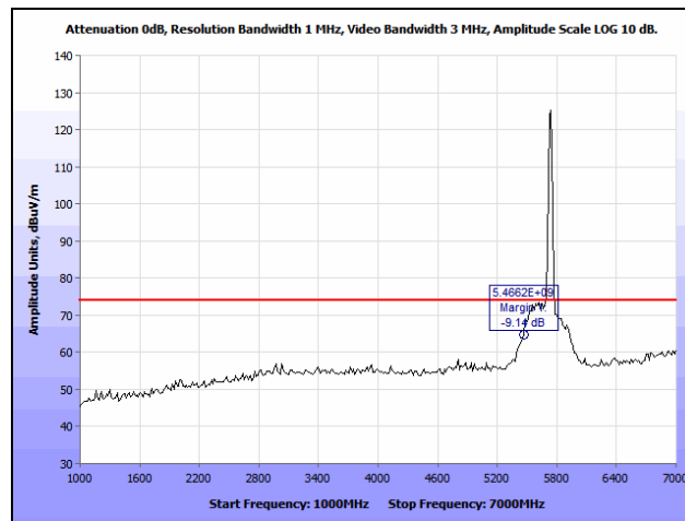
Plot 178. Radiated Spurious Emissions, HT20, Low Channel, 1 GHz – 7 GHz, Peak
