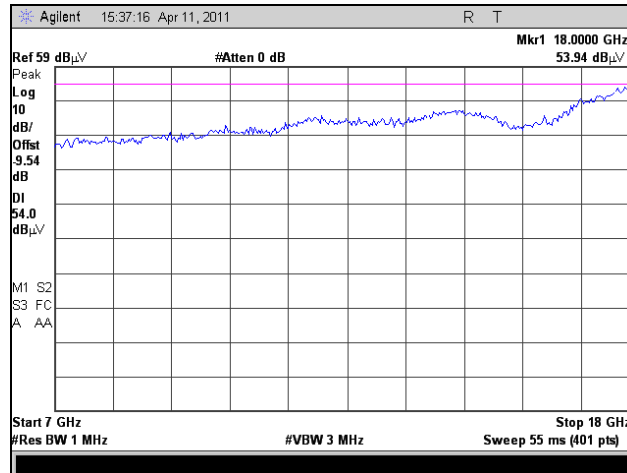
Plot 95 Radiated Spurious Emissions, Low Channel, 802.11a 20 MHz, 7 GHz – 18 GHz
