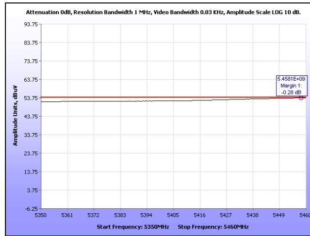
Plot 219. Restricted Band, HT40, Mid Channel
