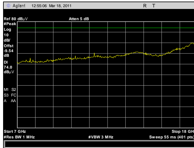
Plot 138. Radiated Spurious Emissions, HT5, High Channel, 7 GHz – 18 GHz, Peak
