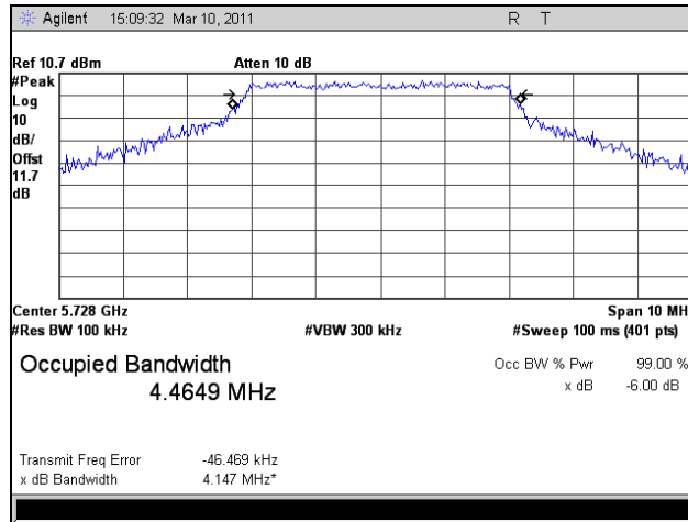
Plot 13. 6 dB Occupied Bandwidth, HT5, Port 1, Low Channel
