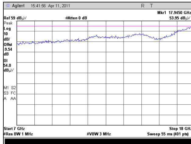
Plot 110. Radiated Spurious Emissions, Low Channel, 802.11a 40 MHz, 7 GHz – 18 GHz
