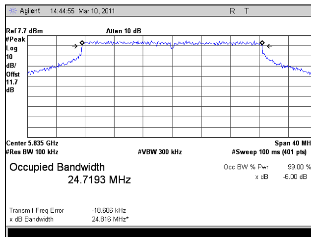
Plot 42. 6 dB Occupied Bandwidth, HT30, Port 2, High Channel
