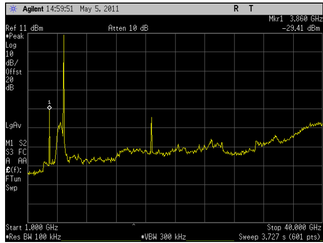
Plot 298. Conducted Spurious, Mid Channel, HT10, Port 2, 1 GHz - 40 GHz
