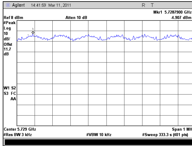
Plot 386. Peak Power Spectral Density, HT10, Port 2, Low Channel
