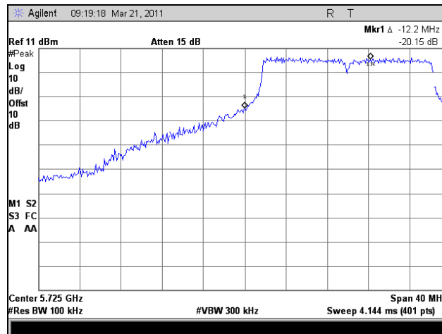
Plot 337. Conducted Band Edge, 802.11a 20 MHz, Low Channel
