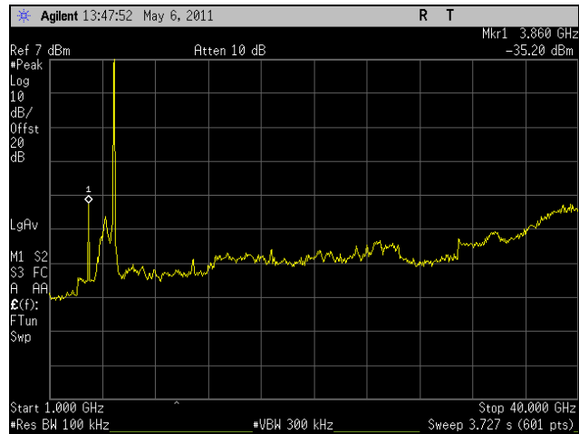
Plot 316. Conducted Spurious, Mid Channel, HT30, Port 1, 1 GHz - 40 GHz
