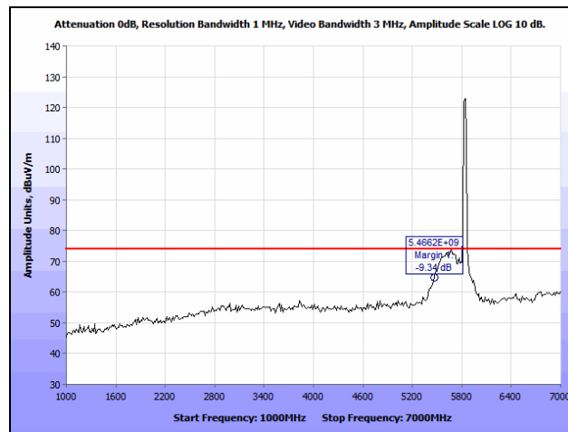
Plot 190. Radiated Spurious Emissions, HT20, High Channel, 1 GHz – 7 GHz, Peak
