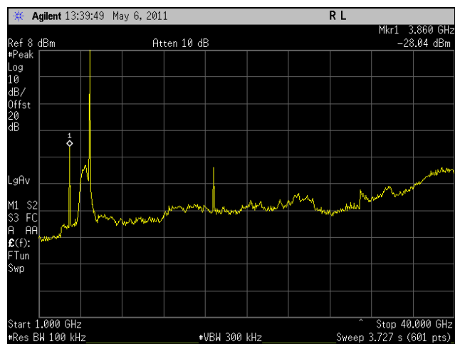
Plot 312. Conducted Spurious, High Channel, HT20, Port 2, 1 GHz - 40 GHz
