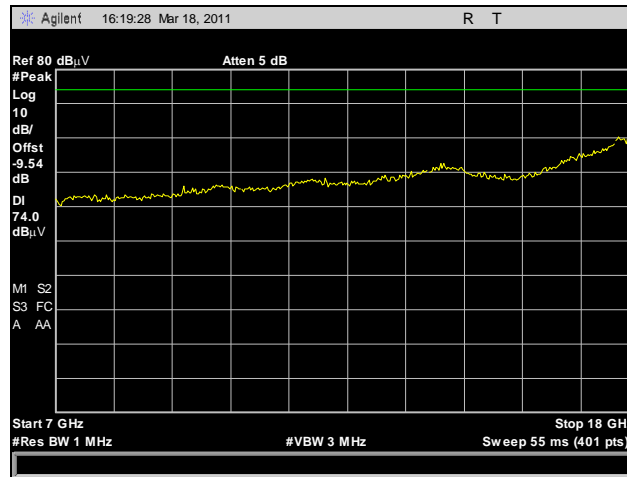
Plot 228. Radiated Spurious Emissions, HT40, High Channel, 7 GHz – 18 GHz, Peak
