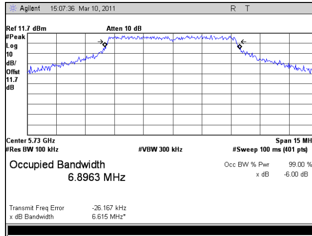
Plot 22. 6 dB Occupied Bandwidth, HT8, Port 2, Low Channel
