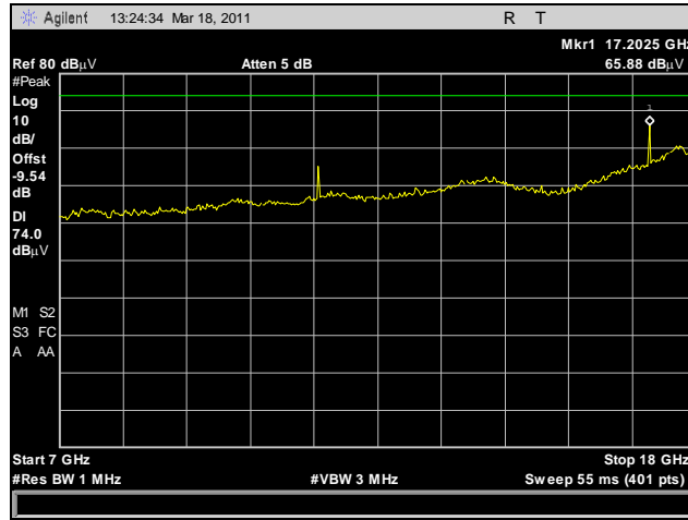
Plot 144. Radiated Spurious Emissions, HT8, Low Channel, 7 GHz – 18 GHz, Peak
