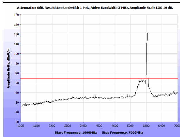
Plot 208. Radiated Spurious Emissions, HT30, High Channel, 1 GHz – 7 GHz, Peak
