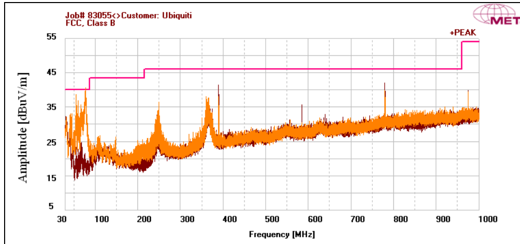
Plot 151. Radiated Spurious Emissions, HT8, High Channel, 30 MHz – 1 GHz
