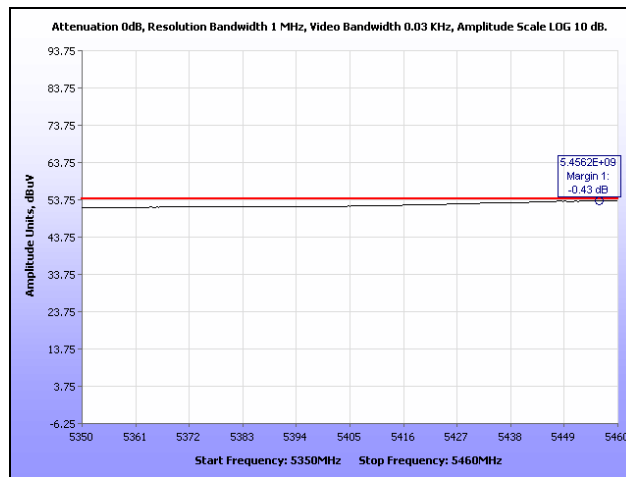
Plot 231. Restricted Band, 802.11a 20 MHz, High Channel
