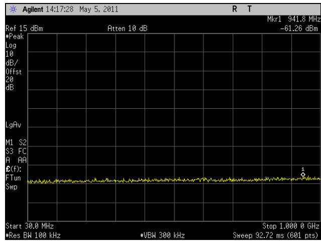
Plot 265. Conducted Spurious, Low Channel, HT5, Port 1, 30 MHz – 1 GHz
