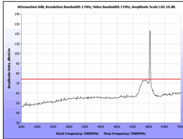
Plot 104. Radiated Spurious Emissions, High Channel, 802.11a 20MHz, 1 GHz – 7 GHz, Peak
