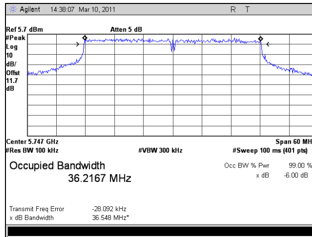
Plot 43. 6 dB Occupied Bandwidth, HT40, Port 1, Low Channel
