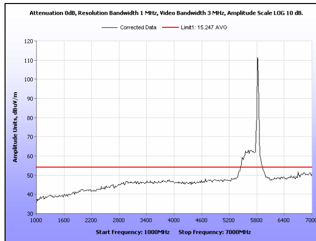
Plot 117. Radiated Spurious Emissions, High Channel, 802.11a 40MHz, 1 GHz – 7 GHz, Average
