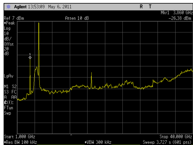
Plot 324. Conducted Spurious, High Channel, HT30, Port 2, 1 GHz - 40 GHz
