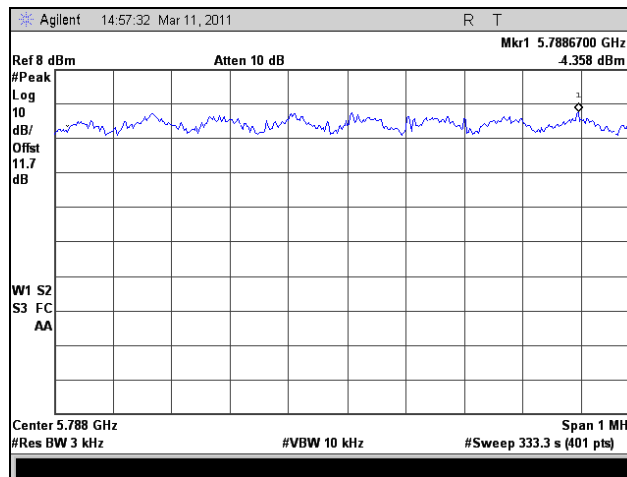
Plot 381. Peak Power Spectral Density, HT8, Port 2, Mid Channel
