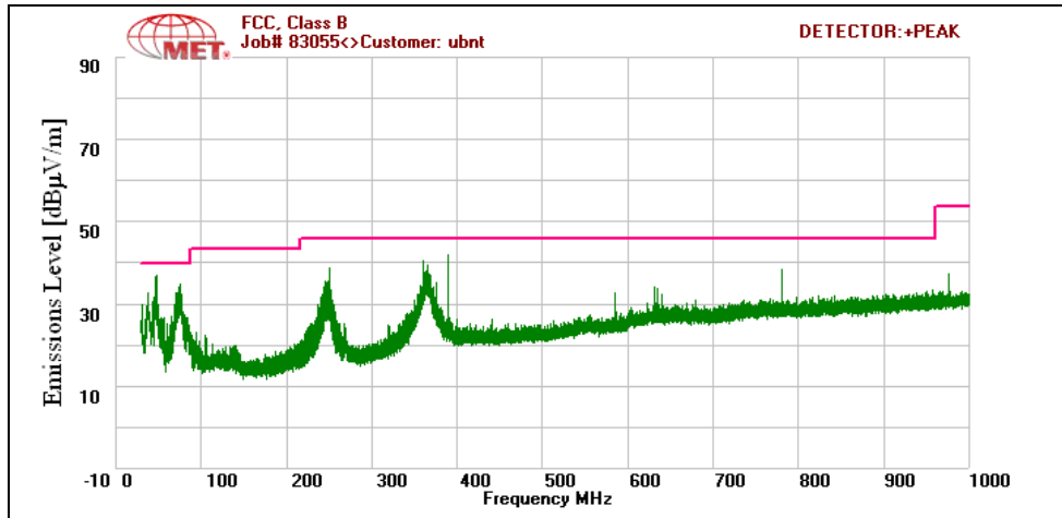
Plot 96. Radiated Spurious Emissions, 802.11a 20 MHz, Mid Channel, 30 MHz – 1 GHz
