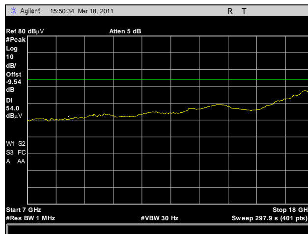
Plot 179. Radiated Spurious Emissions, HT20, Low Channel, 7 GHz – 18 GHz, Average
