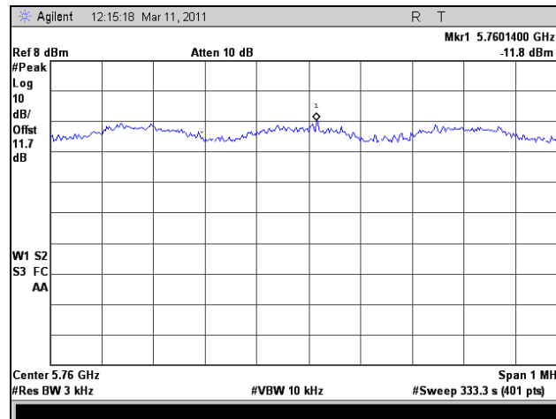
Plot 404. Peak Power Spectral Density, HT40 Port 2, Low Channel
