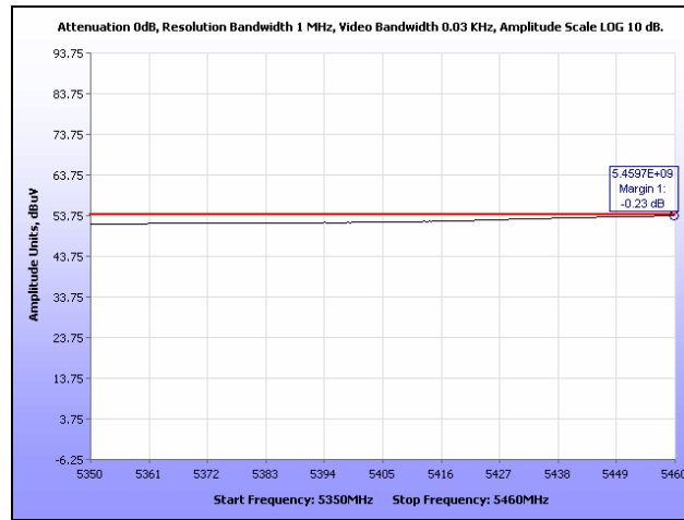
Plot 247. Restricted Band, HT30, Low Channel
