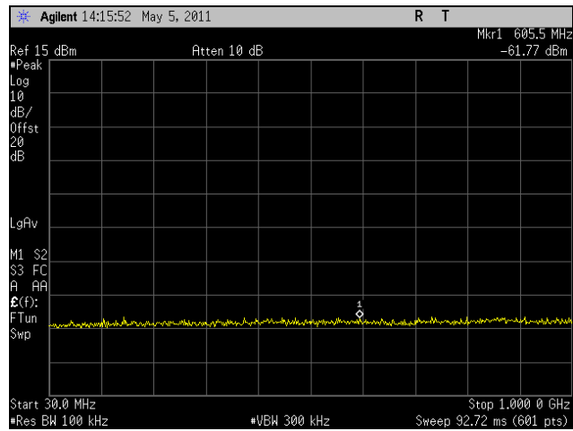
Plot 271. Conducted Spurious, Low Channel, HT5, Port 2, 30 MHz - 1 GHz
