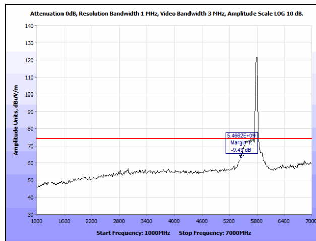
Plot 202. Radiated Spurious Emissions, HT30, Mid Channel, 1 GHz – 7 GHz, Peak
