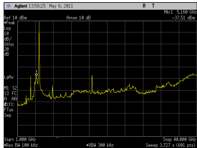
Plot 326. Conducted Spurious, Low Channel, HT40, Port 1, 1 GHz - 40 GHz
