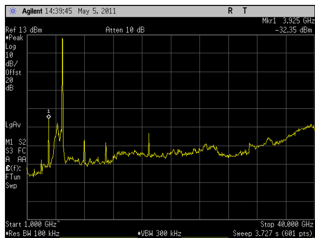
Plot 282. Conducted Spurious, High Channel, HT8, Port 1, 1 GHz - 40 GHz
