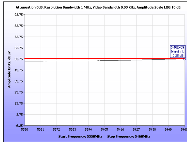
Plot 241. Restricted Band, HT10, Low Channel
