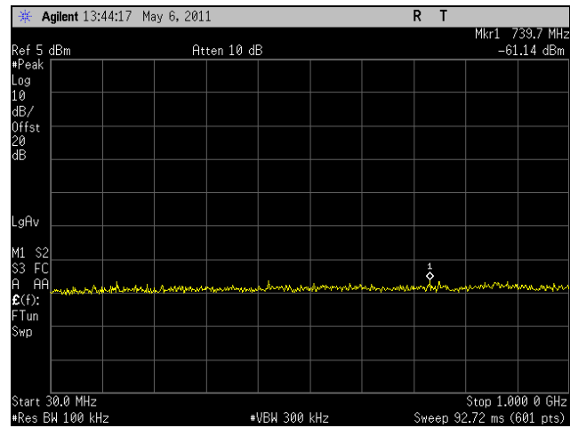
Plot 319. Conducted Spurious, Low Channel, HT30, Port 2, 30 MHz - 1 GHz
