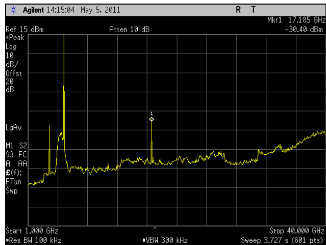
Plot 272. Conducted Spurious, Low Channel, HT5, Port 2, 1 GHz – 40 GHz
