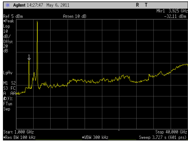
Plot 256. Conducted Spurious, Mid Channel, 802.11a 20 MHz, 1 GHz - 40 GHz
