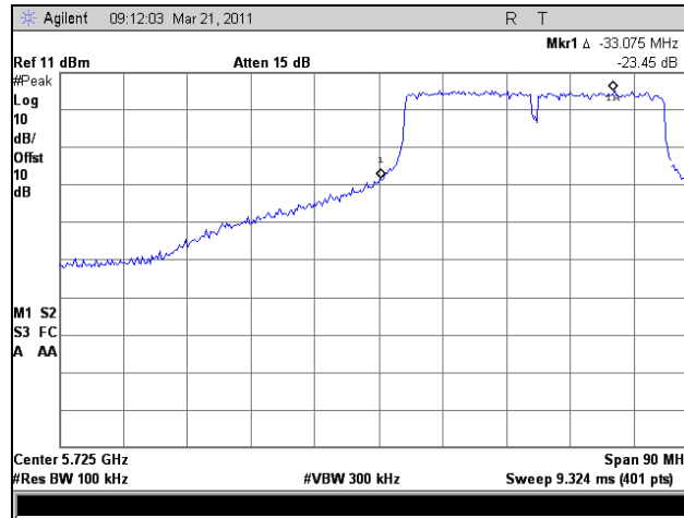
Plot 339. Conducted Band Edge, 802.11a 40 MHz, Low Channel
