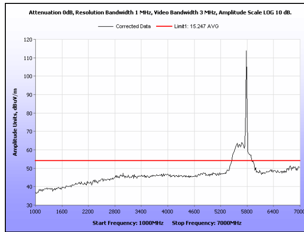
Plot 182. Radiated Spurious Emissions, HT20, Mid Channel, 1 GHz – 7 GHz, Average
