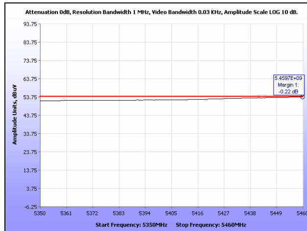
Plot 118. Restricted Band, 802.11a 40 MHz, High Channel
