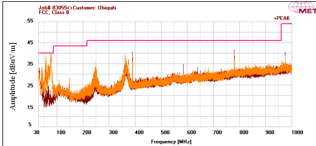
Plot 157. Radiated Spurious Emissions, HT10, Low Channel, 30 MHz – 1 GHz
