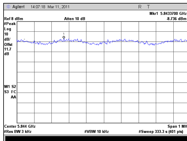
Plot 394. Peak Power Spectral Density, HT20, Port 2, High Channel
