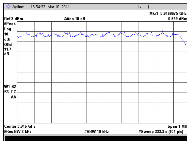
Plot 373. Peak Power Spectral Density, HT5, Port 1, High Channel
