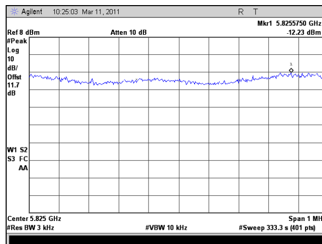
Plot 397. Peak Power Spectral Density, HT30, Port 1, High Channel
