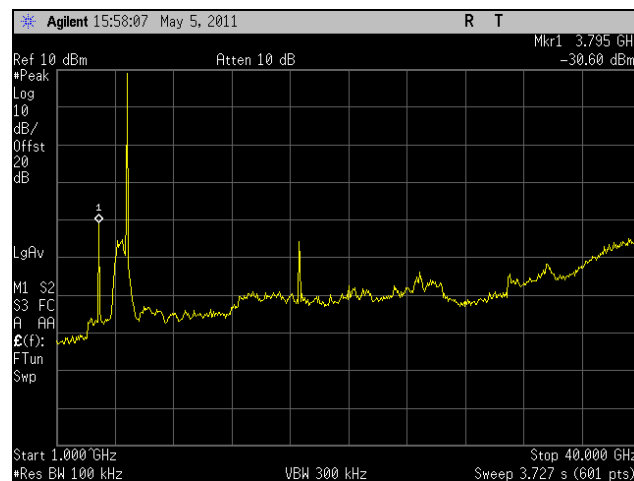
Plot 308. Conducted Spurious, Low Channel, HT20, Port 2, 1 GHz - 40 GHz
