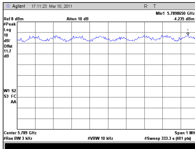
Plot 378. Peak Power Spectral Density, HT8, Port 1, Mid Channel
