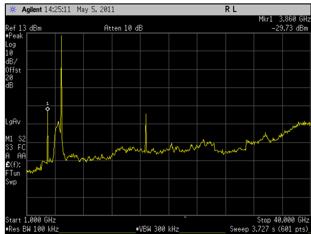
Plot 274. Conducted Spurious, Mid Channel, HT5, Port 2, 1 GHz - 40 GHz
