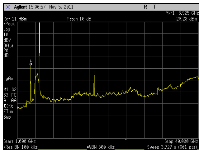
Plot 300. Conducted Spurious, High Channel, HT10, Port 2, 1 GHz - 40 GHz
