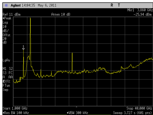
Plot 336. Conducted Spurious, High Channel, HT40, Port 2, 1 GHz - 40 GHz
