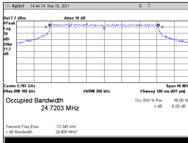
Plot 41. 6 dB Occupied Bandwidth, HT30, Port 2, Mid Channel
