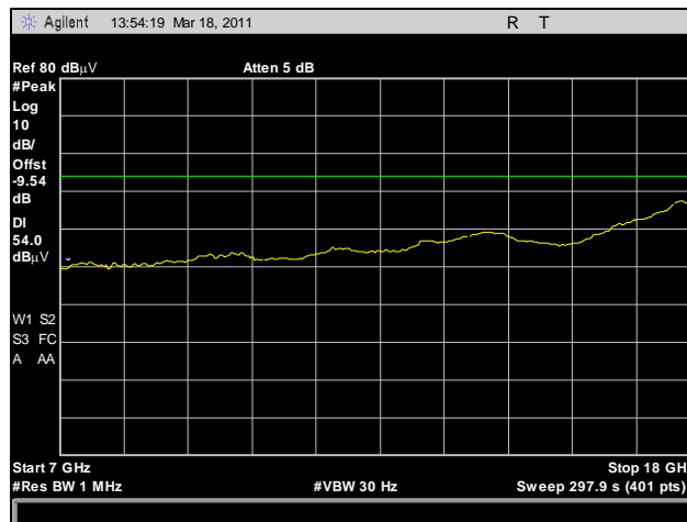
Plot 173. Radiated Spurious Emissions, HT10, High Channel, 7 GHz – 18 GHz, Average
