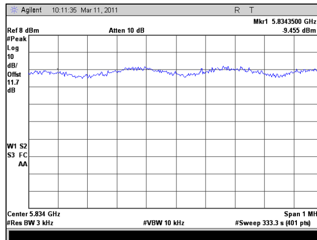
Plot 391. Peak Power Spectral Density, HT20, Port 1, High Channel
