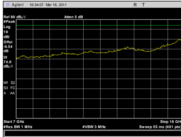
Plot 216. Radiated Spurious Emissions, HT40, Low Channel, 7 GHz – 18 GHz, Peak
