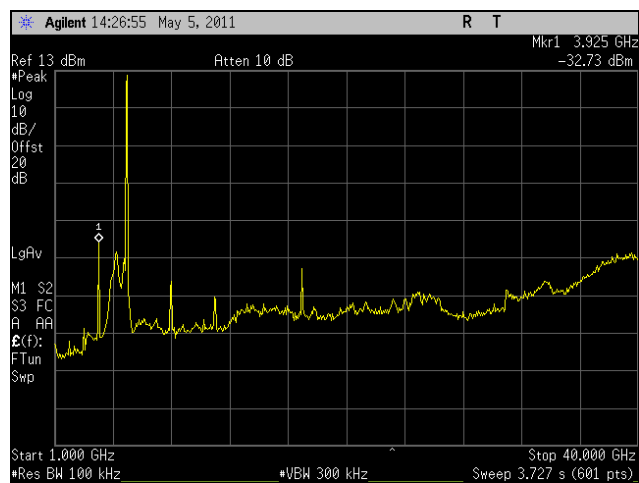
Plot 270. Conducted Spurious, High Channel, HT5, Port 1, 1 GHz - 40 GHz
