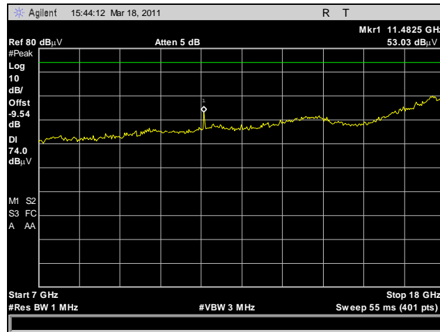
Plot 180. Radiated Spurious Emissions, HT20, Low Channel, 7 GHz – 18 GHz, Peak
