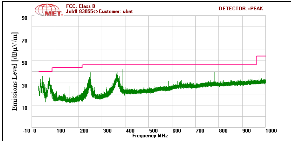
Plot 101. Radiated Spurious Emissions, 802.11a 20 MHz, High Channel, 30 MHz – 1 GHz
