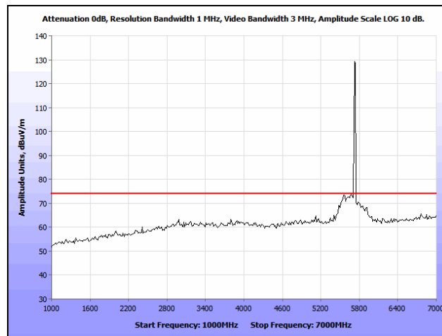
Plot 142. Radiated Spurious Emissions, HT8, Low Channel, 1 GHz – 7 GHz, Peak
