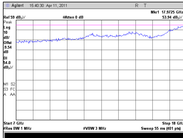
Plot 115. Radiated Spurious Emissions, Mid Channel, 802.11a 40 MHz, 7 GHz – 18 GHz
