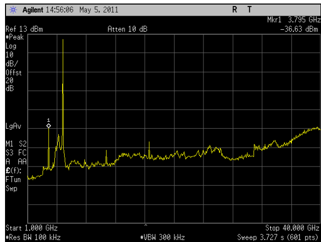
Plot 290. Conducted Spurious, Low Channel, HT10, Port 1, 1 GHz - 40 GHz
