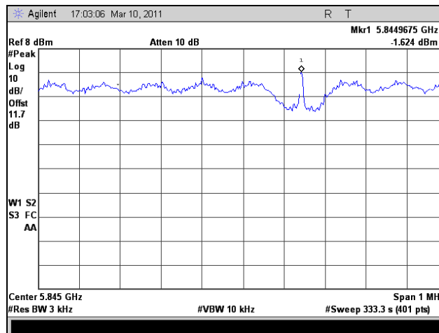
Plot 379. Peak Power Spectral Density, HT8, Port 1, High Channel
