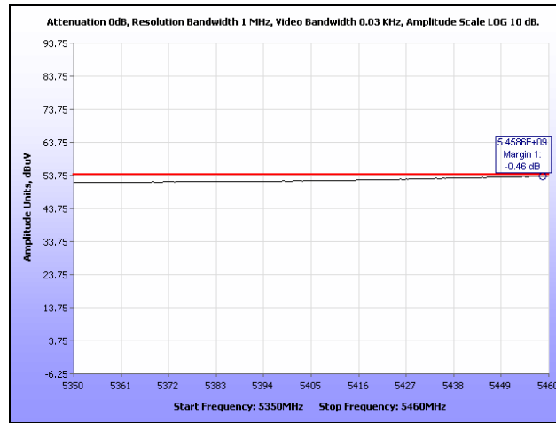
Plot 123. Restricted Band, HT5, Low Channel
