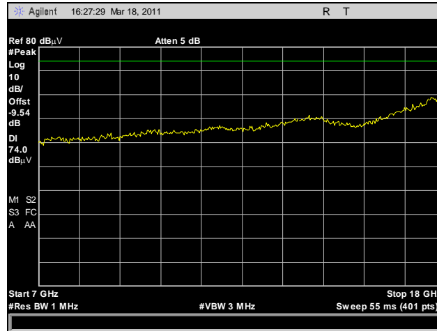
Plot 222. Radiated Spurious Emissions, HT40, Mid Channel, 7 GHz – 18 GHz, Peak
