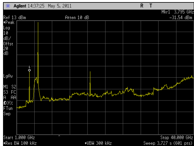
Plot 284. Conducted Spurious, Low Channel, HT8, Port 2, 1 GHz - 40 GHz
