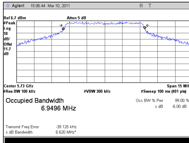
Plot 19. 6 dB Occupied Bandwidth, HT8, Port 1, Low Channel
