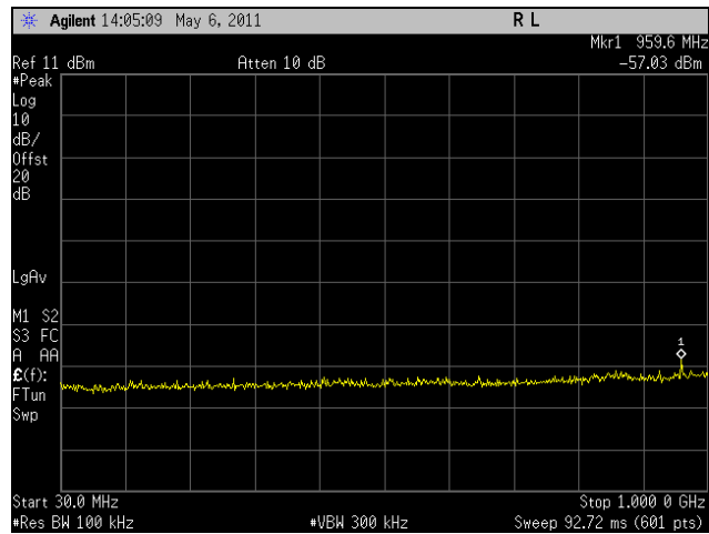
Plot 335. Conducted Spurious, High Channel, HT40, Port 2, 30 MHz - 1 GHz
