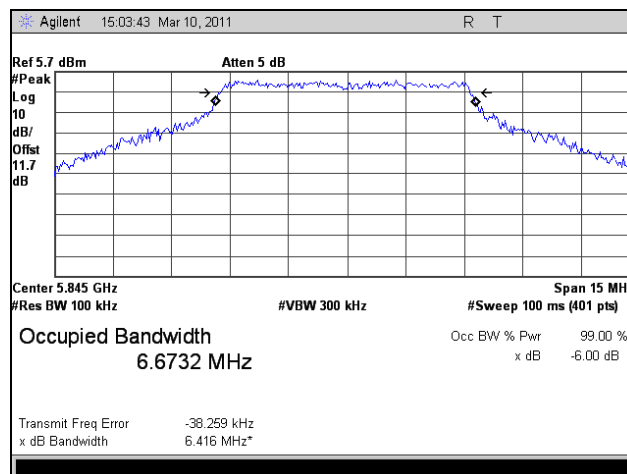
Plot 21. 6 dB Occupied Bandwidth, HT8, Port 1, High Channel
