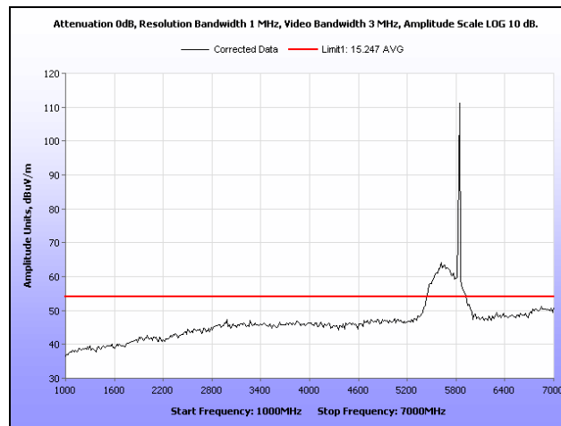
Plot 170. Radiated Spurious Emissions, HT10, High Channel, 1 GHz – 7 GHz, Average
