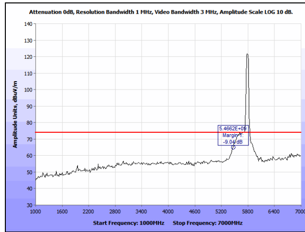
Plot 114. Radiated Spurious Emissions, Mid Channel, 802.11a 40MHz, 1 GHz – 7 GHz, Peak
