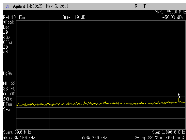
Plot 291. Conducted Spurious, Mid Channel, HT10, Port 1, 30 MHz - 1 GHz
