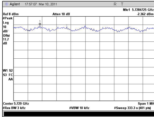
Plot 383. Peak Power Spectral Density, HT10, Port 1, Low Channel
