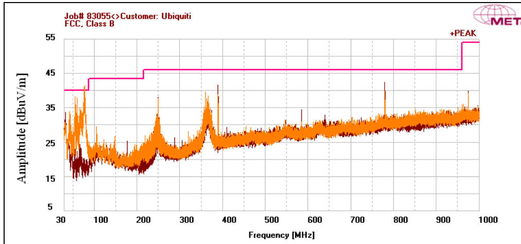
Plot 187. Radiated Spurious Emissions, HT20, High Channel, 30 MHz – 1 GHz
