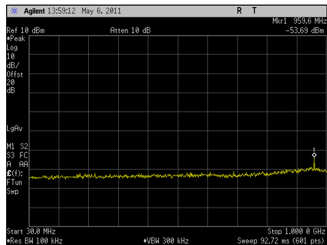
Plot 327. Conducted Spurious, Mid Channel, HT40, Port 1, 30 MHz - 1 GHz
