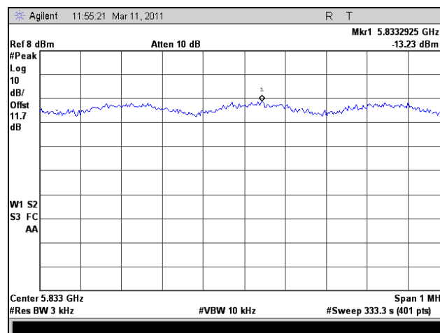
Plot 406. Peak Power Spectral Density, HT40, Port 2, High Channel
