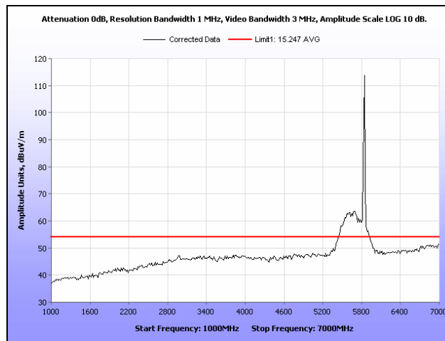
Plot 102. Radiated Spurious Emissions, High Channel, 802.11a 20MHz, 1 GHz – 7 GHz, Average
