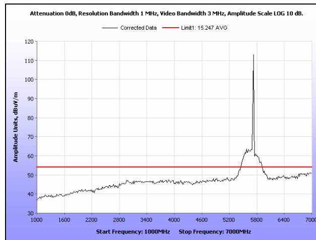
Plot 92. Radiated Spurious Emissions, Low Channel, 802.11a 20MHz, 1 GHz – 7 GHz, Average
