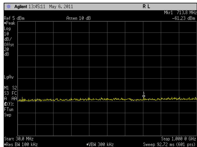
Plot 321. Conducted Spurious, Mid Channel, HT30, Port 2, 30 MHz - 1 GHz
