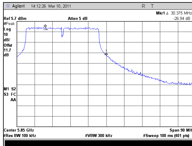
Plot 364. Conducted Band Edge, HT40, High Channel, Port 2
