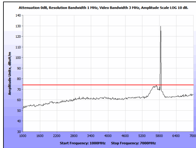
Plot 136. Radiated Spurious Emissions, HT5, High Channel, 1 GHz – 7 GHz, Peak
