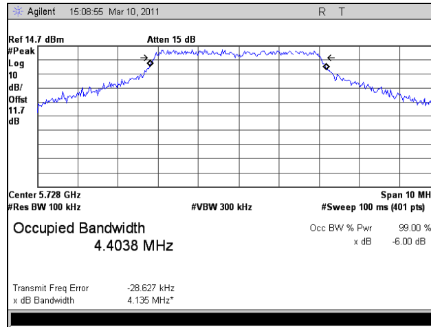
Plot 16. 6 dB Occupied Bandwidth, HT5, Port 2, Low Channel
