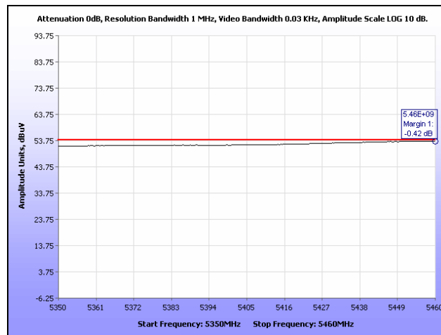
Plot 242. Restricted Band, HT10, Mid Channel
