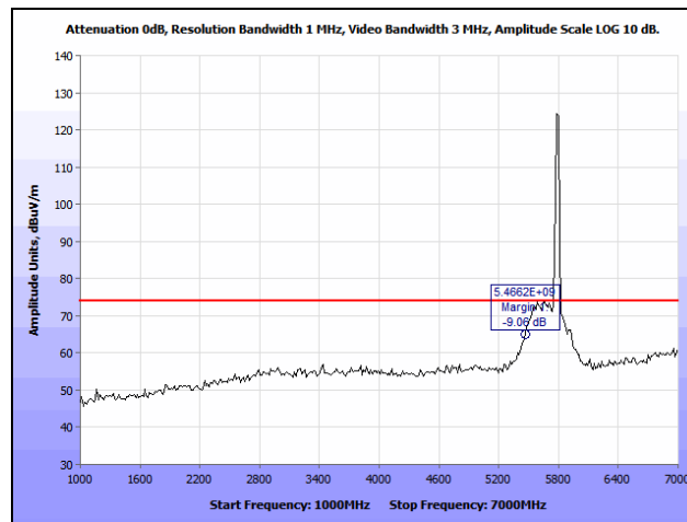
Plot 184. Radiated Spurious Emissions, HT20, Mid Channel, 1 GHz – 7 GHz, Peak
