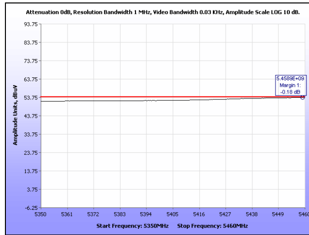
Plot 189. Restricted Band, HT20, High Channel
