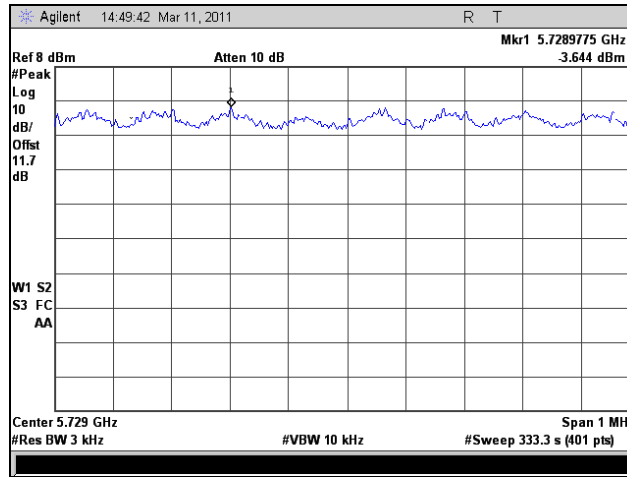
Plot 380. Peak Power Spectral Density, HT8, Port 2, Low Channel
