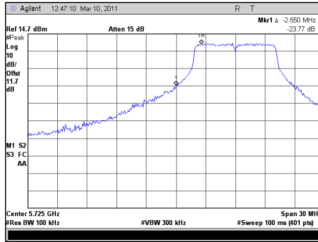
Plot 351. Conducted Band Edge, HT10, Low Channel, Port 2
