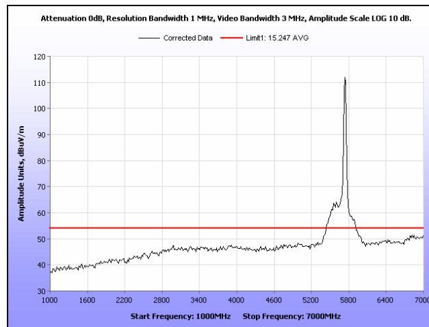
Plot 107. Radiated Spurious Emissions, Low Channel, 802.11a 40MHz, 1 GHz – 7 GHz, Average
