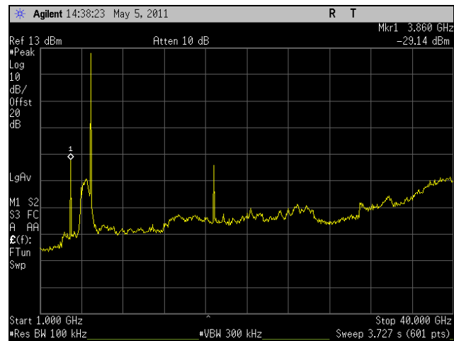
Plot 286. Conducted Spurious, Mid Channel, HT8, Port 2, 1 GHz - 40 GHz
