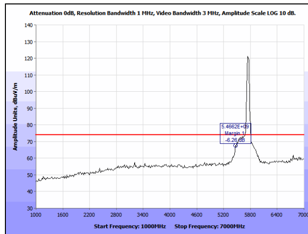
Plot 214. Radiated Spurious Emissions, HT40, Low Channel, 1 GHz – 7 GHz, Peak
