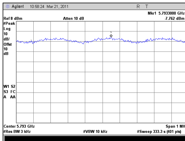
Plot 369. Peak Power Spectral Density, 802.11a 40 MHz, Mid Channel
