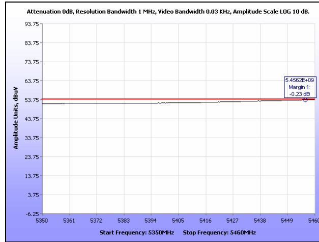
Plot 232. Restricted Band, 802.11a 40 MHz, Low Channel
