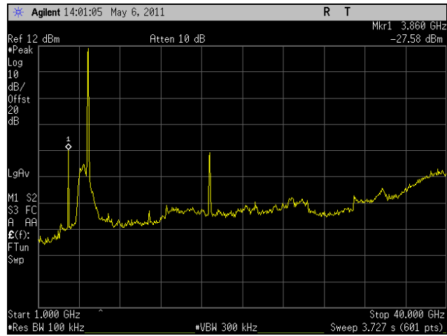
Plot 334. Conducted Spurious, Mid Channel, HT40, Port 2, 1 GHz - 40 GHz
