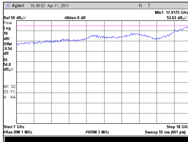
Plot 120. Radiated Spurious Emissions, High Channel, 802.11a 40 MHz, 7 GHz – 18 GHz
