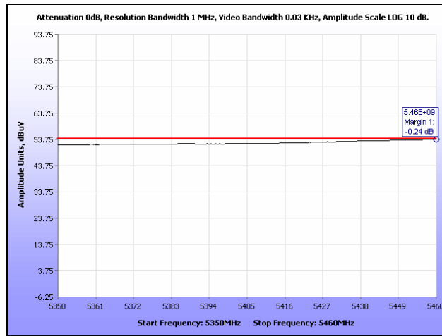
Plot 129. Restricted Band, HT5, Mid Channel
