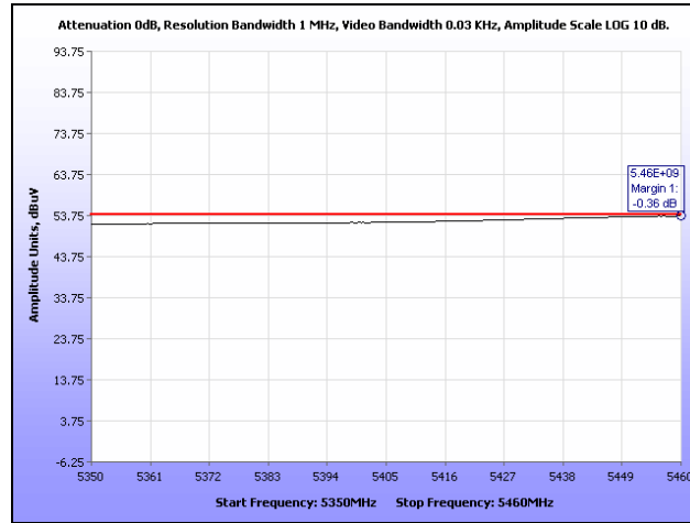
Plot 183. Restricted Band, HT20, Mid Channel
