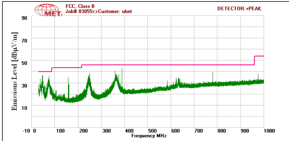
Plot 106. Radiated Spurious Emissions, 802.11a 40 MHz, Low Channel, 30 MHz – 1 GHz
