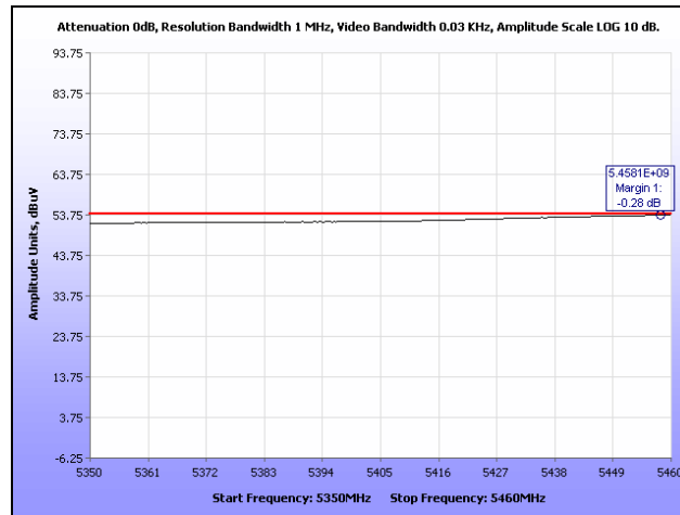
Plot 233. Restricted Band, 802.11a 40 MHz, Mid Channel
