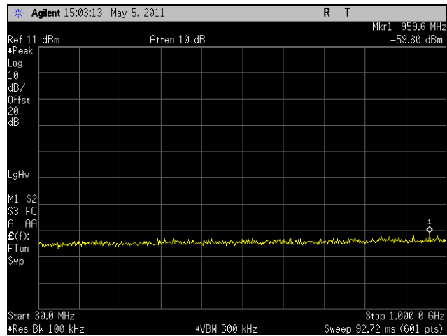
Plot 299. Conducted Spurious, High Channel, HT10, Port 2, 30 MHz - 1 GHz
