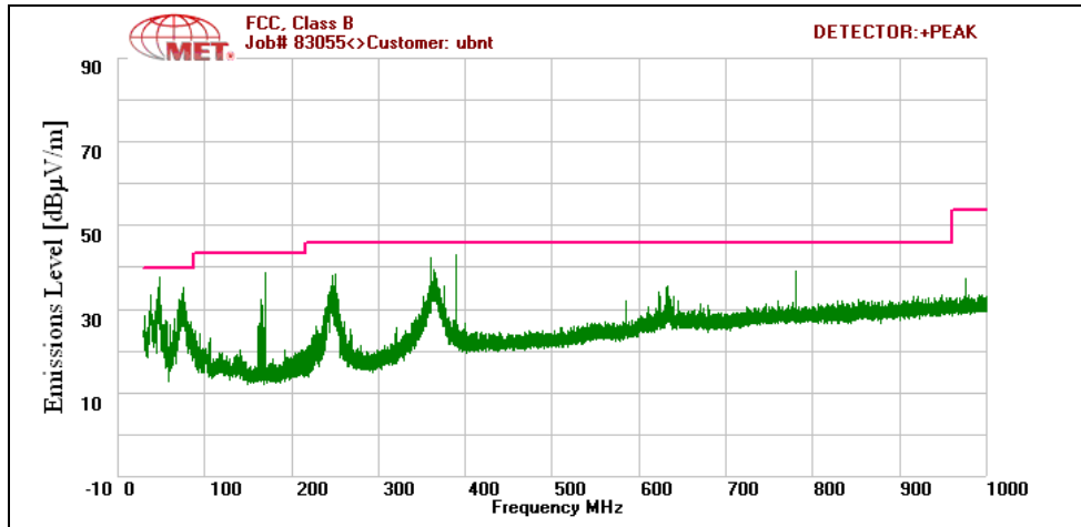
Plot 111. Radiated Spurious Emissions, 802.11a 40 MHz, Mid Channel, 30 MHz – 1 GHz
