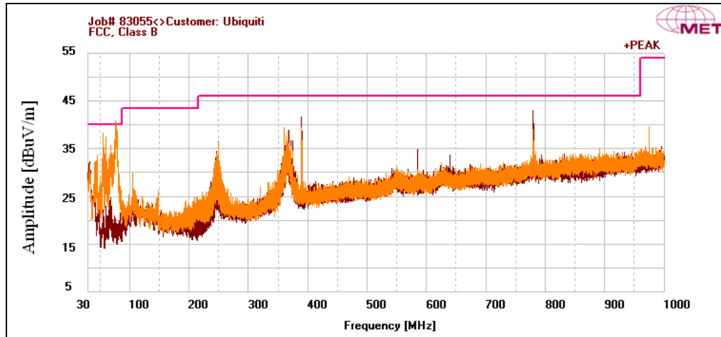
Plot 163. Radiated Spurious Emissions, HT10, Mid Channel, 30 MHz – 1 GHz
