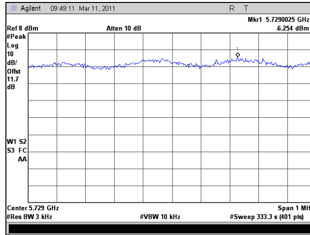
Plot 389. Peak Power Spectral Density, HT20, Port 1, Low Channel
