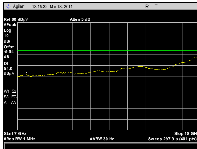
Plot 149. Radiated Spurious Emissions, HT8, Mid Channel, 7 GHz – 18 GHz, Average
