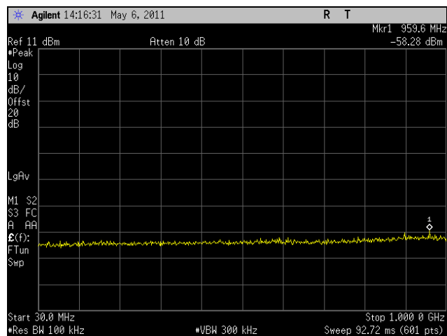
Plot 261. Conducted Spurious, Mid Channel, 802.11a 40 MHz, 30 MHz - 1 GHz
