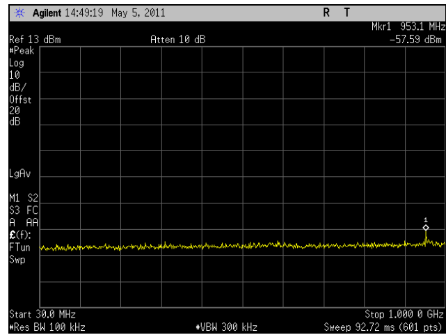
Plot 277. Conducted Spurious, Low Channel, HT8, Port 1, 30 MHz - 1 GHz
