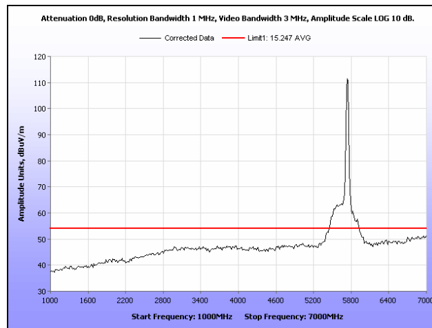
Plot 212. Radiated Spurious Emissions, HT40, Low Channel, 1 GHz – 7 GHz, Average
