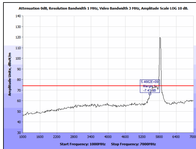
Plot 226. Radiated Spurious Emissions, HT40, High Channel, 1 GHz – 7 GHz, Peak
