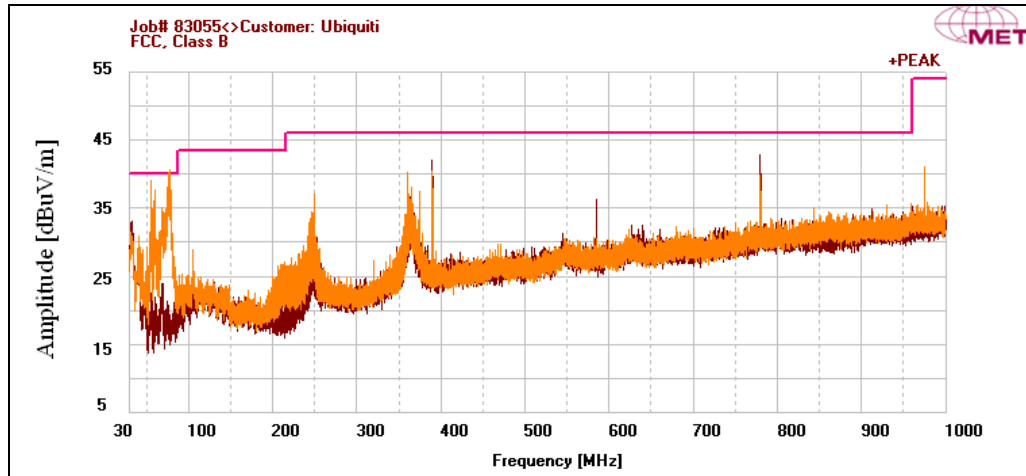
Plot 133. Radiated Spurious Emissions, HT5, High Channel, 30 MHz – 1 GHz
