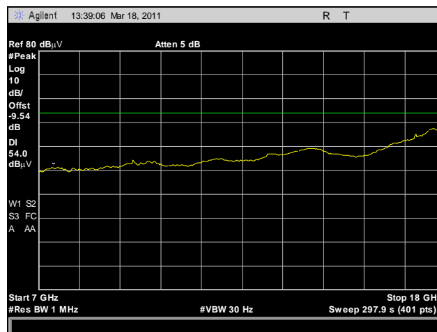
Plot 161. Radiated Spurious Emissions, HT10, Low Channel, 7 GHz – 18 GHz, Average
