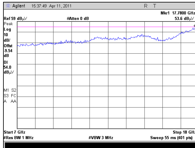
Plot 100. Radiated Spurious Emissions, Mid Channel, 802.11a 20 MHz, 7 GHz – 18 GHz
