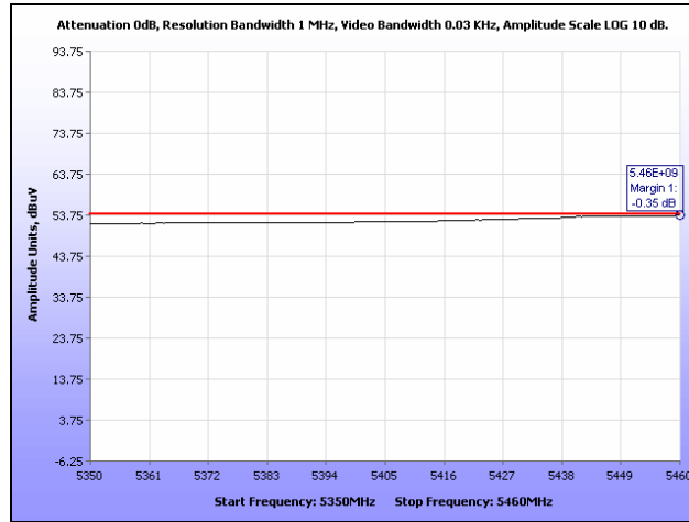
Plot 171. Restricted Band, HT10, High Channel
