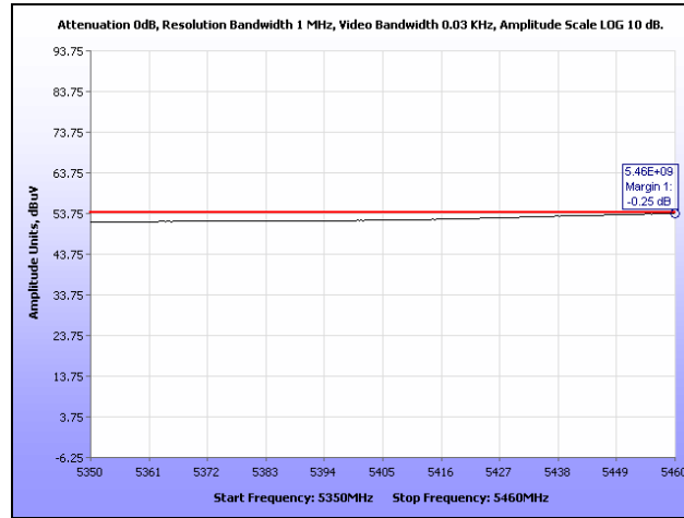
Plot 159. Restricted Band, HT10, Low Channel
