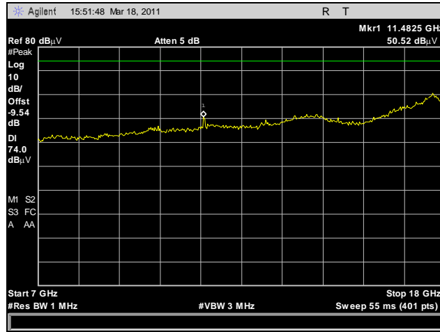
Plot 198. Radiated Spurious Emissions, HT30, Low Channel, 7 GHz – 18 GHz, Peak
