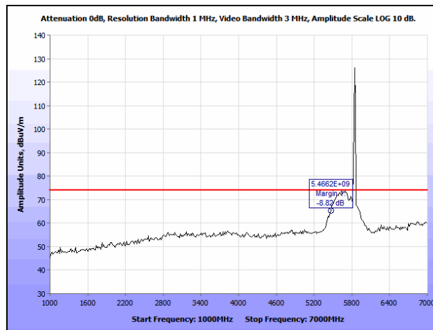
Plot 172. Radiated Spurious Emissions, HT10, High Channel, 1 GHz – 7 GHz, Peak
