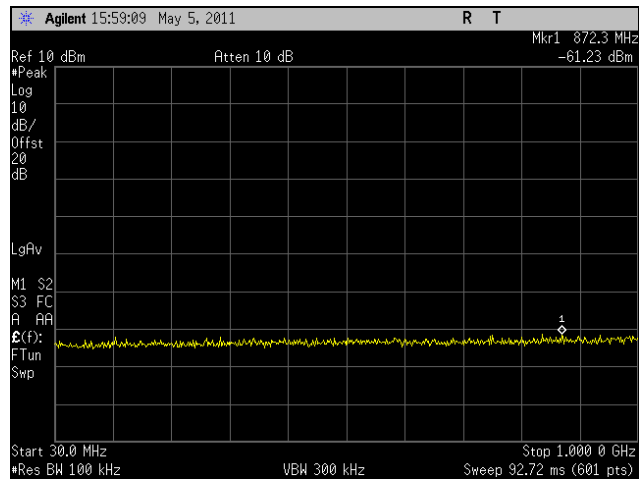
Plot 301. Conducted Spurious, Low Channel, HT20, Port 1, 30 MHz - 1 GHz
