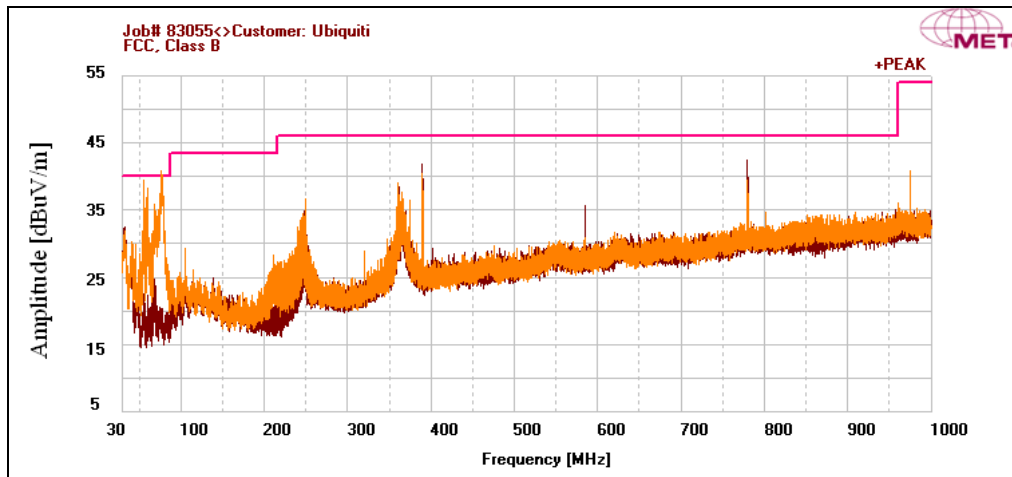
Plot 121. Radiated Spurious Emissions, HT5, Low Channel, 30 MHz – 1 GHz
