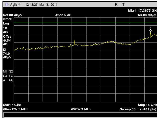
Plot 132. Radiated Spurious Emissions, HT5, Mid Channel, 7 GHz – 18 GHz, Peak
