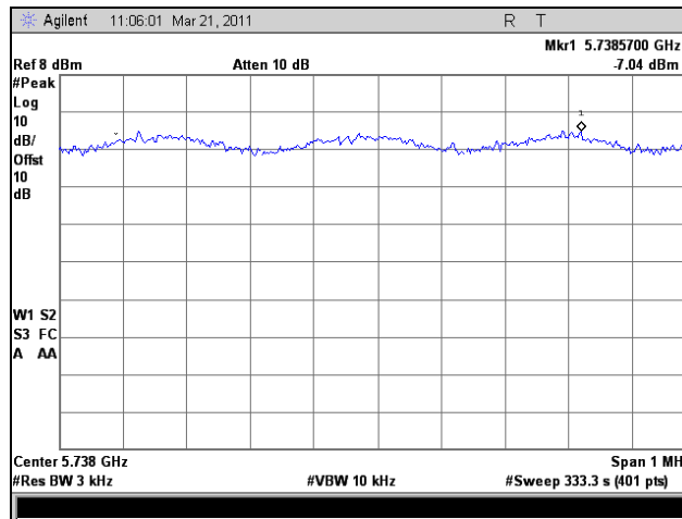
Plot 368. Peak Power Spectral Density, 802.11 40 MHz, Low Channel
