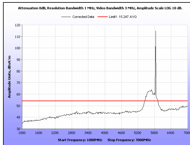
Plot 134. Radiated Spurious Emissions, HT5, High Channel, 1 GHz – 7 GHz, Average
