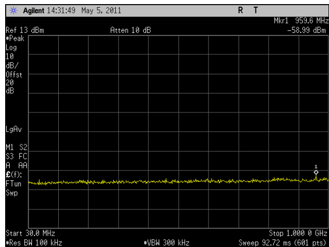
Plot 275. Conducted Spurious, High Channel, HT5, Port 2, 30 MHz - 1 GHz
