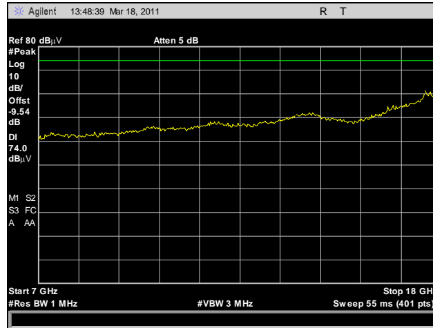
Plot 174. Radiated Spurious Emissions, HT10, High Channel, 7 GHz – 18 GHz, Peak
