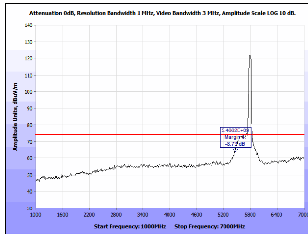
Plot 220. Radiated Spurious Emissions, HT40, Mid Channel, 1 GHz – 7 GHz, Peak
