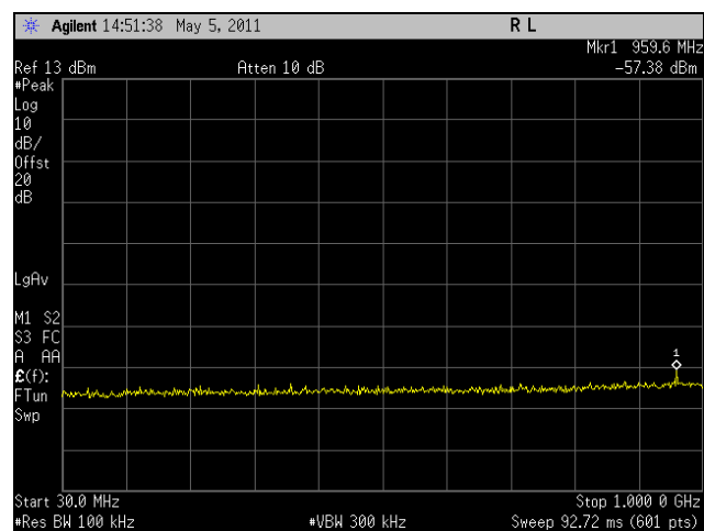
Plot 279. Conducted Spurious, Mid Channel, HT8, Port 1, 30 MHz - 1 GHz
