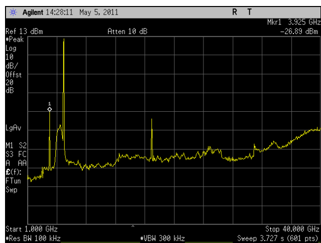
Plot 276. Conducted Spurious, High Channel, HT5, Port 2, 1 GHz - 40 GHz
