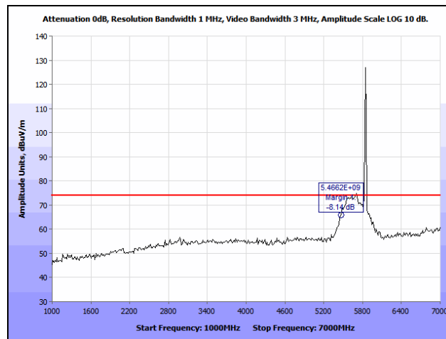
Plot 154. Radiated Spurious Emissions, HT8, High Channel, 1 GHz – 7 GHz, Peak
