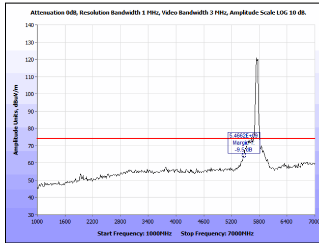
Plot 109. Radiated Spurious Emissions, Low Channel, 802.11a 40MHz, 1 GHz – 7 GHz, Peak
