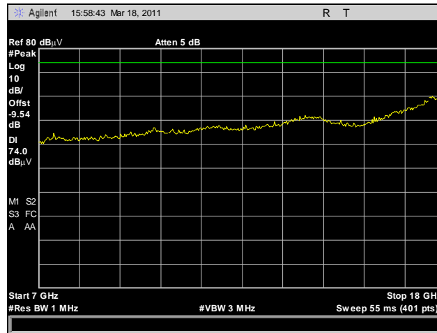
Plot 204. Radiated Spurious Emissions, HT30, Mid Channel, 7 GHz – 18 GHz, Peak
