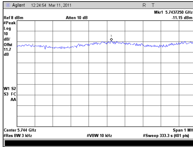
Plot 398. Peak Power Spectral Density, HT30 Port 2, Low Channel
