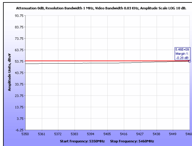
Plot 248. Restricted Band, HT30, Mid Channel
