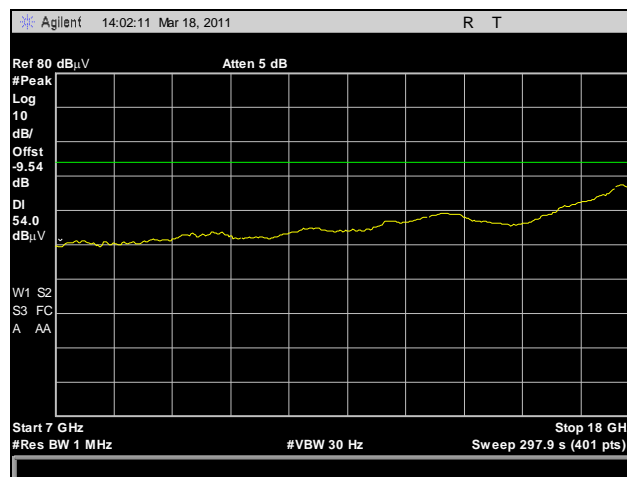
Plot 191. Radiated Spurious Emissions, HT20, High Channel, 7 GHz – 18 GHz, Average
