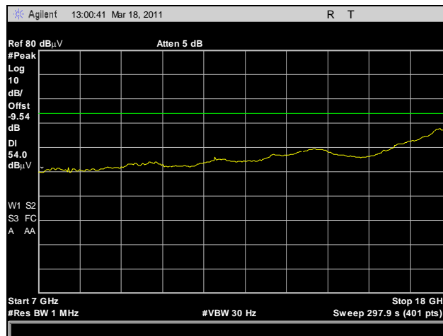
Plot 131. Radiated Spurious Emissions, HT5, Mid Channel, 7 GHz – 18 GHz, Average
