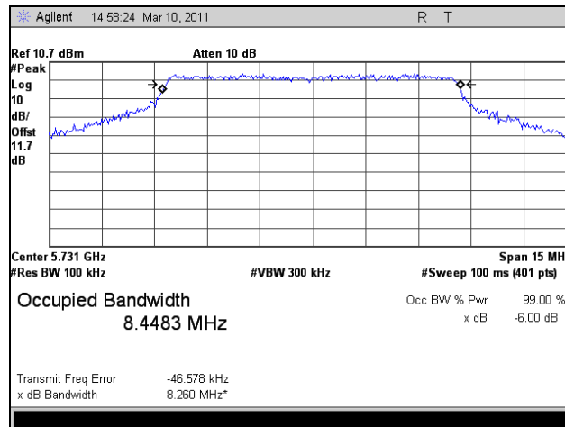
Plot 25. 6 dB Occupied Bandwidth, HT10, Port 1, Low Channel
