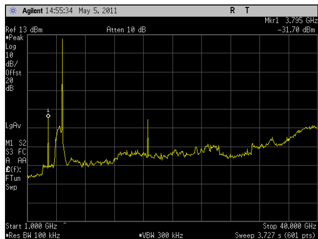
Plot 296. Conducted Spurious, Low Channel, HT10, Port 2, 1 GHz - 40 GHz
