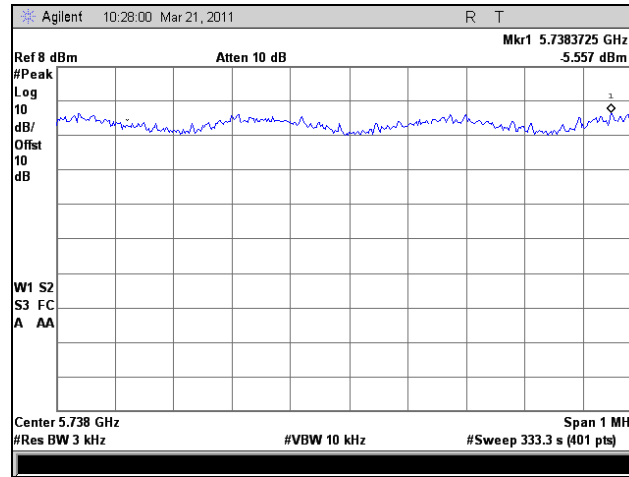
Plot 365. Peak Power Spectral Density, 802.11 20 MHz, Low Channel
