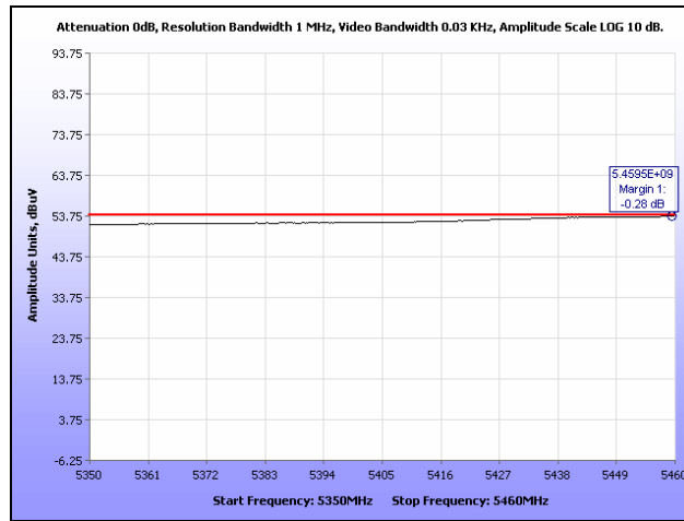
Plot 207. Restricted Band, HT30, High Channel
