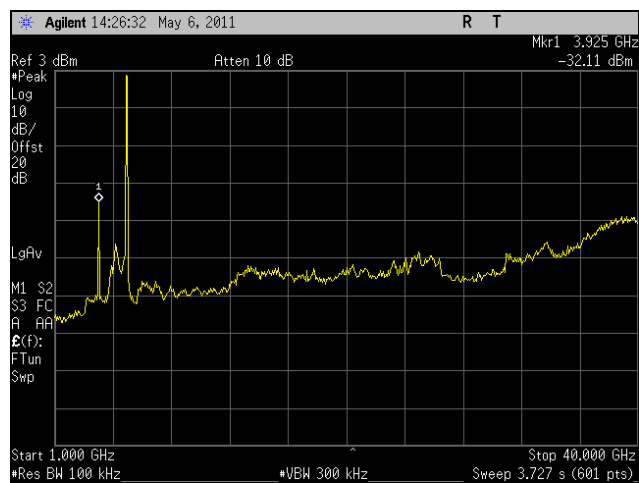
Plot 258. Conducted Spurious, High Channel, 802.11a 20 MHz, 1 GHz - 40 GHz
