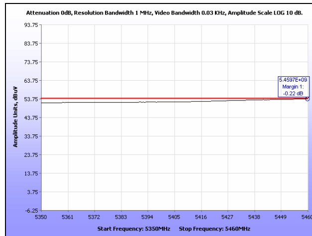
Plot 234. Restricted Band, 802.11a 40 MHz, High Channel
