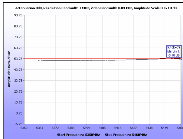
Plot 237. Restricted Band, HT5, High Channel
