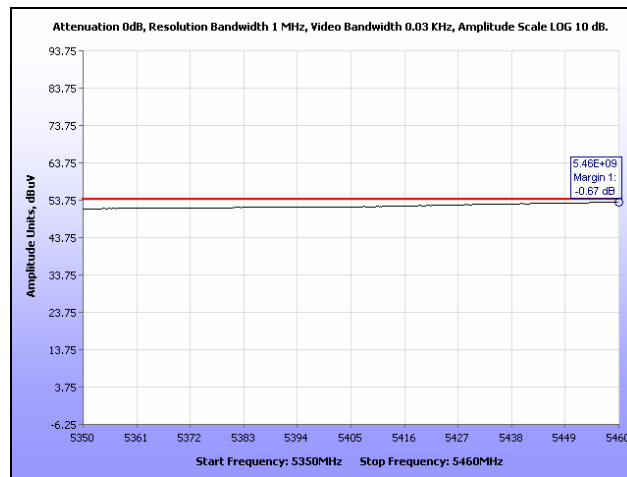
Plot 239. Restricted Band, HT8, Mid Channel
