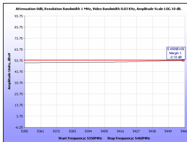
Plot 246. Restricted Band, HT20, High Channel
