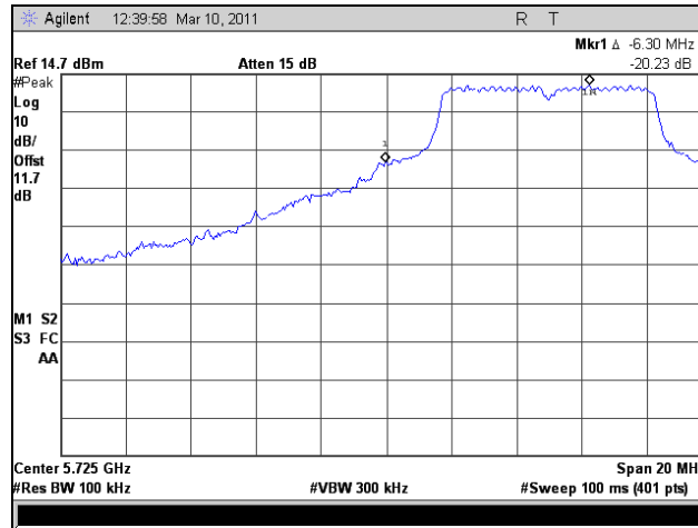
Plot 347. Conducted Band Edge, HT8, Low Channel, Port 2
