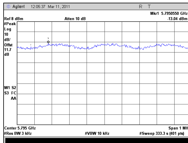
Plot 405. Peak Power Spectral Density, HT40, Port 2, Mid Channel
