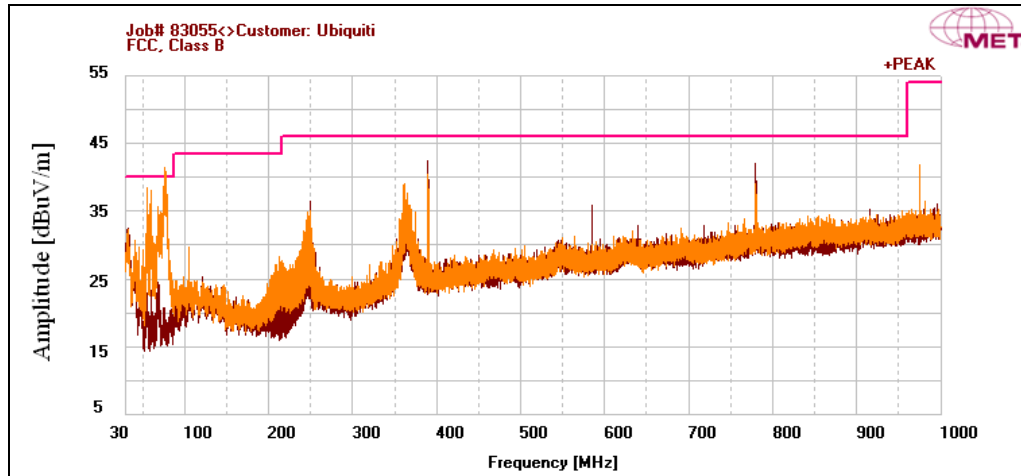
Plot 127. Radiated Spurious Emissions, HT5, Mid Channel, 30 MHz – 1 GHz
