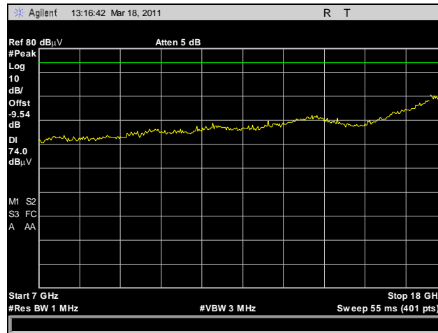
Plot 156. Radiated Spurious Emissions, HT8, High Channel, 7 GHz – 18 GHz, Peak
