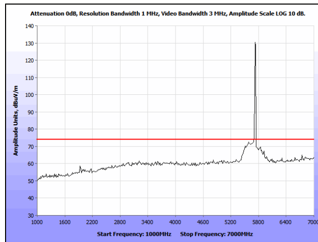
Plot 124. Radiated Spurious Emissions, HT5, Low Channel, 1 GHz – 7 GHz, Peak
