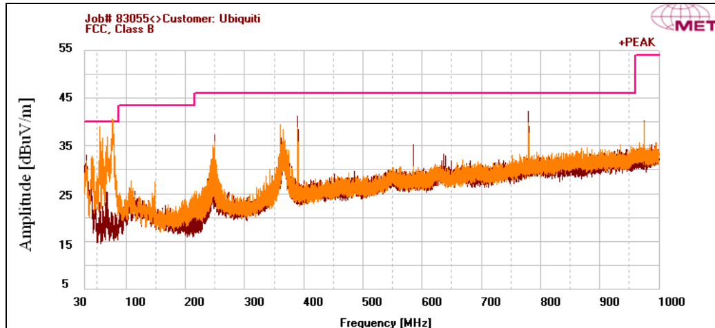
Plot 145. Radiated Spurious Emissions, HT8, Mid Channel, 30 MHz – 1 GHz
