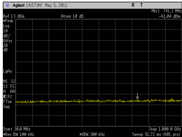
Plot 295. Conducted Spurious, Low Channel, HT10, Port 2, 30 MHz - 1 GHz
