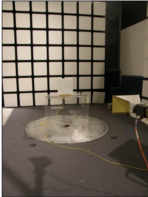
Photograph 6. Radiated Spurious Emissions, Test Setup, 1 GHz – 18 GHz
