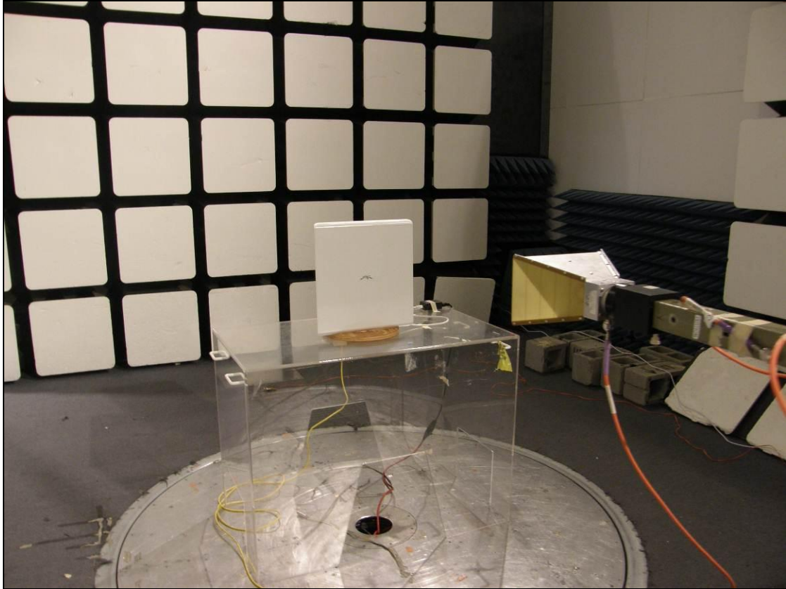
Photograph 4. Radiated Harmonics, Test Setup
