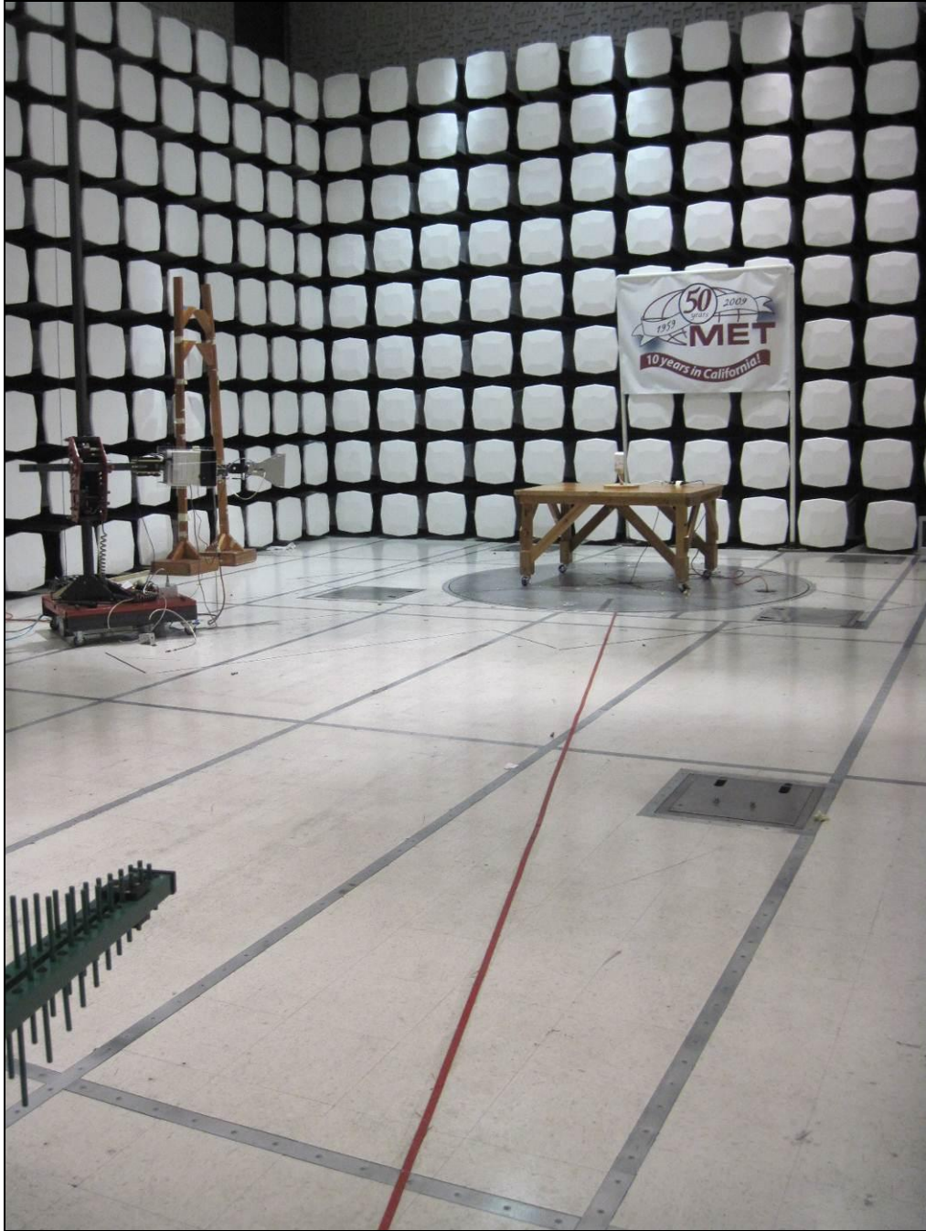
Photograph 2. Radiated Emission, Test Setup
