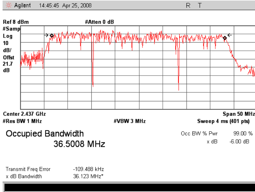
Plot 22. 802.11/n Mid Ch Occupied Band Width
