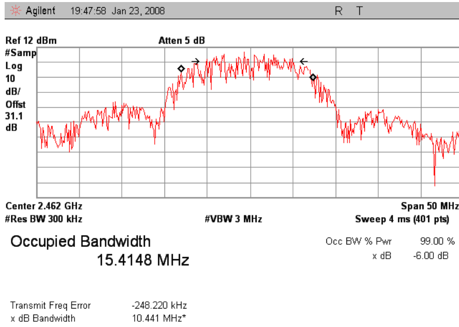
Plot 7. 802.11/b High Ch Occupied Band Width
