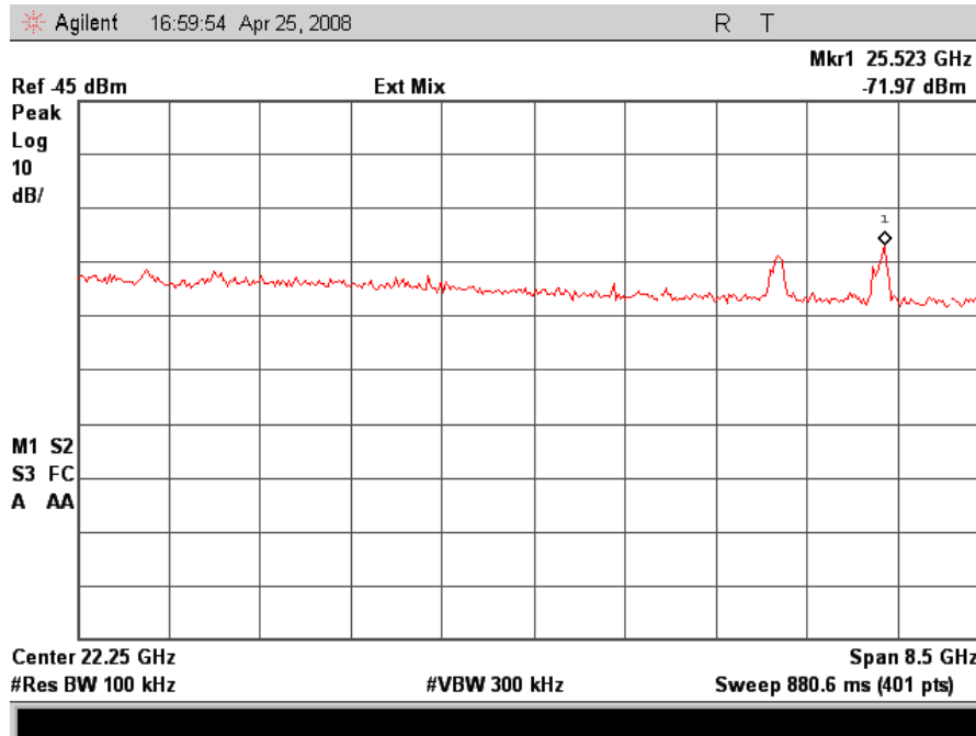
802.11/n – Low Channel Conducted Emissions 18GHz – 26.5GHz
