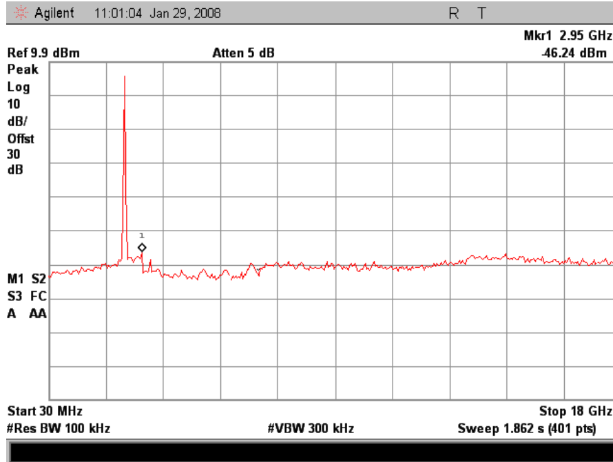
802.11/n – Low Channel Conducted Emissions 30MHz - 18GHz
