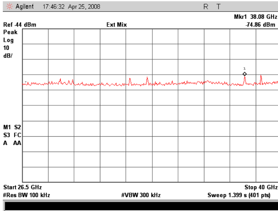
802.11/a – High Channel Conducted Emissions 26.5GHz- 40GHz
