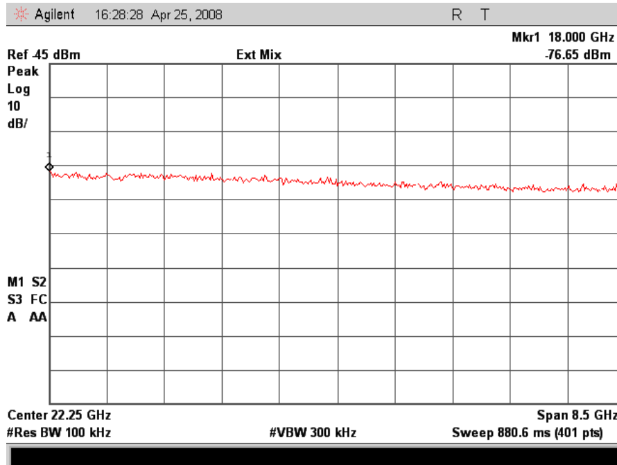
802.11/g – Low Channel Conducted Emissions 18GHz – 26.5GHz
