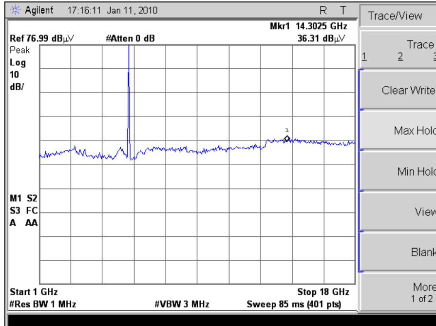
Plot 45. Radiated Spurious Emissions, 802.11n 20MHz Mode Mid Channel
