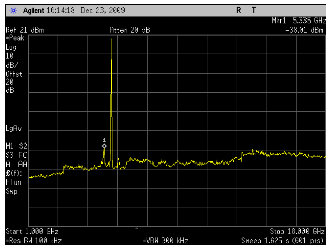
Plot 55. Conducted Spurious 5745MHz Low Channel 802.11n 20MHz Port 1 (1-18GHz)
