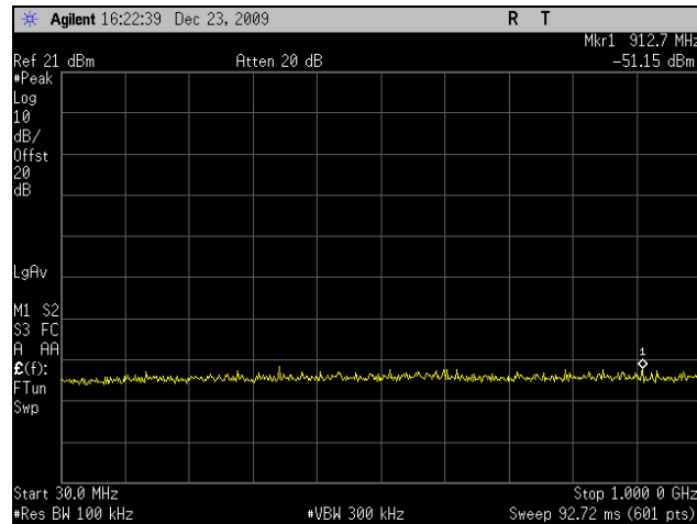
Plot 66. Conducted Spurious 5785MHz Mid Channel 802.11n 40MHz Port 1 (30MHz-1GHz)
