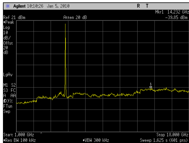
Plot 88. Conducted Spurious 5825MHz High Channel 802.11n 40MHz Port 2 (1-18GHz)
