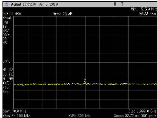
Plot 87. Conducted Spurious 5825MHz High Channel 802.11n 40MHz Port 2 (30MHz-1GHz)
