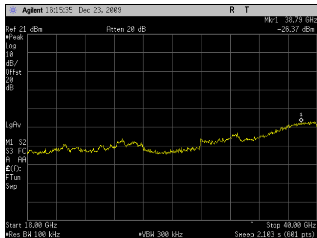
Plot 56. Conducted Spurious 5745MHz Low Channel 802.11n 20MHz Port 1 (18-40GHz)
