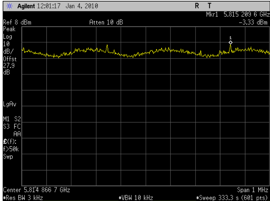
Plot 115. Power Spectral Density 5825MHz High Channel 802.11n 40MHz Combined
