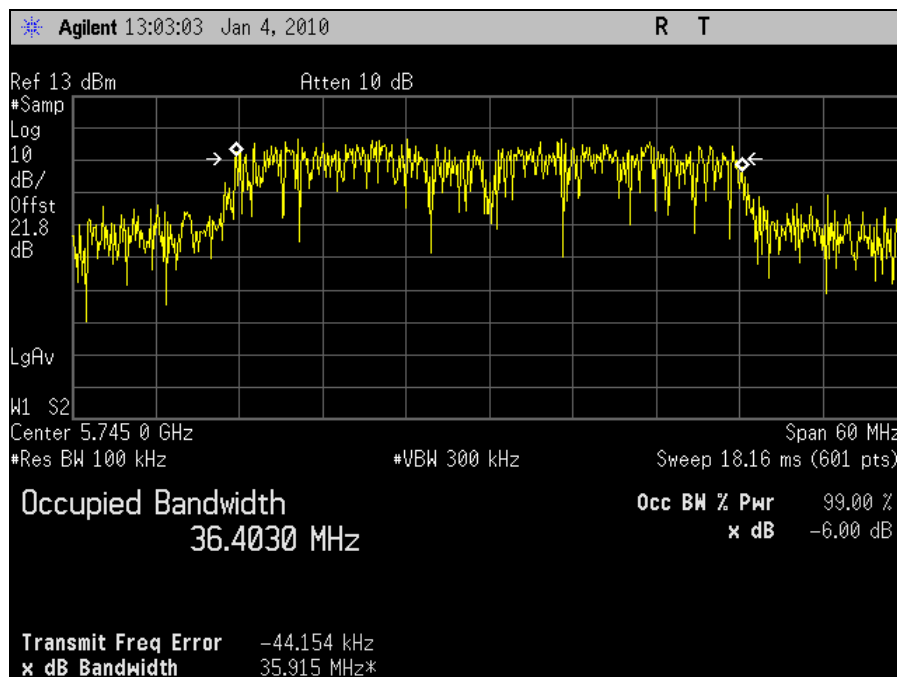
Plot 27. Occupied Bandwidth 5745MHz Low Channel 802.11n 40MHz Port 2 (100kHz)
