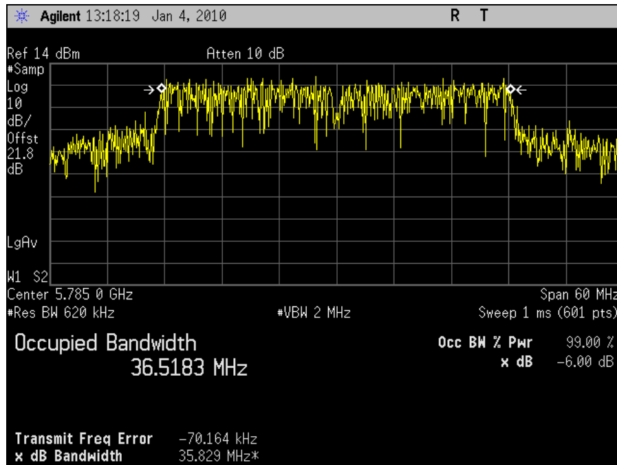
Plot 28. Occupied Bandwidth 5785MHz Mid Channel 802.11n 40MHz Port 2 (99%)
