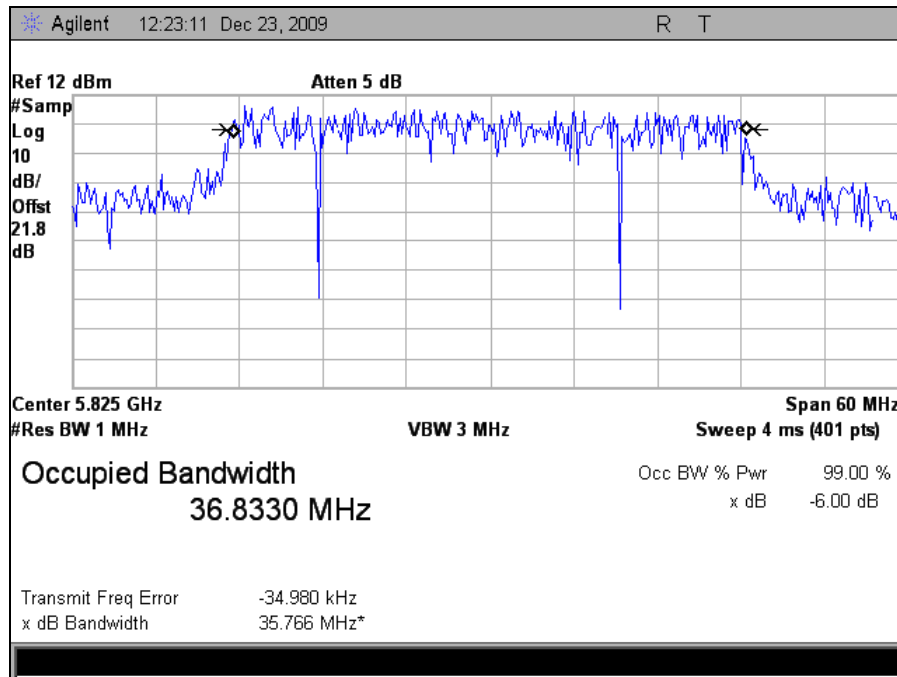
Plot 18. Occupied Bandwidth 5825MHz High Channel 802.11n 40MHz Port 1 (99%)
