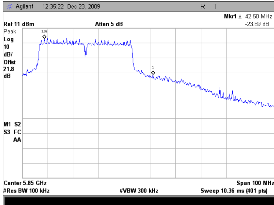
Plot 93. Conducted Band Edge 5825MHz High Channel 802.11n 40MHz Port 1
