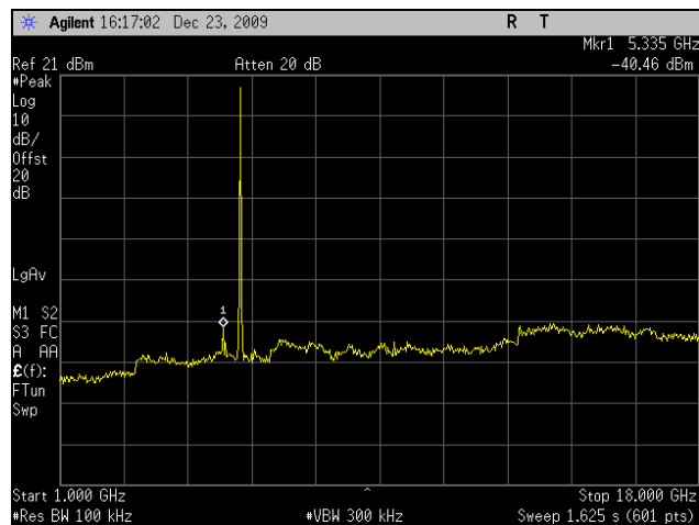
Plot 58. Conducted Spurious 5785MHz Mid Channel 802.11n 20MHz Port 1 (1-18GHz)
