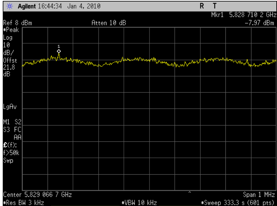
Plot 109. Power Spectral Density 5825MHz High Channel 802.11n 40MHz Port 2
