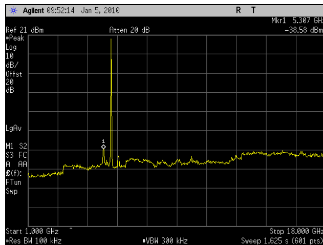
Plot 73. Conducted Spurious 5745MHz Low Channel 802.11n 20MHz Port 2 (1-18GHz)
