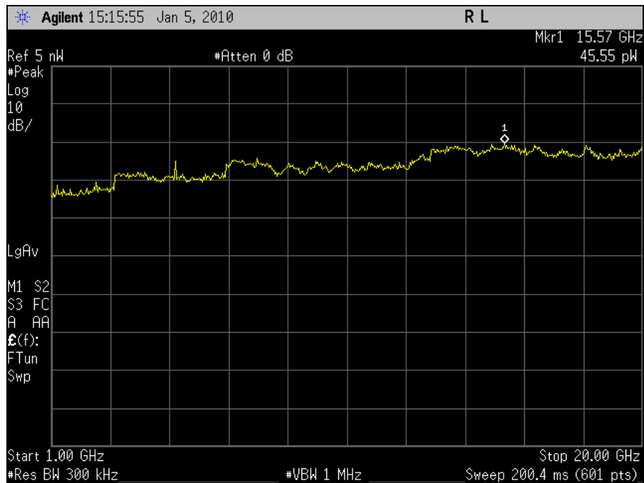
Plot 53. Conducted Receiver Spurious Emission, 1 GHz – 20 GHz, Port 2
