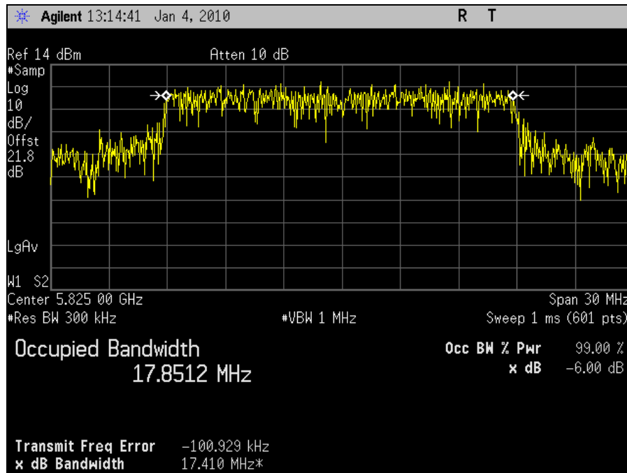
Plot 24. Occupied Bandwidth 5825MHz High Channel 802.11n 20MHz Port 2 (99%)
