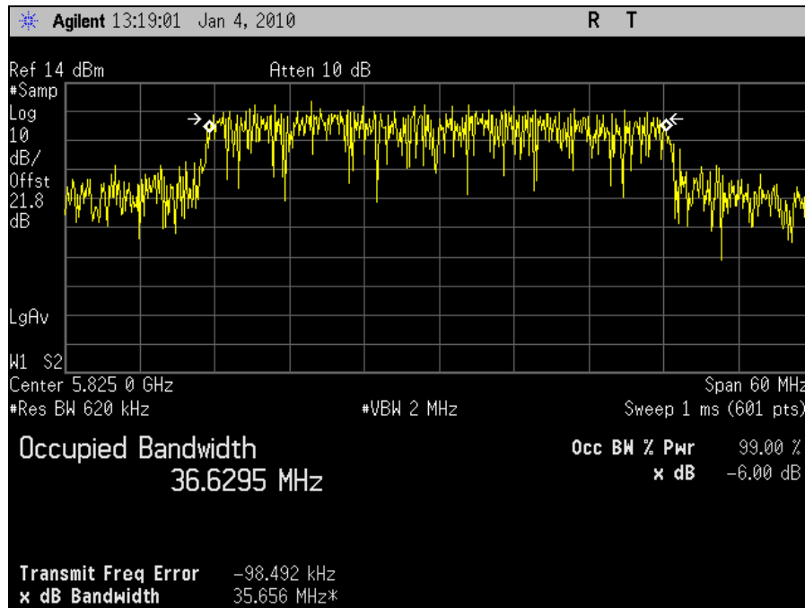
Plot 30. Occupied Bandwidth 5825MHz High Channel 802.11n 40MHz Port 2 (99%)
