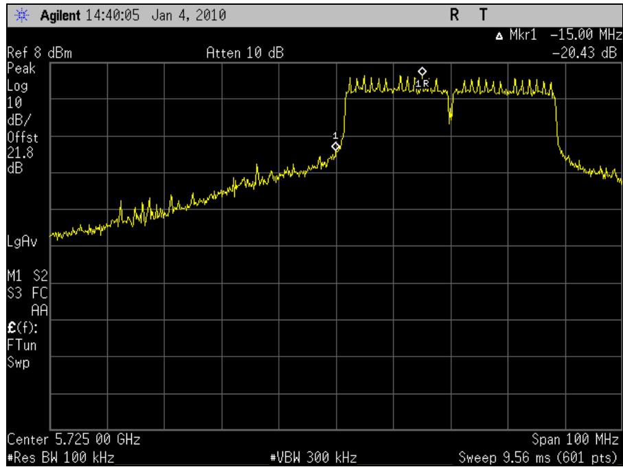
Plot 96. Conducted Band Edge 5745MHz Low Channel 802.11n 40MHz Port 2
