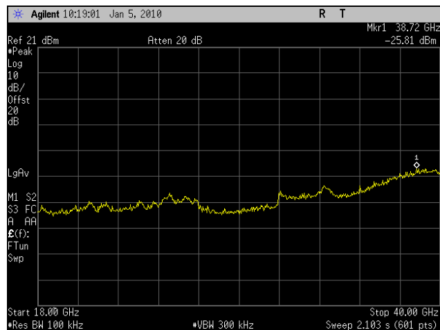
Plot 83. Conducted Spurious 5745MHz Low Channel 802.11n 40MHz Port 2 (18-40GHz)
