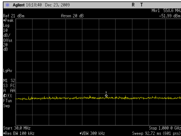
Plot 60. Conducted Spurious 5825MHz High Channel 802.11n 20MHz Port 1 (30MHz-1GHz)
