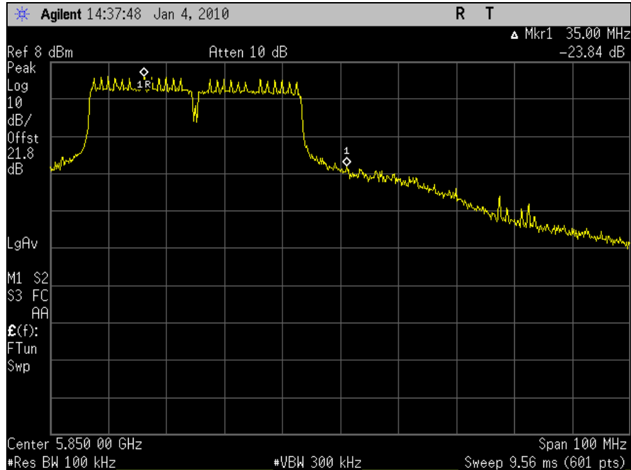
Plot 97. Conducted Band Edge 5825MHz High Channel 802.11n 40MHz Port 2
