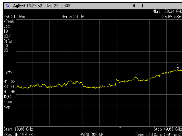
Plot 68. Conducted Spurious 5785MHz Mid Channel 802.11n 40MHz Port 1 (18-40GHz)
