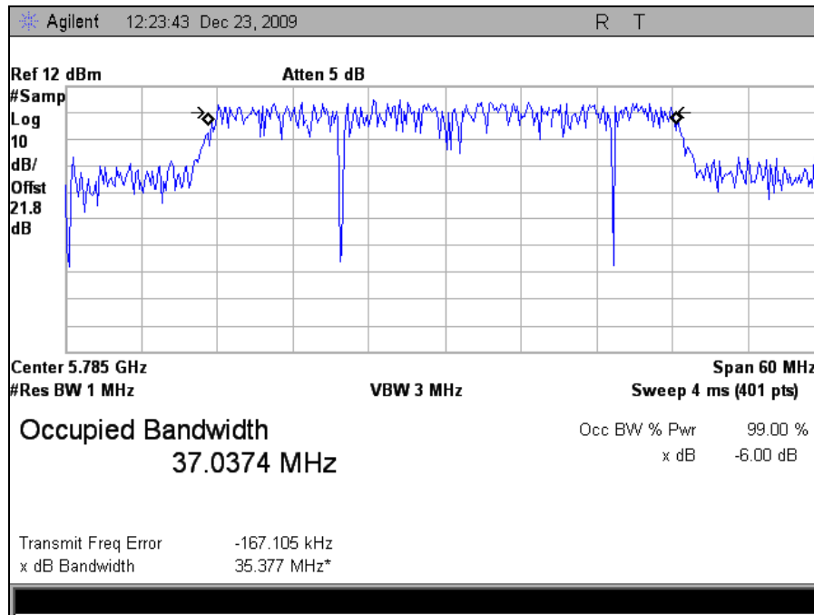
Plot 16. Occupied Bandwidth 5785MHz Mid Channel 802.11n 40MHz Port 1 (99%)
