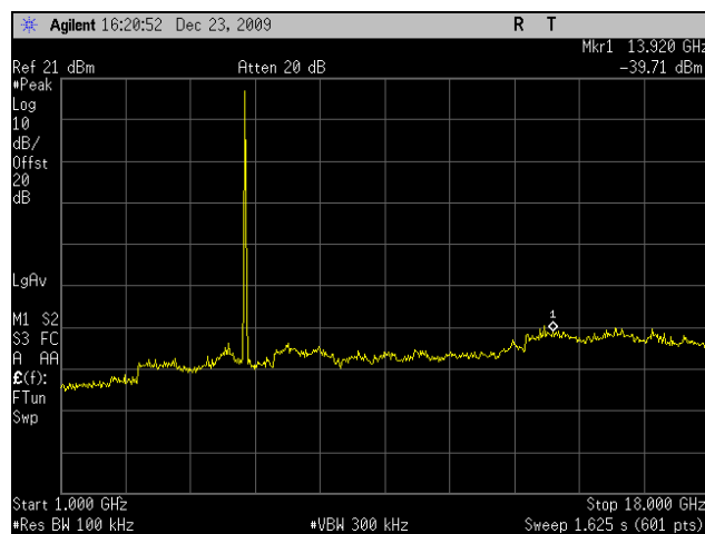
Plot 70. Conducted Spurious 5825MHz High Channel 802.11n 40MHz Port 1 (1-18GHz)
