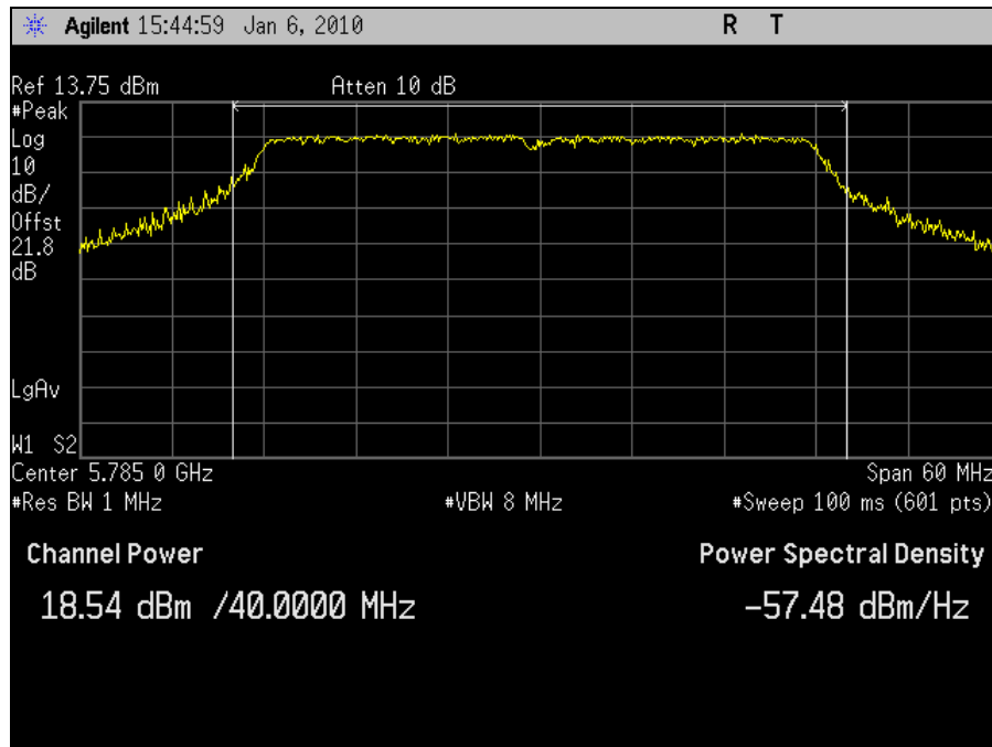
Plot 42. Peak Output Power 5785MHz Mid Channel 802.11n 40MHz Port 2
