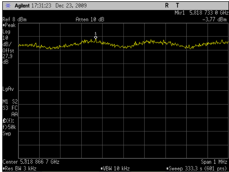
Plot 112. Power Spectral Density 5825MHz High Channel 802.11n 20MHz Combined
