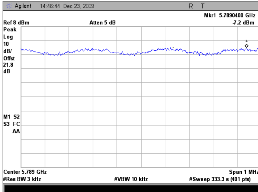
Plot 99. Power Spectral Density 5785MHz Mid Channel 802.11n 20MHz Port 1
