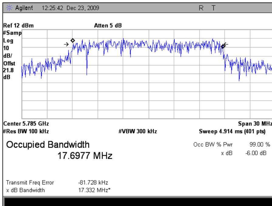
Plot 11. Occupied Bandwidth 5785MHz Mid Channel 802.11n 20MHz Port 1 (100kHz RBW)
