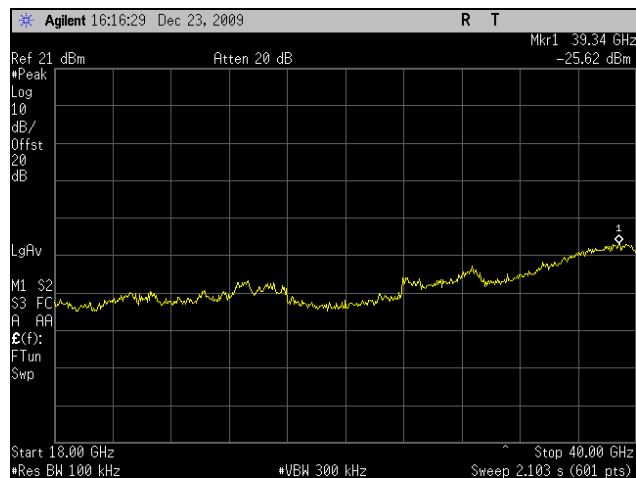
Plot 59. Conducted Spurious 5785MHz Mid Channel 802.11n 20MHz Port 1 (18-40GHz)
