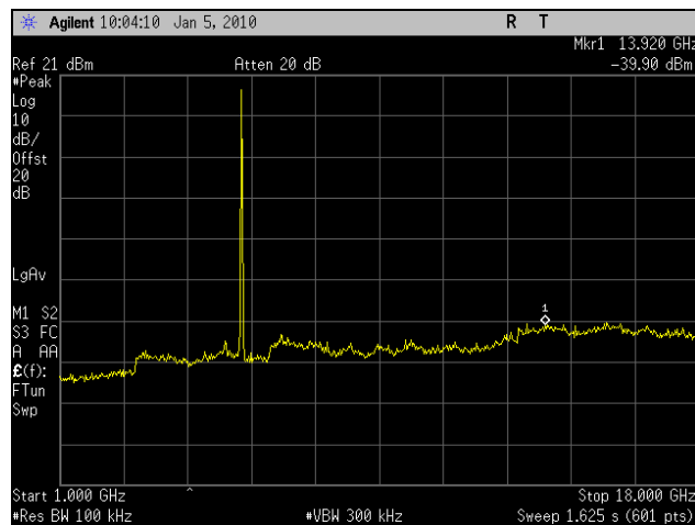
Plot 79. Conducted Spurious 5825MHz High Channel 802.11n 20MHz Port 2 (1-18GHz)
