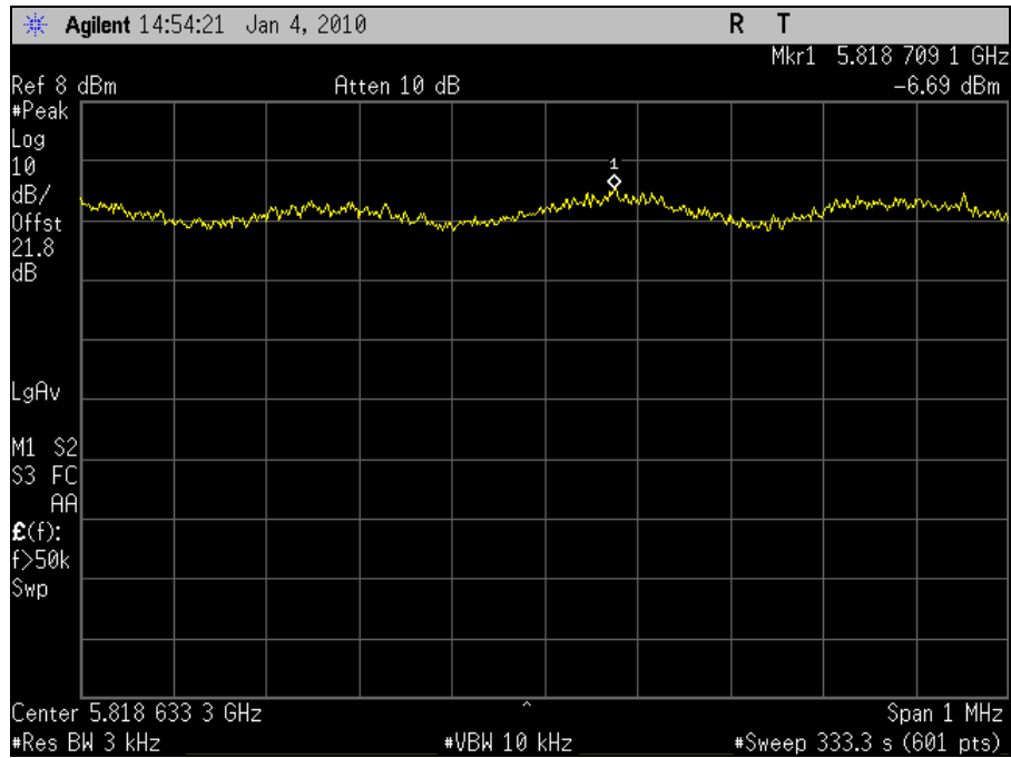
Plot 106. Power Spectral Density 5825MHz High Channel 802.11n 20MHz Port 2
