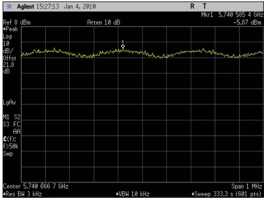
Plot 104. Power Spectral Density 5745MHz Low Channel 802.11n 20MHz Port 2
