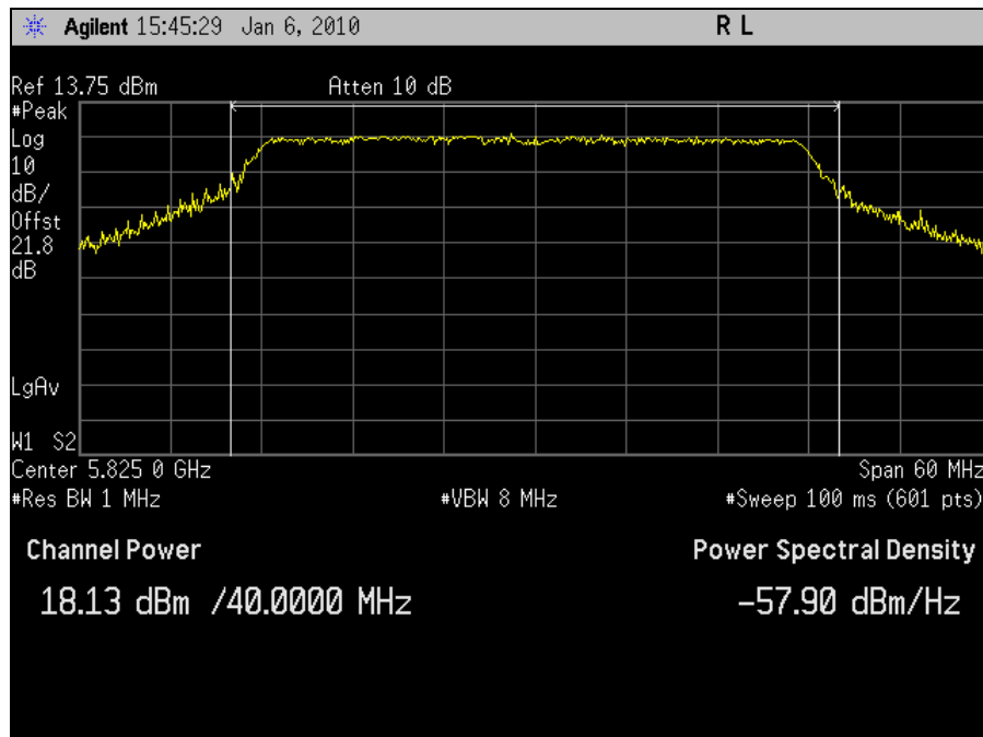
Plot 43. Peak Output Power 5825MHz High Channel 802.11n 40MHz Port 2
