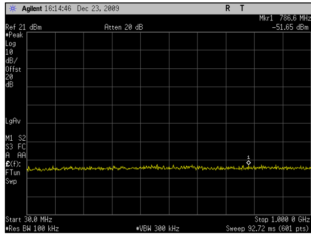
Plot 54. Conducted Spurious 5745MHz Low Channel 802.11n 20MHz Port 1 (30MHz-1GHz)
