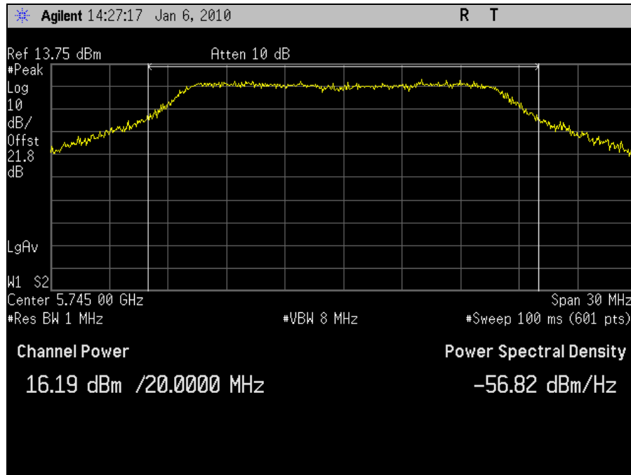
Plot 32. Peak Output Power 5745MHz Low Channel 802.11n 20MHz Port 1
