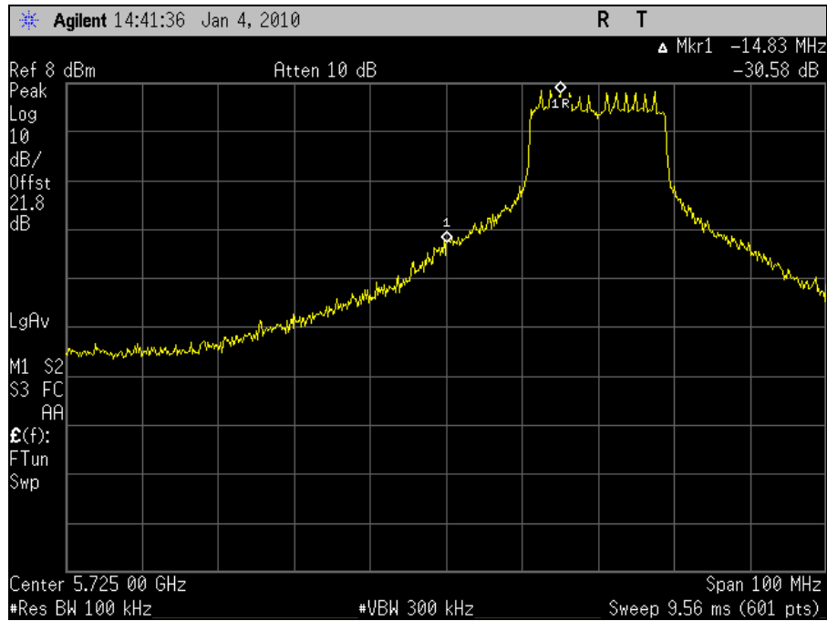
Plot 94. Conducted Band Edge 5745MHz Low Channel 802.11n 20MHz Port 2
