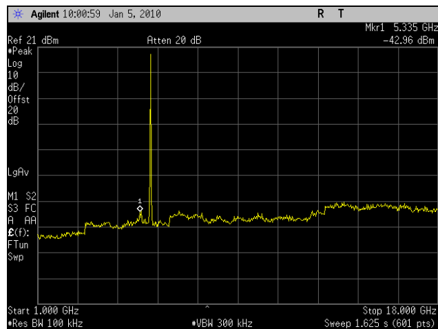
Plot 76. Conducted Spurious 5785MHz Mid Channel 802.11n 20MHz Port 2 (1-18GHz)
