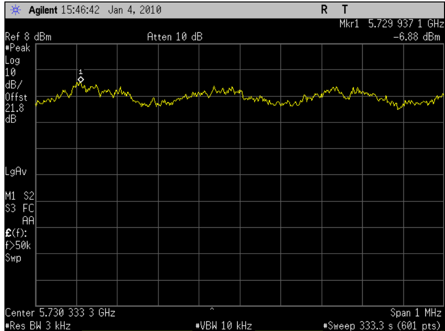
Plot 107. Power Spectral Density 5745MHz Low Channel 802.11n 40MHz Port 2
