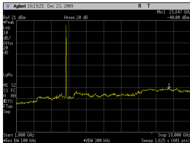
Plot 61. Conducted Spurious 5825MHz High Channel 802.11n 20MHz Port 1 (1-18GHz)
