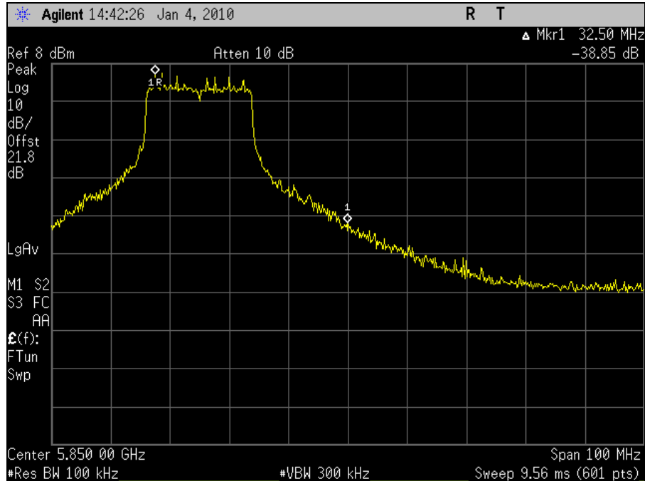
Plot 95. Conducted Band Edge 5825MHz High Channel 802.11n 20MHz Port 2
