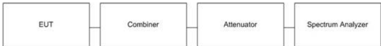
Figure 6. Block Diagram, Peak Power Spectral Density Test Setup, MIMO
