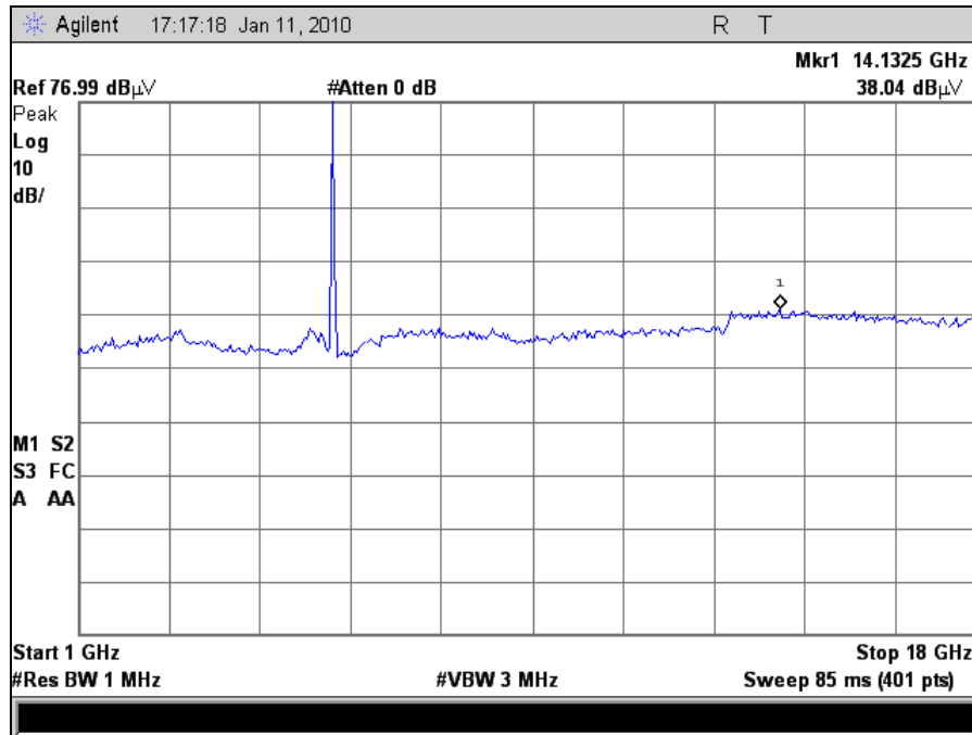
Plot 44. Radiated Spurious Emissions, 802.11n 20MHz Mode Low Channel
