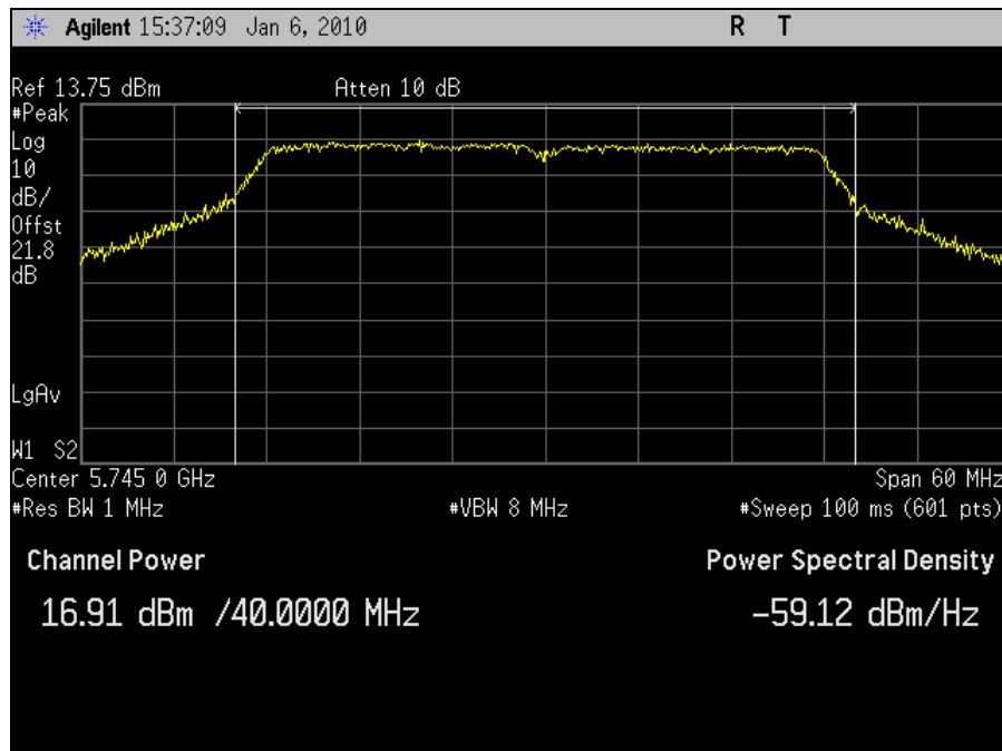
Plot 35. Peak Output Power 5745MHz Low Channel 802.11n 40MHz Port 1
