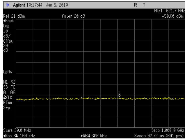
Plot 81. Conducted Spurious 5745MHz Low Channel 802.11n 40MHz Port 2 (30MHz-1GHz)
