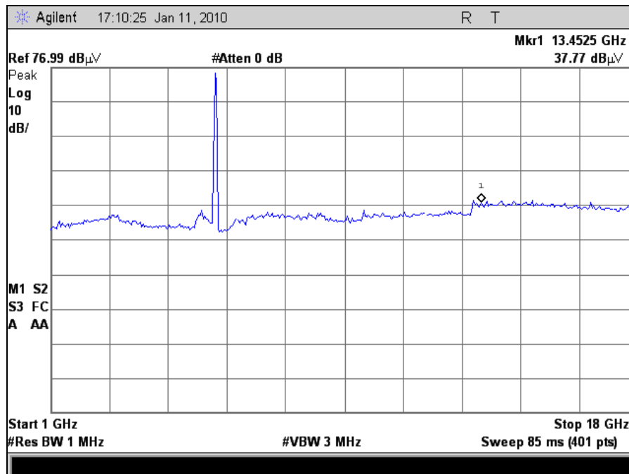
Plot 47. Radiated Spurious Emissions, 802.11n 40MHz Mode Low Channel
