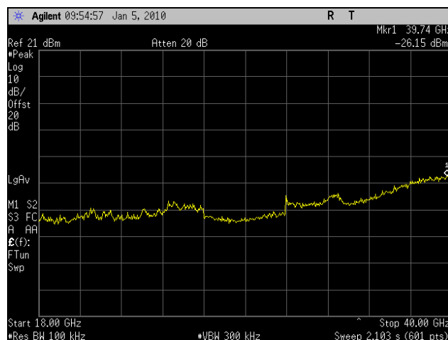
Plot 74. Conducted Spurious 5745MHz Low Channel 802.11n 20MHz Port 2 (18-40GHz)
