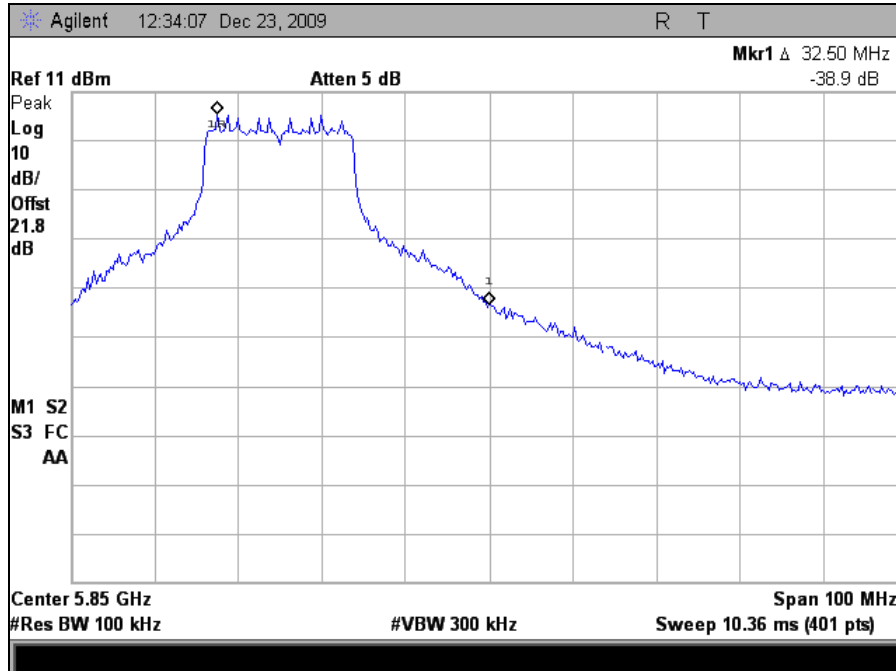
Plot 91. Conducted Band Edge 5825MHz High Channel 802.11n 20MHz Port 1
