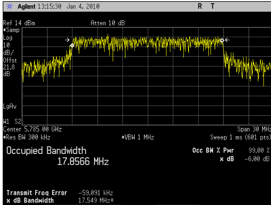
Plot 22. Occupied Bandwidth 5785MHz Mid Channel 802.11n 20MHz Port 2 (99%)
