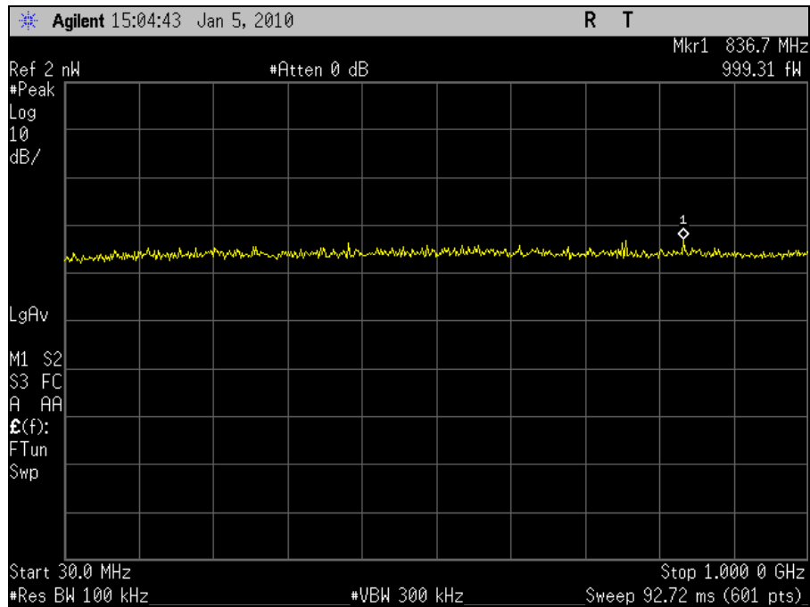
Plot 52. Conducted Receiver Spurious Emission, 30MHz – 1GHz, Port 2
