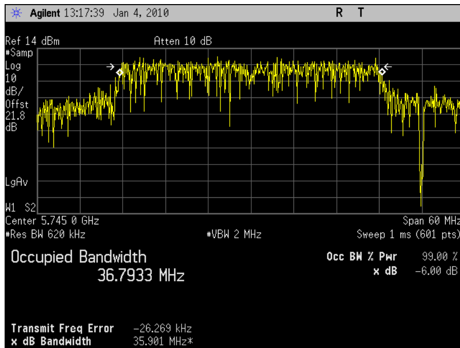
Plot 26. Occupied Bandwidth 5745MHz Low Channel 802.11n 40MHz Port 2 (99%)
