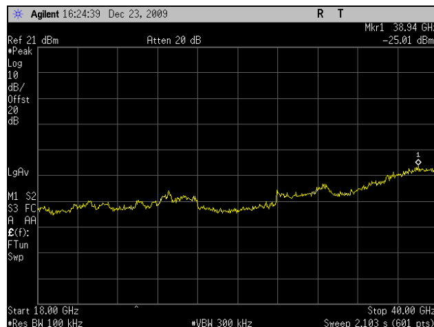
Plot 65. Conducted Spurious 5745MHz Low Channel 802.11n 40MHz Port 1 (18-40GHz)
