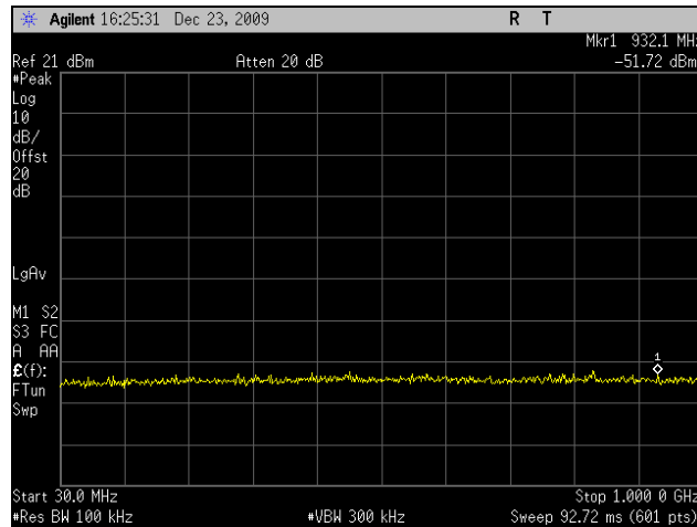
Plot 63. Conducted Spurious 5745MHz Low Channel 802.11n 40MHz Port 1 (30MHz-1GHz)
