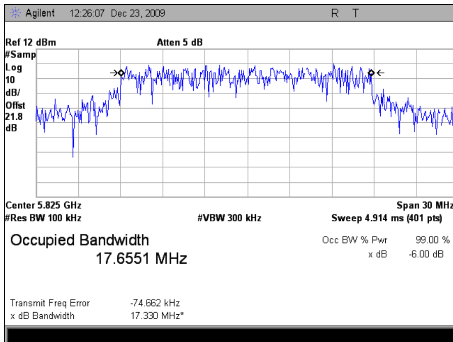
Plot 13. Occupied Bandwidth 5825MHz High Channel 802.11n 20MHz Port 1 (100kHz RBW)
