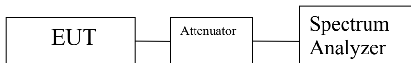
Figure 7. Block Diagram, Peak Power Spectral Density Test Setup
