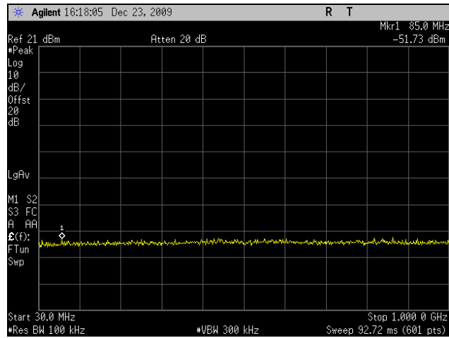
Plot 57. Conducted Spurious 5785MHz Mid Channel 802.11n 20MHz Port 1 (30MHz-1GHz)
