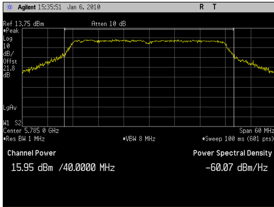
Plot 36. Peak Output Power 5785MHz Mid Channel 802.11n 40MHz Port 1
