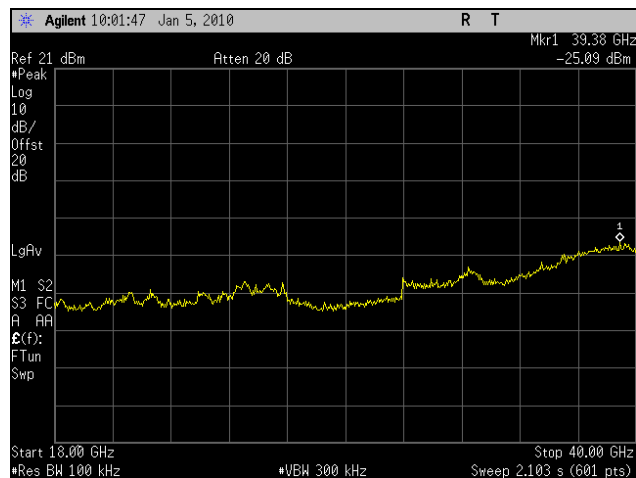
Plot 77. Conducted Spurious 5785MHz Mid Channel 802.11n 20MHz Port 2 (18-40GHz)
