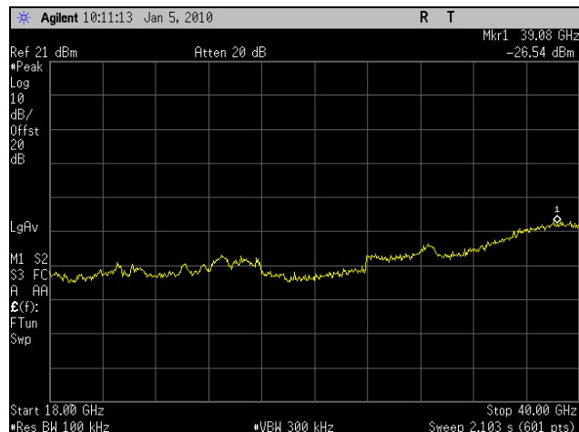
Plot 89. Conducted Spurious 5825MHz High Channel 802.11n 40MHz Port 2 (18-40GHz)
