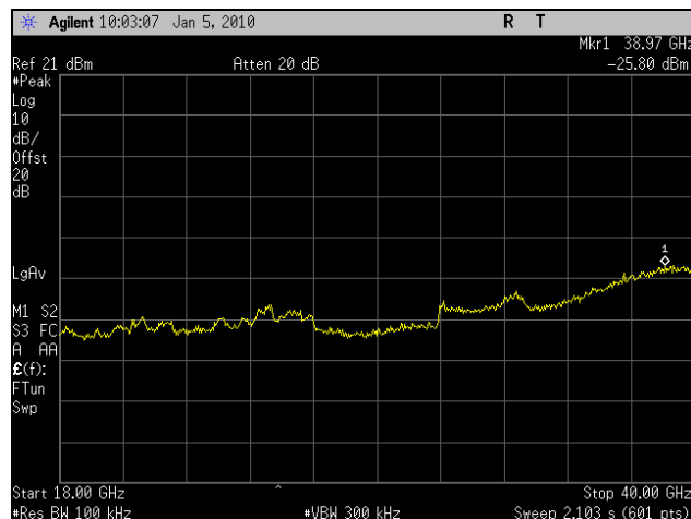
Plot 80. Conducted Spurious 5825MHz High Channel 802.11n 20MHz Port 2 (18-40GHz)
