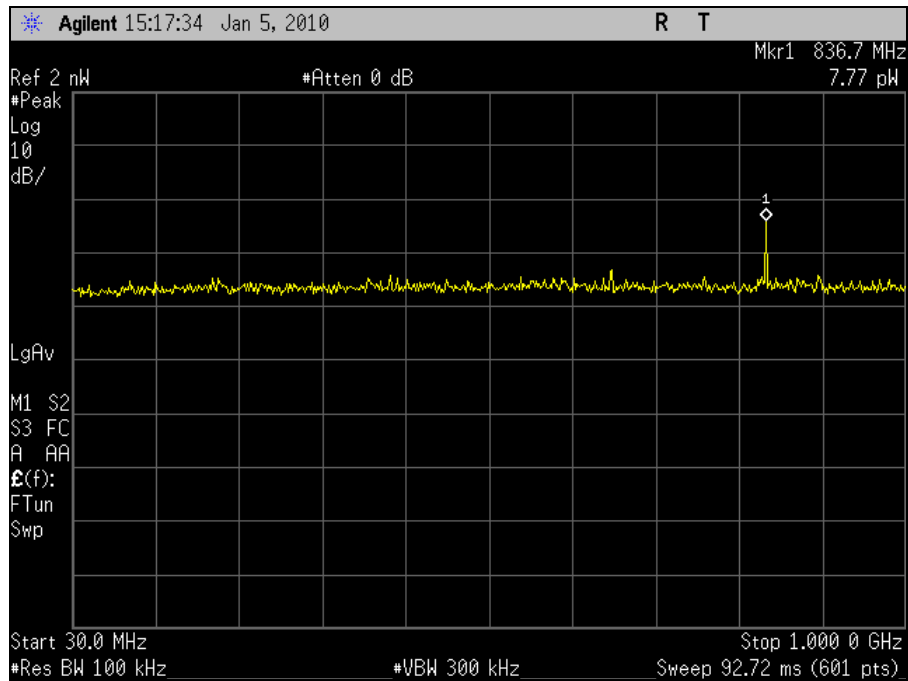
Plot 50. Conducted Receiver Spurious Emission, 30MHz – 1GHz, Port 1
