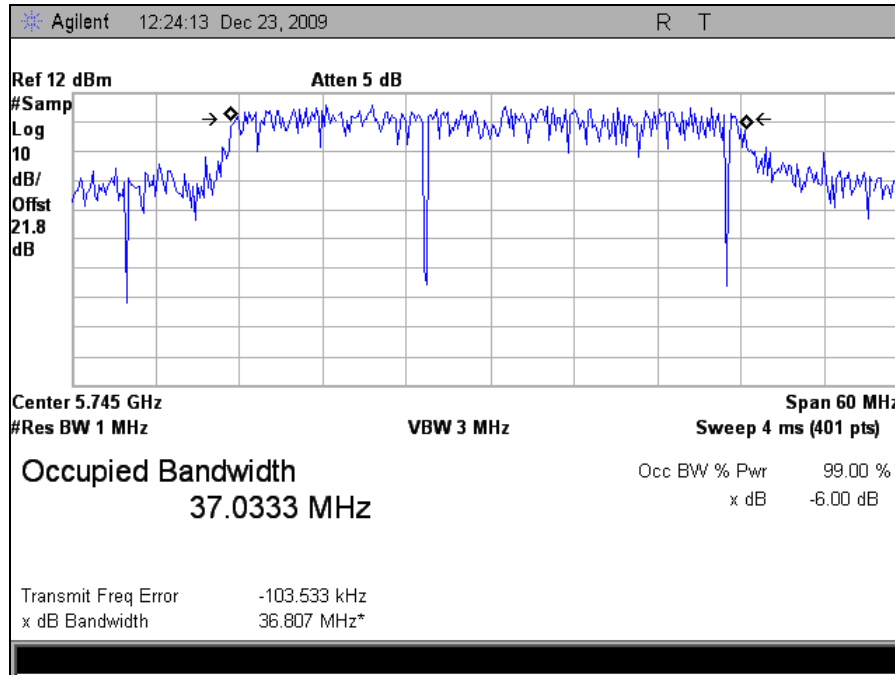
Plot 14. Occupied Bandwidth 5745MHz Low Channel 802.11n 40MHz Port 1 (99%)
