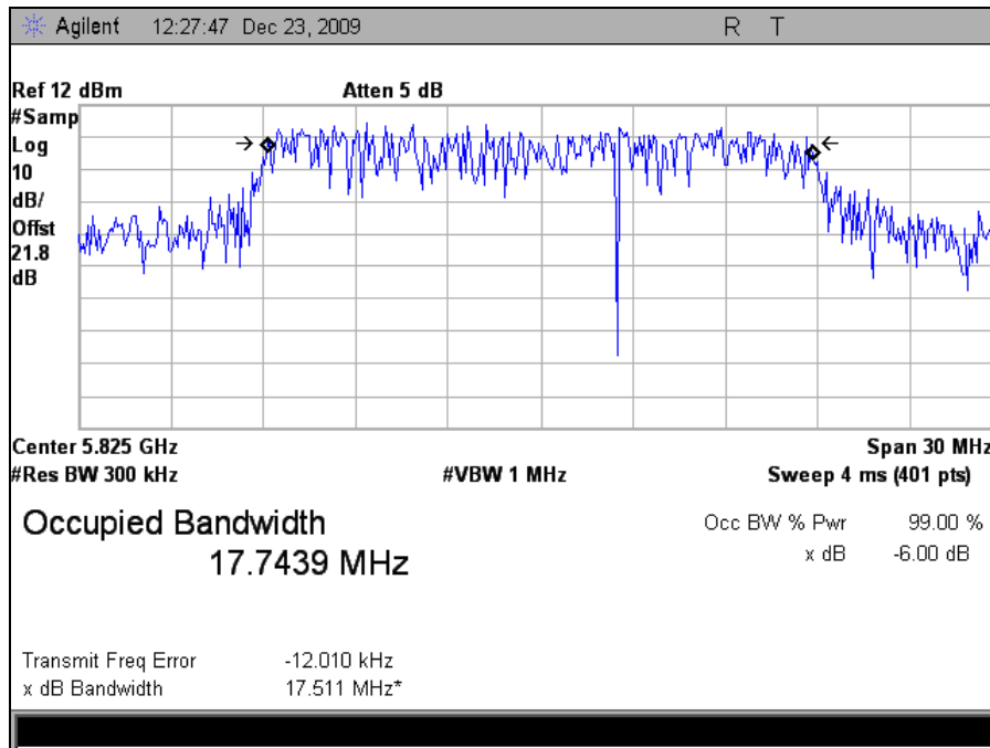
Plot 12. Occupied Bandwidth 5825MHz High Channel 802.11n 20MHz Port 1 (99%)
