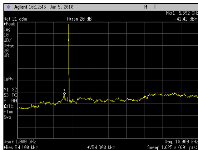
Plot 85. Conducted Spurious 5785MHz Mid Channel 802.11n 40MHz Port 2 (1-18GHz)
