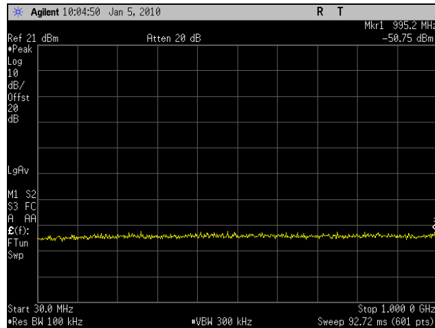
Plot 78. Conducted Spurious 5825MHz High Channel 802.11n 20MHz Port 2 (30MHz-1GHz)
