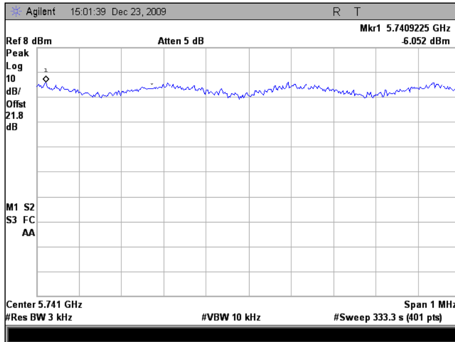
Plot 98. Power Spectral Density 5745MHz Low Channel 802.11n 20MHz Port 1
