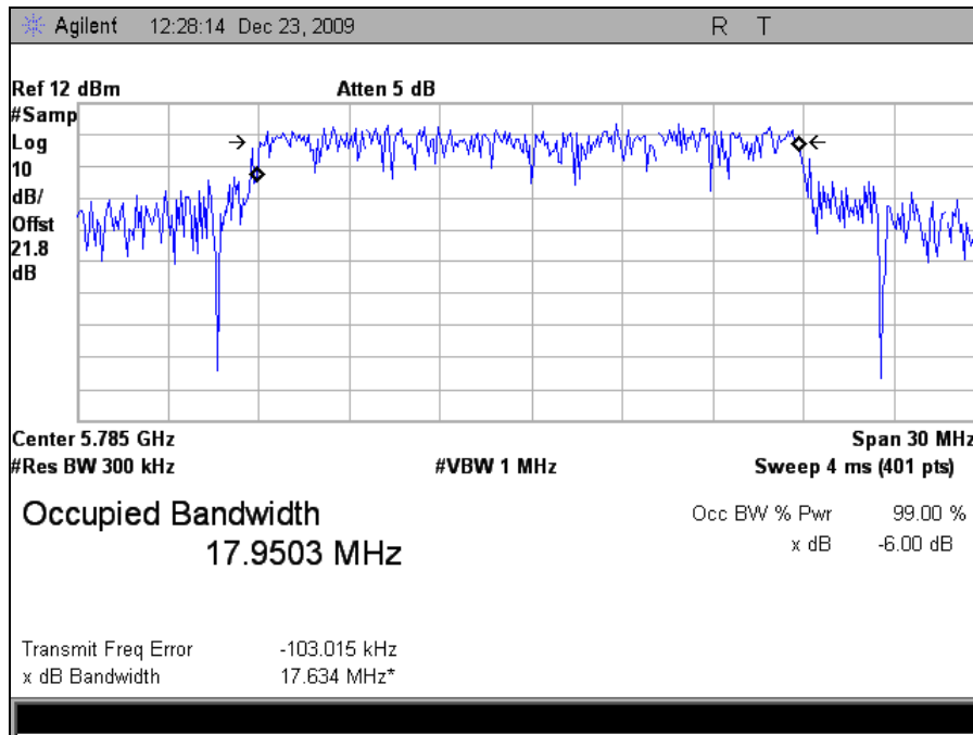
Plot 10. Occupied Bandwidth 5785MHz Mid Channel 802.11n 20MHz Port 1 (99%)
