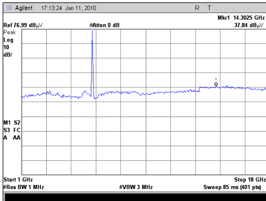
Plot 49. Radiated Spurious Emissions, 802.11n 40MHz Mode High Channel
