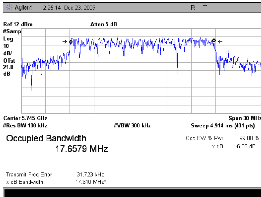
Plot 9. Occupied Bandwidth 5745MHz Low Channel 802.11n 20MHz Port 1 (100kHz RBW)
