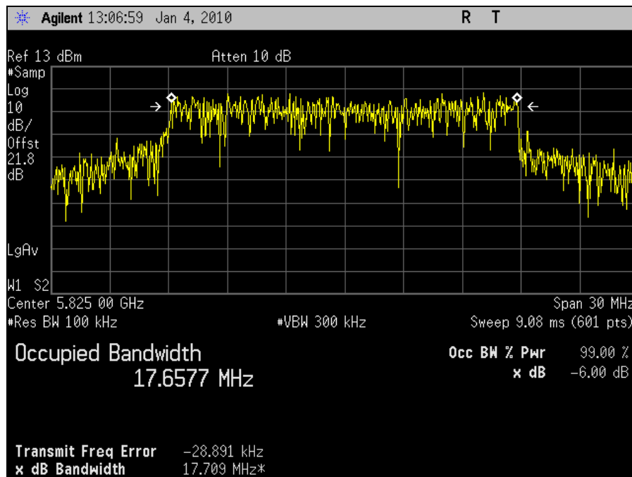
Plot 25. Occupied Bandwidth 5825MHz High Channel 802.11n 20MHz Port 2 (100kHz)
