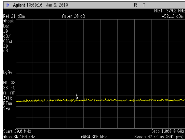
Plot 75. Conducted Spurious 5785MHz Mid Channel 802.11n 20MHz Port 2 (30MHz-1GHz)
