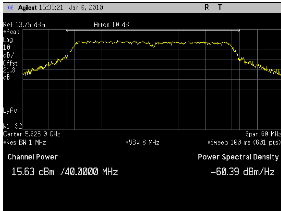
Plot 37. Peak Output Power 5825MHz High Channel 802.11n 40MHz Port 1
