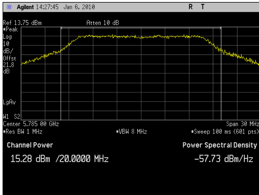
Plot 33. Peak Output Power 5785MHz Mid Channel 802.11n 20MHz Port 1
