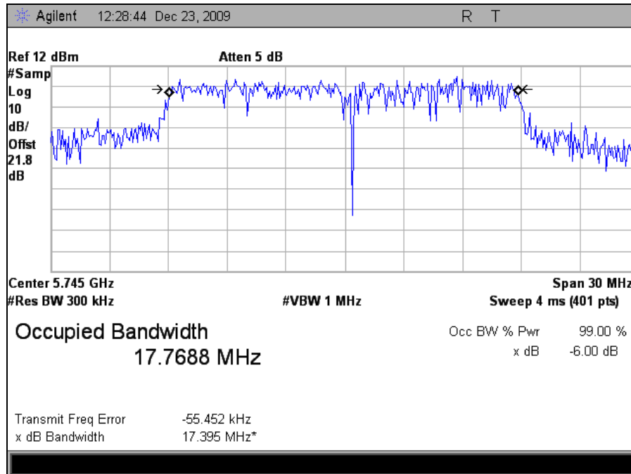
Plot 8. Occupied Bandwidth 5745MHz Low Channel 802.11n 20MHz Port 1 (99%)
