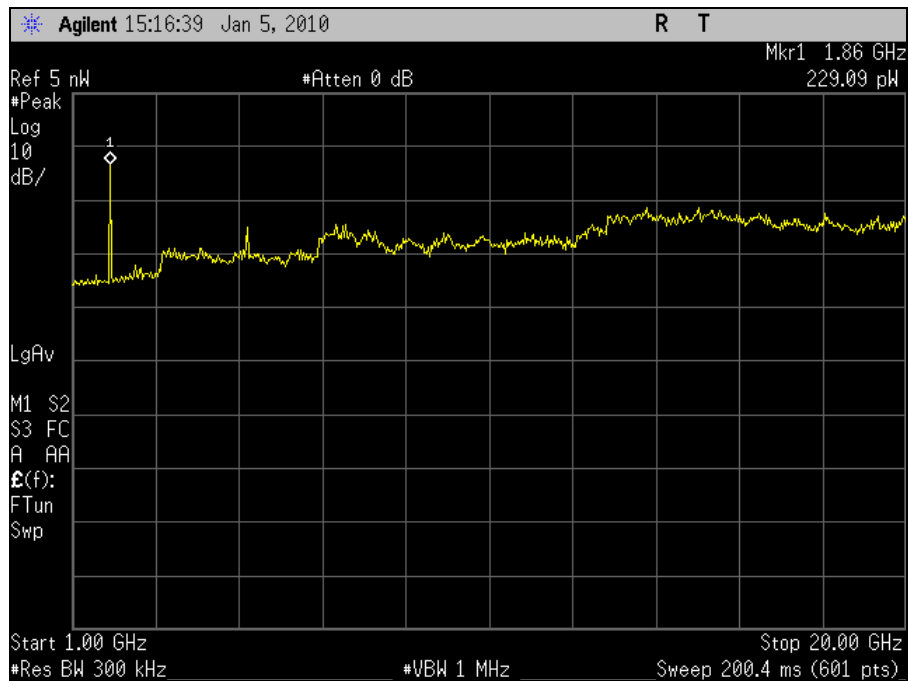
Plot 51. Conducted Receiver Spurious Emission, 1 GHz – 20 GHz, Port 1
