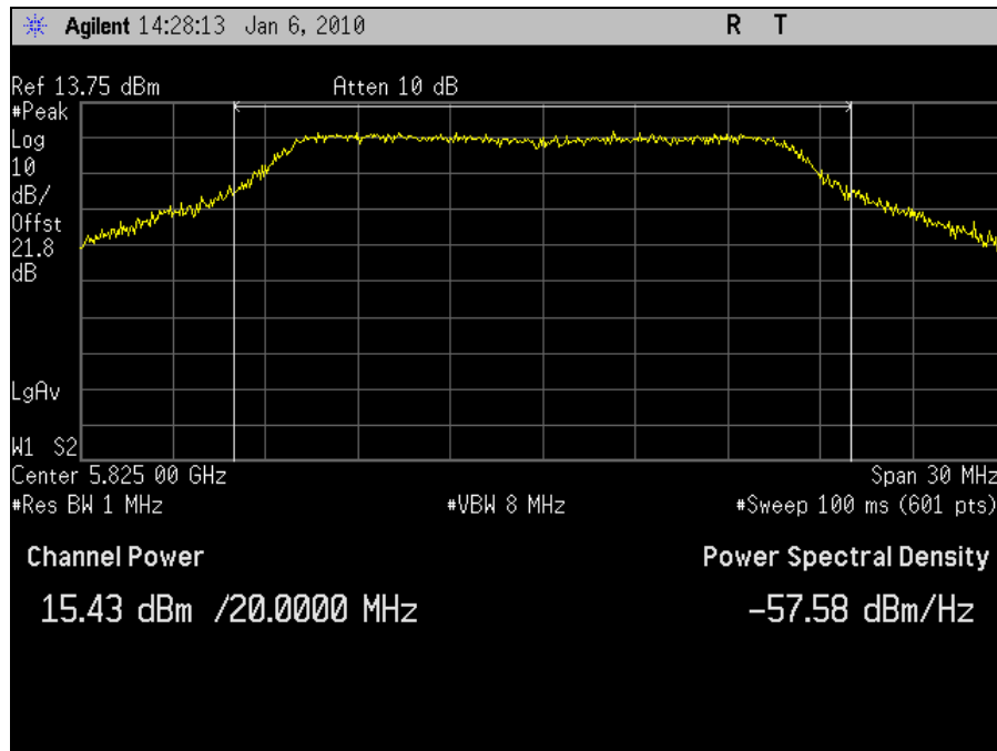
Plot 34. Peak Output Power 5825MHz High Channel 802.11n 20MHz Port 1
