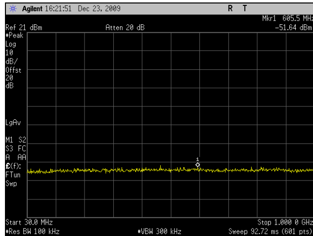
Plot 69. Conducted Spurious 5825MHz High Channel 802.11n 40MHz Port 1 (30MHz-1GHz)
