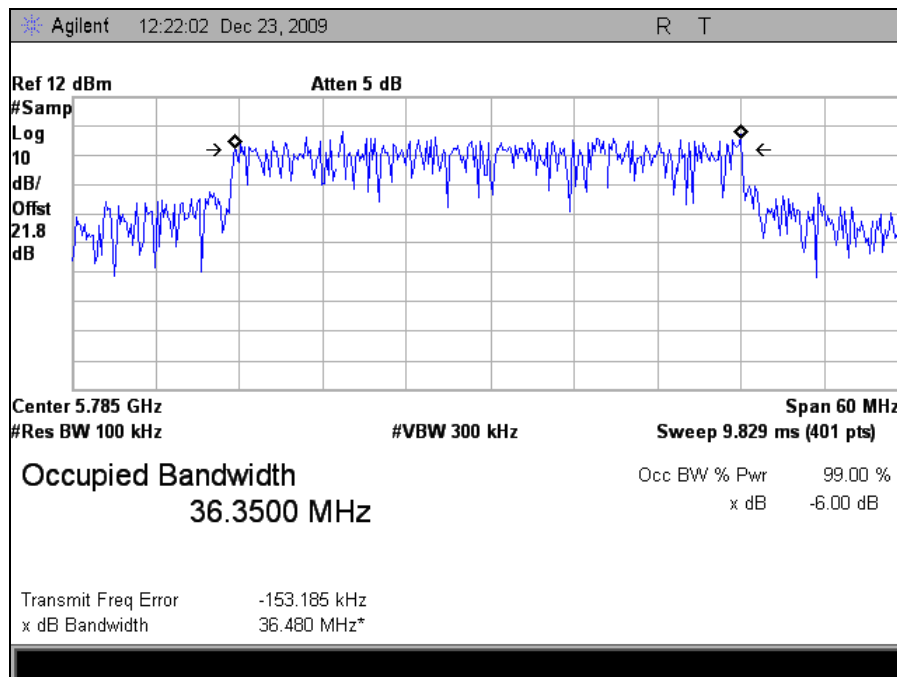
Plot 17. Occupied Bandwidth 5785MHz Mid Channel 802.11n 40MHz Port 1 (100kHz RBW)
