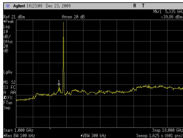
Plot 67. Conducted Spurious 5785MHz Mid Channel 802.11n 40MHz Port 1 (1-18GHz)
