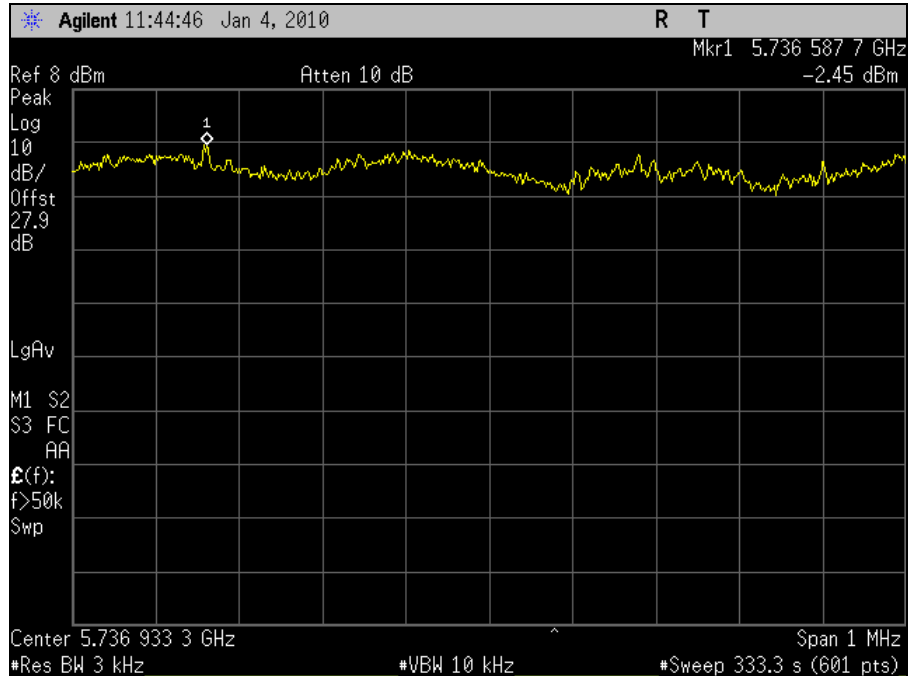
Plot 113. Power Spectral Density 5745MHz Low Channel 802.11n 40MHz Combined
