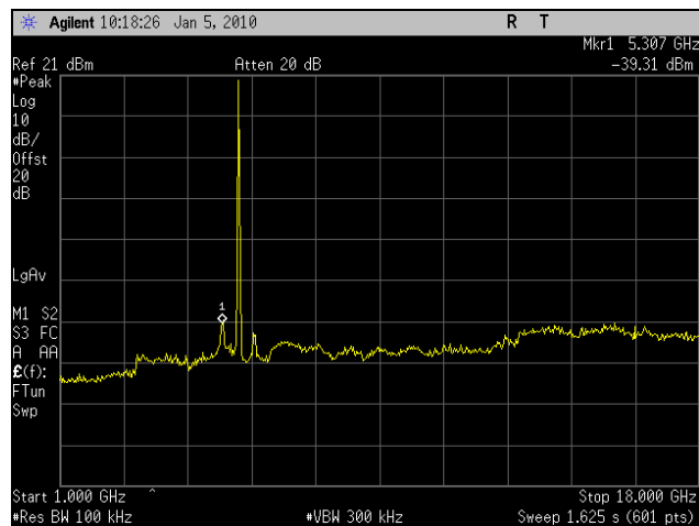
Plot 82. Conducted Spurious 5745MHz Low Channel 802.11n 40MHz Port 2 (1-18GHz)
