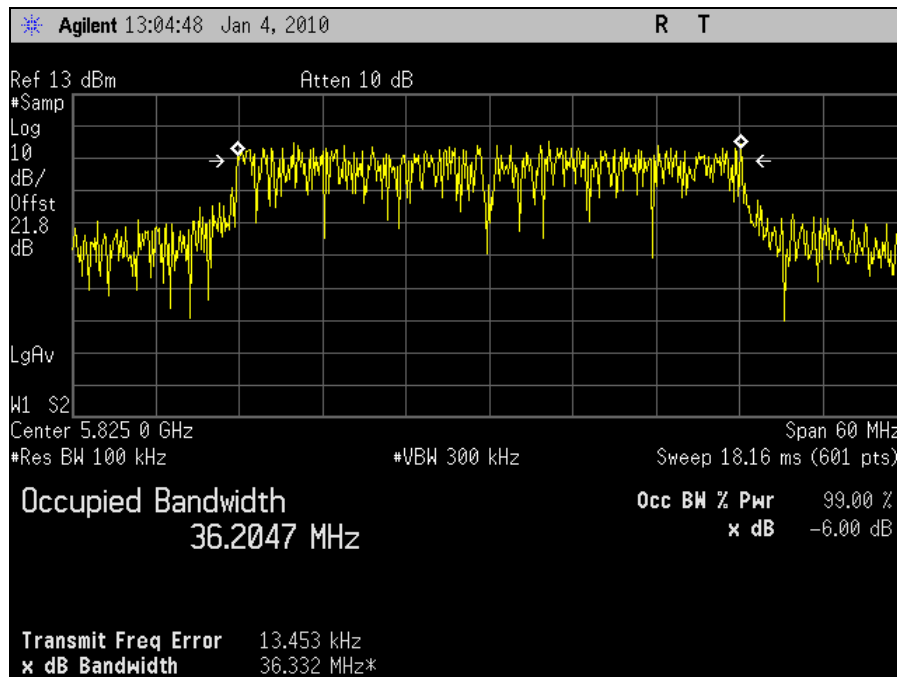
Plot 31. Occupied Bandwidth 5825MHz High Channel 802.11n 40MHz Port 2 (100kHz)
