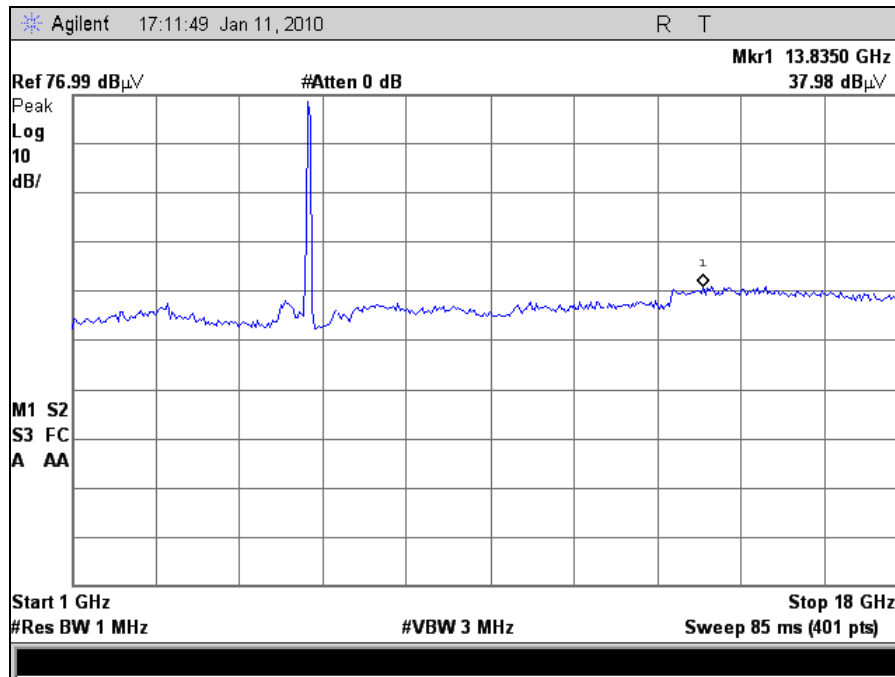
Plot 48. Radiated Spurious Emissions, 802.11n 40MHz Mode Mid Channel
