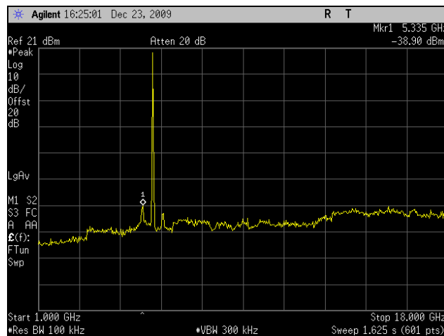
Plot 64. Conducted Spurious 5745MHz Low Channel 802.11n 40MHz Port 1 (1-18GHz)
