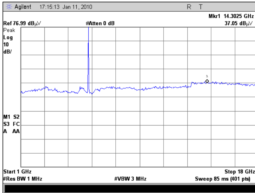
Plot 46. Radiated Spurious Emissions, 802.11n 20MHz Mode High Channel
