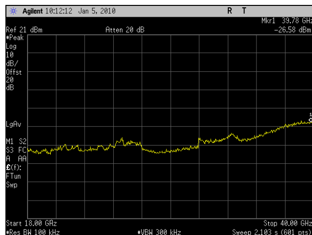
Plot 86. Conducted Spurious 5785MHz Mid Channel 802.11n 40MHz Port 2 (18-40GHz)
