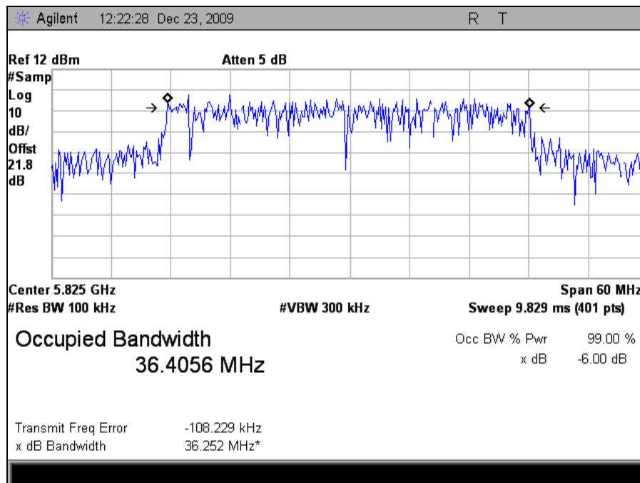
Plot 19. Occupied Bandwidth 5825MHz High Channel 802.11n 40MHz Port 1 (100kHz RBW)
