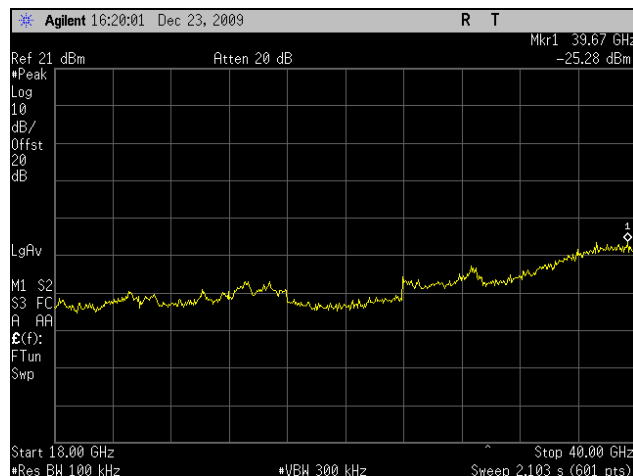
Plot 62. Conducted Spurious 5825MHz High Channel 802.11n 20MHz Port 1 (18-40GHz)
