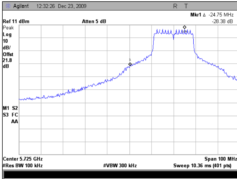
Plot 90. Conducted Band Edge 5745MHz Low Channel 802.11n 20MHz Port 1
