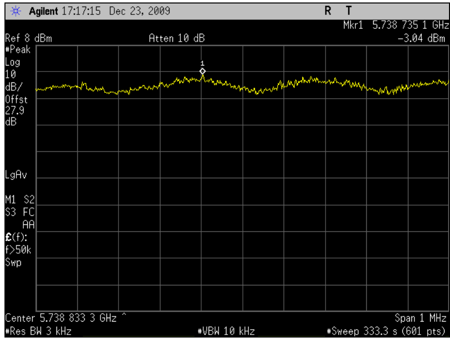
Plot 110. Power Spectral Density 5745MHz Low Channel 802.11n 20MHz Combined
