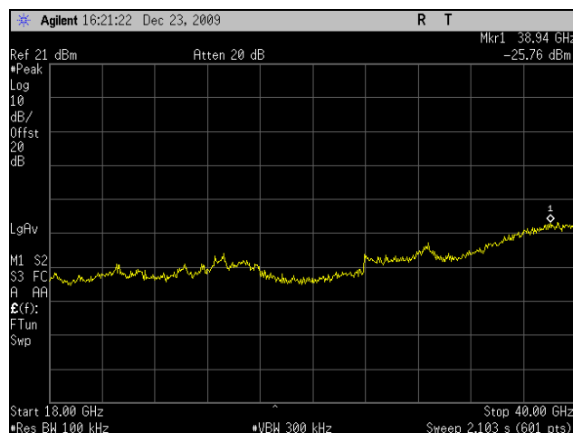
Plot 71. Conducted Spurious 5825MHz High Channel 802.11n 40MHz Port 1 (18-40GHz)
