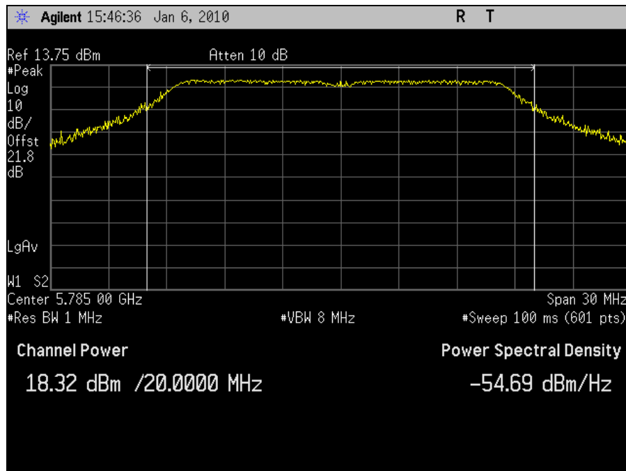
Plot 39. Peak Output Power 5785MHz Mid Channel 802.11n 20MHz Port 2
