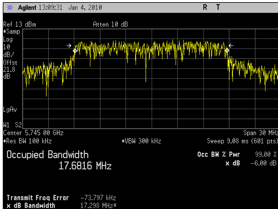
Plot 21. Occupied Bandwidth 5745MHz Low Channel 802.11n 20MHz Port 2 (100kHz)
