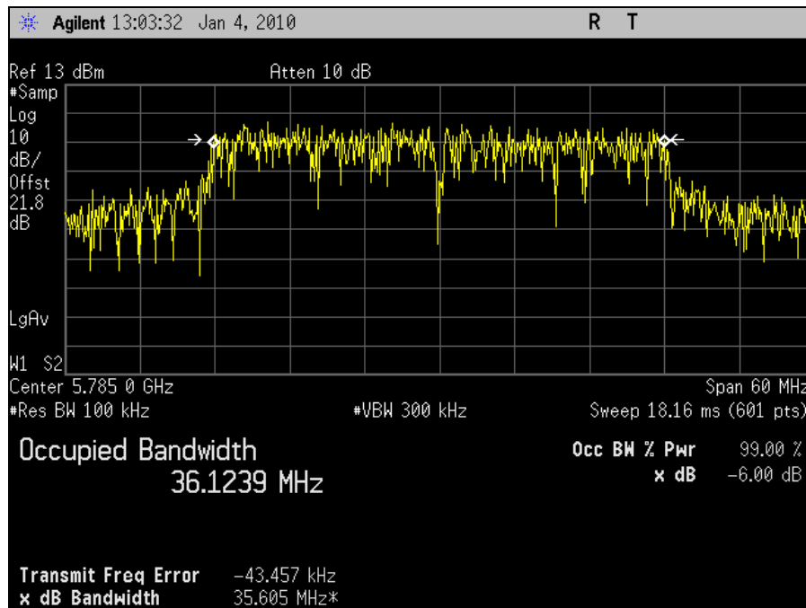
Plot 29. Occupied Bandwidth 5785MHz Mid Channel 802.11n 40MHz Port 2 (100kHz)
