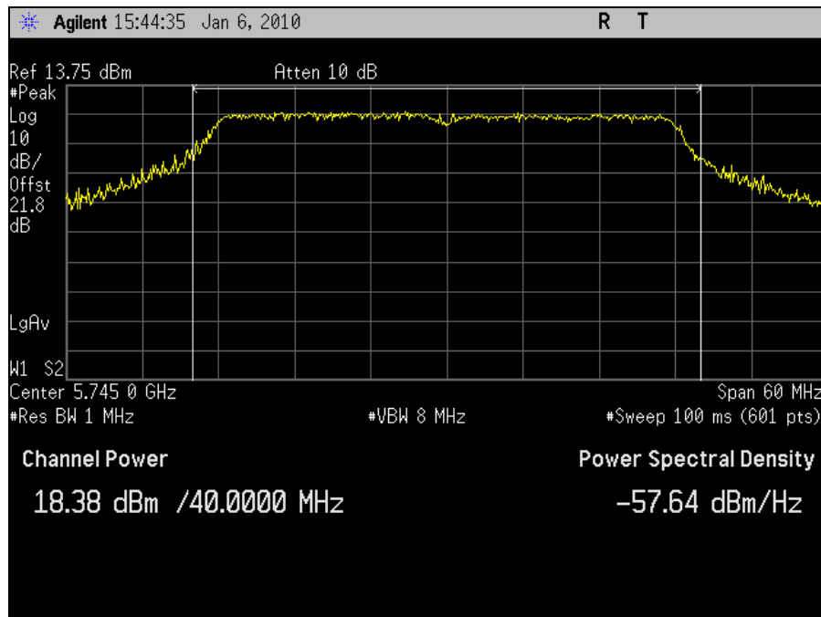
Plot 41. Peak Output Power 5745MHz Low Channel 802.11n 40MHz Port 2
