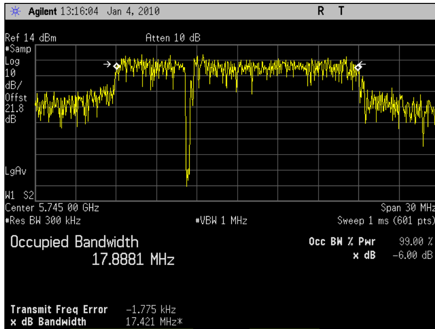
Plot 20. Occupied Bandwidth 5745MHz Low Channel 802.11n 20MHz Port 2 (99%)
