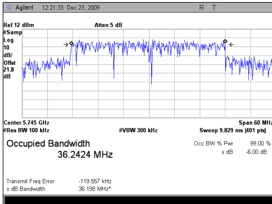
Plot 15. Occupied Bandwidth 5745MHz Low Channel 802.11n 40MHz Port 1 (100kHz RBW)
