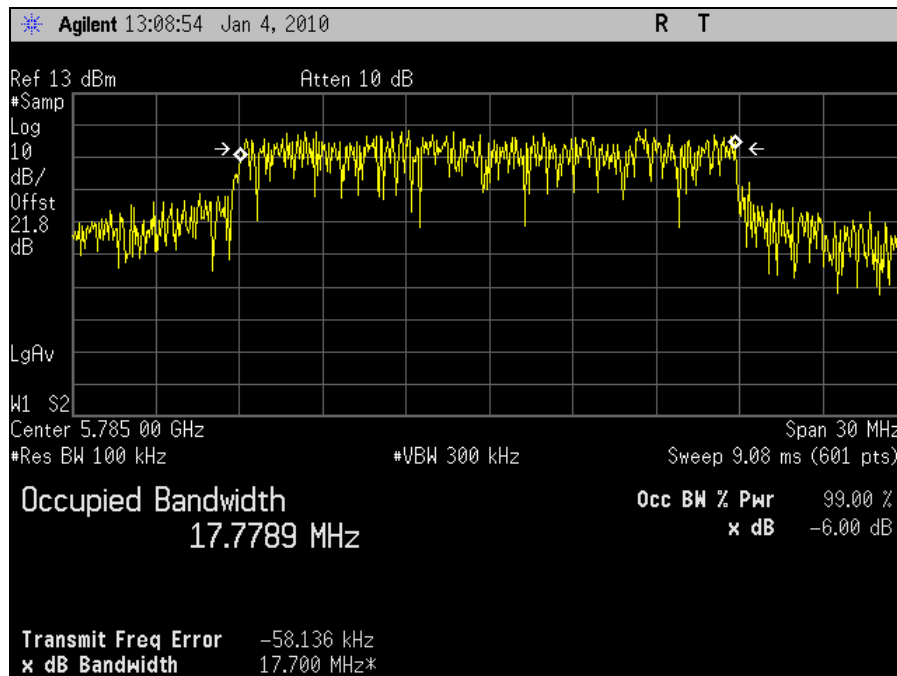
Plot 23. Occupied Bandwidth 5785MHz Mid Channel 802.11n 20MHz Port 2 (100kHz)
