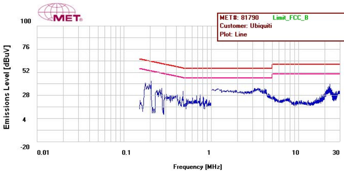
Plot 6. 15.207 Conducted Emission, Phase Line Plot
