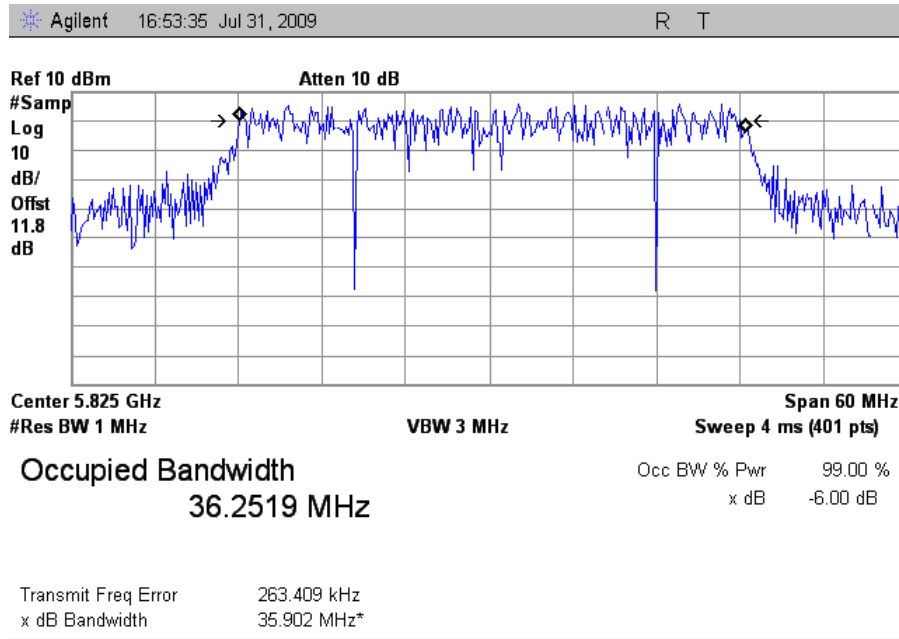
Plot 19. Occupied Band Width, High Channel, HT40 (99%)
