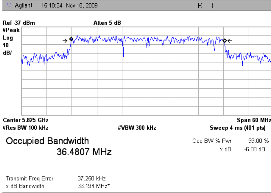
Plot 18. Occupied Band Width, High Channel, HT40
