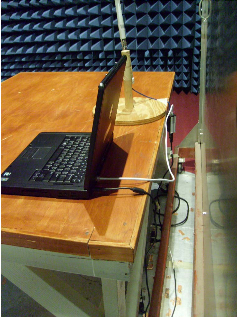
Photograph 5. Conducted Emissions, 15.207, Test Setup (Side View)
