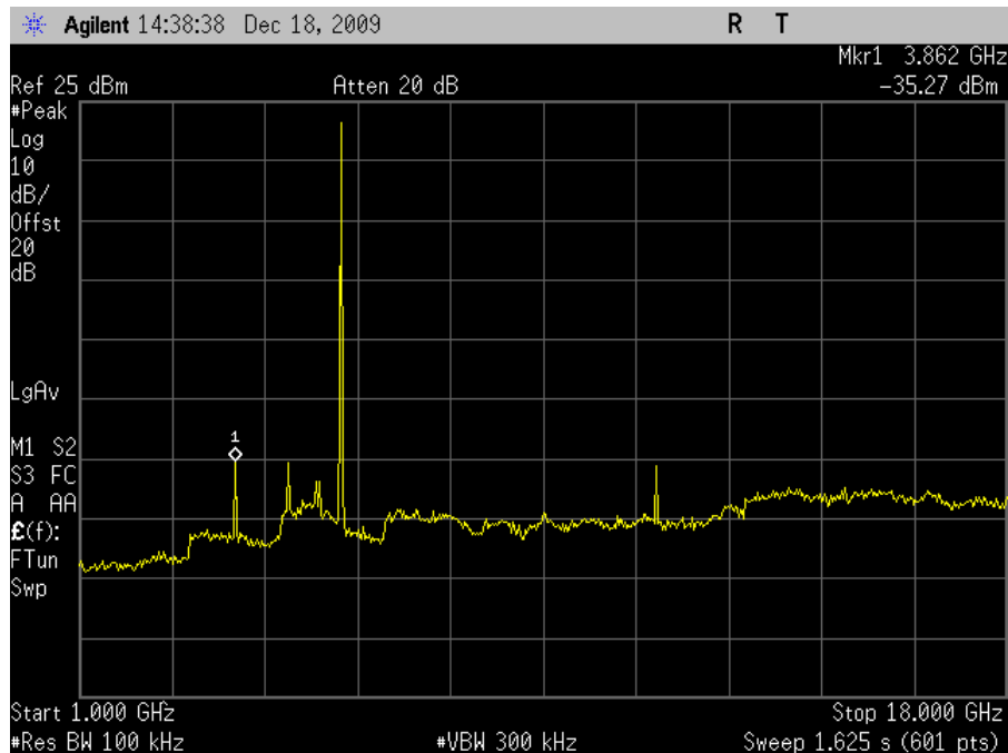
Plot 51. Conducted Spurious 5785MHz Mid Channel 802.11a 1-18GHz
