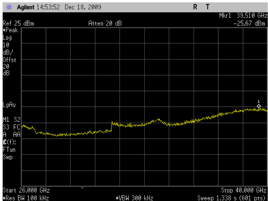
Plot 65. Conducted Spurious 5785MHz Mid Channel 802.11n 20MHz 26-40GHz
