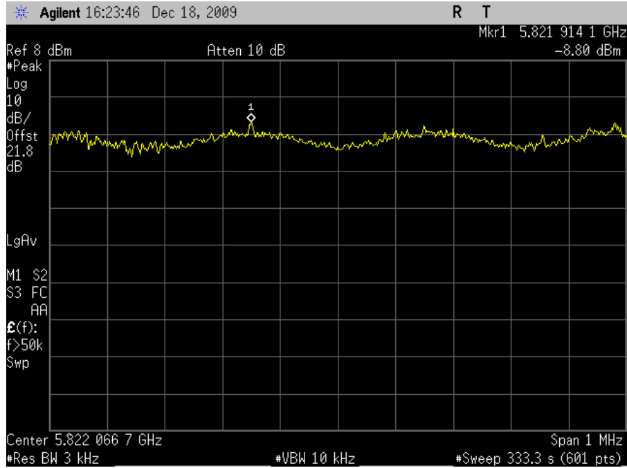
Plot 96. Power Spectral Density 5825MHz High Channel 802.11n 40MHz
