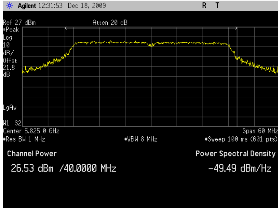
Plot 34. Peak Output Power, 802.11n 40MHz Mode High Channel
