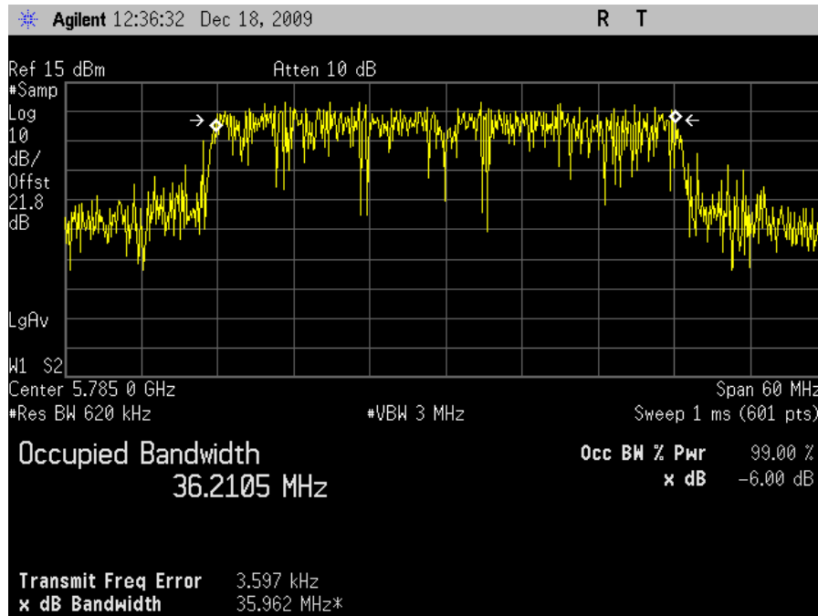
Plot 24. Occupied Band Width, 802.11n 40MHz Mode Mid Channel, 99 % OBW
