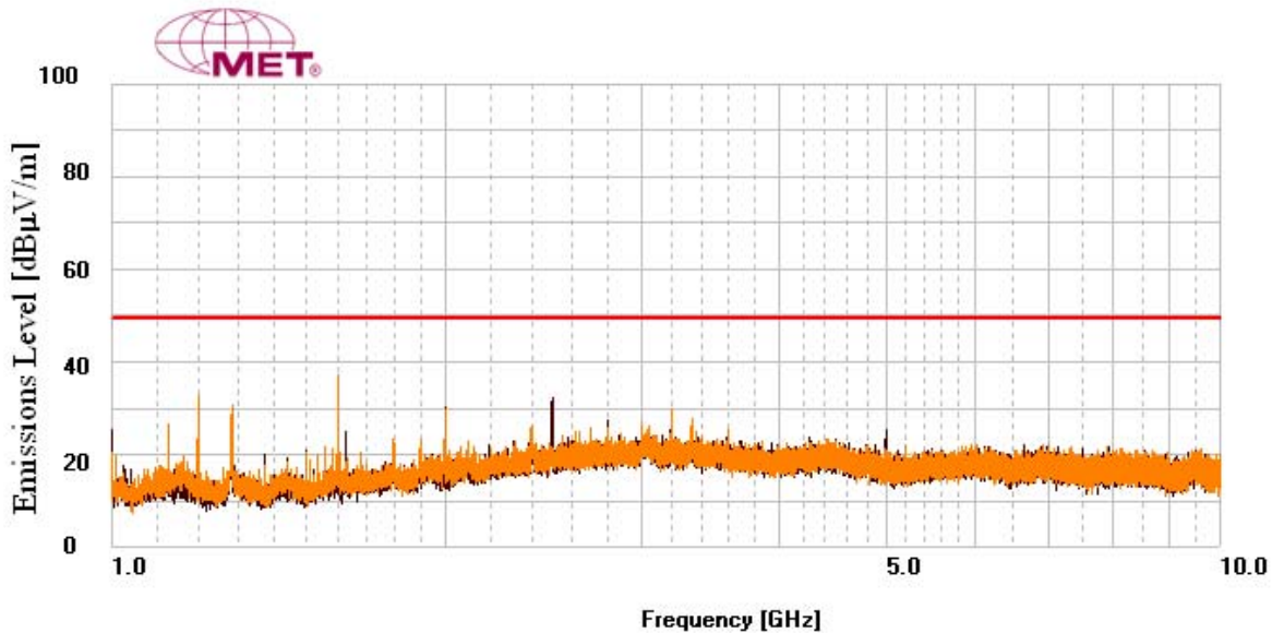
Plot 4. Radiated Emissions, above 1GHz FCC Limits
