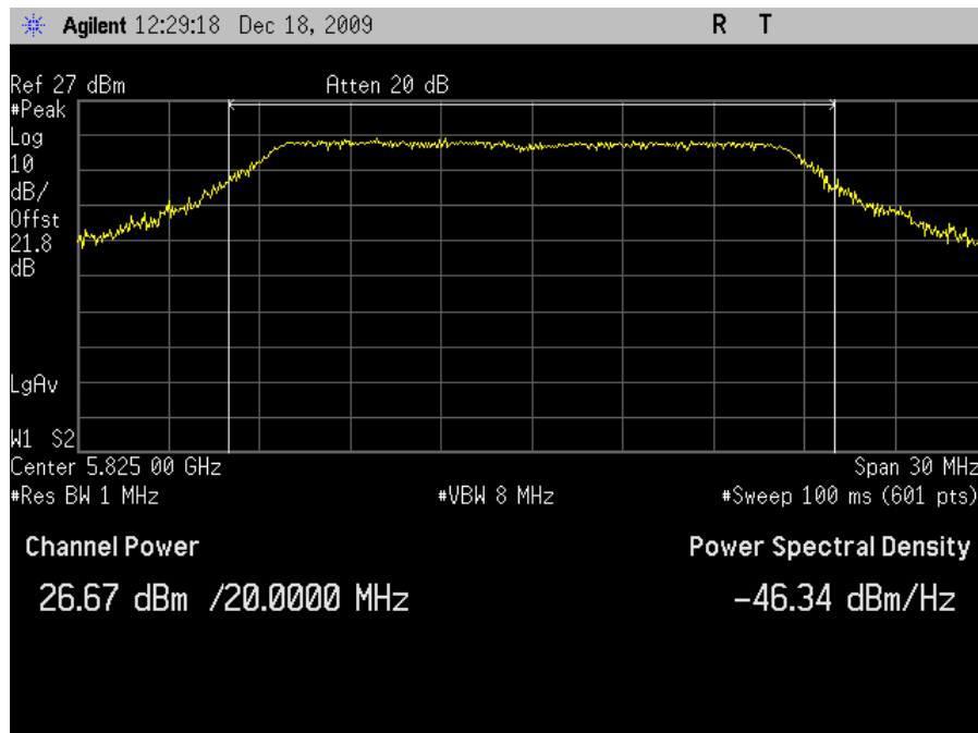
Plot 31. Peak Output Power, 802.11n 20MHz Mode High Channel
