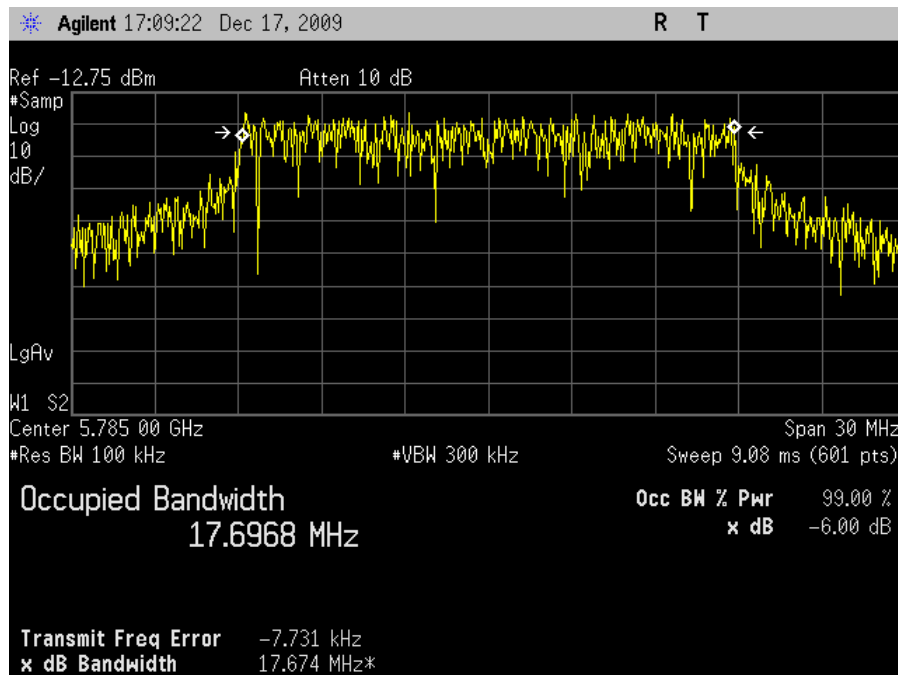
Plot 15. Occupied Band Width, 802.11n 20MHz Mode Mid Channel, FCC, 6 dB
