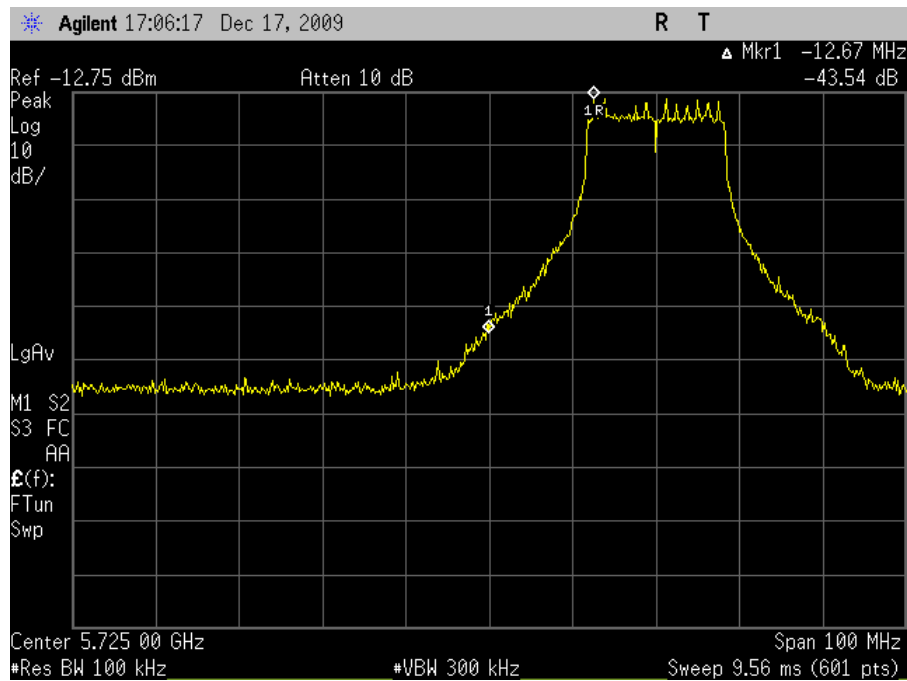
Plot 82. Conducted Band Edge 5745MHz Low Channel 802.11a
