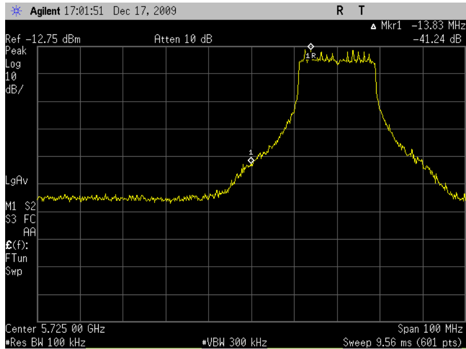
Plot 84. Conducted Band Edge 5745MHz Low Channel 802.11n 20MHz
