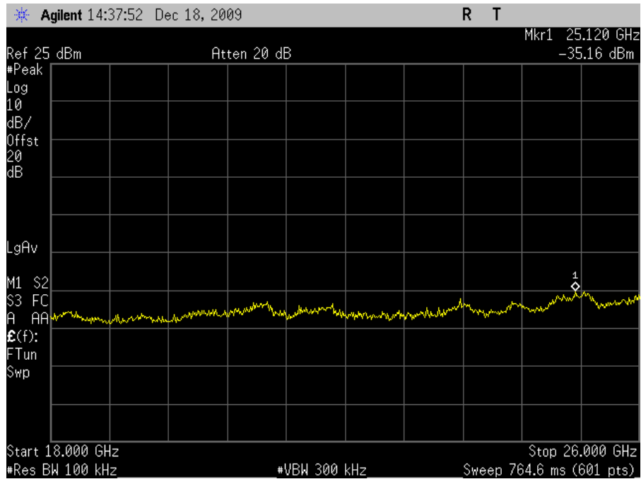
Plot 52. Conducted Spurious 5785MHz Mid Channel 802.11a 18-26GHz
