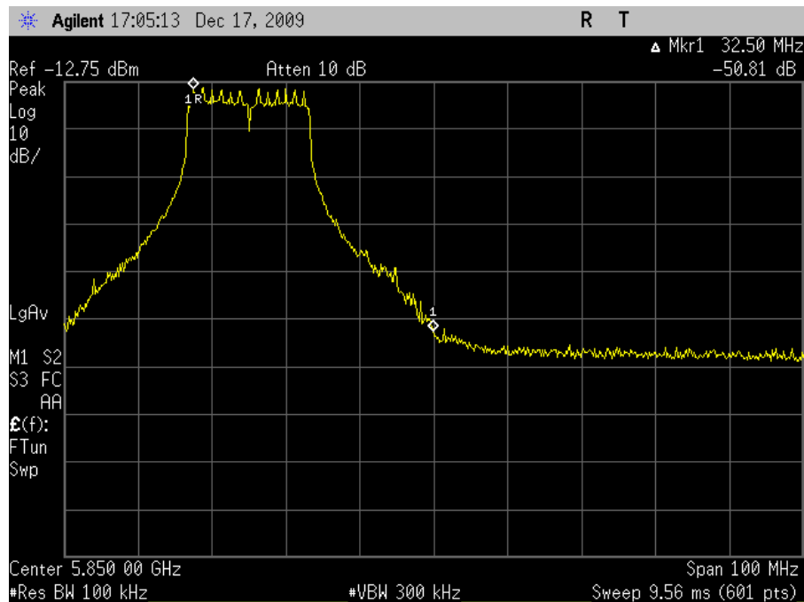
Plot 83. Conducted Band Edge 5825MHz High Channel 802.11a
