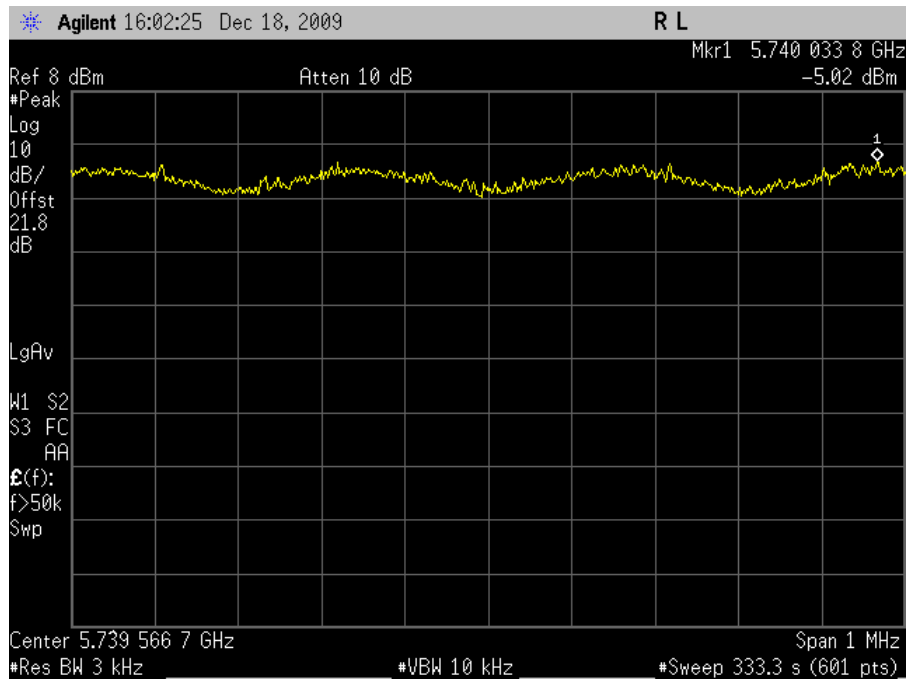
Plot 91. Power Spectral Density 5745MHz Low Channel 802.11n 20MHz
