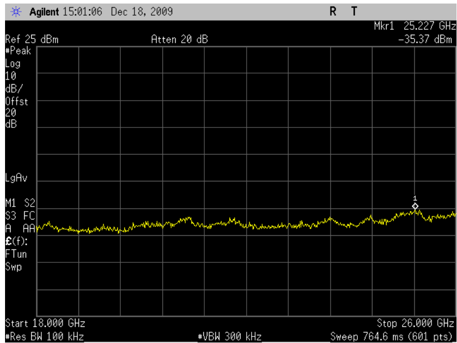
Plot 72. Conducted Spurious 5745MHz Low Channel 802.11n 40MHz 18-26GHz
