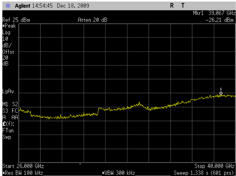
Plot 61. Conducted Spurious 5745MHz Low Channel 802.11n 20MHz 26-40GHz
