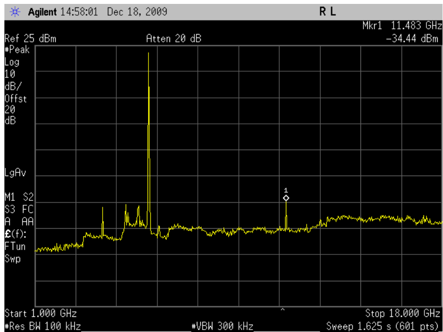
Plot 71. Conducted Spurious 5745MHz Low Channel 802.11n 40MHz 1-18GHz
