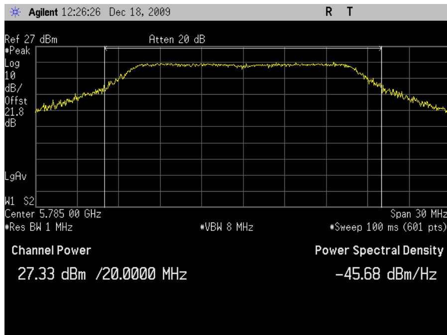
Plot 27. Peak Output Power, 802.11a Mode Mid Channel
