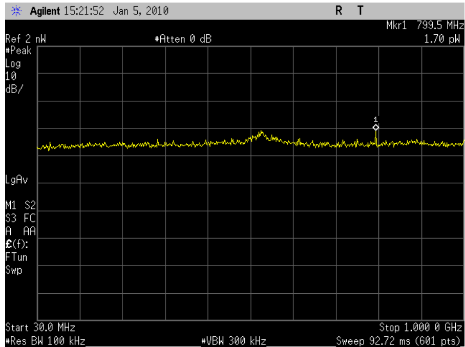
Plot 44. Conducted Receiver Spurious Emission, 30MHz – 1GHz
