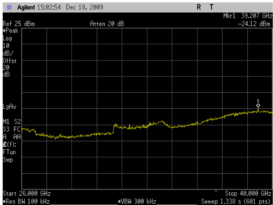
Plot 77. Conducted Spurious 5785MHz Mid Channel 802.11n 40MHz 26-40GHz
