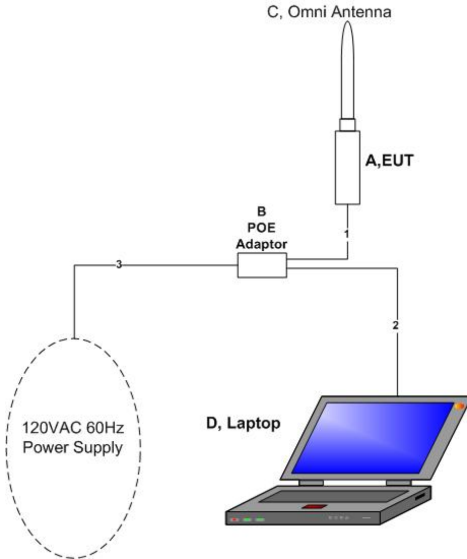
Figure 1. Block Diagram of Test Configuration
