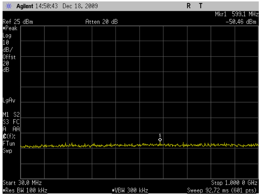
Plot 66. Conducted Spurious 5825MHz High Channel 802.11n 20MHz 30MHz-1GHz
