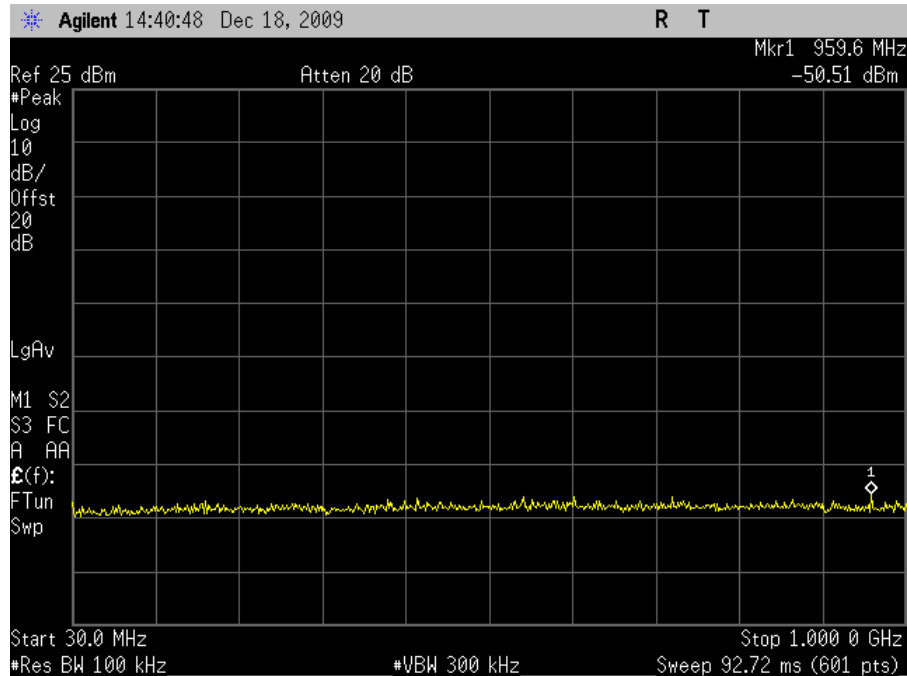
Plot 54. Conducted Spurious 5825MHz High Channel 802.11a 30MHz-1GHz
