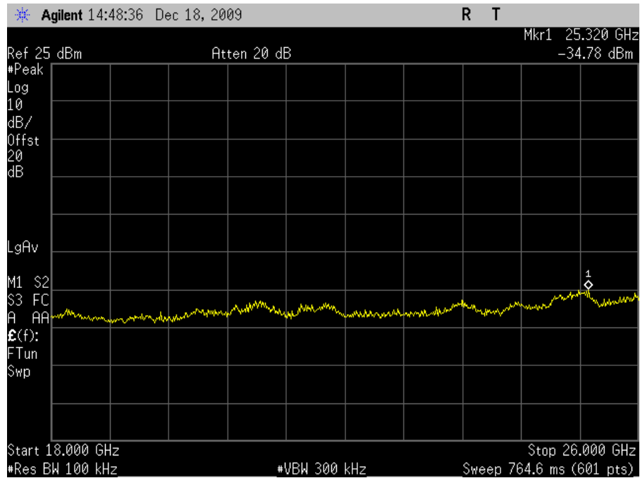
Plot 68. Conducted Spurious 5825MHz High Channel 802.11n 20MHz 18-26GHz
