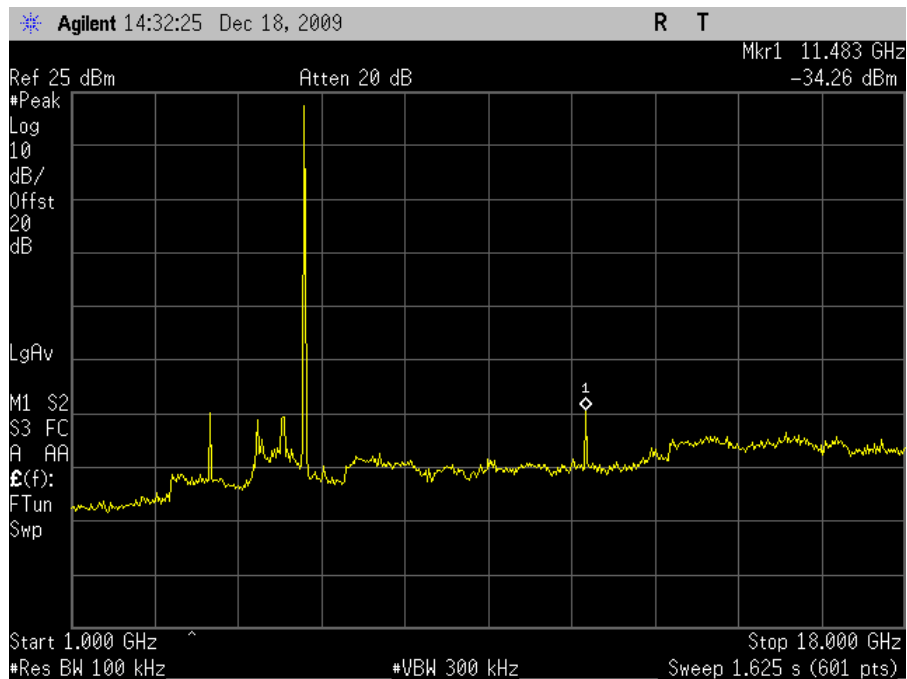
Plot 47. Conducted Spurious 5745MHz Low Channel 802.11a 1-18GHz
