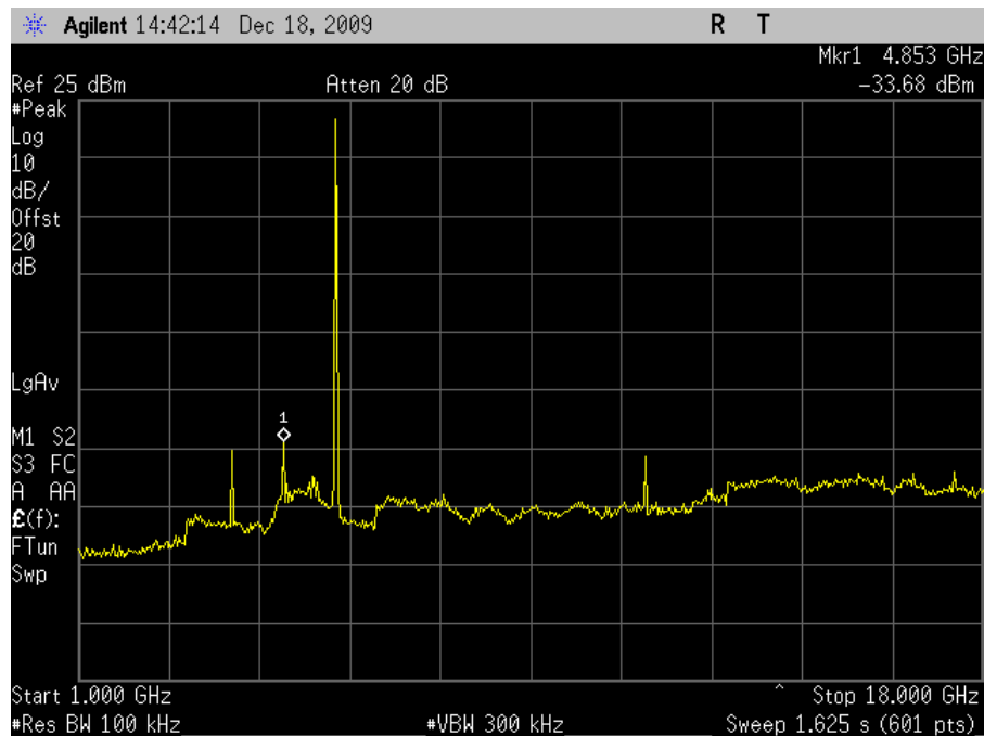
Plot 55. Conducted Spurious 5825MHz High Channel 802.11a 1-18GHz
