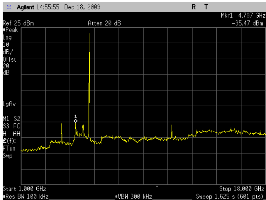
Plot 59. Conducted Spurious 5745MHz Low Channel 802.11n 20MHz 1-18GHz
