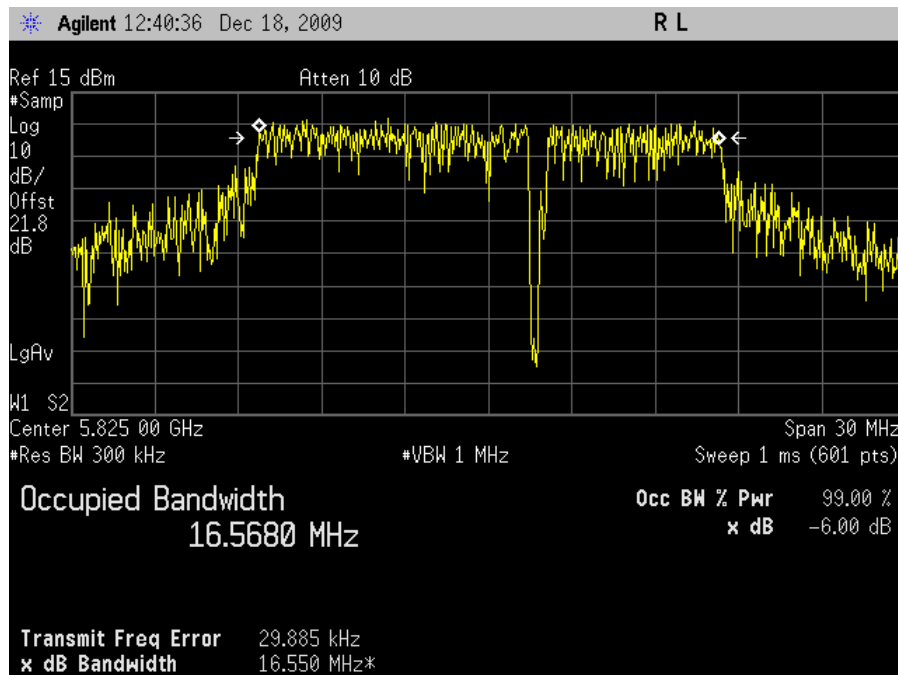
Plot 13. Occupied Band Width, 802.11a Mode High Channel, 99 % OBW
