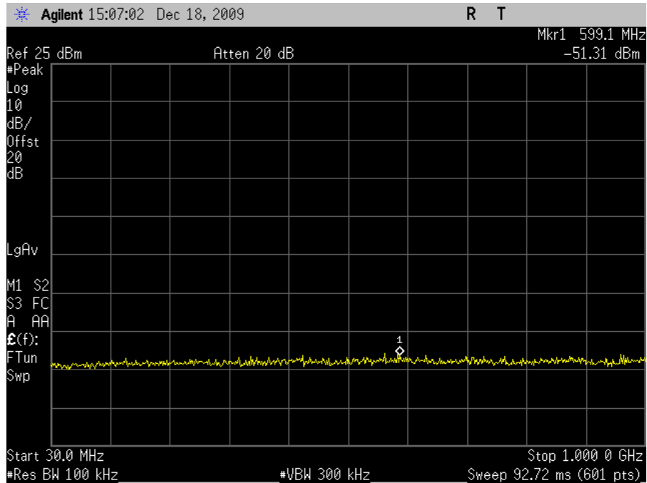
Plot 78. Conducted Spurious 5825MHz High Channel 802.11n 40MHz 30MHz-1GHz
