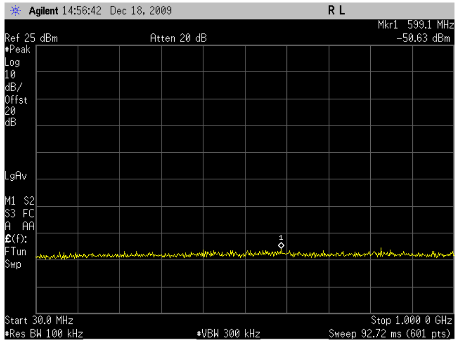
Plot 58. Conducted Spurious 5745MHz Low Channel 802.11n 20MHz 30MHz-1GHz
