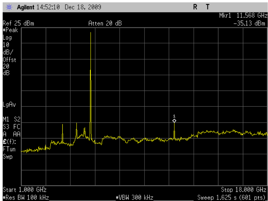
Plot 63. Conducted Spurious 5785MHz Mid Channel 802.11n 20MHz 1-18GHz
