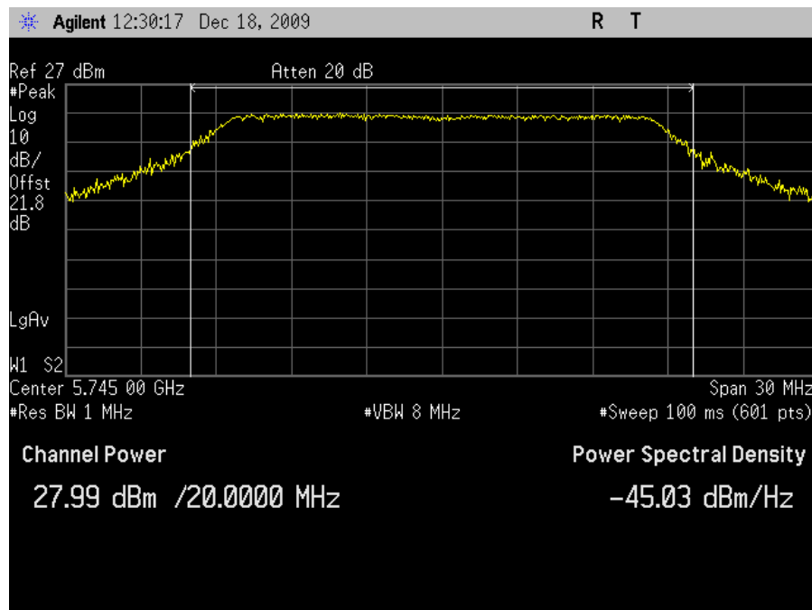
Plot 29. Peak Output Power, 802.11n 20MHz Mode Low Channel
