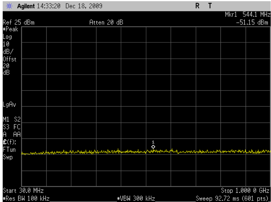
Plot 46. Conducted Spurious 5745MHz Low Channel 802.11a 30MHz-1GHz
