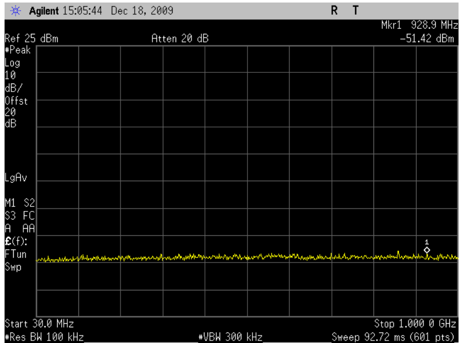
Plot 74. Conducted Spurious 5785MHz Mid Channel 802.11n 40MHz 30MHz-1GHz
