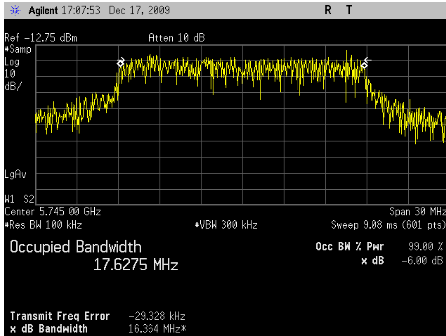
Plot 14. Occupied Band Width, 802.11n 20MHz Mode Low Channel, FCC, 6 dB
