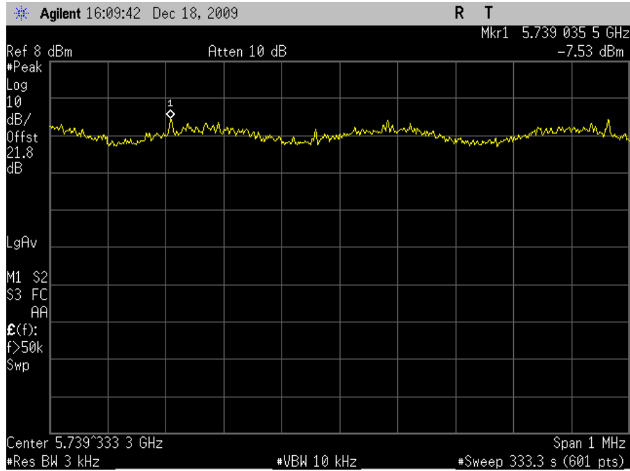
Plot 94. Power Spectral Density 5745MHz Low Channel 802.11n 40MHz
