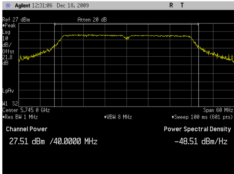
Plot 32. Peak Output Power, 802.11n 40MHz Mode Low Channel
