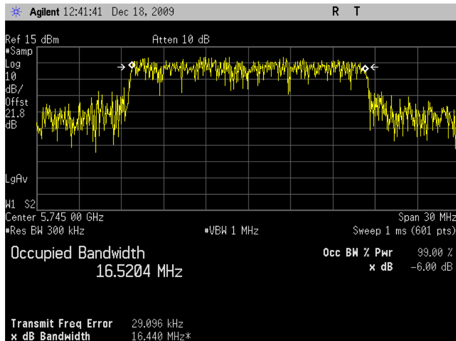
Plot 11. Occupied Band Width, 802.11a Mode Low Channel, 99 % OBW
