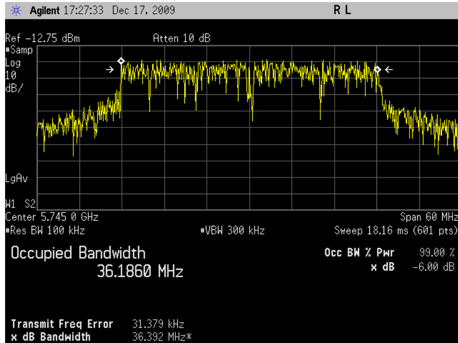
Plot 20. Occupied Band Width, 802.11n 40MHz Mode Low Channel, FCC, 6 dB
