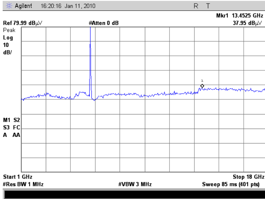
Plot 35. Radiated Spurious 5745MHz Low Channel 802.11a (1-18GHz)
