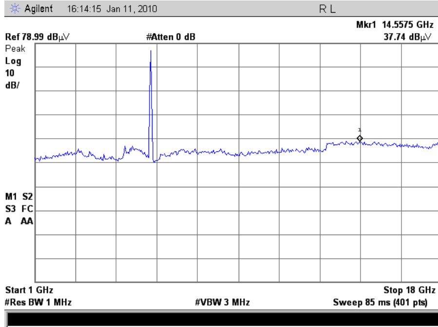
Plot 43. Radiated Spurious 5825MHz High Channel 802.11n 40MHz (1-18GHz)
