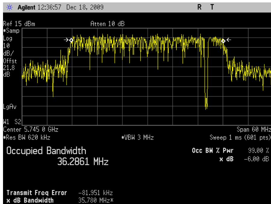
Plot 23. Occupied Band Width, 802.11n 40MHz Mode Low Channel, 99 % OBW
