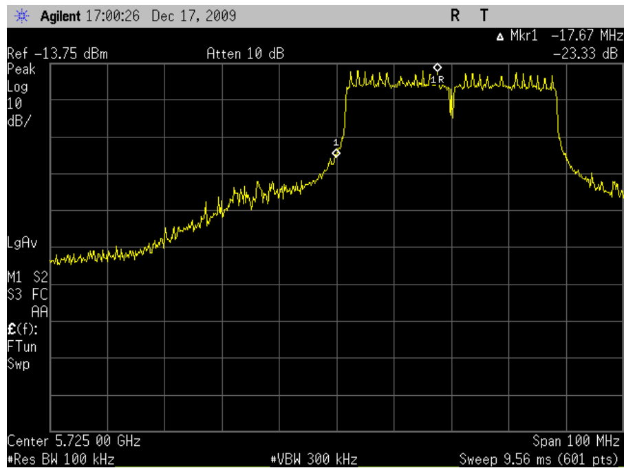
Plot 86. Conducted Band Edge 5745MHz Low Channel 802.11n 40MHz
