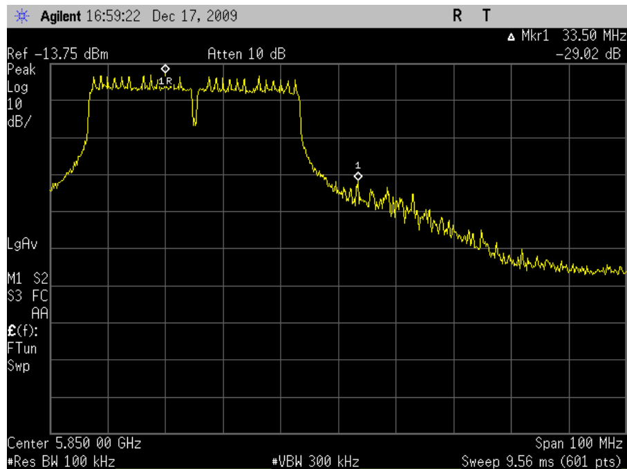
Plot 87. Conducted Band Edge 5825MHz High Channel 802.11n 40MHz
