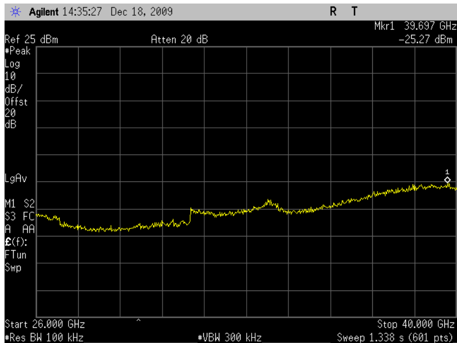
Plot 49. Conducted Spurious 5745MHz Low Channel 802.11a 26-40GHz
