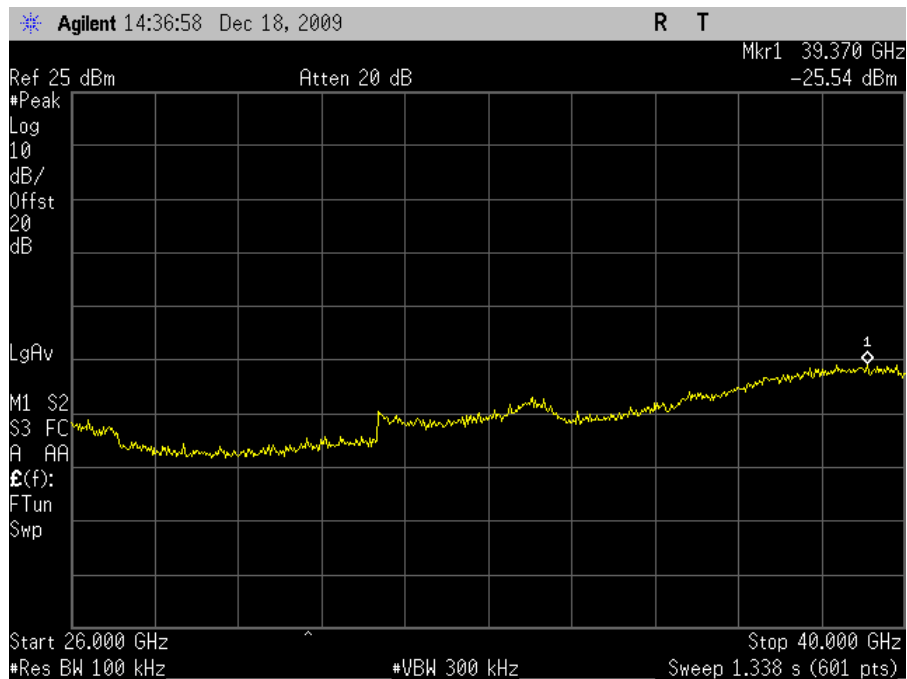
Plot 53. Conducted Spurious 5785MHz Mid Channel 802.11a 26-40GHz
