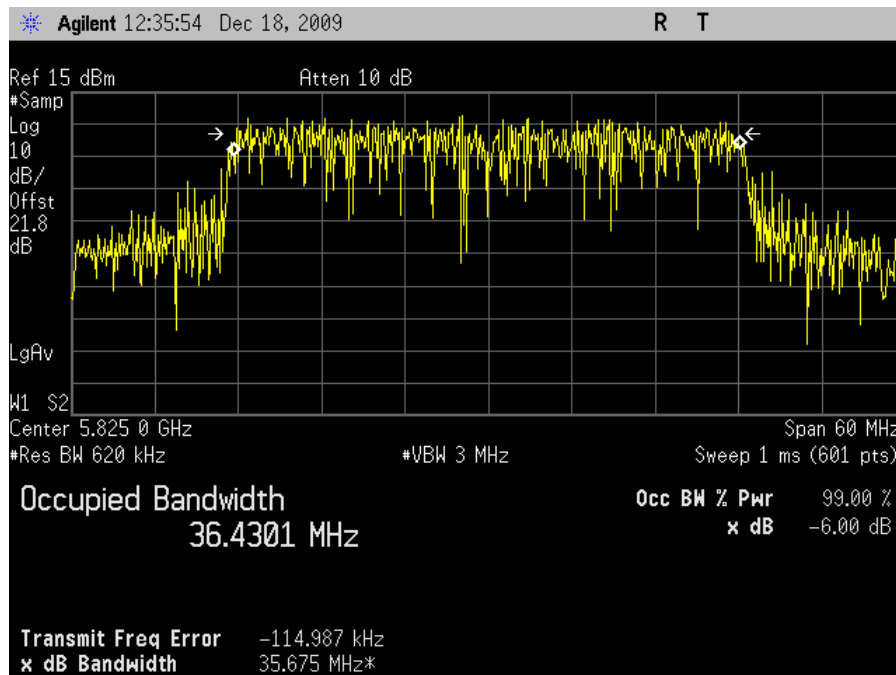
Plot 25. Occupied Band Width, 802.11n 40MHz Mode High Channel, 99 % OBW
