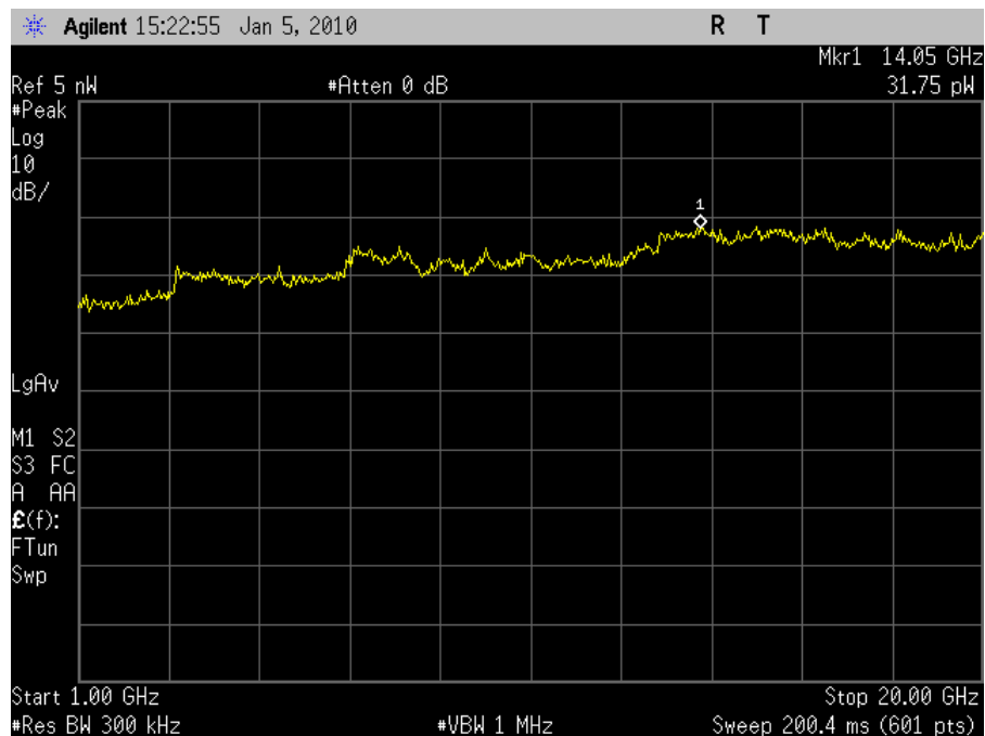
Plot 45. Conducted Receiver Spurious Emission, 1 GHz – 20 GHz
