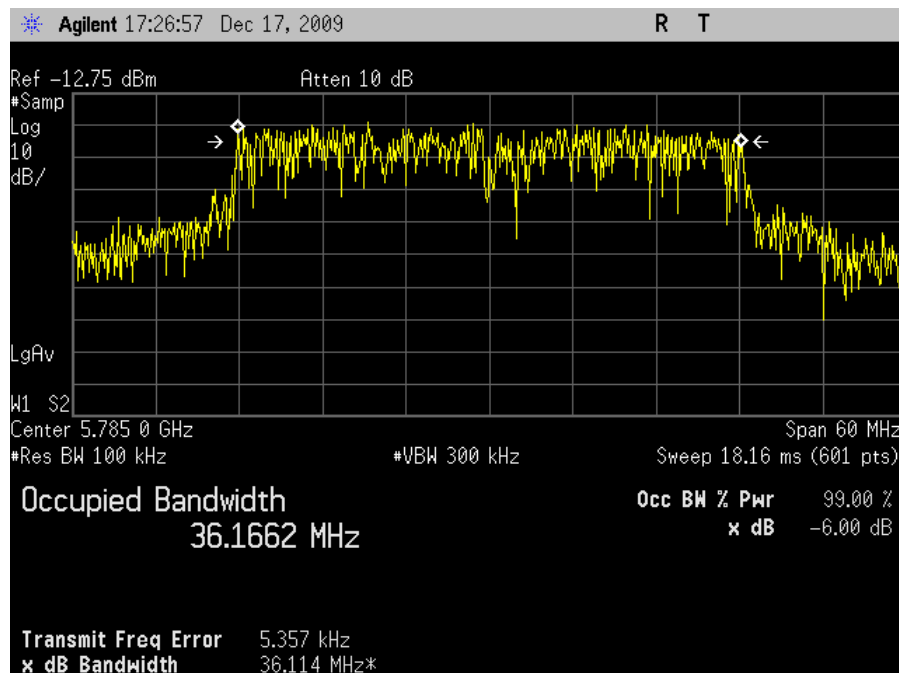
Plot 21. Occupied Band Width, 802.11n 40MHz Mode Mid Channel, FCC, 6 dB
