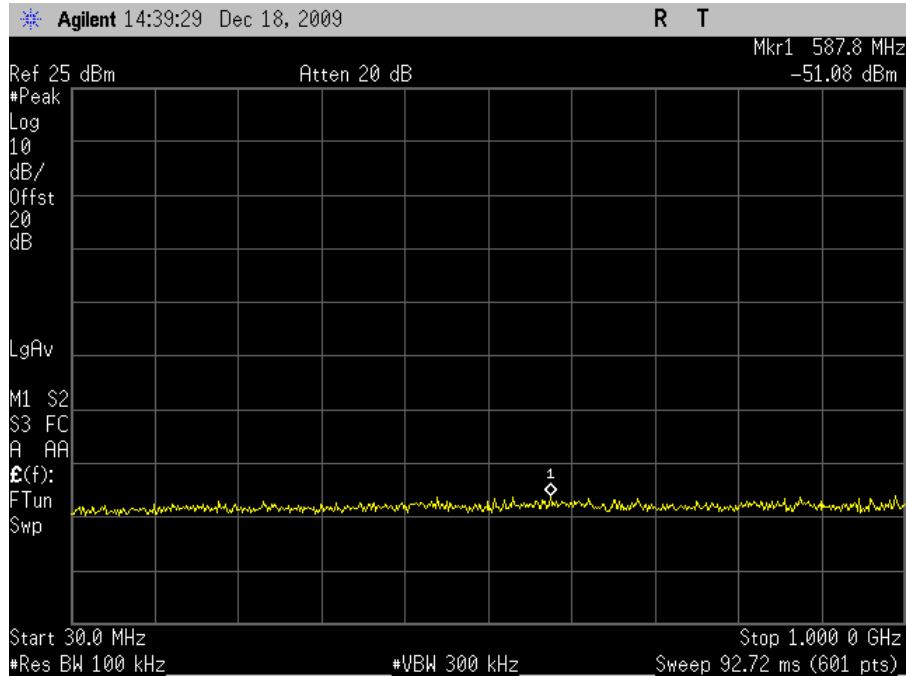
Plot 50. Conducted Spurious 5785MHz Mid Channel 802.11a 30MHz-1GHz
