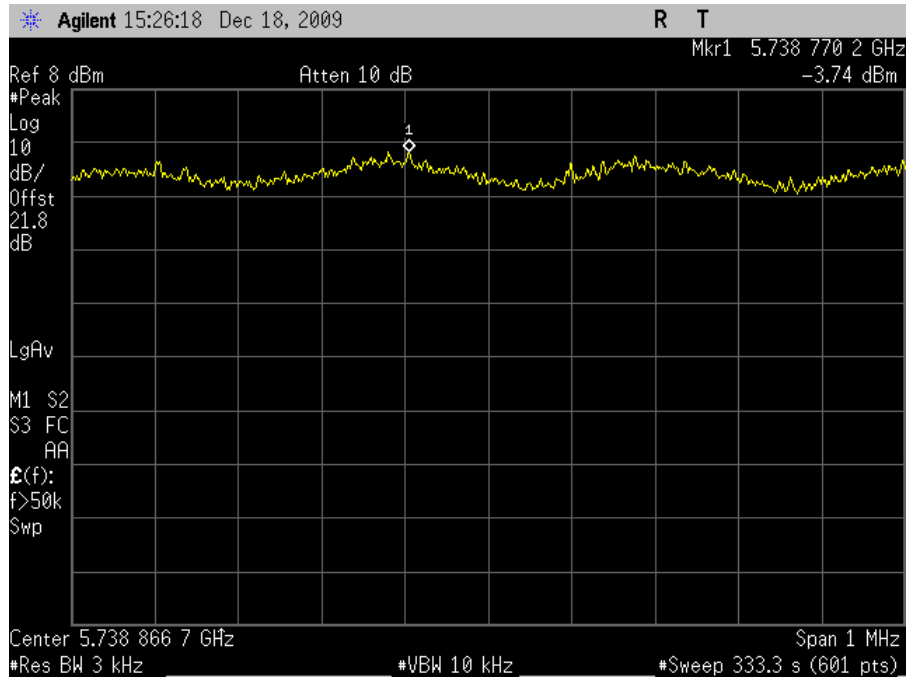
Plot 88. Power Spectral Density 5745MHz Low Channel 802.11a
