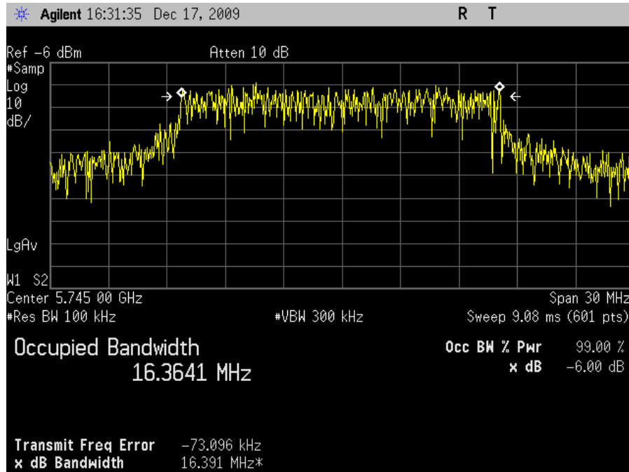
Plot 8. Occupied Band Width, 802.11a Mode Low Channel, FCC, 6 dB
