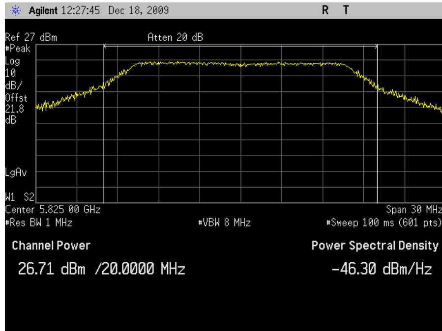
Plot 28. Peak Output Power, 802.11a Mode High Channel
