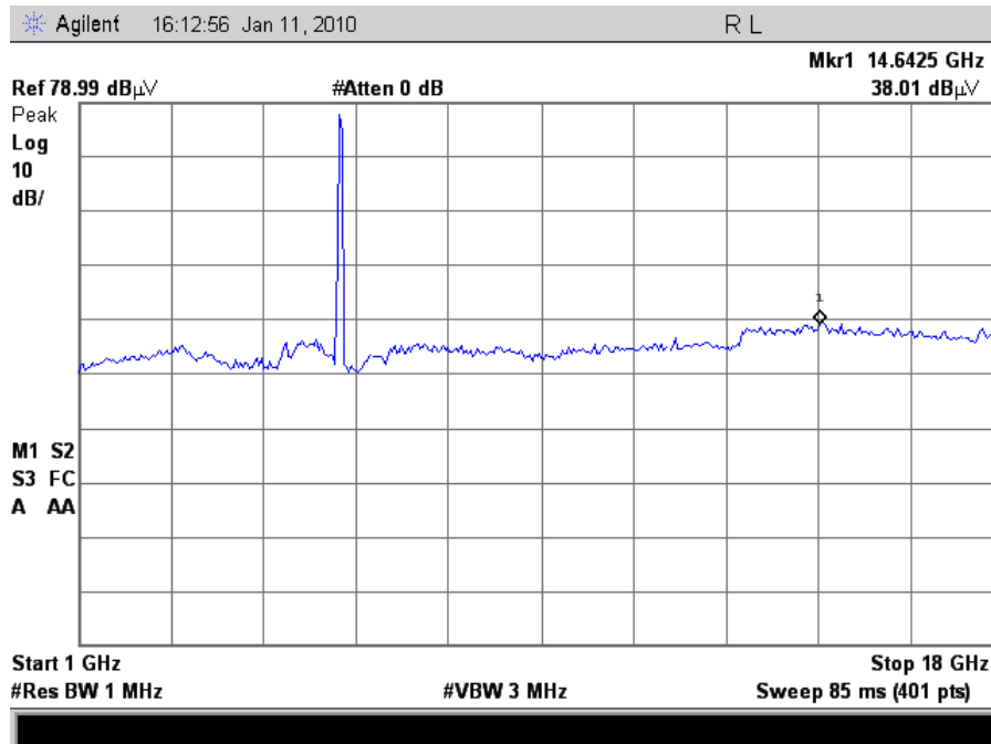
Plot 42. Radiated Spurious 5785MHz Mid Channel 802.11n 40MHz (1-18GHz)
