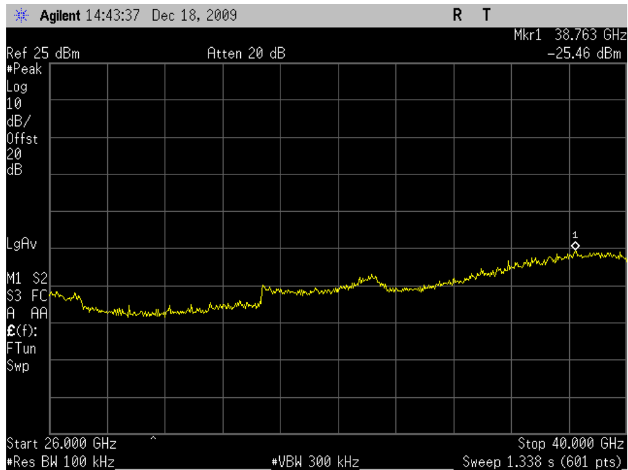
Plot 57. Conducted Spurious 5825MHz High Channel 802.11a 26-40GHz
