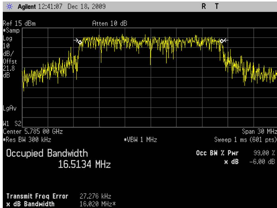
Plot 12. Occupied Band Width, 802.11a Mode Mid Channel, 99 % OBW
