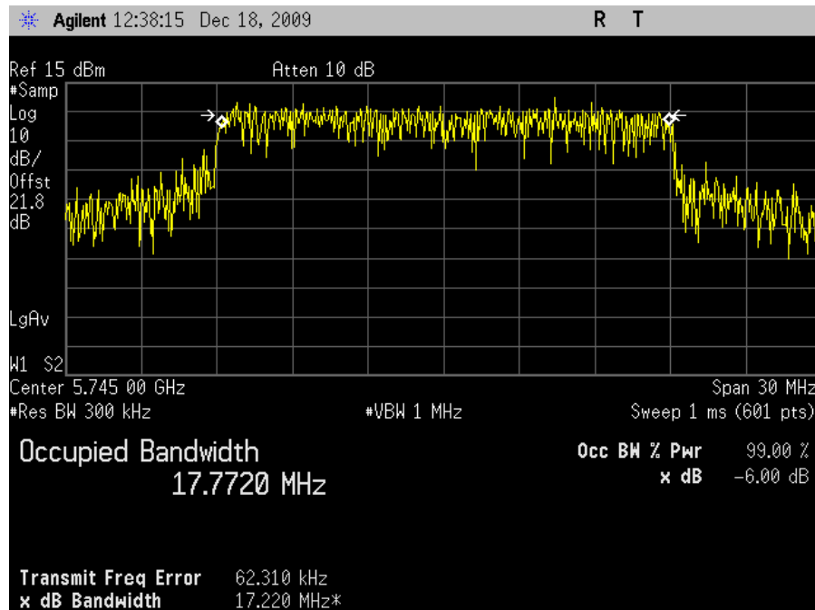
Plot 17. Occupied Band Width, 802.11n 20MHz Mode Low Channel, 99 % OBW
