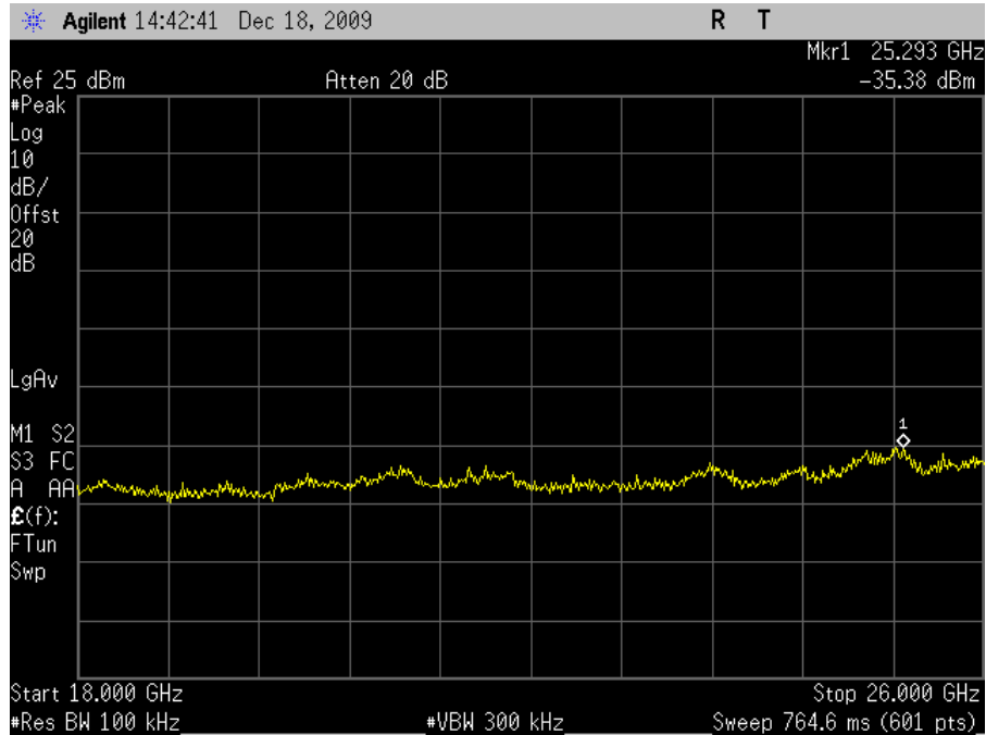
Plot 56. Conducted Spurious 5825MHz High Channel 802.11a 18-26GHz
