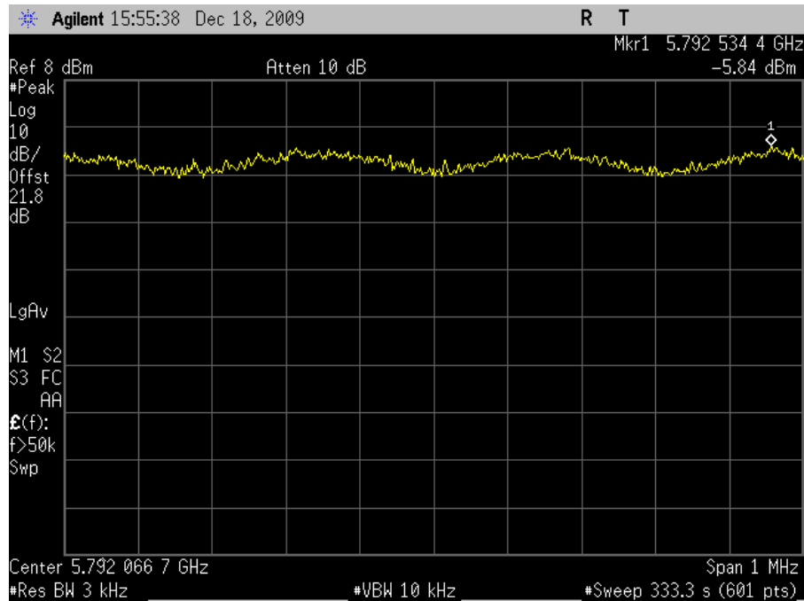
Plot 92. Power Spectral Density 5785MHz Mid Channel 802.11n 20MHz
