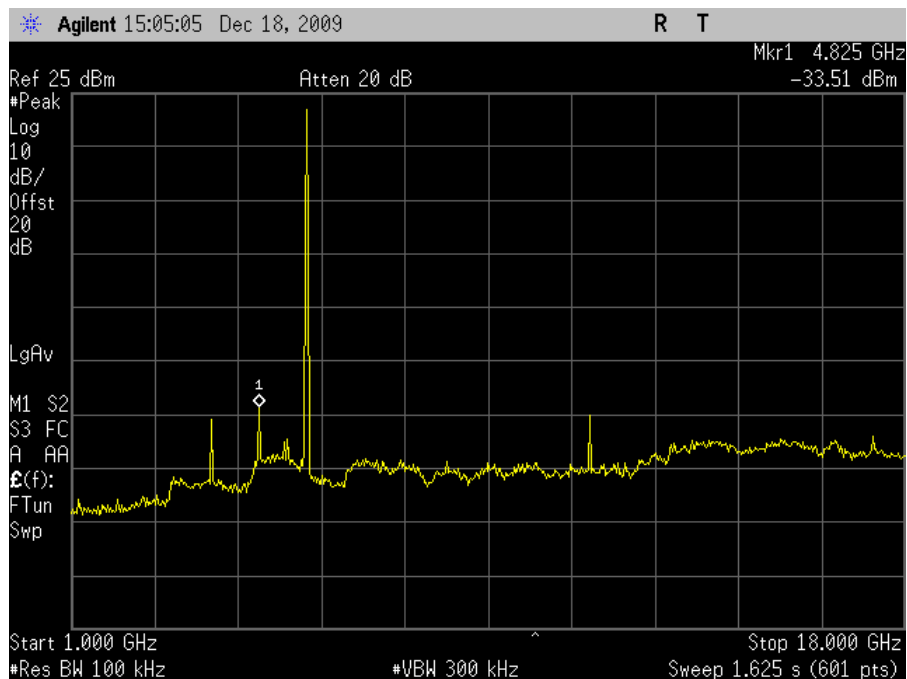
Plot 75. Conducted Spurious 5785MHz Mid Channel 802.11n 40MHz 1-18GHz
