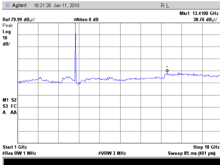
Plot 36. Radiated Spurious 5785MHz Mid Channel 802.11a (1-18GHz)
