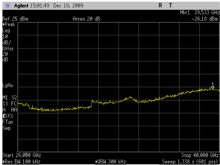
Plot 73. Conducted Spurious 5745MHz Low Channel 802.11n 40MHz 26-40GHz
