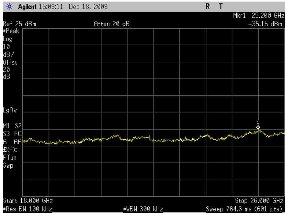
Plot 80. Conducted Spurious 5825MHz High Channel 802.11n 40MHz 18-26GHz
