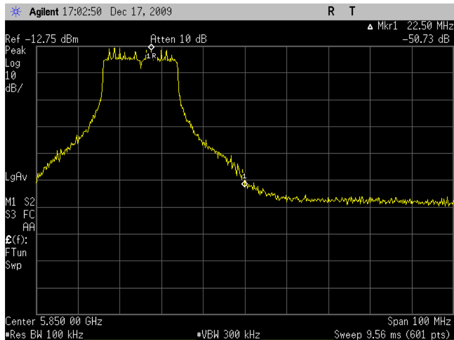
Plot 85. Conducted Band Edge 5825MHz High Channel 802.11n 20MHz
