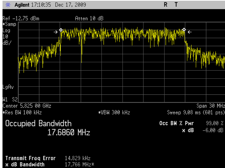
Plot 16. Occupied Band Width, 802.11n 20MHz Mode High Channel, FCC, 6 dB
