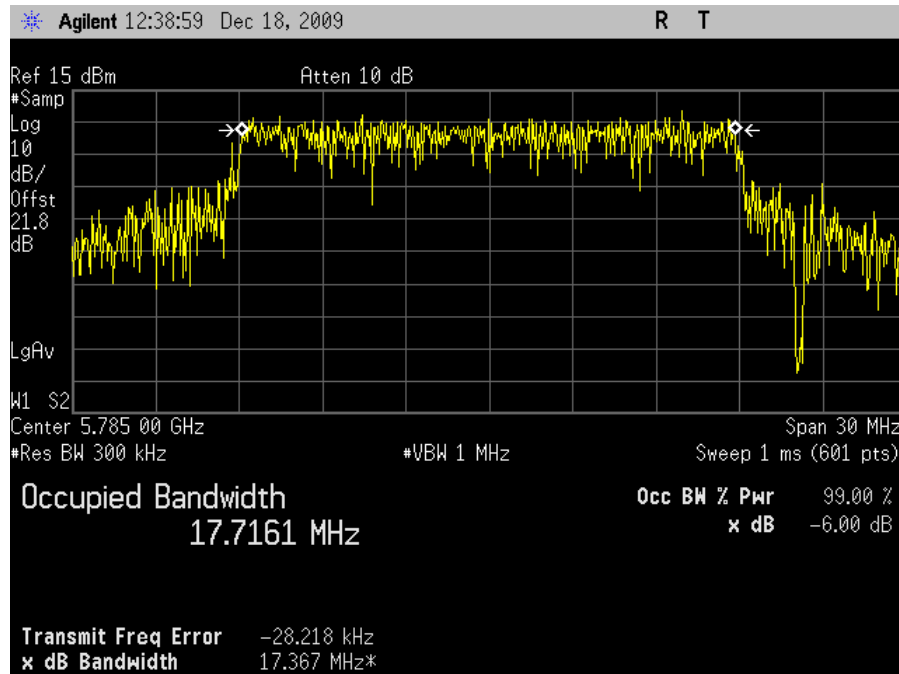
Plot 18. Occupied Band Width, 802.11n 20MHz Mode Mid Channel, 99 % OBW
