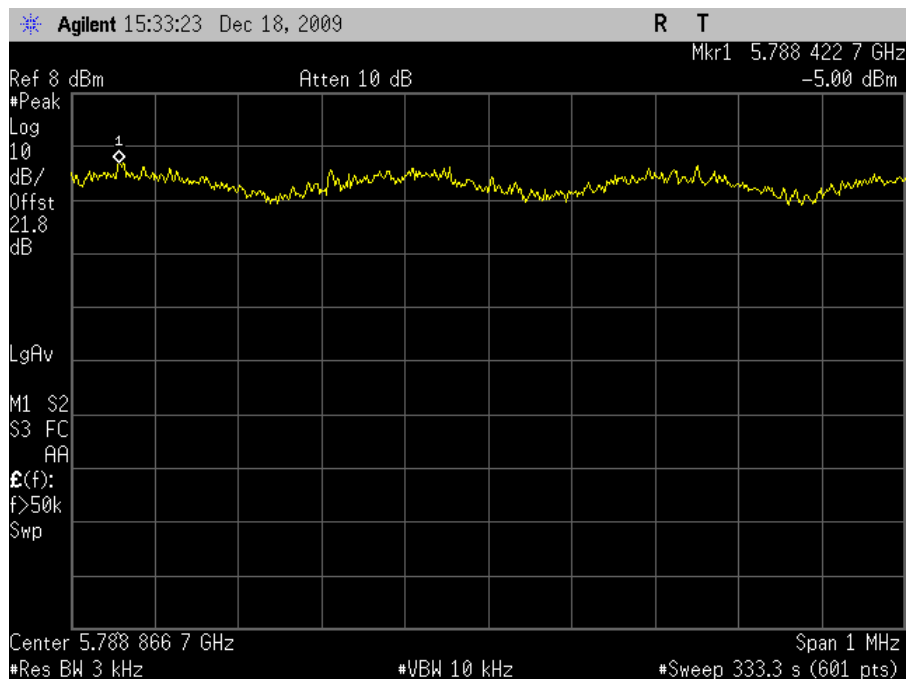
Plot 89. Power Spectral Density 5785MHz Mid Channel 802.11a
