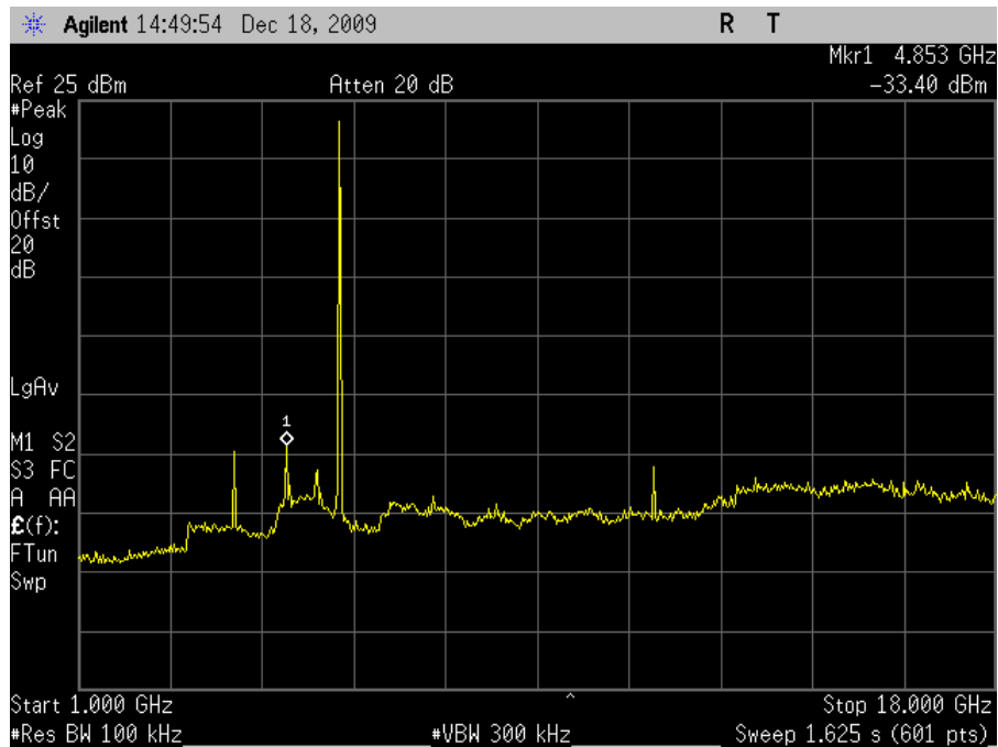
Plot 67. Conducted Spurious 5825MHz High Channel 802.11n 20MHz 1-18GHz
