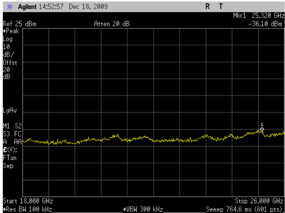
Plot 64. Conducted Spurious 5785MHz Mid Channel 802.11n 20MHz 18-26GHz
