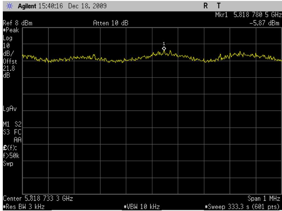
Plot 90. Power Spectral Density 5825MHz High Channel 802.11a
