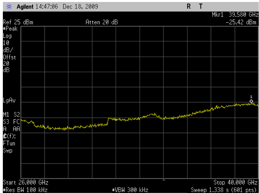
Plot 69. Conducted Spurious 5825MHz High Channel 802.11n 20MHz 26-40GHz
