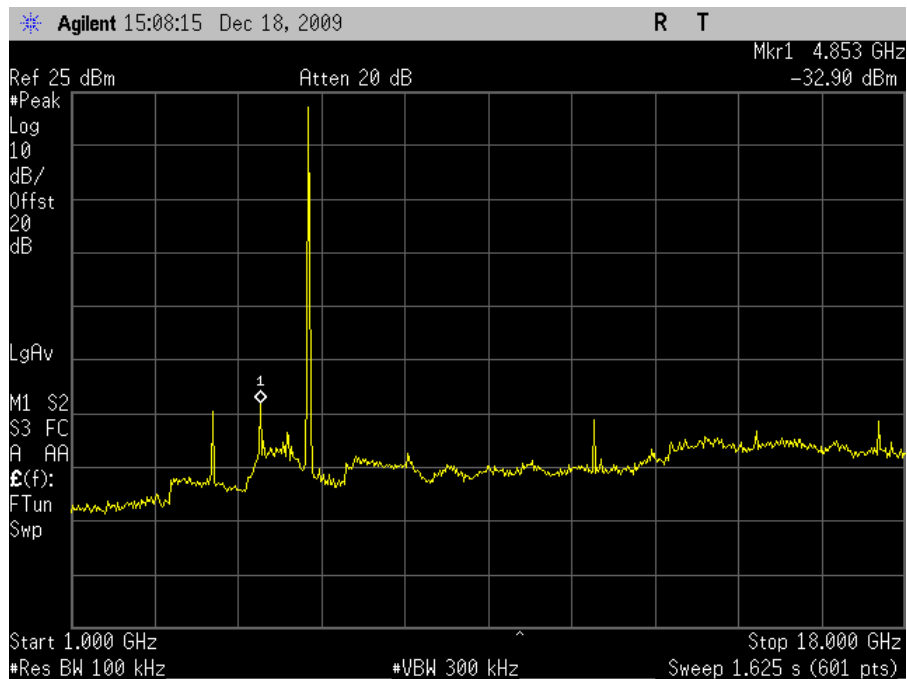
Plot 79. Conducted Spurious 5825MHz High Channel 802.11n 40MHz 1-18GHz
