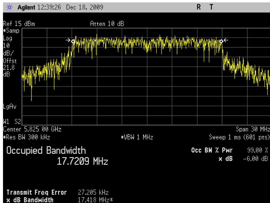
Plot 19. Occupied Band Width, 802.11n 20MHz Mode High Channel, 99 % OBW
