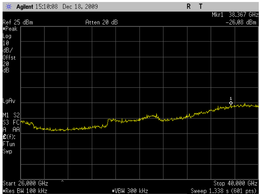
Plot 81. Conducted Spurious 5825MHz High Channel 802.11n 40MHz 26-40GHz
