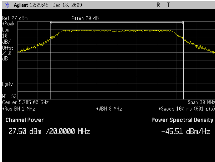
Plot 30. Peak Output Power, 802.11n 20MHz Mode Mid Channel
