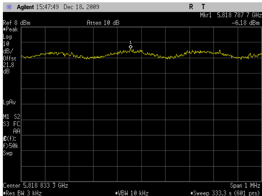
Plot 93. Power Spectral Density 5825MHz High Channel 802.11n 20MHz
