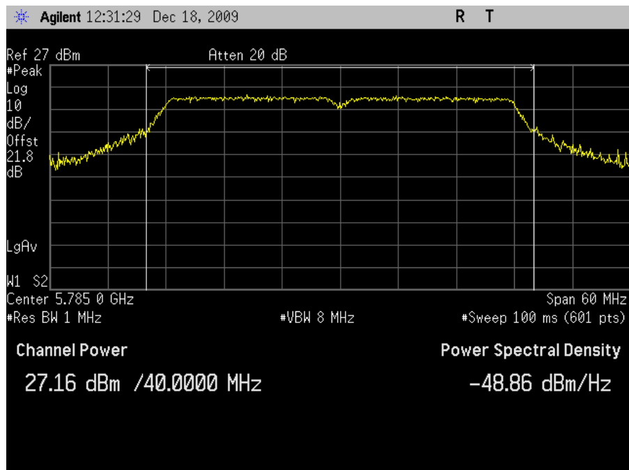
Plot 33. Peak Output Power, 802.11n 40MHz Mode Mid Channel
