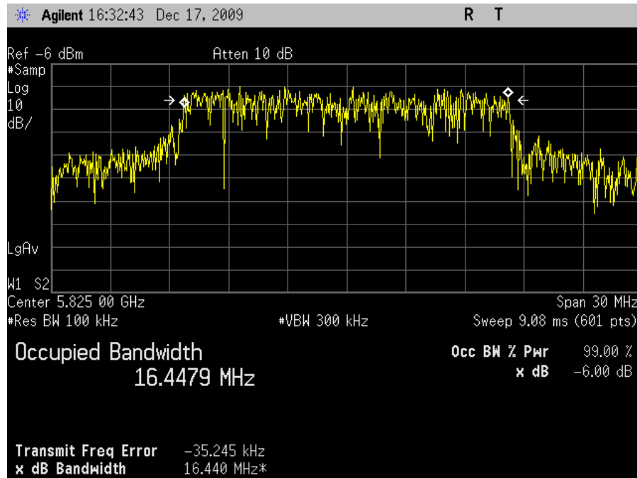
Plot 10. Occupied Band Width, 802.11a Mode High Channel, FCC, 6 dB
