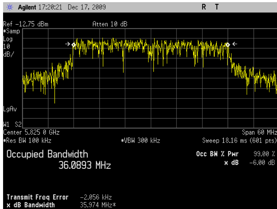
Plot 22. Occupied Band Width, 802.11n 40MHz Mode High Channel, FCC, 6 dB
