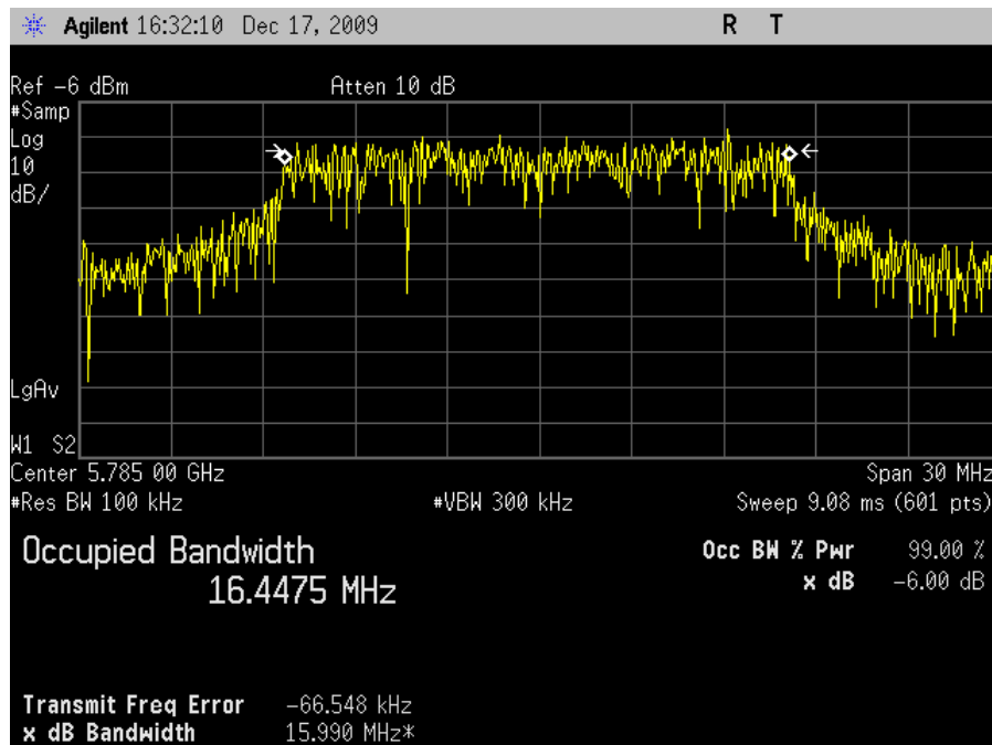
Plot 9. Occupied Band Width, 802.11a Mode Mid Channel, FCC, 6 dB
