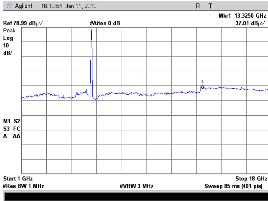
Plot 41. Radiated Spurious 5745MHz Low Channel 802.11n 40MHz (1-18GHz)
