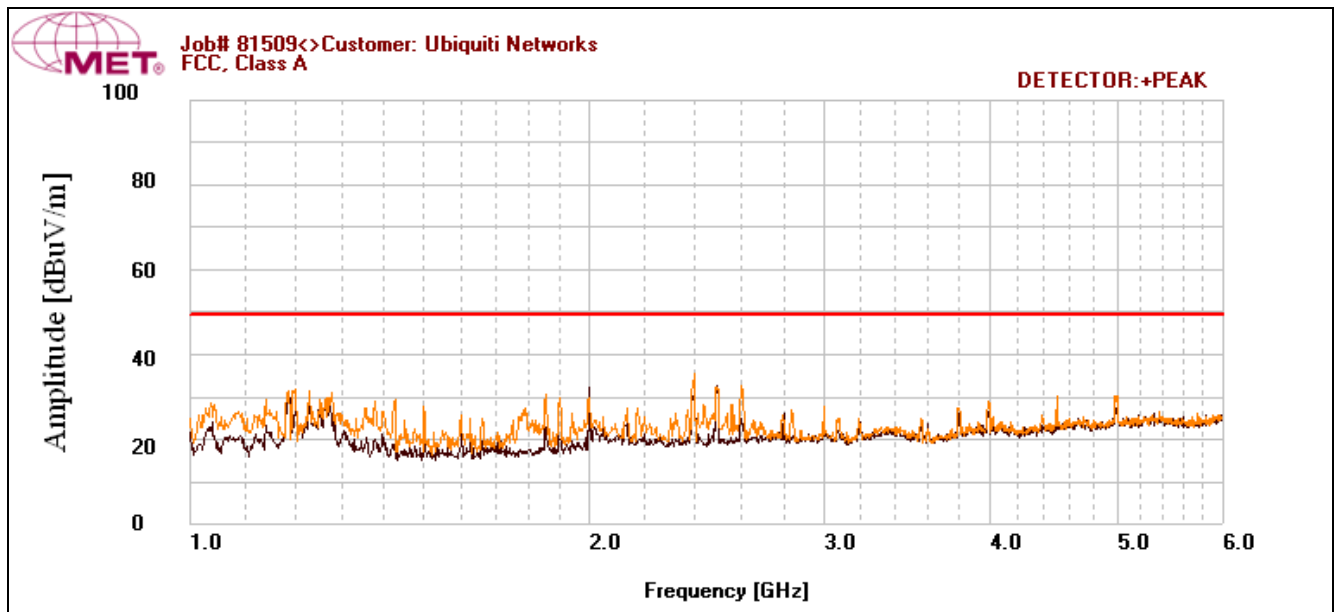
Plot 4. Radiated Emissions, Pre-Scan, FCC Limits, Above 1 GHz
