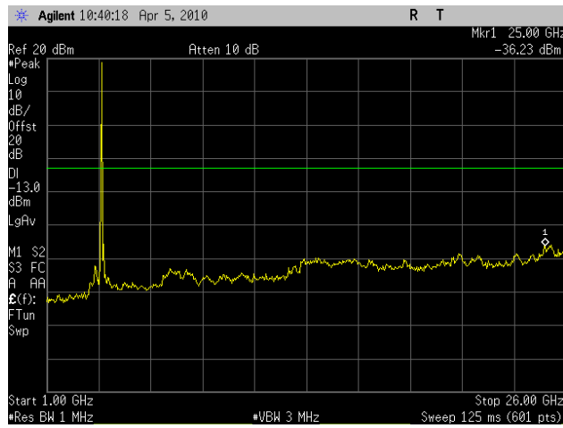
Plot 80. Conducted Spurious Emissions Low Ch, 1 GHz - 26GHz, (HT10) – Port 2
