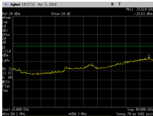
Plot 66. Conducted Spurious Emissions Mid Ch, 26GHz – 40GHz, (HT5) – Port 2
