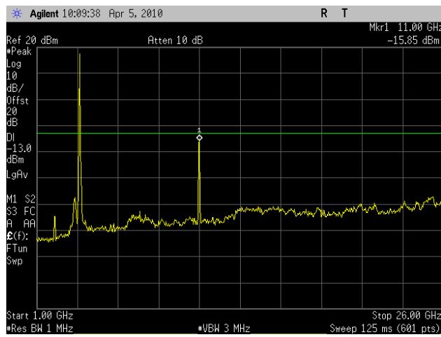
Plot 89. Conducted Spurious Emissions Mid Ch, 1 GHz – 26GHz, (HT20) – Port 1
