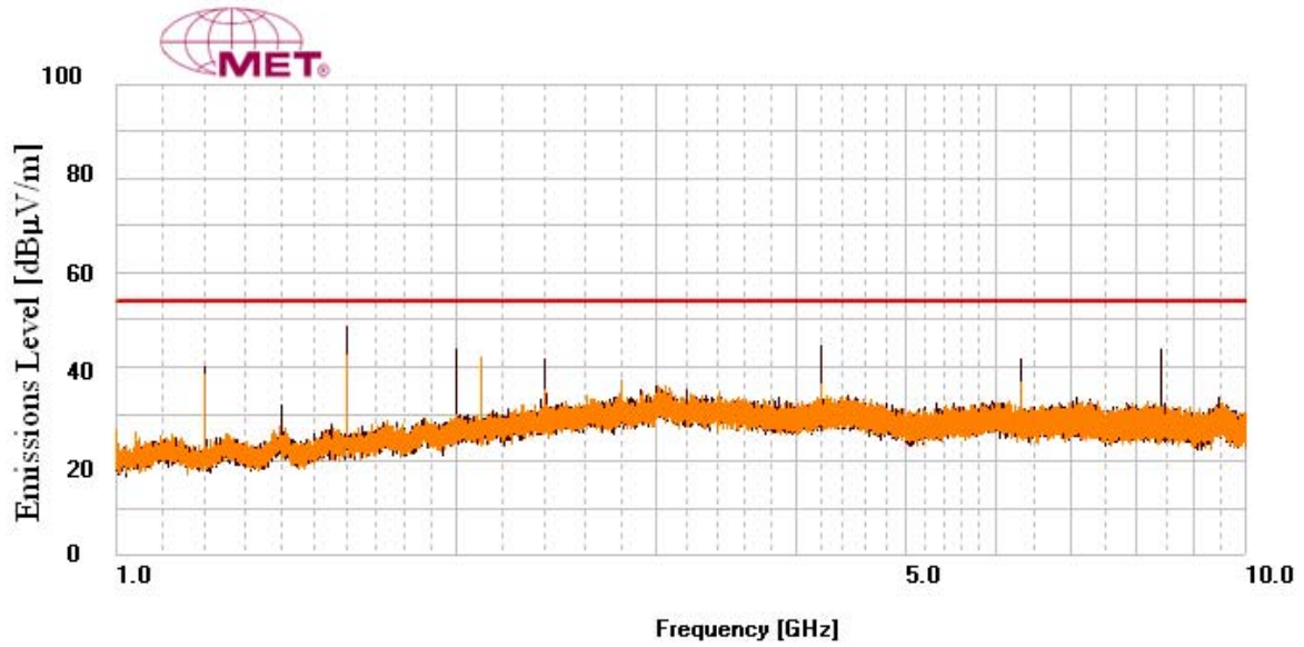
Plot 2. Radiated Emissions 1GHz – 10GHz
