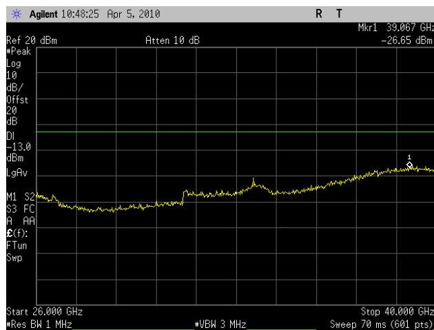
Plot 72. Conducted Spurious Emissions Low Ch, 26GHz – 40GHz, (HT10) – Port 1
