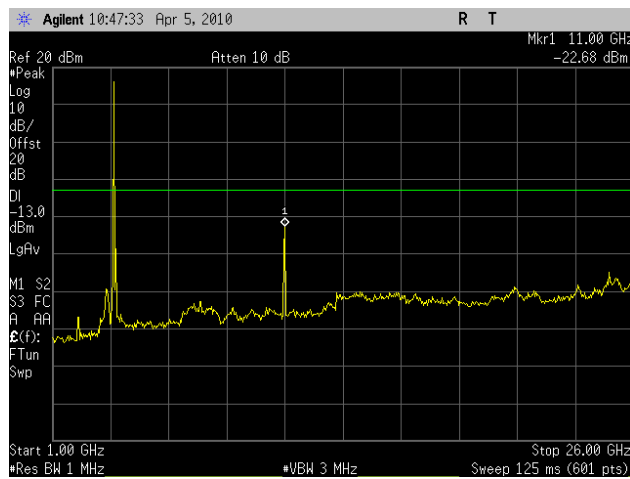
Plot 74. Conducted Spurious Emissions Mid Ch, 1 GHz – 26GHz, (HT10) – Port 1
