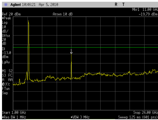
Plot 77. Conducted Spurious Emissions High Ch, 1 GHz – 26GHz, (HT10) – Port 1
