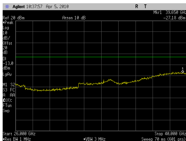
Plot 63. Conducted Spurious Emissions Low Ch, 26GHz – 40GHz, (HT5) – Port 2
