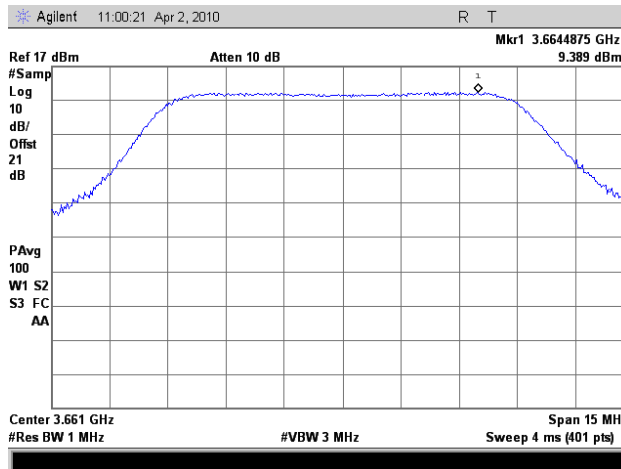
Plot 27. PPSD 10 MHz Mid Ch (Port 1)
