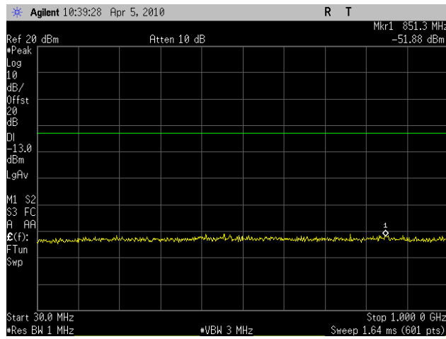
Plot 79. Conducted Spurious Emissions Low Ch, 30 MHz - 1GHz, (HT10) – Port 2
