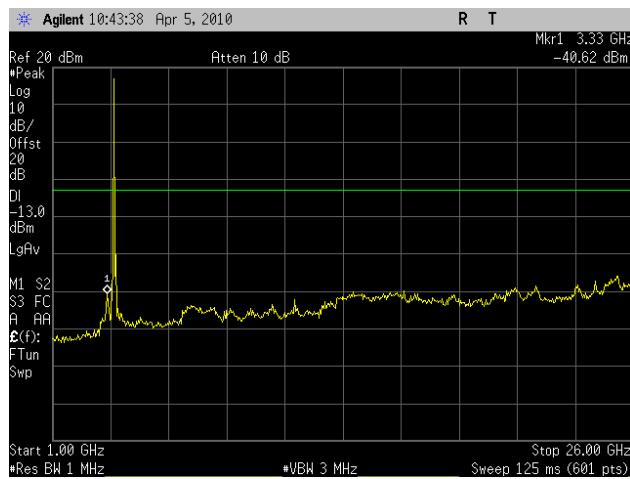
Plot 86. Conducted Spurious Emissions High Ch, 1 GHz – 26GHz, (HT10) – Port 2
