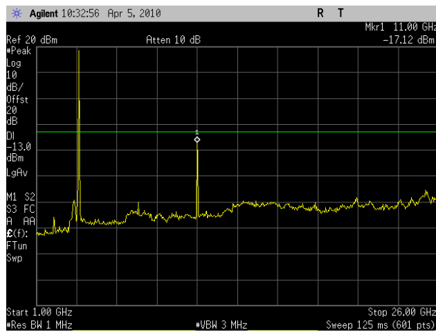
Plot 59. Conducted Spurious Emissions High Ch, 1 GHz – 26GHz, (HT5) – Port 1
