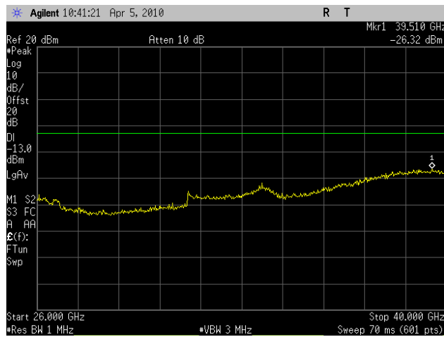
Plot 84. Conducted Spurious Emissions Mid Ch, 26GHz - 40GHz, (HT10) – Port 2
