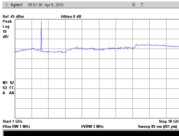
Plot 110. Radiated Spurious Mid Channel, HT10 (1-18GHz) – All Ports
