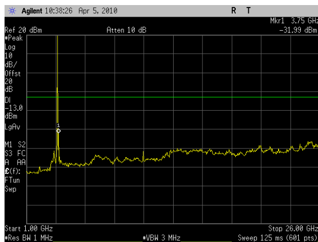
Plot 62. Conducted Spurious Emissions Low Ch, 1 GHz – 26GHz, (HT5) – Port 2
