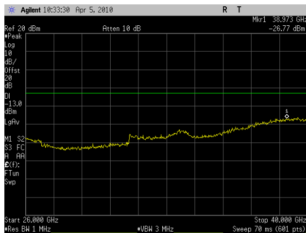
Plot 60. Conducted Spurious Emissions High Ch, 26GHz – 40GHz, (HT5) – Port 1
