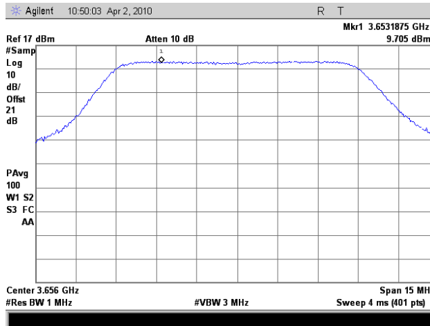
Plot 26. PPSD 10 MHz Low Ch (Port 1)
