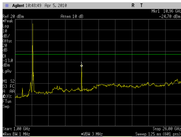
Plot 71. Conducted Spurious Emissions Low Ch, 1 GHz – 26GHz, (HT10) – Port 1
