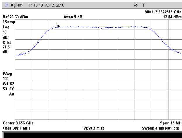
Plot 32. PPSD 10 MHz Low Ch (Combined Ports)
