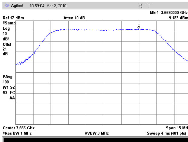
Plot 28. PPSD 10 MHz High Ch (Port 1)
