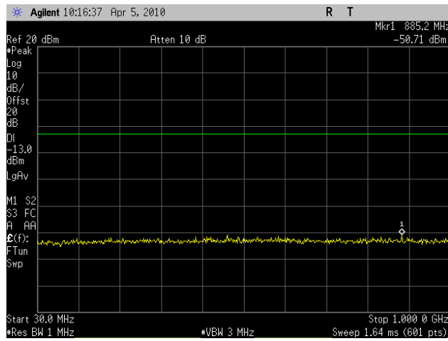
Plot 88. Conducted Spurious Emissions Mid Ch, 30 MHz - 1GHz, (HT20) – Port 1
