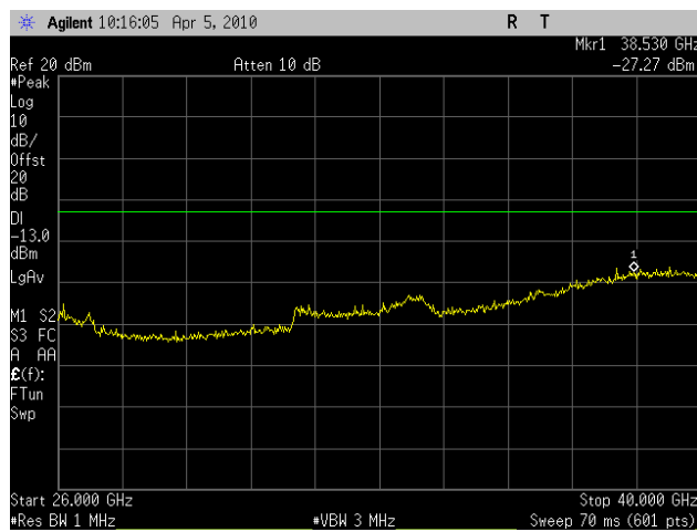
Plot 90. Conducted Spurious Emissions Mid Ch, 26GHz – 40GHz, (HT20) – Port 1
