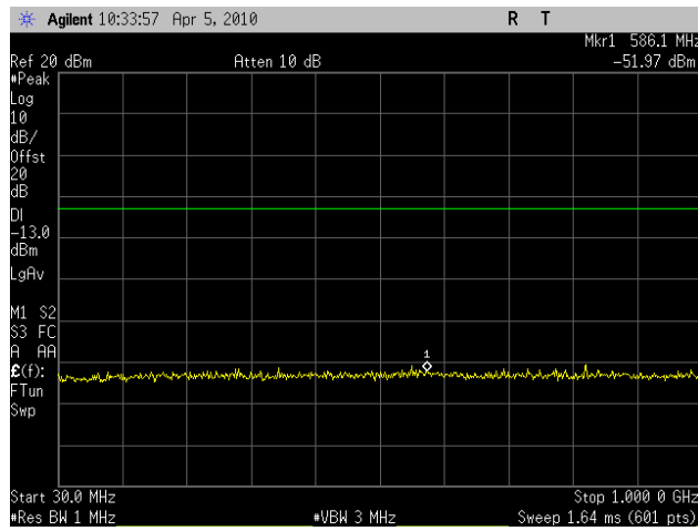
Plot 58. Conducted Spurious Emissions High Ch, 30 MHz - 1GHz, (HT5) – Port 1
