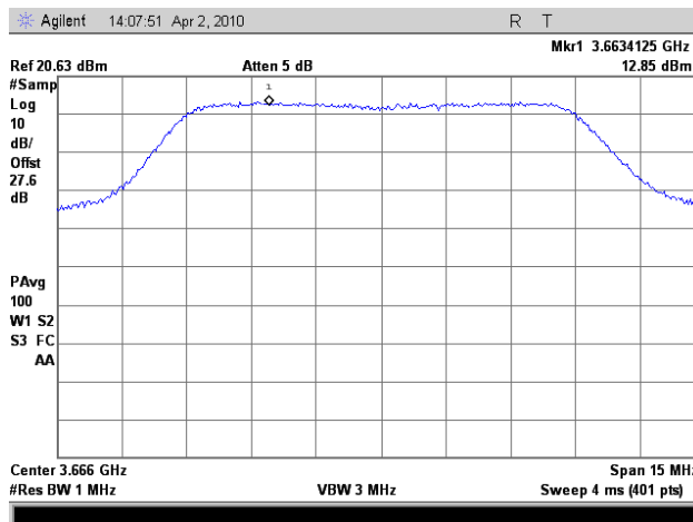
Plot 34. PPSD 10 MHz High Ch (Combined Ports)
