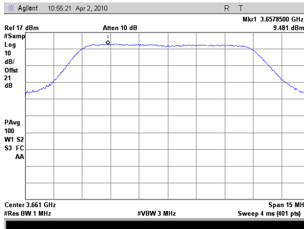
Plot 30. PPSD 10 MHz Mid Ch (Port 2)
