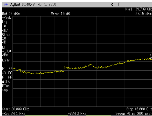
Plot 81. Conducted Spurious Emissions Low Ch, 26GHz - 40GHz, (HT10) – Port 2
