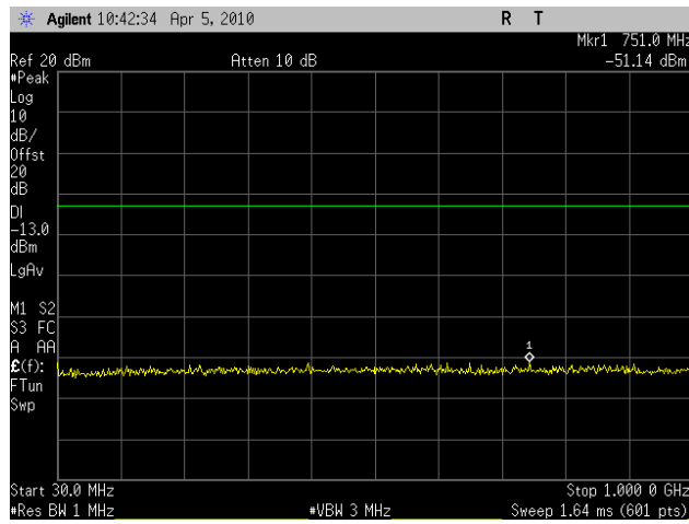
Plot 82. Conducted Spurious Emissions Mid Ch, 30 MHz - 1GHz, (HT10) – Port 2
