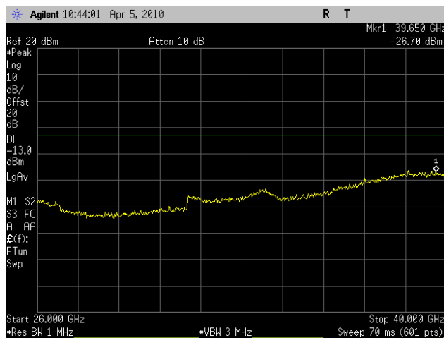
Plot 87. Conducted Spurious Emissions High Ch, 26GHz – 40GHz, (HT10) – Port 2
