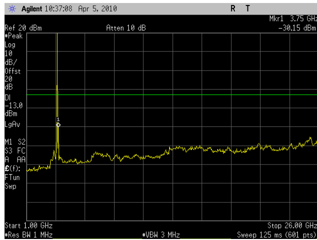
Plot 65. Conducted Spurious Emissions Mid Ch, 1 GHz – 26GHz, (HT5) – Port 2
