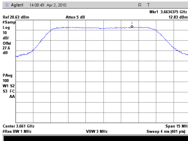
Plot 33. PPSD 10 MHz Mid Ch (Combined Ports)
