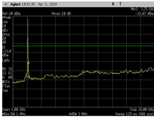
Plot 83. Conducted Spurious Emissions Mid Ch, 1 GHz - 26GHz, (HT10) – Port 2
