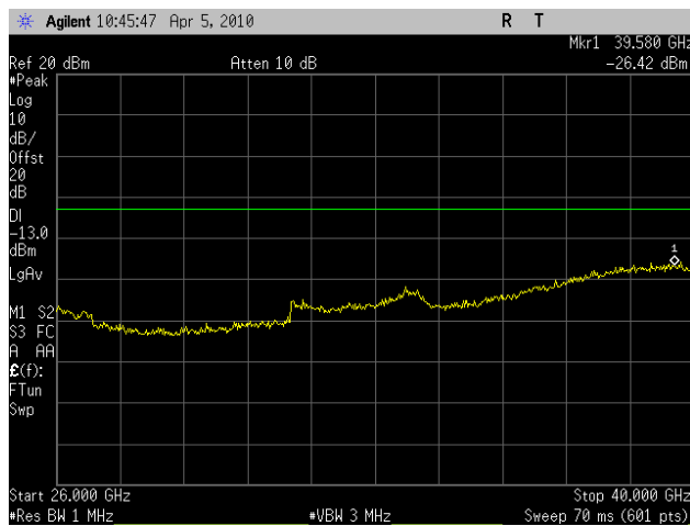
Plot 78. Conducted Spurious Emissions High Ch, 26GHz – 40GHz, (HT10) – Port 1
