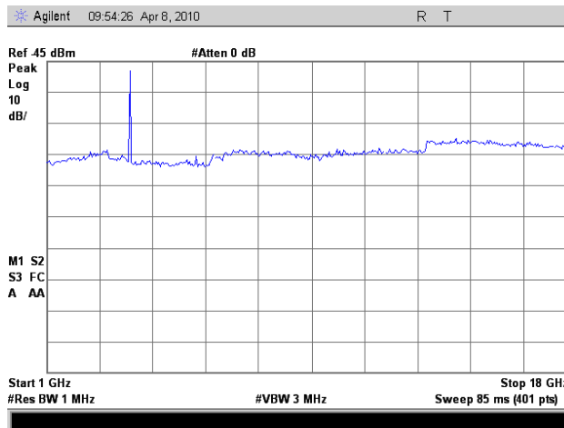
Plot 111. Radiated Spurious High Channel, HT10 (1-18GHz) – All Ports
