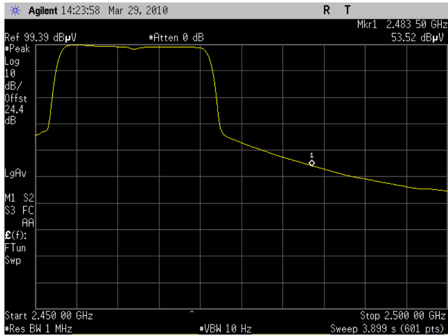
Plot 74. Radiated Band Edge 2462MHz Channel 11 802.11n (Average)
