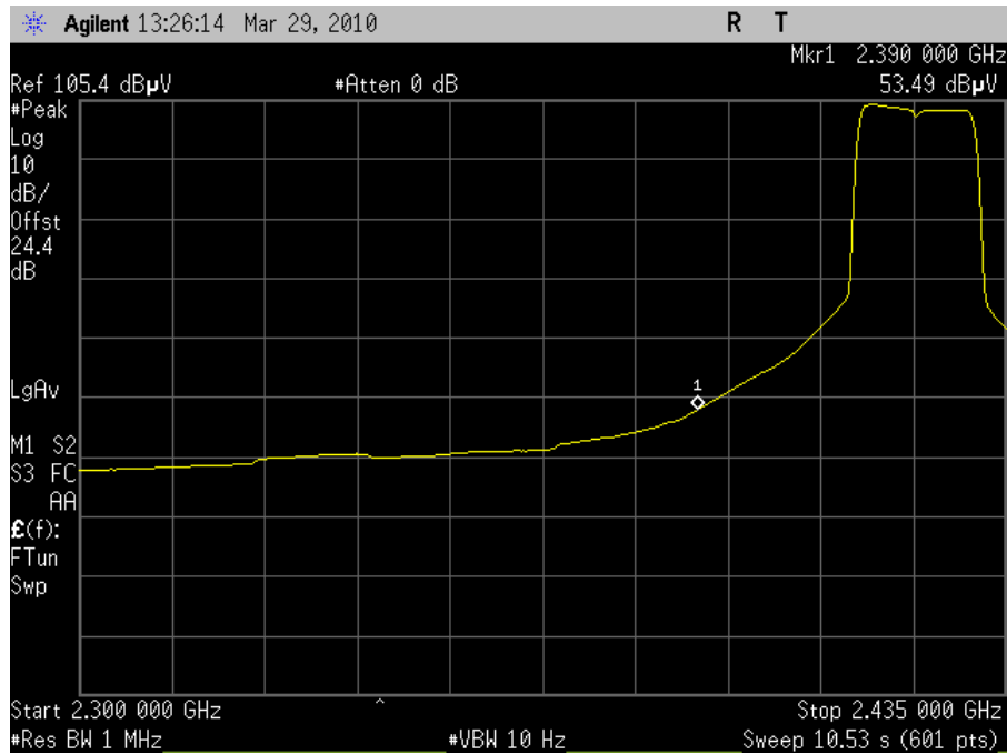
Plot 52. Radiated Band Edge 2422MHz Channel 3 802.11g (Average)
