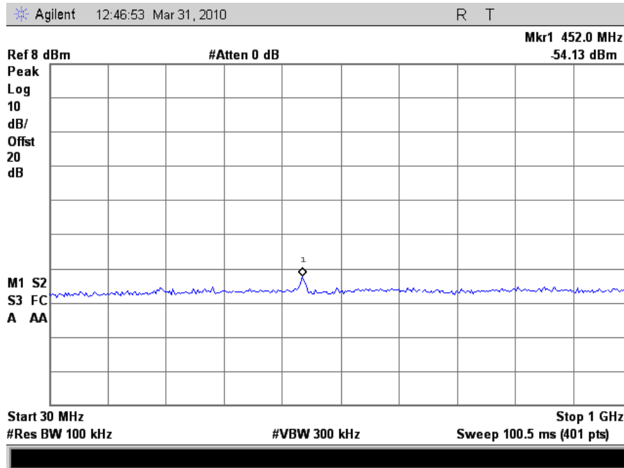
Plot 78. Conducted Spurious 2412MHz Low Channel 802.11g (30MHz-1GHz)
