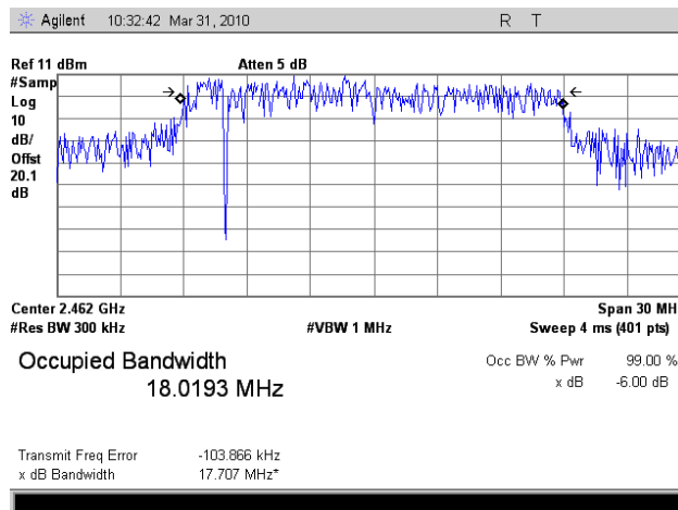
Plot 19. Occupied Band Width, 802.11n Mode, High Channel, 99 % OBW
