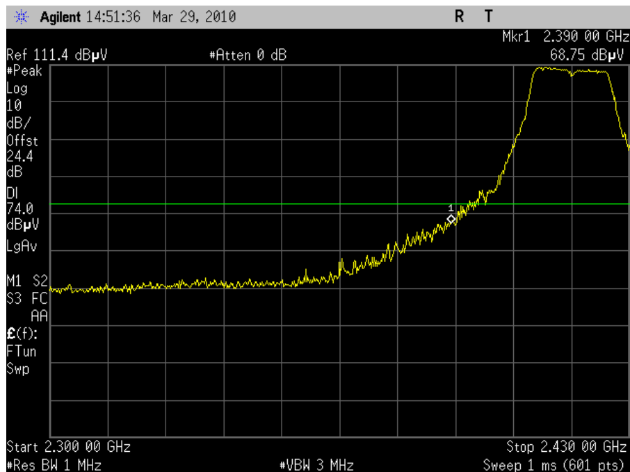
Plot 65. Radiated Band Edge 2417MHz Channel 2 802.11n (Peak)
