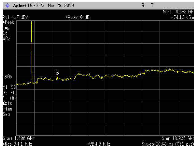
Plot 46. Radiated Spurious 2437MHz Mid Channel 802.11n (1-18GHz)
