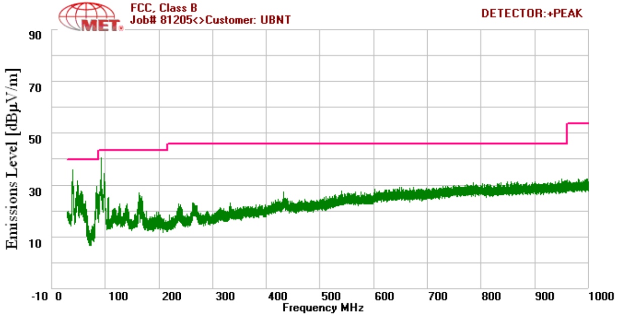
Plot 36. 15.209 Radiated Emissions 2412MHz Low Channel 802.11g (30MHz – 1GHz)
