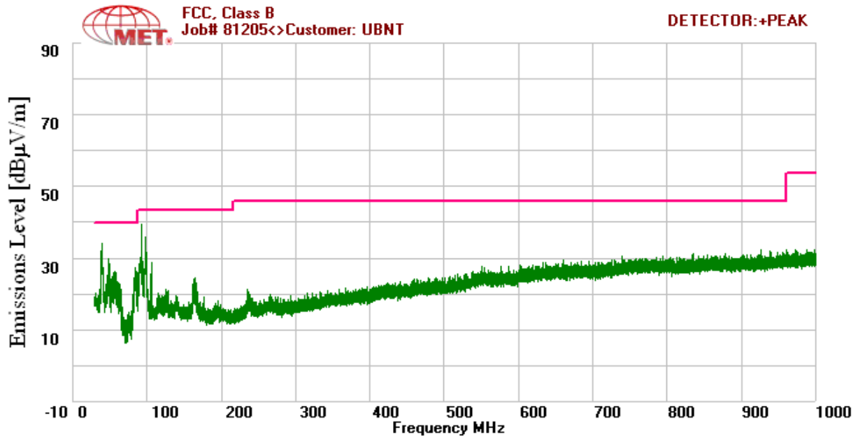
Plot 39. 15.209 Radiated Emissions 2412MHz Low Channel 802.11n (30MHz – 1GHz)
