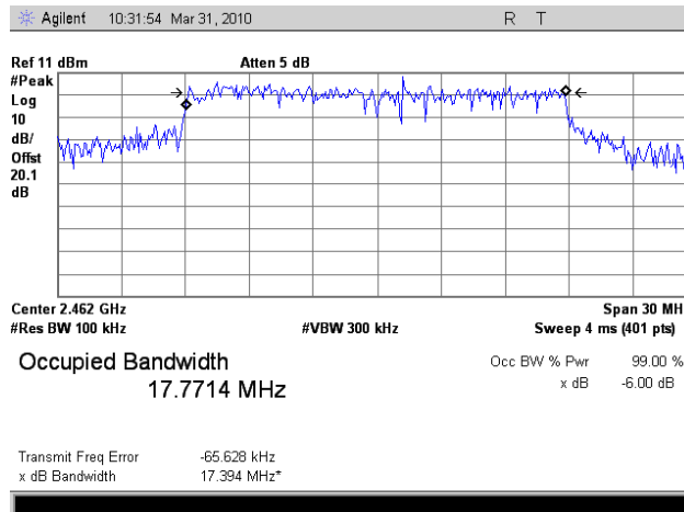
Plot 16. Occupied Band Width, 802.11n Mode, High Channel, FCC, 6 dB
