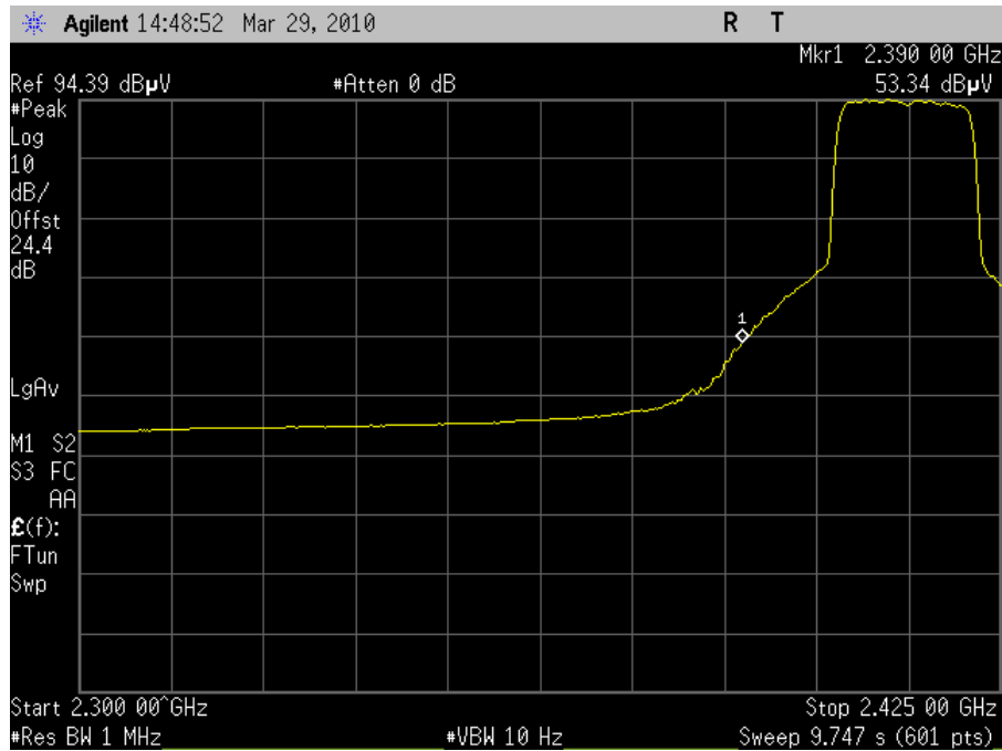
Plot 62. Radiated Band Edge 2412MHz Channel 1 802.11n (Average)
