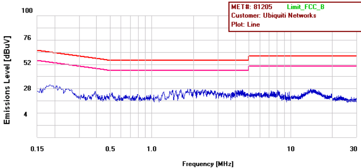
Plot 6. 15.207 Conducted Emissions, Phase Line
