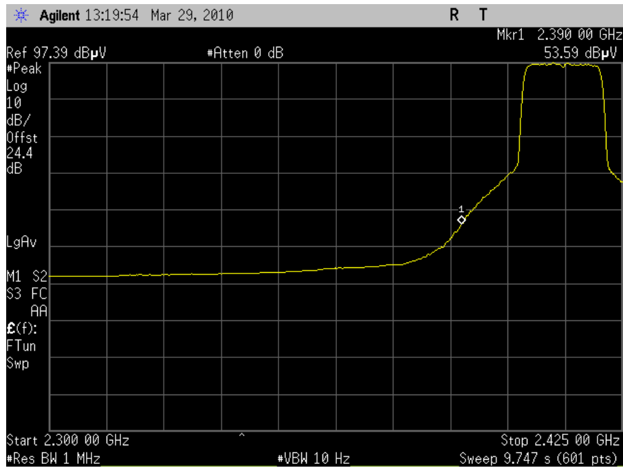
Plot 48. Radiated Band Edge 2412MHz Channel 1 802.11g (Average)
