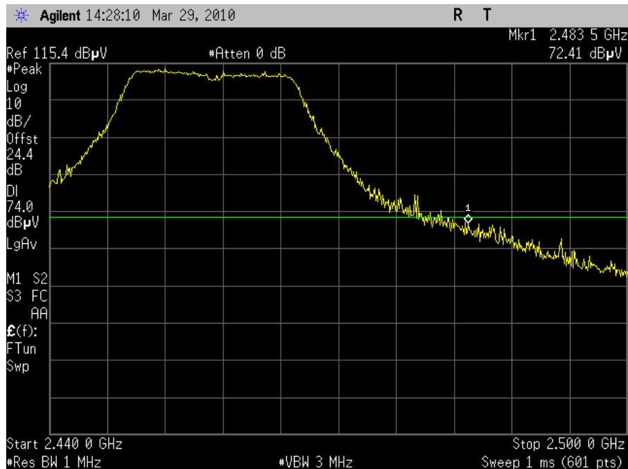
Plot 73. Radiated Band Edge 2462MHz Channel 10 802.11n (Peak)
