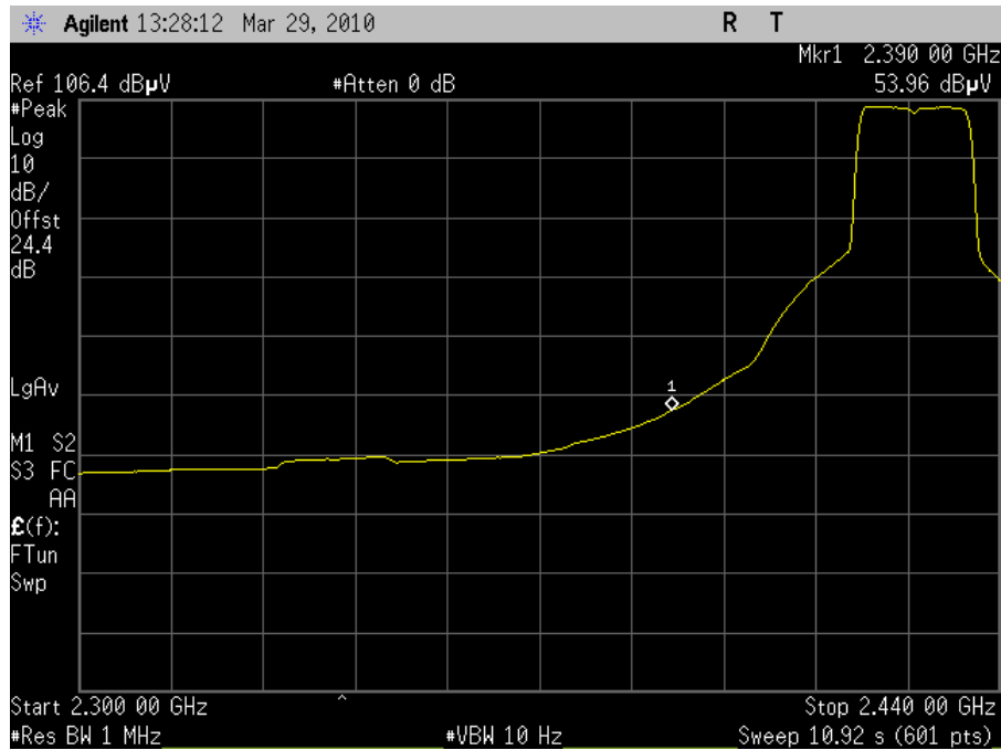
Plot 54. Radiated Band Edge 2427MHz Channel 4 802.11g (Average)
