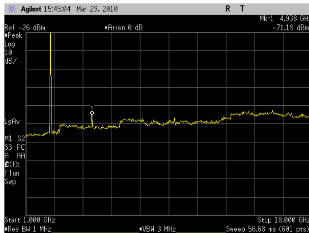
Plot 47. Radiated Spurious 2462MHz High Channel 802.11n (1-18GHz)
