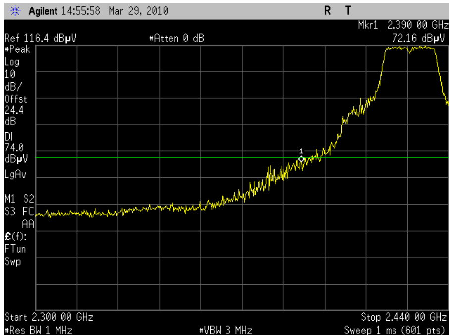
Plot 69. Radiated Band Edge 2427MHz Channel 4 802.11n (Peak)
