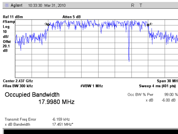
Plot 18. Occupied Band Width, 802.11n Mode, Mid Channel, 99% OBW
