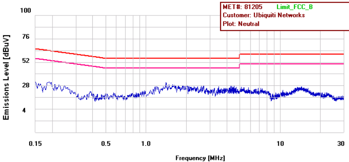
Plot 7. 15.207 Conducted Emissions, Neutral Line
