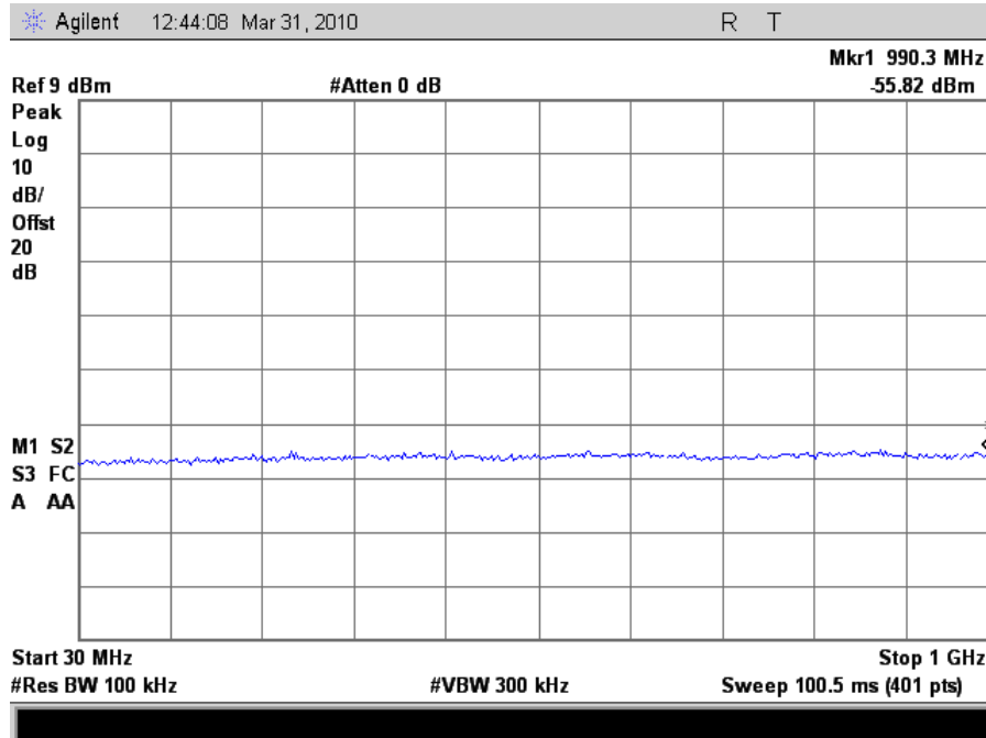
Plot 82. Conducted Spurious 2462MHz High Channel 802.11g (30MHz-1GHz)
