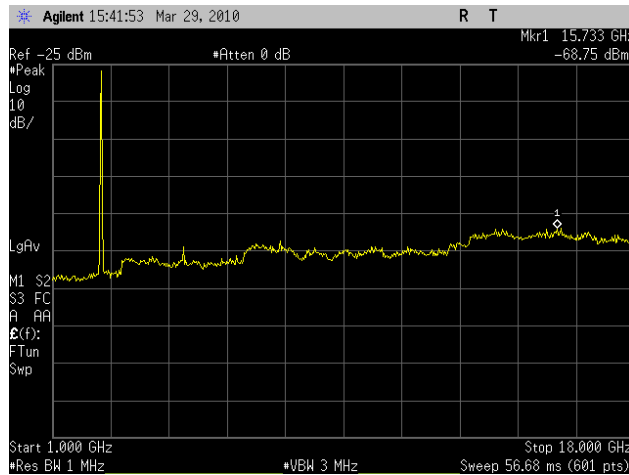
Plot 45. Radiated Spurious 2437MHz Low Channel 802.11n (1-18GHz)
