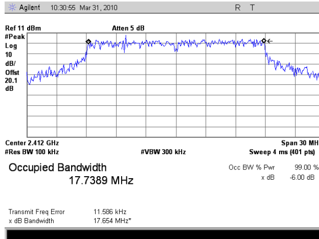
Plot 14. Occupied Band Width, 802.11n Mode, Low Channel, FCC, 6 dB
