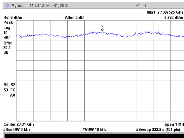
Plot 95. Power Spectral Density 2437MHz Mid Channel 802.11g
