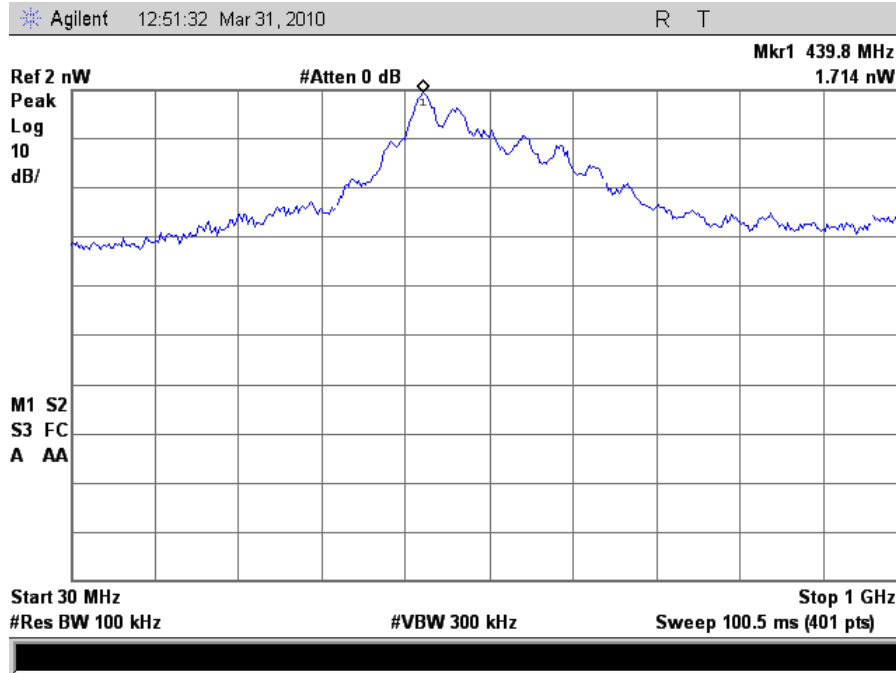
Plot 76. Receiver Spurious Emission, 30MHz – 1 GHz
