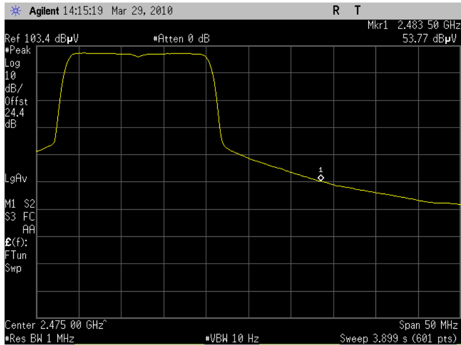
Plot 60. Radiated Band Edge 2462MHz Channel 11 802.11g (Average)
