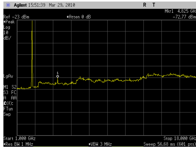
Plot 42. Radiated Spurious 2412MHz Low Channel 802.11g (1-18GHz)
