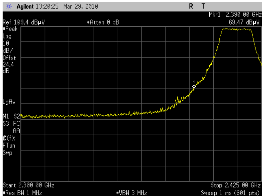
Plot 49. Radiated Band Edge 2412MHz Channel 1 802.11g (Peak)
