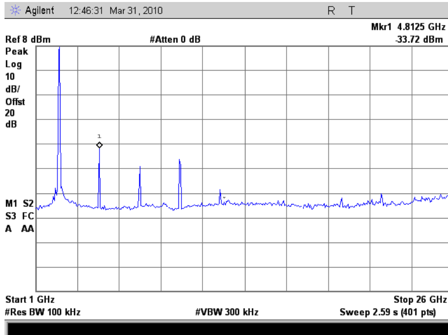
Plot 79. Conducted Spurious 2412MHz Low Channel 802.11g (1-26GHz)
