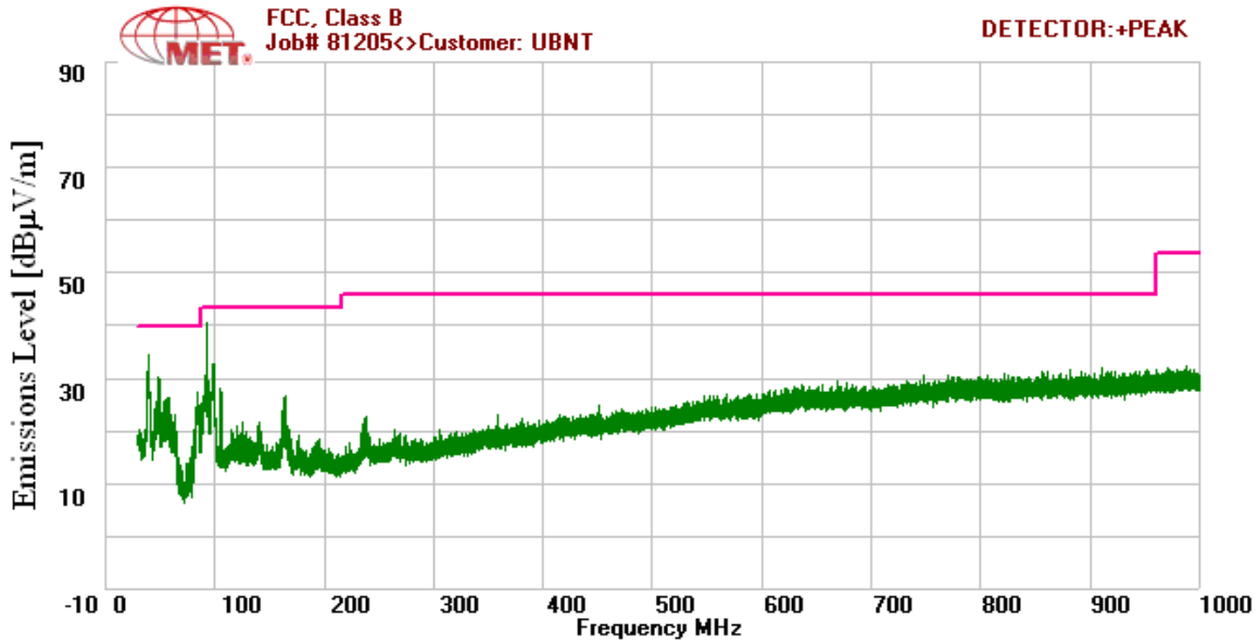
Plot 38. 15.209 Radiated Emissions 2462MHz High Channel 802.11g (30MHz – 1GHz)
