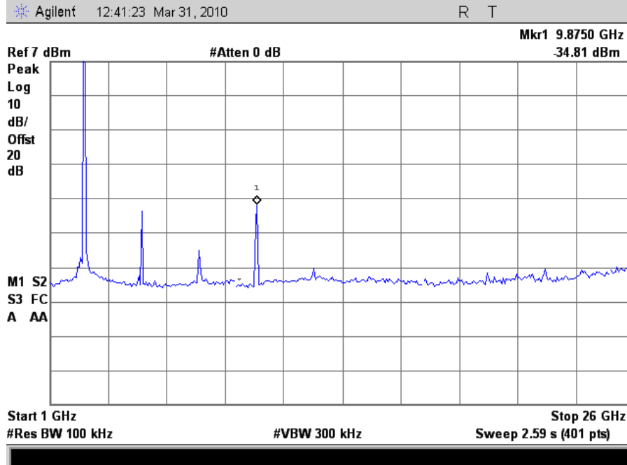
Plot 89. Conducted Spurious 2462MHz High Channel 802.11n (1-26GHz)
