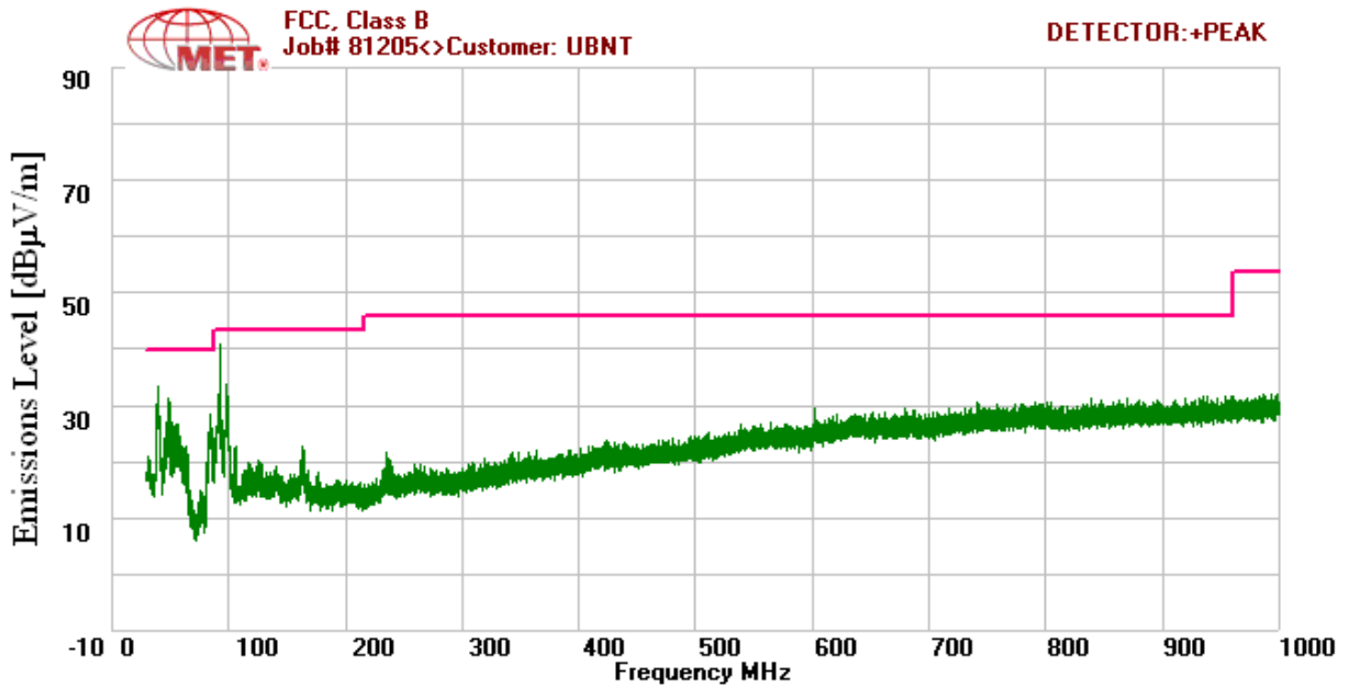
Plot 37. 15.209 Radiated Emissions 2437MHz Mid Channel 802.11g (30MHz – 1GHz)
