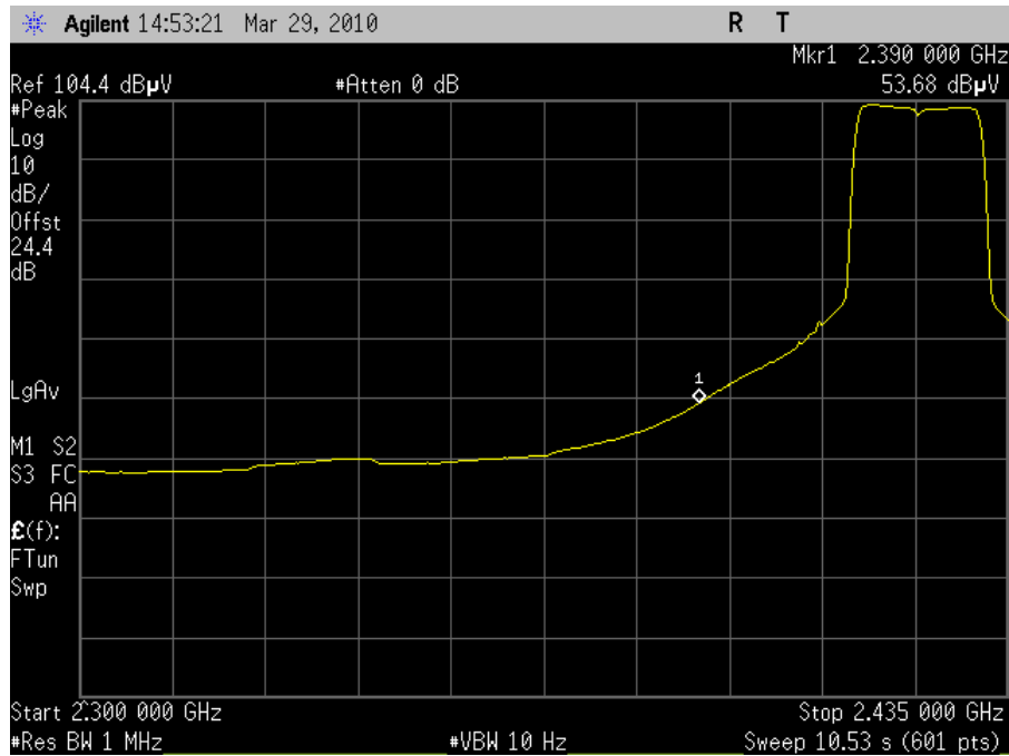
Plot 66. Radiated Band Edge 2422MHz Channel 3 802.11n (Average)
