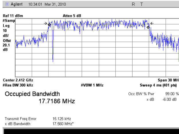
Plot 17. Occupied Band Width, 802.11n Mode, Low Channel, 99 % OBW
