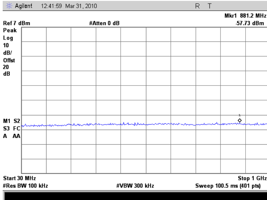
Plot 88. Conducted Spurious 2462MHz High Channel 802.11n (30MHz-1GHz)
