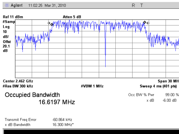
Plot 13. Occupied Band Width, 802.11g Mode, High Channel, 99 % OBW
