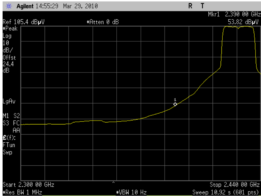
Plot 68. Radiated Band Edge 2427MHz Channel 4 802.11n (Average)
