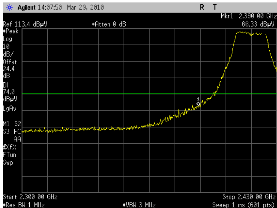
Plot 51. Radiated Band Edge 2417MHz Channel 2 802.11g (Peak)
