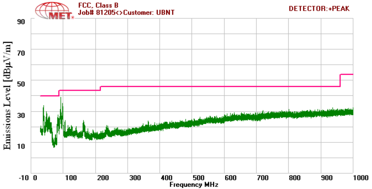
Plot 41. 15.209 Radiated Emissions 2462MHz High Channel 802.11n (30MHz – 1GHz)
