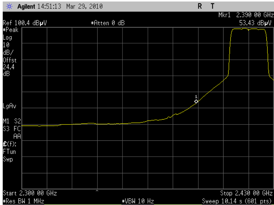
Plot 64. Radiated Band Edge 2417MHz Channel 2 802.11n (Average)
