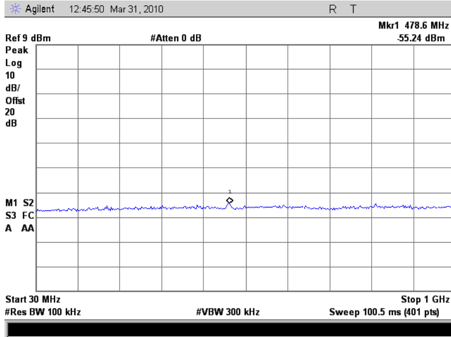
Plot 80. Conducted Spurious 2437MHz Mid Channel 802.11g (30MHz-1GHz)
