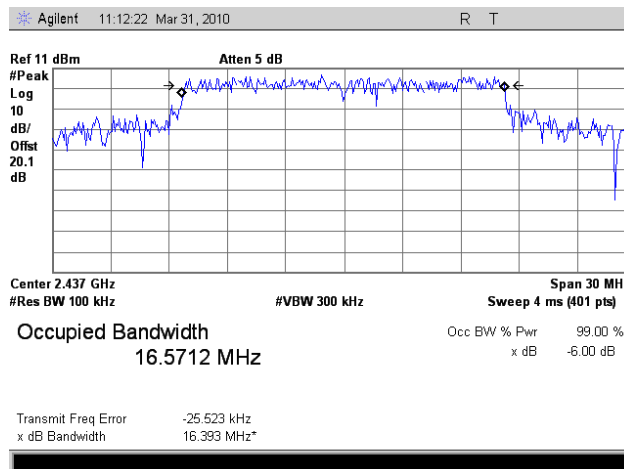
Plot 9. Occupied Band Width, 802.11g Mode, Mid Channel, FCC, 6 dB
