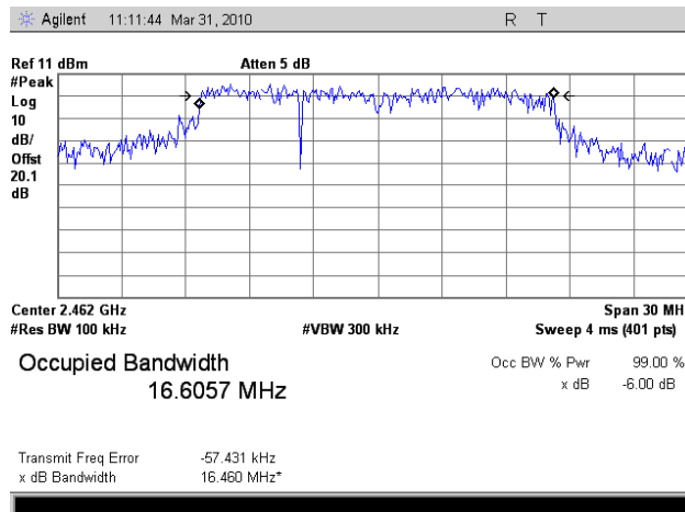
Plot 10. Occupied Band Width, 802.11g Mode, High Channel, FCC, 6 dB
