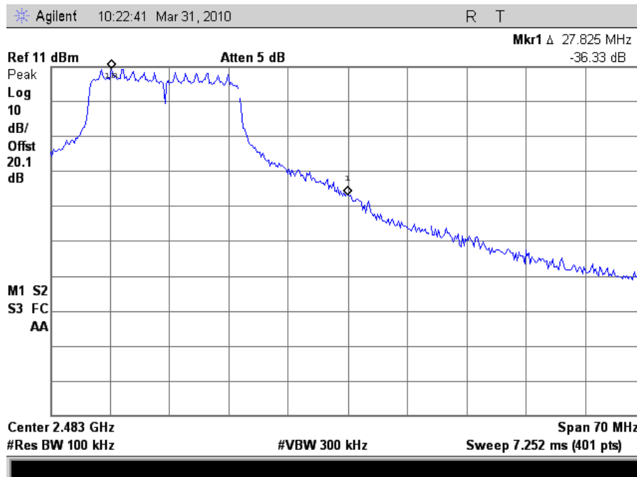
Plot 93. Conducted Band Edge 2462MHz High Channel 802.11n
