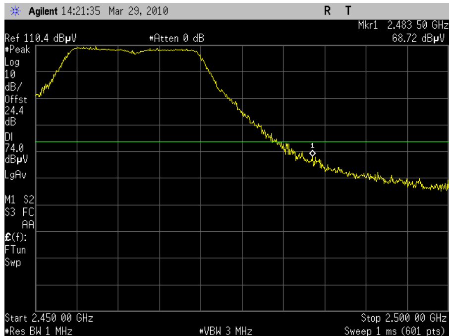
Plot 61. Radiated Band Edge 2462MHz Channel 11 802.11g (Peak)
