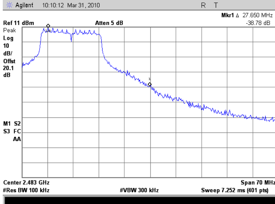
Plot 91. Conducted Band Edge 2462MHz High Channel 802.11g
