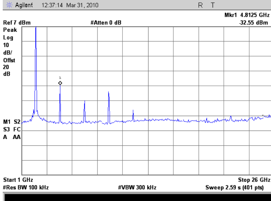
Plot 85. Conducted Spurious 2412MHz Low Channel 802.11n (1-26GHz)
