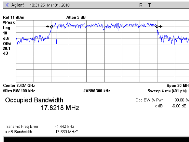
Plot 15. Occupied Band Width, 802.11n Mode, Mid Channel, FCC, 6 dB
