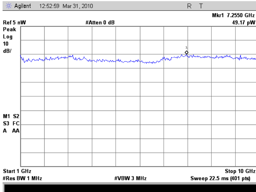
Plot 77. Receiver Spurious Emission, 1 GHz – 10 GHz
