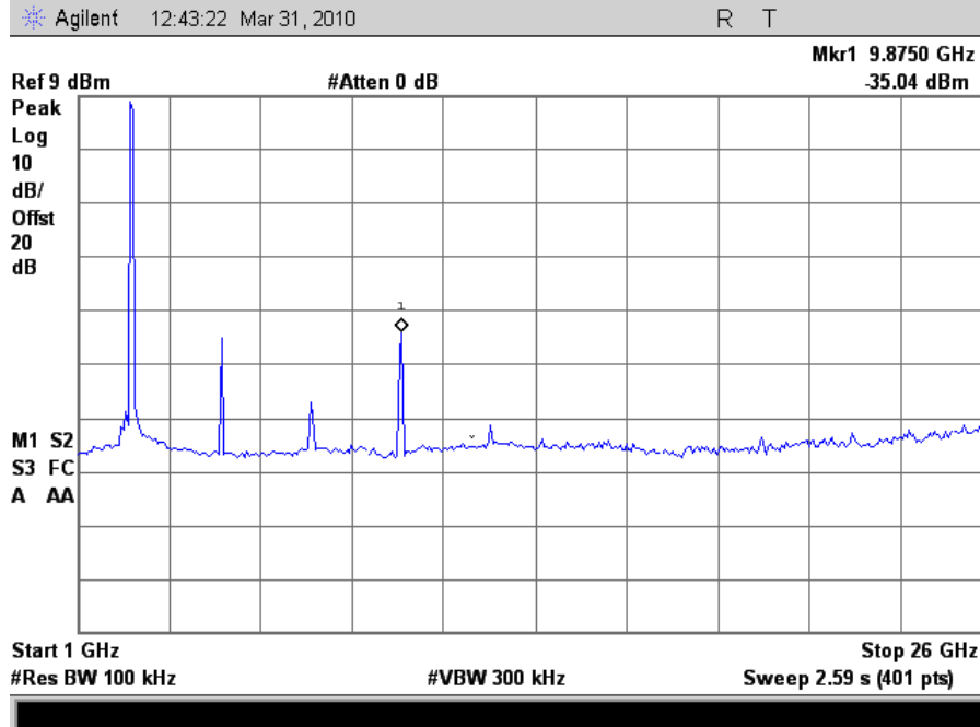
Plot 83. Conducted Spurious 2462MHz High Channel 802.11g (1-26GHz)
