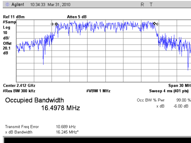
Plot 11. Occupied Band Width, 802.11g Mode, Low Channel, 99 % OBW
