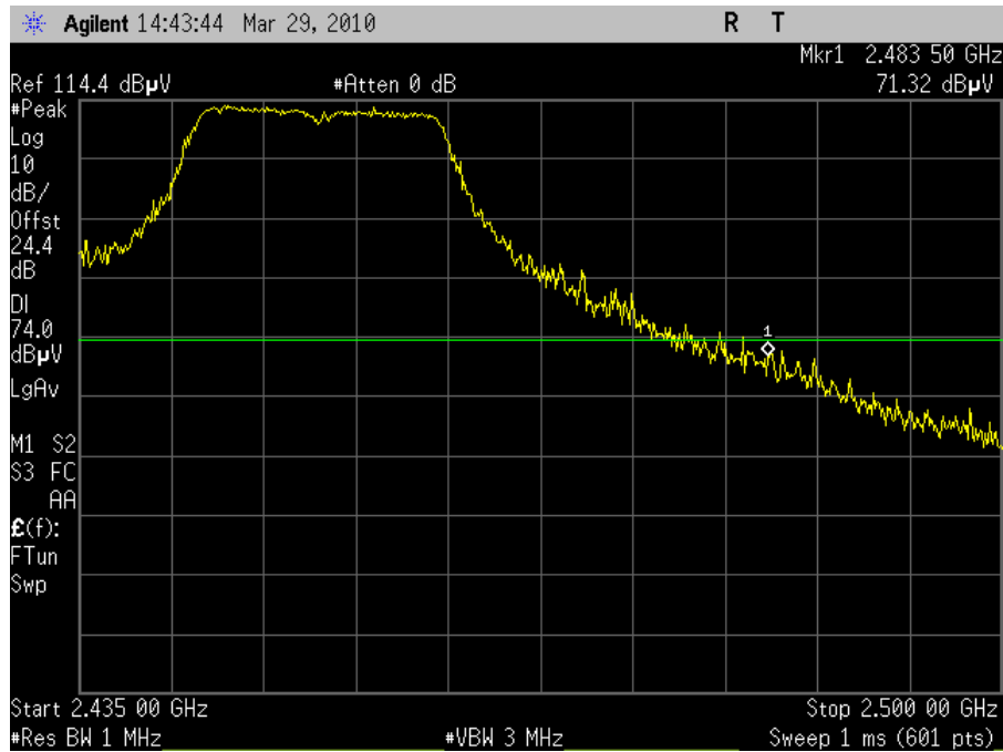
Plot 70. Radiated Band Edge 2462MHz Channel 9 802.11n (Average)
