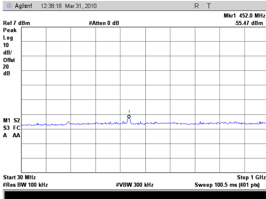
Plot 84. Conducted Spurious 2412MHz Low Channel 802.11n (30MHz-1GHz)
