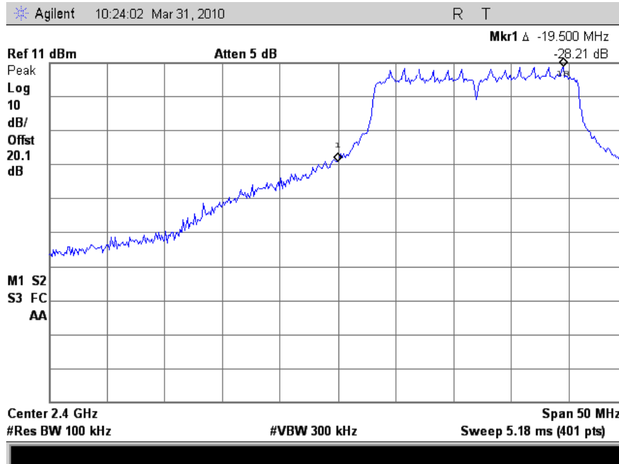
Plot 92. Conducted Band Edge 2412MHz Low Channel 802.11n
