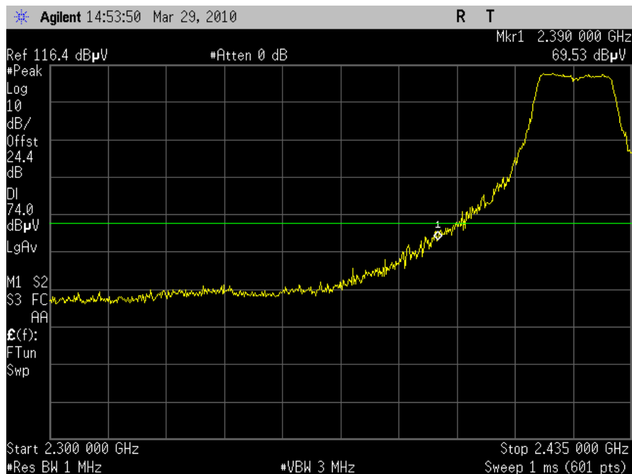
Plot 67. Radiated Band Edge 2422MHz Channel 3 802.11n (Peak)
