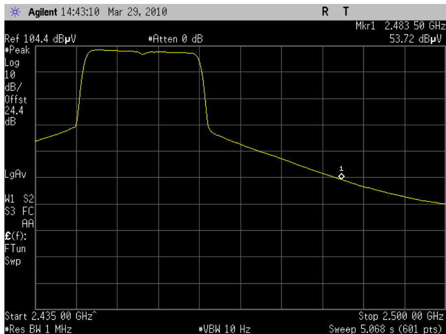
Plot 71. Radiated Band Edge 2462MHz Channel 9 802.11n (Peak)
