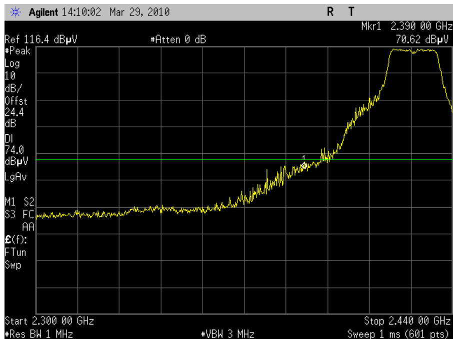
Plot 55. Radiated Band Edge 2427MHz Channel 4 802.11g (Peak)
