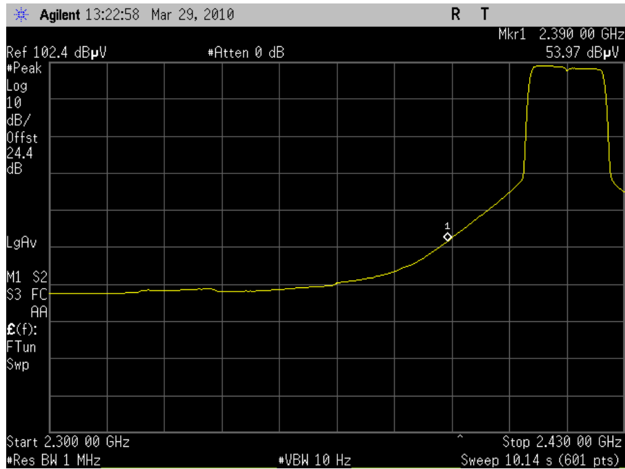
Plot 50. Radiated Band Edge 2417MHz Channel 2 802.11g (Average)
