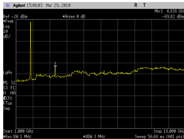
Plot 44. Radiated Spurious 2462MHz High Channel 802.11g (1-18GHz)
