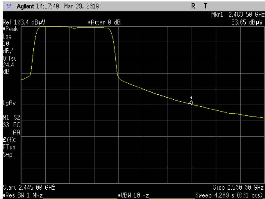
Plot 58. Radiated Band Edge 2462MHz Channel 10 802.11g (Average)
