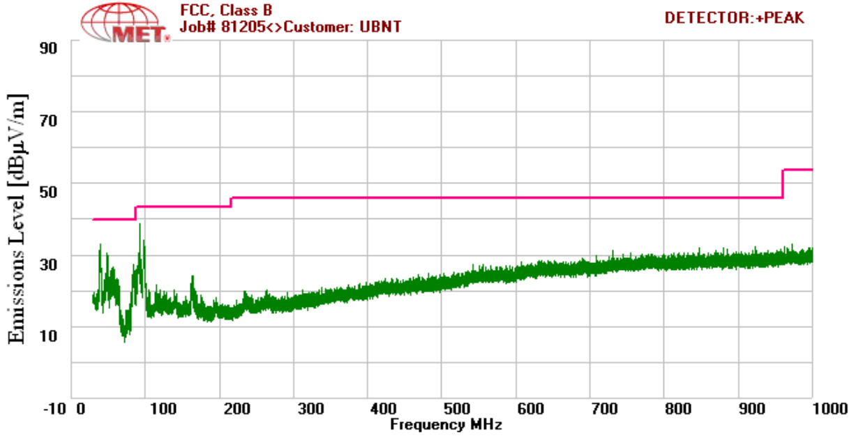
Plot 40. 15.209 Radiated Emissions 2437MHz Mid Channel 802.11n (30MHz – 1GHz)
