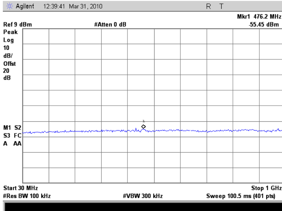
Plot 86. Conducted Spurious 2437MHz Mid Channel 802.11n (30MHz-1GHz)
