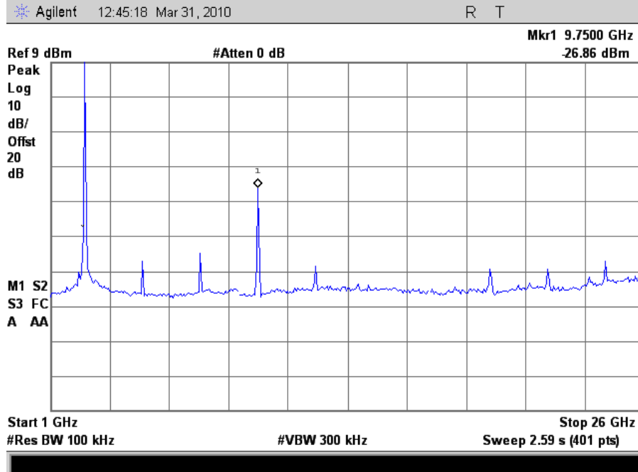
Plot 81. Conducted Spurious 2437MHz Mid Channel 802.11g (1-26GHz)
