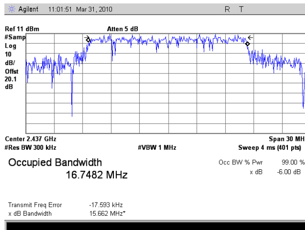
Plot 12. Occupied Band Width, 802.11g Mode, Mid Channel, 99% OBW
