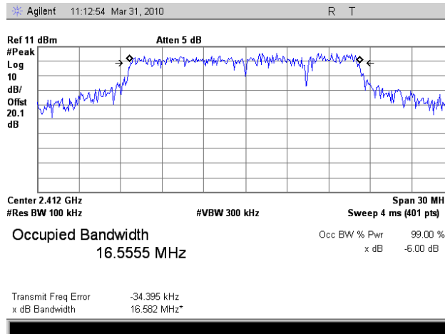
Plot 8. Occupied Band Width, 802.11g Mode, Low Channel, FCC, 6 dB
