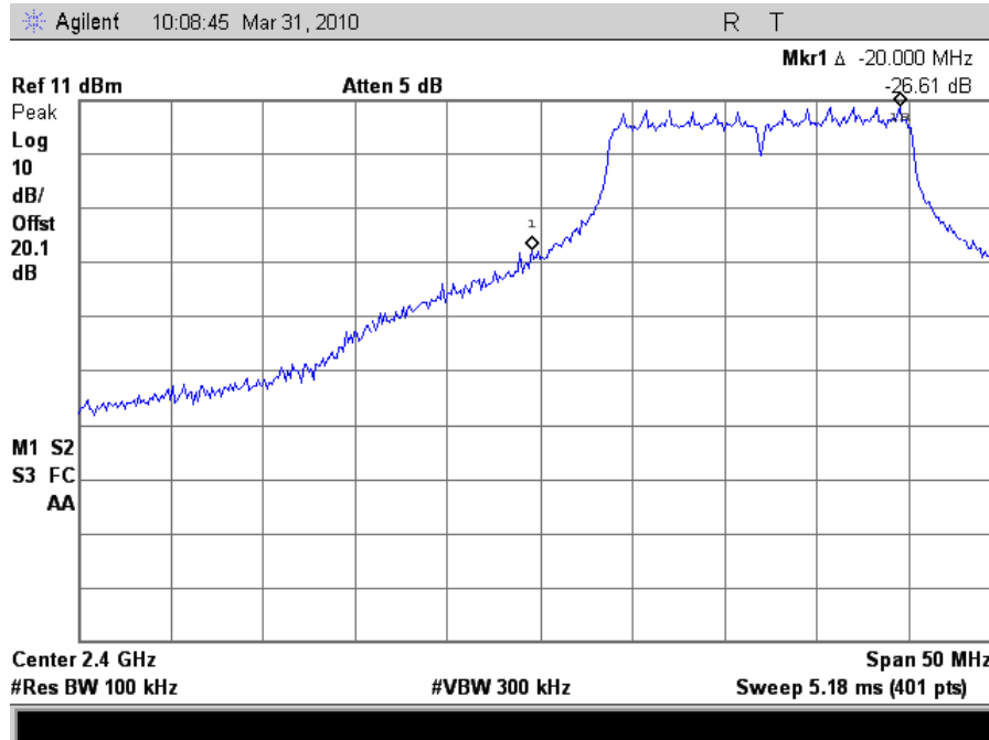
Plot 90. Conducted Band Edge 2412MHz Low Channel 802.11g
