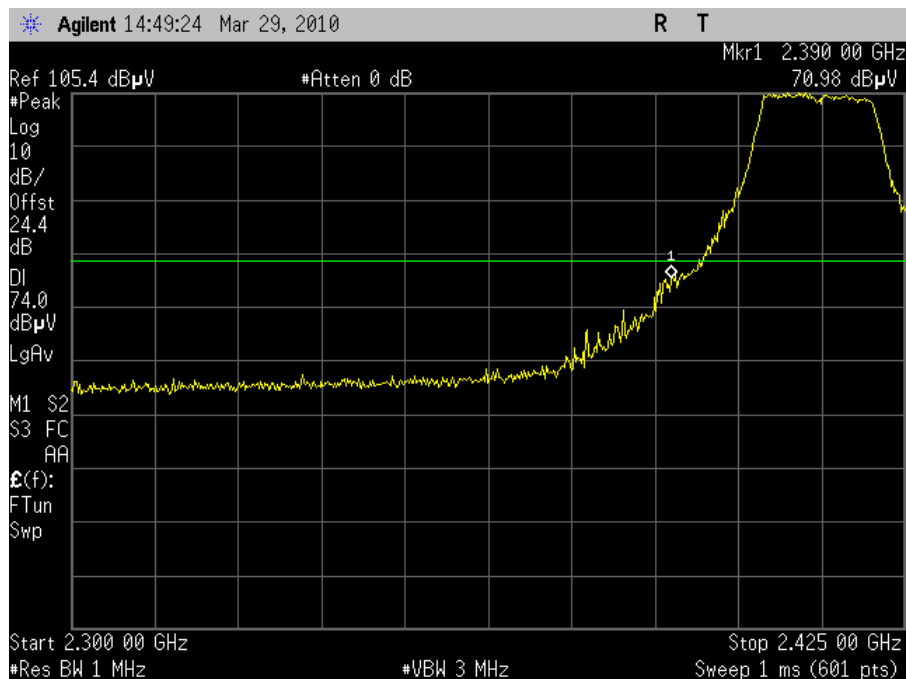
Plot 63. Radiated Band Edge 2412MHz Channel 1 802.11n (Peak)
