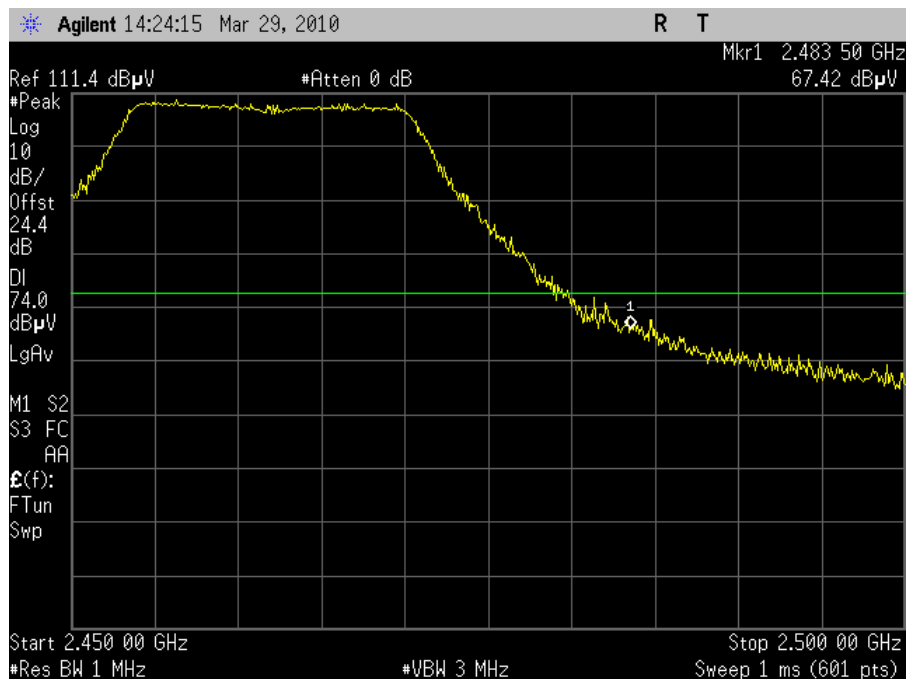
Plot 75. Radiated Band Edge 2462MHz Channel 11 802.11n (Peak)
