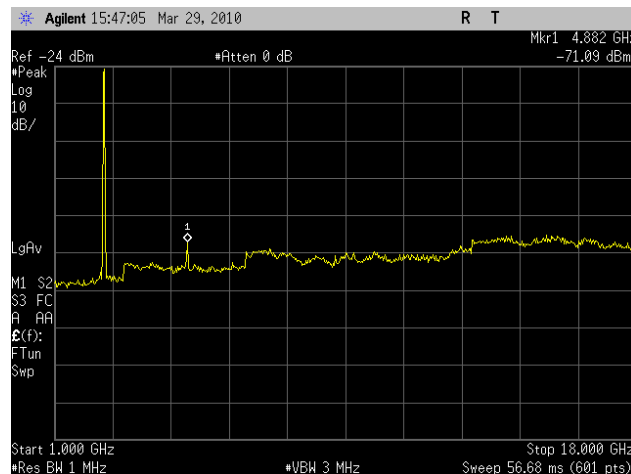
Plot 43. Radiated Spurious 2437MHz Mid Channel 802.11g (1-18GHz)
