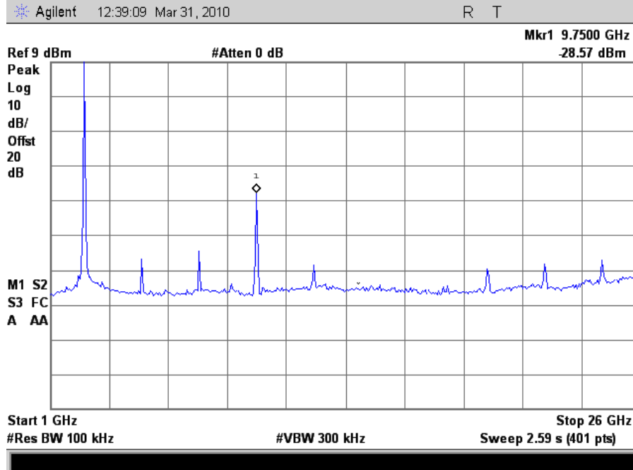
Plot 87. Conducted Spurious 2437MHz Mid Channel 802.11n (1-26GHz)
