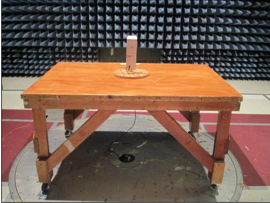
Photograph 9. Radiated Harmonic/Spurious Emissions, Test Setup
