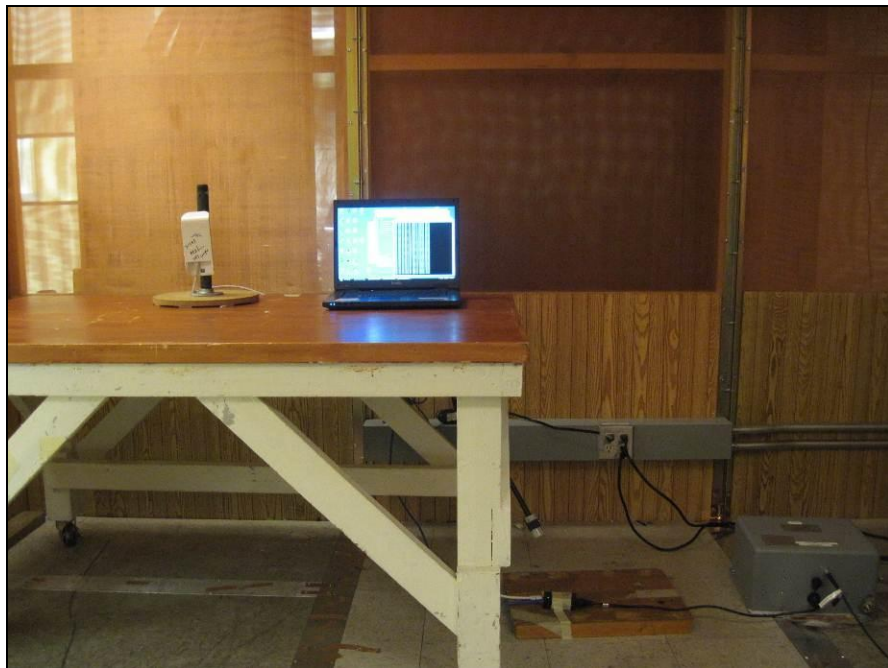
Photograph 4. Conducted Emissions, 15.207(a), Test Setup
