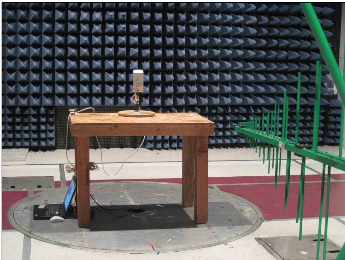
Photograph 2. Radiated Emission, Test Setup, CETUS
