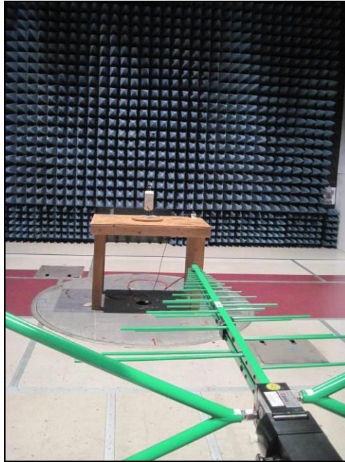
Photograph 3. Radiated Emission, Test Setup, GME
