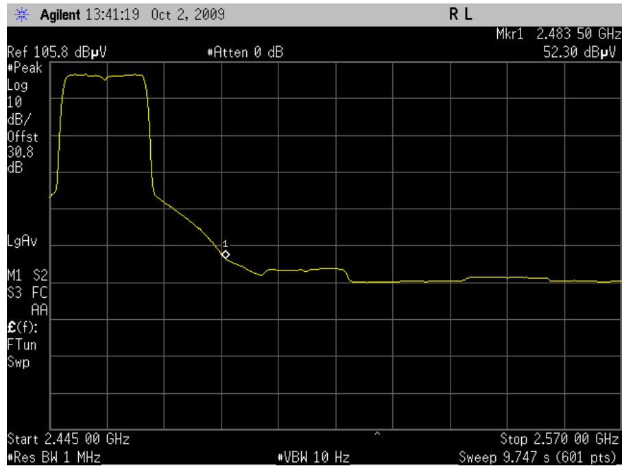
Plot 76. Channel 10 Upper Band Edge, Average - HT20 (Dish Antenna)
