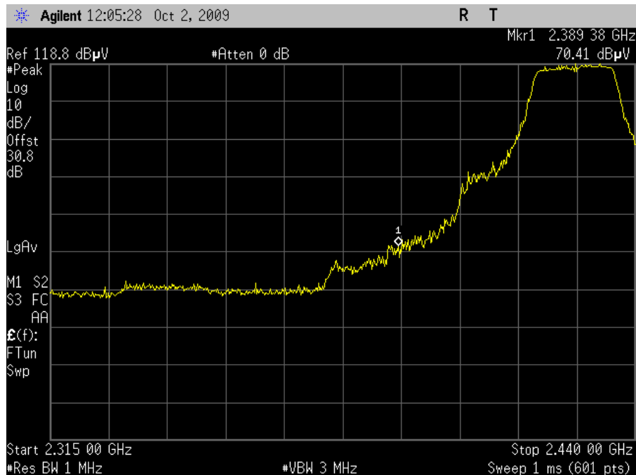
Plot 55. Channel 4 Lower Band Edge, Peak – HT20 (Dish Antenna)
