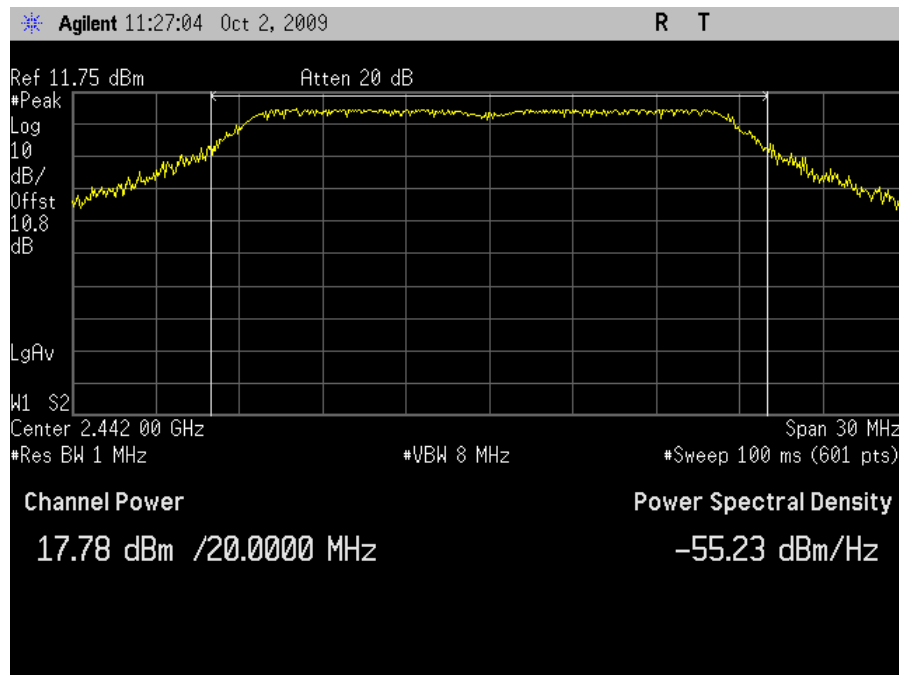
Plot 33. Peak Output Power, HT20 Channel 7 - Grid Antenna
