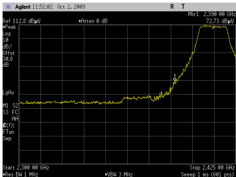
Plot 49. Channel 1 Lower Band Edge, Peak – HT20 (Dish Antenna)
