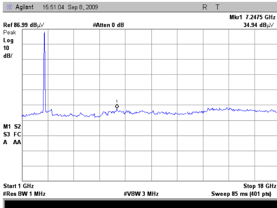
Plot 44. Radiated Spurious Emissions, Mid Channel, HT20 (Grid Antenna)
