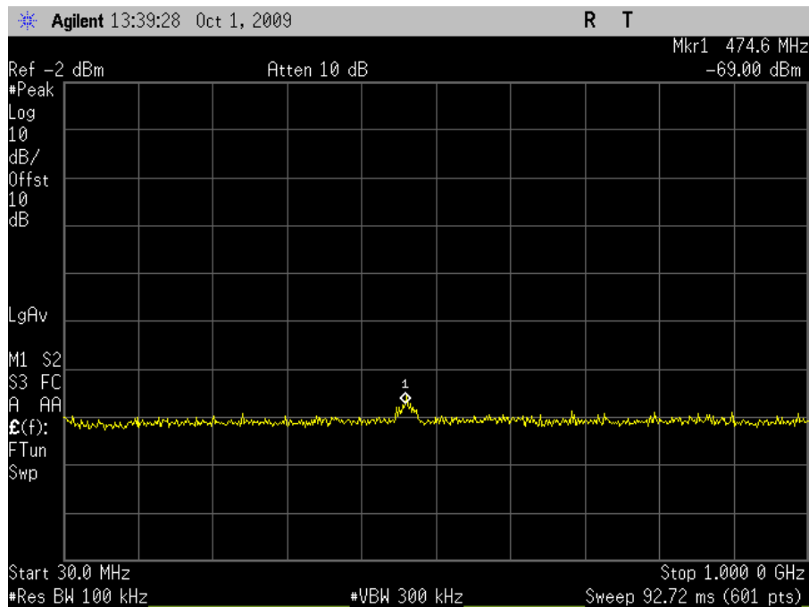
Plot 131. Conducted Emissions, Mid Channel, 30 MHz – 1 GHz (HT40)
