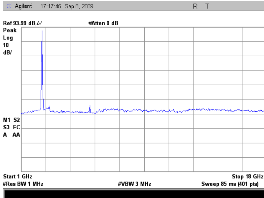
Plot 40. Radiated Spurious Emissions, Low Channel, HT20 (Dish Antenna)
