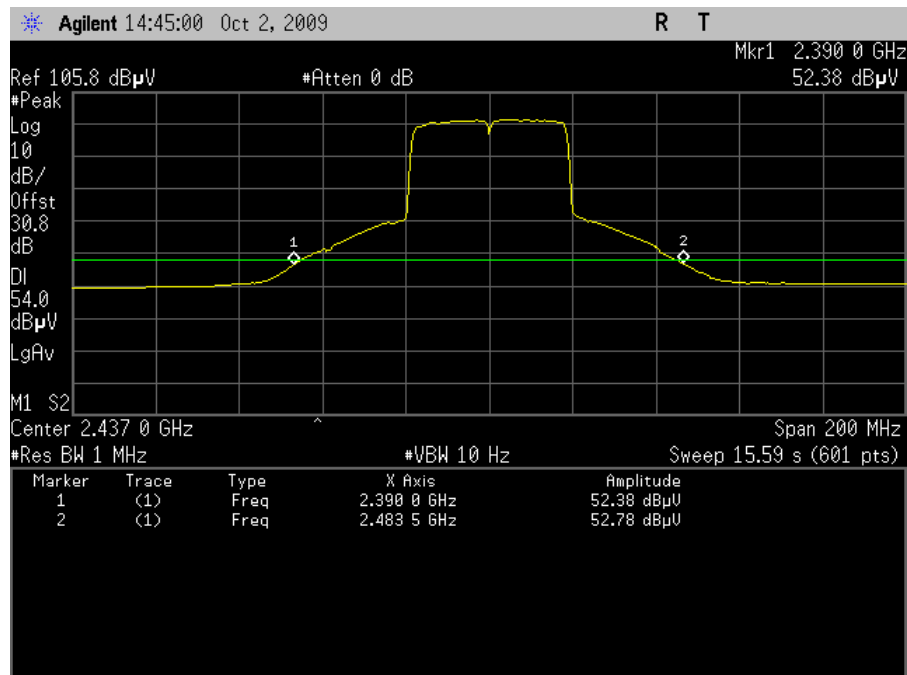
Plot 114. Band Edge, Average 200MHz Span – HT40 (Dish Antenna)
