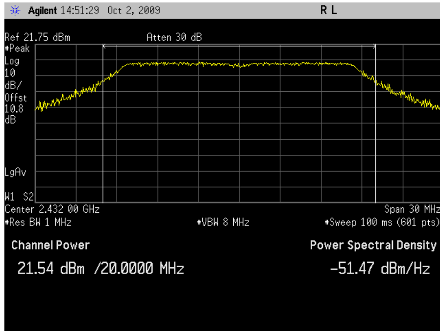
Plot 20. Peak Output Power, HT20 Channel 5 - Dish Antenna
