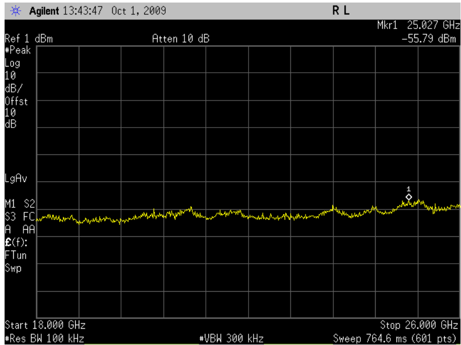
Plot 124. Conducted Emissions, Low Channel, 18 GHz – 26 GHz (HT20)
