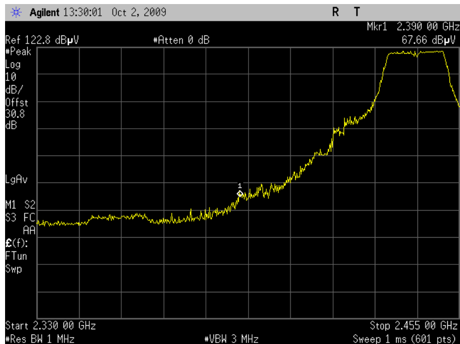
Plot 61. Channel 7 Lower Band Edge, Peak – HT20 (Dish Antenna)
