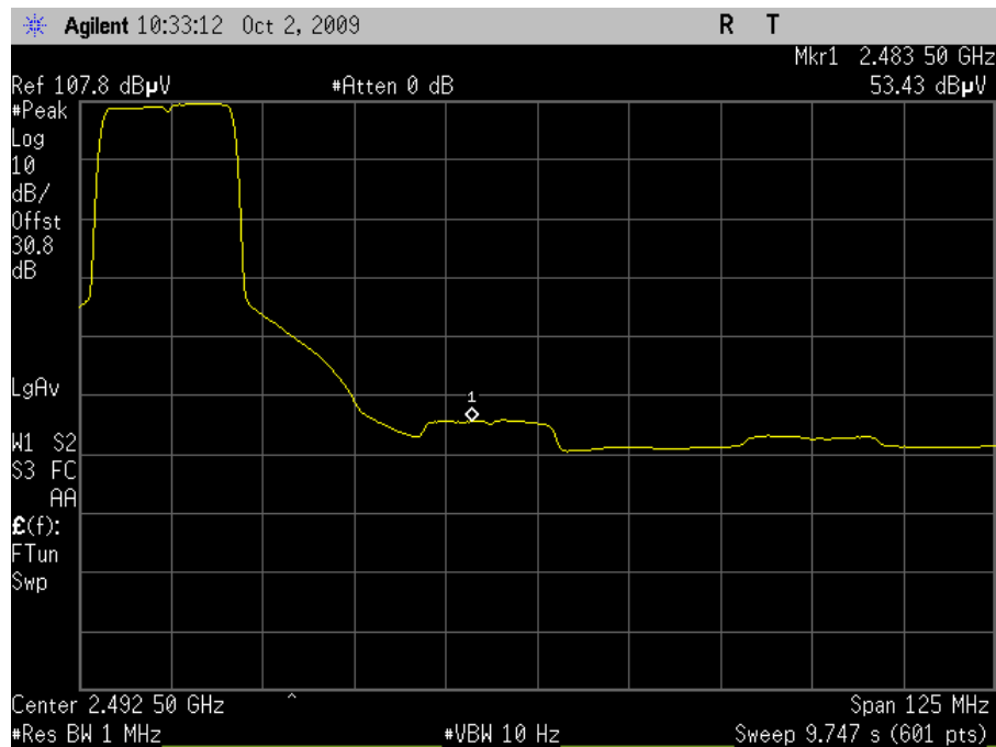
Plot 102. Channel 7 Upper Band Edge, Average - HT20 (Grid Antenna)
