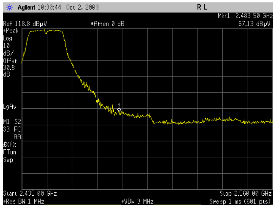
Plot 105. Channel 8 Upper Band Edge, Peak – HT20 (Grid Antenna)
