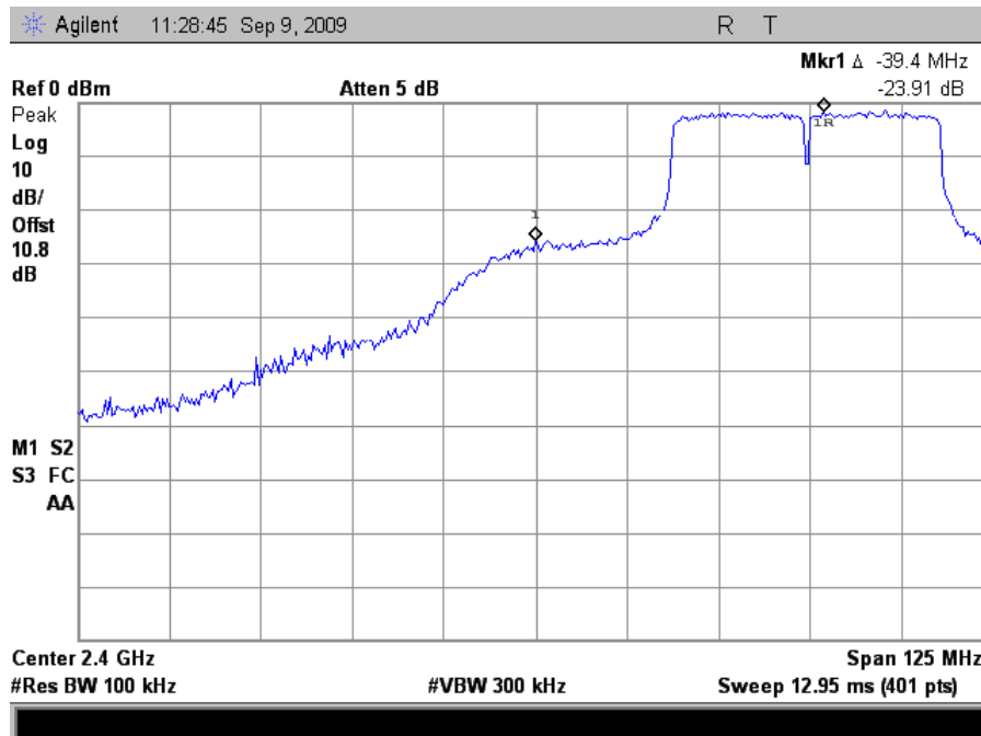
Plot 137. Conducted Band Edge, Low Channel HT40
