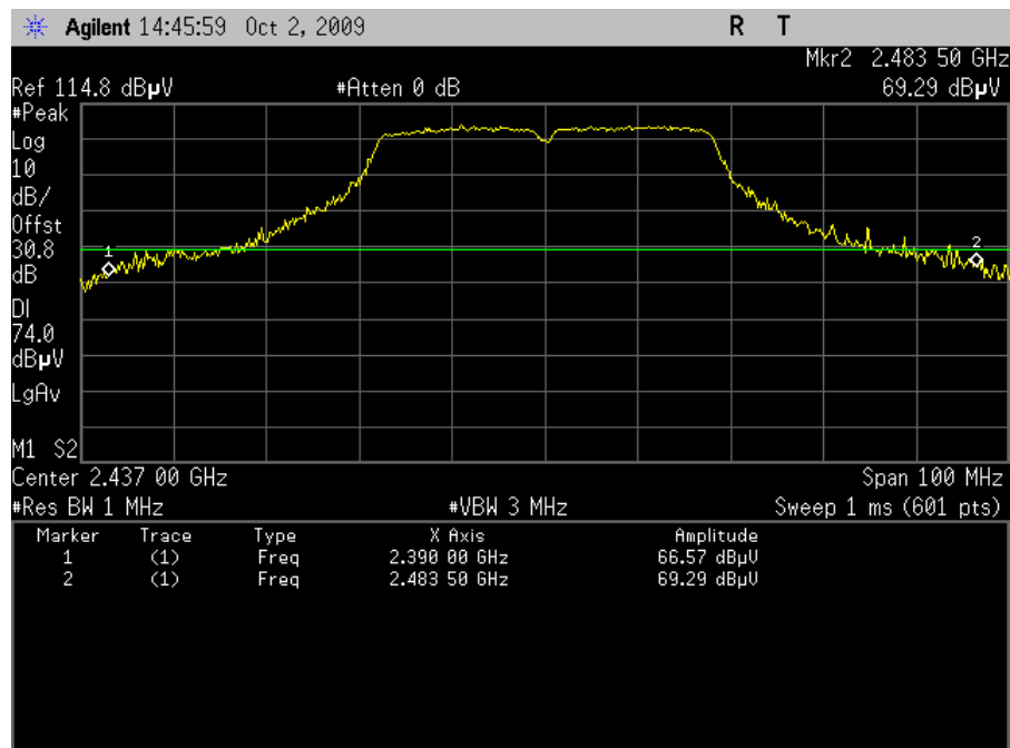
Plot 113. Band Edge, Peak 100MHz Span – HT40 (Dish Antenna)
