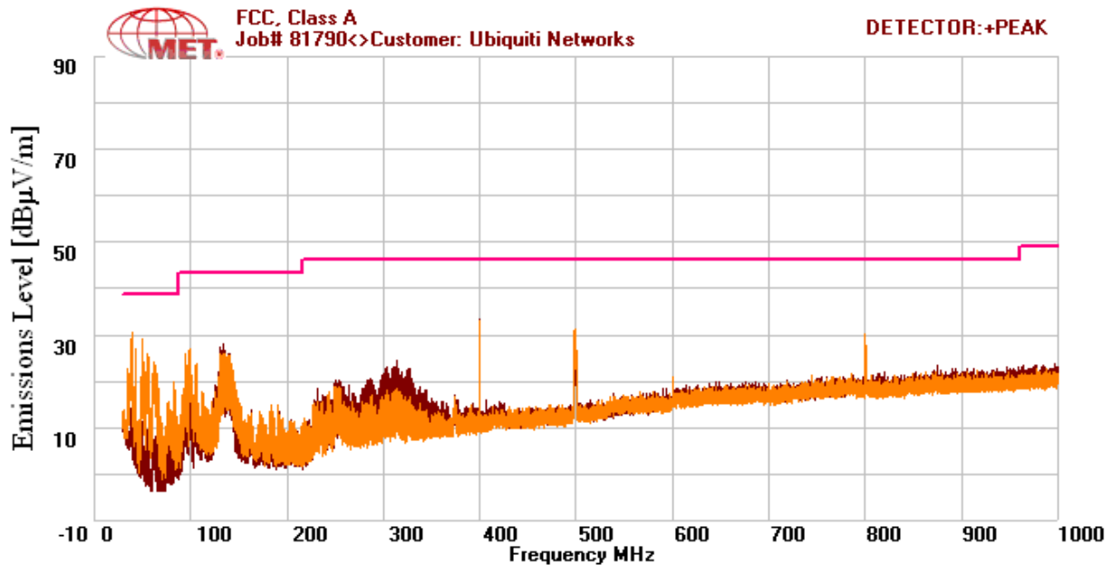
Plot 3. Radiated Emission Limits for FCC Part 15 Subpart B
