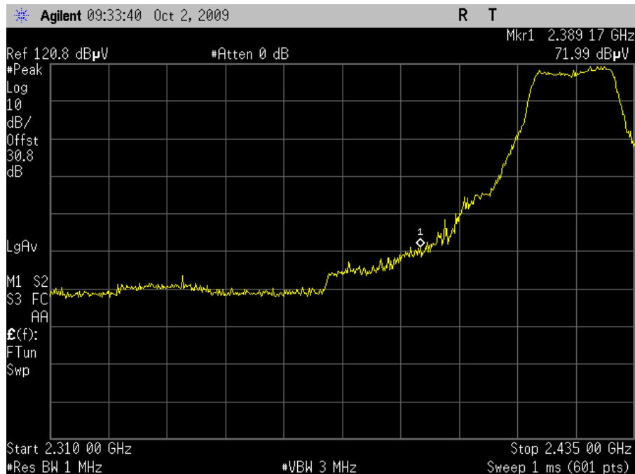
Plot 85. Channel 3 Lower Band Edge, Peak – HT20 (Grid Antenna)
