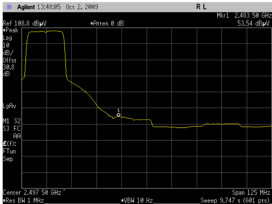
Plot 72. Channel 8 Upper Band Edge, Average - HT20 (Dish Antenna)
