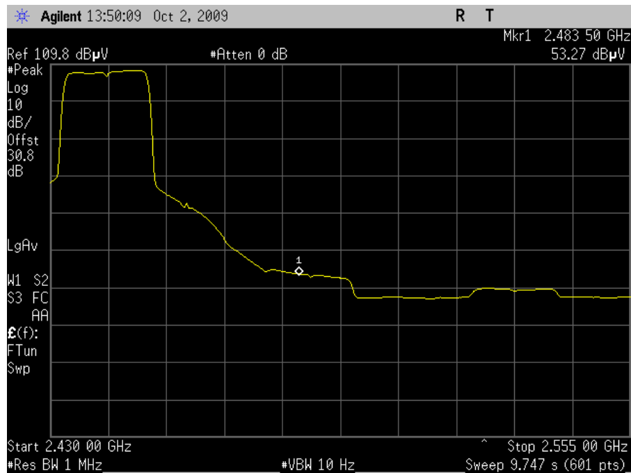
Plot 70. Channel 7 Upper Band Edge, Average - HT20 (Dish Antenna)
