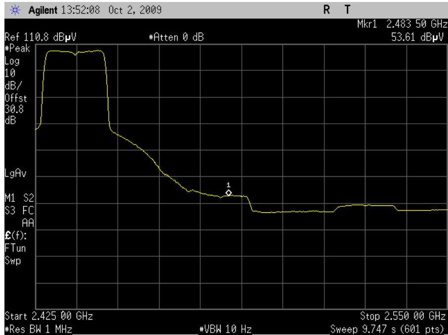
Plot 68. Channel 6 Upper Band Edge, Average - HT20 (Dish Antenna)
