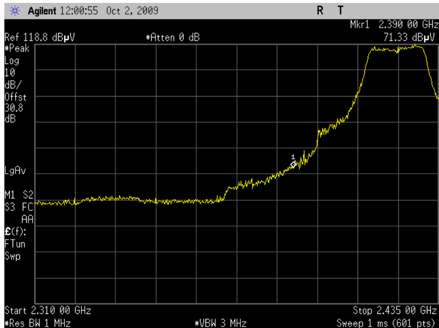
Plot 53. Channel 3 Lower Band Edge, Peak – HT20 (Dish Antenna)
