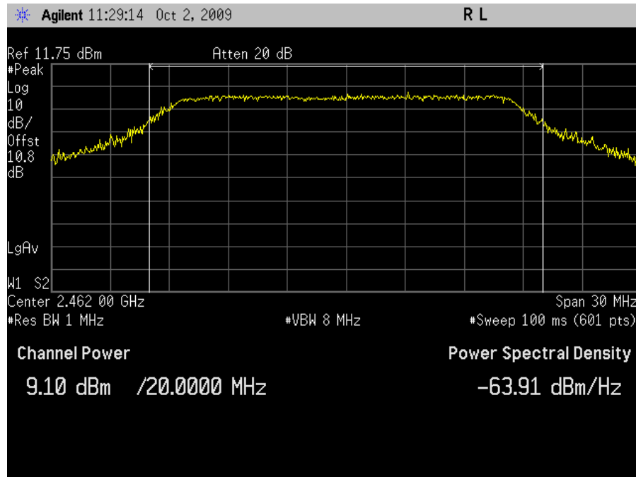
Plot 37. Peak Output Power, HT20 Channel 11 - Grid Antenna
