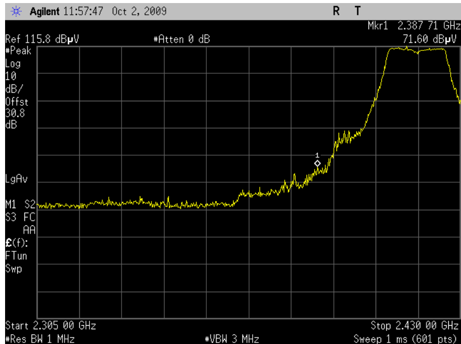
Plot 51. Channel 2 Lower Band Edge, Peak – HT20 (Dish Antenna)
