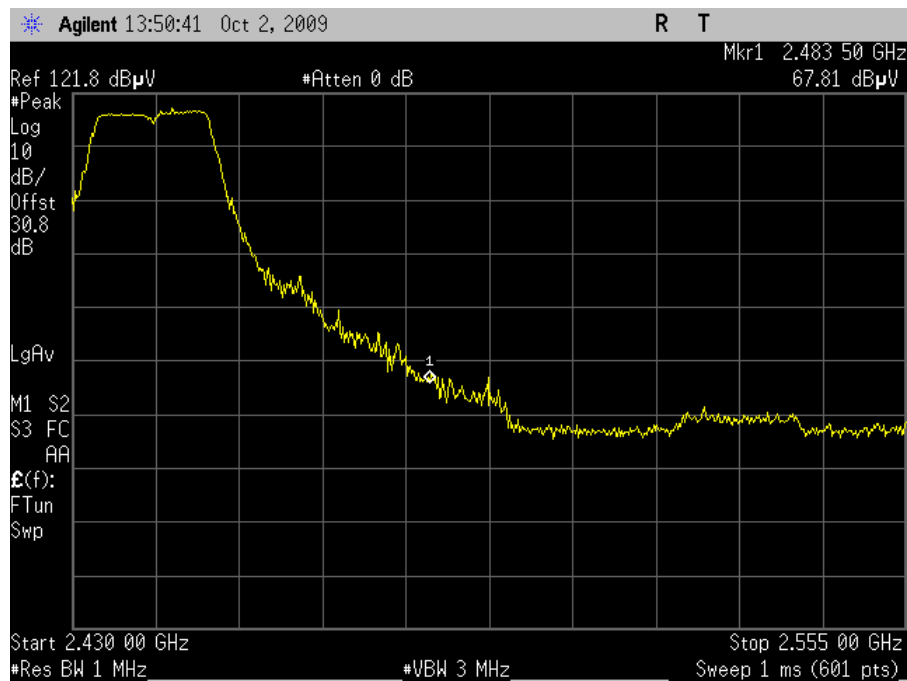
Plot 71. Channel 7 Upper Band Edge, Peak – HT20 (Dish Antenna)
