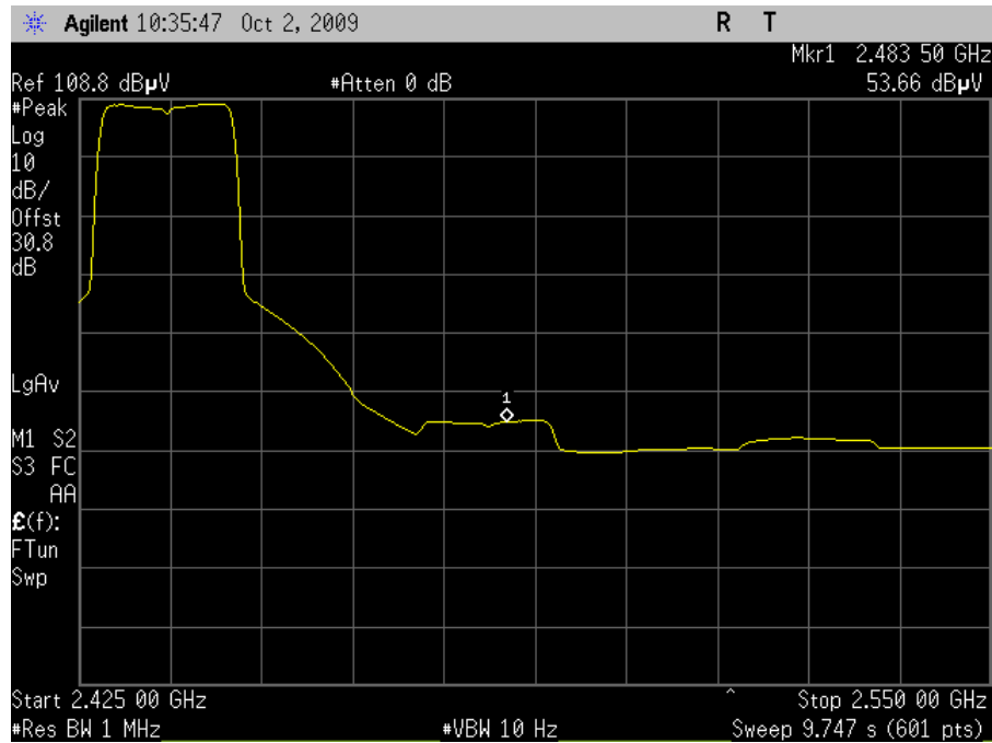
Plot 100. Channel 6 Upper Band Edge, Average - HT20 (Grid Antenna)
