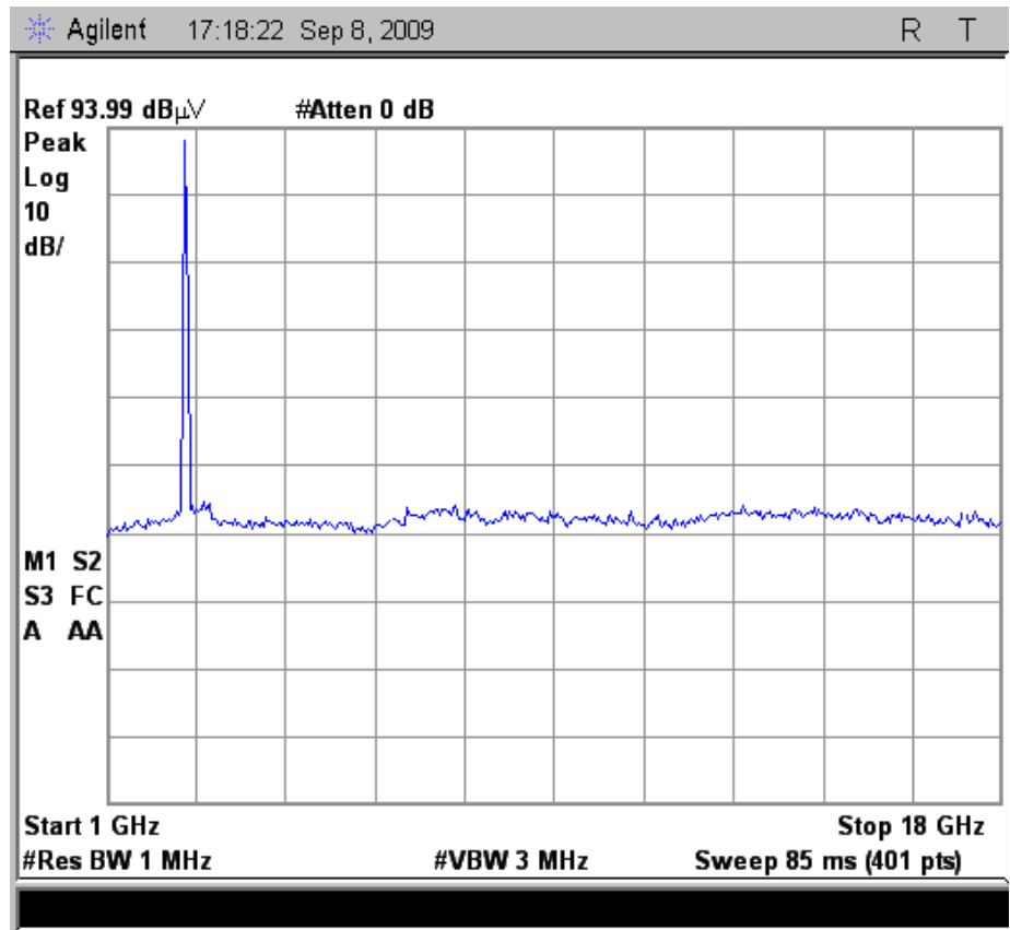
Plot 42. Radiated Spurious Emissions, High Channel, HT20 (Dish Antenna)
