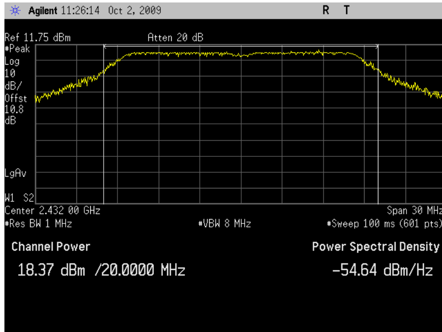
Plot 31. Peak Output Power, HT20 Channel 5 - Grid Antenna
