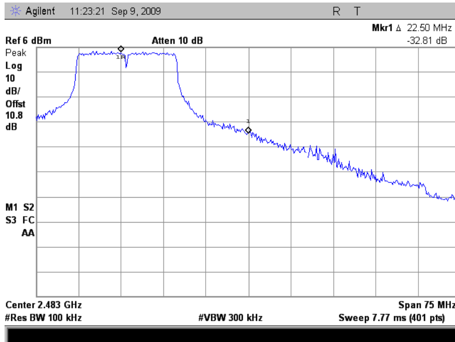
Plot 134. Conducted Band Edge, High Channel HT20
