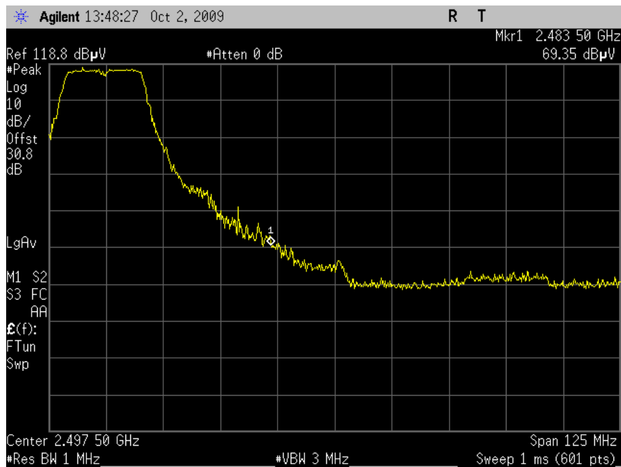
Plot 73. Channel 8 Upper Band Edge, Peak – HT20 (Dish Antenna)
