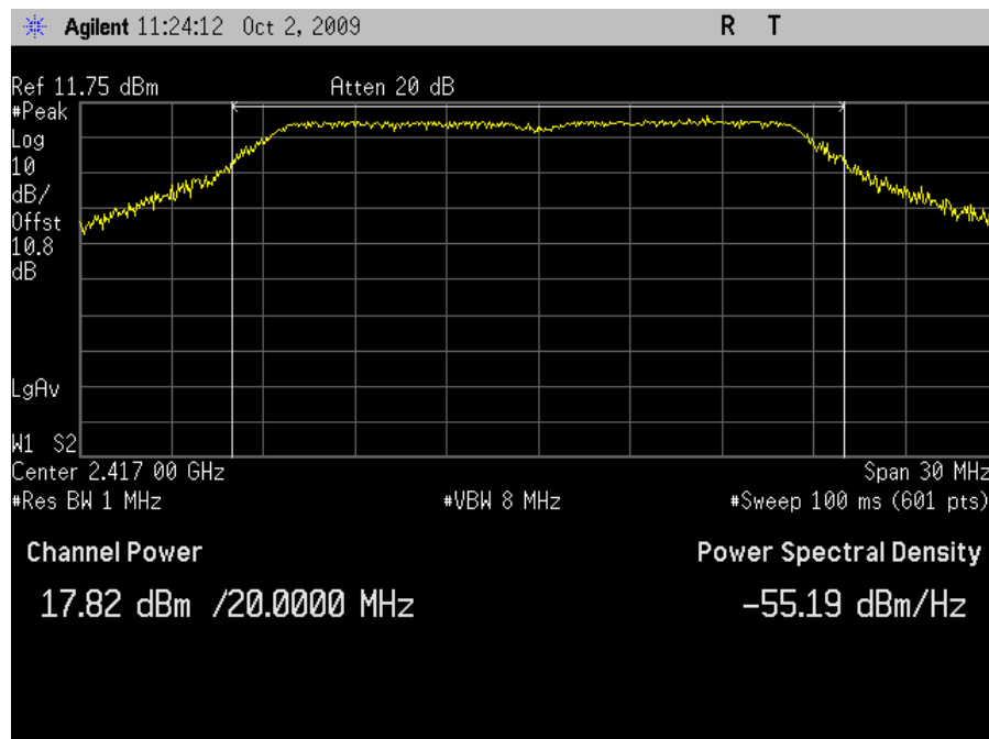
Plot 28. Peak Output Power, HT20 Channel 2 - Grid Antenna
