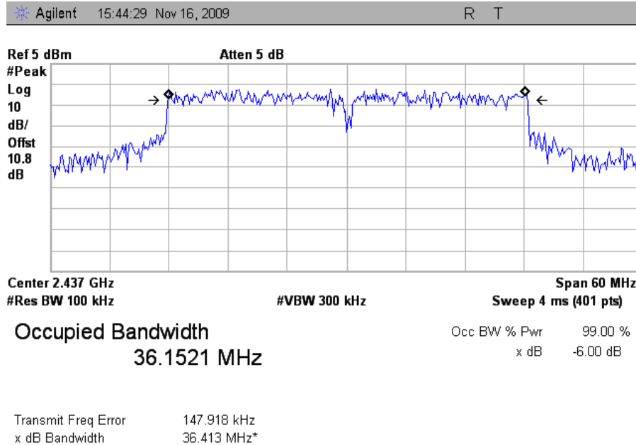
Plot 14. Occupied Band Width, Mid Channel, HT40
