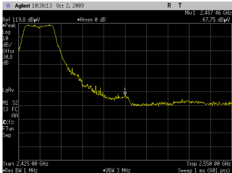
Plot 101. Channel 6 Upper Band Edge, Peak – HT20 (Grid Antenna)
