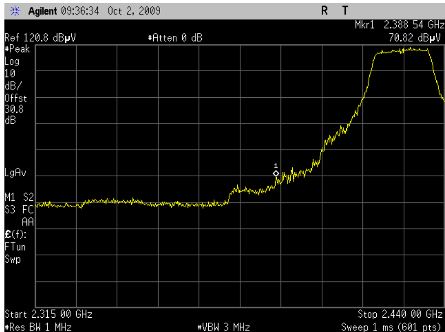
Plot 87. Channel 4 Lower Band Edge, Peak – HT20 (Grid Antenna)
