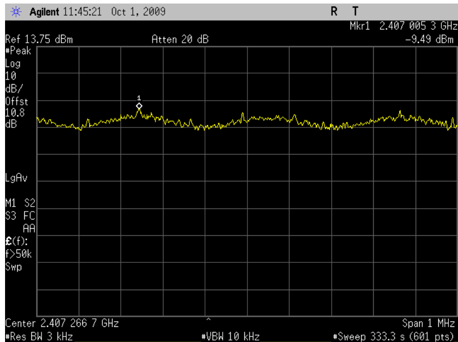
Plot 138. Peak Power Spectral Density, Low Channel HT20
