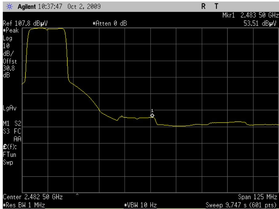
Plot 98. Channel 5 Upper Band Edge, Average - HT20 (Grid Antenna)
