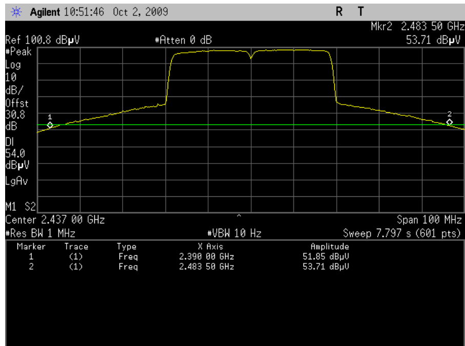
Plot 116. Band Edge, Average 100MHz Span – HT40 (Grid Antenna)
