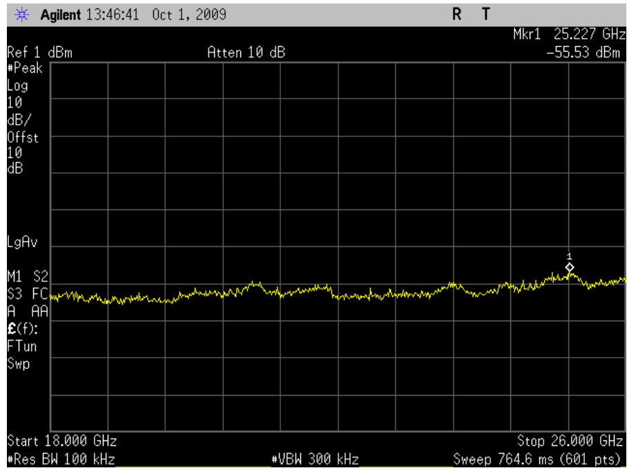
Plot 130. Conducted Emissions, High Channel, 18 GHz – 26 GHz (HT20)
