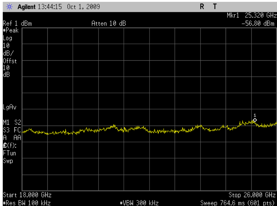
Plot 127. Conducted Emissions, Mid Channel, 18 GHz – 26 GHz (HT20)
