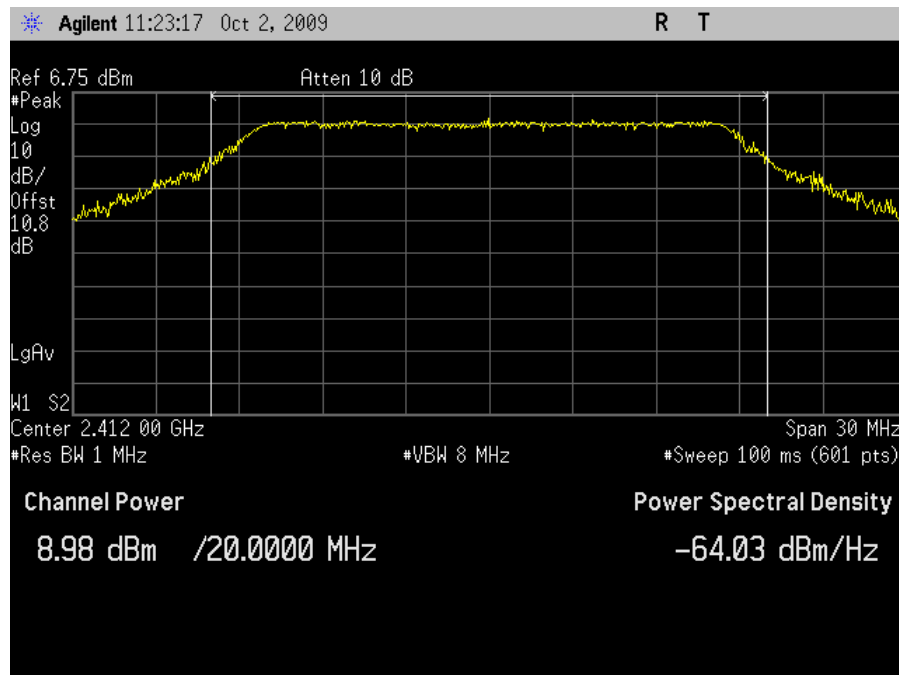
Plot 27. Peak Output Power, HT20 Channel 1 - Grid Antenna
