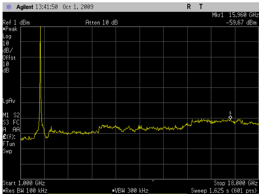
Plot 123. Conducted Emissions, Low Channel, 1 GHz – 18 GHz (HT20)
