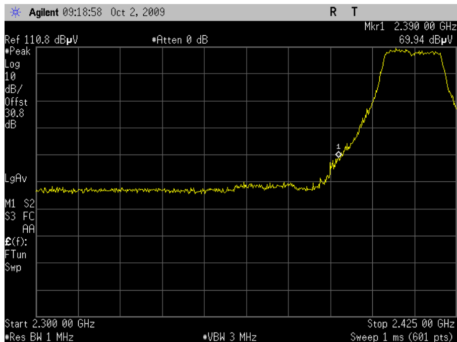
Plot 81. Channel 1 Lower Band Edge, Peak – HT20 (Grid Antenna)
