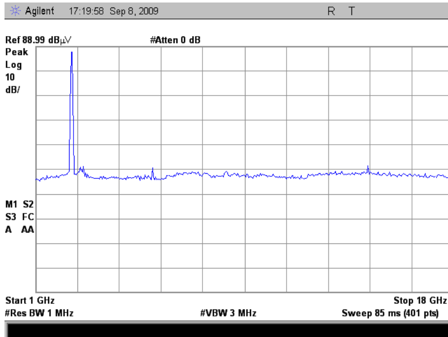
Plot 46. Radiated Spurious Emissions, Mid Channel, HT40 (Dish Antenna)
