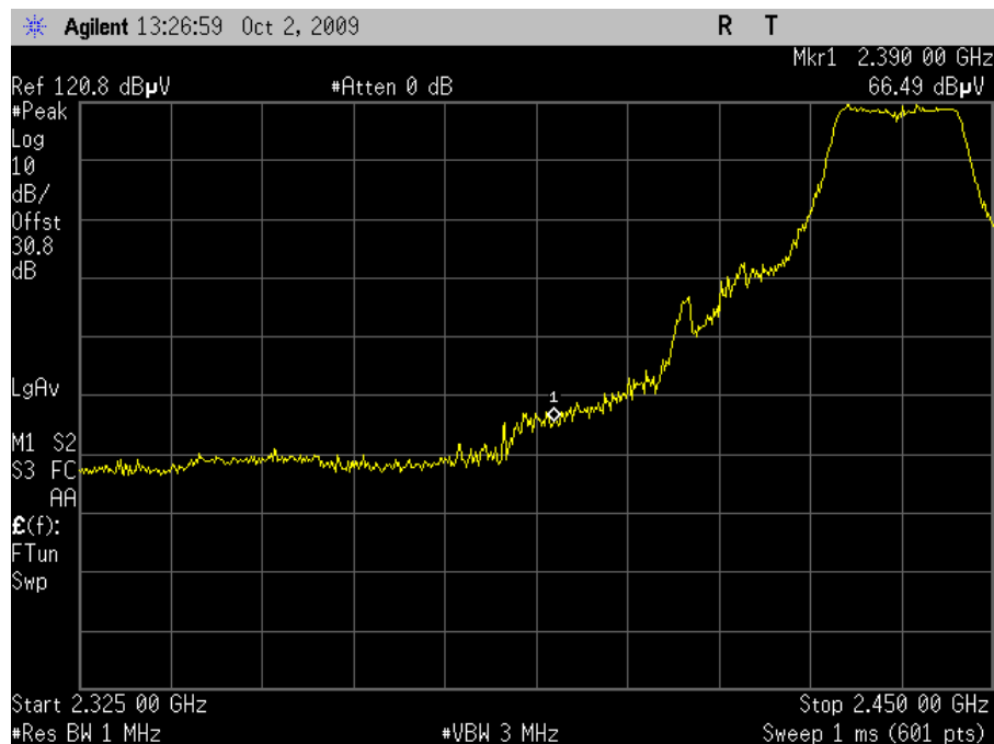
Plot 59. Channel 6 Lower Band Edge, Peak – HT20 (Dish Antenna)
