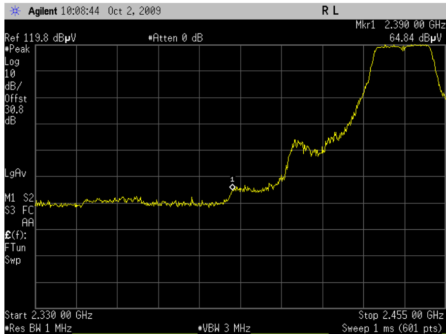
Plot 93. Channel 7 Lower Band Edge, Peak – HT20 (Grid Antenna)
