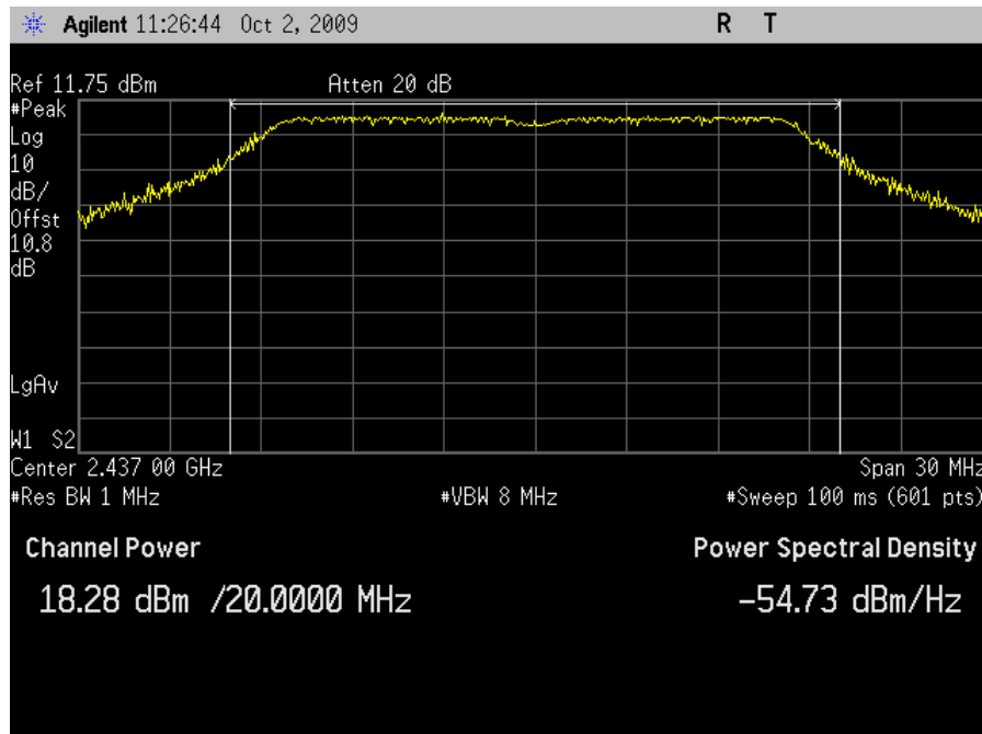
Plot 32. Peak Output Power, HT20 Channel 6 - Grid Antenna
