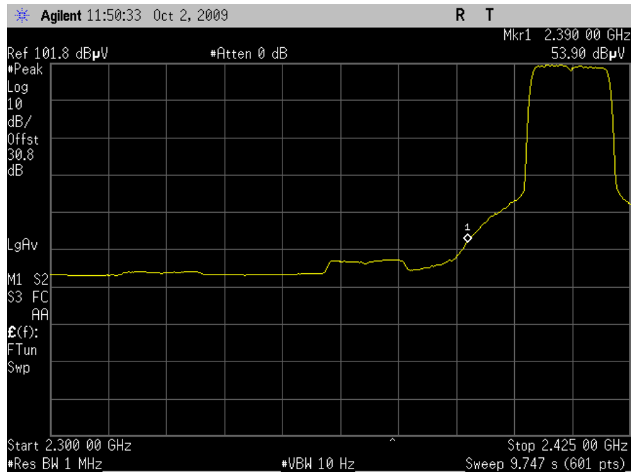
Plot 48. Channel 1 Lower Band Edge, Average - HT20 (Dish Antenna)
