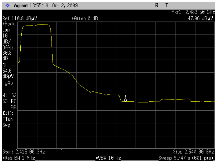
Plot 64. Channel 4 Upper Band Edge, Average - HT20 (Dish Antenna)
