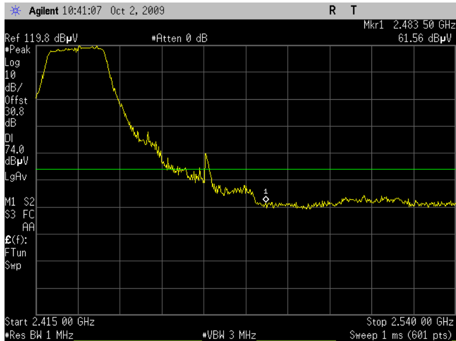
Plot 97. Channel 4 Upper Band Edge, Peak – HT20 (Grid Antenna)
