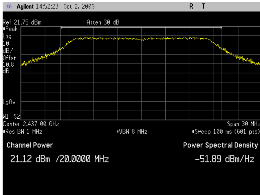
Plot 21. Peak Output Power, HT20 Channel 6 - Dish Antenna
