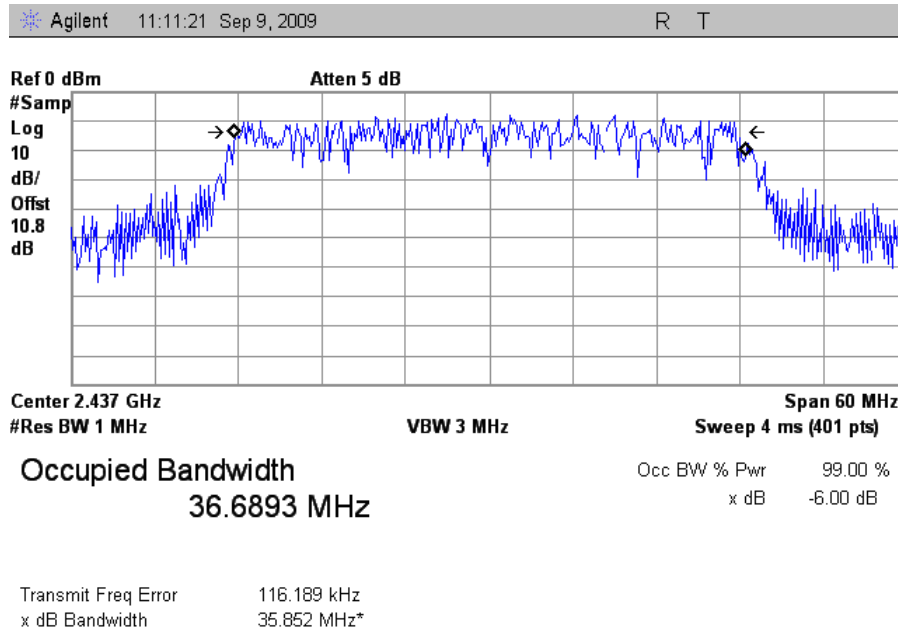
Plot 15. Occupied Band Width, Mid Channel, HT40 (99%)
