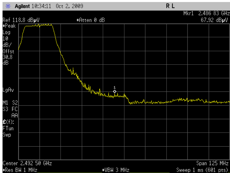
Plot 103. Channel 7 Upper Band Edge, Peak – HT20 (Grid Antenna)
