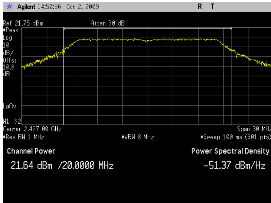
Plot 19. Peak Output Power, HT20 Channel 4 - Dish Antenna
