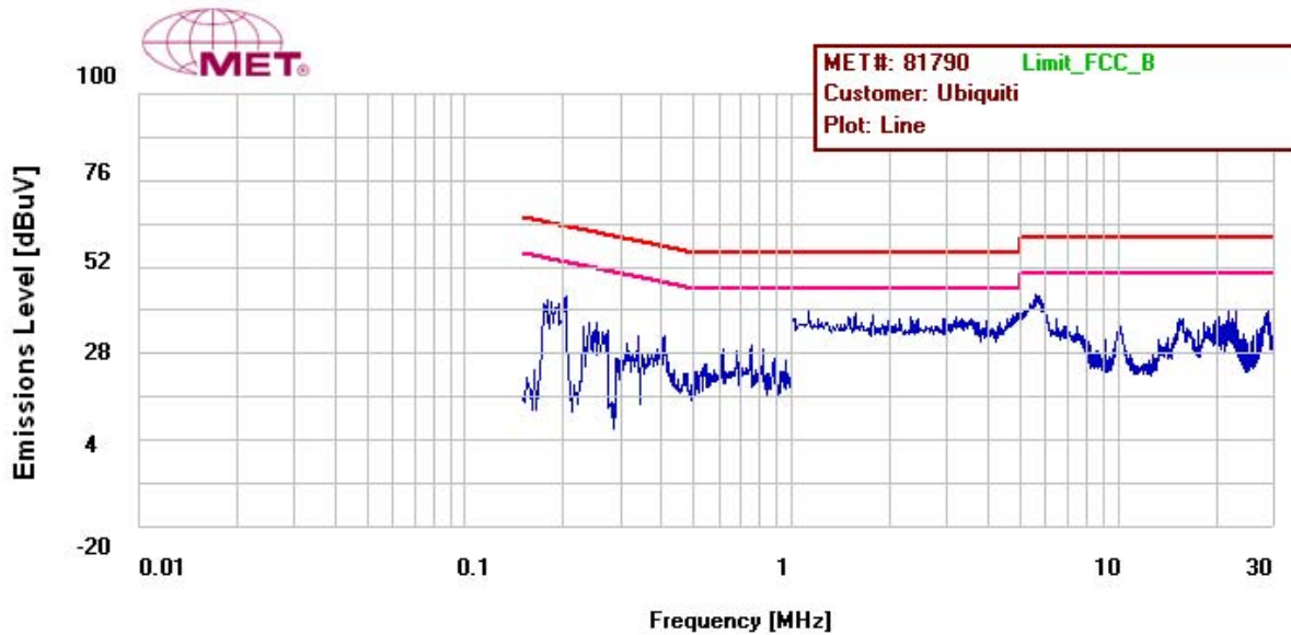
Plot 6. 15.207 Conducted Emissions, Phase Line
