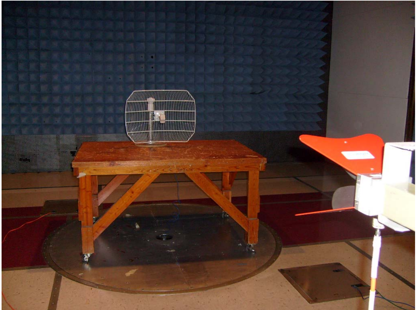
Photograph 7. Radiated Spurious, Test Setup (Grid Antenna)
