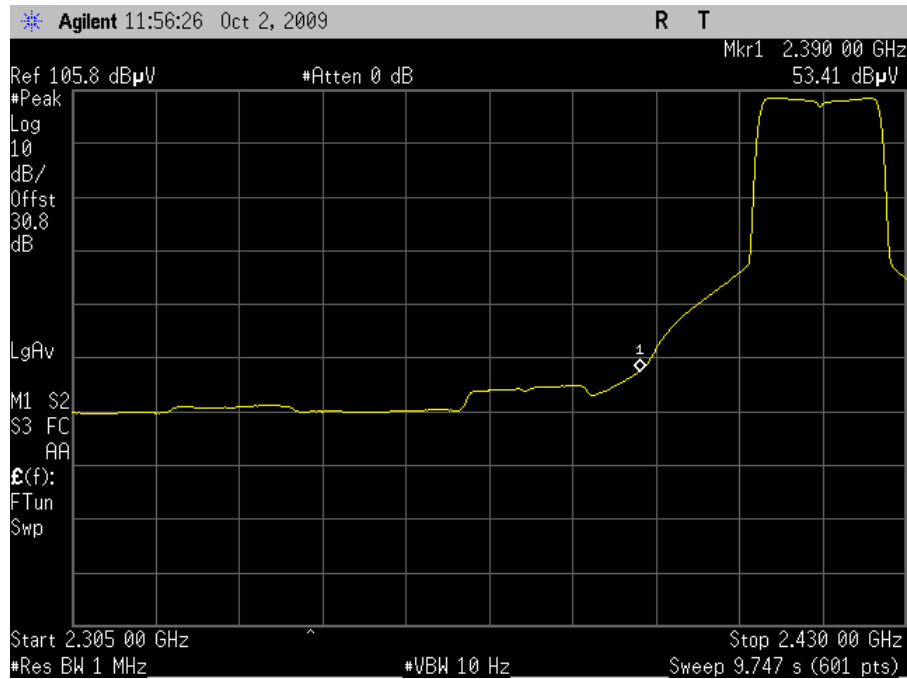
Plot 50. Channel 2 Lower Band Edge, Average - HT20 (Dish Antenna)
