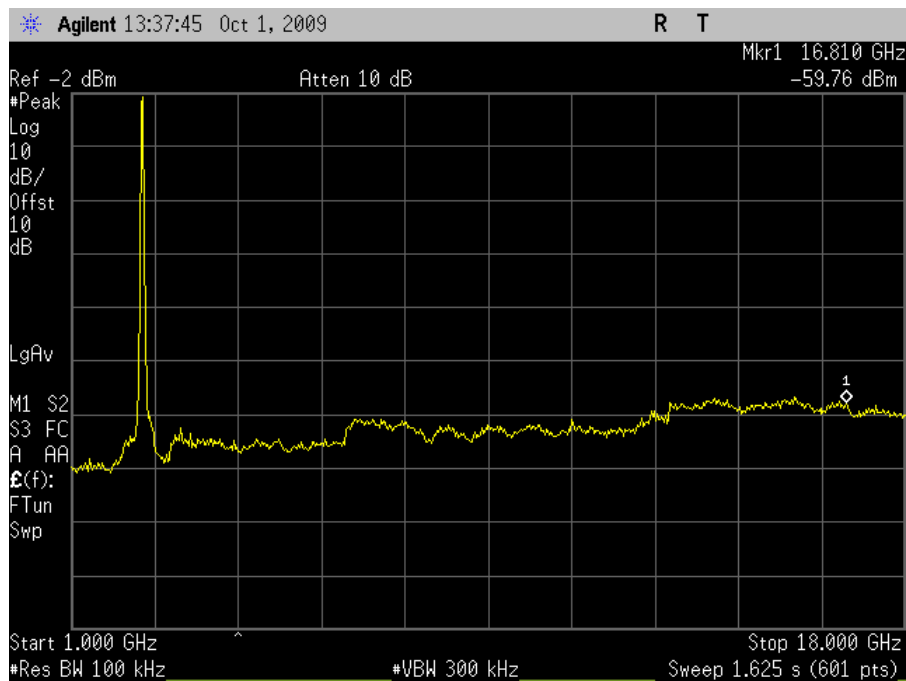
Plot 132. Conducted Emissions, Mid Channel, 1 GHz – 18 GHz (HT40)
