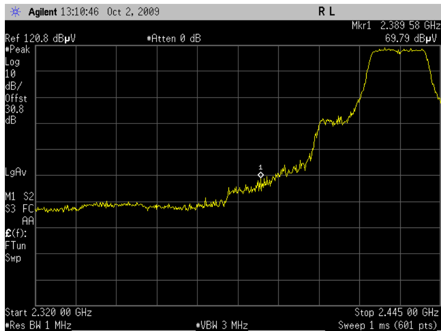
Plot 57. Channel 5 Lower Band Edge, Peak – HT20 (Dish Antenna)
