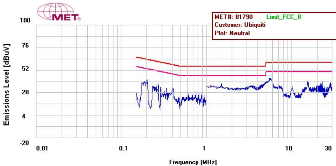
Plot 7. 15.207 Conducted Emissions, Neutral Line
