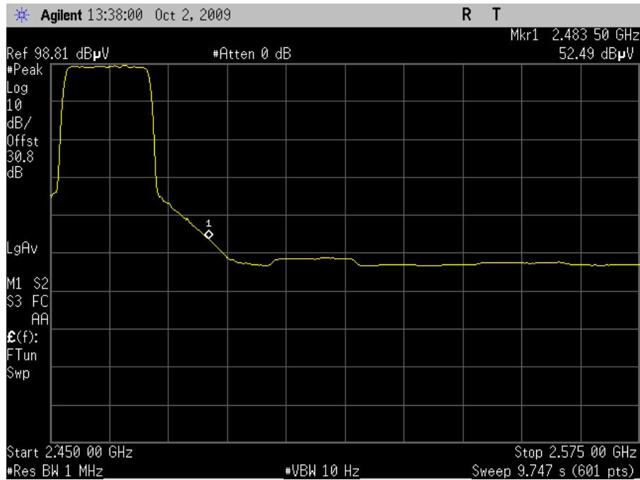
Plot 78. Channel 11 Upper Band Edge, Average - HT20 (Dish Antenna)
