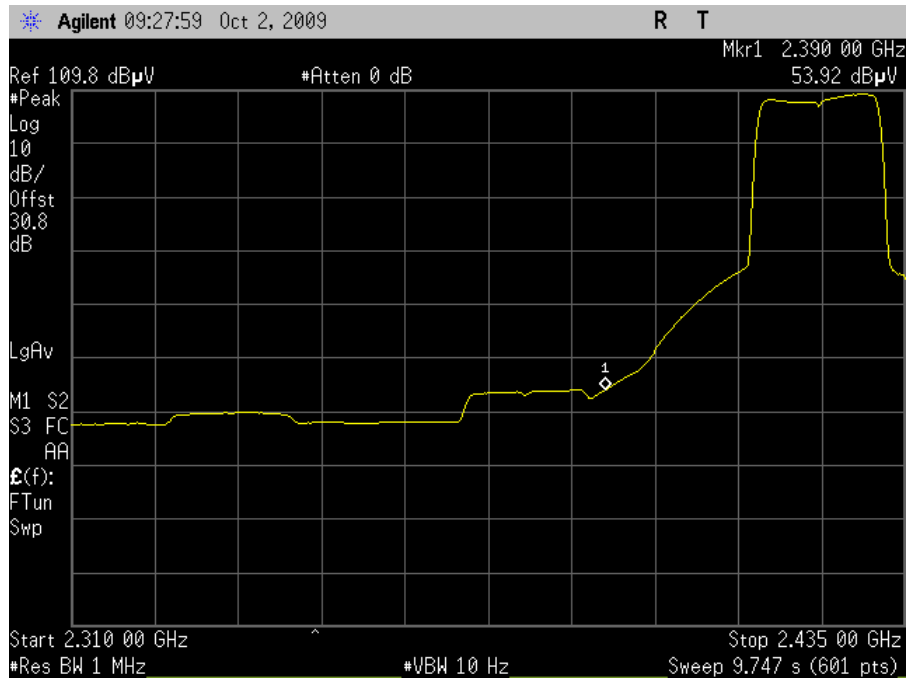
Plot 84. Channel 3 Lower Band Edge, Average - HT20 (Grid Antenna)
