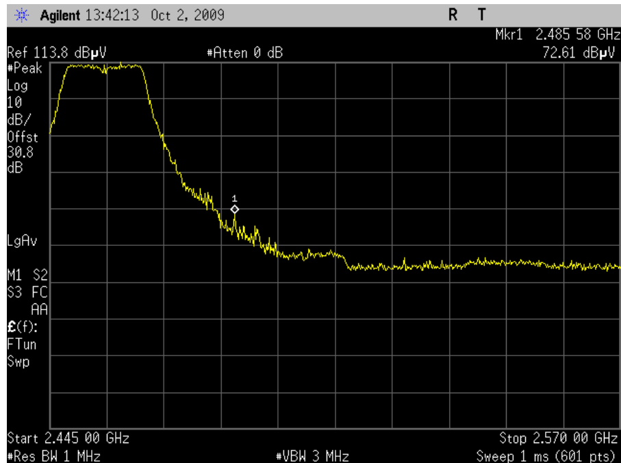
Plot 77. Channel 10 Upper Band Edge, Peak – HT20 (Dish Antenna)
