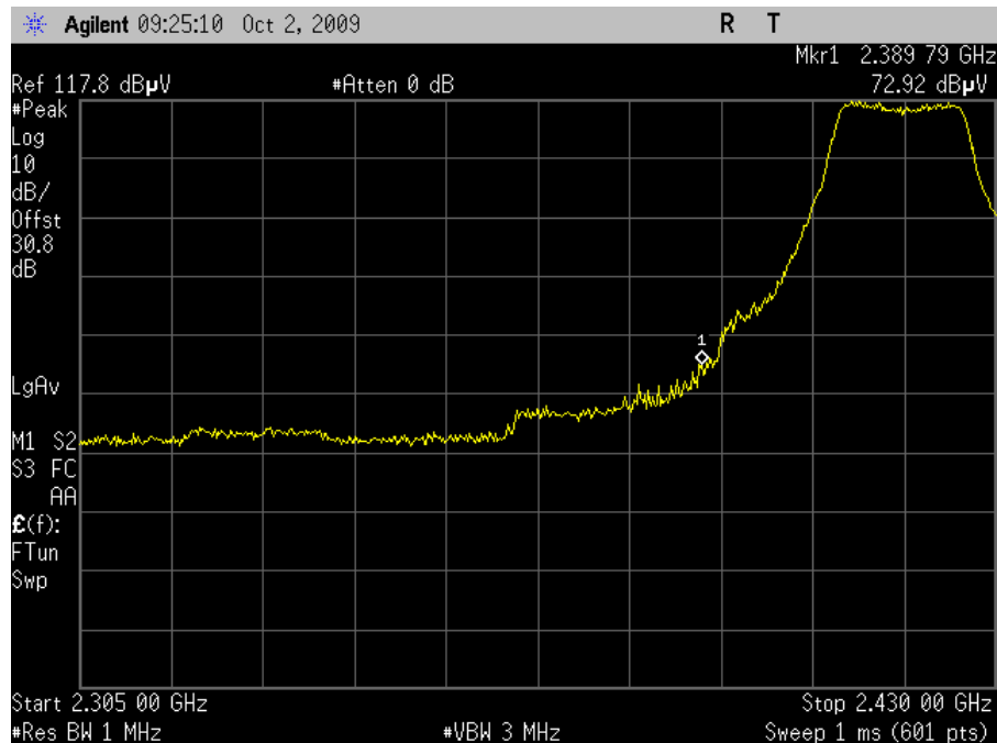
Plot 83. Channel 2 Lower Band Edge, Peak – HT20 (Grid Antenna)
