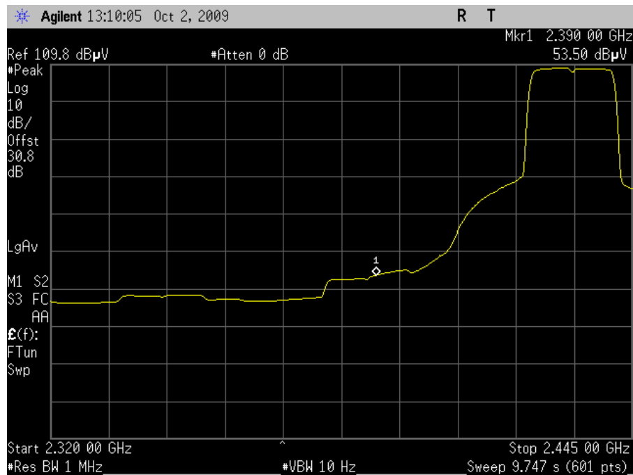
Plot 56. Channel 5 Lower Band Edge, Average - HT20 (Dish Antenna)
