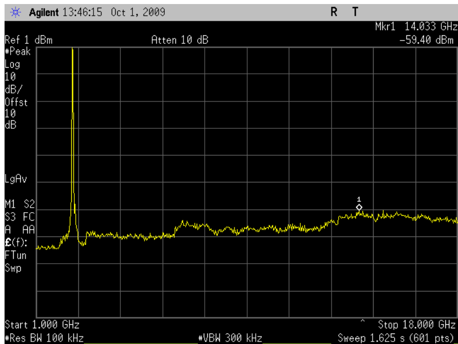
Plot 129. Conducted Emissions, High Channel, 1 GHz – 18 GHz (HT20)
