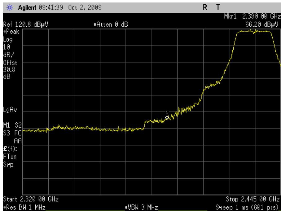
Plot 89. Channel 5 Lower Band Edge, Peak – HT20 (Grid Antenna)
