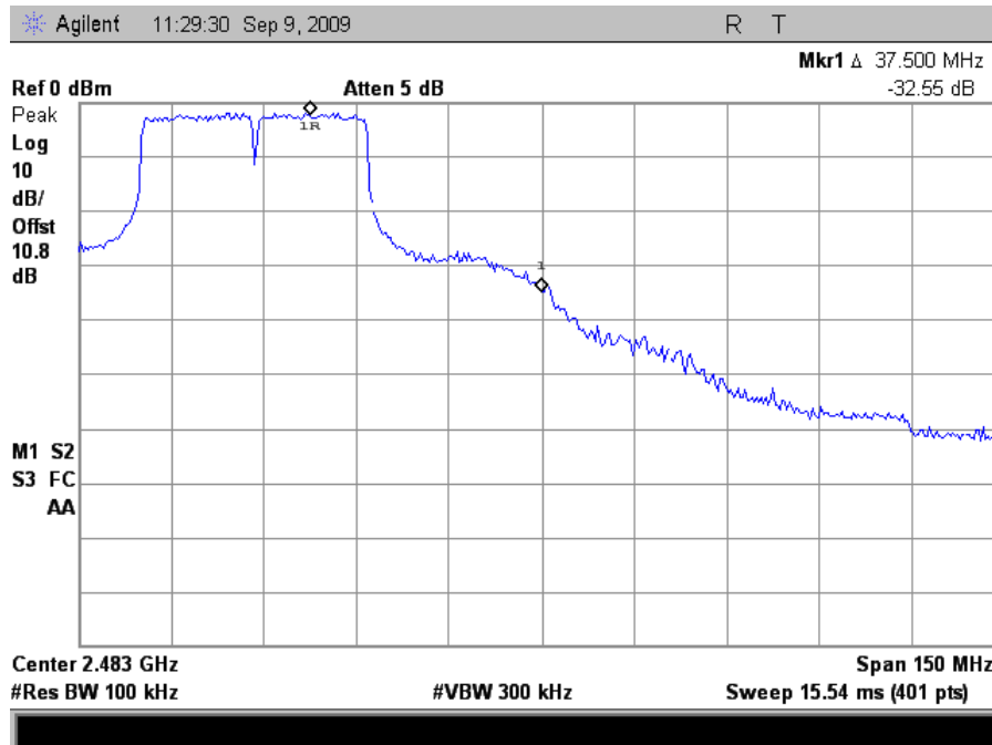
Plot 136. Conducted Band Edge, High Channel HT40
