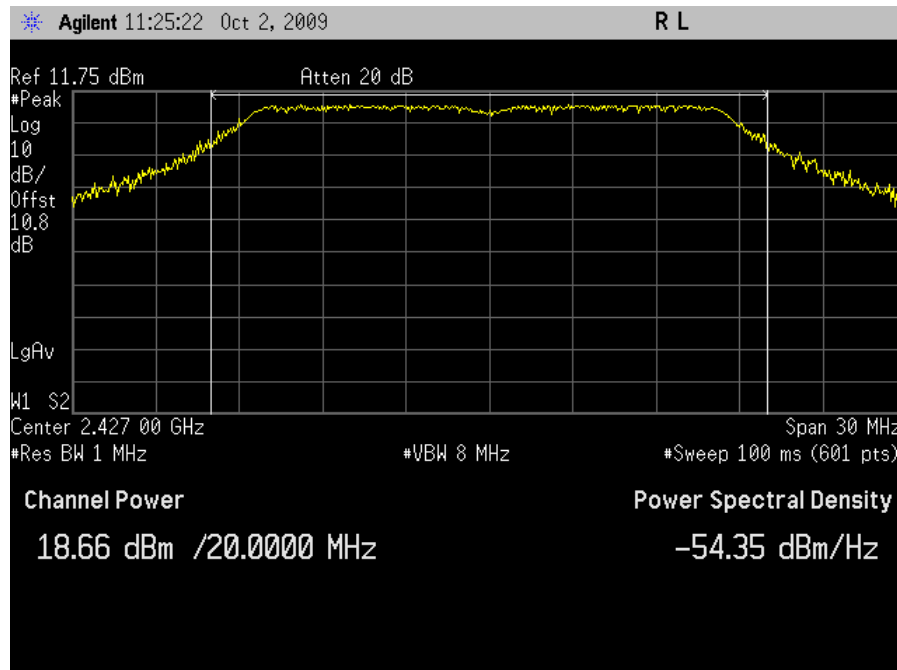
Plot 30. Peak Output Power, HT20 Channel 4 - Grid Antenna
