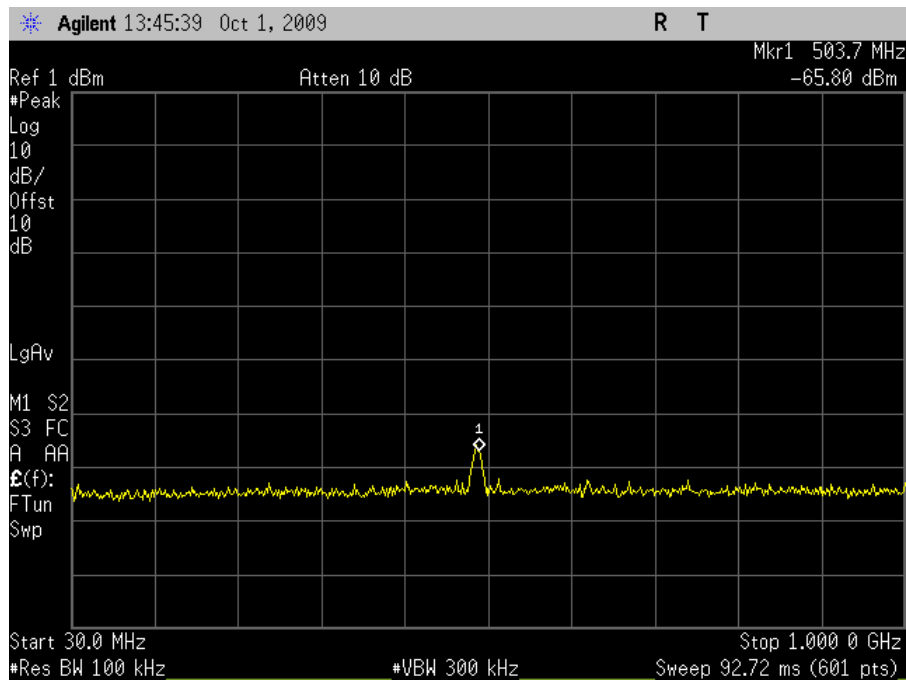
Plot 128. Conducted Emissions, High Channel, 30 MHz – 1 GHz (HT20)
