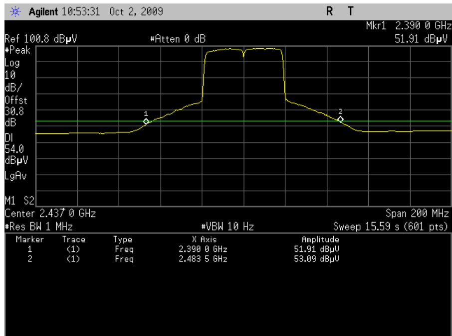
Plot 118. Band Edge, Average 200MHz Span – HT40 (Grid Antenna)
