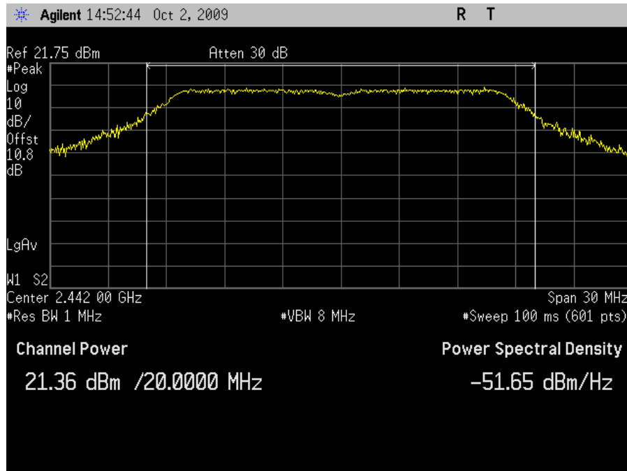
Plot 22. Peak Output Power, HT20 Channel 7 - Dish Antenna
