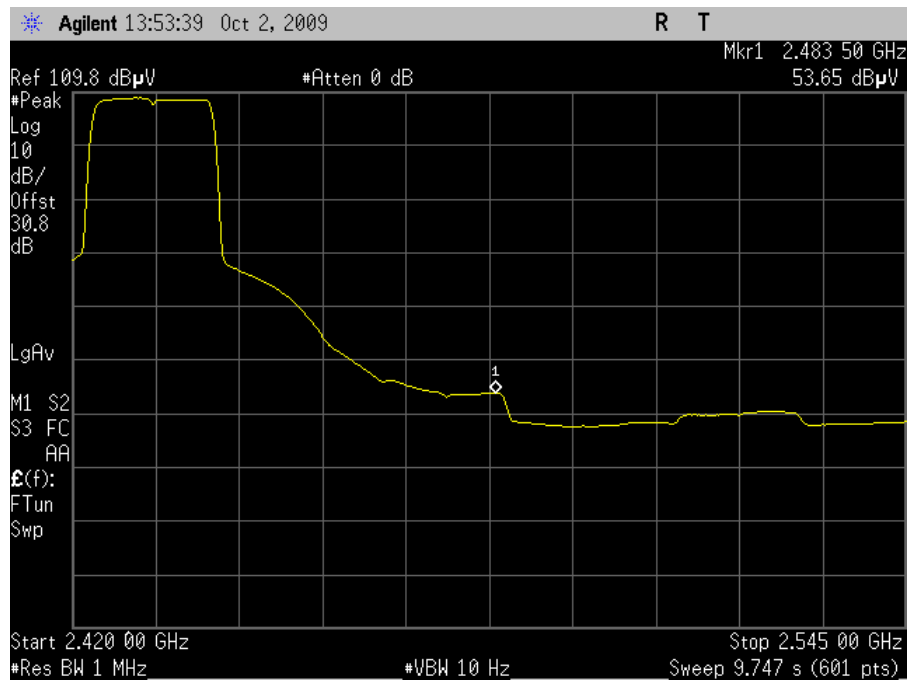
Plot 66. Channel 5 Upper Band Edge, Average - HT20 (Dish Antenna)
