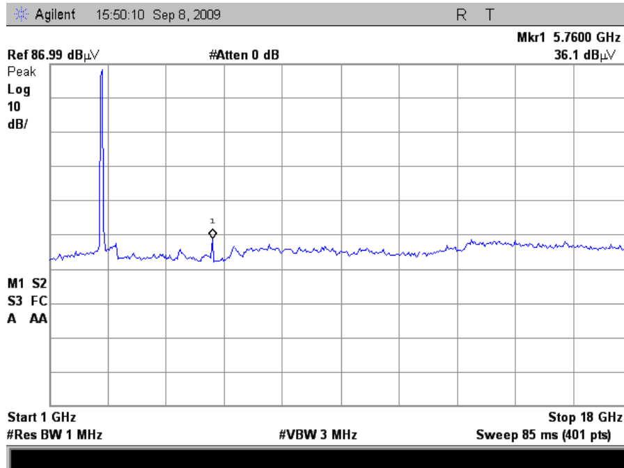
Plot 43. Radiated Spurious Emissions, Low Channel, HT20 (Grid Antenna)
