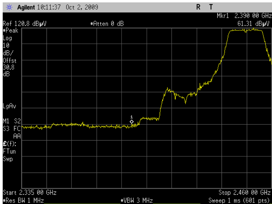
Plot 95. Channel 8 Lower Band Edge, Peak – HT20 (Grid Antenna)
