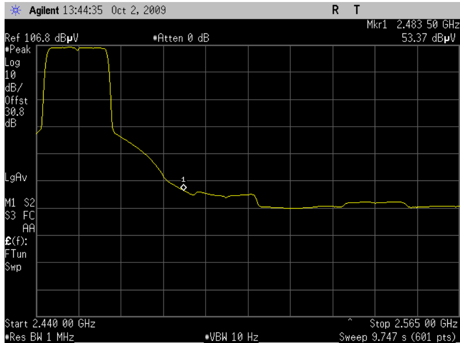
Plot 74. Channel 9 Upper Band Edge, Average - HT20 (Dish Antenna)
