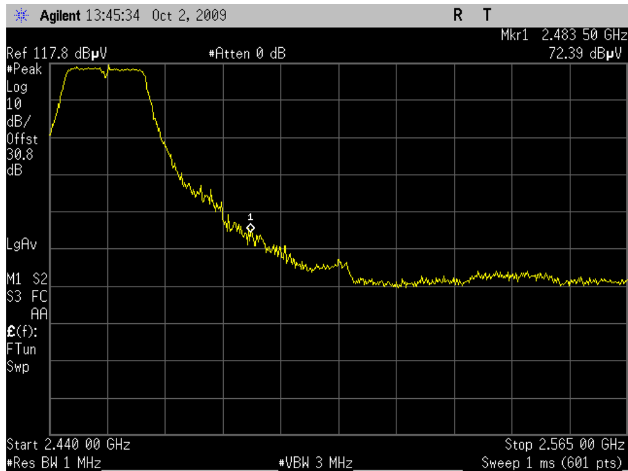
Plot 75. Channel 9 Upper Band Edge, Peak – HT20 (Dish Antenna)
