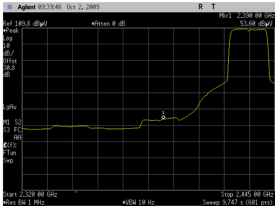
Plot 88. Channel 5 Lower Band Edge, Average - HT20 (Grid Antenna)
