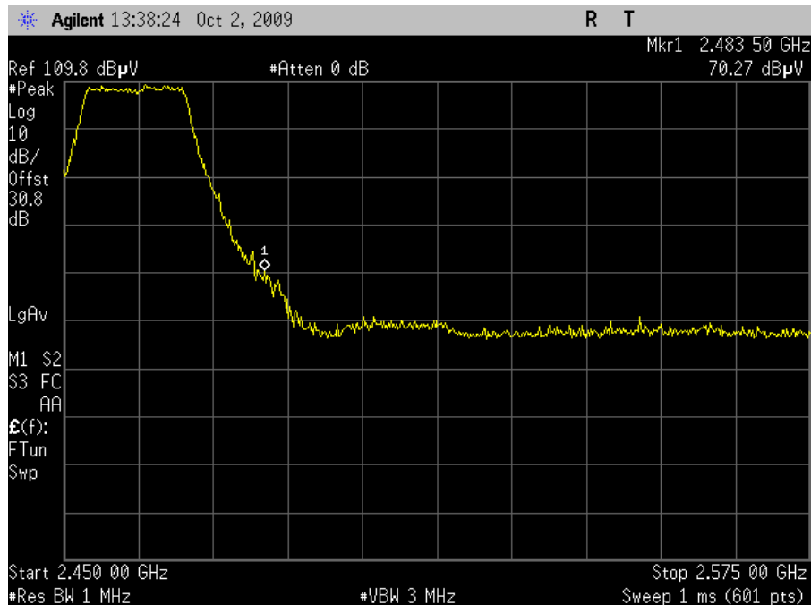
Plot 79. Channel 11 Upper Band Edge, Peak – HT20 (Dish Antenna)
