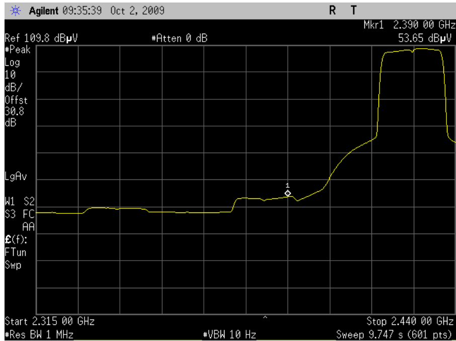
Plot 86. Channel 4 Lower Band Edge, Average - HT20 (Grid Antenna)
