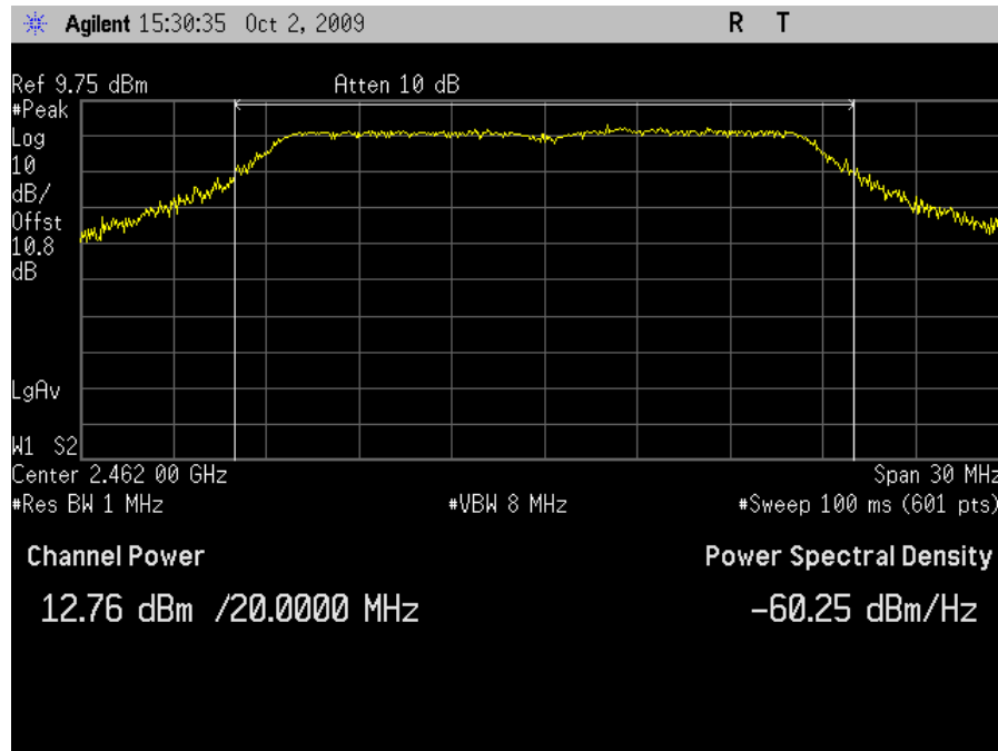
Plot 26. Peak Output Power, HT20 Channel 11 - Dish Antenna
