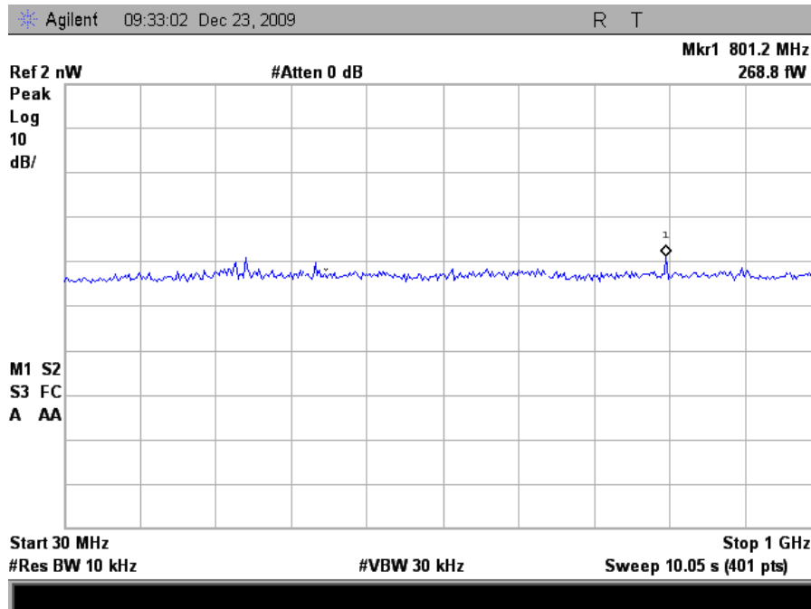
Plot 120. Receiver Spurious Emissions, 30MHz – 1GHz
