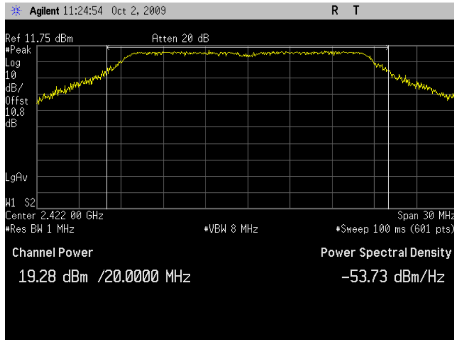
Plot 29. Peak Output Power, HT20 Channel 3 - Grid Antenna
