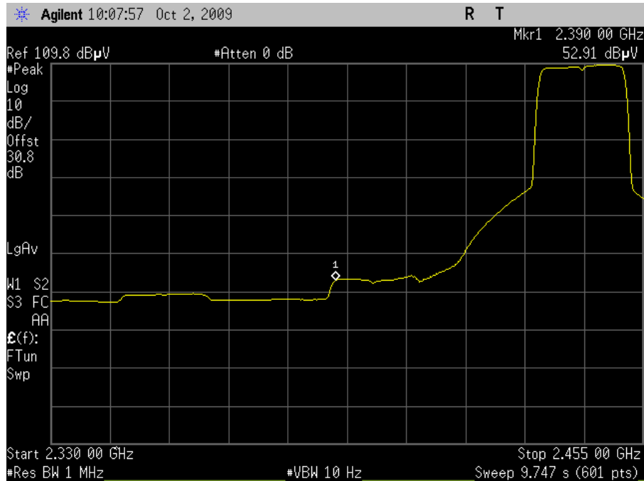
Plot 92. Channel 7 Lower Band Edge, Average - HT20 (Grid Antenna)
