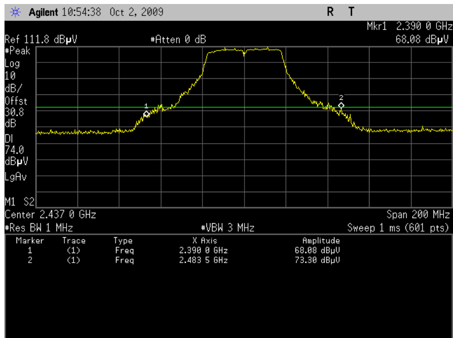
Plot 119. Band Edge, Peak 200MHz Span – HT40 (Grid Antenna)
