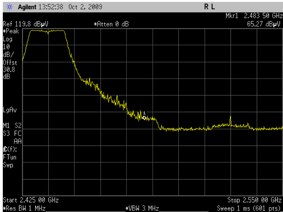
Plot 69. Channel 6 Upper Band Edge, Peak – HT20 (Dish Antenna)
