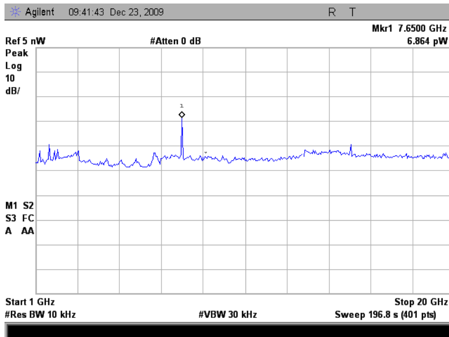
Plot 121. Receiver Spurious Emissions, 1GHz – 20GHz
