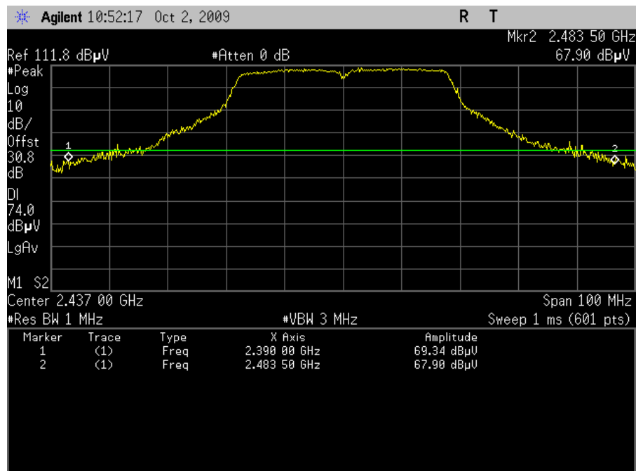
Plot 117. Band Edge, Peak 100MHz Span – HT40 (Grid Antenna)
