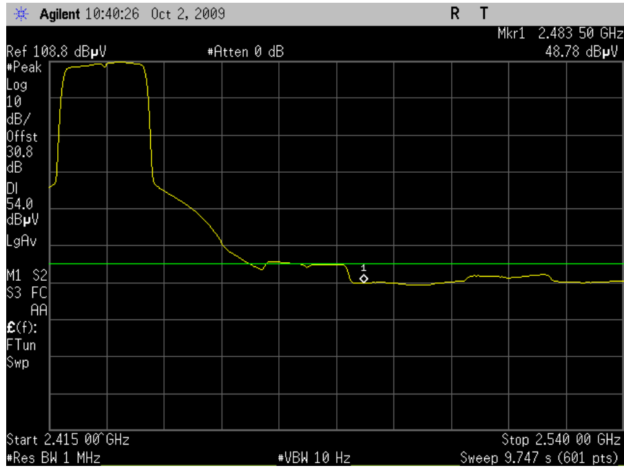
Plot 96. Channel 4 Upper Band Edge, Average - HT20 (Grid Antenna)
