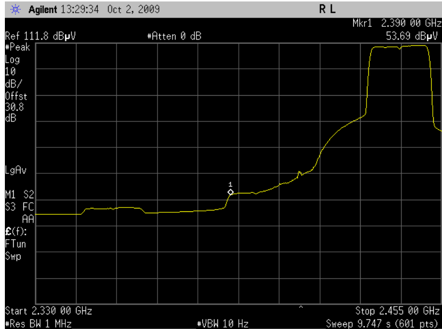
Plot 60. Channel 7 Lower Band Edge, Average - HT20 (Dish Antenna)
