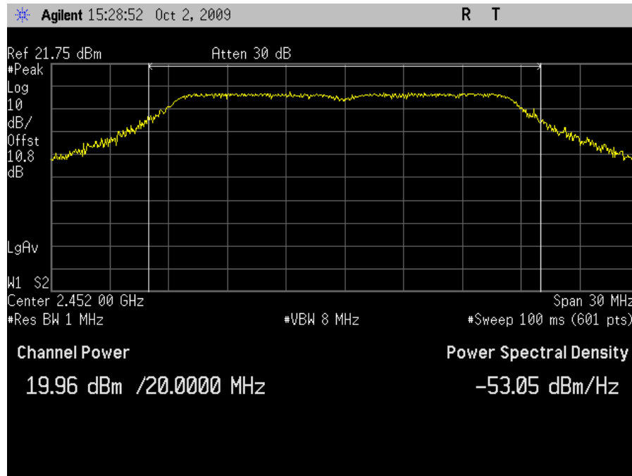
Plot 24. Peak Output Power, HT20 Channel 9 - Dish Antenna
