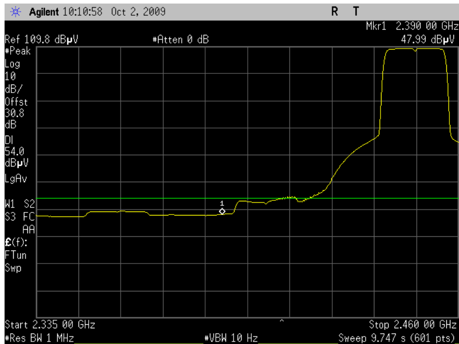
Plot 94. Channel 8 Lower Band Edge, Average - HT20 (Grid Antenna)
