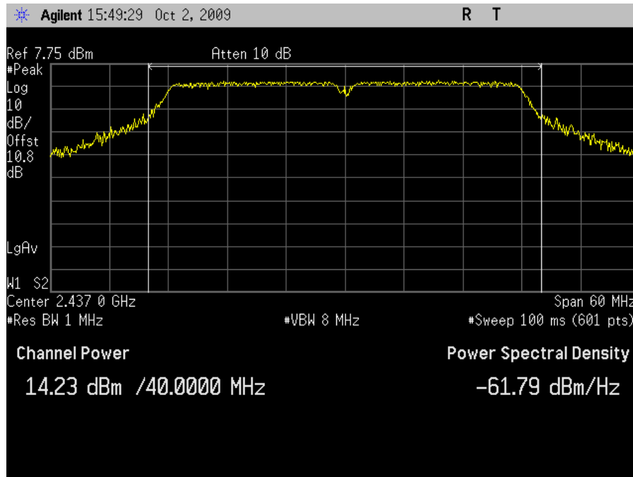
Plot 38. Peak Output Power, HT40 Channel 6 - Dish Antenna
