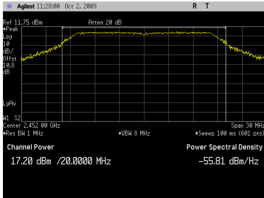
Plot 35. Peak Output Power, HT20 Channel 9 - Grid Antenna
