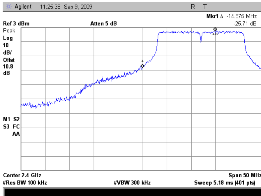
Plot 135. Conducted Band Edge, Low Channel HT20
