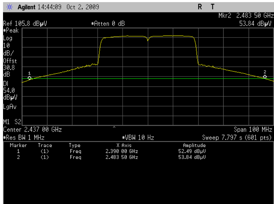
Plot 112. Band Edge, Average 100MHz Span – HT40 (Dish Antenna)
