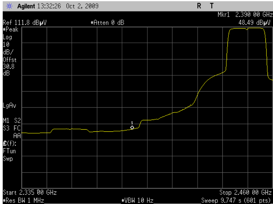
Plot 62. Channel 8 Lower Band Edge, Average - HT20 (Dish Antenna)
