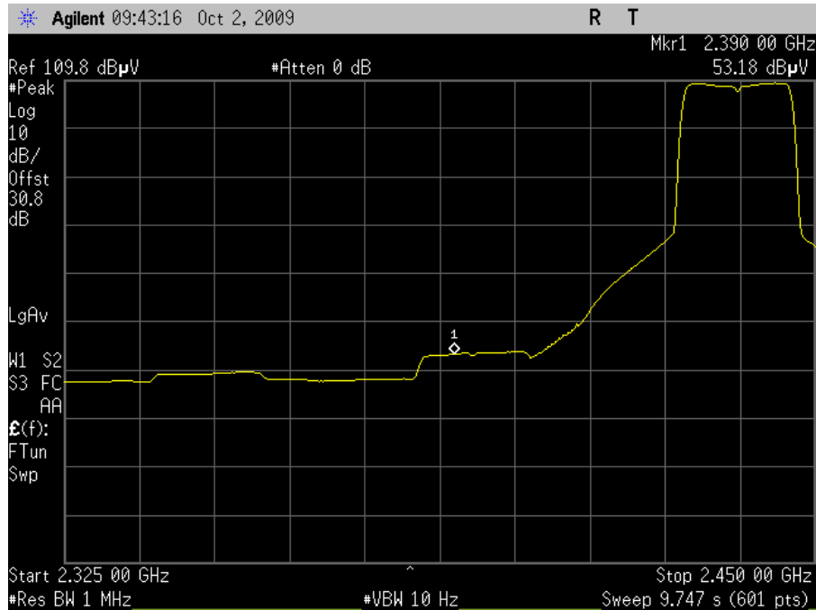
Plot 90. Channel 6 Lower Band Edge, Average - HT20 (Grid Antenna)
