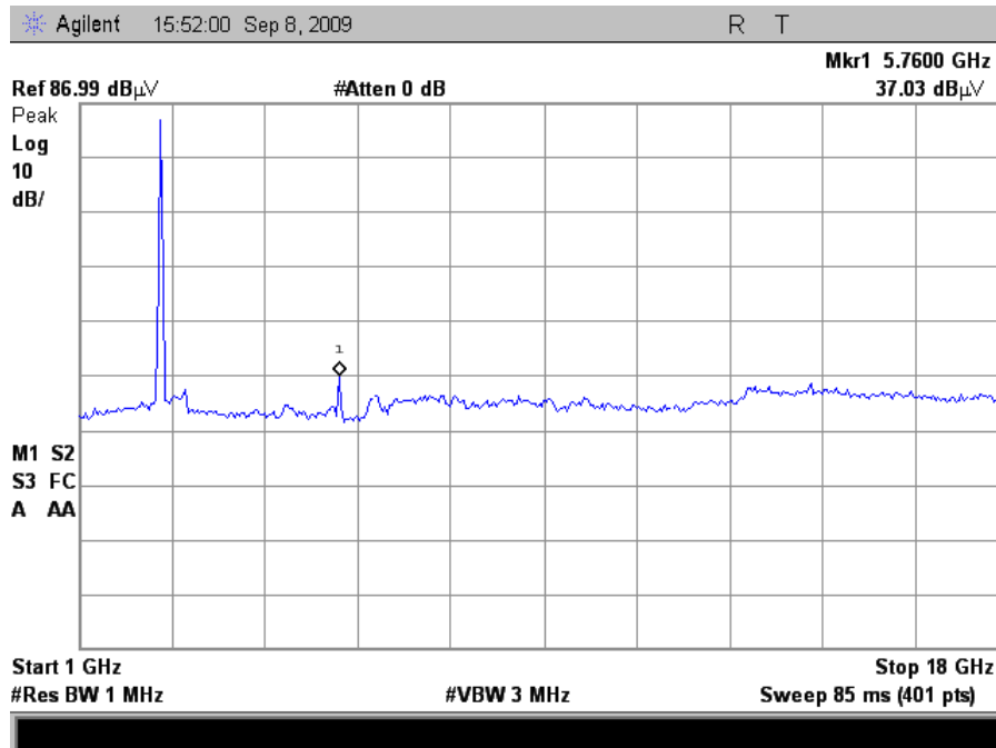
Plot 45. Radiated Spurious Emissions, High Channel, HT20 (Grid Antenna)
