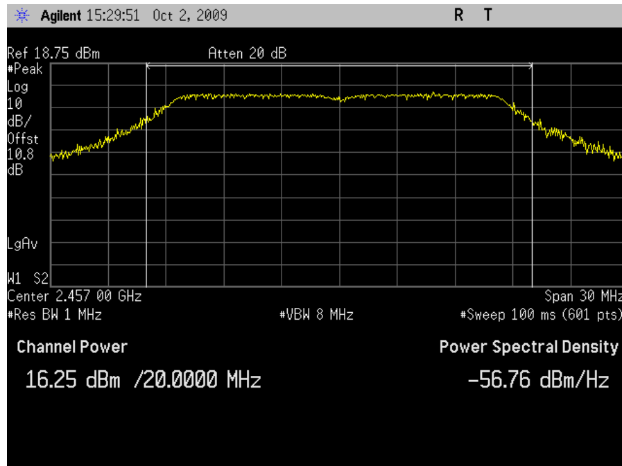
Plot 25. Peak Output Power, HT20 Channel 10 - Dish Antenna
