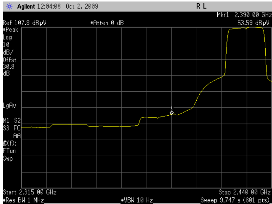
Plot 54. Channel 4 Lower Band Edge, Average - HT20 (Dish Antenna)
