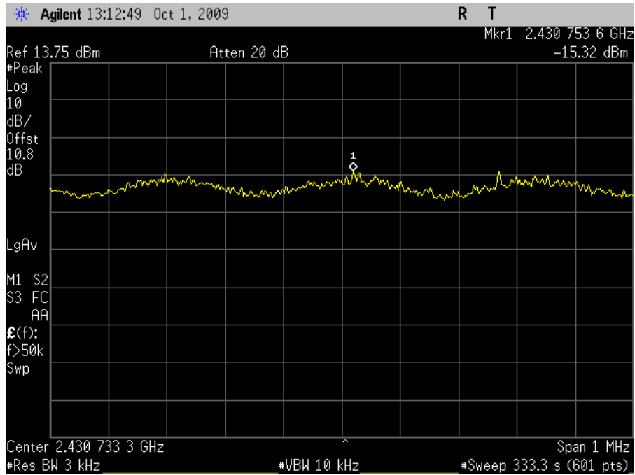
Plot 141. Peak Power Spectral Density, Mid Channel HT40
