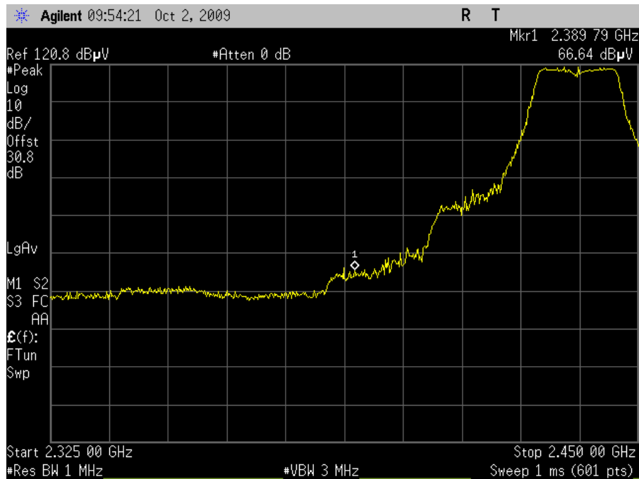
Plot 91. Channel 6 Lower Band Edge, Peak – HT20 (Grid Antenna)
