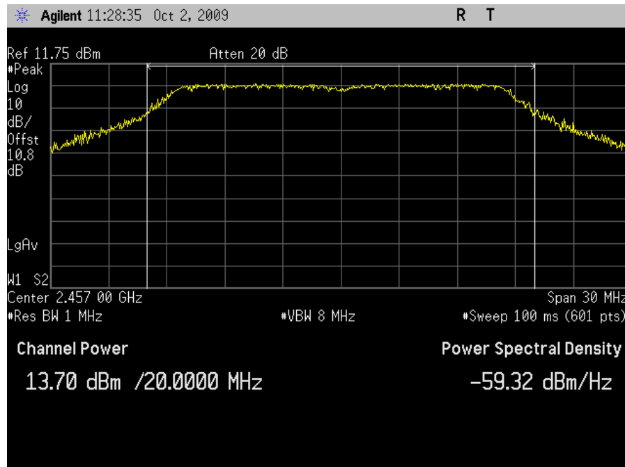
Plot 36. Peak Output Power, HT20 Channel 10 - Grid Antenna
