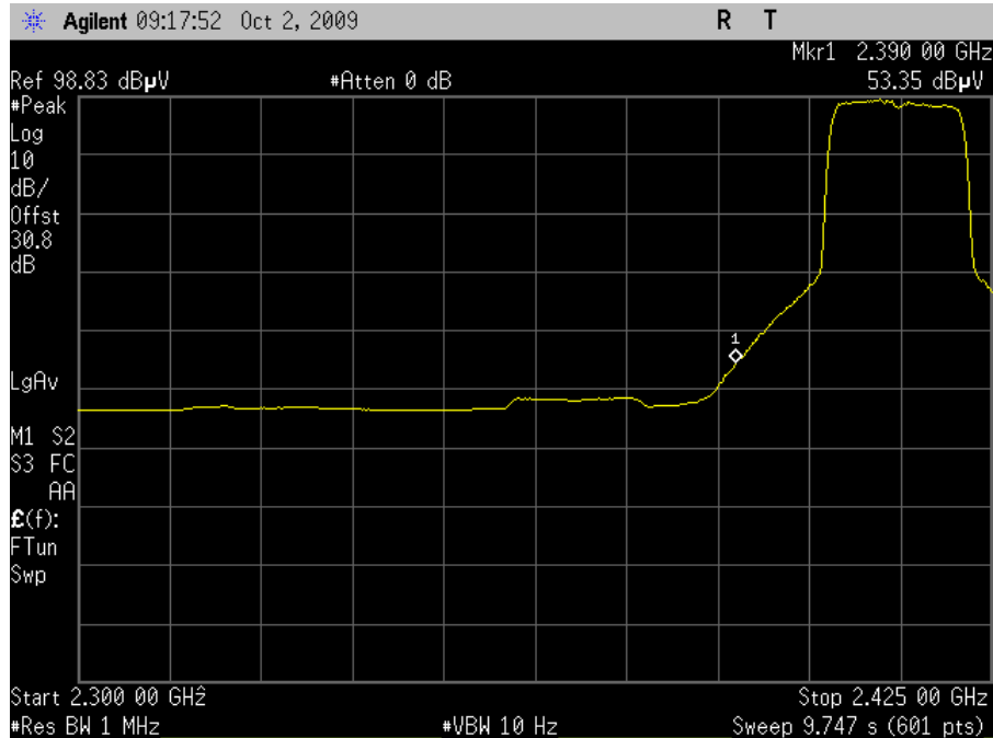
Plot 80. Channel 1 Lower Band Edge, Average - HT20 (Grid Antenna)
