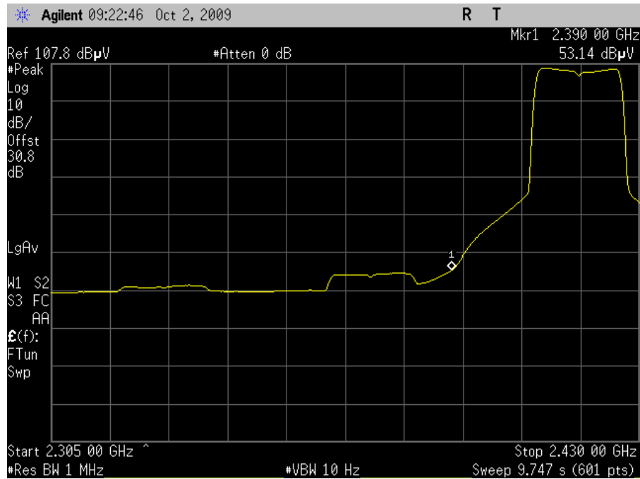
Plot 82. Channel 2 Lower Band Edge, Average - HT20 (Grid Antenna)
