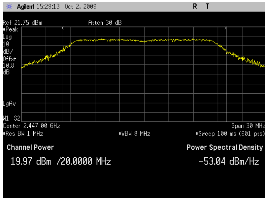
Plot 23. Peak Output Power, HT20 Channel 8 - Dish Antenna
