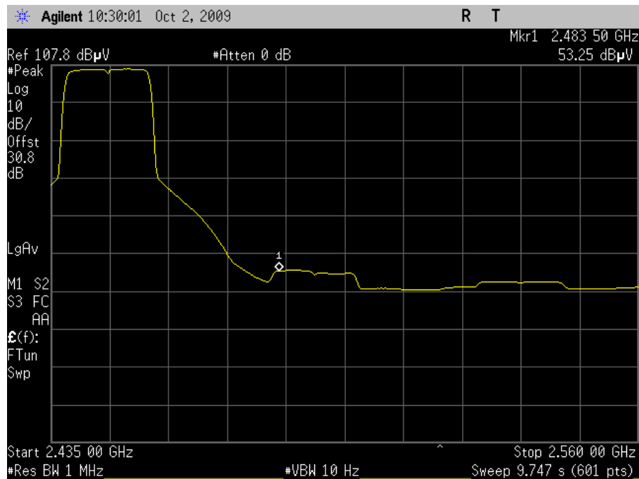
Plot 104. Channel 8 Upper Band Edge, Average - HT20 (Grid Antenna)
