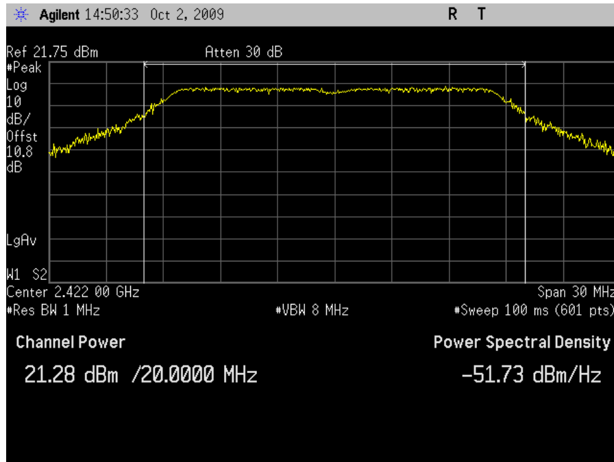
Plot 18. Peak Output Power, HT20 Channel 3 - Dish Antenna
