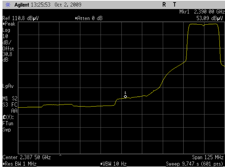
Plot 58. Channel 6 Lower Band Edge, Average - HT20 (Dish Antenna)
