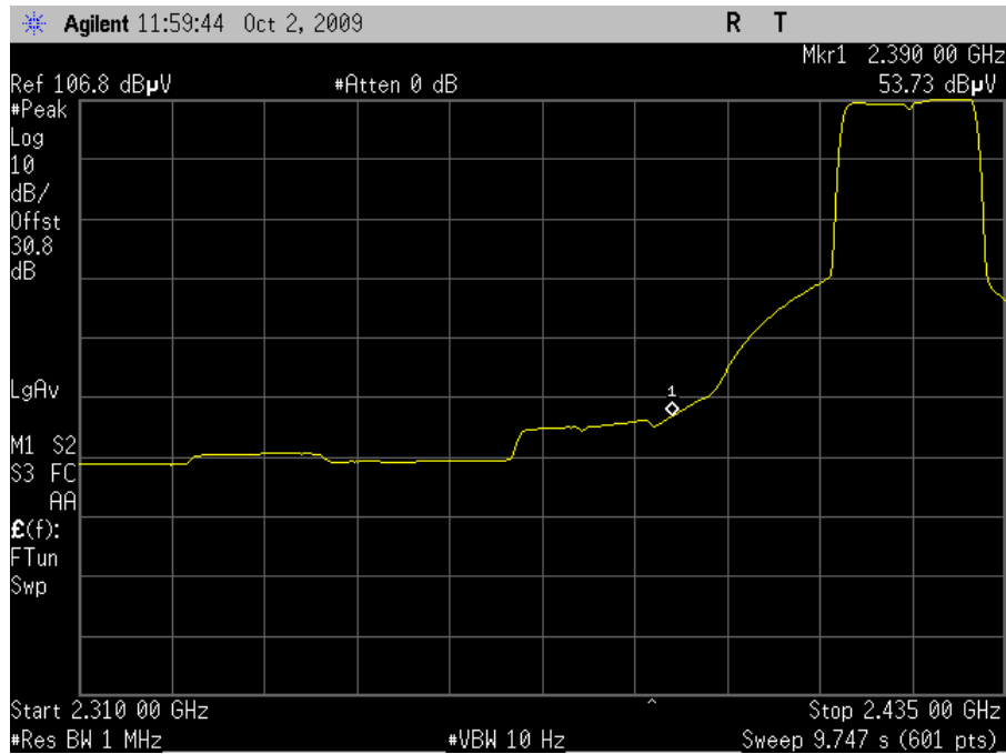
Plot 52. Channel 3 Lower Band Edge, Average - HT20 (Dish Antenna)
