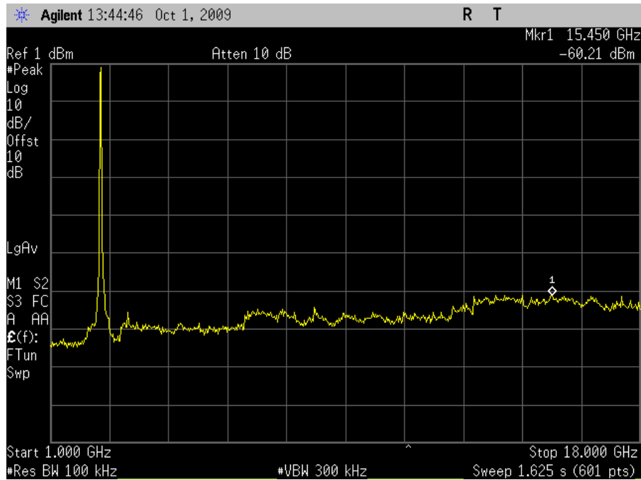
Plot 126. Conducted Emissions, Mid Channel, 1 GHz – 18 GHz (HT20)
