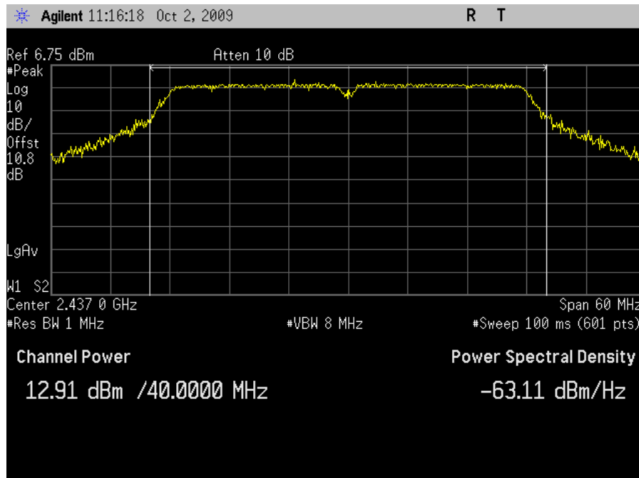
Plot 39. Peak Output Power, HT40 Channel 6 - Grid Antenna
