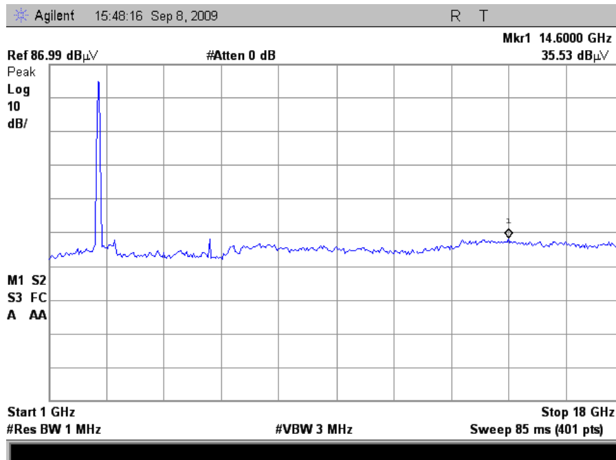
Plot 47. Radiated Spurious Emissions, Mid Channel, HT40 (Grid Antenna)
