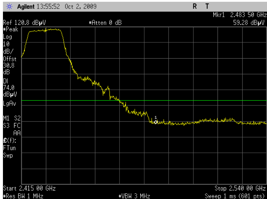
Plot 65. Channel 4 Upper Band Edge, Peak – HT20 (Dish Antenna)
