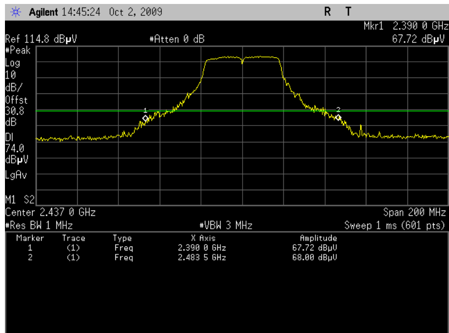
Plot 115. Band Edge, Peak 200MHz Span – HT40 (Dish Antenna)
