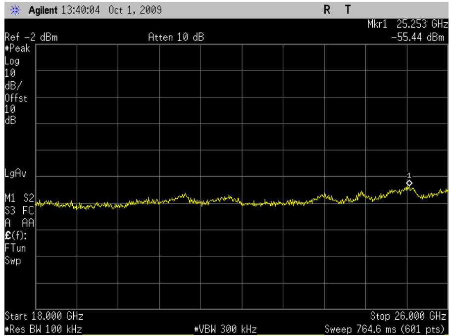
Plot 133. Conducted Emissions, Mid Channel, 18 GHz – 26 GHz (HT40)
