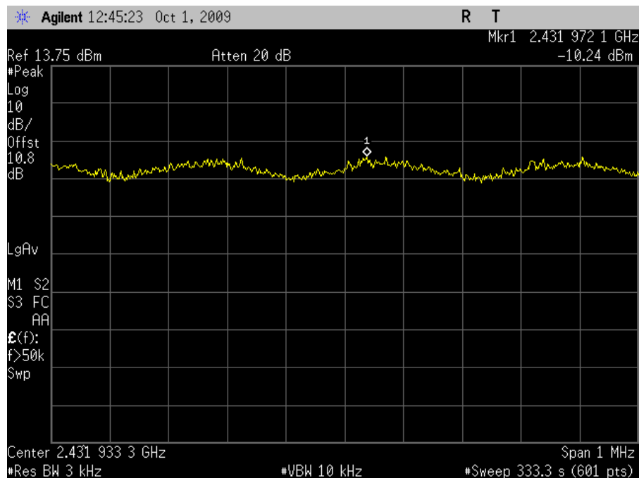
Plot 139. Peak Power Spectral Density, Mid Channel HT20
