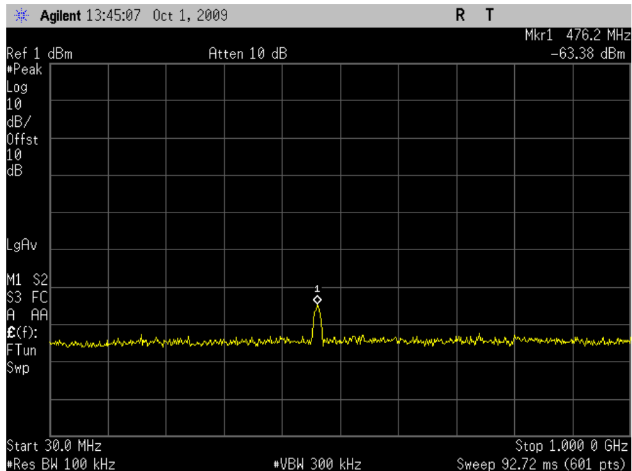
Plot 125. Conducted Emissions, Mid Channel, 30 MHz – 1 GHz (HT20)
