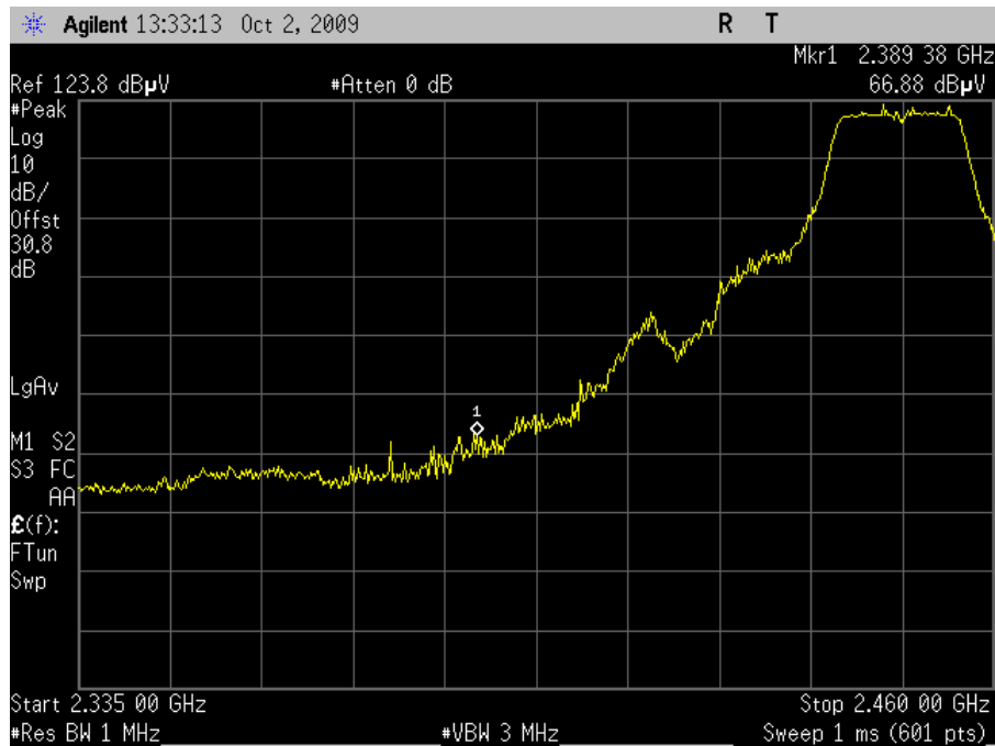
Plot 63. Channel 8 Lower Band Edge, Peak – HT20 (Dish Antenna)
