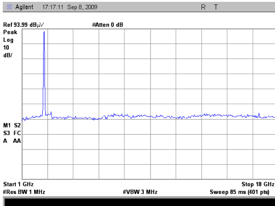
Plot 41. Radiated Spurious Emissions, Mid Channel, HT20 (Dish Antenna)
