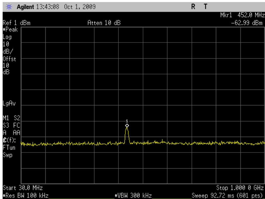
Plot 122. Conducted Emissions, Low Channel, 30 MHz – 1 GHz (HT20)
