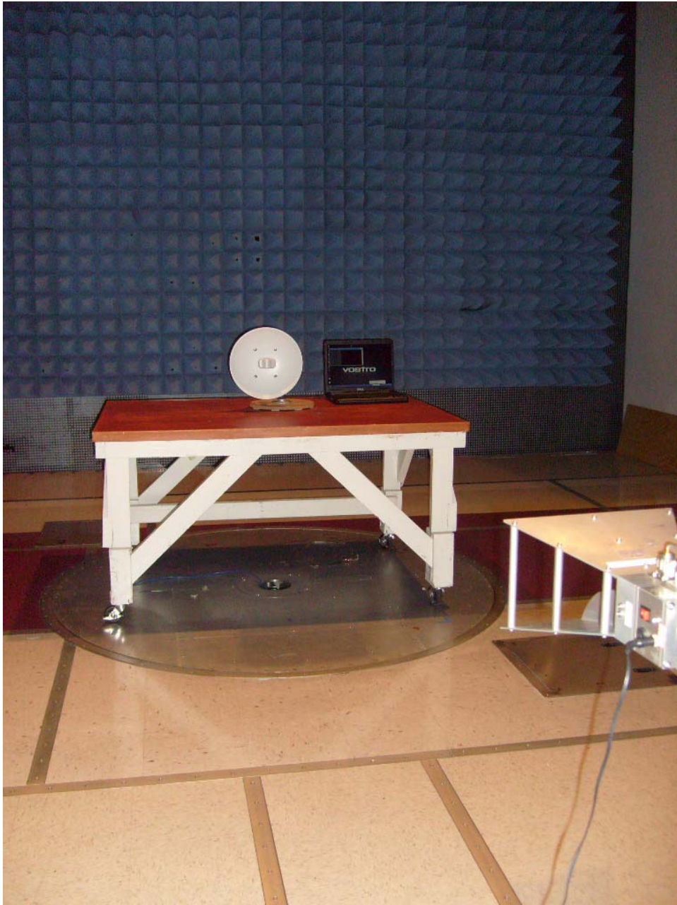
Photograph 4. Radiated Emission, above 1GHz Test Setup
