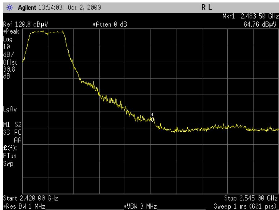
Plot 67. Channel 5 Upper Band Edge, Peak – HT20 (Dish Antenna)
