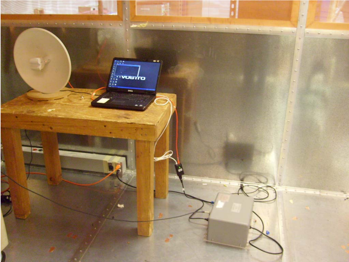
Photograph 5. CEV 15.107 Setup
