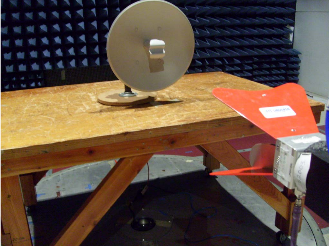
Photograph 3. Radiated restricted band setup @1m
