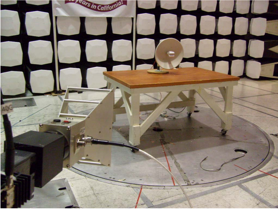
Photograph 2. 15.109, Radiated Emission 1GHz - 10GHz Setup
