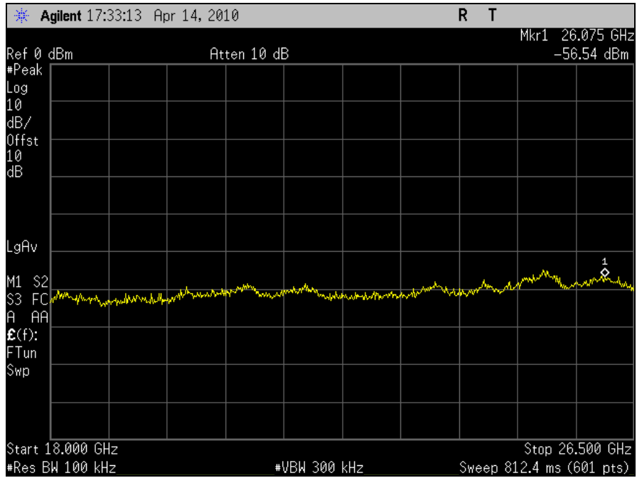
Plot 91. Conducted Spurious Emission, 802.11n 20MHz, Port J6, Channel 6, 18GHz - 26.5GHz
