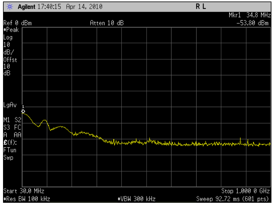
Plot 86. Conducted Spurious Emission, 802.11n 20MHz, Port J6, Channel 1, 30MHz - 1GHz
