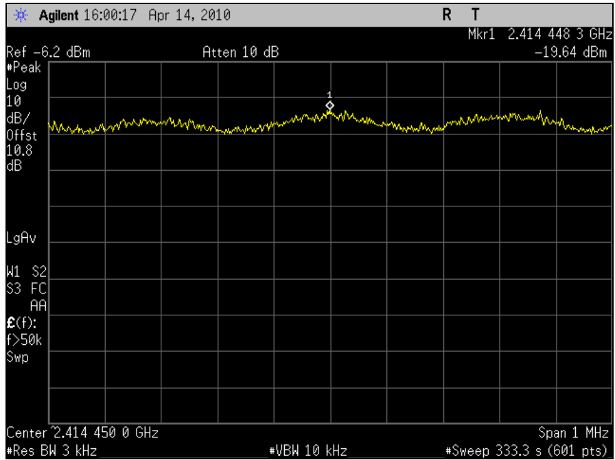
Plot 105. Spectral Power Density, 802.11n 20MHz, Port J5, Channel 1
