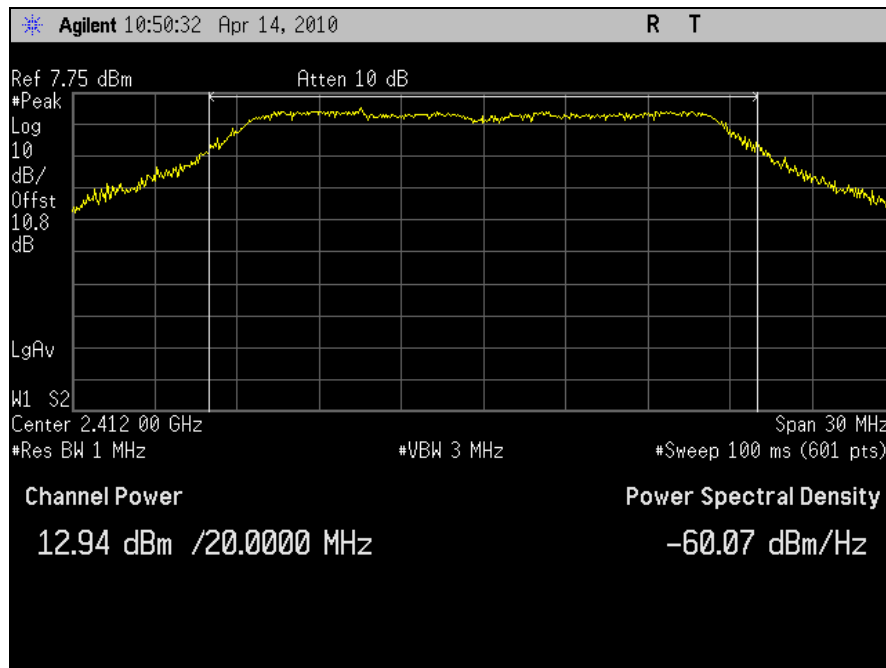
Plot 33. Conducted Output Power, 802.11n 20MHz, Port J6, Channel 1 (2412MHz)
