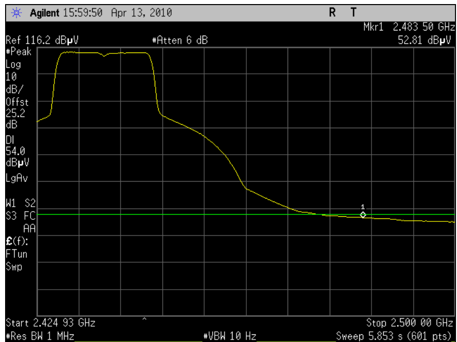
Plot 62. Radiated Restricted Band, Channel 6 - High, 802.11n 20MHz, Average
