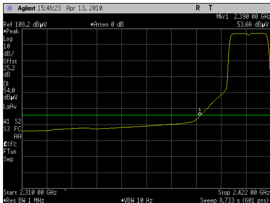
Plot 52. Radiated Restricted Band, Channel 1, 802.11n 20MHz, Average
