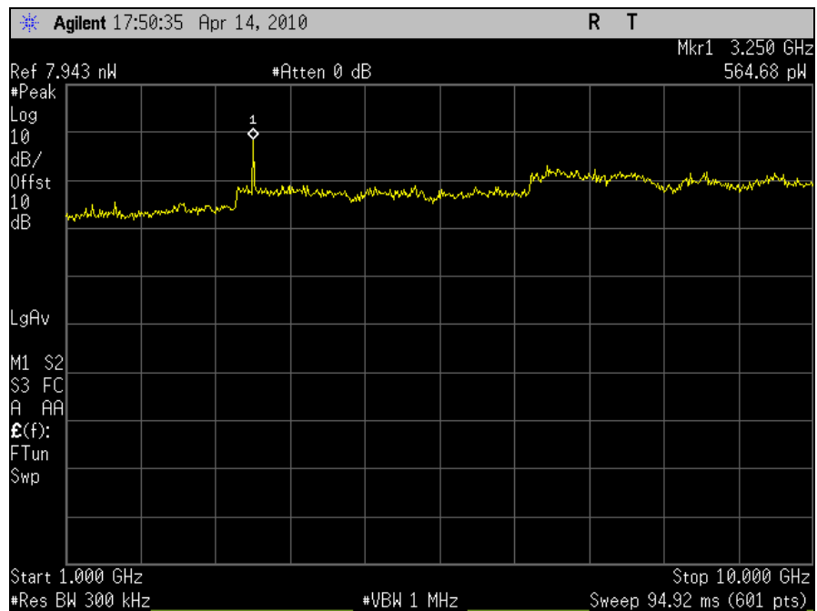
Plot 76. Conducted Rx Spurious 1 GHz – 10 GHz, Port J6
