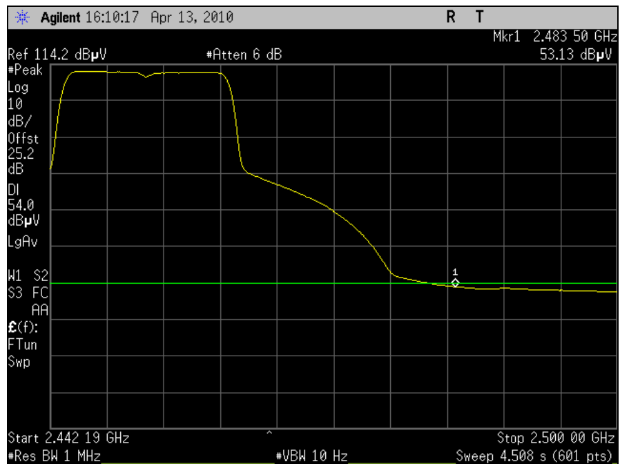
Plot 66. Radiated Restricted Band, Channel 9, 802.11n 20MHz, Average
