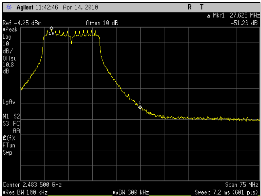
Plot 102. Upper Conducted Band Edge, 802.11n 20MHz
