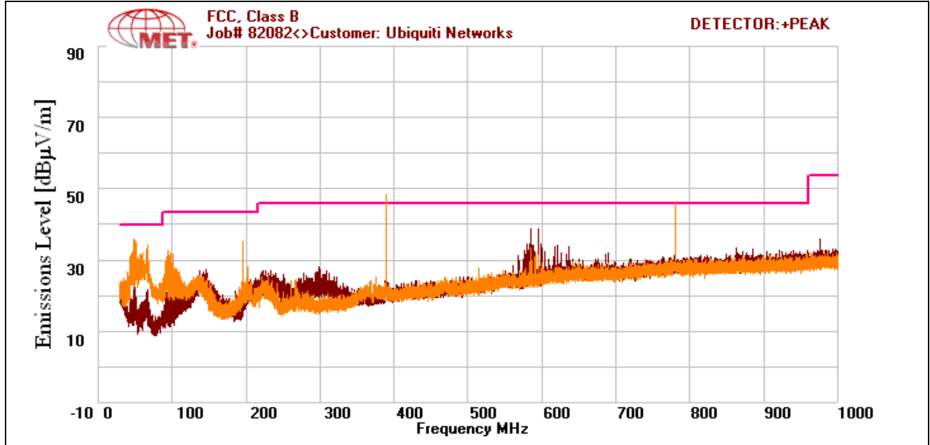
Plot 45. Radiated Emissions, Mid Channel
