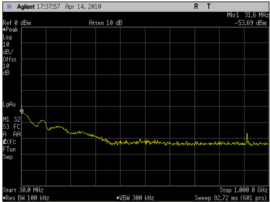
Plot 98. Conducted Spurious Emission, 802.11n 40MHz, Port J6, Channel 6, 30MHz - 1GHz
