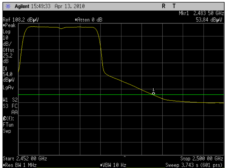
Plot 70. Radiated Restricted Band, Channel 11, 802.11n 20MHz, Average
