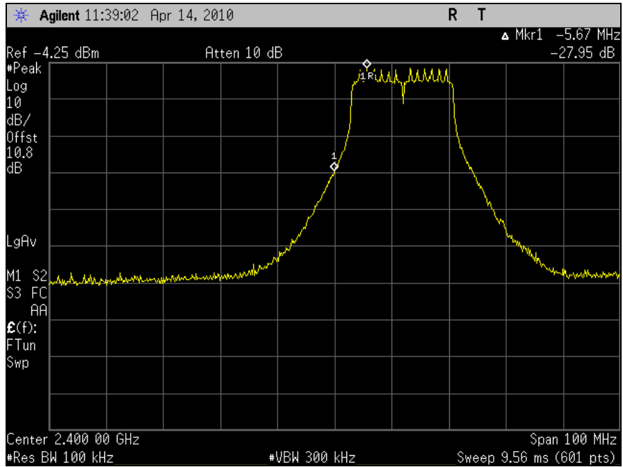
Plot 101. Lower Conducted Band Edge, 802.11n 20MHz
