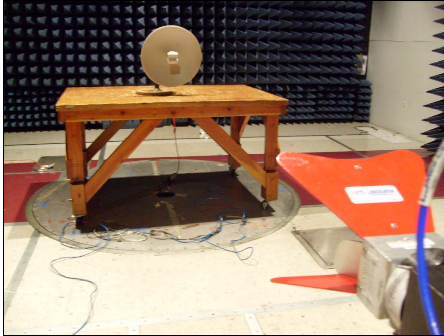
Photograph 6. Radiated Spurious Emissions, Test Setup @ 3m
