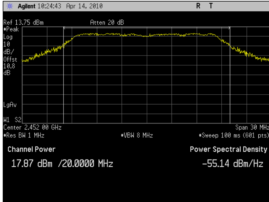
Plot 30. Conducted Output Power, 802.11n 20MHz, Port J5, Channel 9 (2452MHz)
