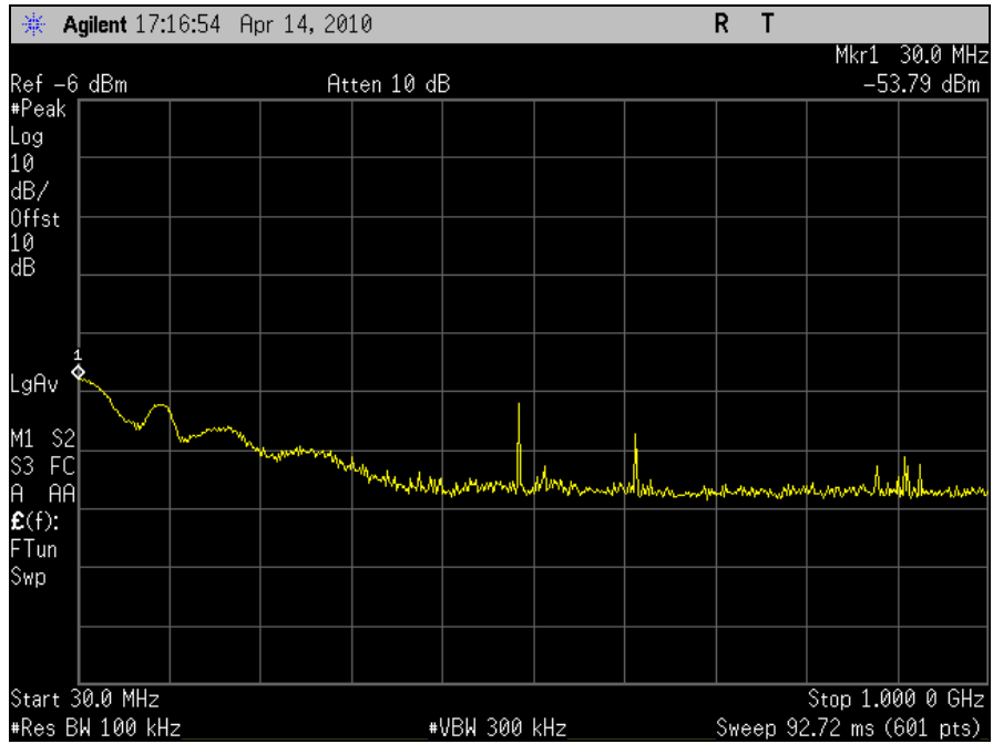
Plot 77. Conducted Spurious Emission, 802.11n 20MHz, Port J5, Channel 1, 30MHz - 1GHz
