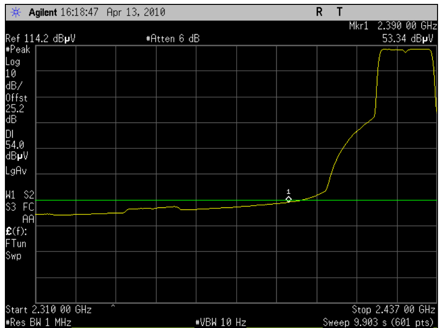
Plot 58. Radiated Restricted Band, Channel 4, 802.11n 20MHz, Average
