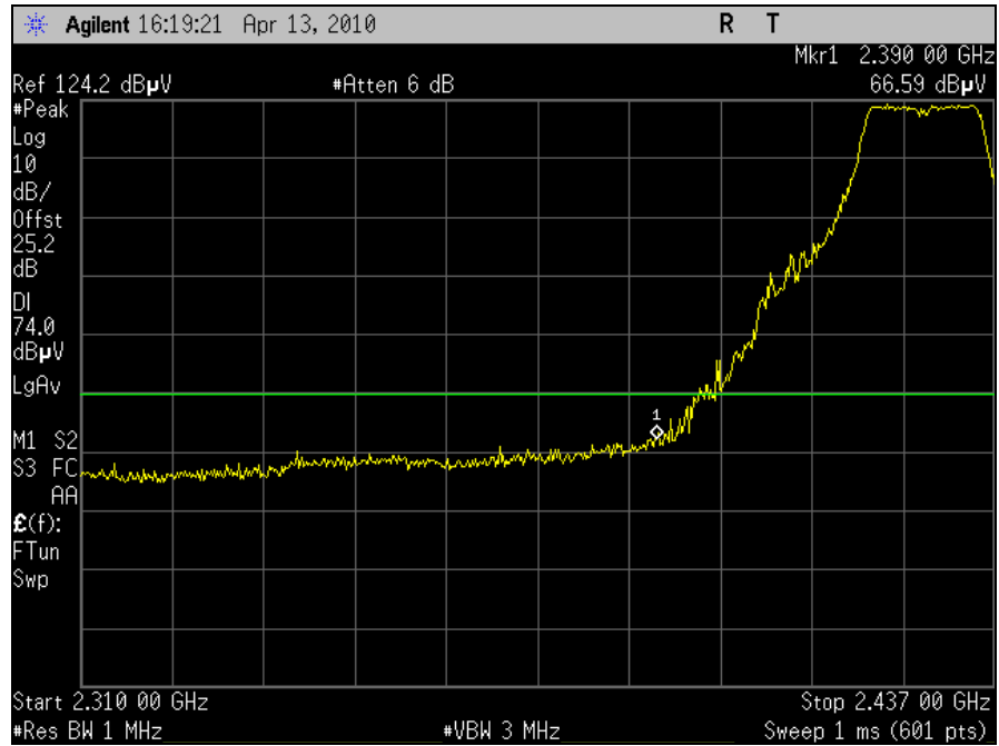
Plot 57. Radiated Restricted Band, Channel 4, 802.11n 20MHz, Peak
