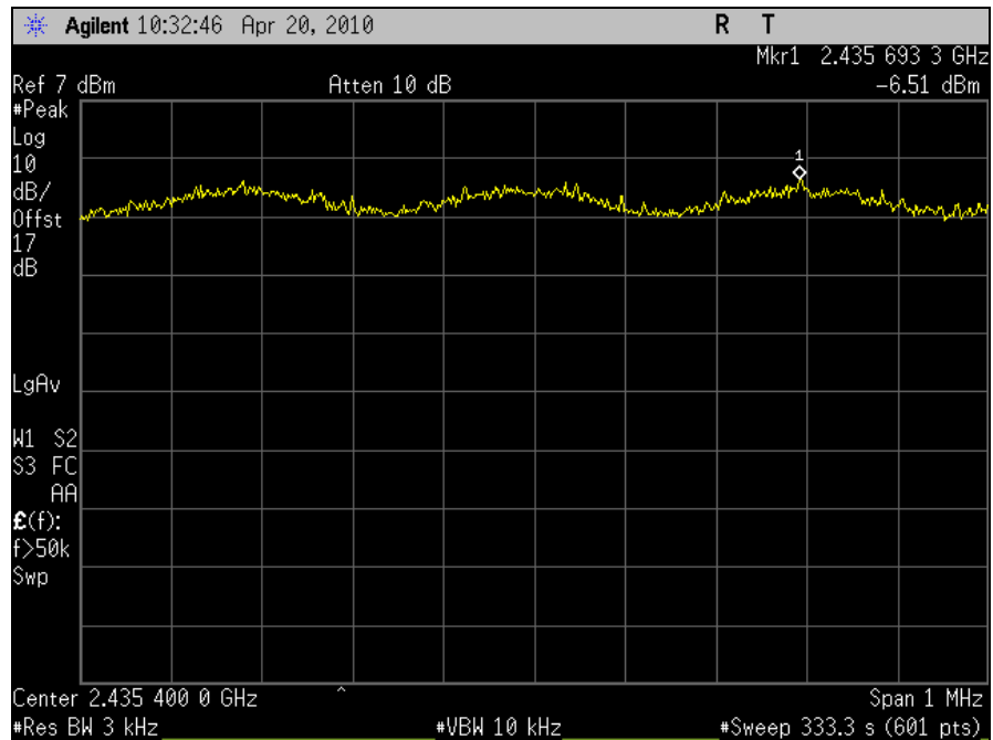
Plot 114. Spectral Power Density, 802.11n 20MHz, Combined Ports, Channel 6
