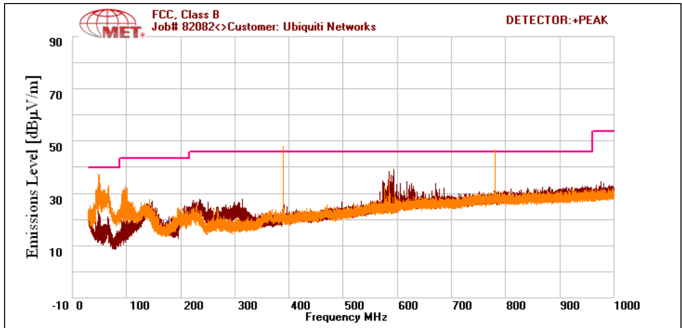
Plot 44. Radiated Emissions, Low Channel
