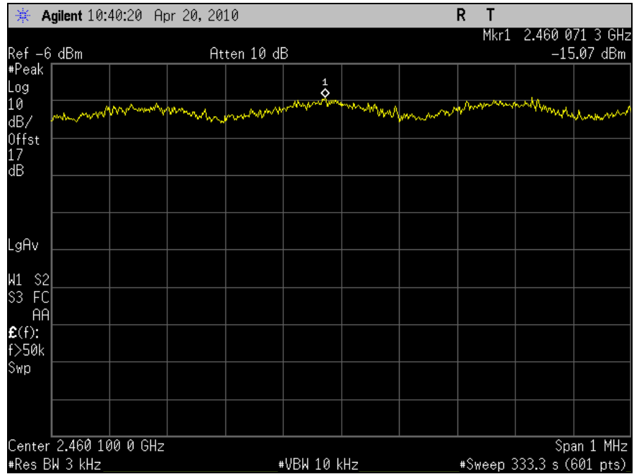
Plot 115. Spectral Power Density, 802.11n 20MHz, Combined Ports, Channel 11
