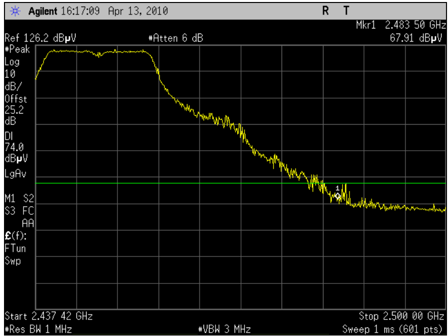
Plot 63. Radiated Restricted Band, Channel 8, 802.11n 20MHz, Peak
