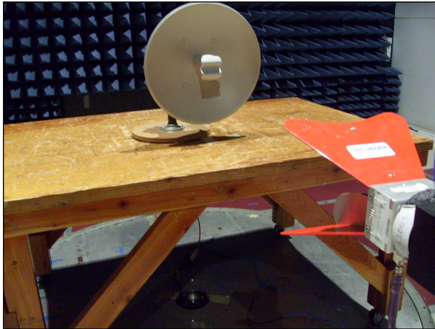
Photograph 8. Radiated Restricted Band, Test Setup @ 1m
