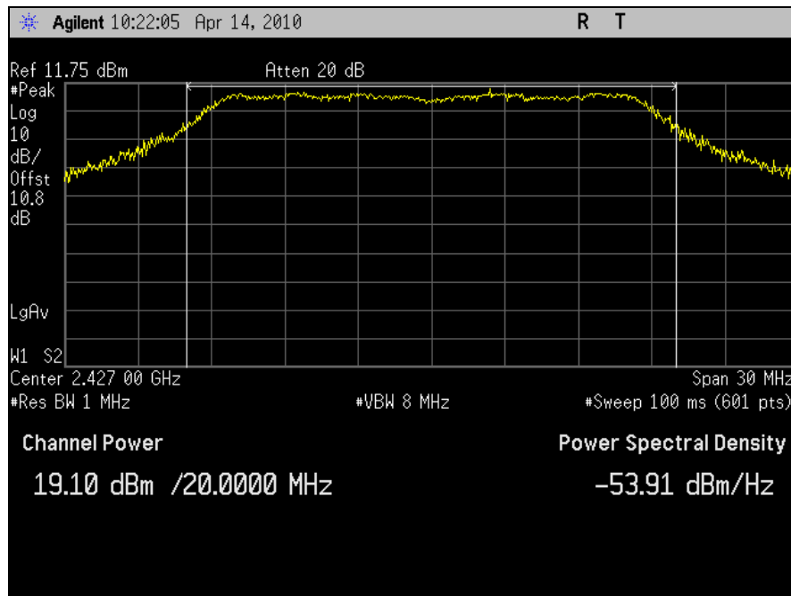
Plot 27. Conducted Output Power, 802.11n 20MHz, Port J5, Channel 4 (2427MHz)
