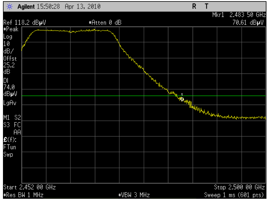
Plot 69. Radiated Restricted Band, Channel 11, 802.11n 20MHz, Peak
