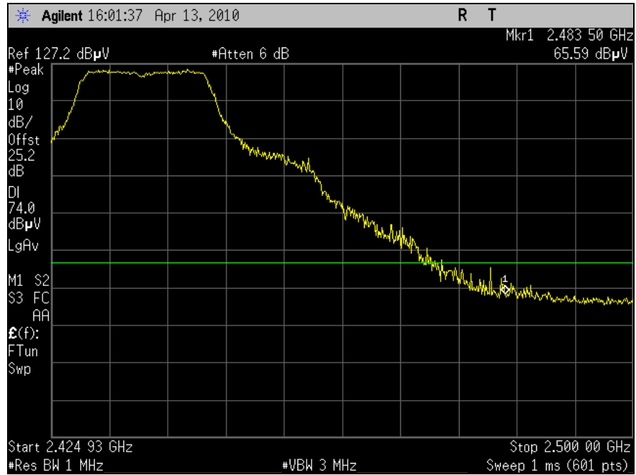
Plot 61. Radiated Restricted Band, Channel 6 - High, 802.11n 20MHz, Peak
