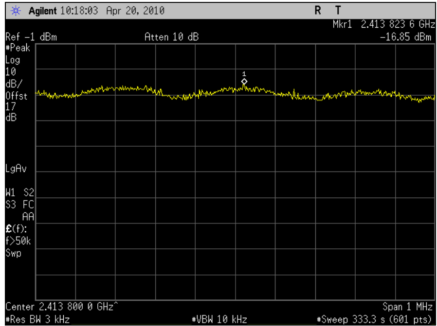
Plot 113. Spectral Power Density, 802.11n 20MHz, Combined Ports, Channel 1
