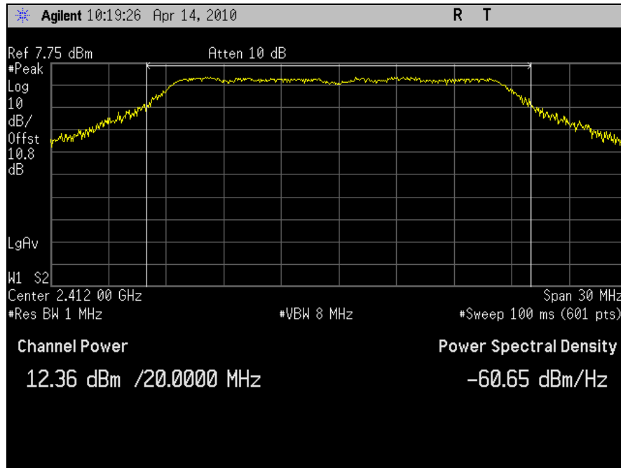
Plot 24. Conducted Output Power, 802.11n 20MHz, Port J5, Channel 1 (2412MHz)
