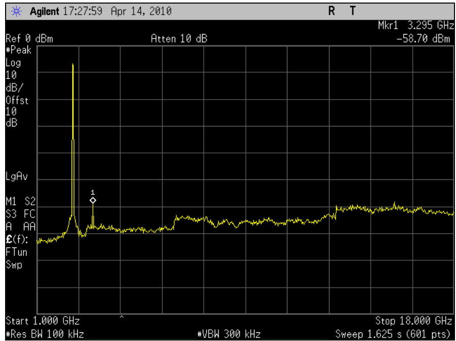
Plot 84. Conducted Spurious Emission, 802.11n 20MHz, Port J5, Channel 11, 1G-18GHz
