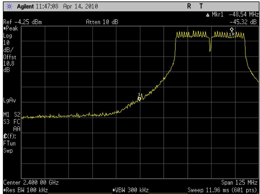
Plot 103. Lower Conducted Band Edge, 802.11n 40MHz
