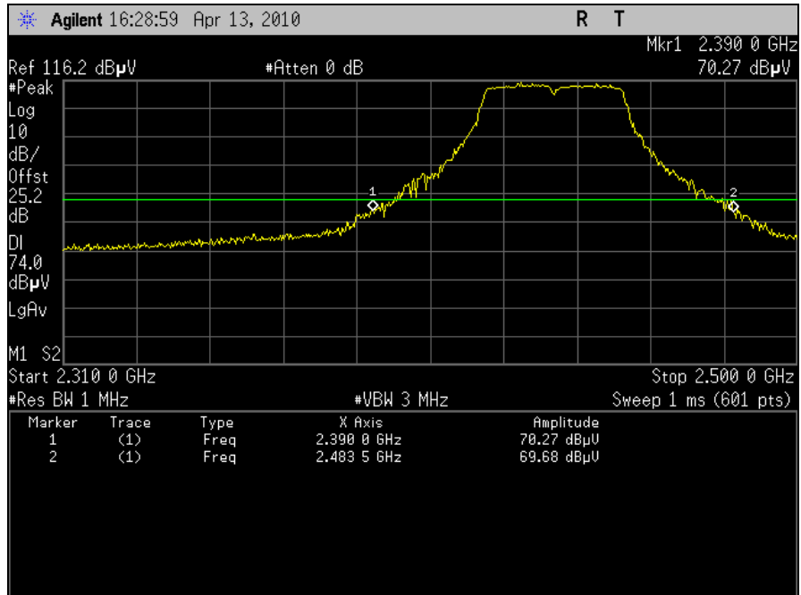
Plot 71. Radiated Restricted Band, Channel 6, 802.11n 40MHz, Peak
