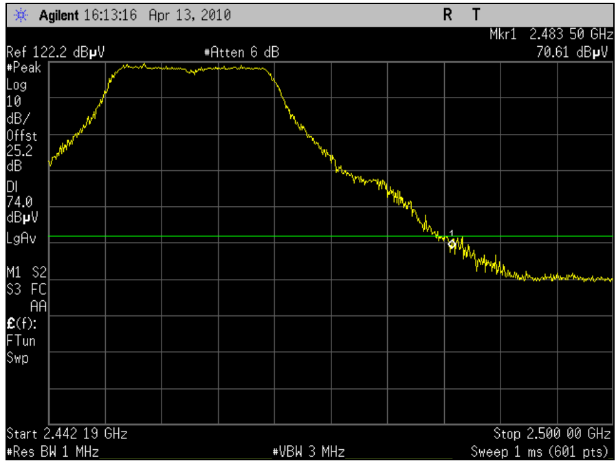
Plot 67. Radiated Restricted Band, Channel 10, 802.11n 20MHz, Peak
