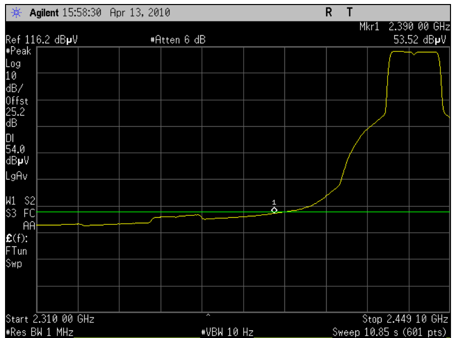
Plot 60. Radiated Restricted Band, Channel 6 - Low, 802.11n 20MHz, Average
