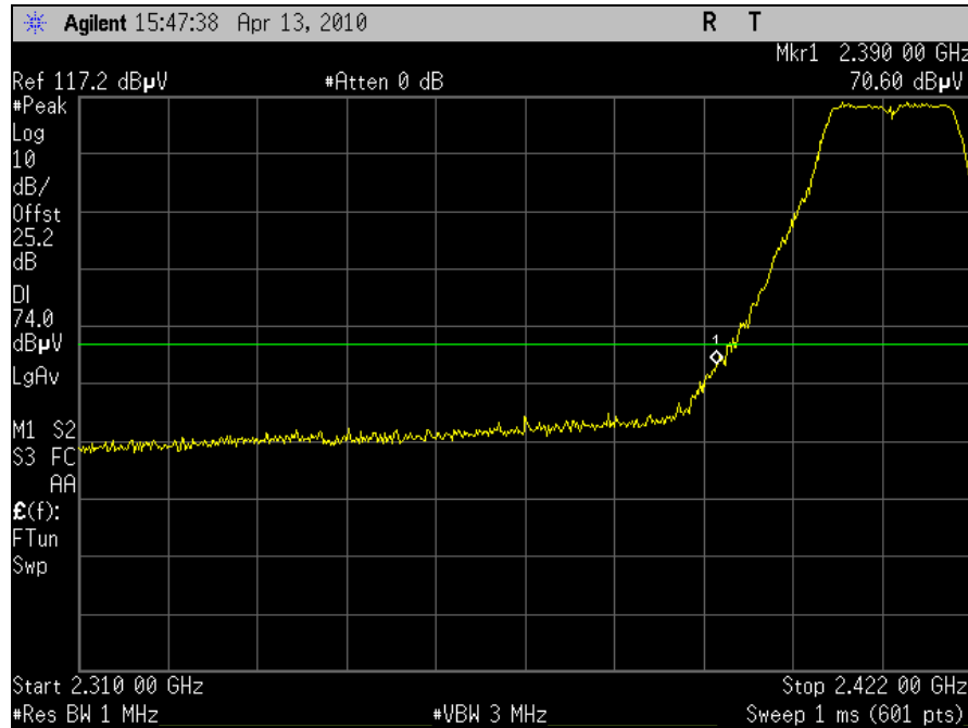
Plot 51. Radiated Restricted Band, Channel 1, 802.11n 20MHz, Peak
