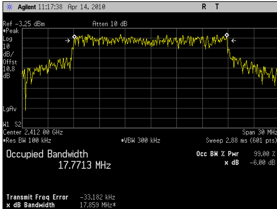
Plot 8. 6dB Occupied Bandwidth, 802.11n 20MHz, Port J5, Channel 1
