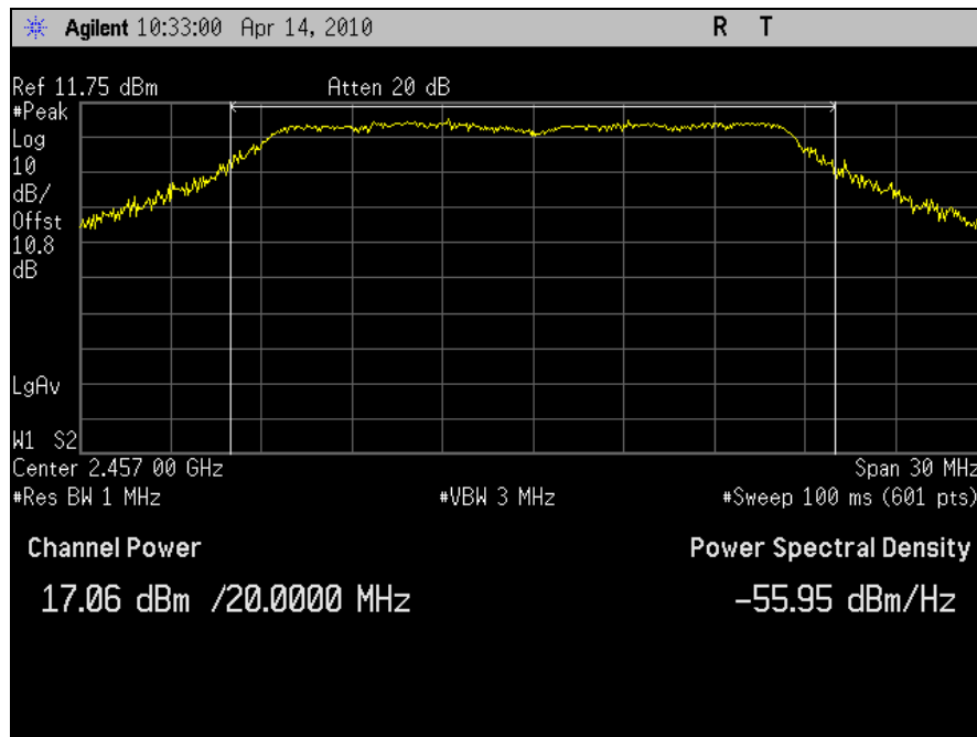
Plot 31. Conducted Output Power, 802.11n 20MHz, Port J5, Channel 10 (2457MHz)
