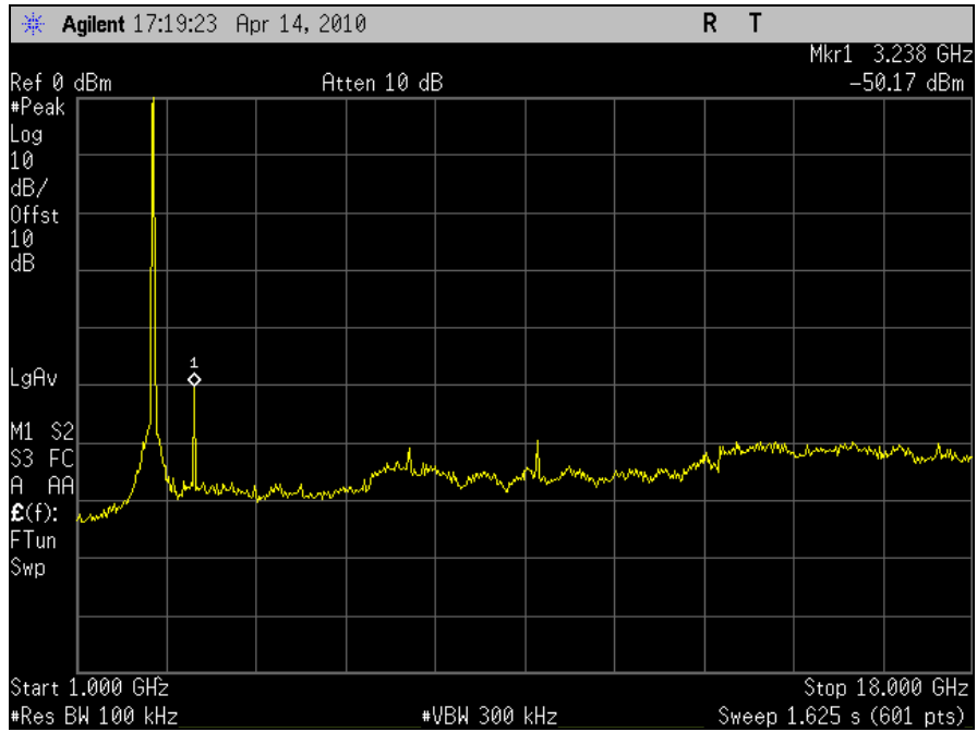
Plot 81. Conducted Spurious Emission, 802.11n 20MHz, Port J5, Channel 6, 1G-18GHz
