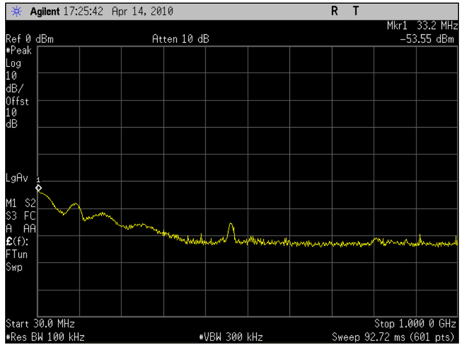
Plot 80. Conducted Spurious Emission, 802.11n 20MHz, Port J5, Channel 6, 30MHz - 1GHz
