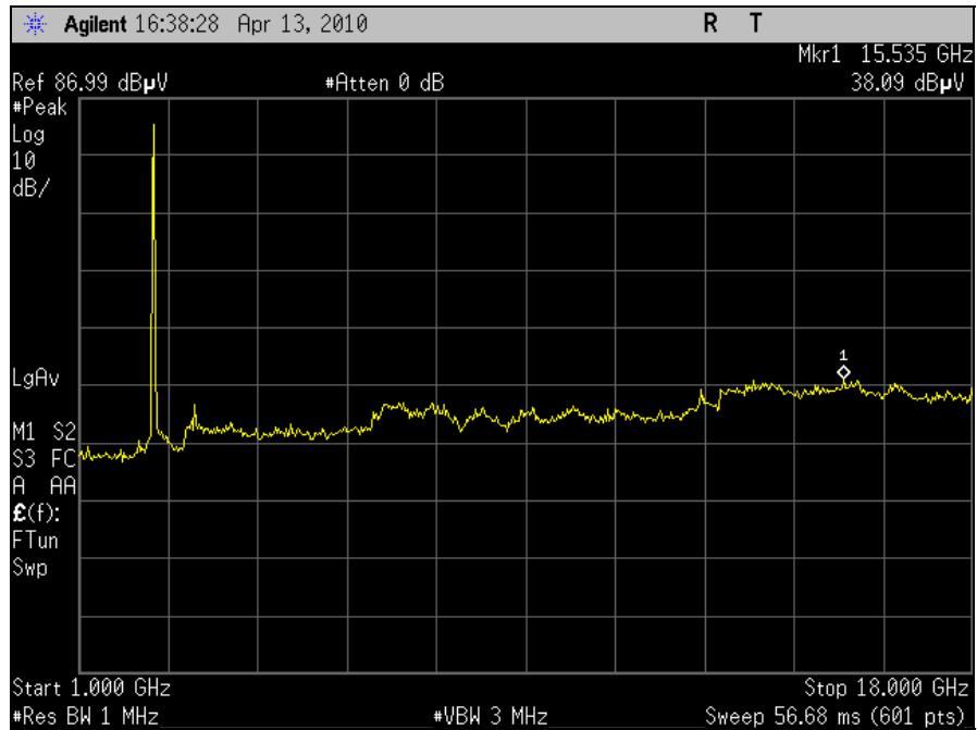
Plot 47. Radiated Spurious Emission, 802.11n 20MHz, Ch1, 1-18GHz
