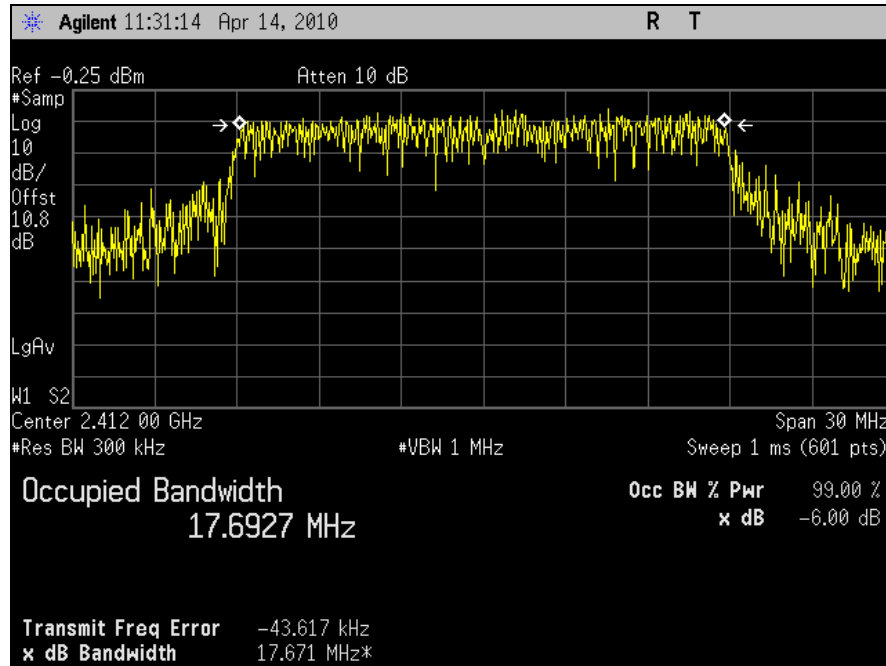
Plot 16. 99% Occupied Bandwidth, 802.11n 20MHz, Port J5, Channel 1
