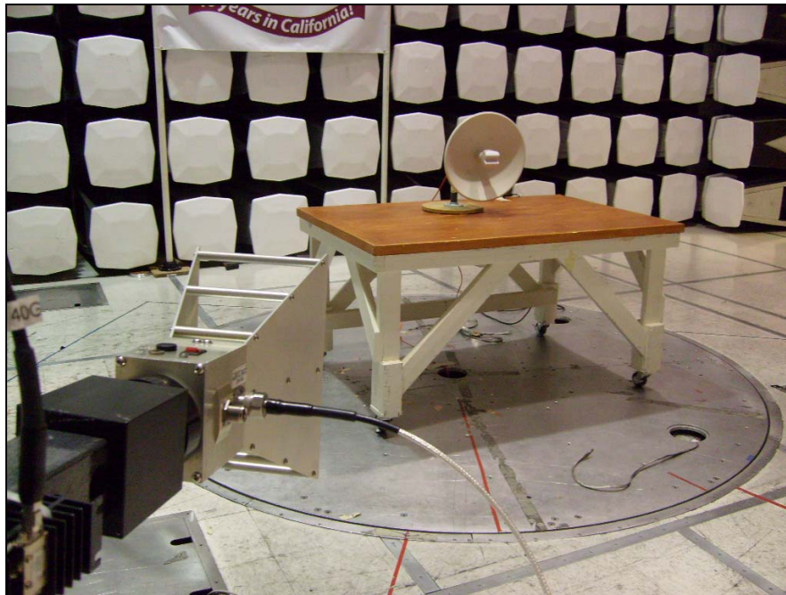
Photograph 7. Radiated Emissions, Test Setup, 1 GHz – 10 GHz
