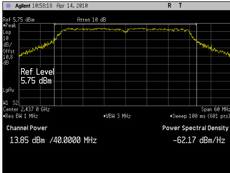
Plot 42. Conducted Output Power, 802.11n 40MHz, Port J5, Channel 6 (2437MHz)
