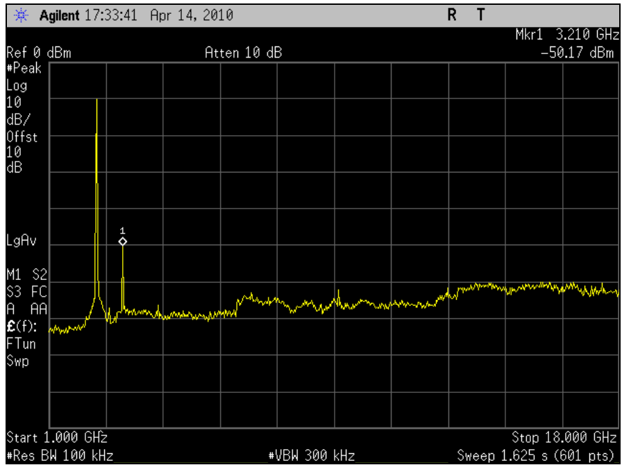
Plot 90. Conducted Spurious Emission, 802.11n 20MHz, Port J6, Channel 6, 1GHz - 18GHz
