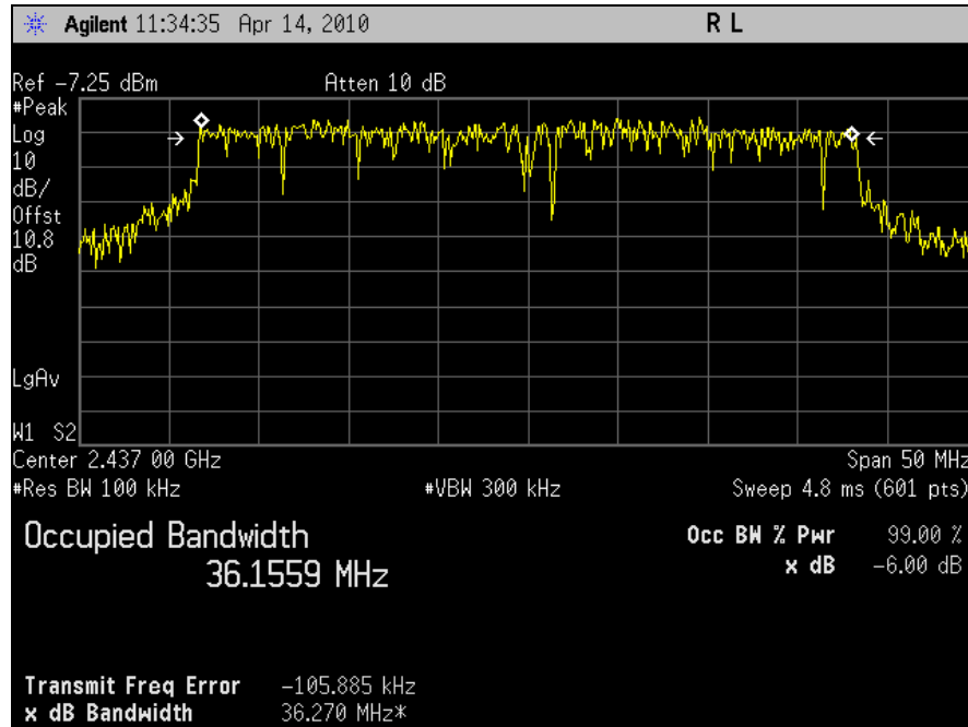
Plot 14. 6dB Occupied Bandwidth, 802.11n 40MHz, Port J5, Channel 6
