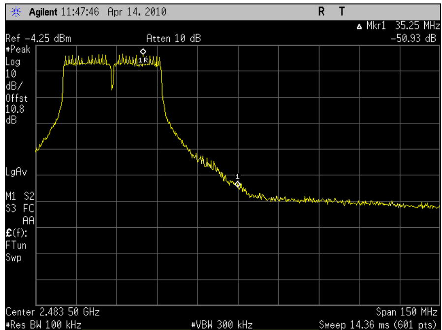
Plot 104. Upper Conducted Band Edge, 802.11n 40MHz
