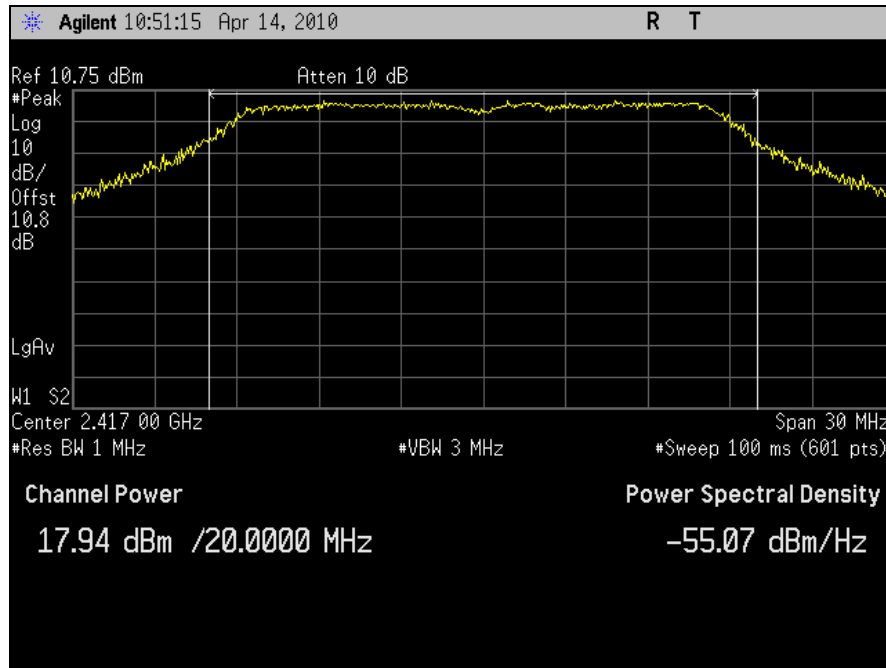
Plot 34. Conducted Output Power, 802.11n 20MHz, Port J6, Channel 2 (2417MHz)
