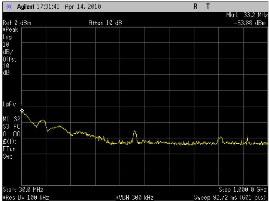
Plot 92. Conducted Spurious Emission, 802.11n 20MHz, Port J6, Channel 11, 30MHz - 1GHz
