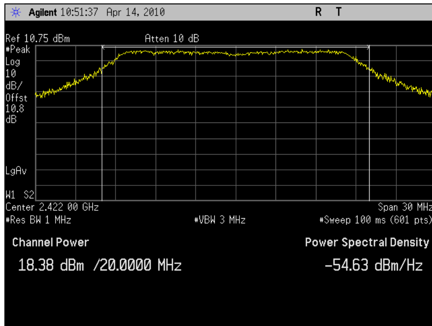
Plot 35. Conducted Output Power, 802.11n 20MHz, Port J6, Channel 3 (2422MHz)
