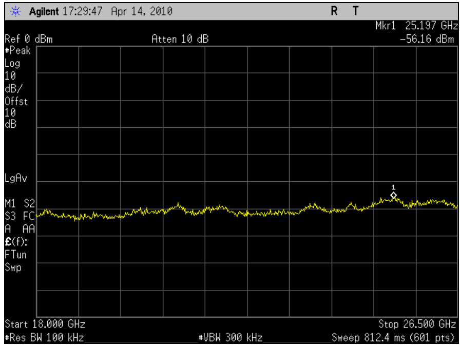
Plot 97. Conducted Spurious Emission, 802.11n 40MHz, Port J5, Channel 6, 18GHz-26.5GHz
