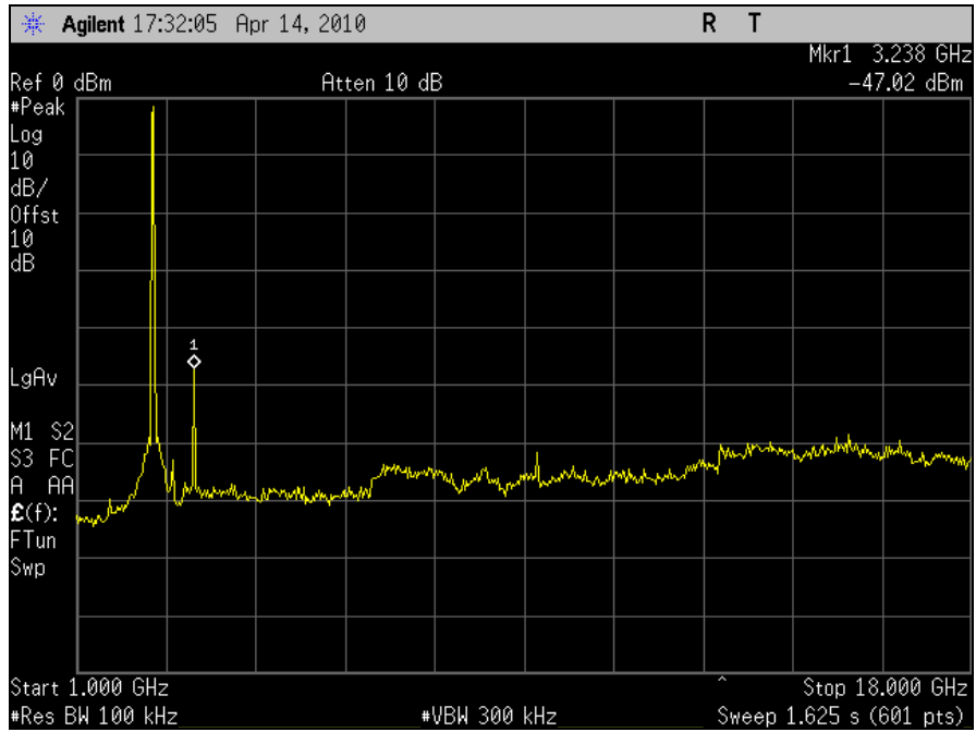
Plot 93. Conducted Spurious Emission, 802.11n 20MHz, Port J6, Channel 11, 1GHz - 18GHz
