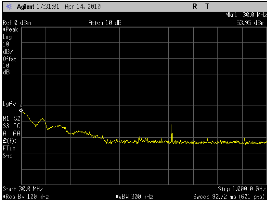
Plot 95. Conducted Spurious Emission, 802.11n 40MHz, Port J5, Channel 6, 30MHz - 1GHz
