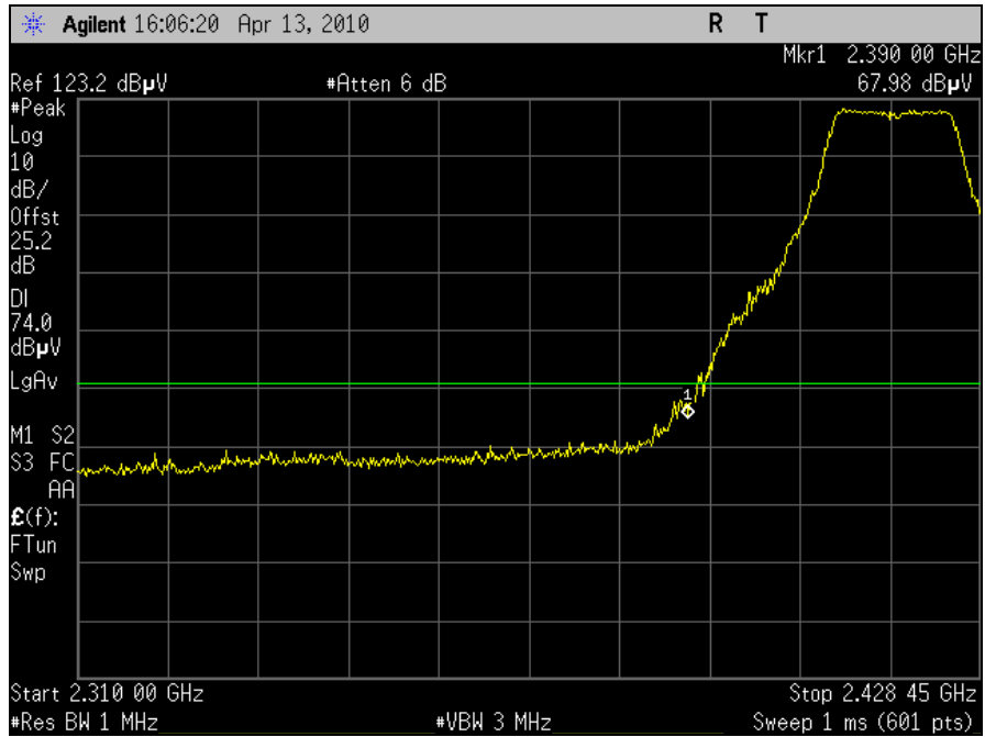
Plot 53. Radiated Restricted Band, Channel 2, 802.11n 20MHz, Peak
