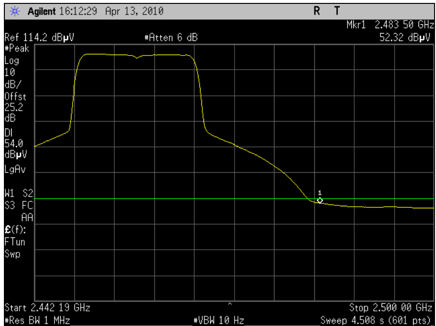
Plot 68. Radiated Restricted Band, Channel 10, 802.11n 20MHz, Average
