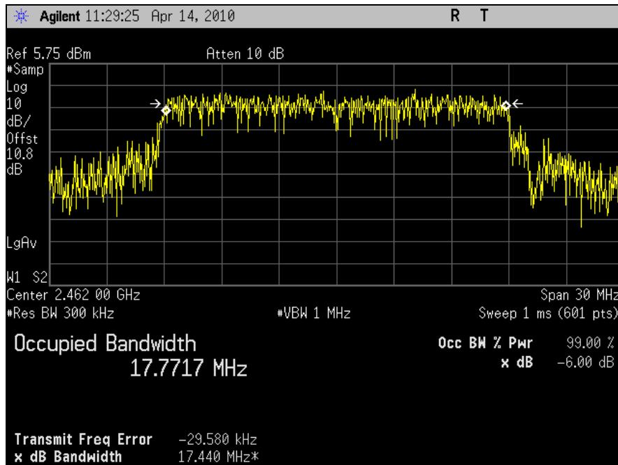
Plot 21. 99% Occupied Bandwidth, 802.11n 20MHz, Port J6, Channel 11
