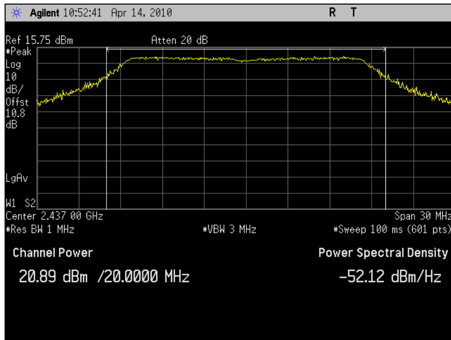
Plot 37. Conducted Output Power, 802.11n 20MHz, Port J6, Channel 6 (2437MHz)
