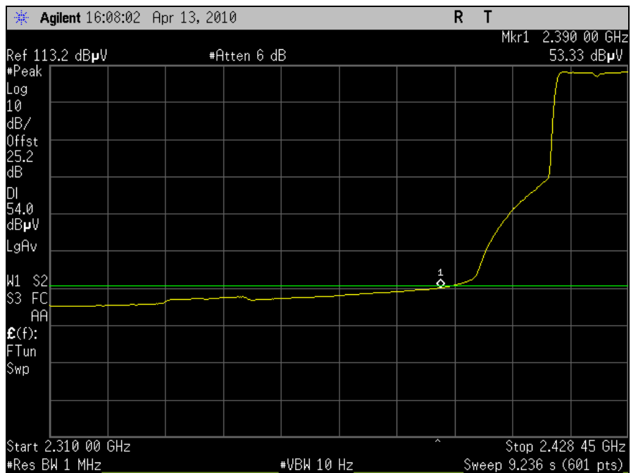
Plot 56. Radiated Restricted Band, Channel 3, 802.11n 20MHz, Average
