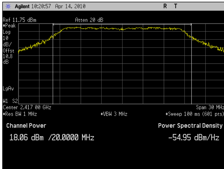
Plot 25. Conducted Output Power, 802.11n 20MHz, Port J5, Channel 2 (2417MHz)
