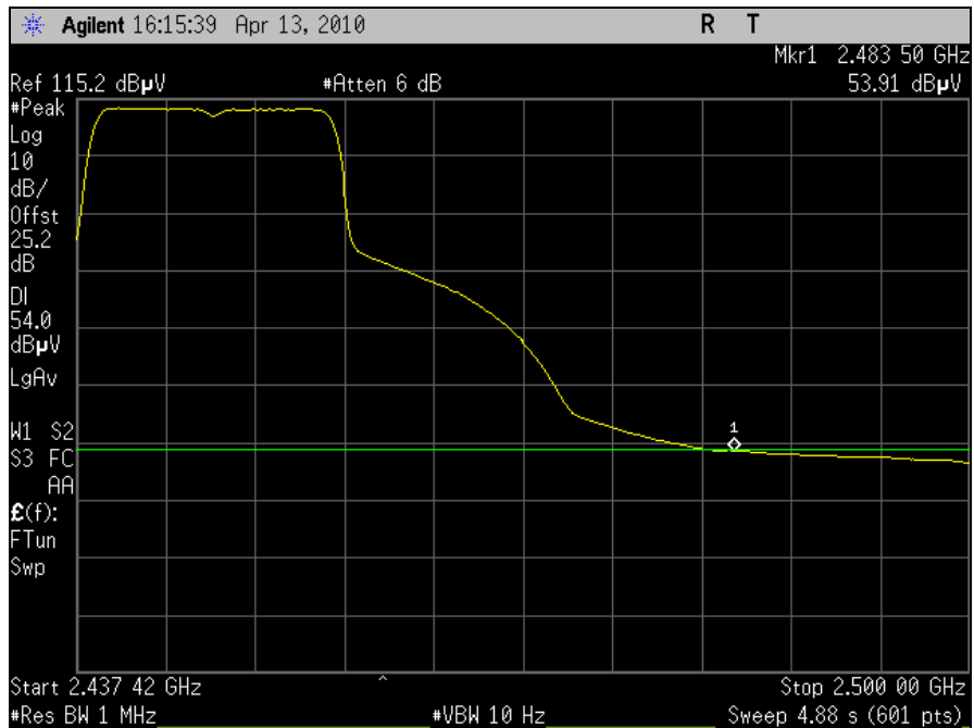
Plot 64. Radiated Restricted Band, Channel 8, 802.11n 20MHz, Average
