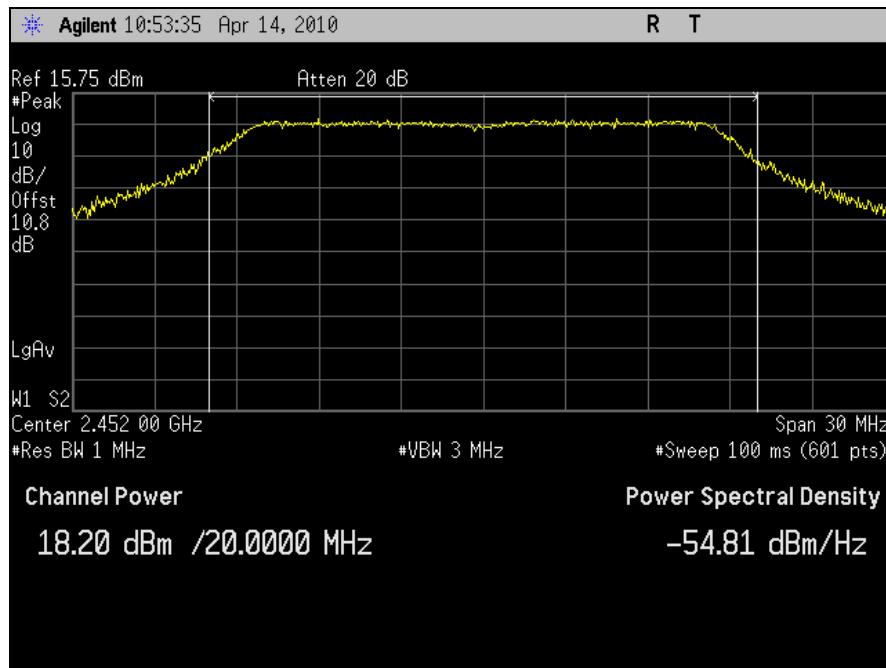
Plot 39. Conducted Output Power, 802.11n 20MHz, Port J6, Channel 9 (2452MHz)
