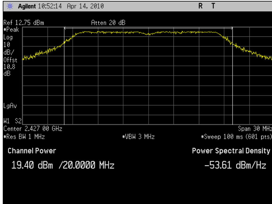
Plot 36. Conducted Output Power, 802.11n 20MHz, Port J6, Channel 4 (2427MHz)
