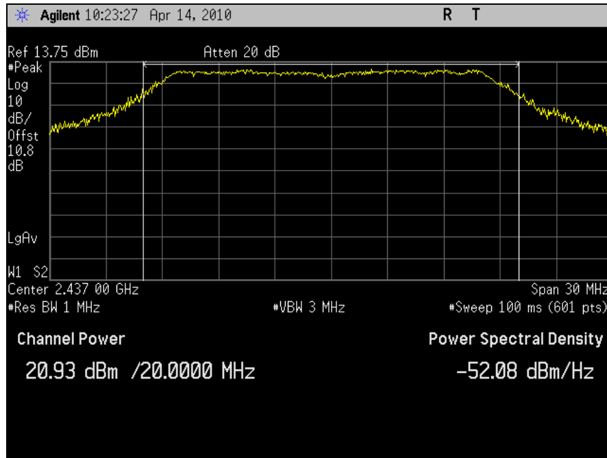
Plot 28. Conducted Output Power, 802.11n 20MHz, Port J5, Channel 6 (2437MHz)
