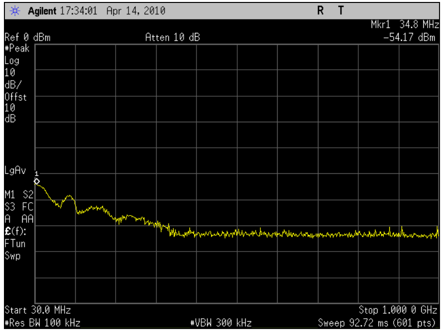
Plot 89. Conducted Spurious Emission, 802.11n 20MHz, Port J6, Channel 6, 30MHz - 1GHz
