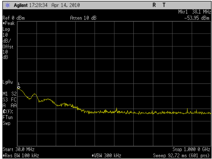
Plot 83. Conducted Spurious Emission, 802.11n 20MHz, Port J5, Channel 11, 30MHz - 1GHz
