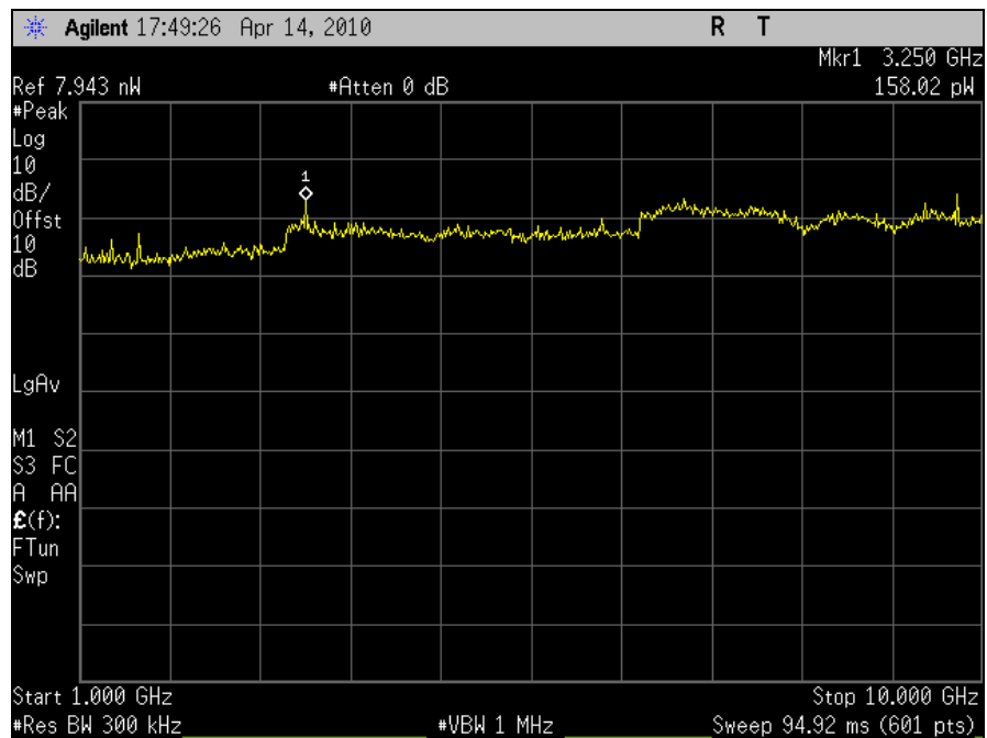
Plot 74. Conducted Rx Spurious 1 GHz – 10 GHz, Port J5
