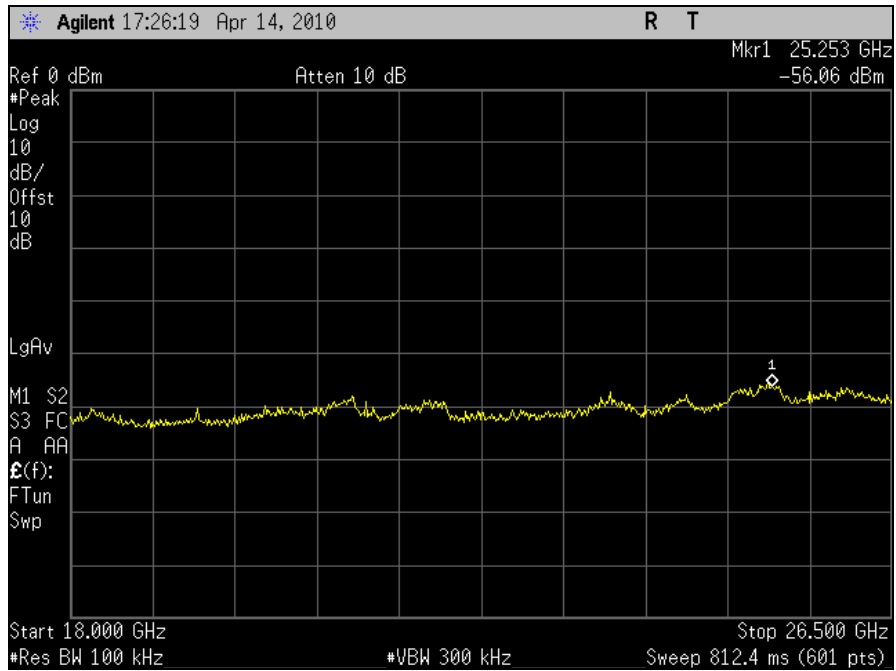
Plot 82. Conducted Spurious Emission, 802.11n 20MHz, Port J5, Channel 6, 18GHz - 26.5GHz
