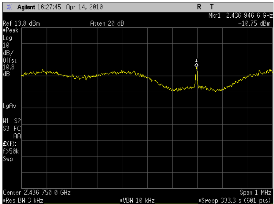
Plot 106. Spectral Power Density, 802.11n 20MHz, Port J5, Channel 6
