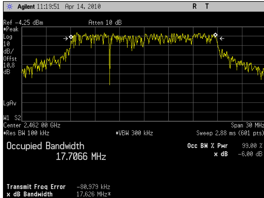
Plot 10. 6dB Occupied Bandwidth, 802.11n 20MHz, Port J5, Channel 11
