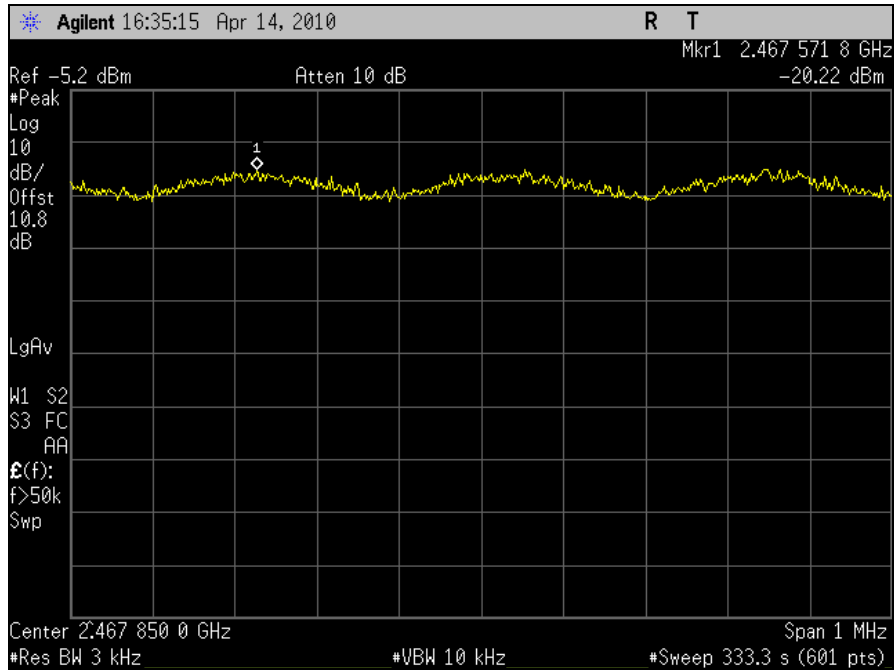
Plot 107. Spectral Power Density, 802.11n 20MHz, Port J5, Channel 11
