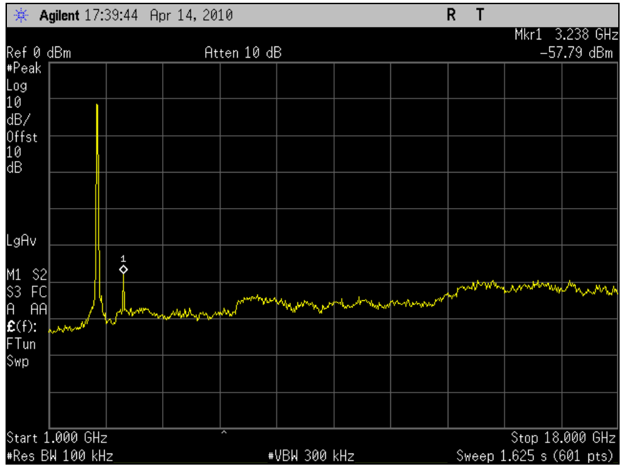
Plot 87. Conducted Spurious Emission, 802.11n 20MHz, Port J6, Channel 1, 1GHz - 18GHz
