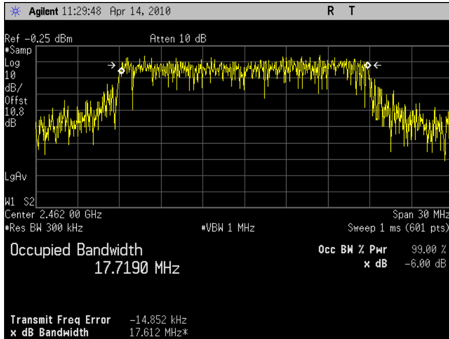
Plot 18. 99% Occupied Bandwidth, 802.11n 20MHz, Port J5, Channel 11
