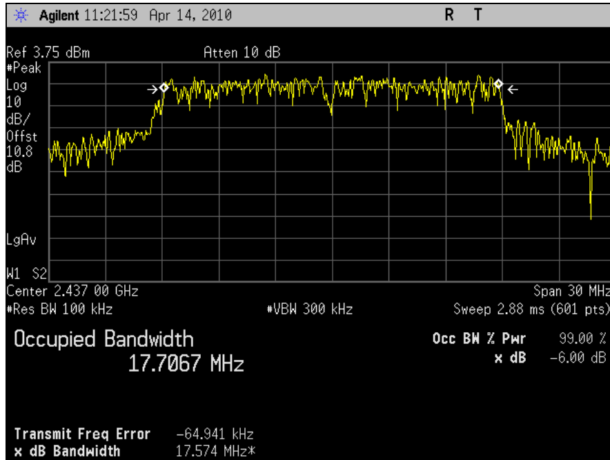
Plot 12. 6dB Occupied Bandwidth, 802.11n 20MHz, Port J6, Channel 6
