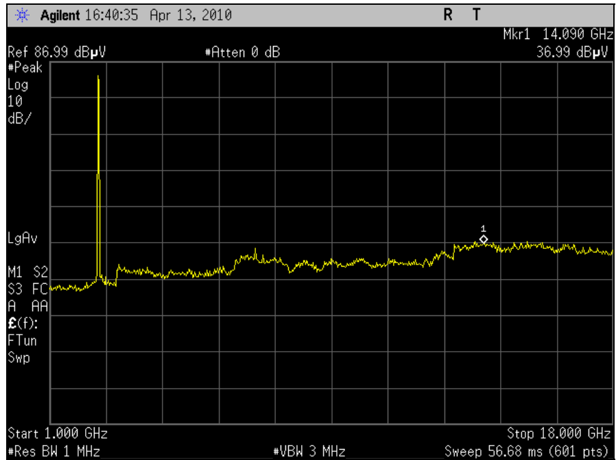
Plot 49. Radiated Spurious Emission, 802.11n 20MHz, Ch11, 1-18GHz
