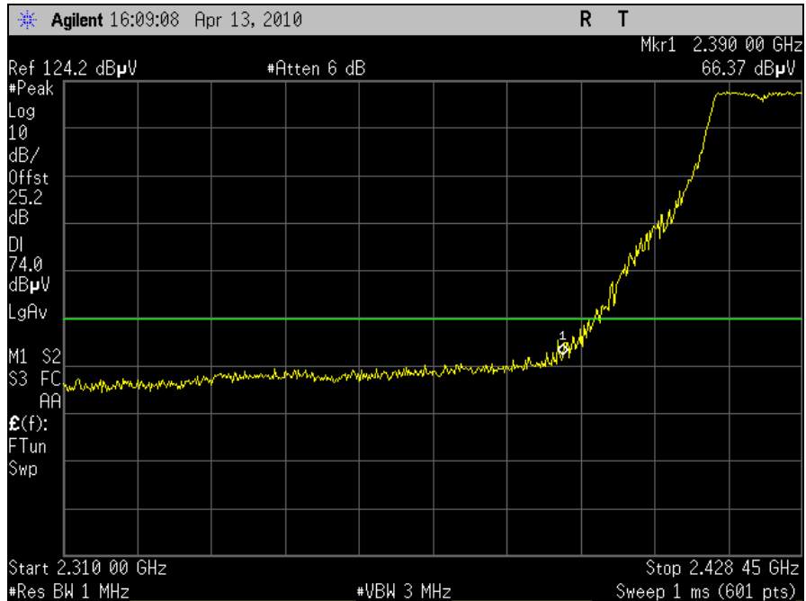
Plot 55. Radiated Restricted Band, Channel 3, 802.11n 20MHz, Peak
