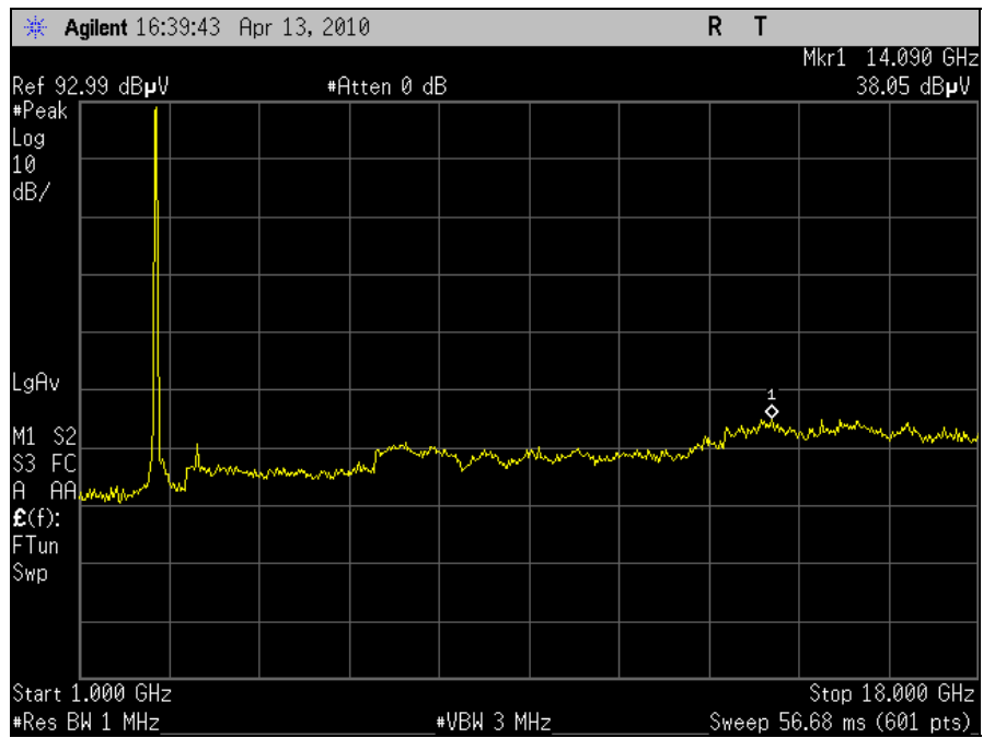
Plot 48. Radiated Spurious Emission, 802.11n 20MHz, Ch6, 1-18GHz
