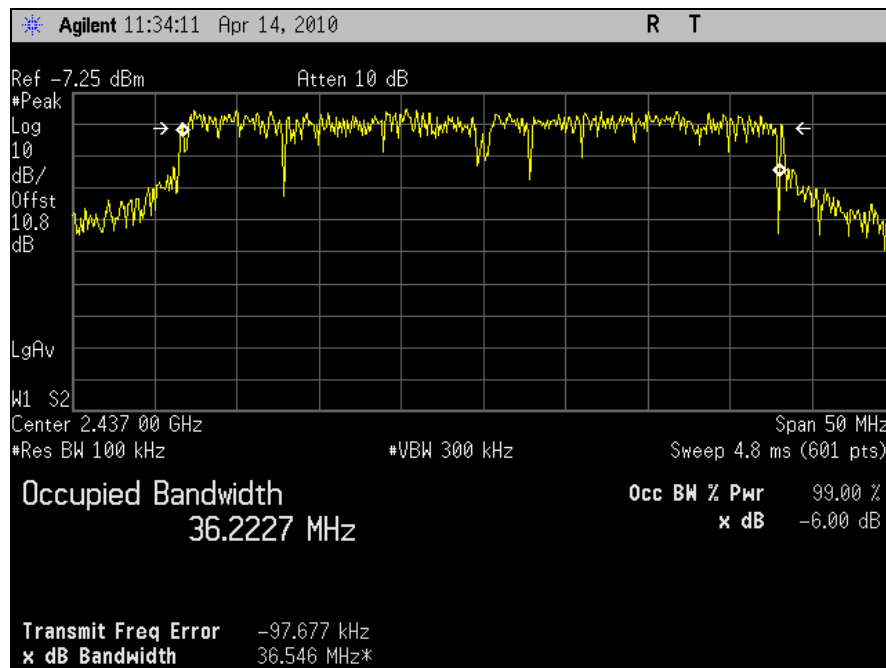
Plot 15. 6dB Occupied Bandwidth, 802.11n 40MHz, Port J6, Channel 6
