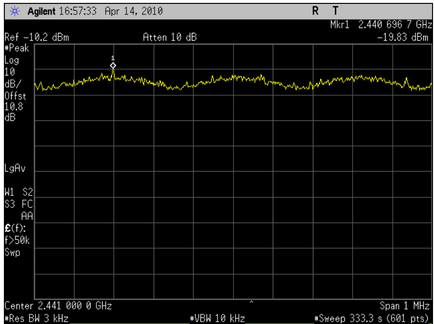
Plot 112. Spectral Power Density, 802.11n 40MHz, Port J6, Channel 6
