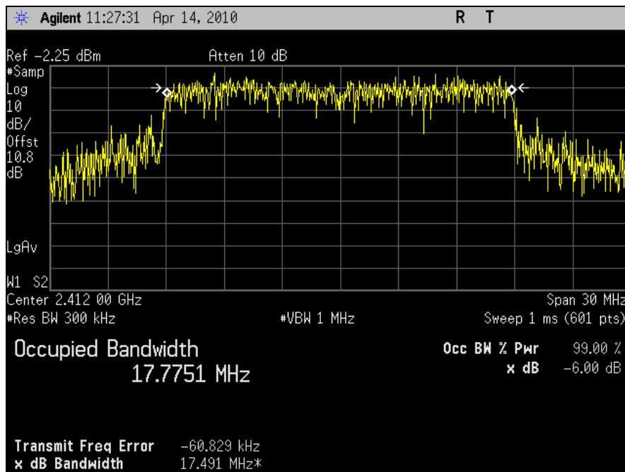
Plot 19. 99% Occupied Bandwidth, 802.11n 20MHz, Port J6, Channel 1
