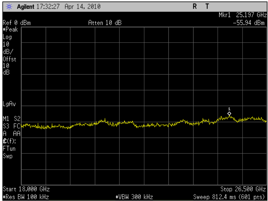
Plot 94. Conducted Spurious Emission, 802.11n 20MHz, Port J6, Channel 11, 18GHz - 26.5GHz
