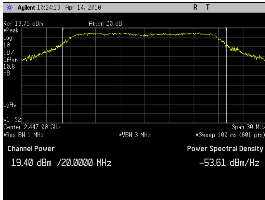
Plot 29. Conducted Output Power, 802.11n 20MHz, Port J5, Channel 8 (2447MHz)
