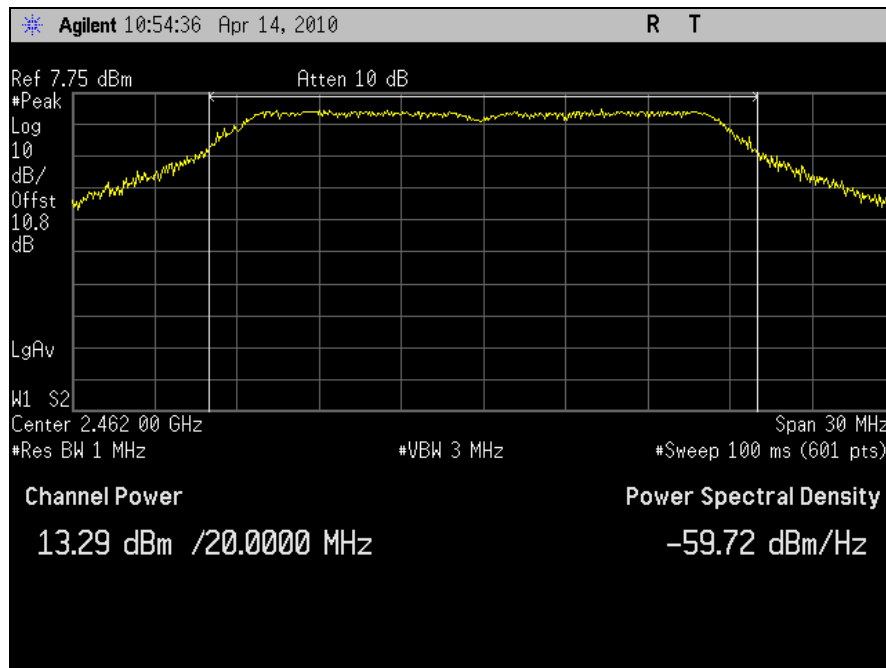
Plot 41. Conducted Output Power, 802.11n 20MHz, Port J6, Channel 11 (2462MHz)
