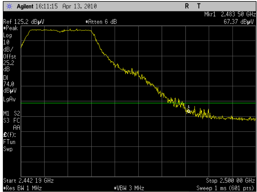
Plot 65. Radiated Restricted Band, Channel 9, 802.11n 20MHz, Peak
