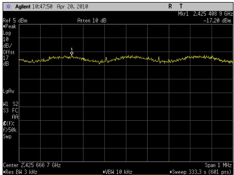
Plot 116. Spectral Power Density, 802.11n 40MHz, Combined Ports, Channel 6
