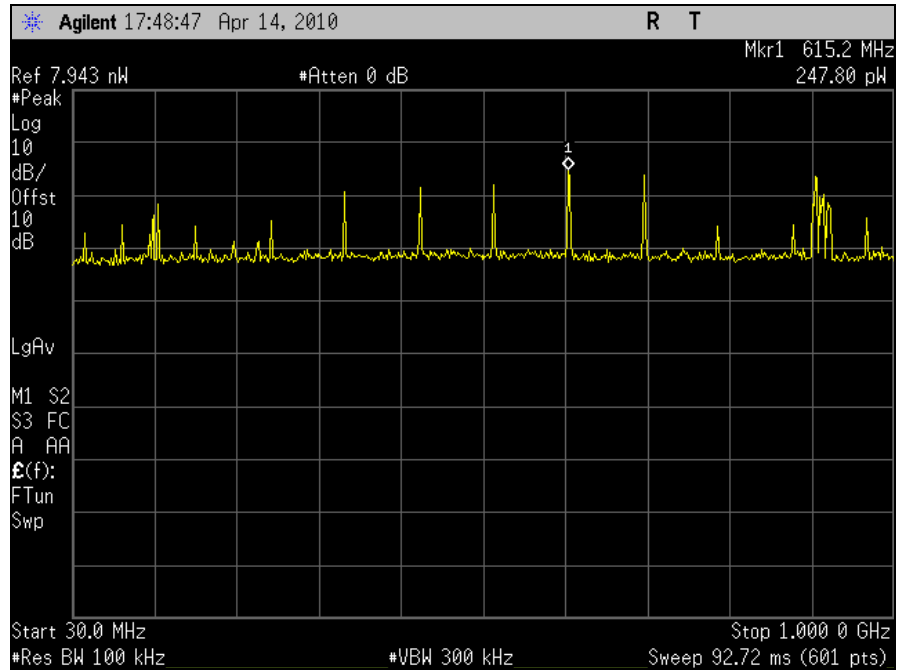
Plot 73. Conducted Rx Spurious 30 MHz – 1 GHz, Port J5
