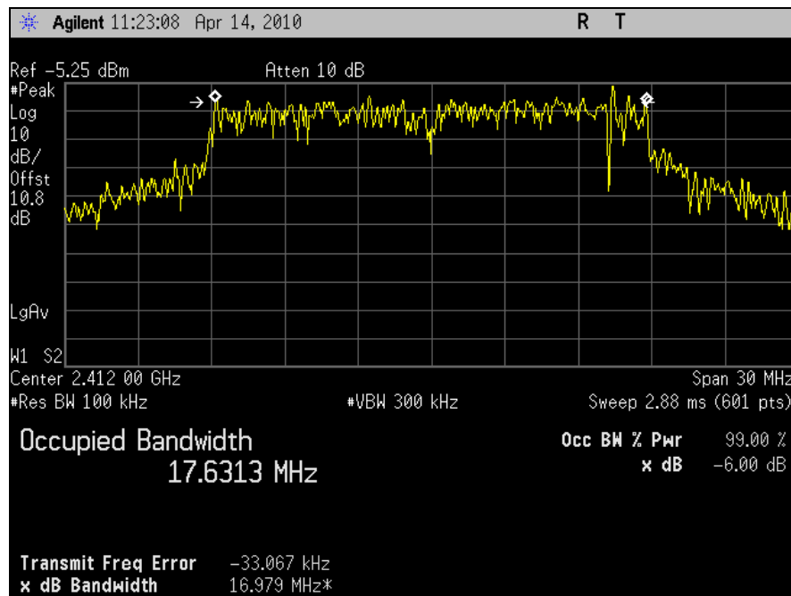
Plot 11. 6dB Occupied Bandwidth, 802.11n 20MHz, Port J6, Channel 1
