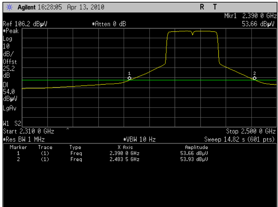
Plot 72. Radiated Restricted Band, Channel 6, 802.11n 40MHz, Average
