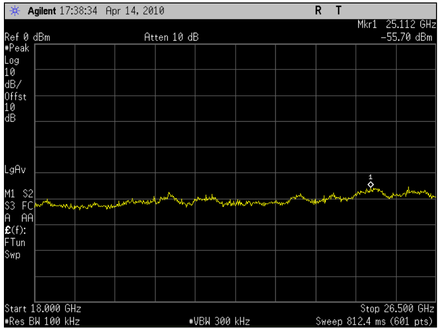
Plot 100. Conducted Spurious Emission, 802.11n 40MHz, Port J6, Channel 6, 18GHz-26.5GHz
