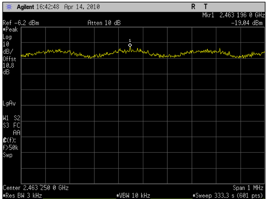
Plot 110. Spectral Power Density, 802.11n 20MHz, Port J5, Channel 11
