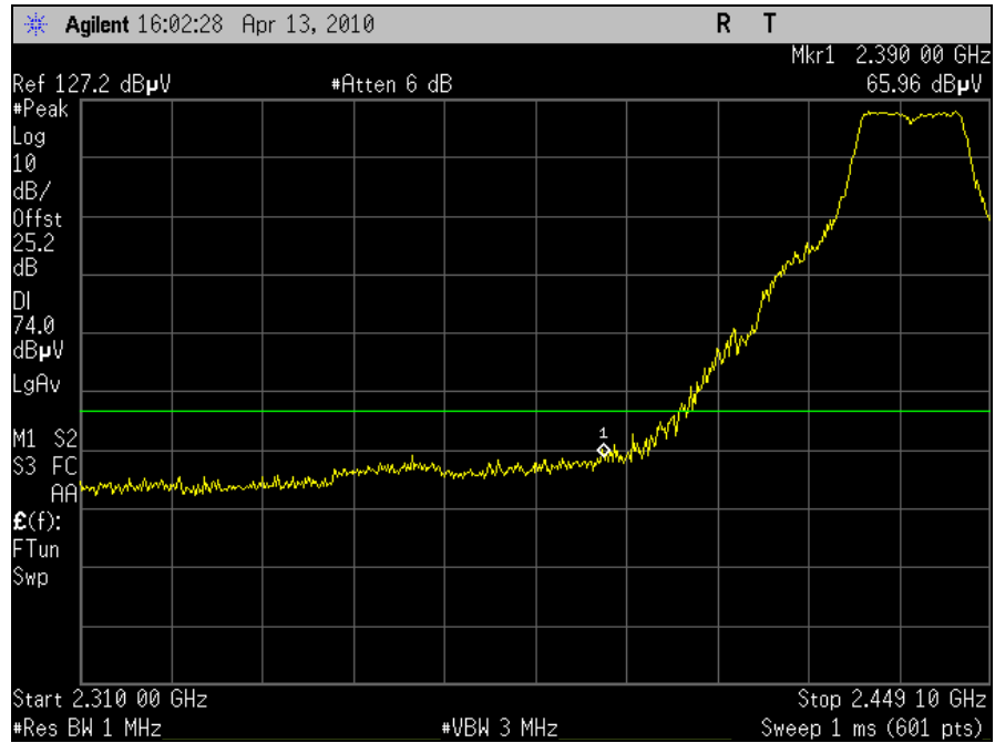
Plot 59. Radiated Restricted Band, Channel 6 - Low, 802.11n 20MHz, Peak
