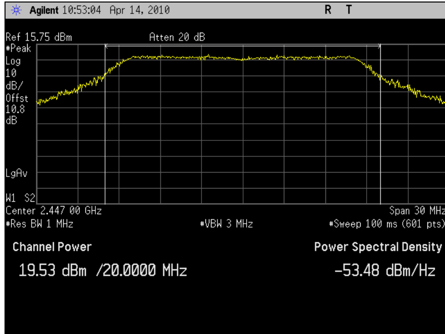
Plot 38. Conducted Output Power, 802.11n 20MHz, Port J6, Channel 8 (2447MHz)
