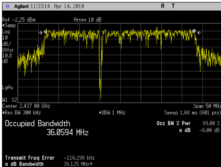
Plot 23. 99% Occupied Bandwidth, 802.11n 40MHz, Port J6, Channel 6
