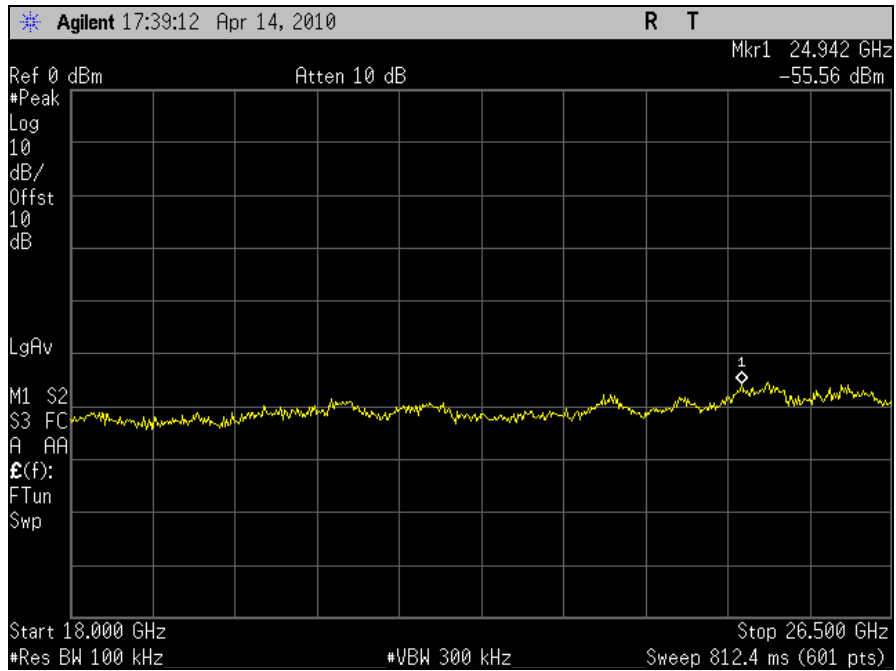
Plot 88. Conducted Spurious Emission, 802.11n 20MHz, Port J6, Channel 1, 18GHz - 26.5GHz
