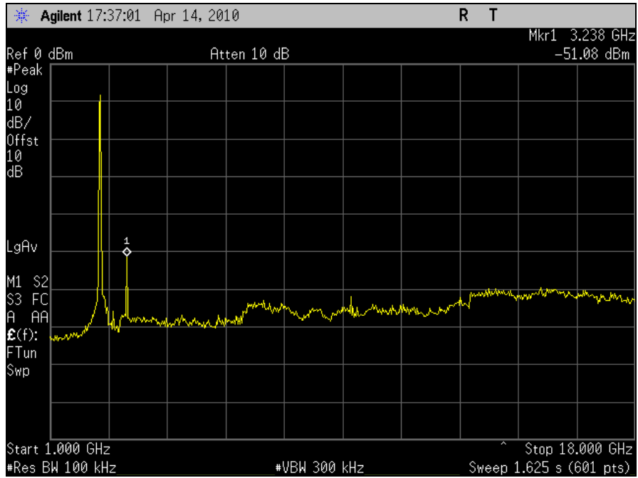
Plot 99. Conducted Spurious Emission, 802.11n 40MHz, Port J6, Channel 6, 1GHz - 18GHz
