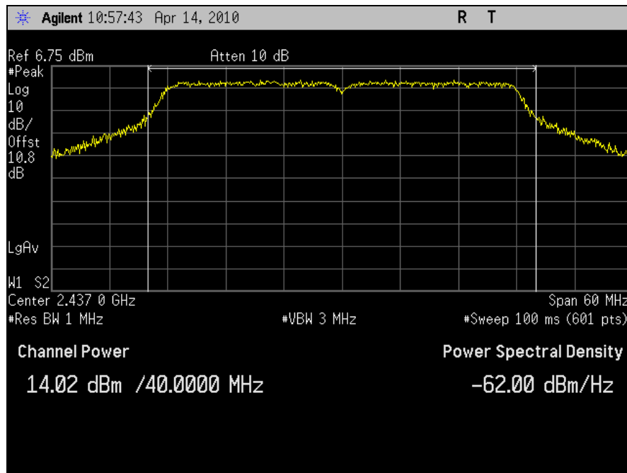
Plot 43. Conducted Output Power, 802.11n 40MHz, Port J6, Channel 6 (2437MHz)
