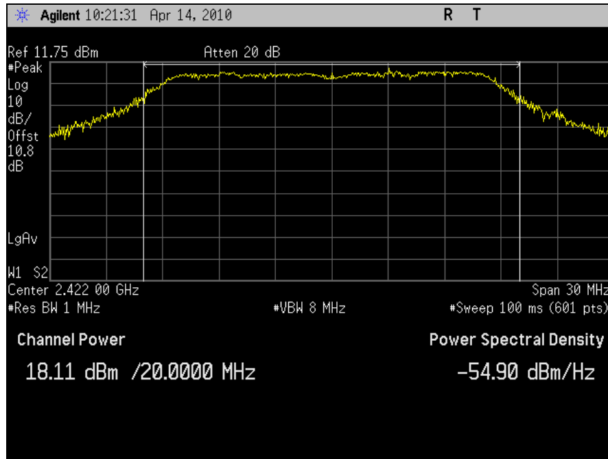
Plot 26. Conducted Output Power, 802.11n 20MHz, Port J5, Channel 3 (2422MHz)
