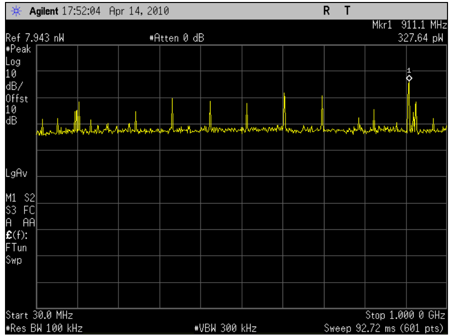
Plot 75. Conducted Rx Spurious 30 MHz – 1 GHz, Port J6
