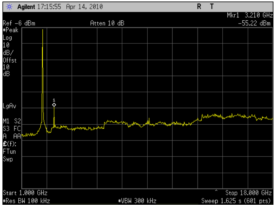
Plot 78. Conducted Spurious Emission, 802.11n 20MHz, Port J5, Channel 1, 1G-18GHz
