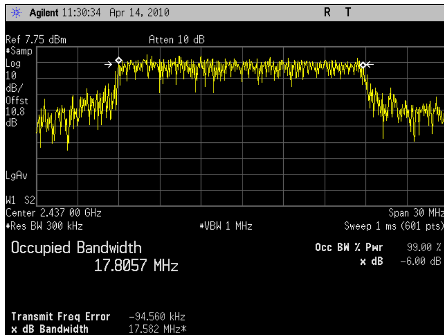
Plot 17. 99% Occupied Bandwidth, 802.11n 20MHz, Port J5, Channel 6
