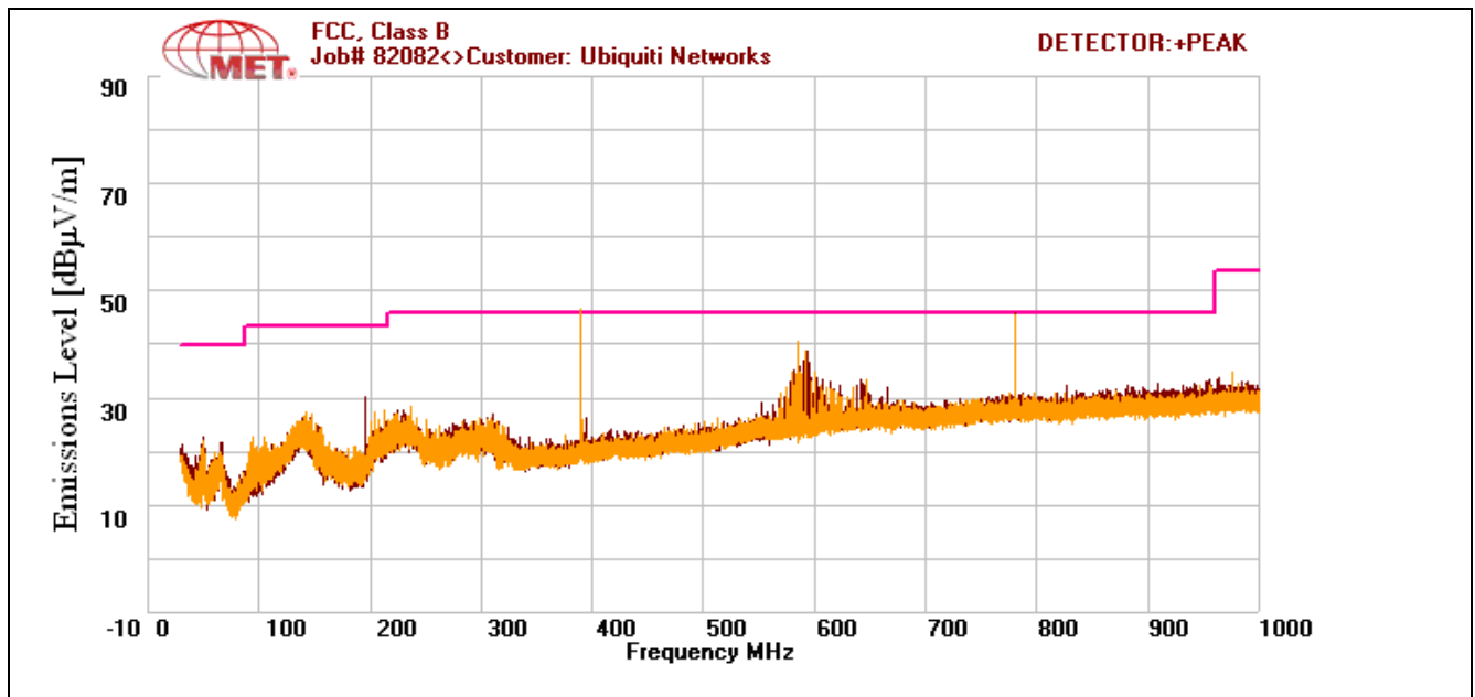
Plot 46. Radiated Emissions, High Channel
