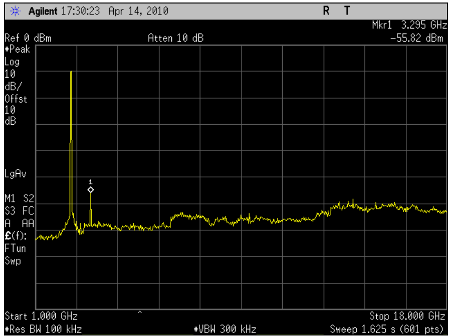
Plot 96. Conducted Spurious Emission, 802.11n 40MHz, Port J5, Channel 6, 1GHz - 18GHz
