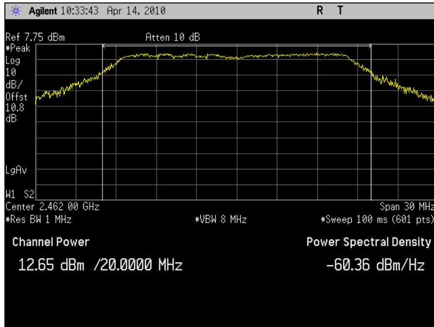
Plot 32. Conducted Output Power, 802.11n 20MHz, Port J5, Channel 11 (2462MHz)
