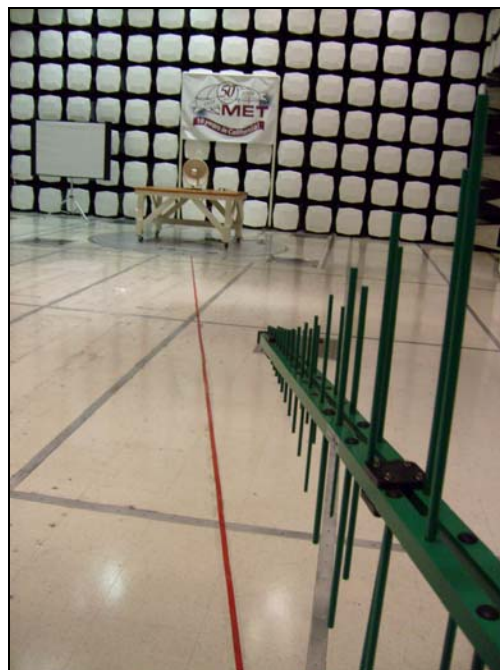
Photograph 4. Radiated Emission, Test Setup, IC Limits
