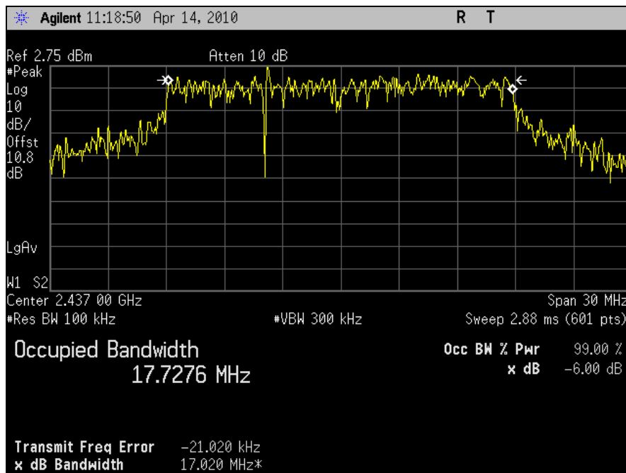
Plot 9. 6dB Occupied Bandwidth, 802.11n 20MHz, Port J5, Channel 6
