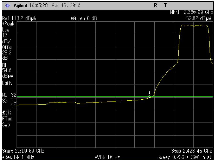
Plot 54. Radiated Restricted Band, Channel 2, 802.11n 20MHz, Average
