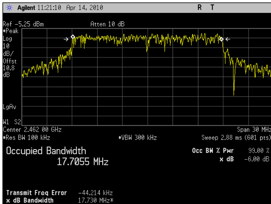
Plot 13. 6dB Occupied Bandwidth, 802.11n 20MHz, Port J6, Channel 11
