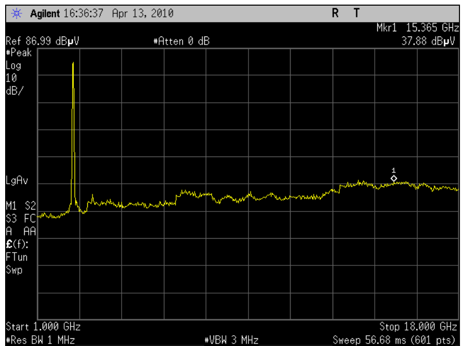
Plot 50. Radiated Spurious Emission, 802.11n 40MHz, Ch6, 1-18GHz
