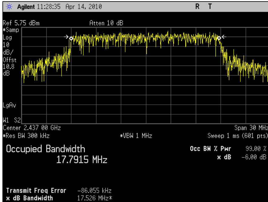
Plot 20. 99% Occupied Bandwidth, 802.11n 20MHz, Port J6, Channel 6
