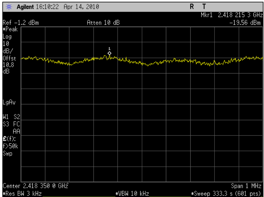
Plot 108. Spectral Power Density, 802.11n 20MHz, Port J6, Channel 1
