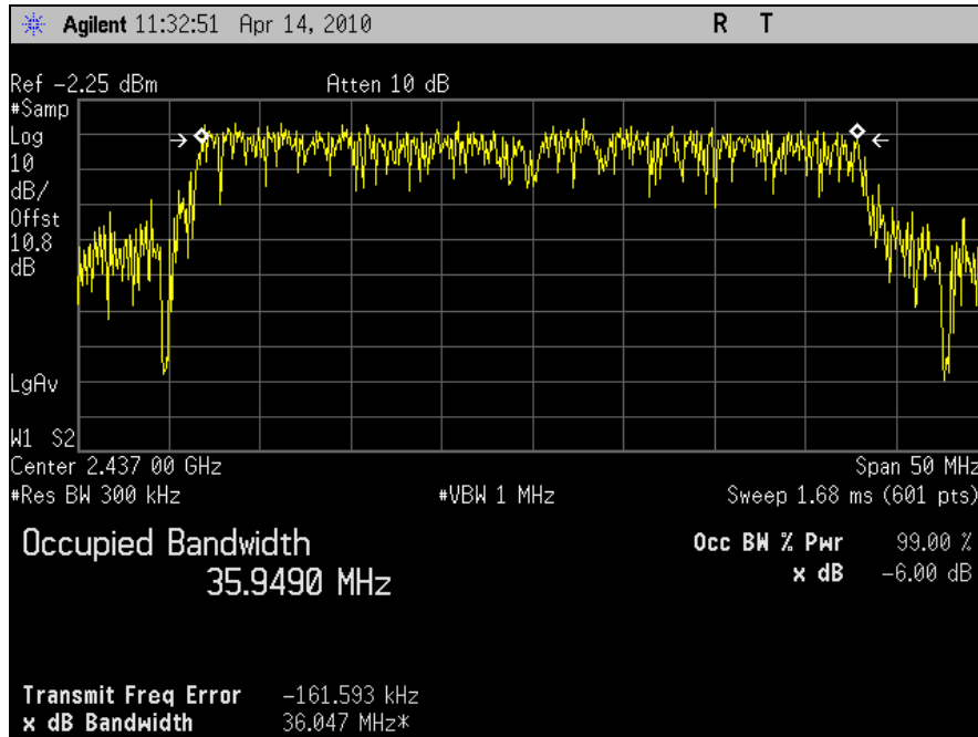
Plot 22. 99% Occupied Bandwidth, 802.11n 40MHz, Port J5, Channel 6
