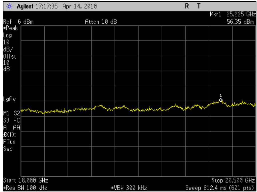
Plot 79. Conducted Spurious Emission, 802.11n 20MHz, Port J5, Channel 1, 18GHz - 26.5GHz
