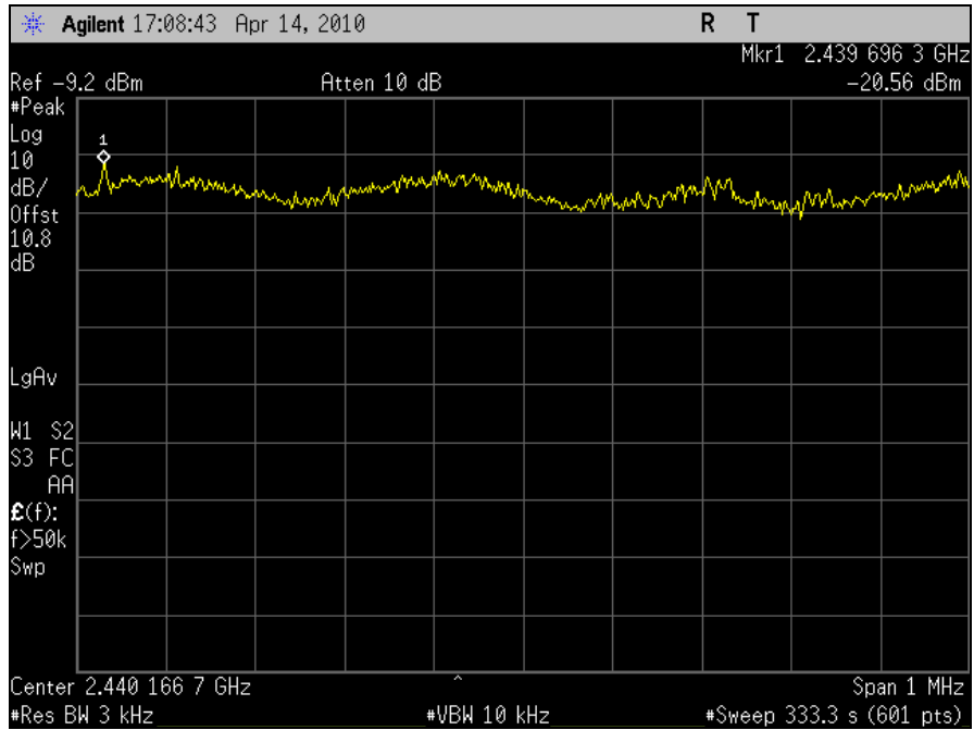
Plot 111. Spectral Power Density, 802.11n 40MHz, Port J5, Channel 6
