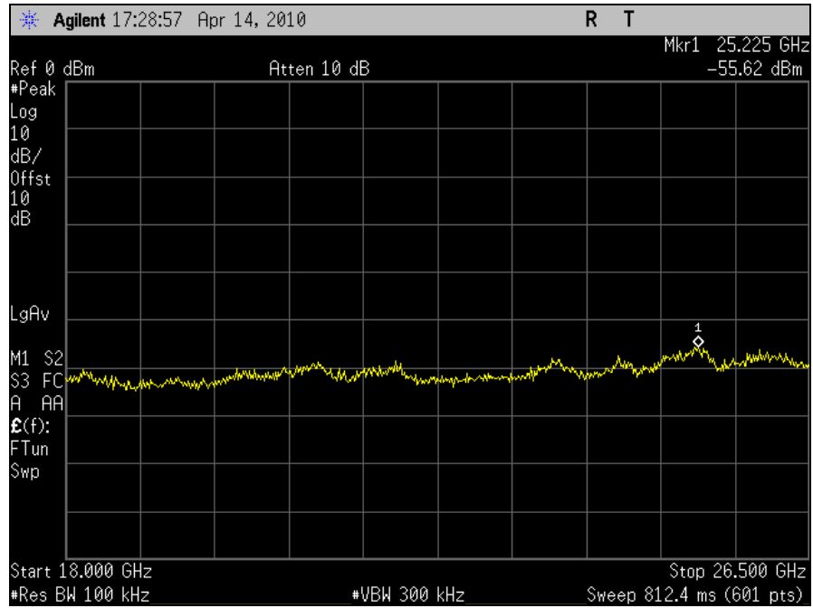
Plot 85. Conducted Spurious Emission, 802.11n 20MHz, Port J5, Channel 11, 18GHz - 26.5GHz
