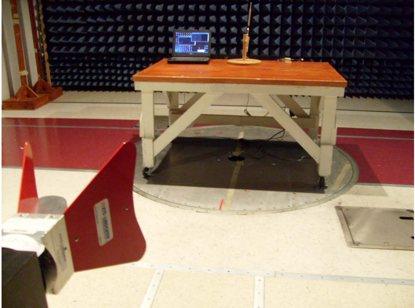
Photograph 3. Radiated Emission, 1-2GHz Test Setup
