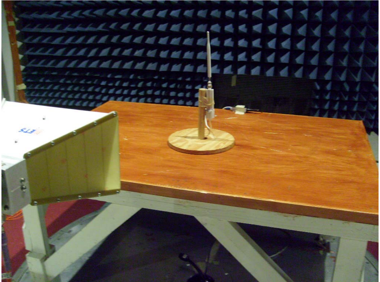
Photograph 7. Restricted Band, Test Setup (6dBi Omni)
