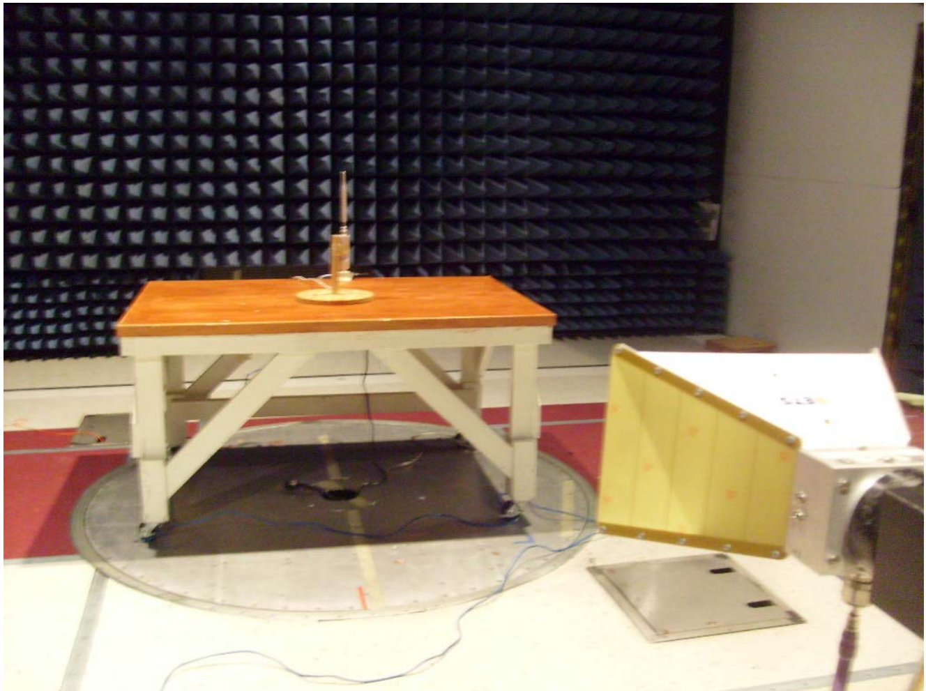
Photograph 5. Radiated Harmonic Emission, Test Setup (6dBi Omni)
