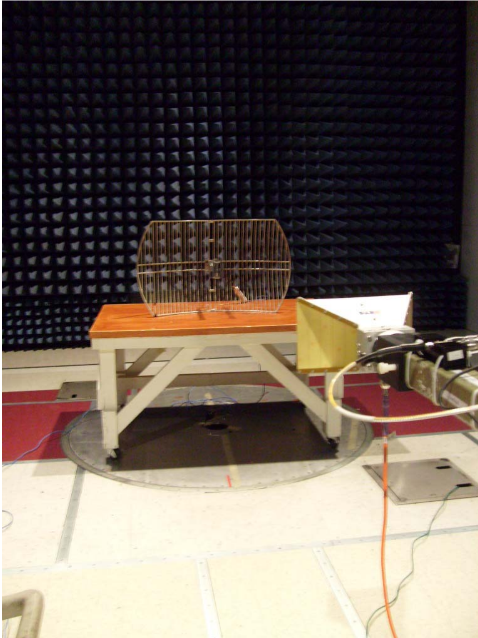
Photograph 6. Radiated Harmonic Emission, Test Setup (24dBi Grid)
