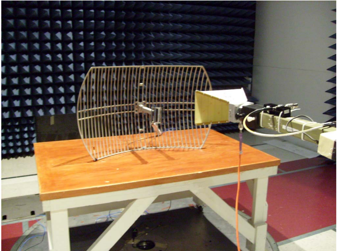
Photograph 8. Restricted Band, Test Setup (24dBi Grid)
