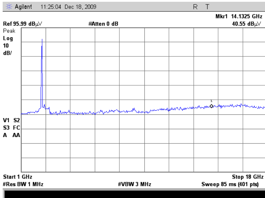
Plot 55. Radiated Spurious Emissions, 802.11g Mode Low Channel (24dBi Grid)
