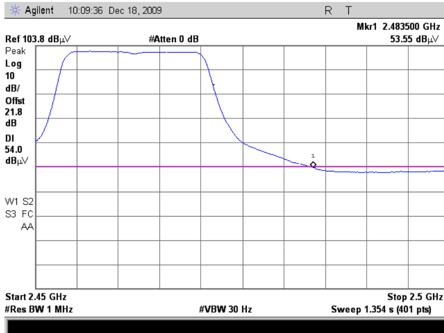
Plot 90. Radiated Restricted Band Edge, 802.11g Mode Channel 11, Average (24dB Grid)
