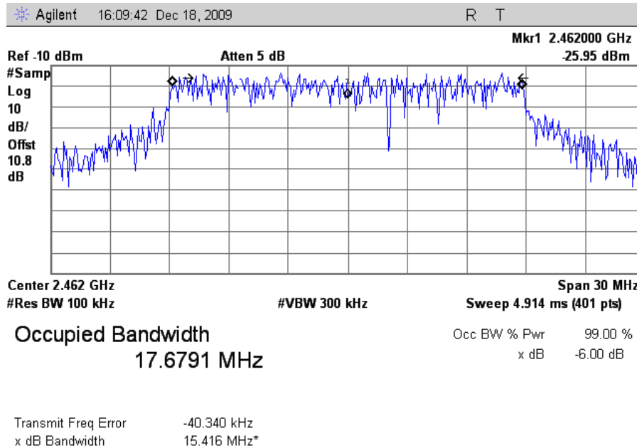
Plot 16. Occupied Band Width, 802.11n 20MHz Mode High Channel, FCC, 6 dB
