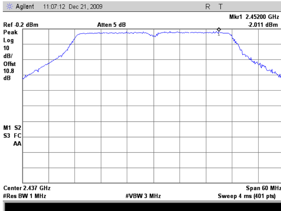
Plot 177. Peak Power Spectral Density, 802.11n 40MHz Mode Mid Channel Peak Determination (24dBi Grid Antenna)
