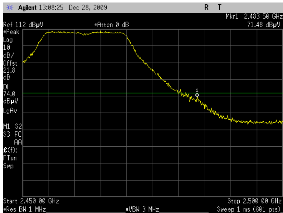
Plot 75. Radiated Restricted Band Edge, 802.11g Mode Channel 11, Peak (6dBi Omni)
