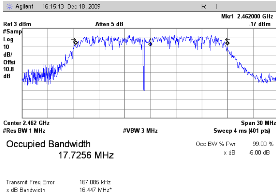
Plot 13. Occupied Band Width, 802.11g Mode High Channel, 99 % OBW
