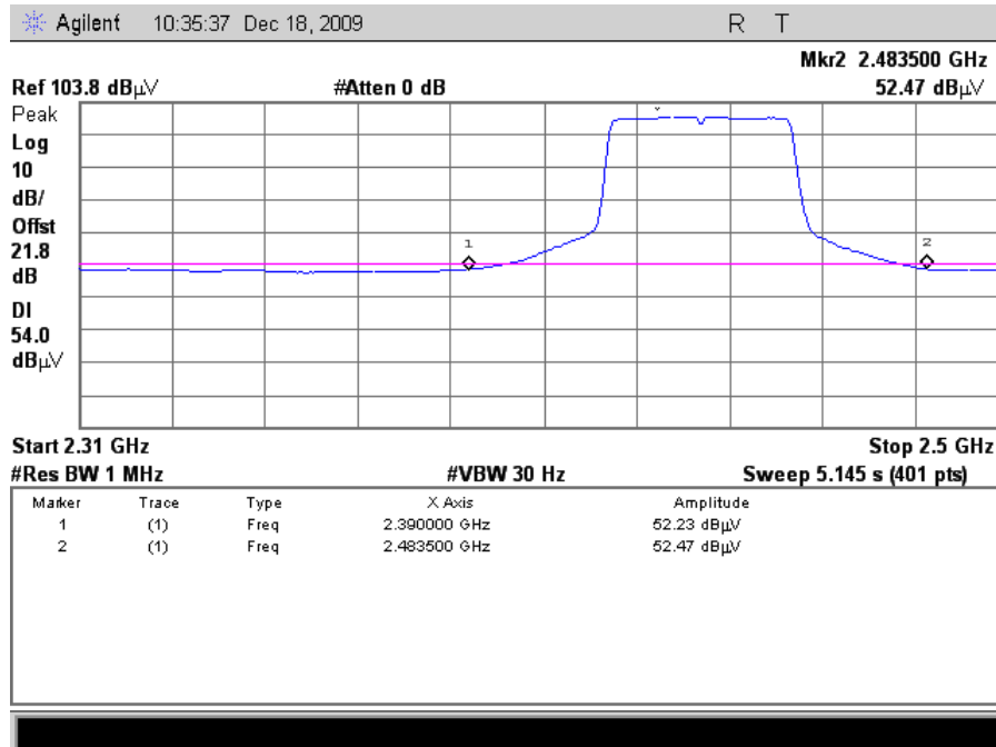
Plot 120. Radiated Restricted Band Edge, 802.11n 40MHz Mode Channel 6, Average (24dB Grid)
