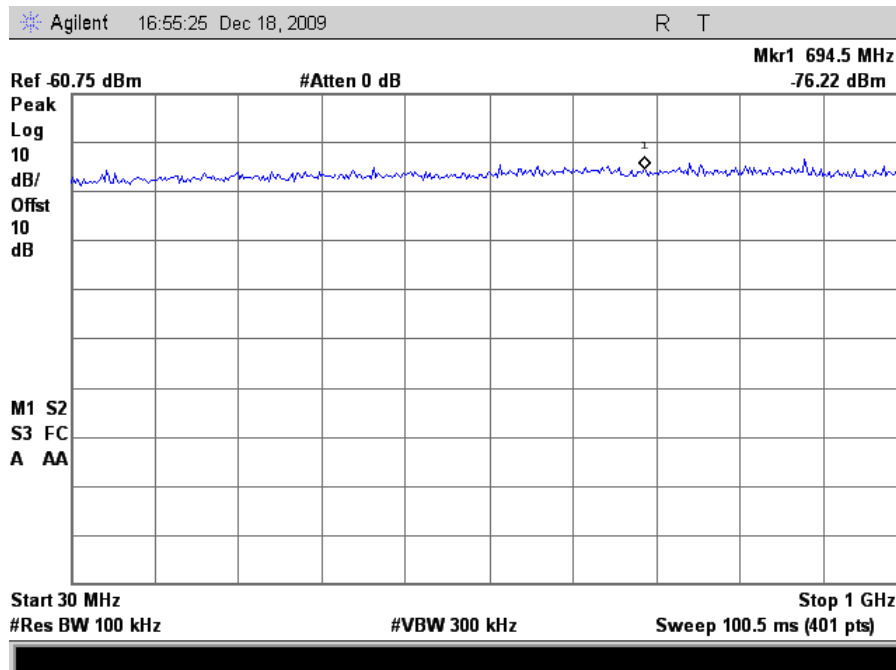
Plot 125. Conducted Emissions, 802.11g Mode Mid Channel, 30 MHz – 1 GHz
