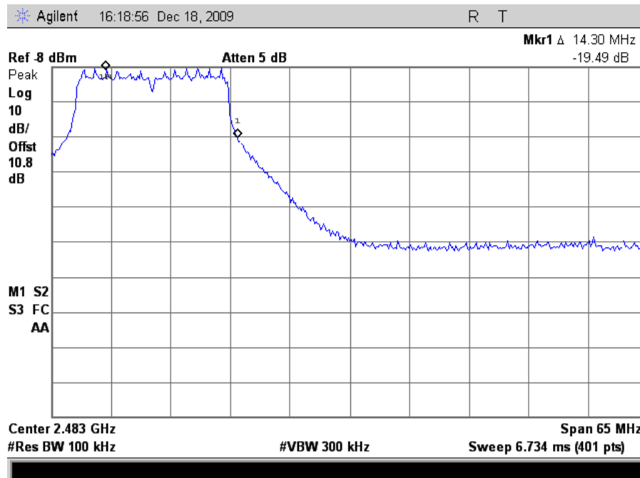
Plot 144. Conducted Band Edge, 802.11g Mode, High
