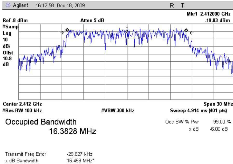
Plot 8. Occupied Band Width, 802.11g Mode Low Channel, FCC, 6 dB
