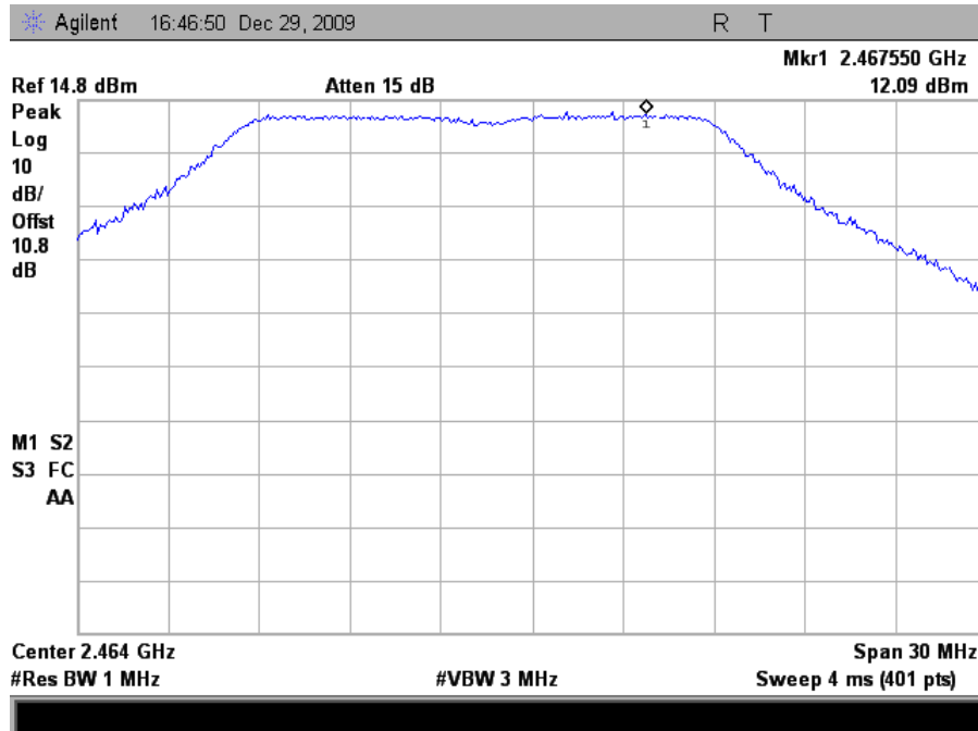
Plot 155. Peak Power Spectral Density, 802.11g Mode High Channel Peak Determination (6dBi Omni Antenna)
