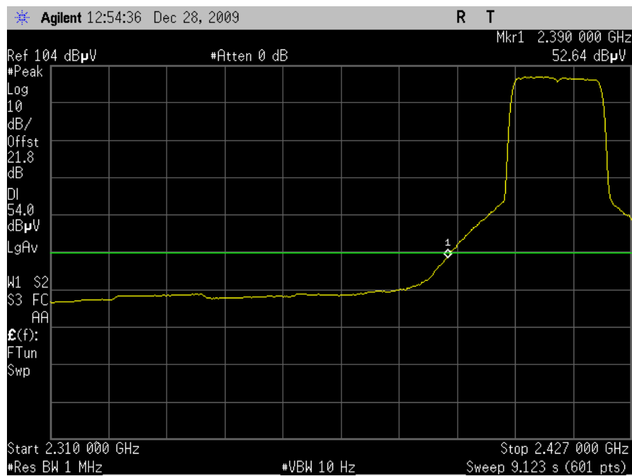
Plot 92. Radiated Restricted Band Edge, 802.11n 20MHz Mode Channel 1, Average (6dBi Omni)
