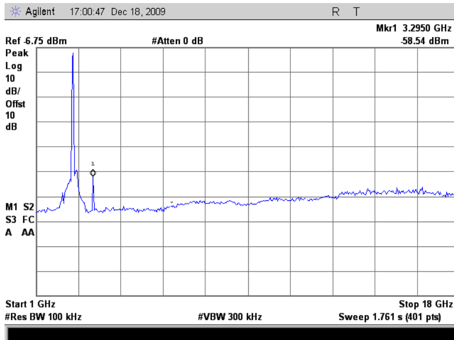
Plot 129. Conducted Emissions, 802.11g Mode High Channel, 1 GHz – 18 GHz
