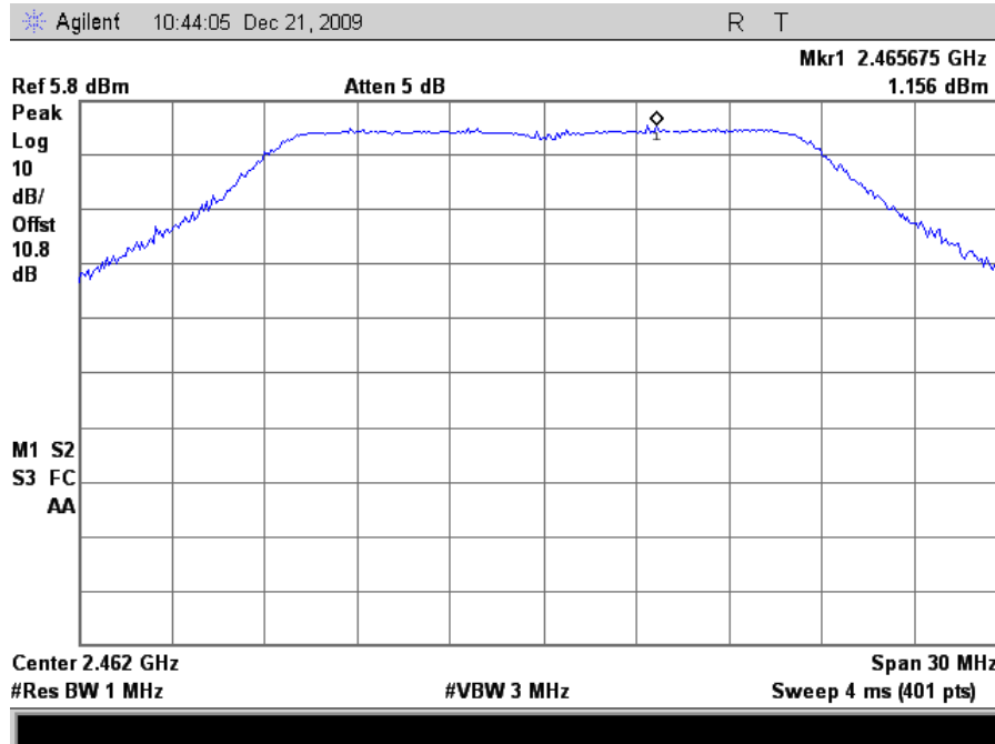
Plot 175. Peak Power Spectral Density, 802.11n 20MHz Mode High Channel Peak Determination (24dBi Grid Antenna)
