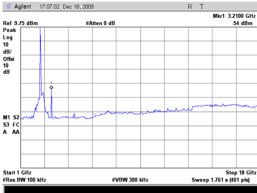
Plot 132. Conducted Emissions, 802.11n 20MHz Mode Low Channel, 1 GHz – 18 GHz
