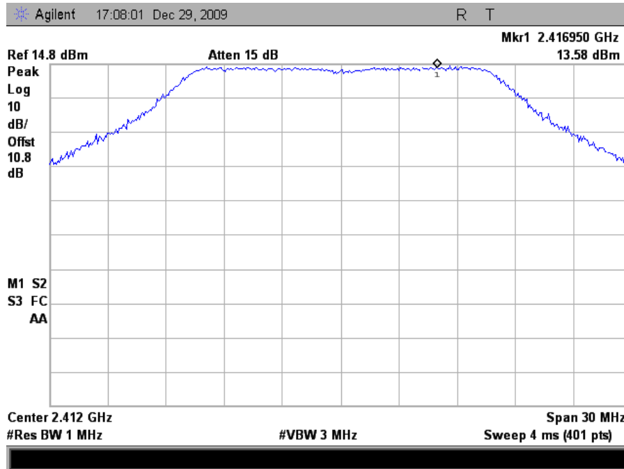
Plot 151. Peak Power Spectral Density, 802.11g Mode Low Channel Peak Determination (6dBi Omni Antenna)
