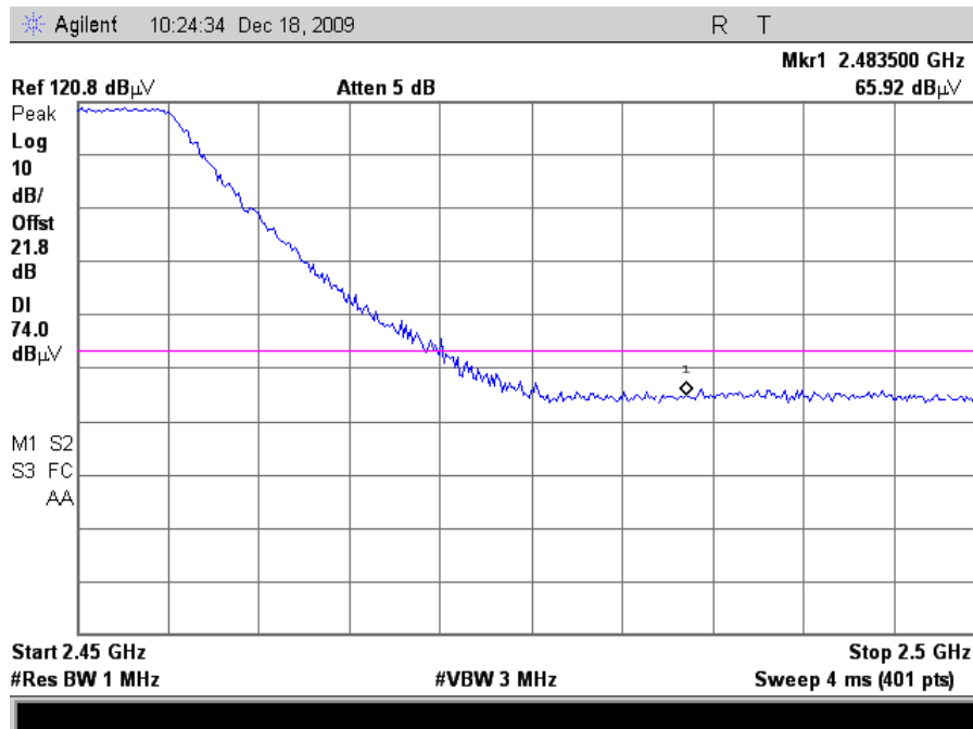
Plot 111. Radiated Restricted Band Edge, 802.11n 20MHz Mode Channel 8, Peak (24dB Grid)
