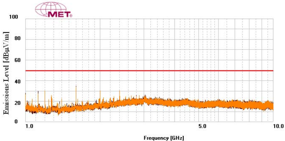
Plot 4. Radiated Emissions, FCC above 1GHZ Limits Plot
