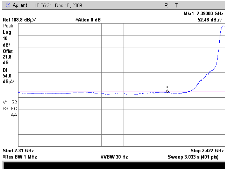
Plot 82. Radiated Restricted Band Edge, 802.11g Mode Channel 4, Average (24dB Grid)
