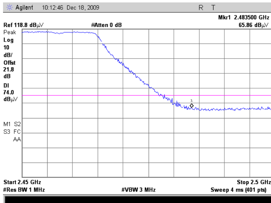
Plot 89. Radiated Restricted Band Edge, 802.11g Mode Channel 10, Peak (24dB Grid)
