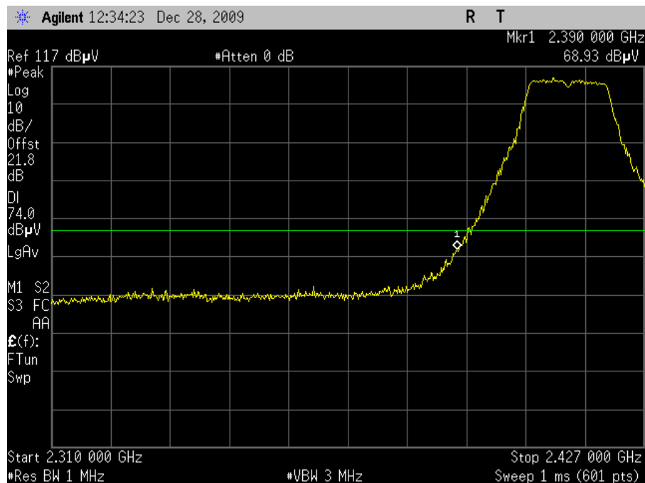
Plot 67. Radiated Restricted Band Edge, 802.11g Mode Channel 1, Peak (6dBi Omni)
