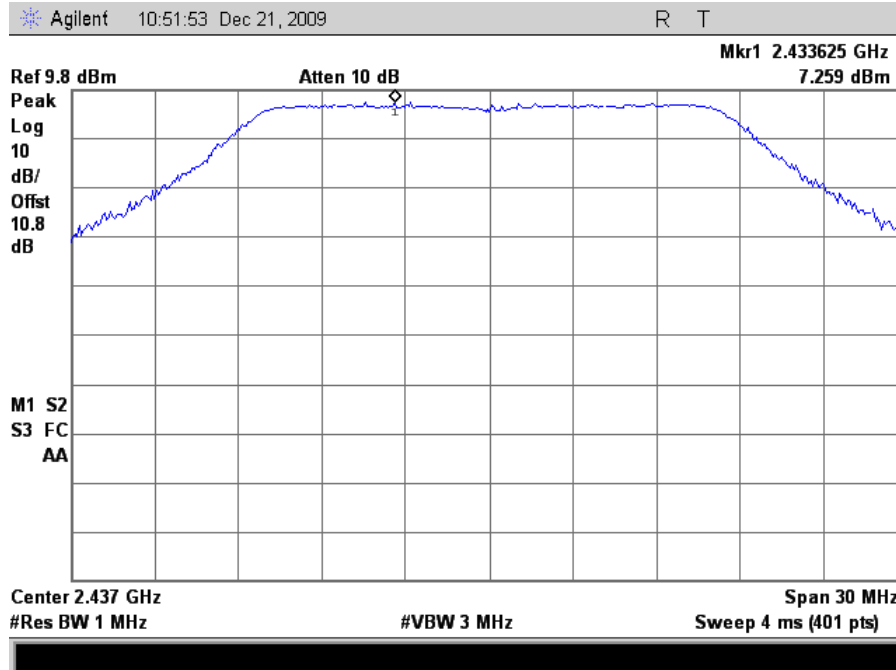
Plot 173. Peak Power Spectral Density, 802.11n 20MHz Mode Mid Channel Peak Determination (24dBi Grid Antenna)
