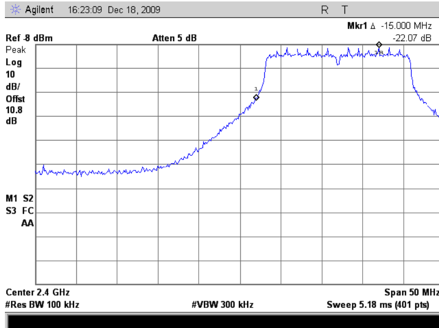
Plot 145. Conducted Band Edge, 802.11n 20MHz Mode, Low
