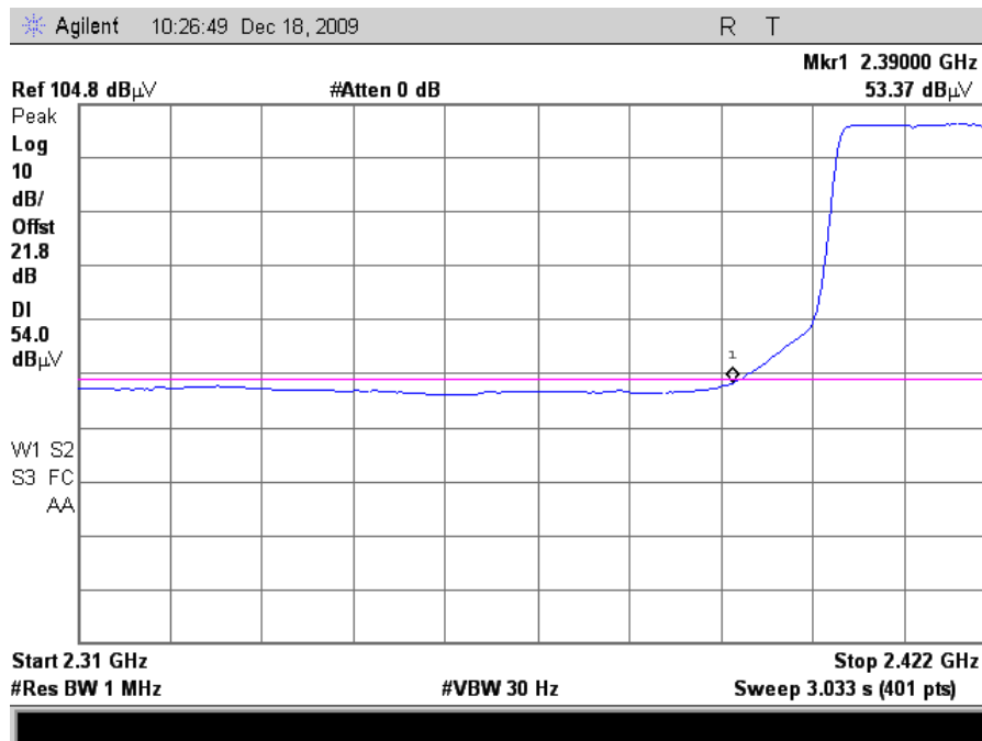
Plot 102. Radiated Restricted Band Edge, 802.11n 20MHz Mode Channel 1, Average (24dB Grid)
