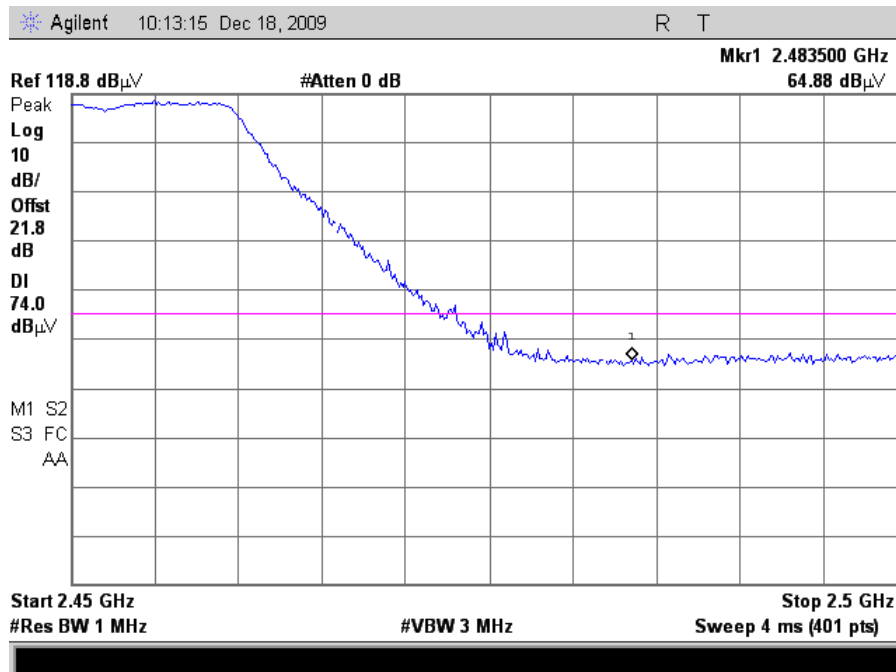
Plot 87. Radiated Restricted Band Edge, 802.11g Mode Channel 9, Peak (24dB Grid)
