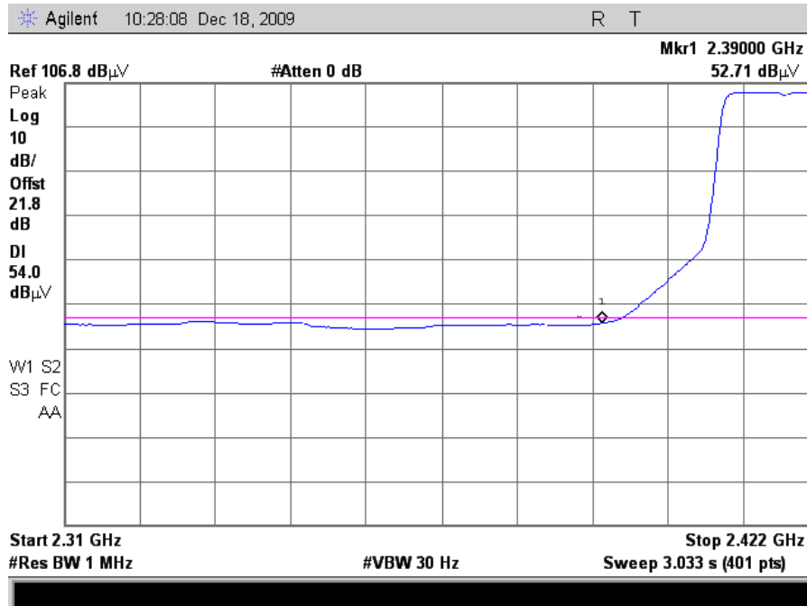
Plot 104. Radiated Restricted Band Edge, 802.11n 20MHz Mode Channel 2, Average (24dB Grid)
