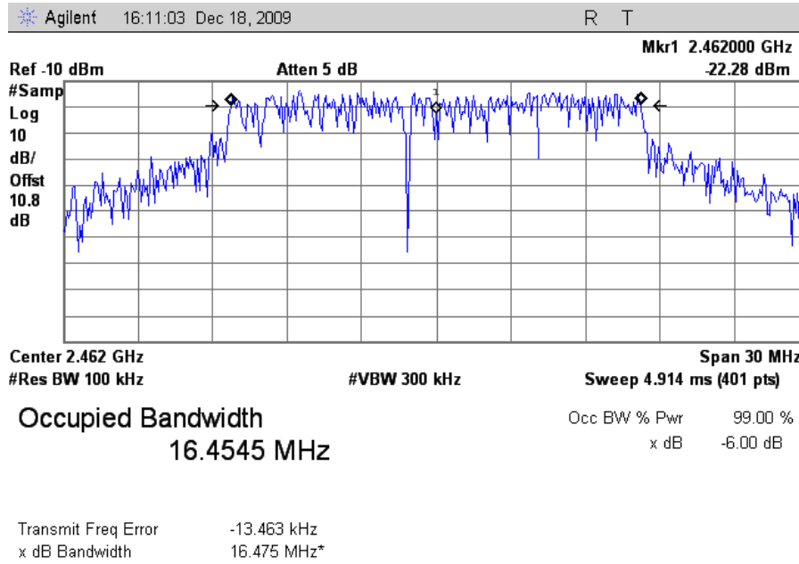
Plot 10. Occupied Band Width, 802.11g Mode High Channel, FCC, 6 dB
