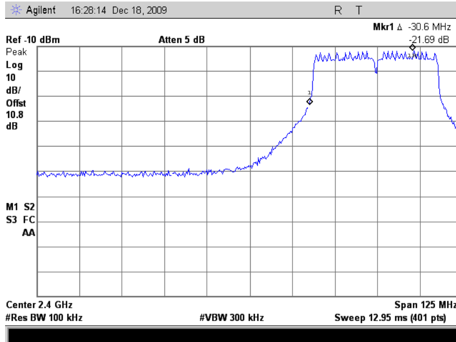
Plot 147. Conducted Band Edge, 802.11n 40MHz Mode, Low
