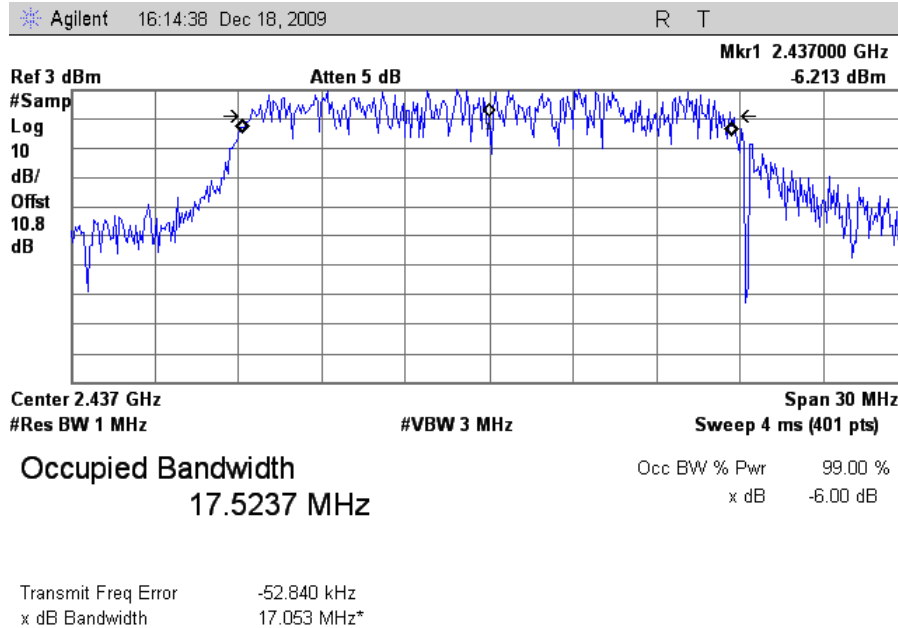
Plot 12. Occupied Band Width, 802.11g Mode Mid Channel, 99% OBW
