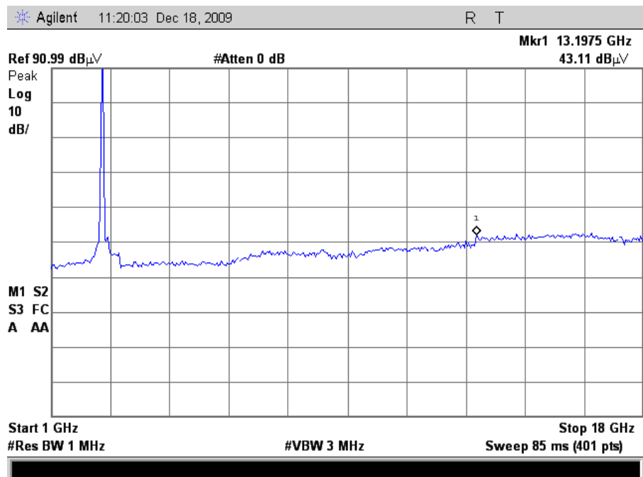
Plot 65. Radiated Spurious Emissions, 802.11n 40MHz Mode Mid Channel (24dBi Grid)
