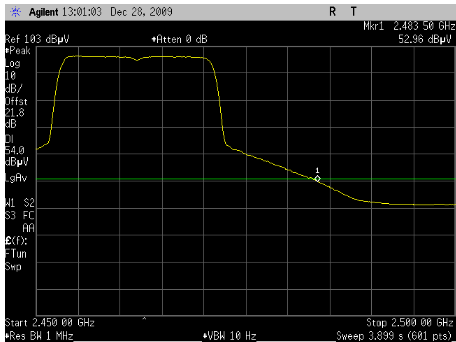
Plot 100. Radiated Restricted Band Edge, 802.11n 20MHz Mode Channel 11, Average (6dBi Omni)
