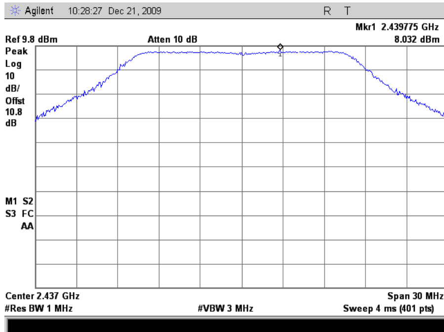
Plot 167. Peak Power Spectral Density, 802.11g Mode Mid Channel Peak Determination (24dBi Grid Antenna)
