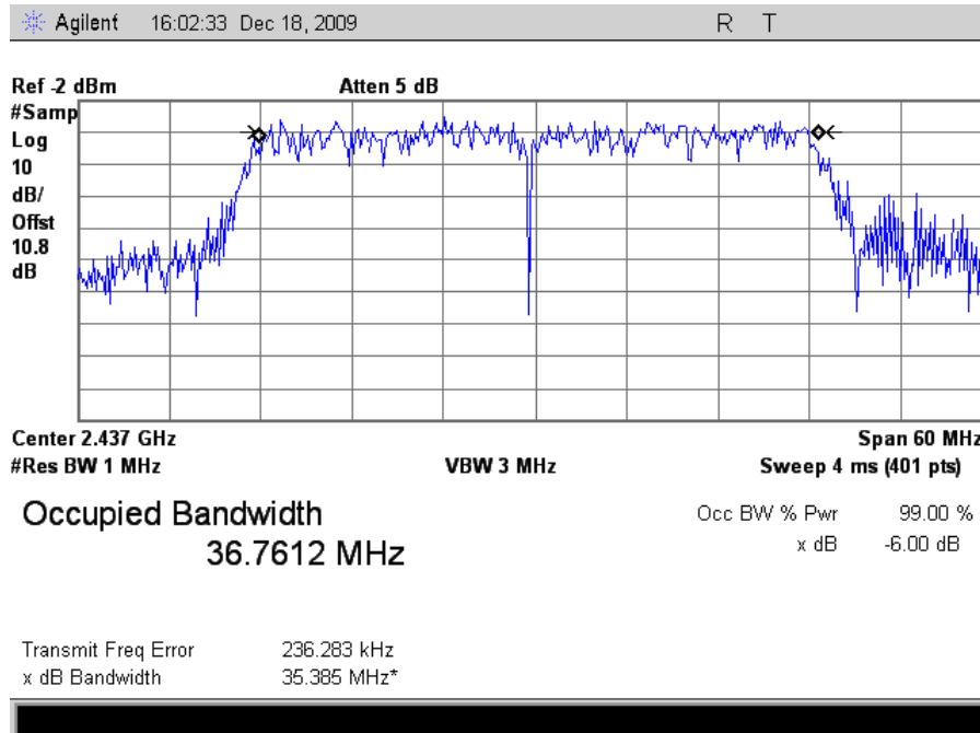
Plot 21. Occupied Band Width, 802.11n 40MHz Mode Mid Channel, 99 % OBW
