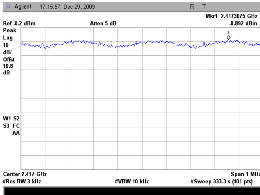
Plot 152. Peak Power Spectral Density, 802.11g Mode Low Channel (6dBi Omni Antenna)
