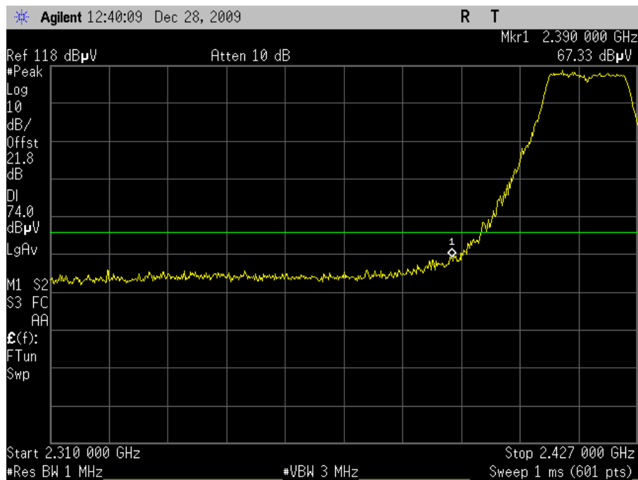
Plot 69. Radiated Restricted Band Edge, 802.11g Mode Channel 2, Peak (6dBi Omni)
