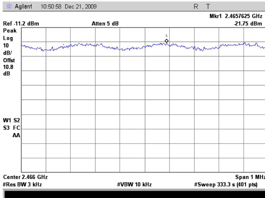
Plot 176. Peak Power Spectral Density, 802.11n 20MHz Mode High Channel (24dBi Grid Antenna)
