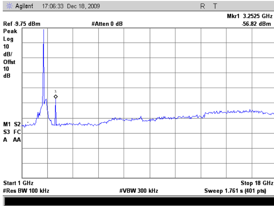
Plot 135. Conducted Emissions, 802.11n 20MHz Mode Mid Channel, 1 GHz – 18 GHz
