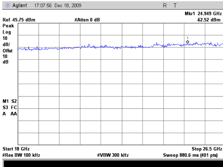
Plot 133. Conducted Emissions, 802.11n 20MHz Mode Low Channel, 18 GHz – 26.5 GHz
