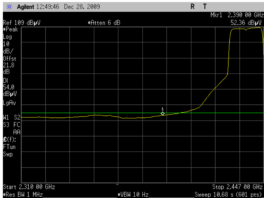
Plot 96. Radiated Restricted Band Edge, 802.11n 20MHz Mode Channel 6, Average (6dBi Omni)
