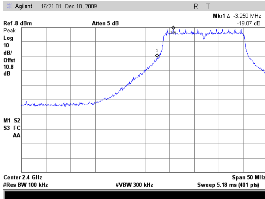
Plot 143. Conducted Band Edge, 802.11g Mode, Low
