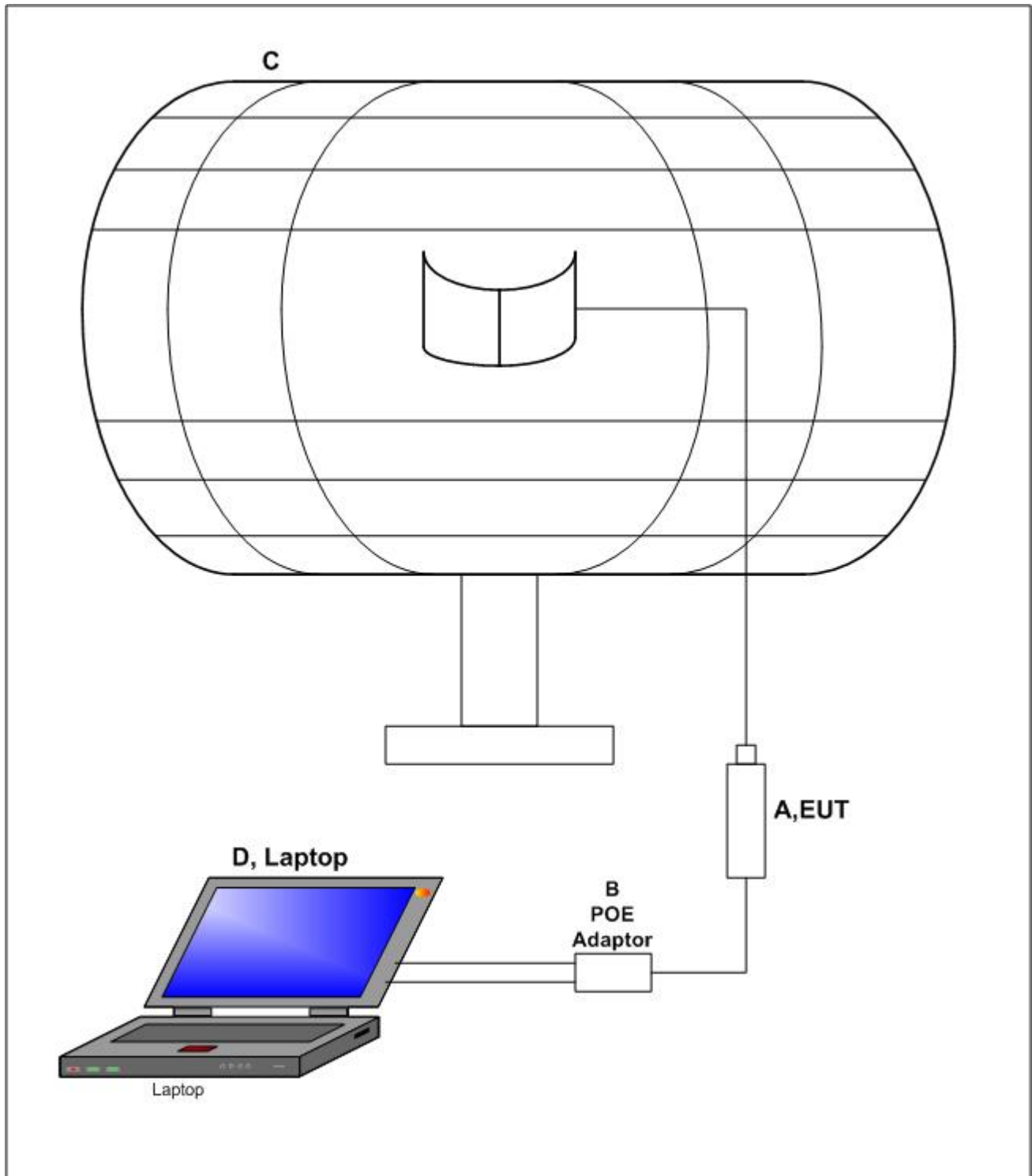
Figure 1. Block Diagram of Test Configuration, Dish Antenna
