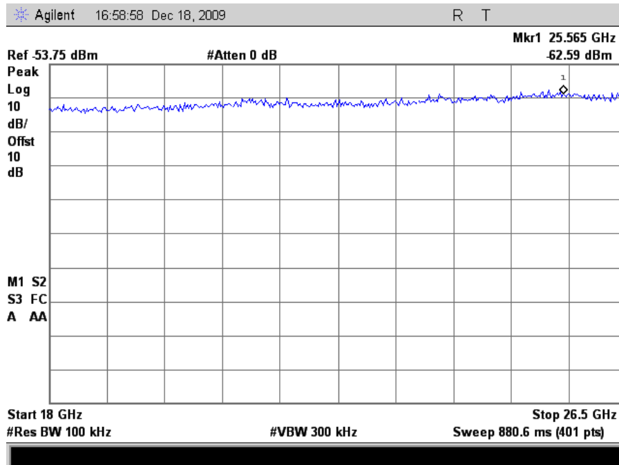
Plot 124. Conducted Emissions, 802.11g Mode Low Channel, 18 GHz – 26.5 GHz
