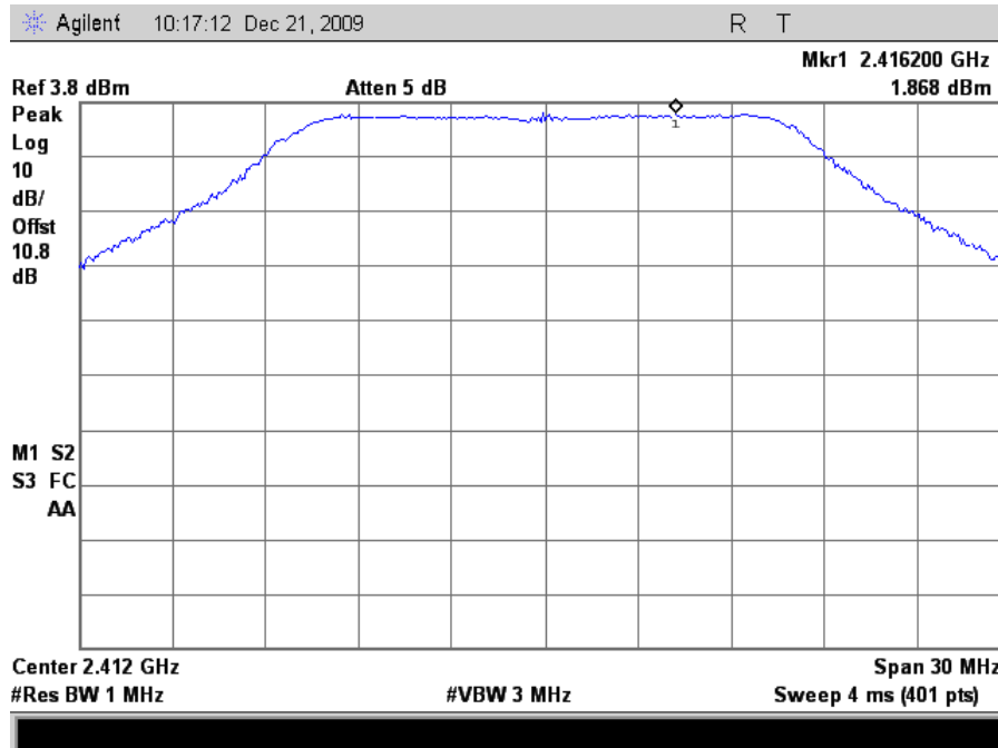
Plot 165. Peak Power Spectral Density, 802.11g Mode Low Channel Peak Determination (24dBi Grid Antenna)
