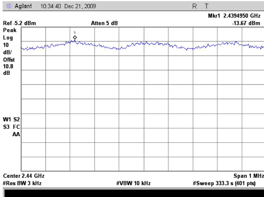
Plot 168. Peak Power Spectral Density, 802.11g Mode Mid Channel (24dBi Grid Antenna)
