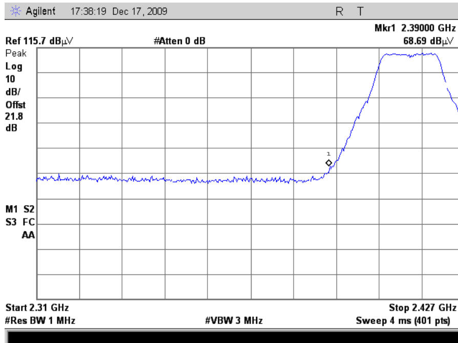
Plot 77. Radiated Restricted Band Edge, 802.11g Mode Channel 1, Peak (24dB Grid)
