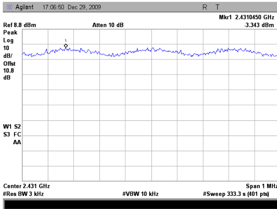
Plot 154. Peak Power Spectral Density, 802.11g Mode Mid Channel (6dBi Omni Antenna)
