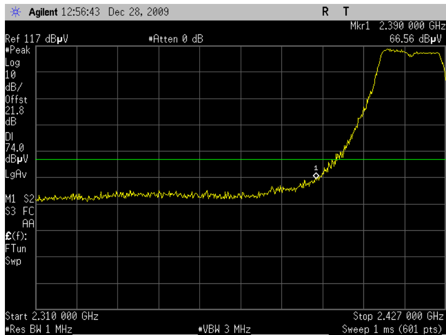
Plot 95. Radiated Restricted Band Edge, 802.11n 20MHz Mode Channel 2, Peak (6dBi Omni)
