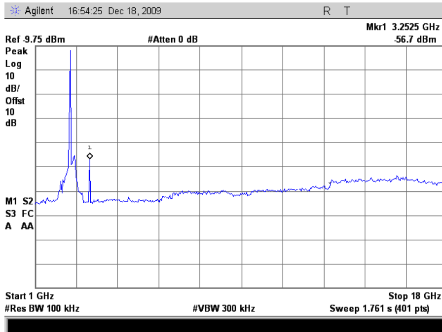
Plot 126. Conducted Emissions, 802.11g Mode Mid Channel, 1 GHz – 18 GHz
