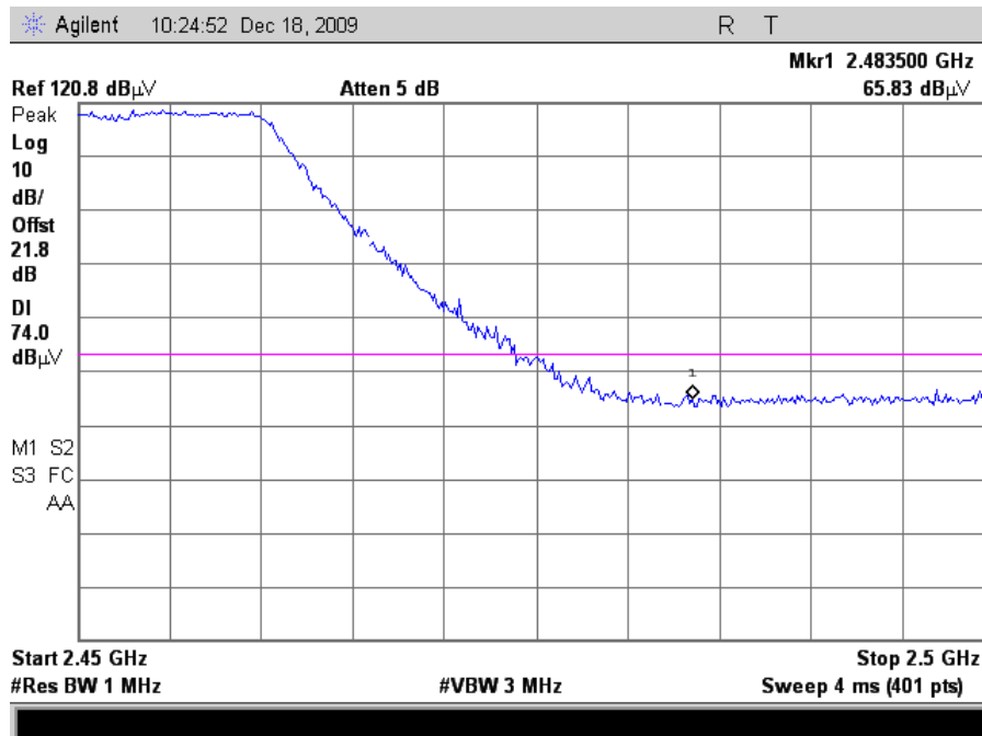
Plot 113. Radiated Restricted Band Edge, 802.11n 20MHz Mode Channel 9, Peak (24dB Grid)
