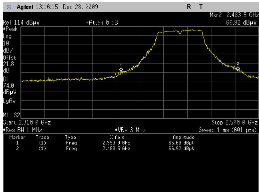
Plot 119. Radiated Restricted Band Edge, 802.11n 40MHz Mode Channel 6, Peak (6dBi Omni)
