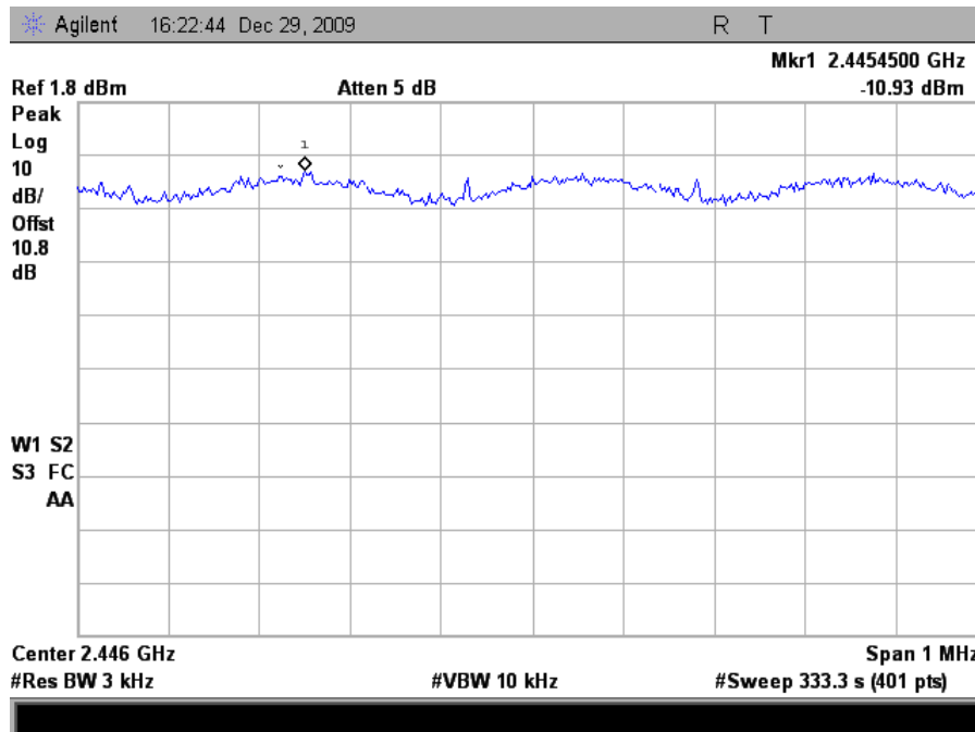
Plot 164. Peak Power Spectral Density, 802.11n 40MHz Mode Mid Channel (6dBi Omni Antenna)
