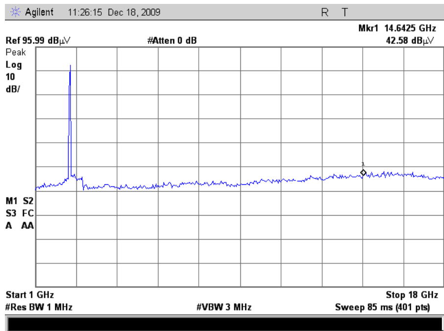
Plot 61. Radiated Spurious Emissions, 802.11n 20MHz Mode Low Channel (24dBi Grid)
