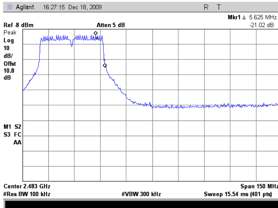
Plot 148. Conducted Band Edge, 802.11n 40MHz Mode, High
