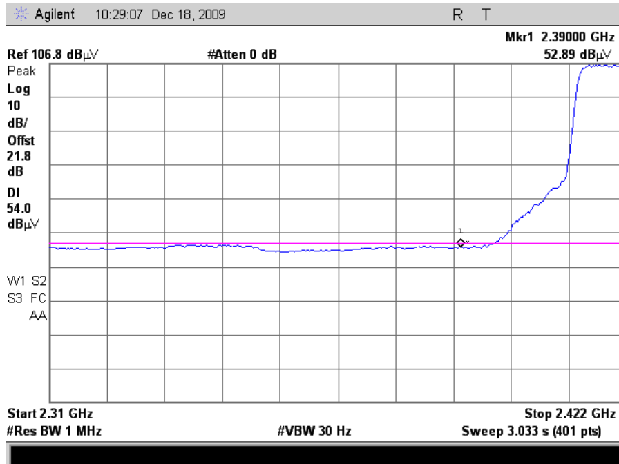
Plot 106. Radiated Restricted Band Edge, 802.11n 20MHz Mode Channel 3, Average (24dB Grid)
