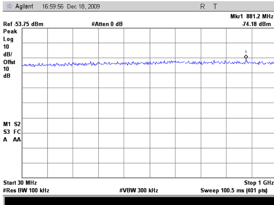
Plot 128. Conducted Emissions, 802.11g Mode High Channel, 30 MHz – 1 GHz
