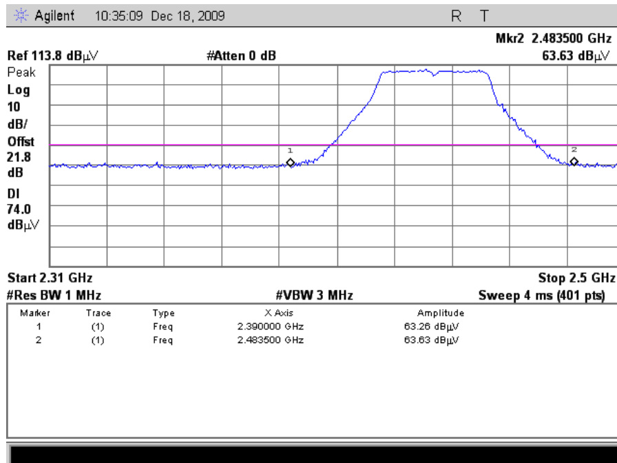
Plot 121. Radiated Restricted Band Edge, 802.11n 40MHz Mode Channel 6, Peak (24dB Grid)
