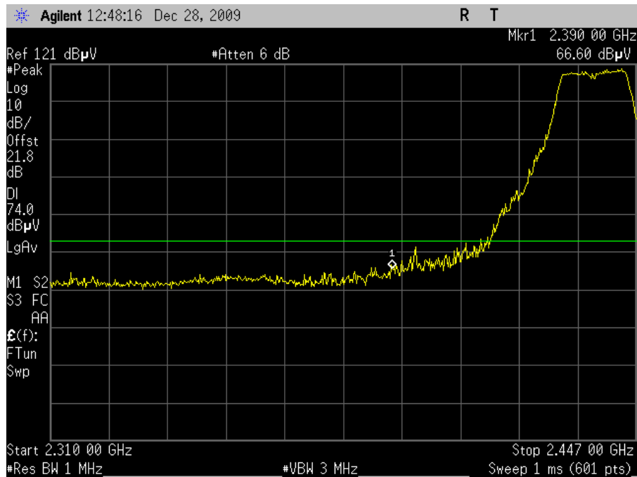
Plot 71. Radiated Restricted Band Edge, 802.11g Mode Channel 6, Peak (6dBi Omni)
