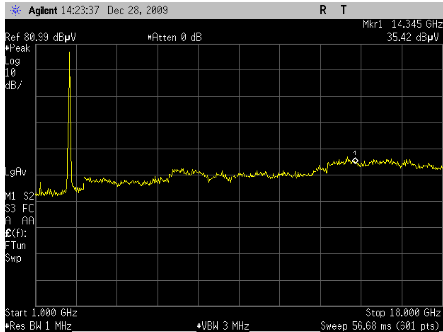
Plot 58. Radiated Spurious Emissions, 802.11n 20MHz Mode Low Channel (6dBi Omni)
