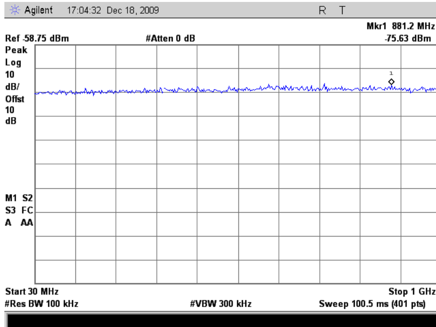
Plot 137. Conducted Emissions, 802.11n 20MHz Mode High Channel, 30 MHz – 1 GHz
