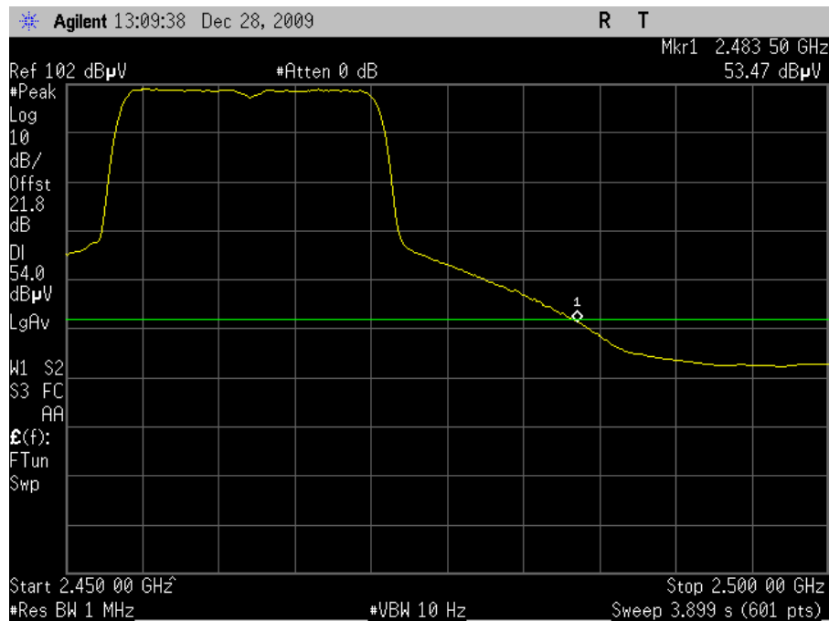
Plot 74. Radiated Restricted Band Edge, 802.11g Mode Channel 11, Average (6dBi Omni)
