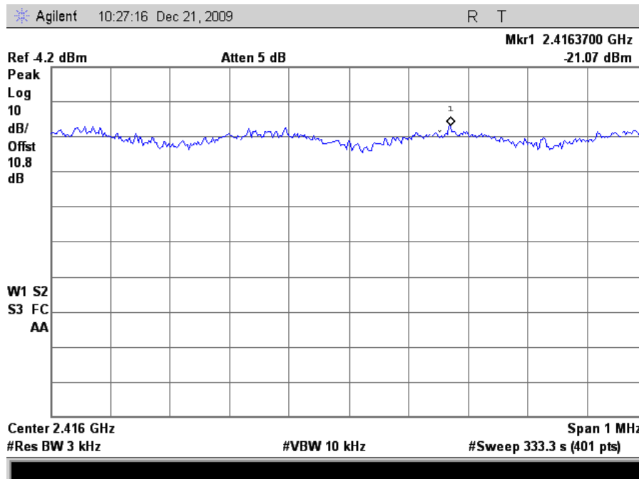
Plot 166. Peak Power Spectral Density, 802.11g Mode Low Channel (24dBi Grid Antenna)
