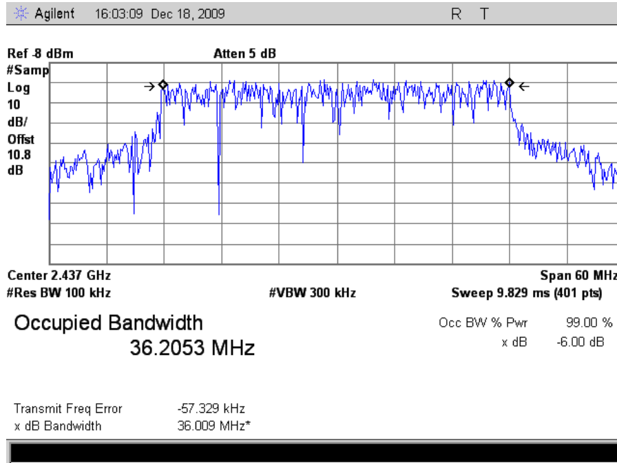
Plot 20. Occupied Band Width, 802.11n 40MHz Mode Mid Channel, FCC, 6 dB
