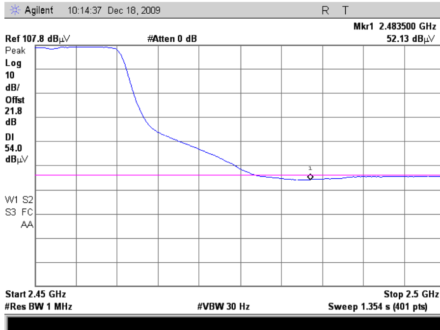
Plot 86. Radiated Restricted Band Edge, 802.11g Mode Channel 9, Average (24dB Grid)
