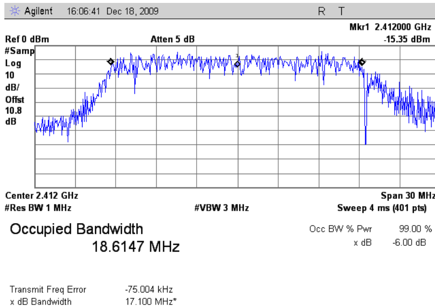
Plot 17. Occupied Band Width, 802.11n 20MHz Mode Low Channel, 99 % OBW
