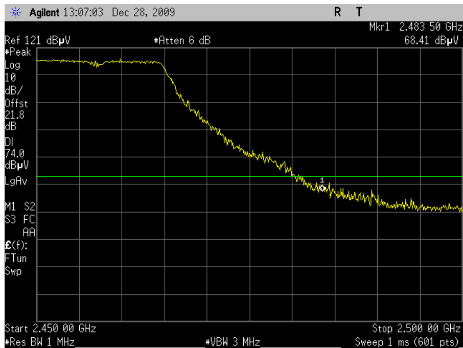
Plot 73. Radiated Restricted Band Edge, 802.11g Mode Channel 10, Peak (6dBi Omni)
