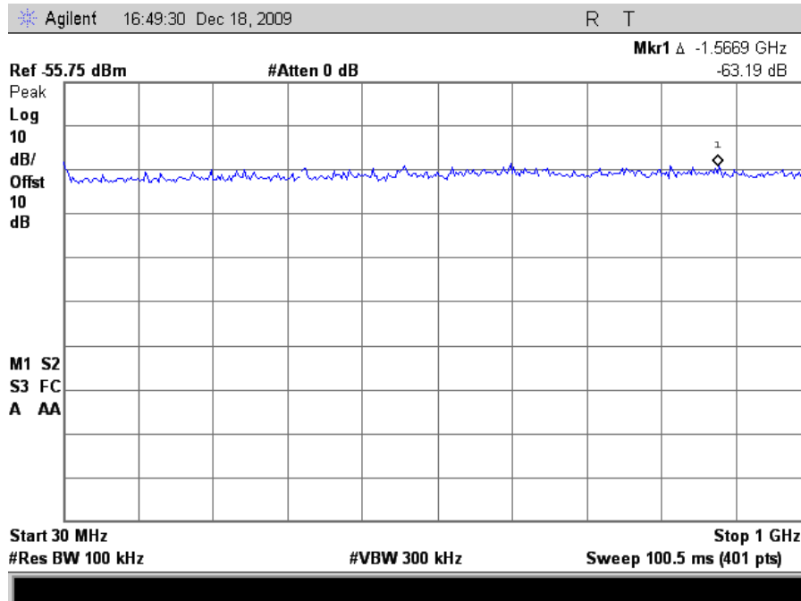
Plot 140. Conducted Emissions, 802.11n 40MHz Mode Mid Channel, 30 MHz – 1 GHz
