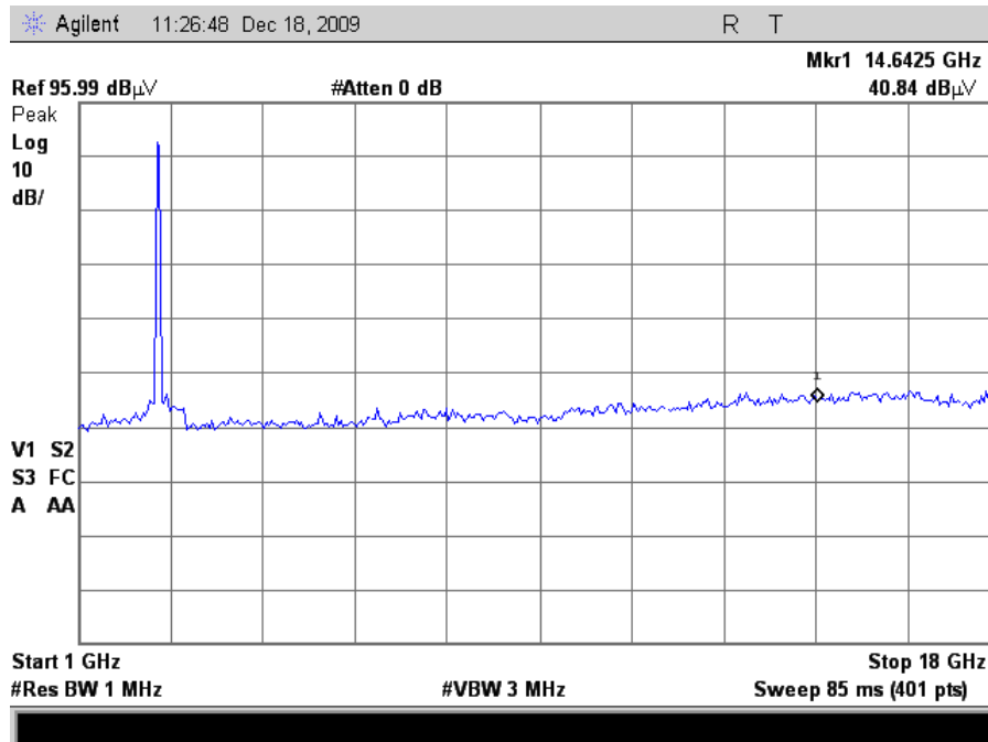
Plot 62. Radiated Spurious Emissions, 802.11n 20MHz Mode Mid Channel (24dB \mu Grid)
