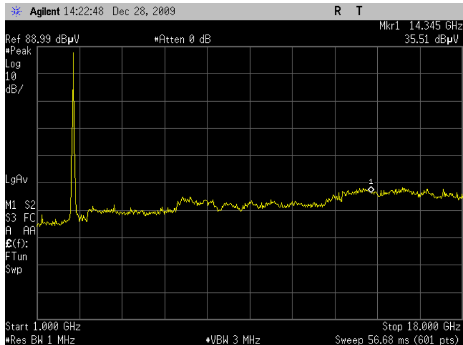
Plot 59. Radiated Spurious Emissions, 802.11n 20MHz Mode Mid Channel (6dBi Omni)
