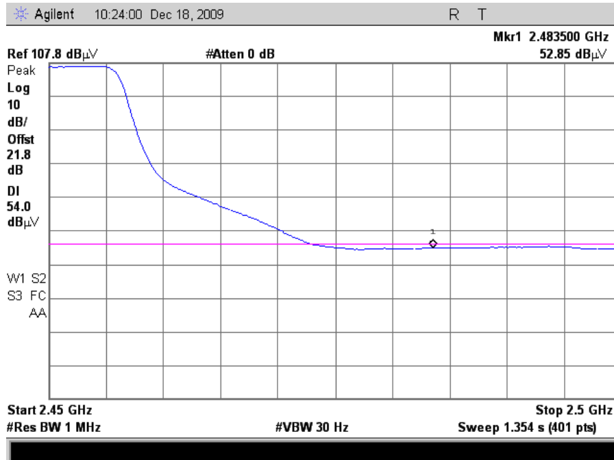
Plot 110. Radiated Restricted Band Edge, 802.11n 20MHz Mode Channel 8, Average (24dB Grid)
