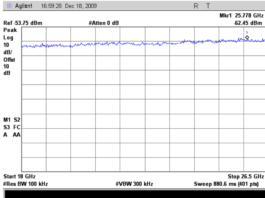
Plot 130. Conducted Emissions, 802.11g Mode High Channel, 18 GHz – 26.5 GHz
