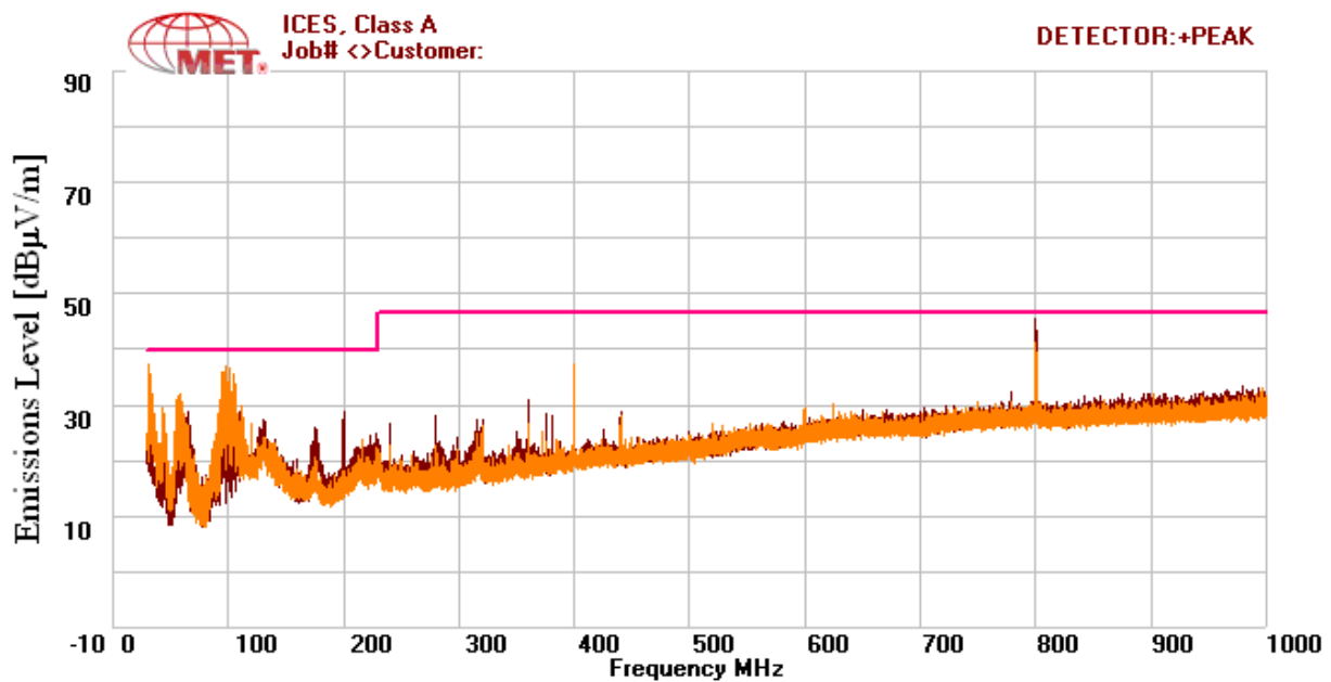
Plot 5. Radiated Emissions, ICES-003 Limits Plot
