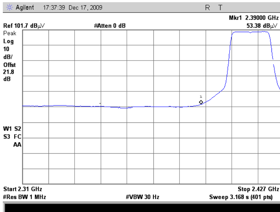
Plot 76. Radiated Restricted Band Edge, 802.11g Mode Channel 1, Average (24dB Grid)
