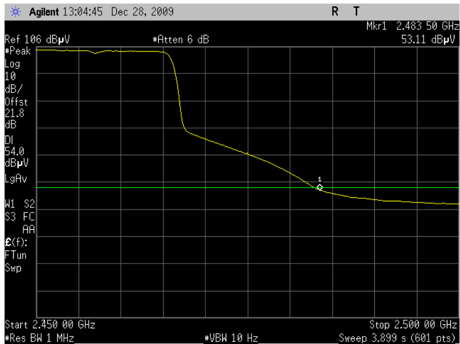
Plot 98. Radiated Restricted Band Edge, 802.11n 20MHz Mode Channel 10, Average (6dBi Omni)
