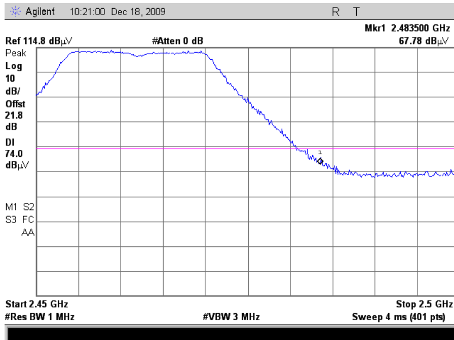
Plot 117. Radiated Restricted Band Edge, 802.11n 20MHz Mode Channel 11, Peak (24dB Grid)
