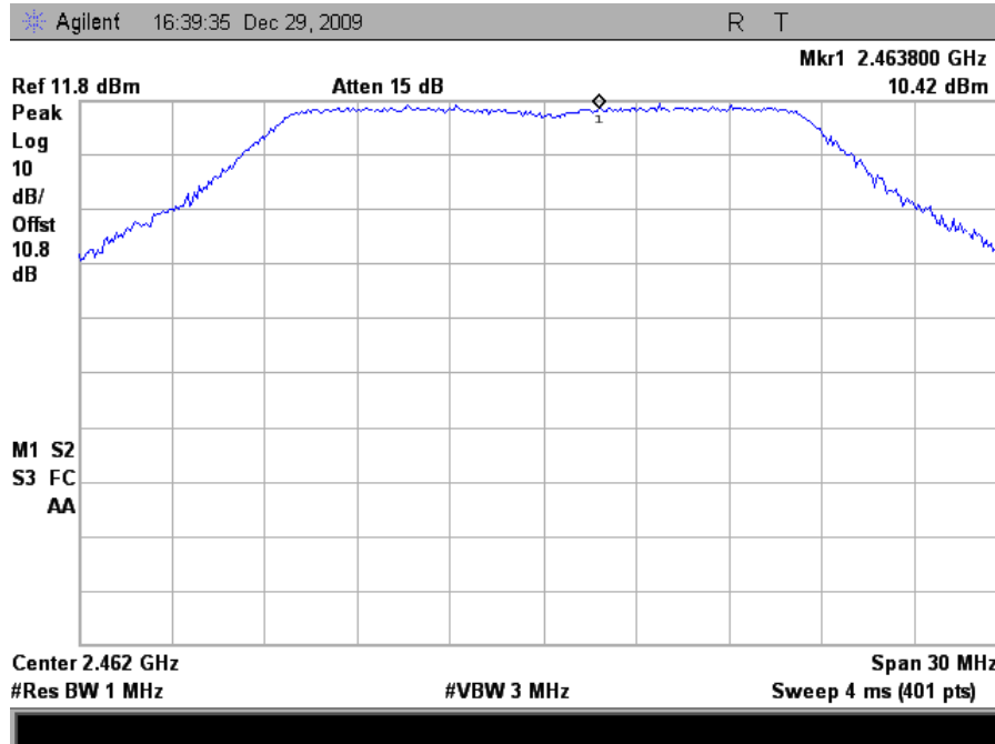
Plot 161. Peak Power Spectral Density, 802.11n 20MHz Mode High Channel Peak Determination (6dBi Omni Antenna)
