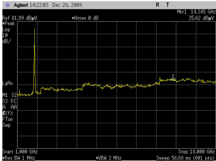
Plot 60. Radiated Spurious Emissions, 802.11n 20MHz Mode High Channel (6dBi Omni)
