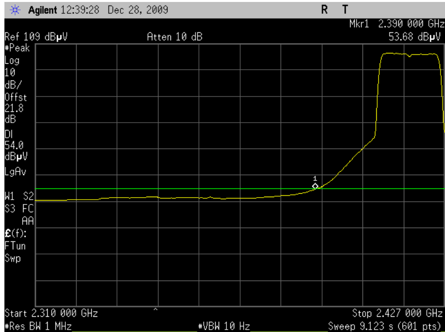
Plot 68. Radiated Restricted Band Edge, 802.11g Mode Channel 2, Average (6dBi Omni)
