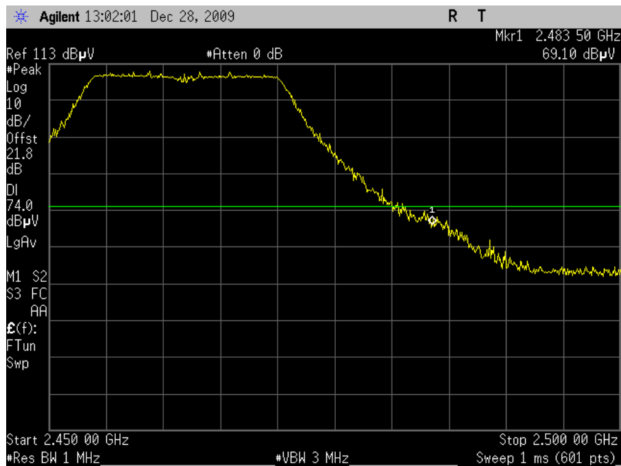
Plot 101. Radiated Restricted Band Edge, 802.11n 20MHz Mode Channel 11, Peak (6dBi Omni)
