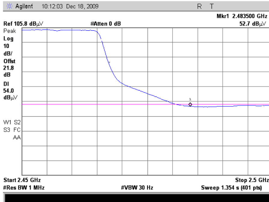
Plot 88. Radiated Restricted Band Edge, 802.11g Mode Channel 10, Average (24dB Grid)
