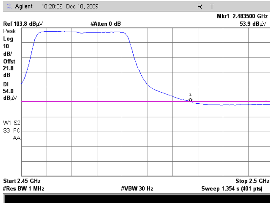
Plot 116. Radiated Restricted Band Edge, 802.11n 20MHz Mode Channel 11, Average (24dB Grid)
