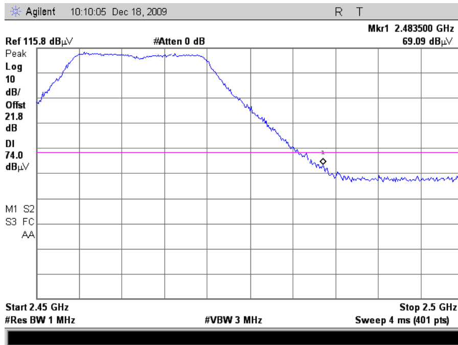
Plot 91. Radiated Restricted Band Edge, 802.11g Mode Channel 11, Peak (24dB Grid)
