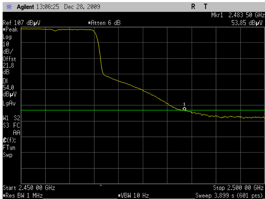
Plot 72. Radiated Restricted Band Edge, 802.11g Mode Channel 10, Average (6dBi Omni)
