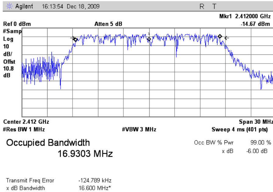
Plot 11. Occupied Band Width, 802.11g Mode Low Channel, 99 % OBW
