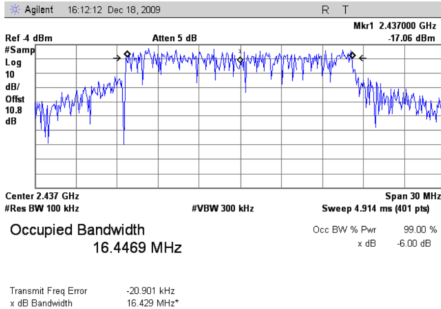
Plot 9. Occupied Band Width, 802.11g Mode Mid Channel, FCC, 6 dB
