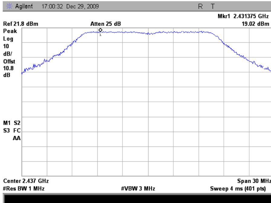
Plot 153. Peak Power Spectral Density, 802.11g Mode Mid Channel Peak Determination (6dBi Omni Antenna)
