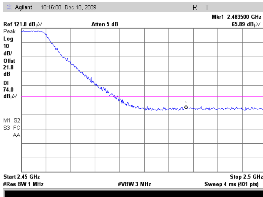
Plot 85. Radiated Restricted Band Edge, 802.11g Mode Channel 8, Peak (24dBi Grid)
