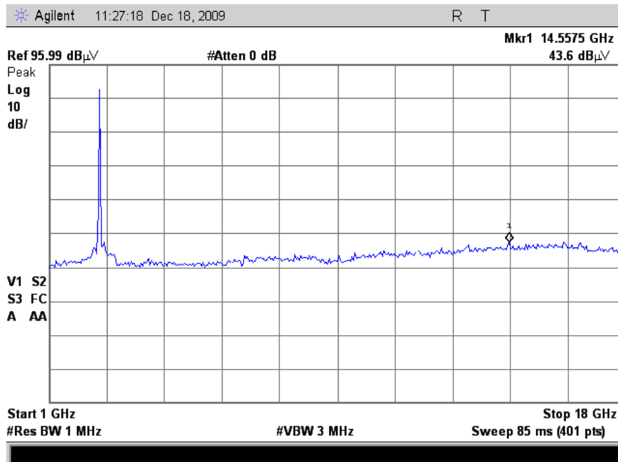
Plot 63. Radiated Spurious Emissions, 802.11n 20MHz Mode High Channel (24dB \mu Grid)
