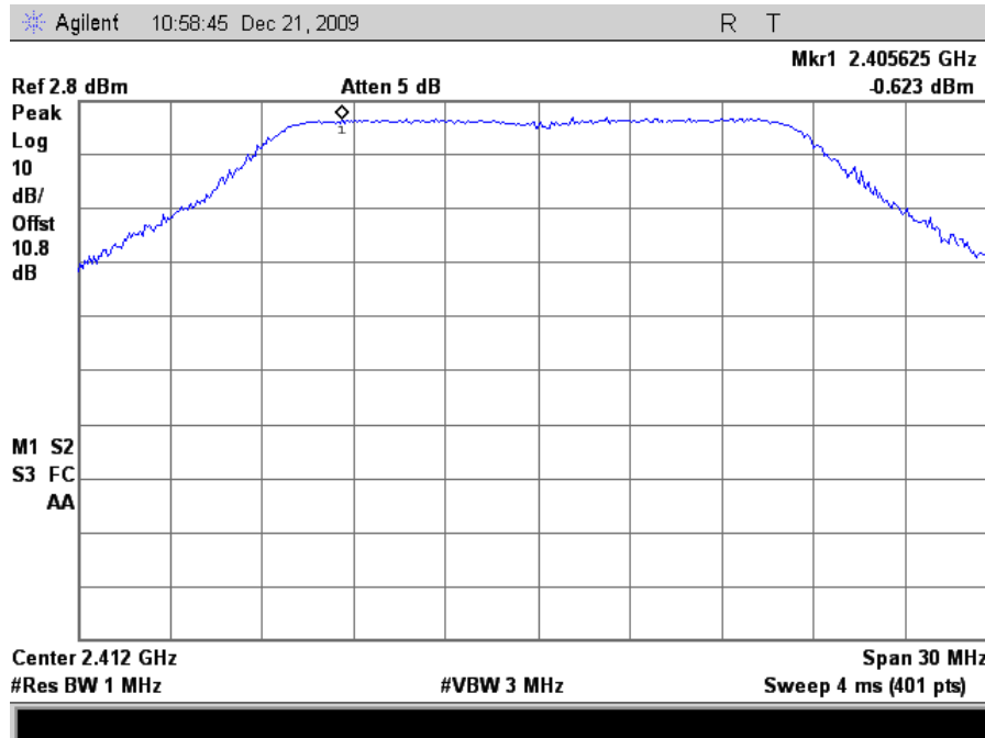
Plot 171. Peak Power Spectral Density, 802.11n 20MHz Mode Low Channel Peak Determination (24dBi Grid Antenna)
