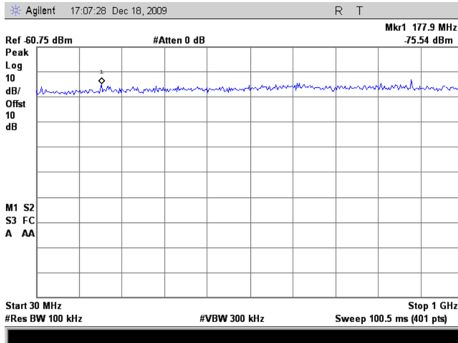
Plot 131. Conducted Emissions, 802.11n 20MHz Mode Low Channel, 30 MHz – 1 GHz
