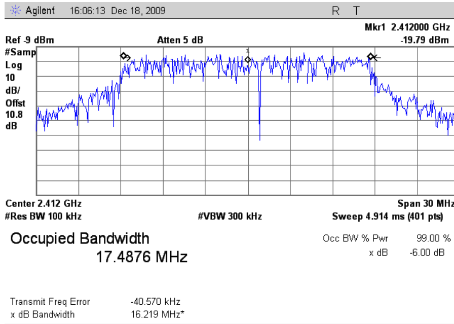
Plot 14. Occupied Band Width, 802.11n 20MHz Mode Low Channel, FCC, 6 dB
