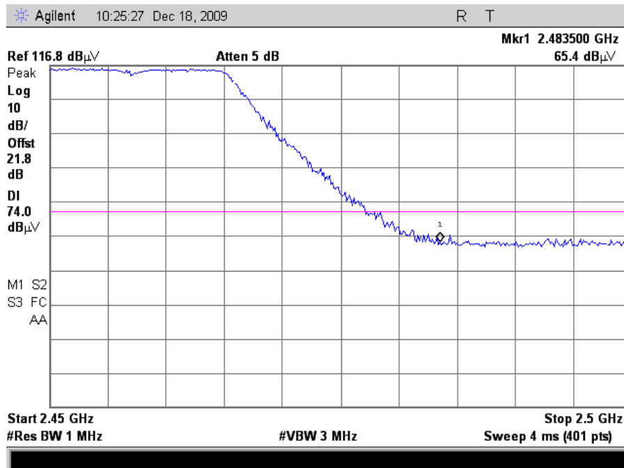
Plot 115. Radiated Restricted Band Edge, 802.11n 20MHz Mode Channel 10, Peak (24dB Grid)
