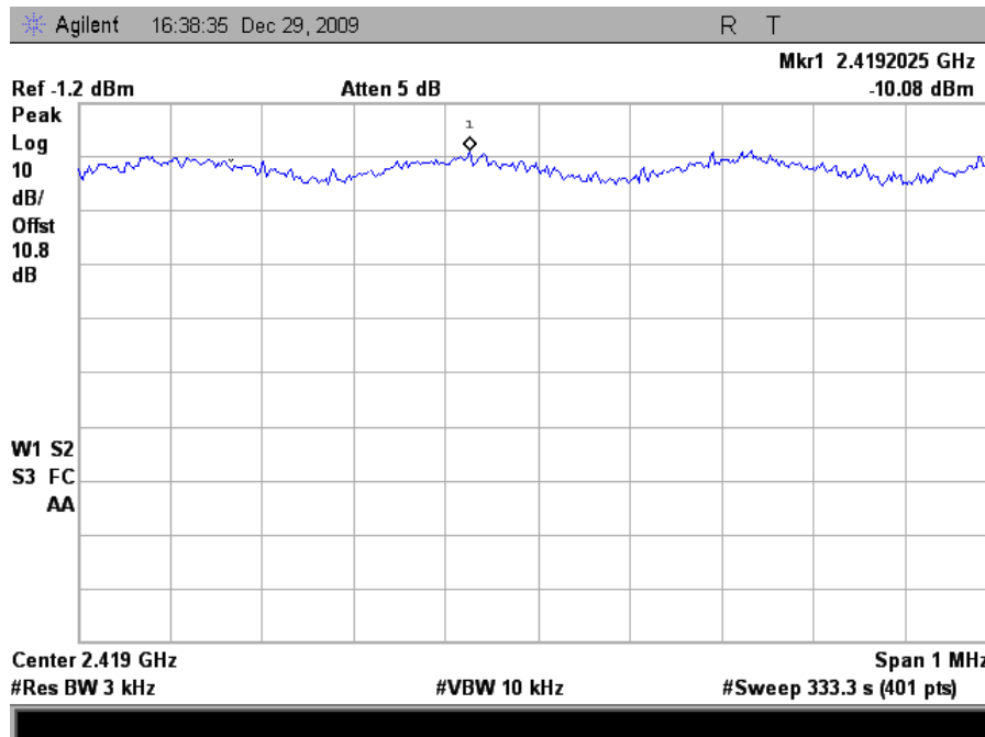
Plot 158. Peak Power Spectral Density, 802.11n 20MHz Mode Low Channel (6dBi Omni Antenna)
