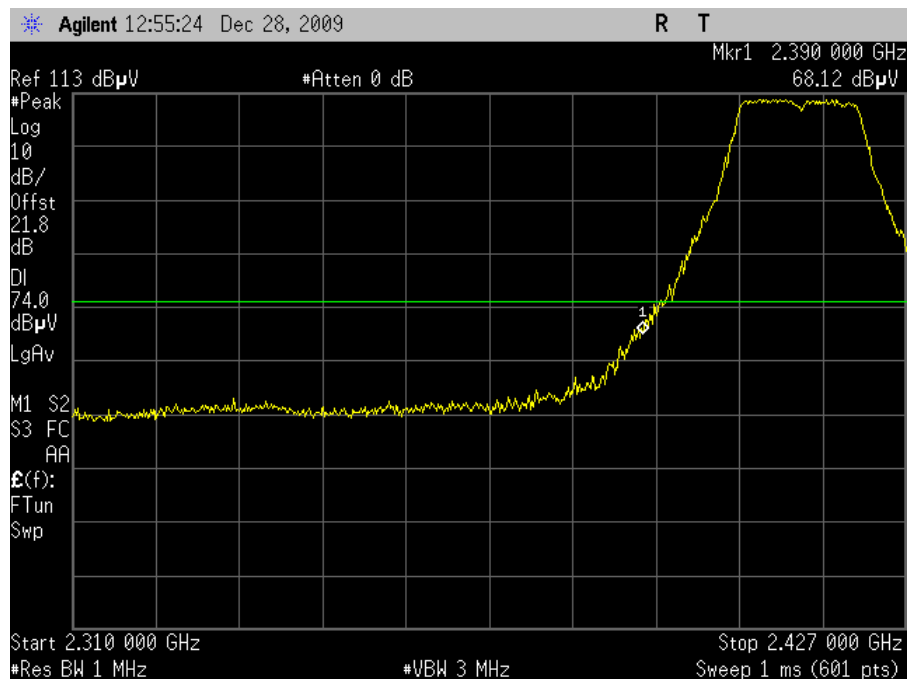
Plot 93. Radiated Restricted Band Edge, 802.11n 20MHz Mode Channel 1, Peak (6dBi Omni)
