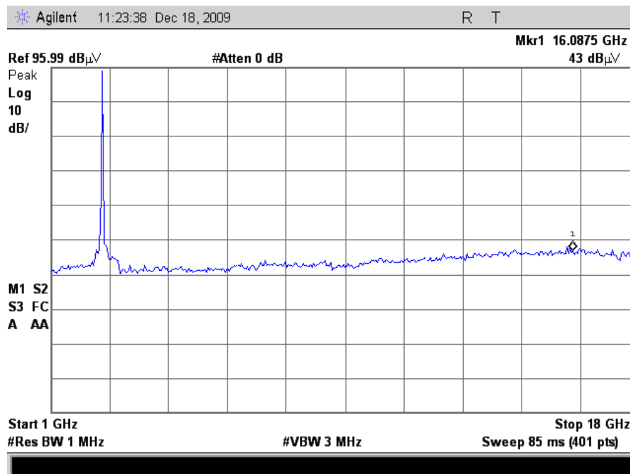
Plot 57. Radiated Spurious Emissions, 802.11g Mode High Channel (24dBm Grid)
