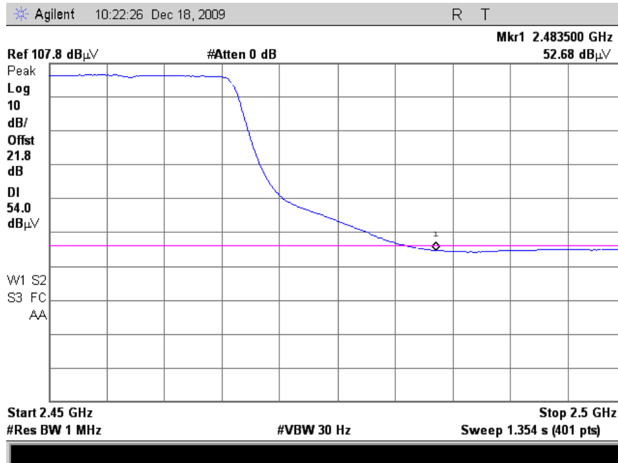
Plot 114. Radiated Restricted Band Edge, 802.11n 20MHz Mode Channel 10, Average (24dB Grid)
