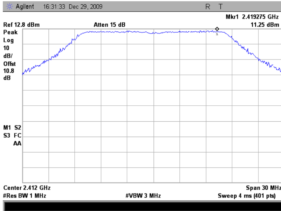
Plot 157. Peak Power Spectral Density, 802.11n 20MHz Mode Low Channel Peak Determination (6dBi Omni Antenna)
