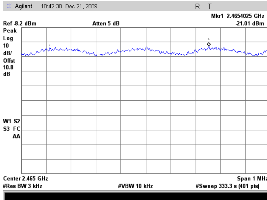
Plot 170. Peak Power Spectral Density, 802.11g Mode High Channel (24dBi Grid Antenna)
