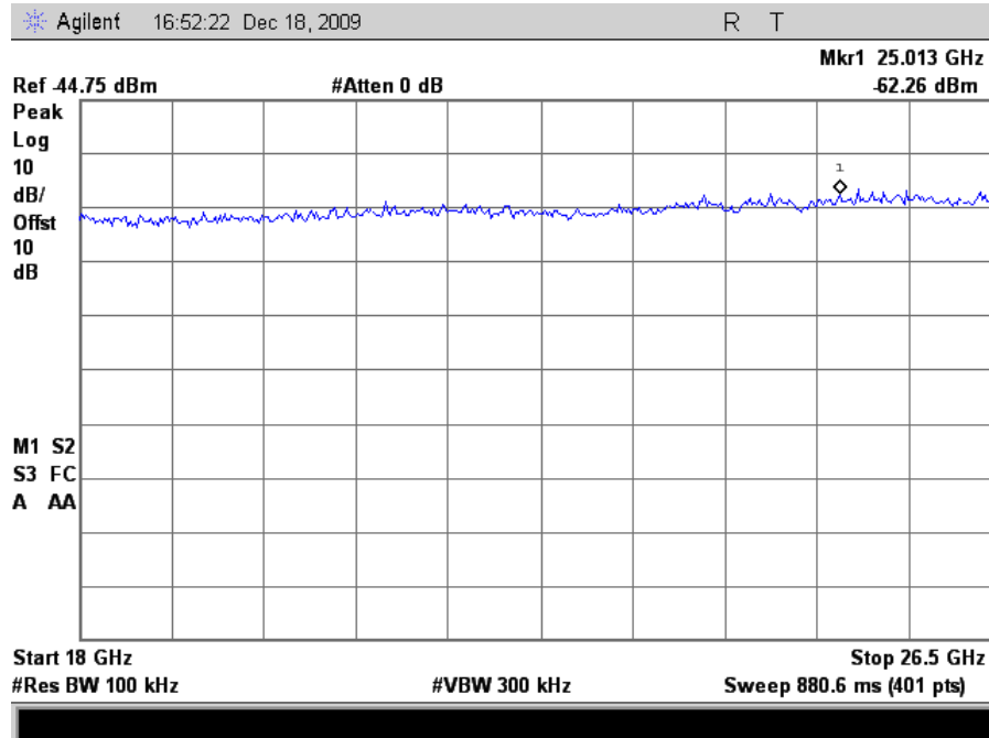
Plot 142. Conducted Emissions, 802.11n 40MHz Mode Mid Channel, 18 GHz – 26.5 GHz
