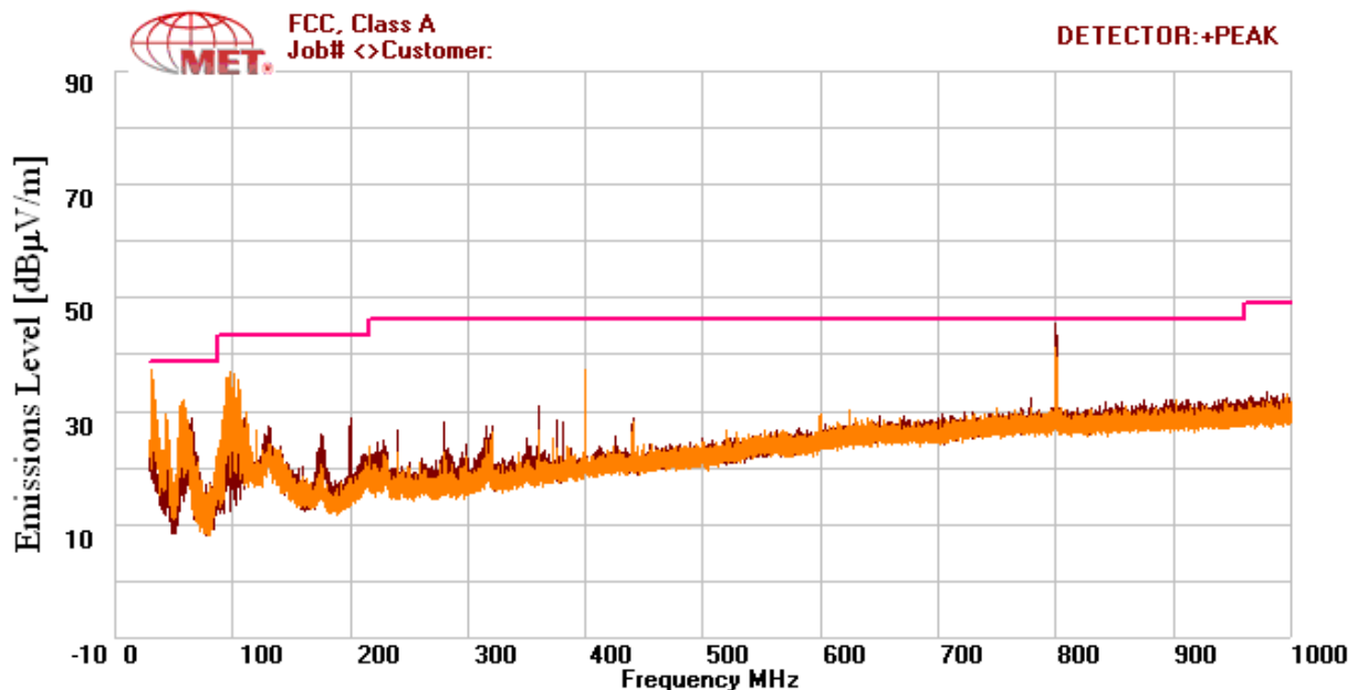
Plot 3. Radiated Emissions, FCC Limits Plot
