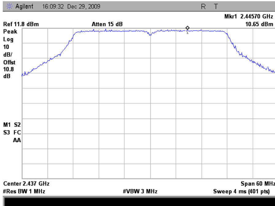
Plot 163. Peak Power Spectral Density, 802.11n 40MHz Mode Mid Channel Peak Determination (6dBi Omni Antenna)
