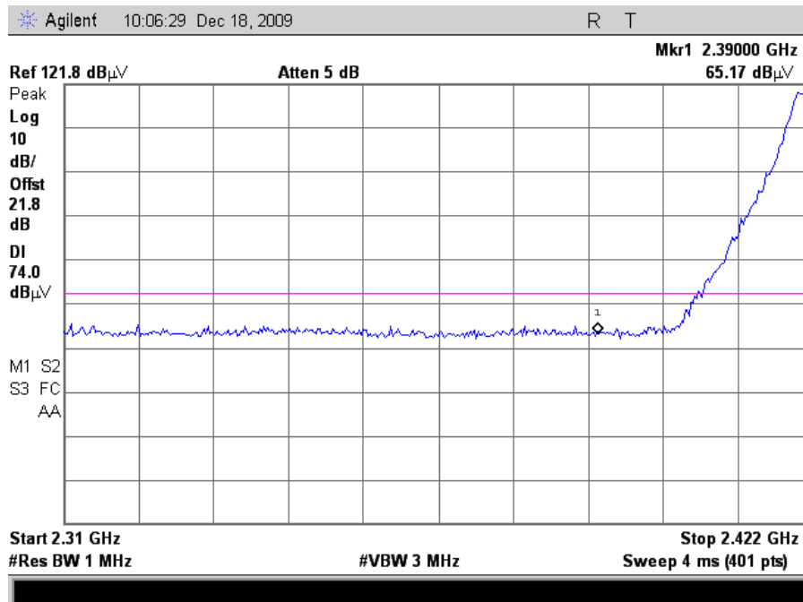
Plot 83. Radiated Restricted Band Edge, 802.11g Mode Channel 4, Peak (24dB Grid)
