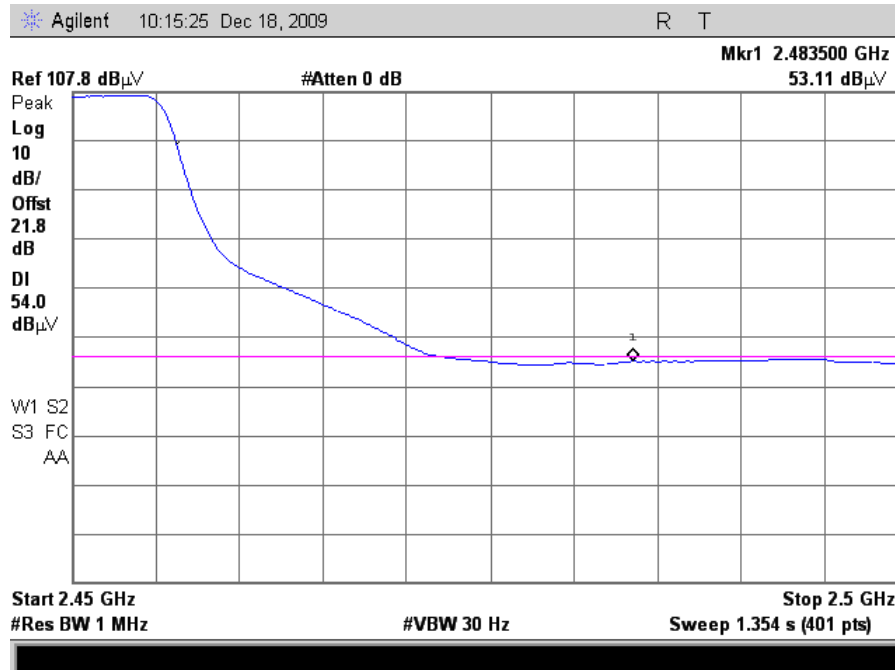
Plot 84. Radiated Restricted Band Edge, 802.11g Mode Channel 8, Average (24dBi Grid)
