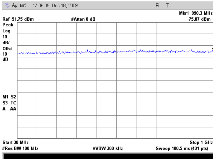
Plot 134. Conducted Emissions, 802.11n 20MHz Mode Mid Channel, 30 MHz – 1 GHz
