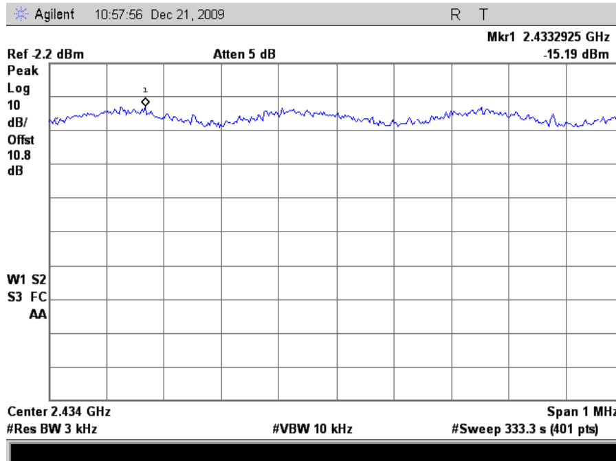
Plot 174. Peak Power Spectral Density, 802.11n 20MHz Mode Mid Channel (24dBi Grid Antenna)
