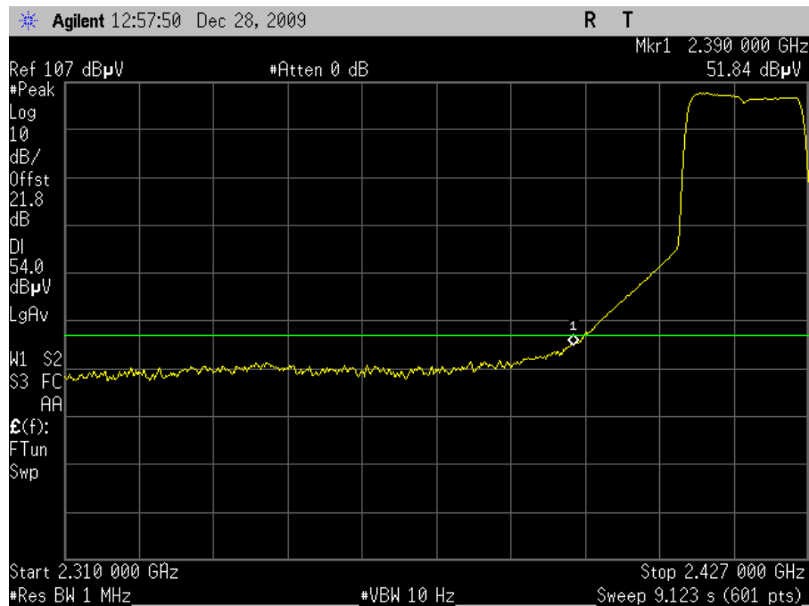
Plot 94. Radiated Restricted Band Edge, 802.11n 20MHz Mode Channel 2, Average (6dBi Omni)
