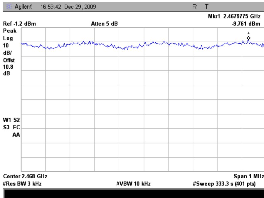
Plot 156. Peak Power Spectral Density, 802.11g Mode High Channel (6dBi Omni Antenna)
