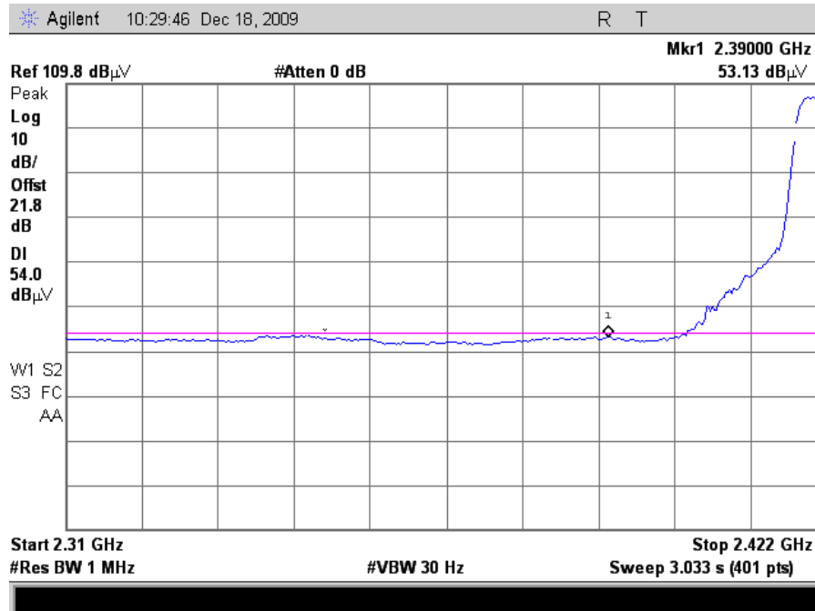
Plot 108. Radiated Restricted Band Edge, 802.11n 20MHz Mode Channel 4, Average (24dB Grid)
