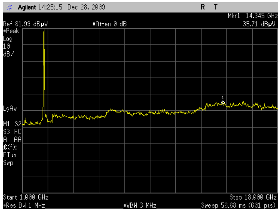
Plot 64. Radiated Spurious Emissions, 802.11n 40MHz Mode Mid Channel (6dBi Omni)
