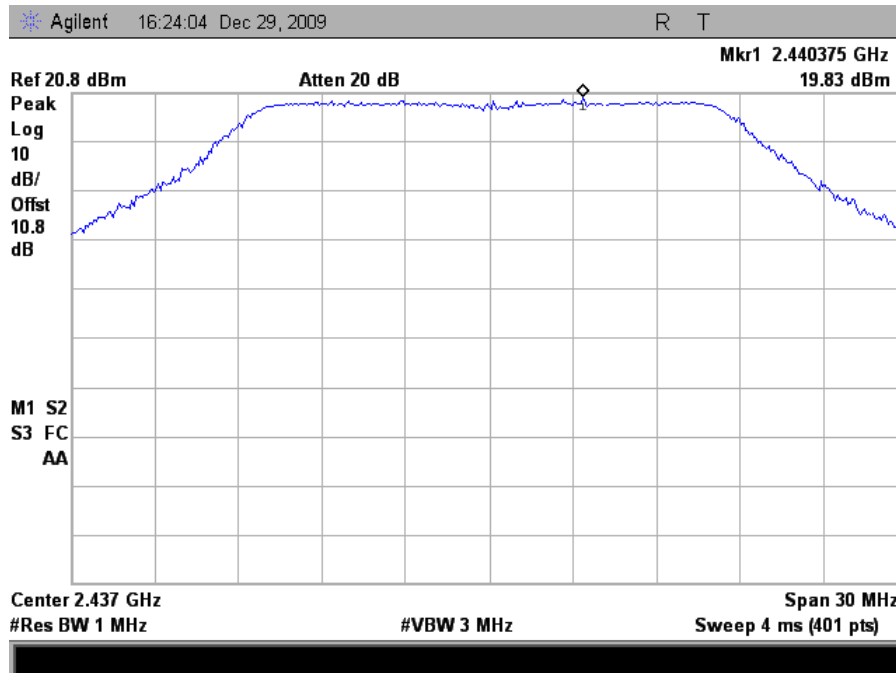
Plot 159. Peak Power Spectral Density, 802.11n 20MHz Mode Mid Channel Peak Determination (6dBi Omni Antenna)
