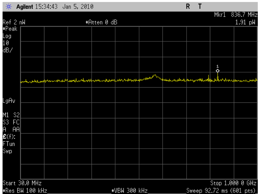
Plot 149. Conducted Receiver Spurious Emission, 30MHz – 1GHz
