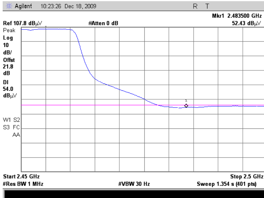
Plot 112. Radiated Restricted Band Edge, 802.11n 20MHz Mode Channel 9, Average (24dB Grid)
