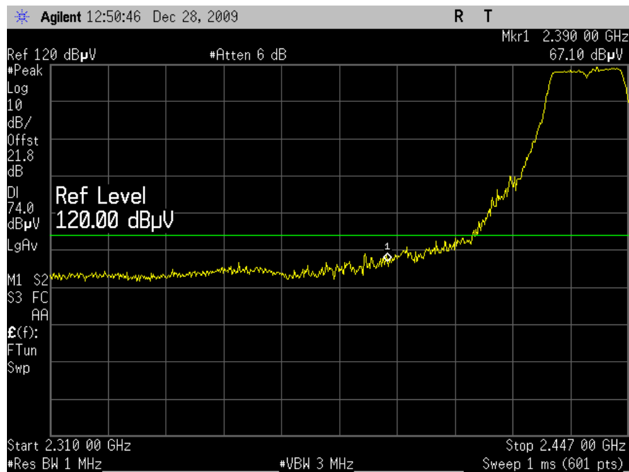
Plot 97. Radiated Restricted Band Edge, 802.11n 20MHz Mode Channel 6, Peak (6dBi Omni)
