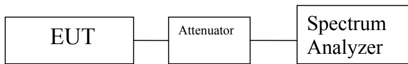
Figure 6. Block Diagram, Peak Power Spectral Density Test Setup
