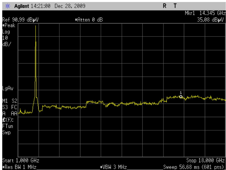
Plot 53. Radiated Spurious Emissions, 802.11g Mode Mid Channel (6dBi Omni)
