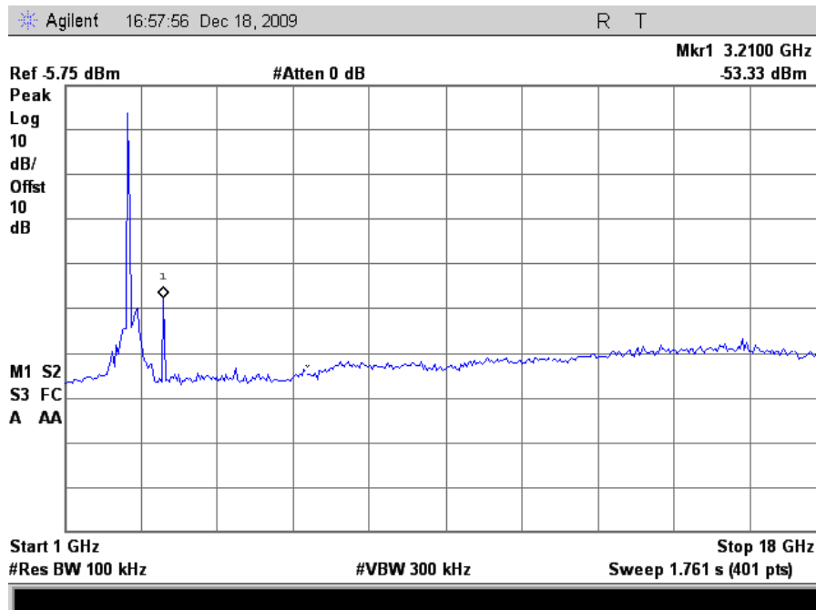
Plot 123. Conducted Emissions, 802.11g Mode Low Channel, 1 GHz – 18 GHz
