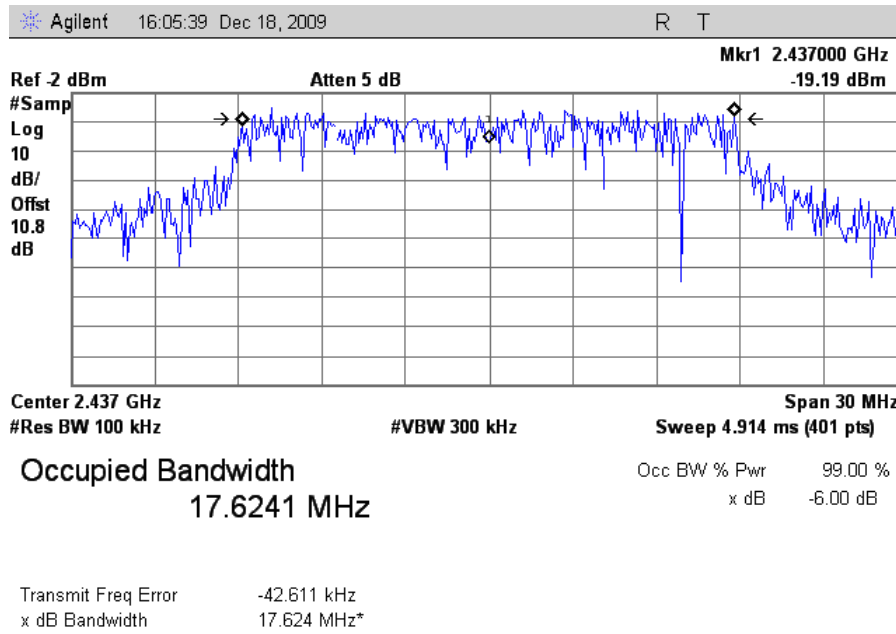
Plot 15. Occupied Band Width, 802.11n 20MHz Mode Mid Channel, FCC, 6 dB
