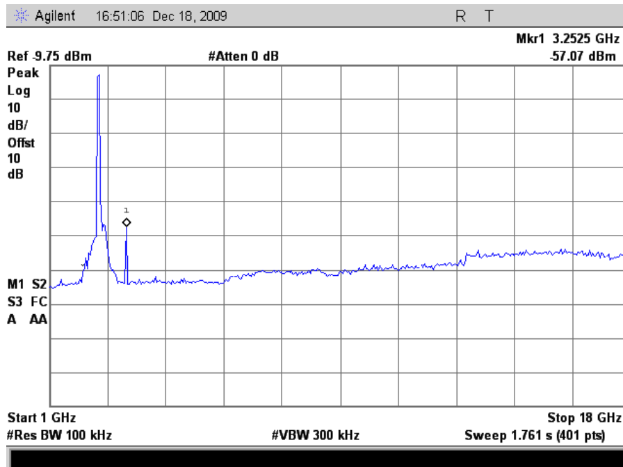
Plot 141. Conducted Emissions, 802.11n 40MHz Mode Mid Channel, 1 GHz – 18 GHz
