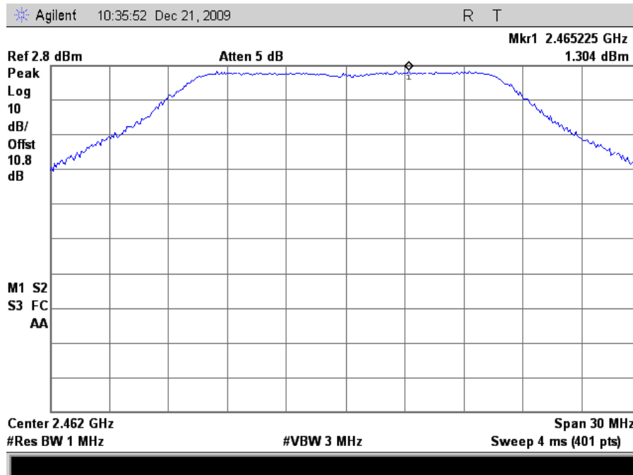
Plot 169. Peak Power Spectral Density, 802.11g Mode High Channel Peak Determination (24dBi Grid Antenna)
