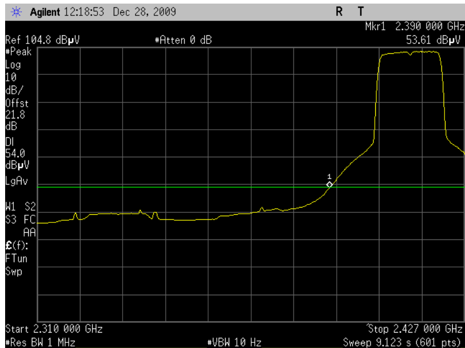
Plot 66. Radiated Restricted Band Edge, 802.11g Mode Channel 1, Average (6dBi Omni)
