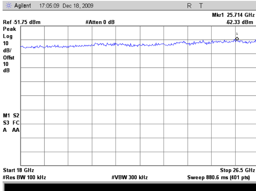
Plot 139. Conducted Emissions, 802.11n 20MHz Mode High Channel, 18 GHz – 26.5 GHz
