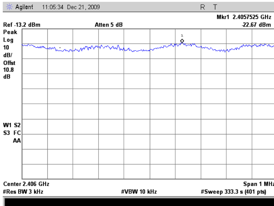
Plot 172. Peak Power Spectral Density, 802.11n 20MHz Mode Low Channel (24dBi Grid Antenna)
