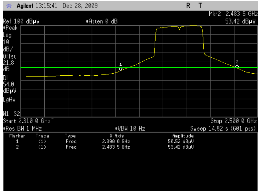
Plot 118. Radiated Restricted Band Edge, 802.11n 40MHz Mode Channel 6, Average (6dBi Omni)
