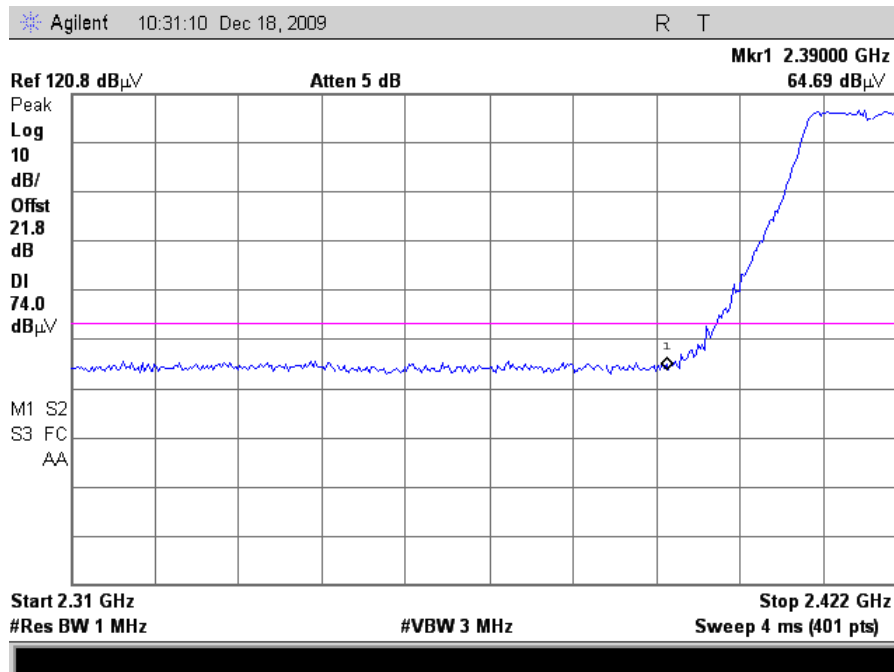
Plot 105. Radiated Restricted Band Edge, 802.11n 20MHz Mode Channel 2, Peak (24dB Grid)
