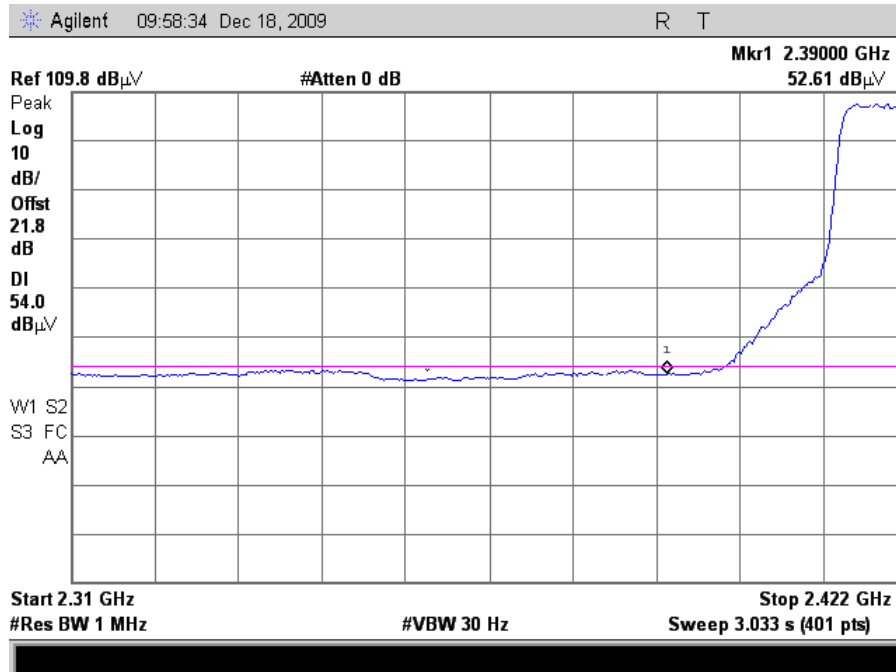
Plot 80. Radiated Restricted Band Edge, 802.11g Mode Channel 3, Average (24dB Grid)
