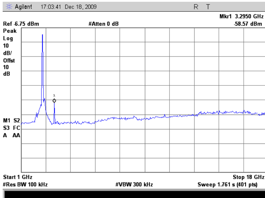
Plot 138. Conducted Emissions, 802.11n 20MHz Mode High Channel, 1 GHz – 18 GHz
