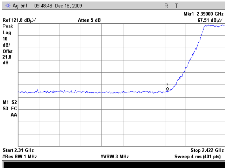
Plot 79. Radiated Restricted Band Edge, 802.11g Mode Channel 2, Peak (24dB Grid)
