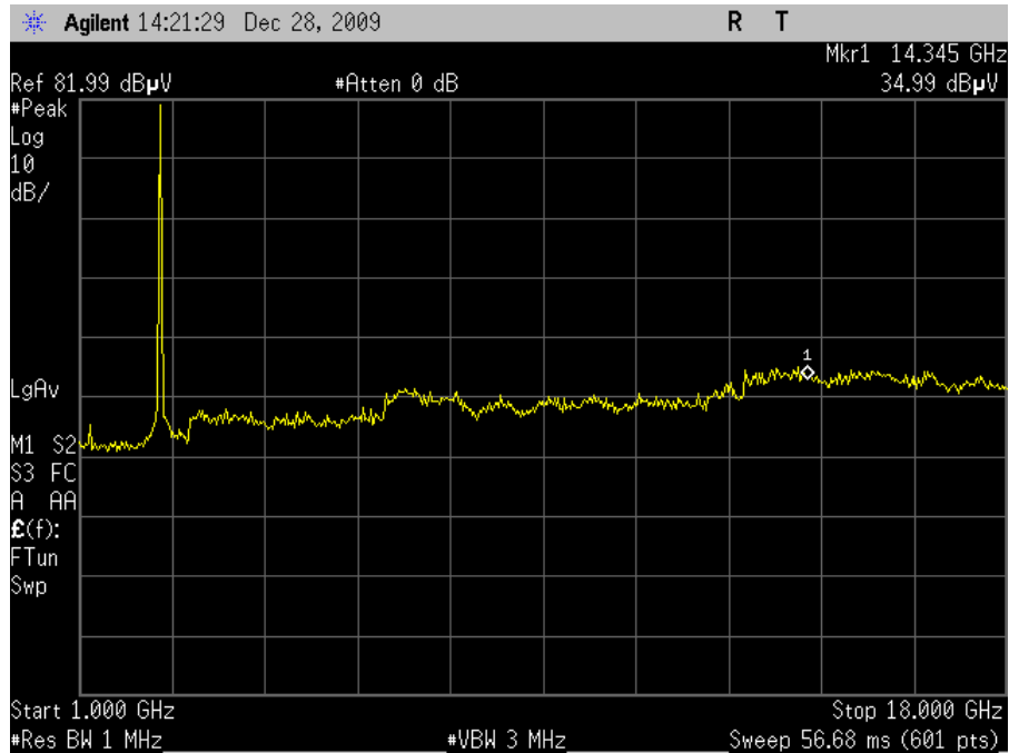
Plot 54. Radiated Spurious Emissions, 802.11g Mode High Channel (6dBi Omni)
