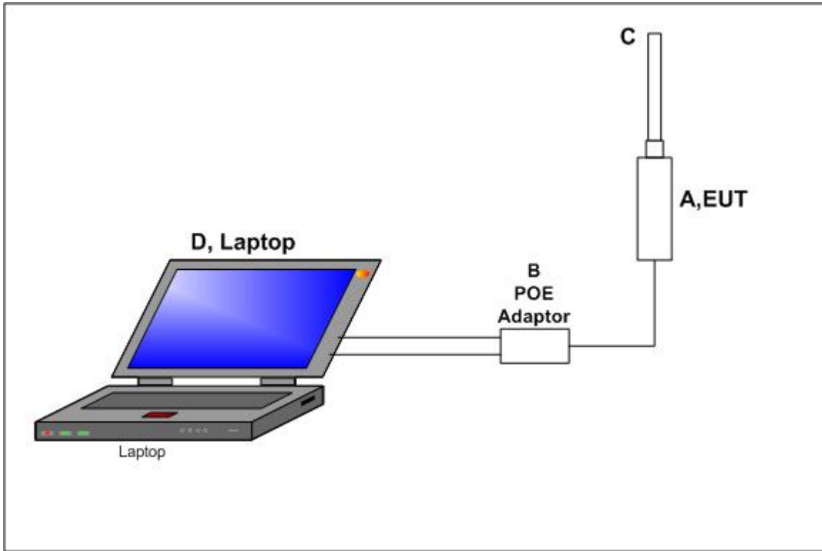
Figure 2. Block Diagram of Test Configuration, Omni Antenna
