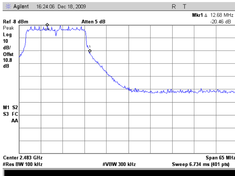
Plot 146. Conducted Band Edge, 802.11n 20MHz Mode, High
