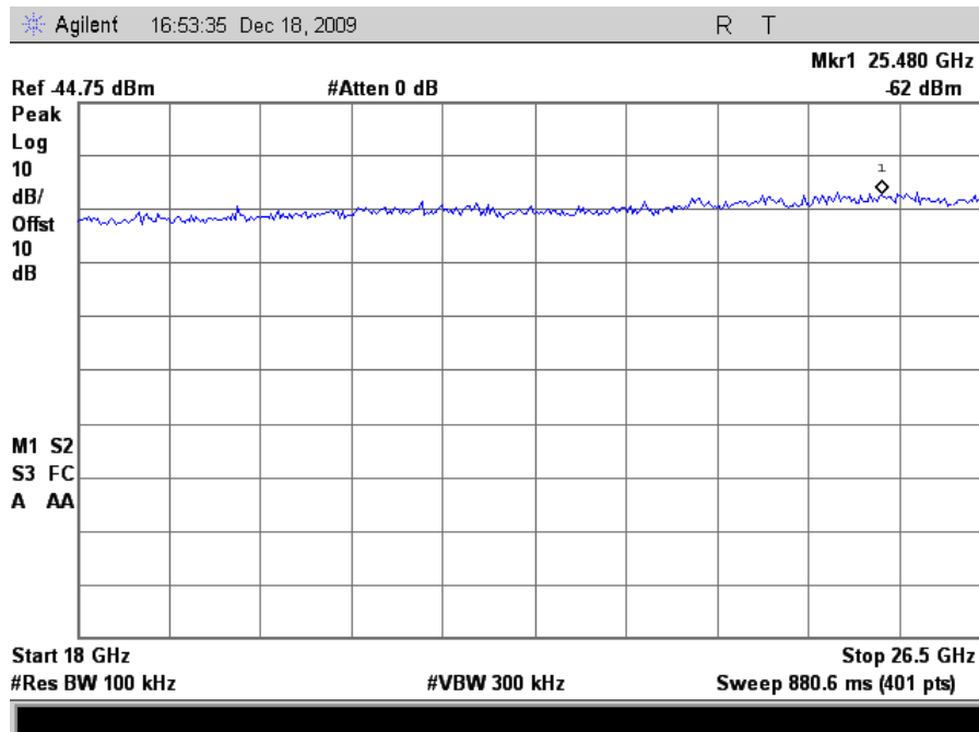
Plot 127. Conducted Emissions, 802.11g Mode Mid Channel, 18 GHz – 26.5 GHz
