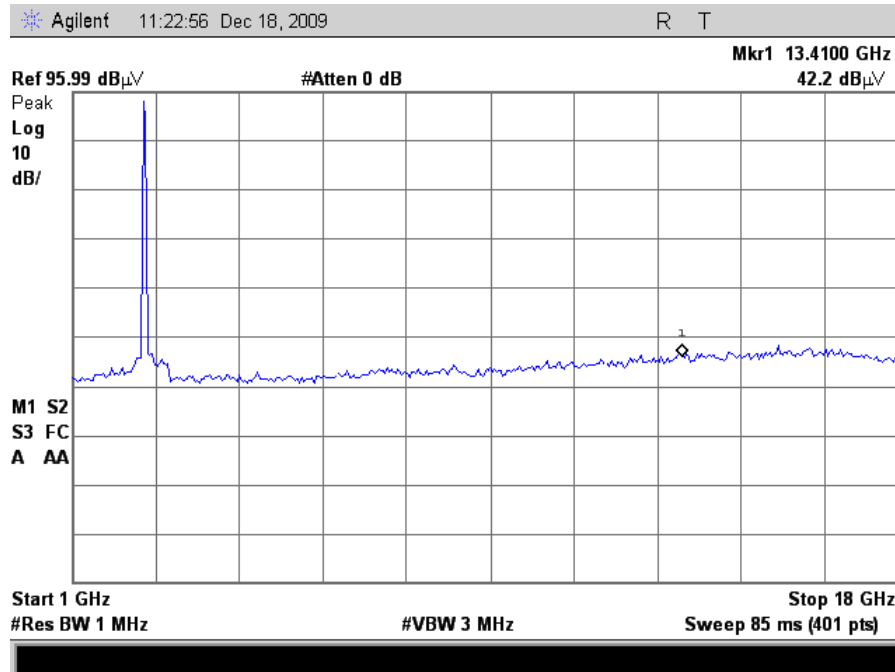
Plot 56. Radiated Spurious Emissions, 802.11g Mode Mid Channel (24dBm Grid)
