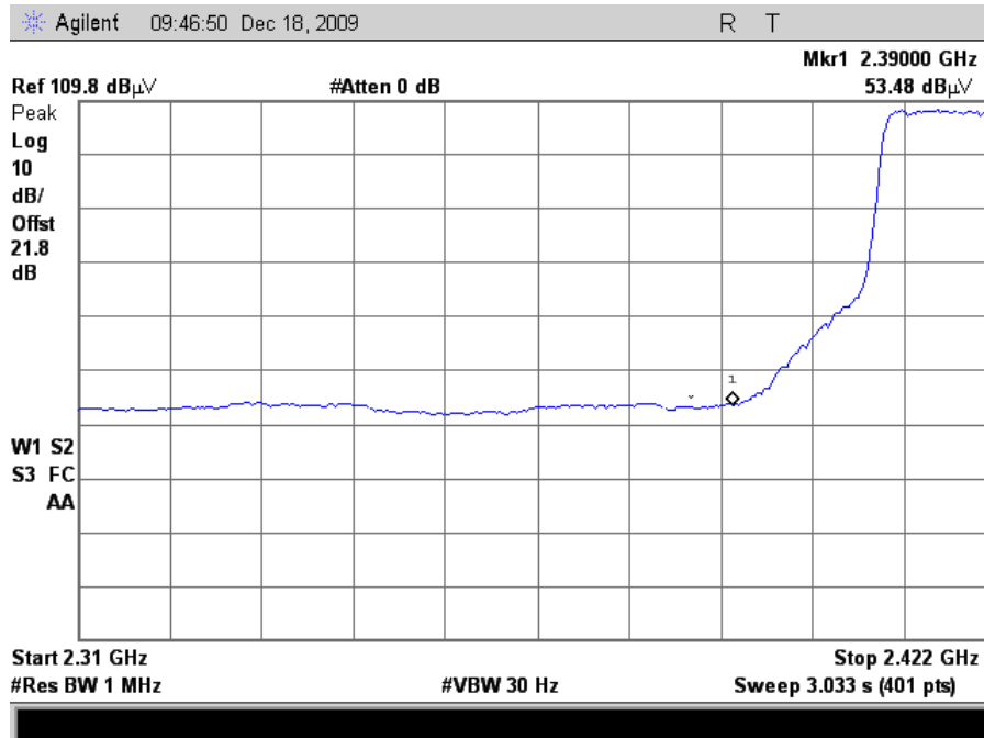
Plot 78. Radiated Restricted Band Edge, 802.11g Mode Channel 2, Average (24dB Grid)
