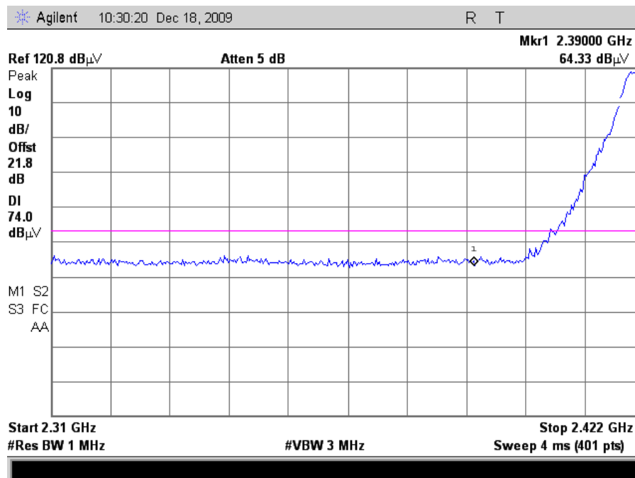
Plot 109. Radiated Restricted Band Edge, 802.11n 20MHz Mode Channel 4, Peak (24dB Grid)
