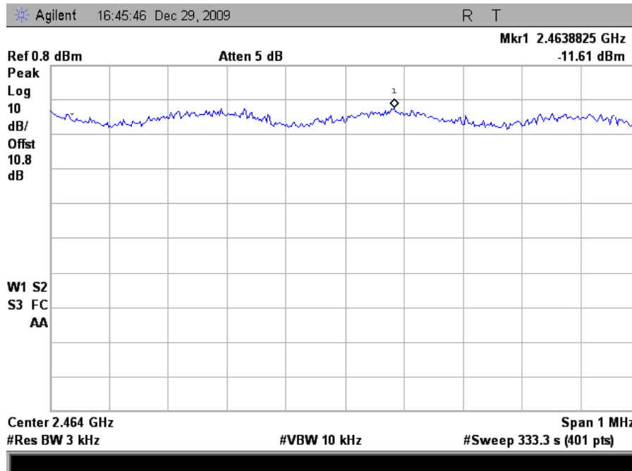
Plot 162. Peak Power Spectral Density, 802.11n 20MHz Mode High Channel (6dBi Omni Antenna)
