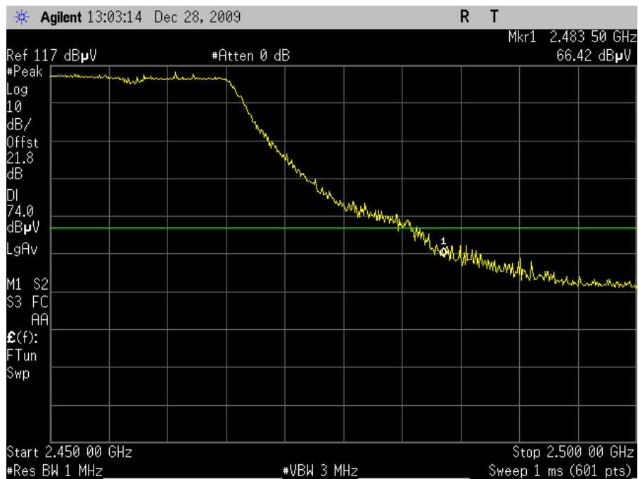
Plot 99. Radiated Restricted Band Edge, 802.11n 20MHz Mode Channel 10, Peak (6dBi Omni)
