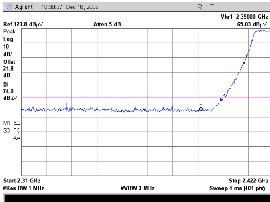
Plot 107. Radiated Restricted Band Edge, 802.11n 20MHz Mode Channel 3, Peak (24dB Grid)
