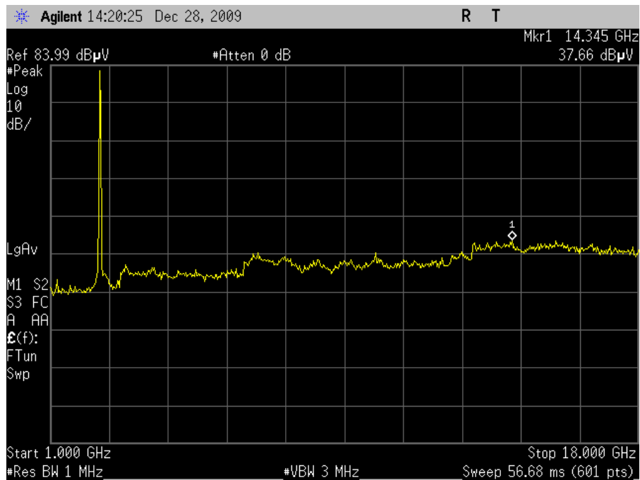
Plot 52. Radiated Spurious Emissions, 802.11g Mode Low Channel (6dBi Omni)
