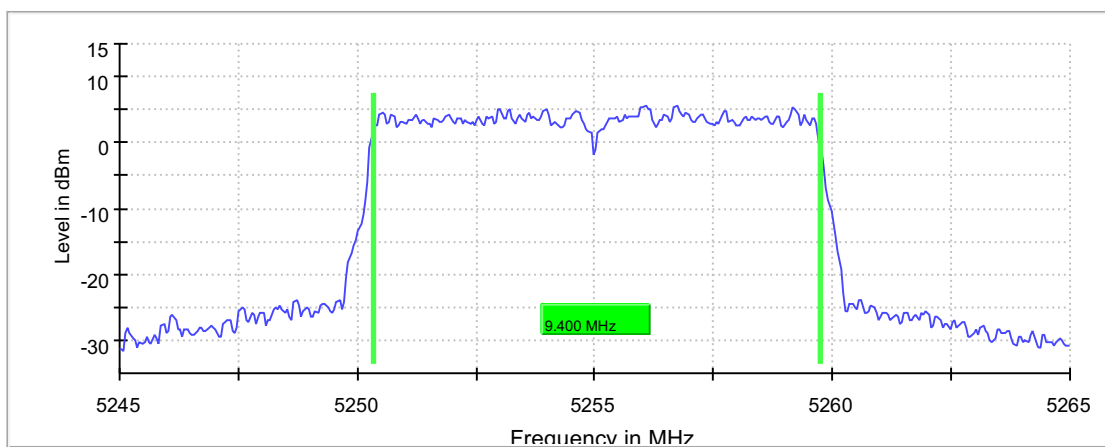
99 % Bandwidth
