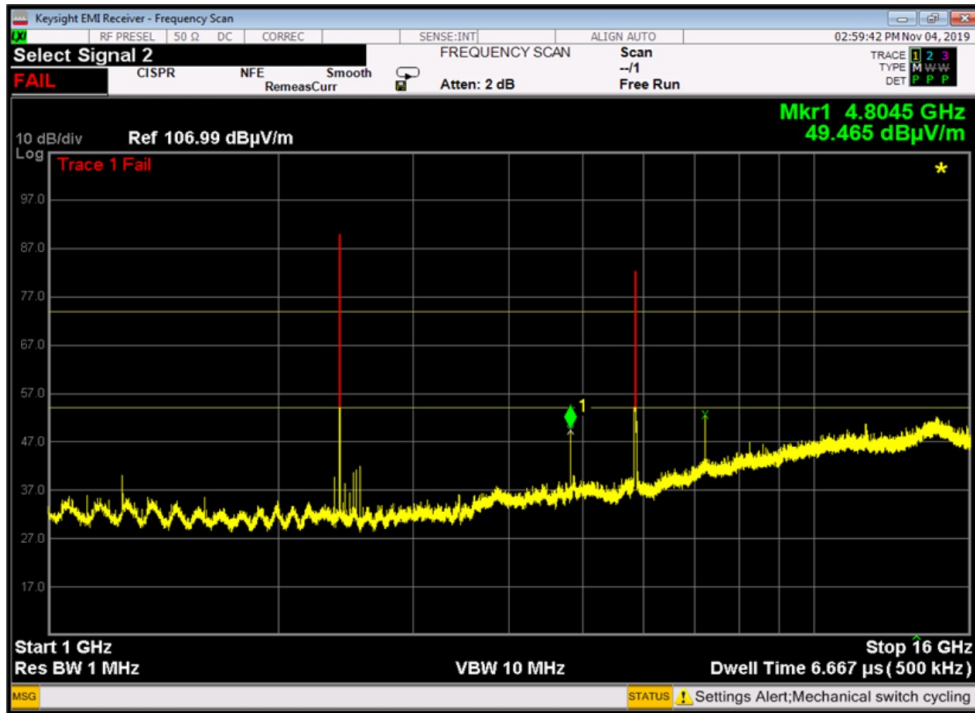
Graph 9: Worst Case Receiver Plot (1-16GHz; Horizontal, at 5840MHz, 20MHz BW)
