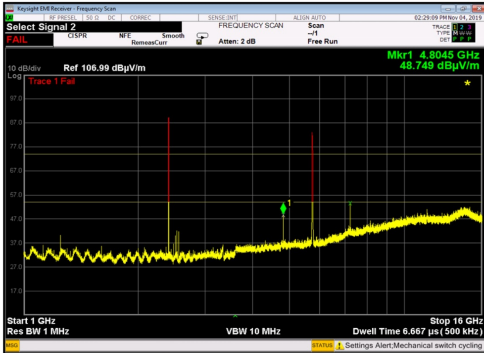
Graph 5: Worst Case Receiver Plot (1-16GHz; Horizontal, at 5735, 20MHz BW)
