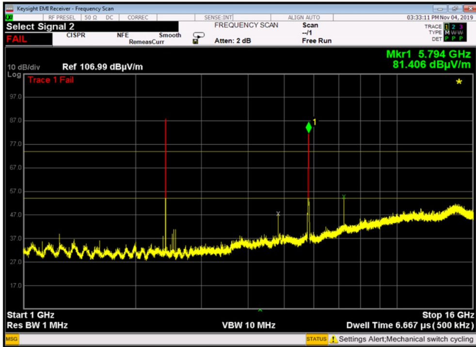
Graph 7: Worst Case Receiver Plot (1-16GHz; Horizontal, at 5790MHz, 30MHz
