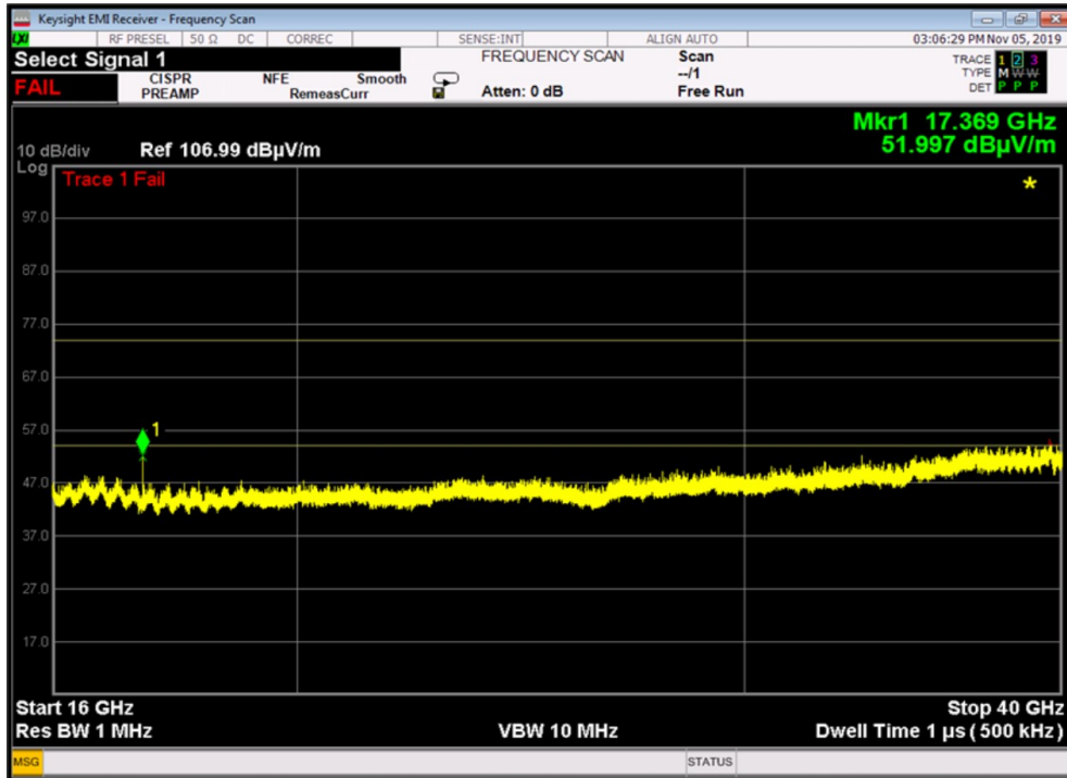
Graph 8: Worst Case Receiver Plot (16-40GHz; Vertical, at 5790MHz, 10MHz BW)
