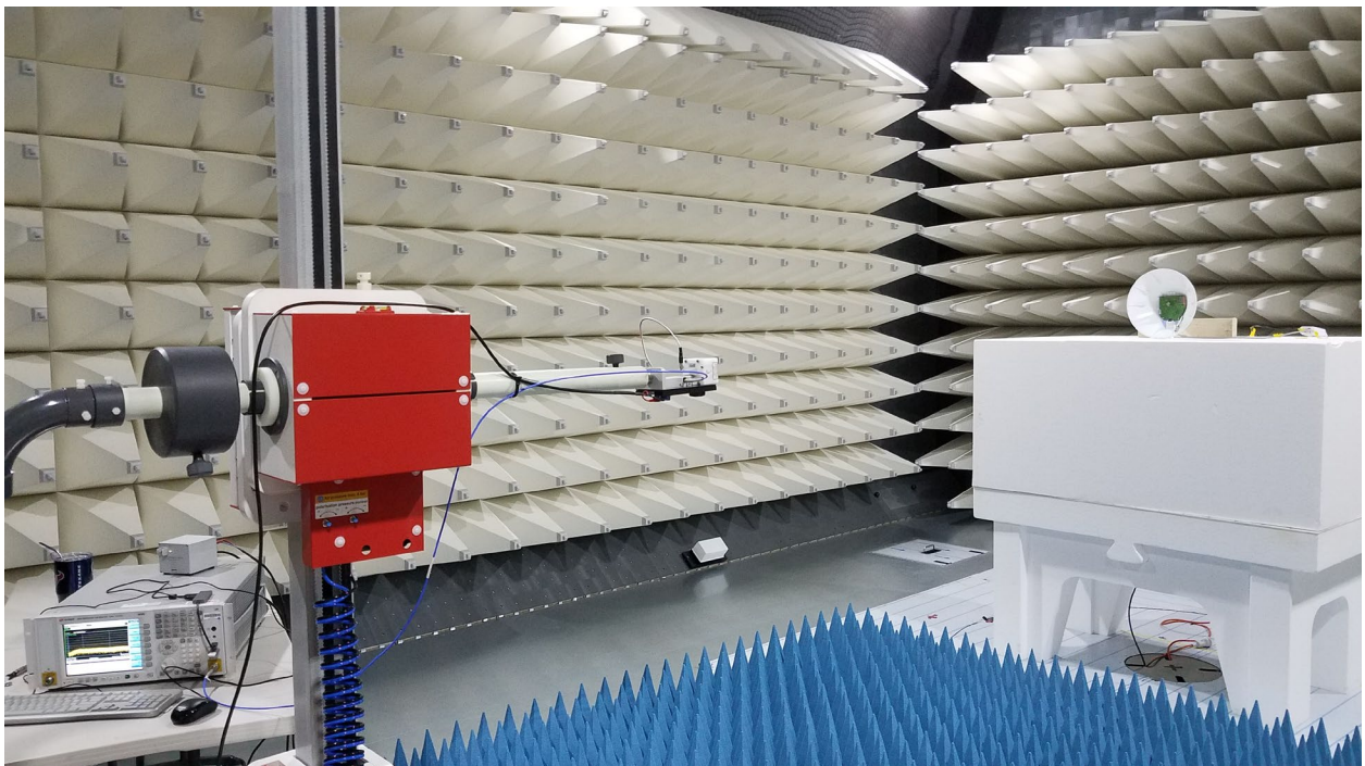
Radiated Emissions 16 GHz – 40 GHz
