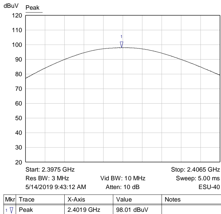
Graph 4: Lowest Channel Output Power Plot
