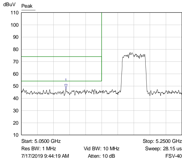
Graph 28: Band Edge Transmitting 5185 MHz at TP12 – Conducted Antenna Port Measurement (J3)
