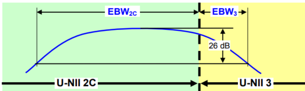
Figure 4. Non-overlapping emissions bandwidths (KDB 789033 D02 v02r01, p 19)
