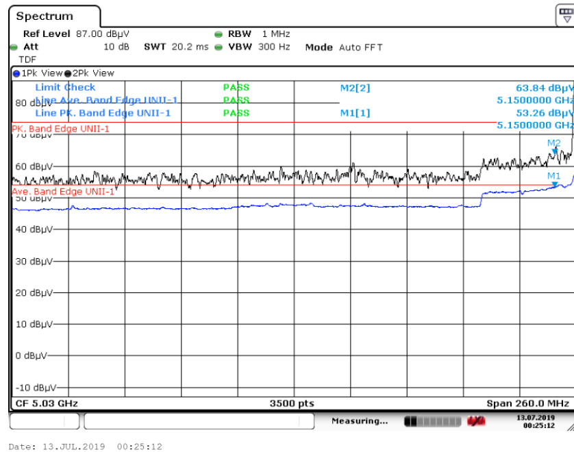
Graph 39: Band Edge Transmitting 5180 MHz at TP4 – Conducted Antenna Port Measurement (J3)
