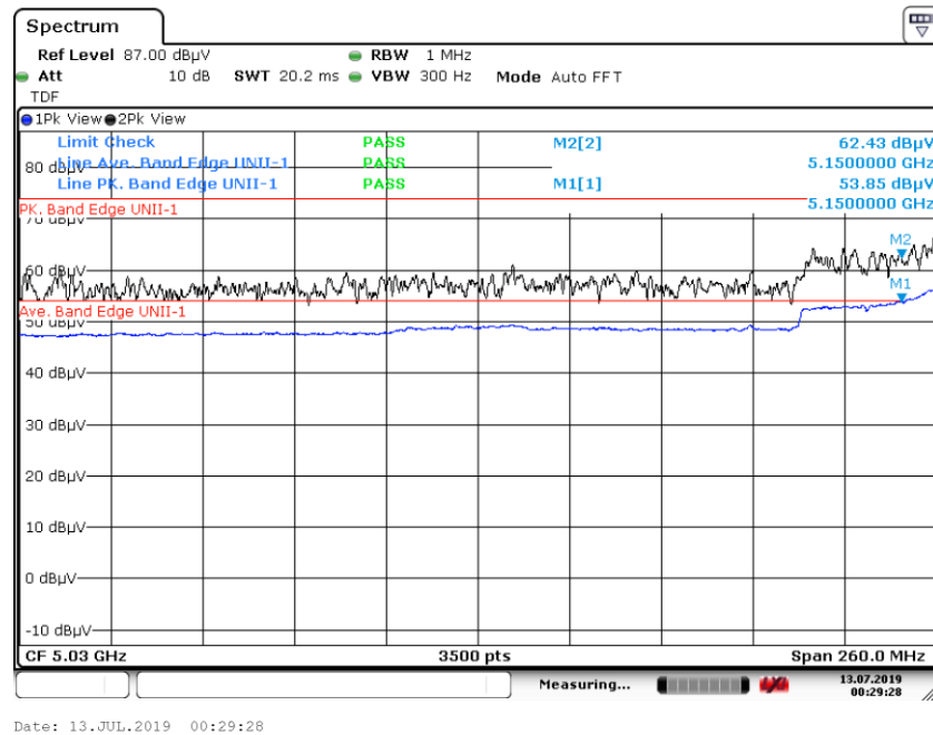
Graph 41: Band Edge Transmitting 5185 MHz at TP6 – Conducted Antenna Port Measurement (J3)
