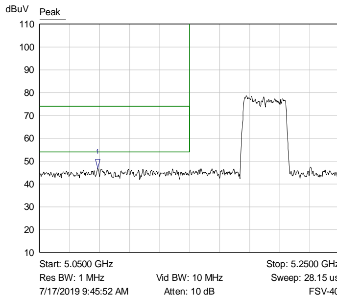
Graph 30: Band Edge Transmitting 5190 MHz at TP13 – Conducted Antenna Port Measurement (J2)
