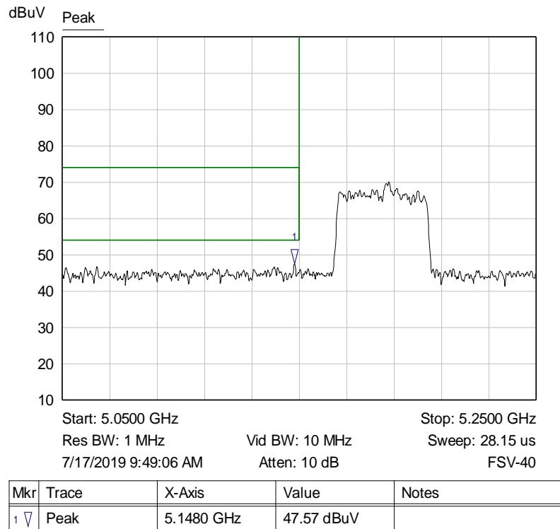
Graph 39: Band Edge Transmitting 5180 MHz at TP4 – Conducted Antenna Port Measurement (J3)
