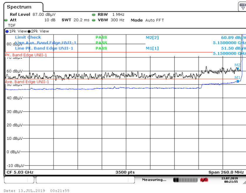
Graph 37: Band Edge Transmitting 5175 MHz at TP2 – Conducted Antenna Port Measurement (J3)
