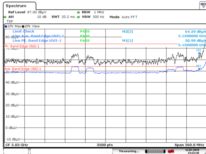
Graph 6: Band Edge Transmitting 5170 MHz at TP14 – Conducted Antenna Port Measurement (J2)
