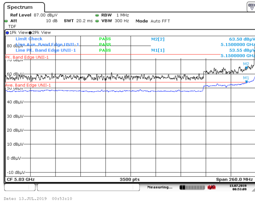
Graph 54: Band Edge Transmitting 5185 MHz at TP4 – Conducted Antenna Port Measurement (J2)
