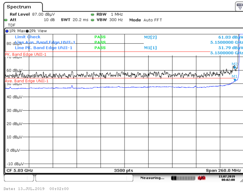
Graph 22: Band Edge Transmitting 5170 MHz at TP2 – Conducted Antenna Port Measurement (J3)
