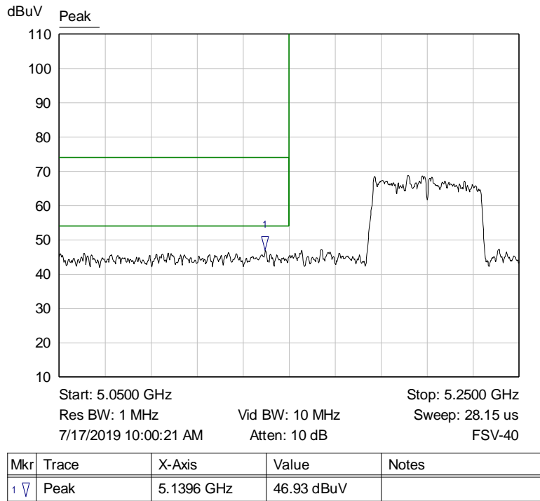
Graph 56: Band Edge Transmitting 5190 MHz at TP6 – Conducted Antenna Port Measurement (J2)
