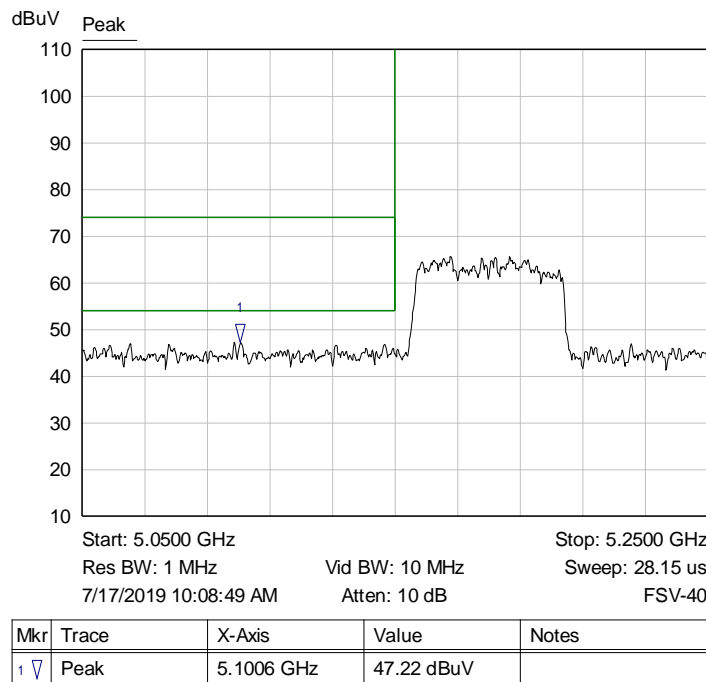
Graph 51: Band Edge Transmitting 5180 MHz at TP2 – Radiated Cabinet Emission Measurement
