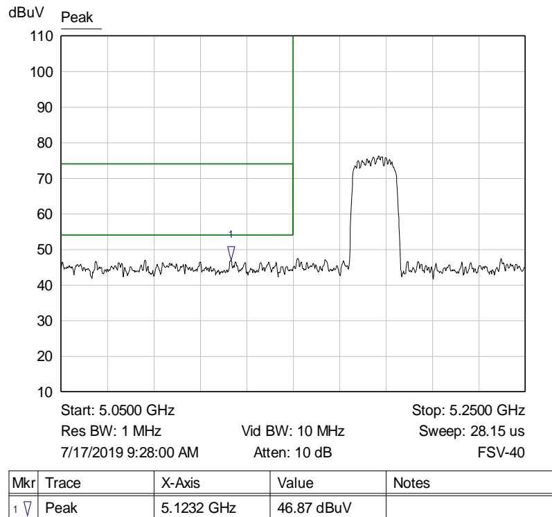
Graph 13: 5170 MHz at TP9 Bandwidth – Conducted Antenna Port Measurement (J3)
