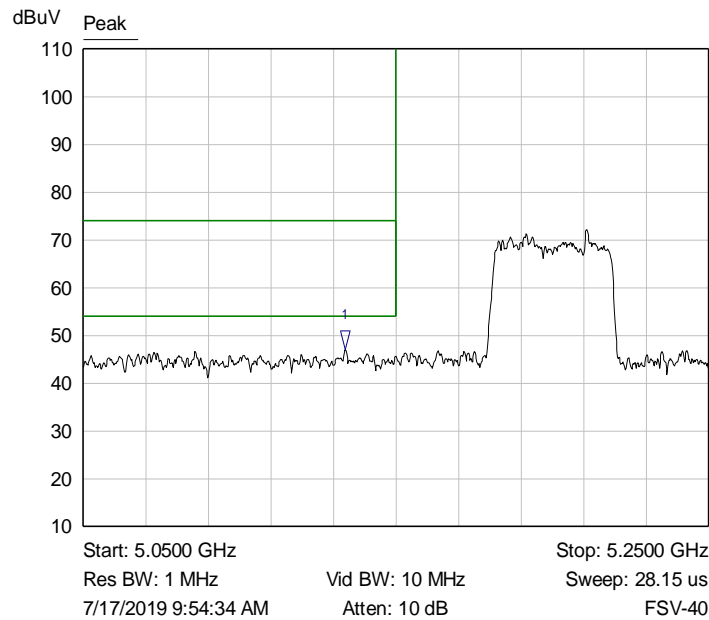
Graph 43: Band Edge Transmitting 5190 MHz at TP7 – Conducted Antenna Port Measurement
