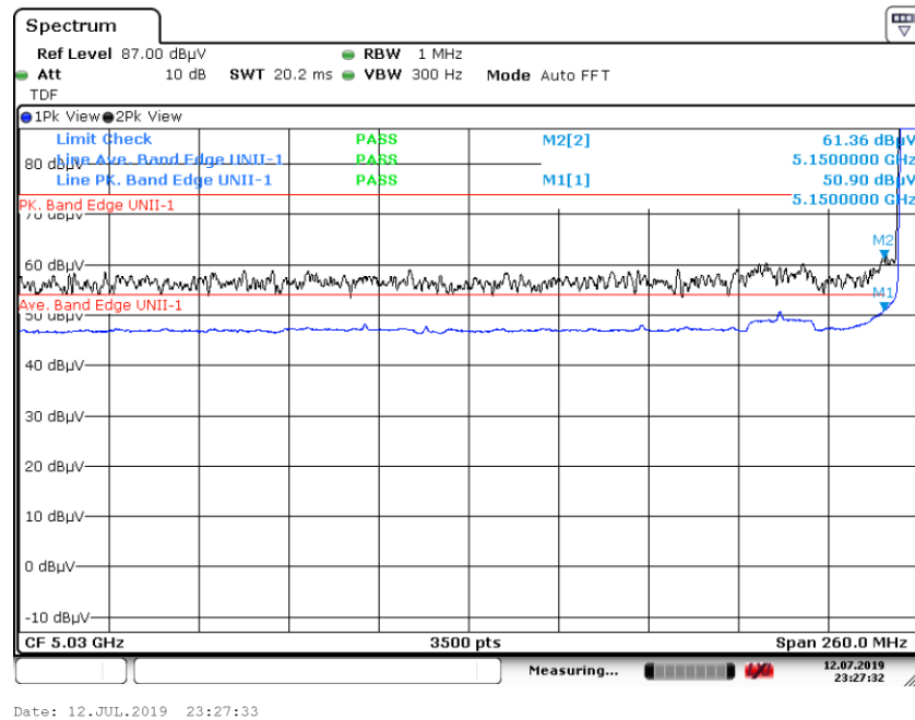
Graph 11: Band Edge Transmitting 5165 MHz at TP2 – Conducted Antenna Port Measurement (J2)
