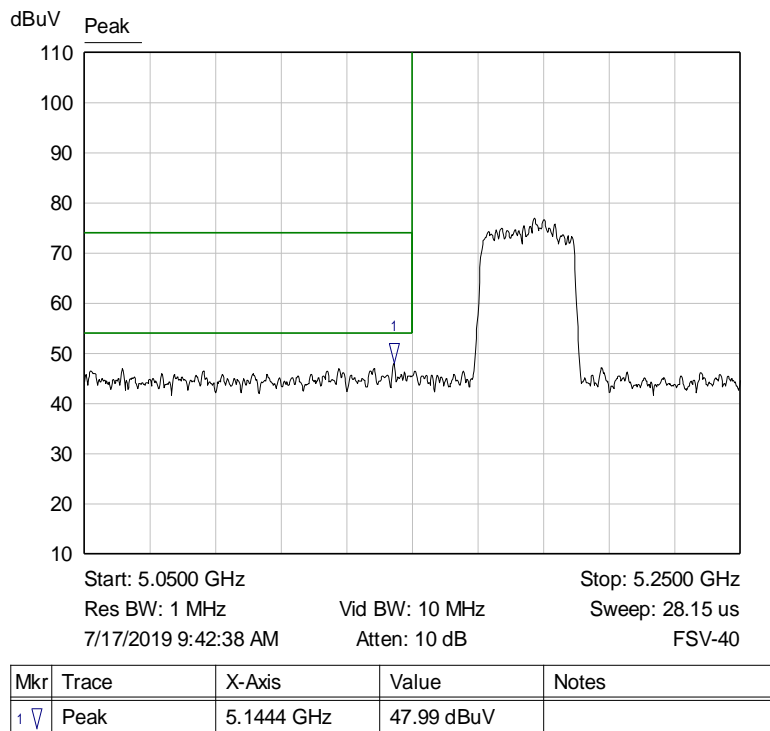
Graph 26: Band Edge Transmitting 5180 MHz at TP11 – Conducted Antenna Port Measurement (J3)
