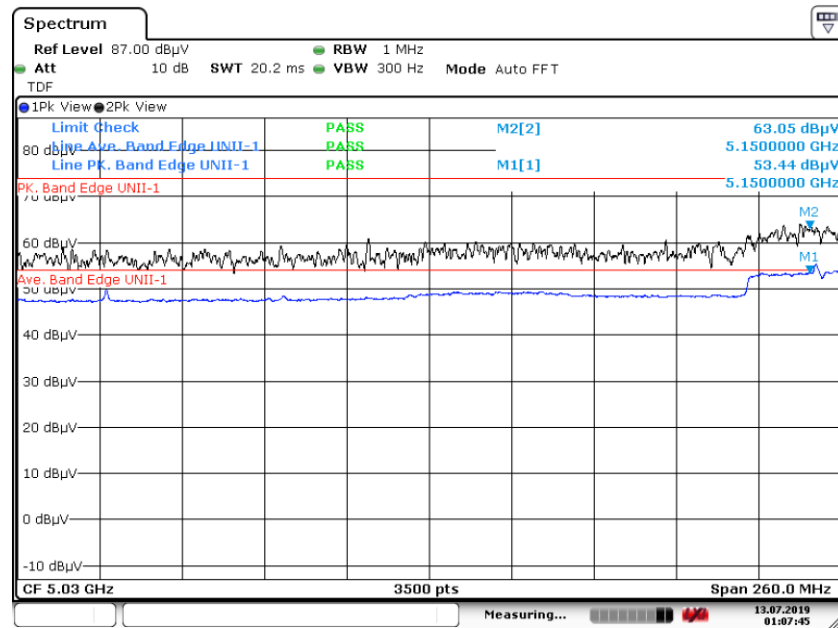
Graph 58: Band Edge Transmitting 5210 MHz at TP7 – Conducted Antenna Port Measurement (J3)
