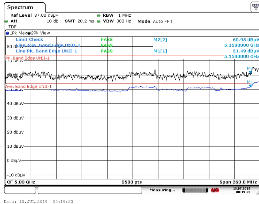
Graph 32: Band Edge Transmitting 5200 MHz at TP15 – Conducted Antenna Port Measurement (J2)
