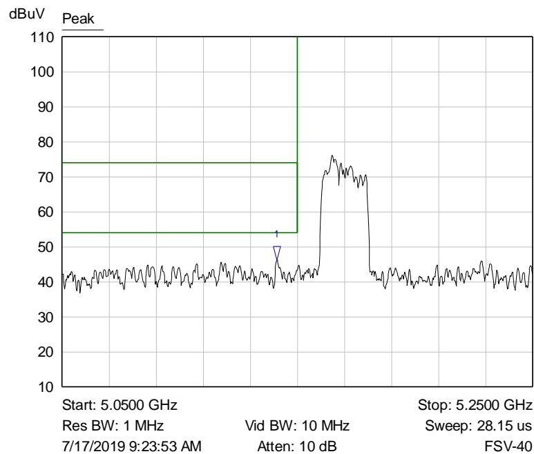
Graph 11: Band Edge Transmitting 5165 MHz at TP2 – Conducted Antenna Port Measurement (J2)
