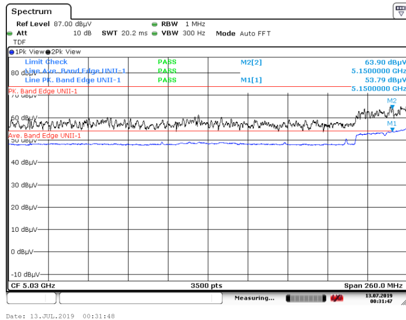
Graph 43: Band Edge Transmitting 5190 MHz at TP7 – Conducted Antenna Port Measurement
