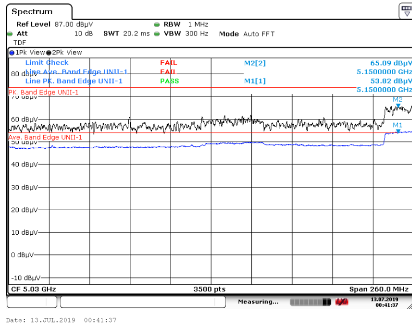
Graph 47: Band Edge Transmitting 5215 MHz at TP15 – Conducted Antenna Port Measurement (J3)
