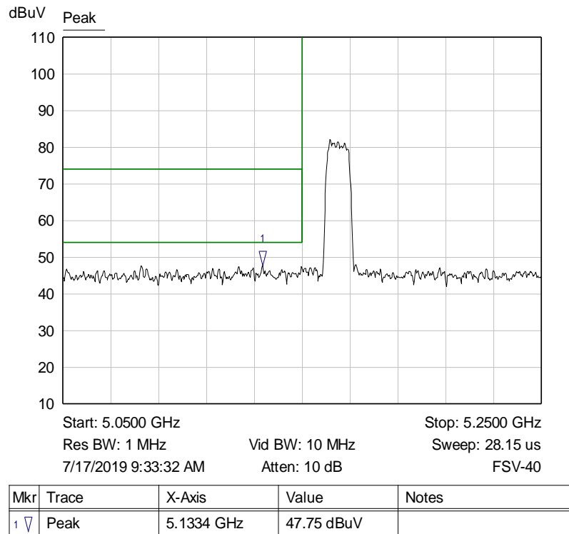
Graph 2: Band Edge Transmitting 5160 MHz at TP2 – Conducted Antenna Port Measurement (J3)
