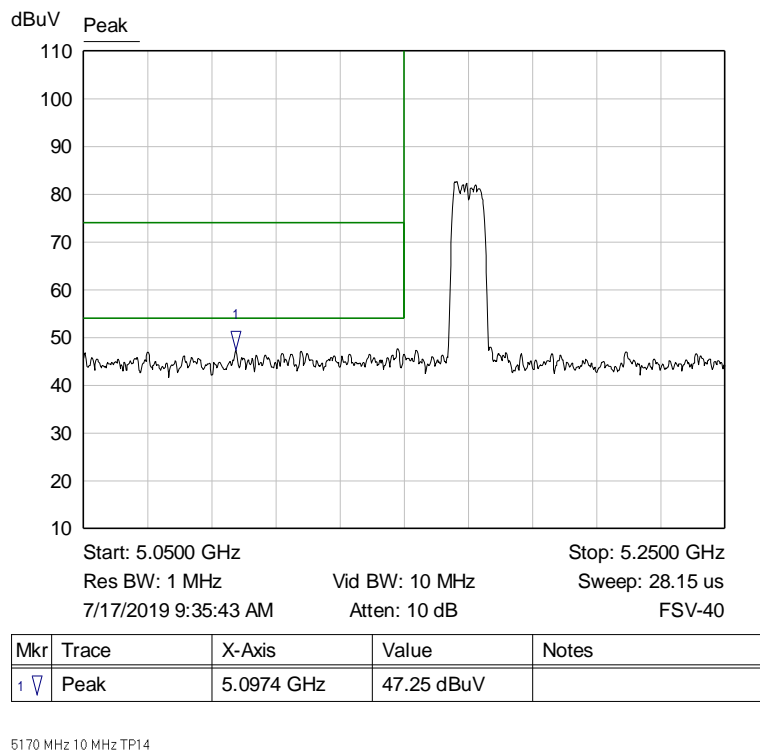
Graph 5: Band Edge Transmitting 5170 MHz at TP14 – Radiated Cabinet Emission Measurement
