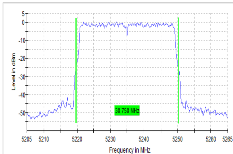
Graph 35: Highest Channel Minimum 26 dB Bandwidth
