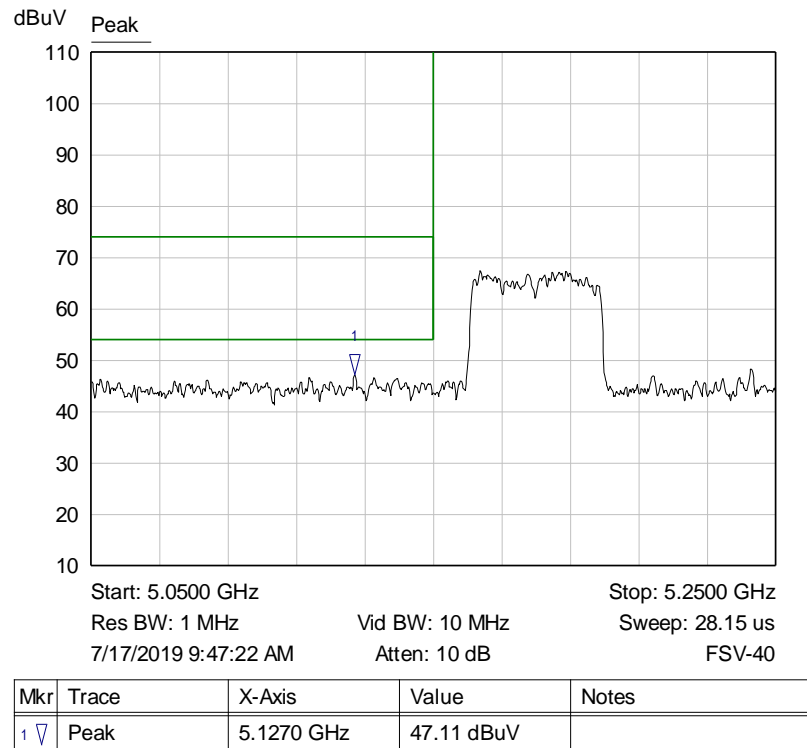
Graph 37: Band Edge Transmitting 5175 MHz at TP2 – Conducted Antenna Port Measurement (J3)
