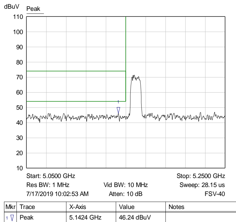
Graph 1: Band Edge Transmitting 5160 MHz at TP2– Radiated Cabinet Emission Measurement
