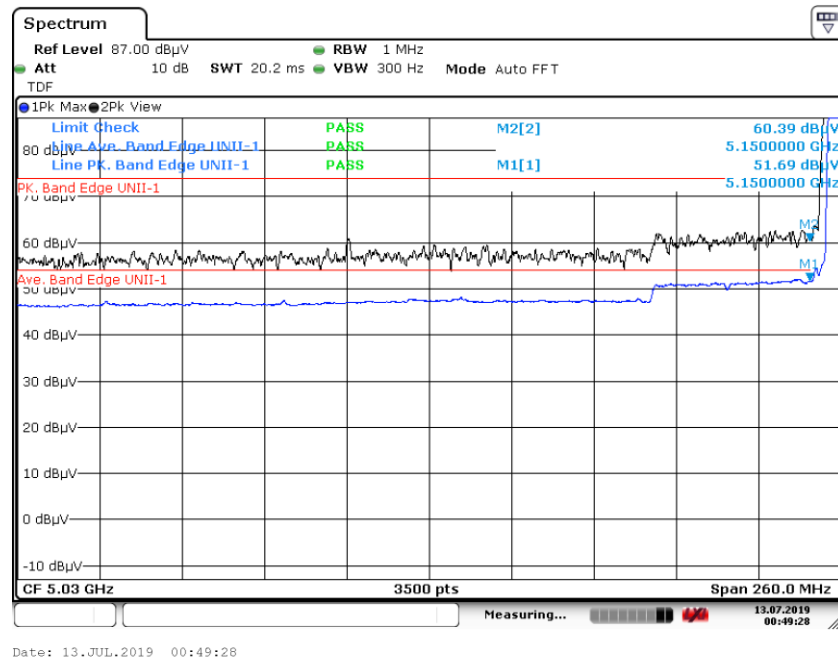
Graph 52: Band Edge Transmitting 5180 MHz at TP2 – Conducted Antenna Port Measurement (J3)
