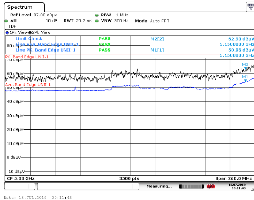
Graph 28: Band Edge Transmitting 5185 MHz at TP12 – Conducted Antenna Port Measurement (J3)
