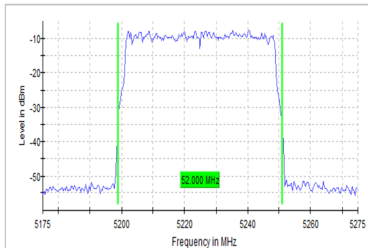
Graph 50: Highest Channel Minimum 26 dB Bandwidth
