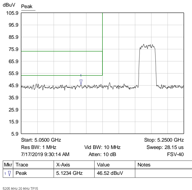
Graph 16: Band Edge Transmitting 5205 MHz at TP15 – Radiated Cabinet Emission Measurement
