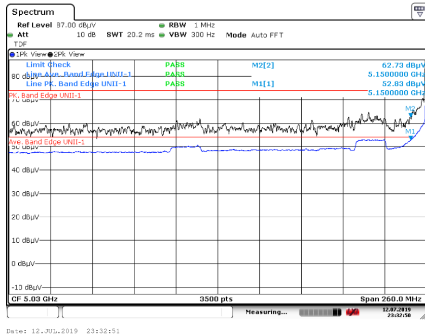
Graph 13: 5170 MHz at TP9 Bandwidth – Conducted Antenna Port Measurement (J3)
