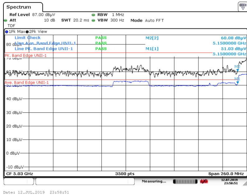
Graph 17: Band Edge Transmitting 5205 MHz at TP15 – Conducted Antenna Port Measurement (J2)
