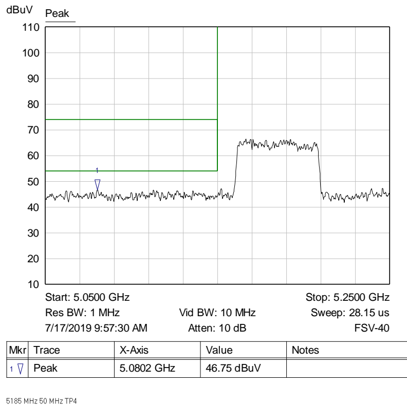
Graph 53: Band Edge Transmitting 5185 MHz at TP4 – Radiated Cabinet Emission Measurement
