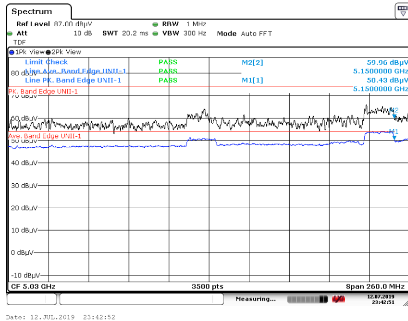
Graph 15: Band Edge Transmitting 5185 MHz at TP10 – Conducted Antenna Port Measurement (J3)
