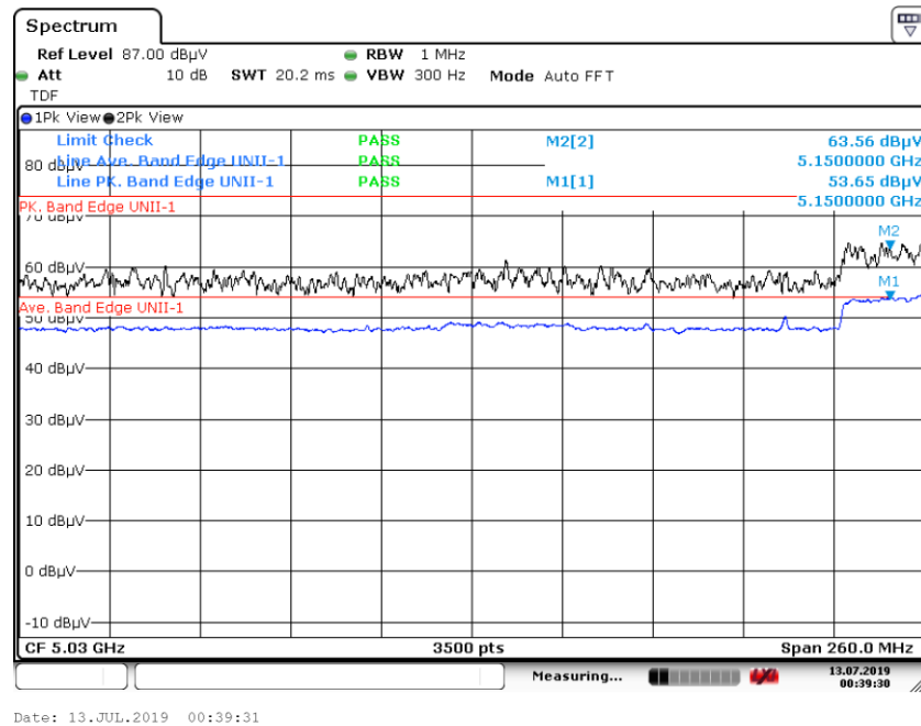
Graph 45: Band Edge Transmitting 5200 MHz at TP8 – Conducted Antenna Port Measurement (J2)
