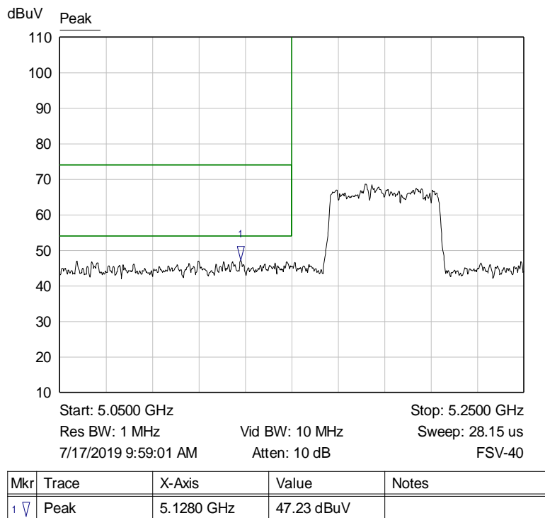
Graph 54: Band Edge Transmitting 5185 MHz at TP4 – Conducted Antenna Port Measurement (J2)
