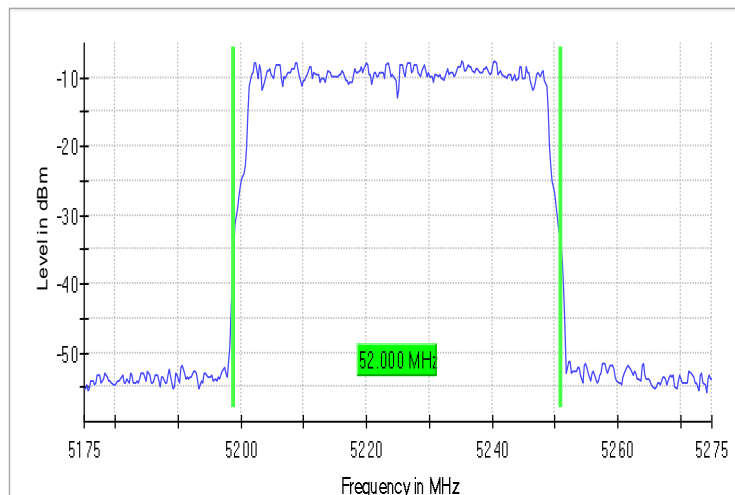
Graph 61: Highest Channel 26 dB Bandwidth
