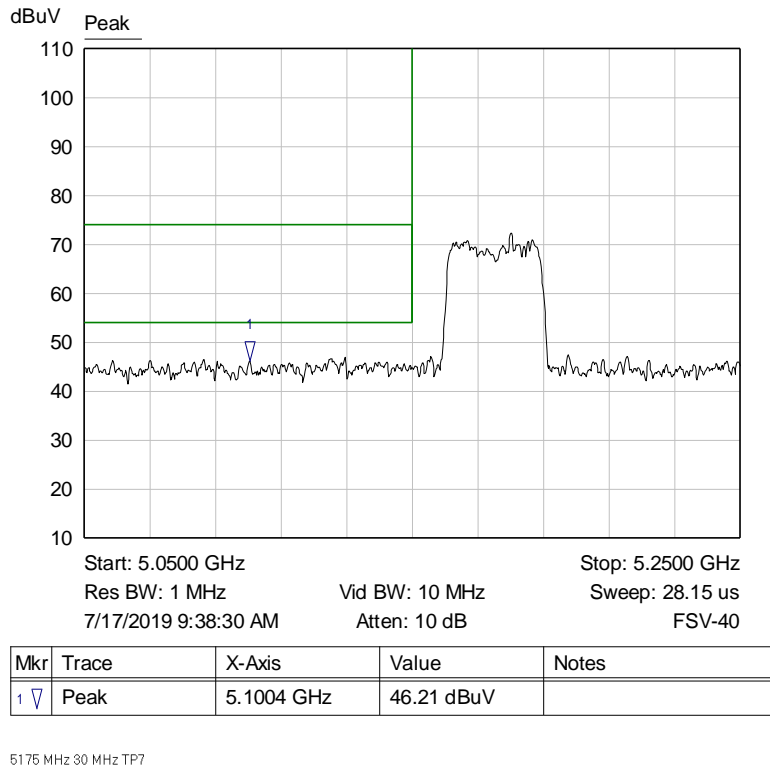
Graph 23: Band Edge Transmitting 5175 MHz at TP7 – Radiated Cabinet Emission Measurement
