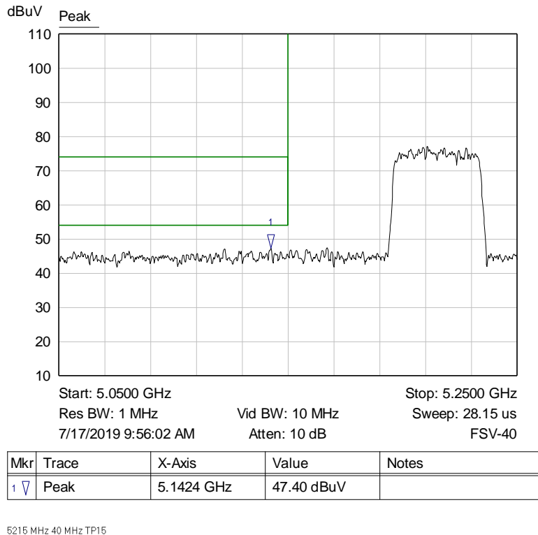
Graph 46: Band Edge Transmitting 5215 MHz at TP15 – Radiated Cabinet Emission Measurement
