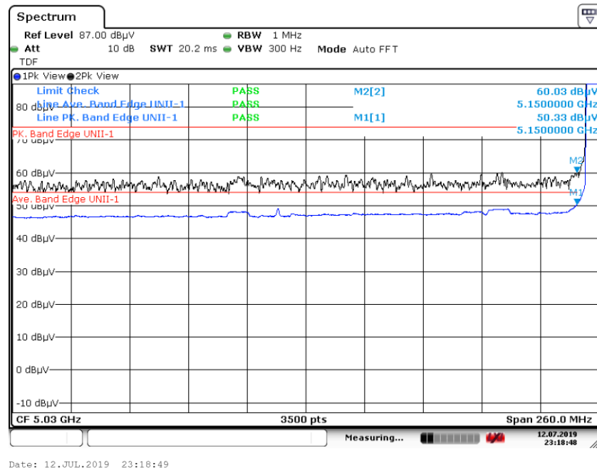
Graph 2: Band Edge Transmitting 5160 MHz at TP2 – Conducted Antenna Port Measurement (J3)
