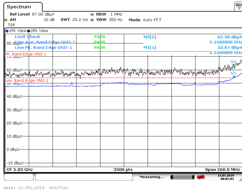
Graph 26: Band Edge Transmitting 5180 MHz at TP11 – Conducted Antenna Port Measurement (J3)
