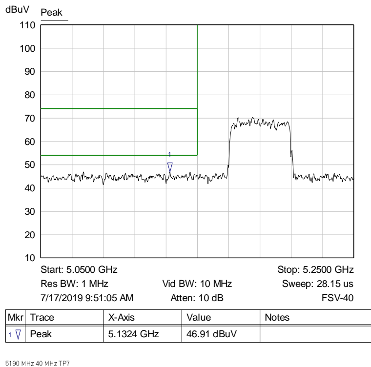
Graph 42: Band Edge Transmitting 5190 MHz at TP7 – Radiated Cabinet Emission Measurement
