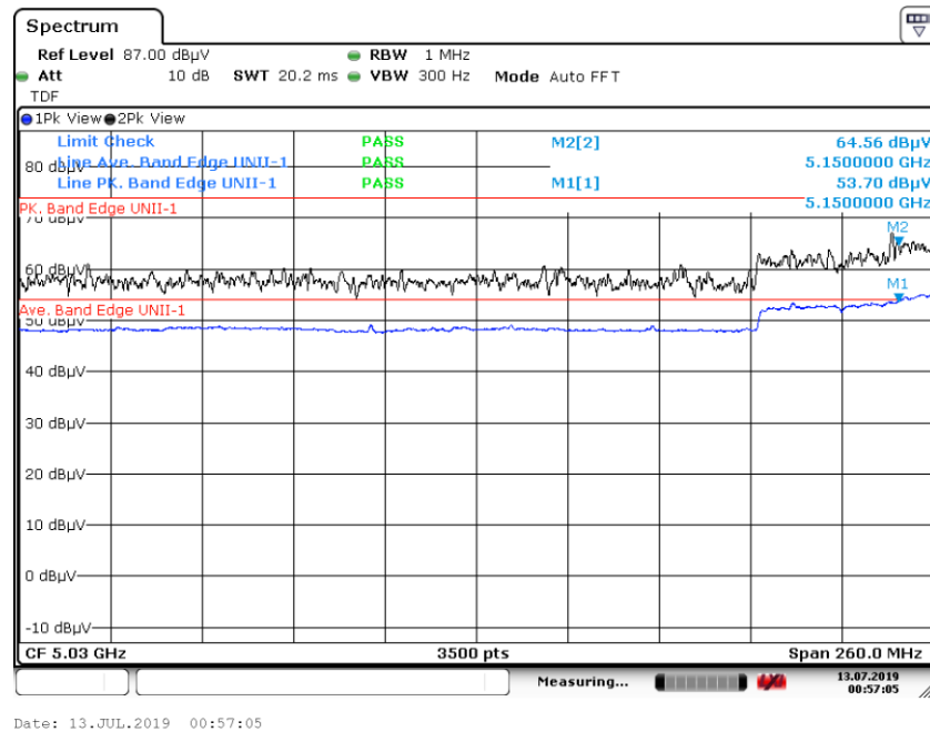
Graph 56: Band Edge Transmitting 5190 MHz at TP6 – Conducted Antenna Port Measurement (J2)
