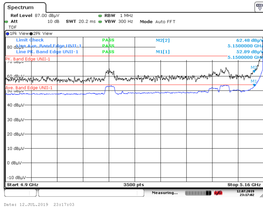
Graph 4: Band Edge Transmitting 5165 MHz at TP12 – Conducted Antenna Port Measurement (J3)
