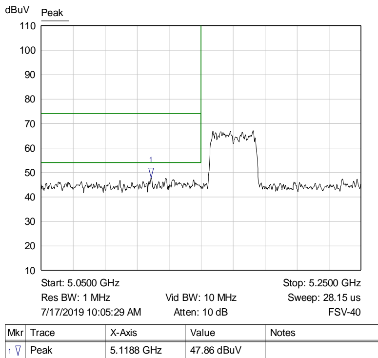
Graph 21: Band Edge Transmitting 5170 MHz at TP2 – Radiated Cabinet Emission Measurement
