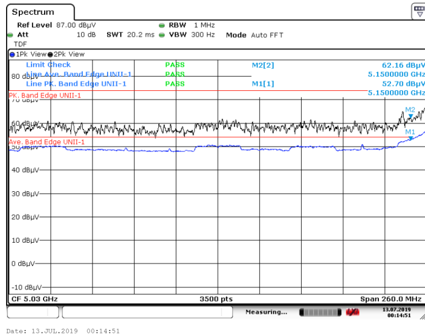
Graph 30: Band Edge Transmitting 5190 MHz at TP13 – Conducted Antenna Port Measurement (J2)
