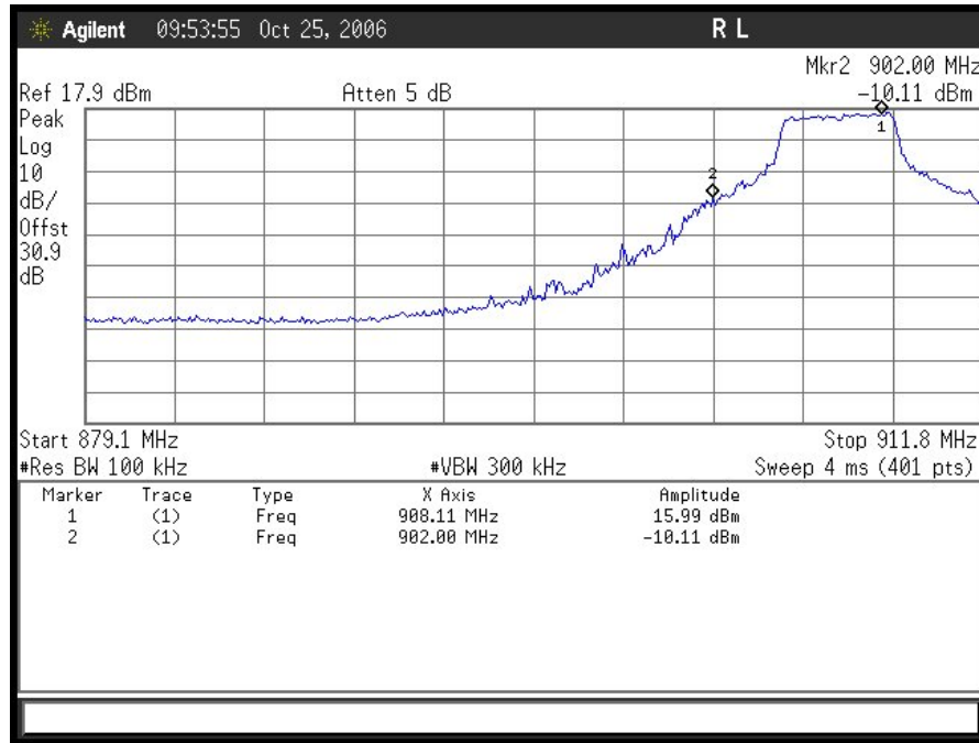
Plot 19. 802.11/b – 907MHz Lower Band Edge (OFDM 5MHz)
