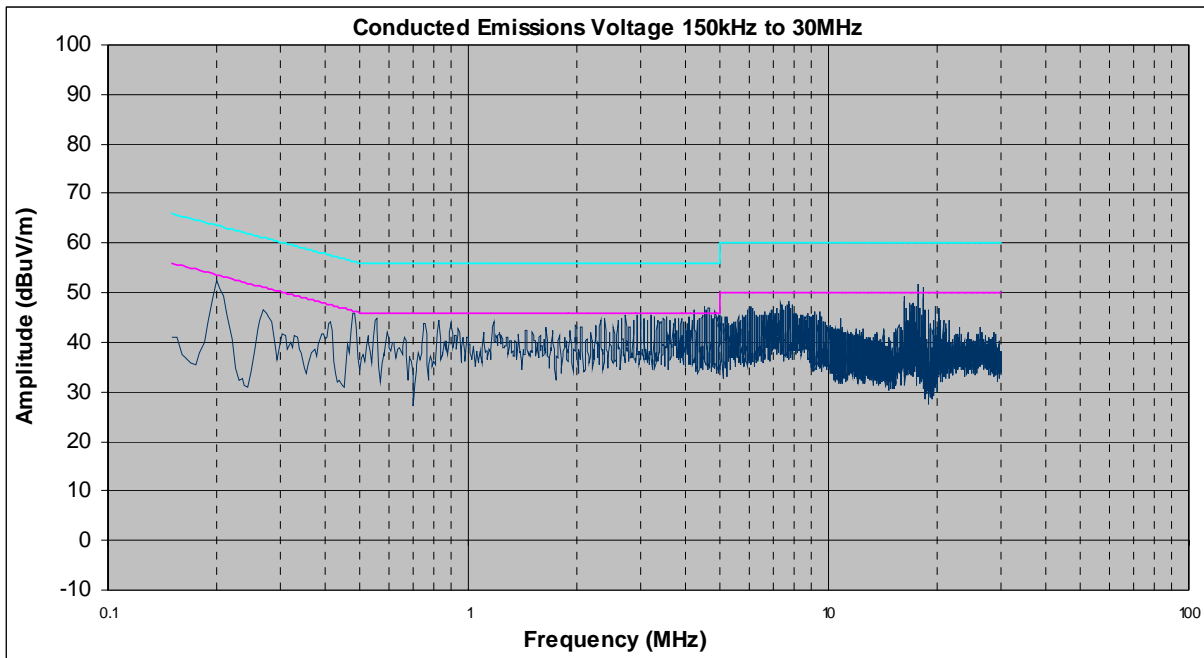
Plot 4. Conducted Emissions, Phase Line Plot
