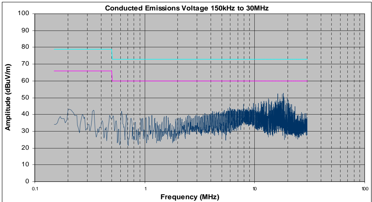
Plot 2. Conducted Emission, Neutral Line Plots
