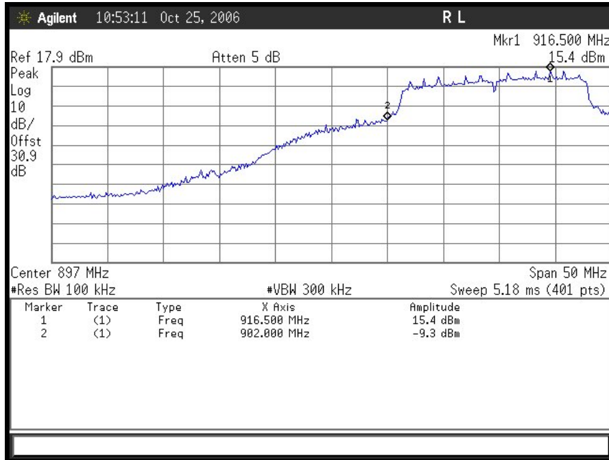
Plot 21. 802.11/b – 912MHz Lower Band Edge (OFDM 20MHz)
