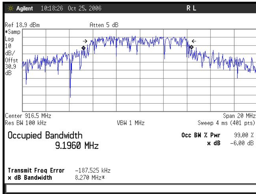
Plot 7. 10MHz Occupied Band Width. (OFDM)
