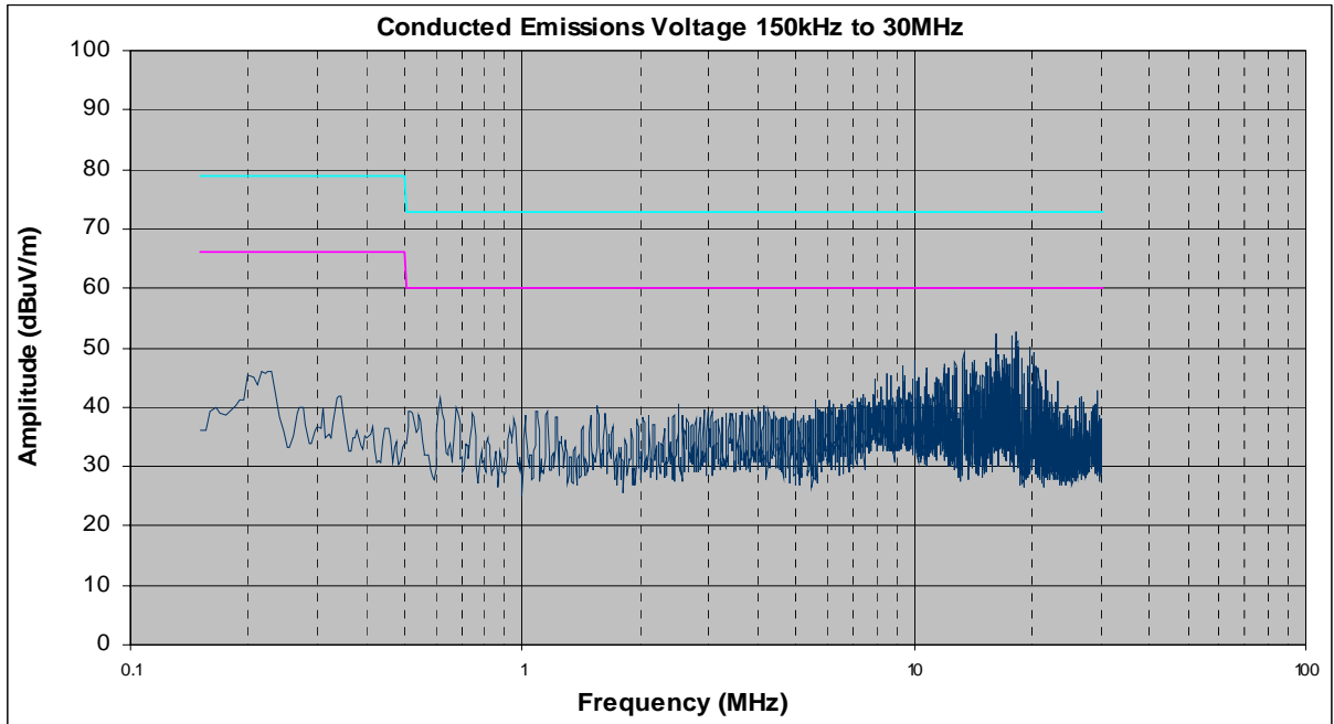
Plot 1. Conducted Emission, Phase Line Plots
