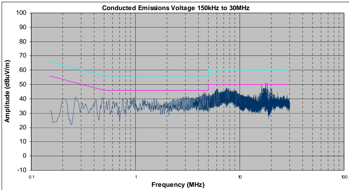
Plot 5. Conducted Emissions, Neutral Line Plot
