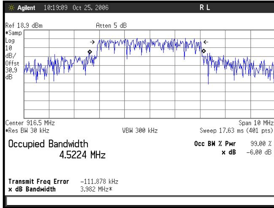
Plot 6. 5MHz Occupied Band Width. (OFDM)
