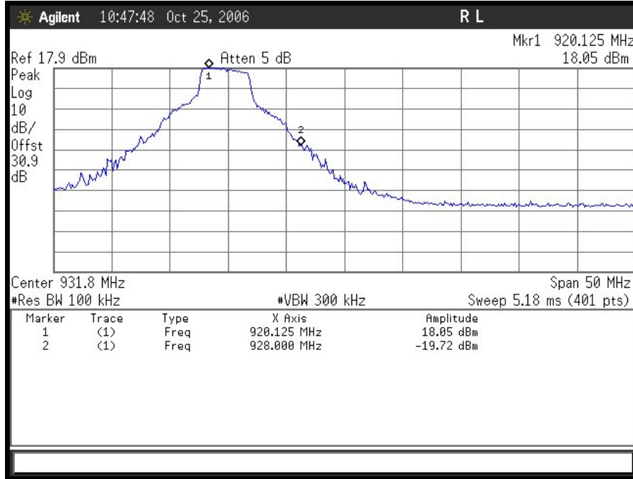
Plot 23. 802.11/b – 922MHz Upper Band Edge (OFDM 5MHz)
