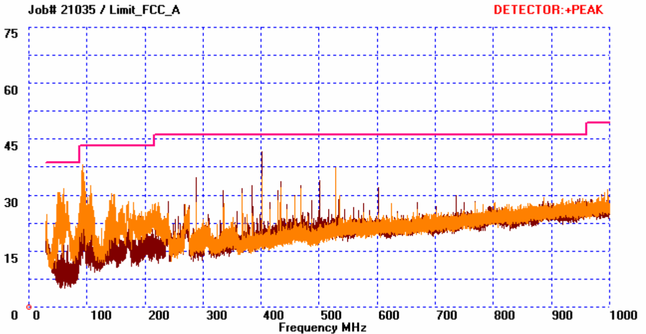
Plot 3. Radiated Emissions Test Plot
