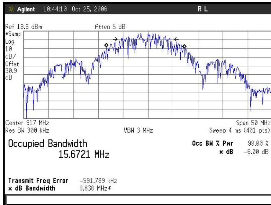
Plot 9. 20MHz Occupied Band Width. (DSSS)
