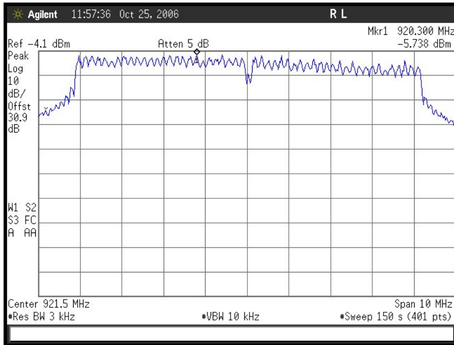
Plot 33. 802.11/g – High Ch Peak Power Spectral Density – OFDM 10MHz
