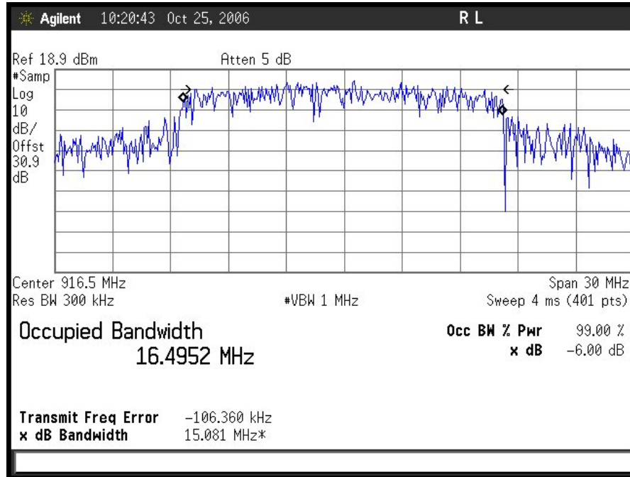
Plot 8. 20MHz Occupied Band Width. (OFDM)
