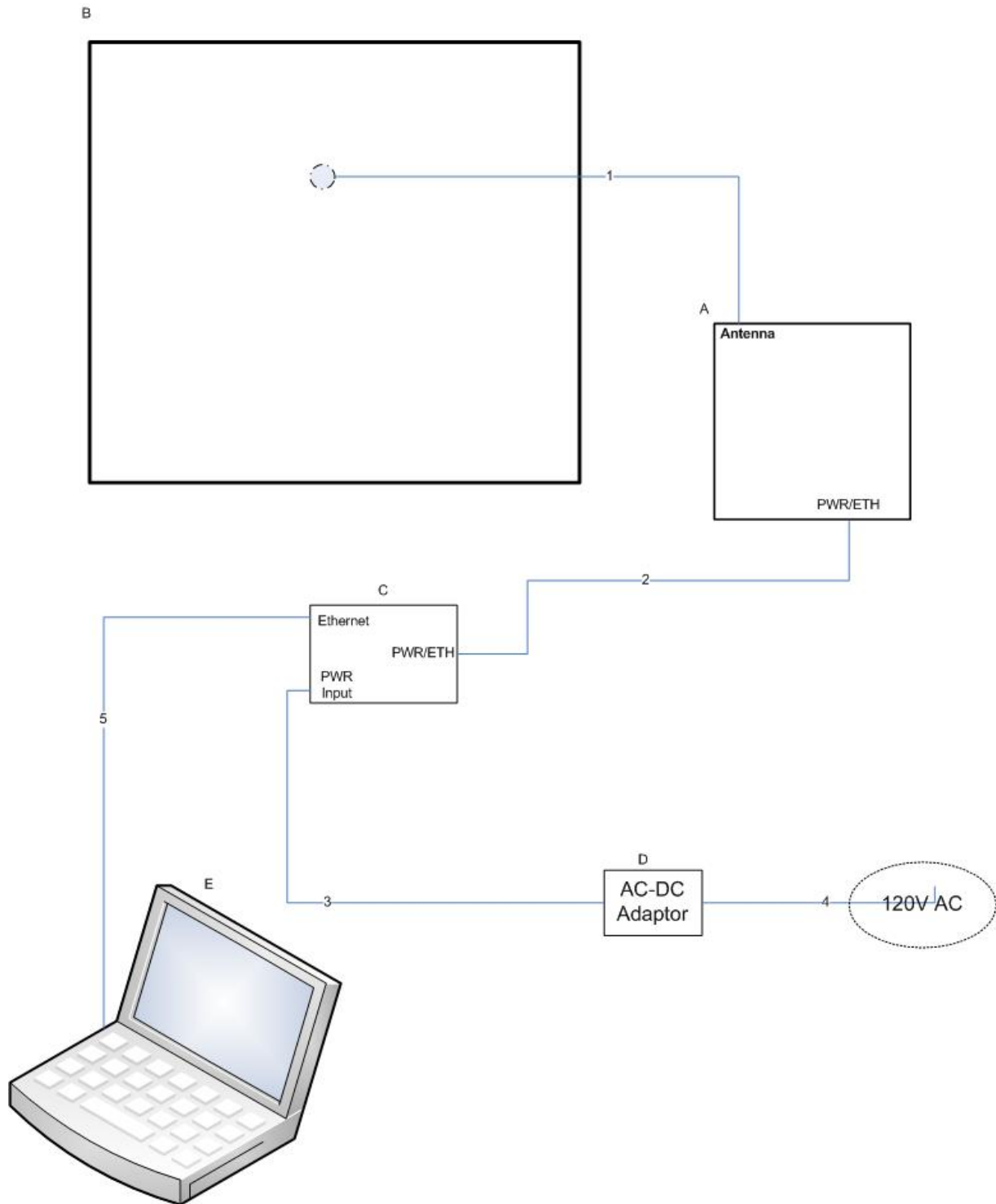
Figure 3. Block Diagram of Test Configuration (Radiated Measurement)
