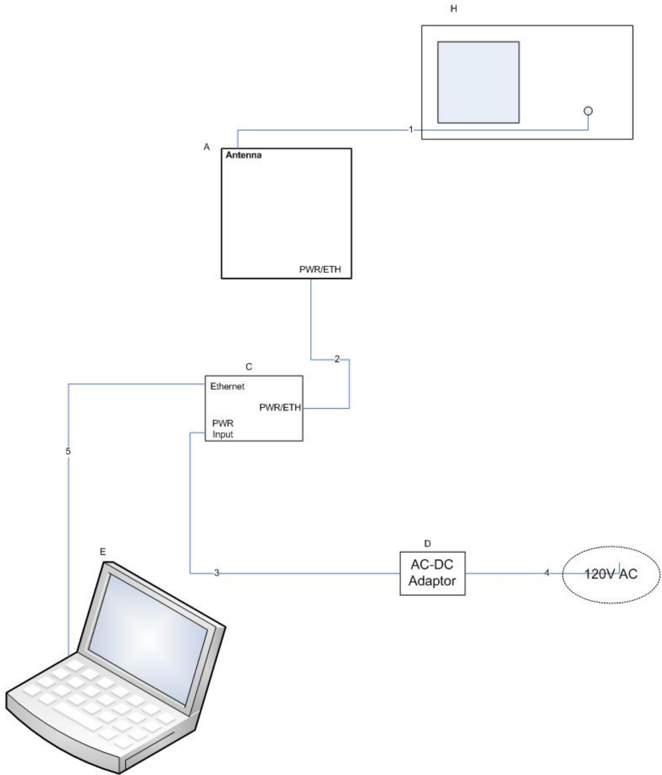
Figure 2. Block Diagram of Test Configuration (Conducted Measurement)
