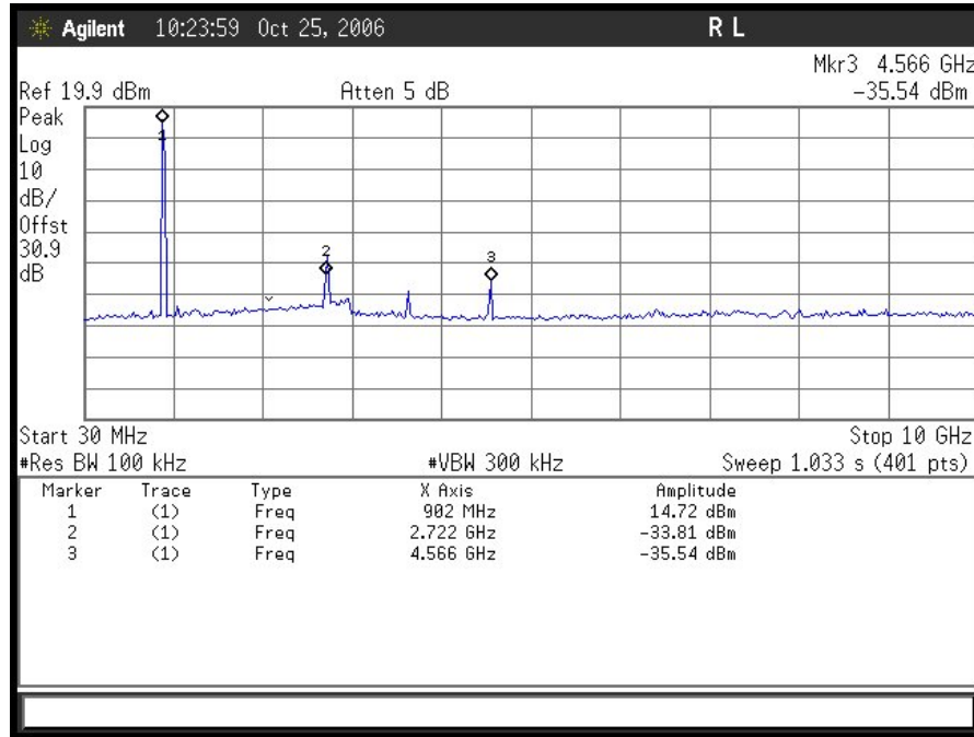
Plot 10. 802.11/b – Low Channel Conducted Emissions 30MHz - 10GHz (OFDM – 5MHz)
