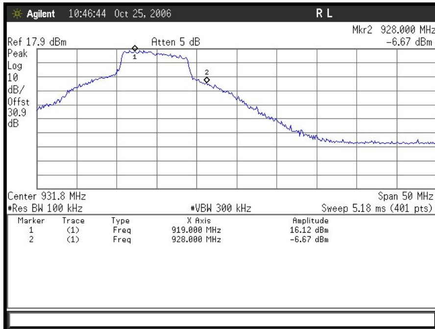
Plot 24. 802.11/b – 922MHz Upper Band Edge (OFDM 10MHz)
