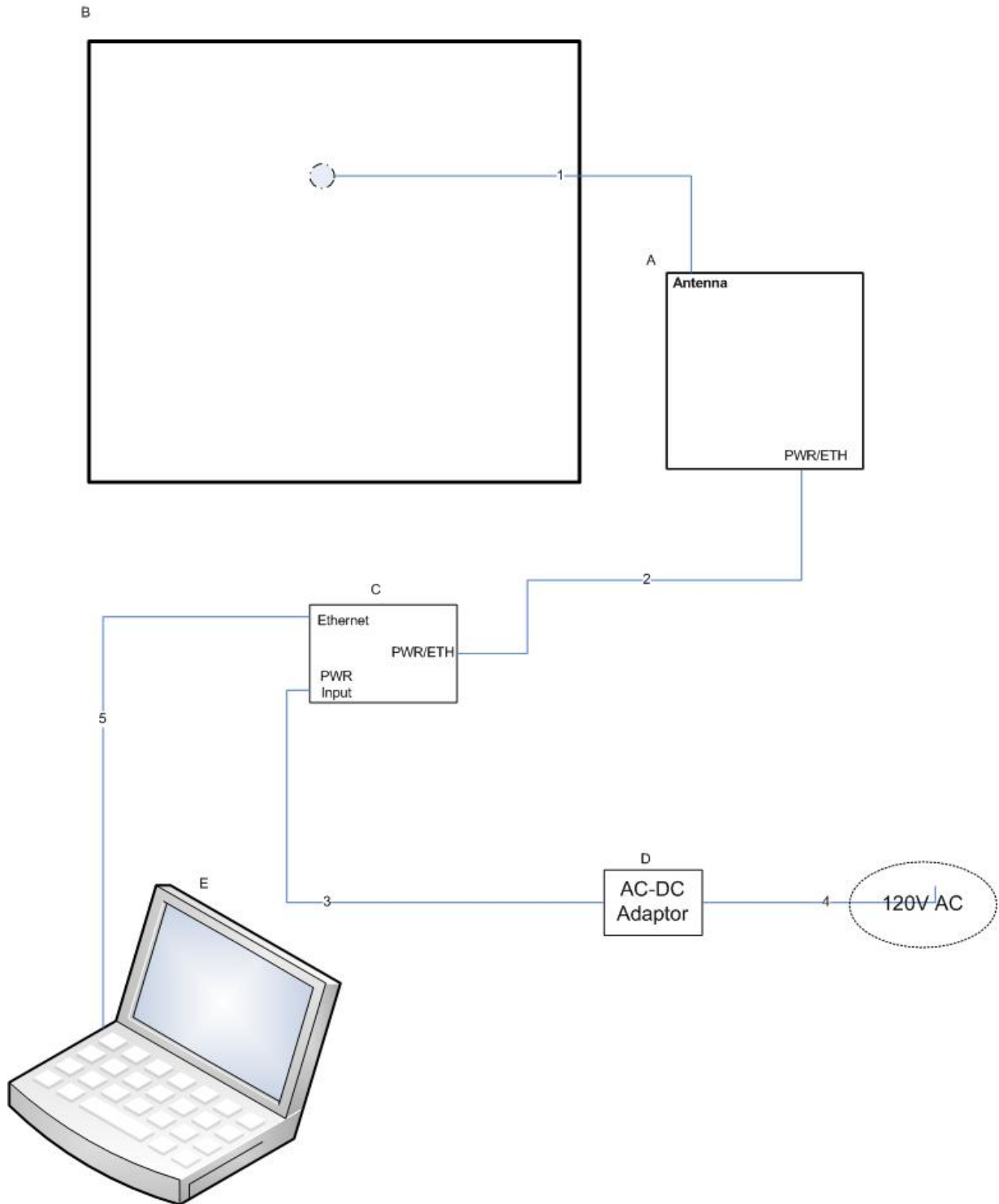
Figure 1. Block Diagram of Test Configuration (Emissions)
