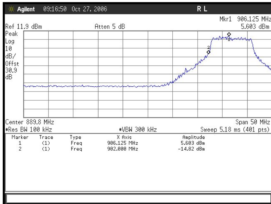
Plot 20. 802.11/b – 907MHz Lower Band Edge (OFDM 10MHz)
