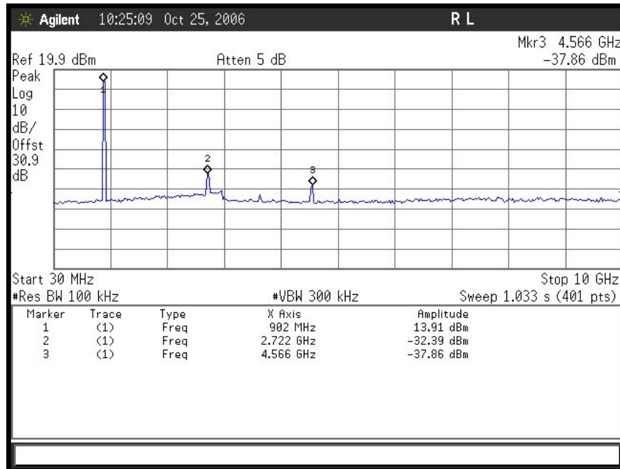
Plot 11. 802.11/b – Low Channel Conducted Emissions 30MHz - 10GHz (OFDM – 10MHz)
