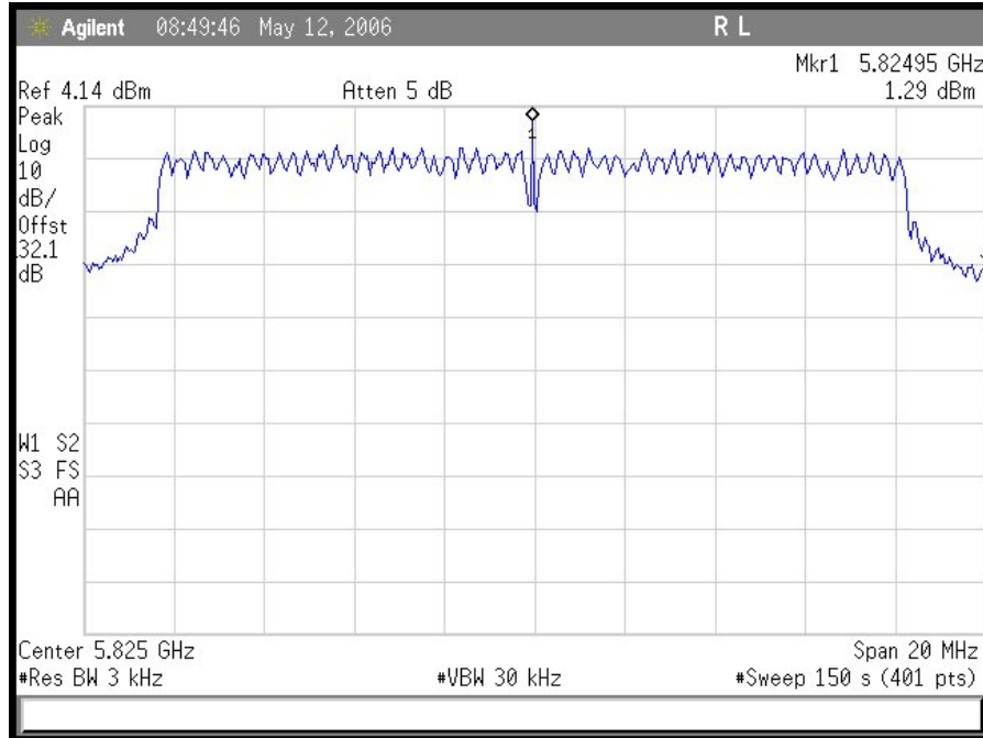
Plot 15. High Ch PPSD
