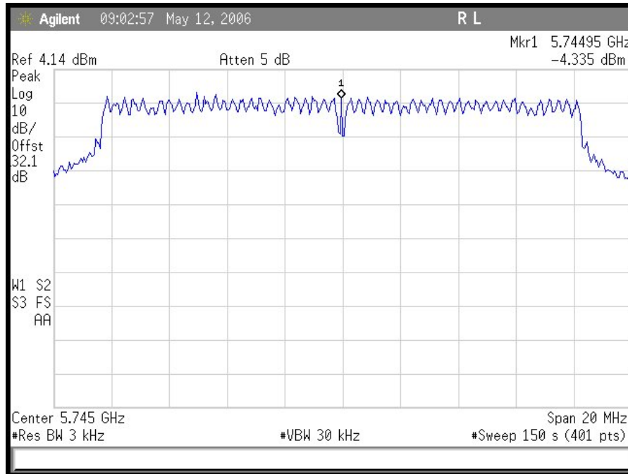
Plot 13. Low Ch PPSD
