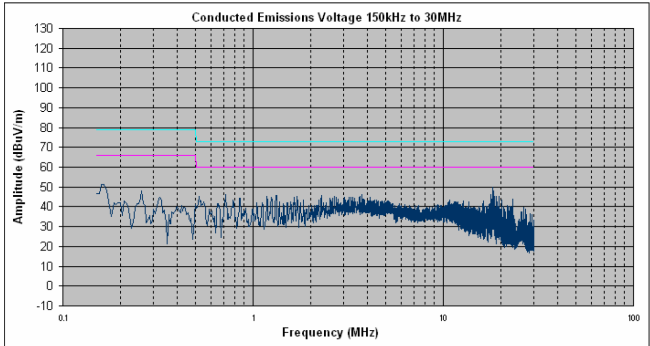
Conducted Emission Limits, Neutral Line Plots
