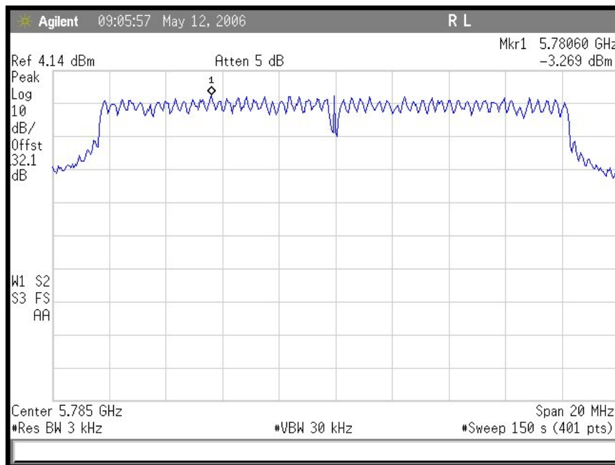
Plot 14. Mid Ch PPSD
