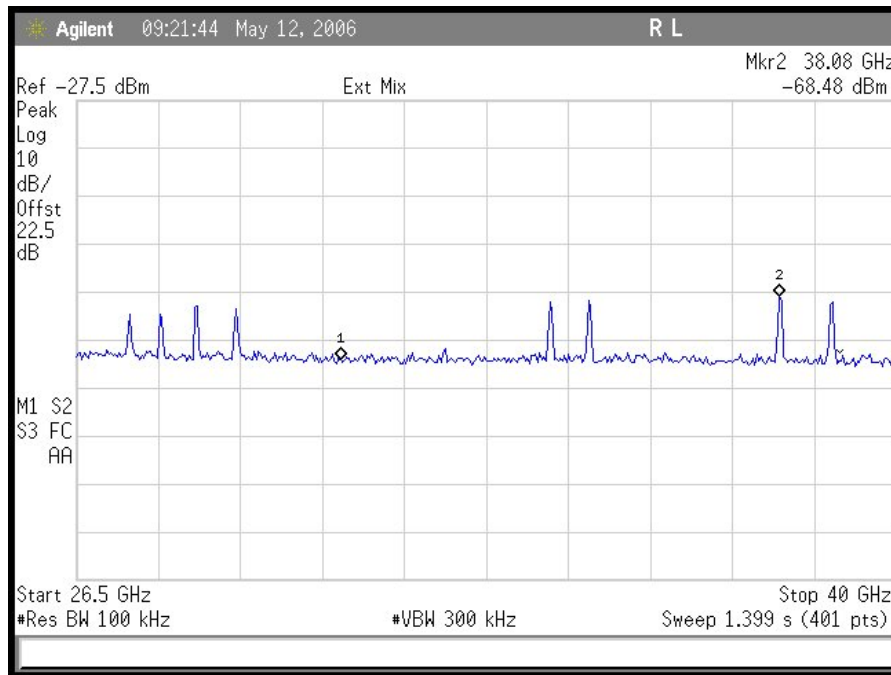
Plot 12. Hi Channel Conducted Emissions 26.5 – 40 GHz
