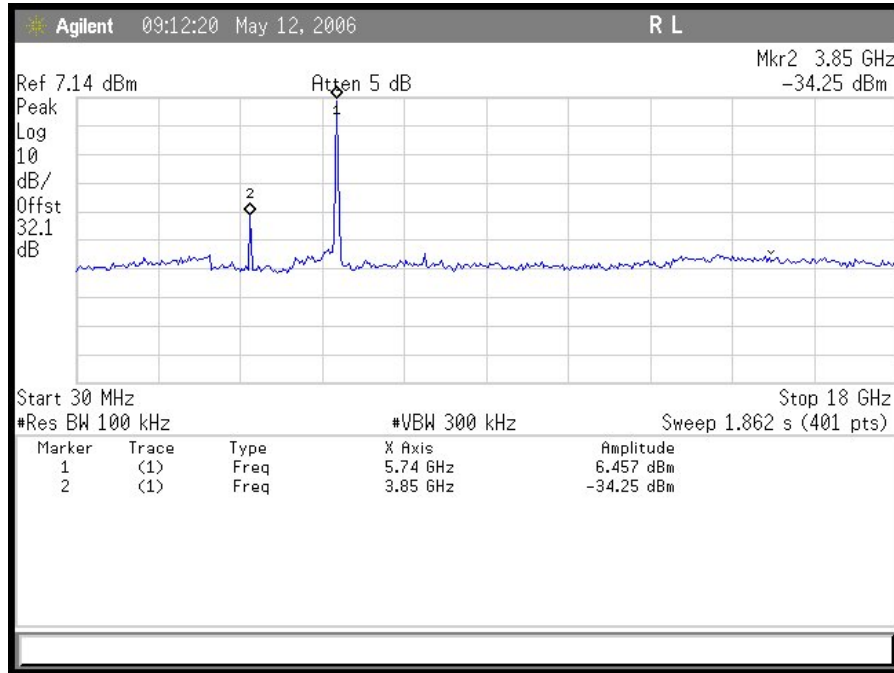
Plot 4. Low Channel Conducted Emissions 30 MHz- 18GHz
