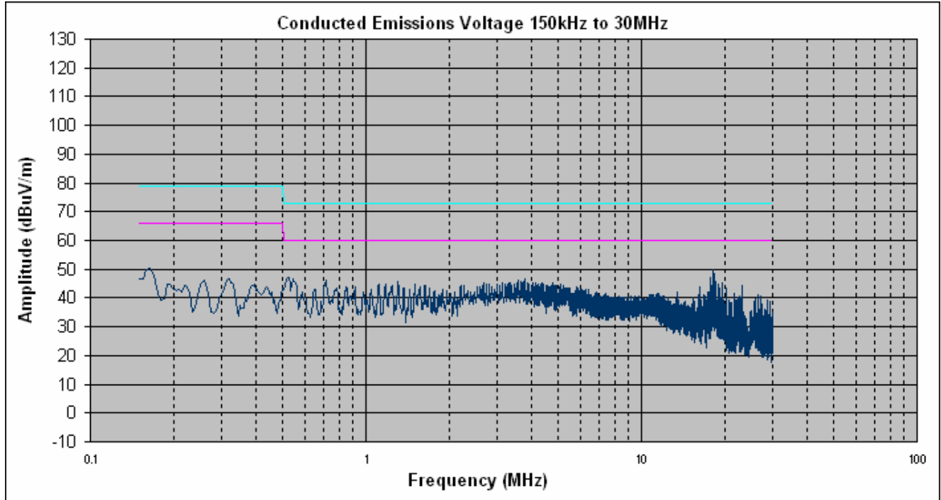
Conducted Emission Limits, Phase Line Plots
