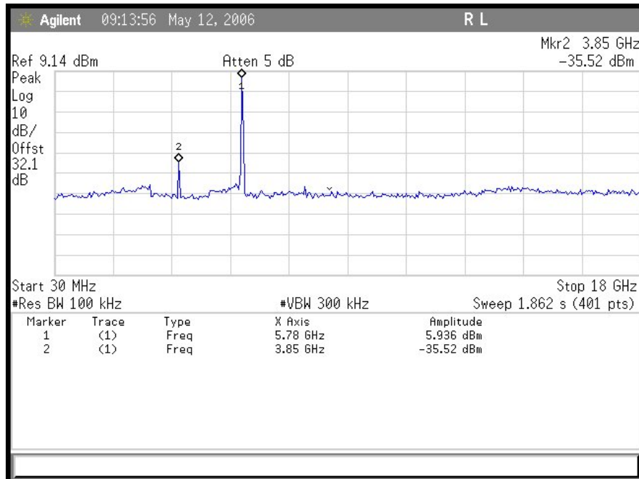
Plot 7. Mid Channel Conducted Emissions 30 MHz- 18GHz
