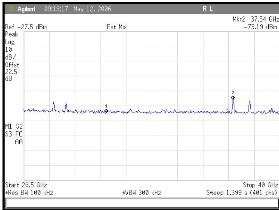
Plot 6. Low Channel Conducted Emissions 26.5 – 40 GHz
