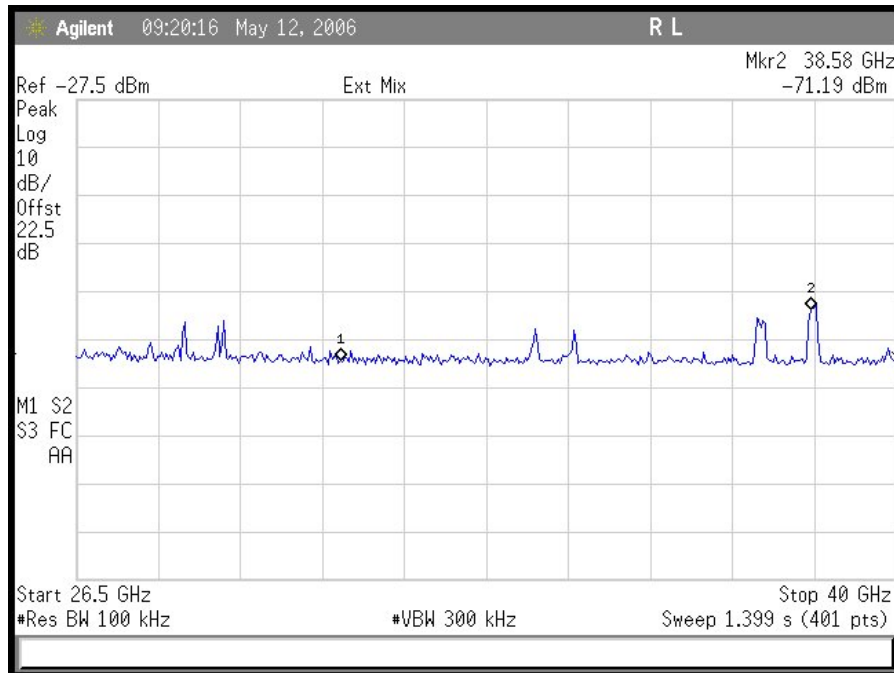
Plot 9. Mid Channel Conducted Emissions 26.5 – 40 GHz
