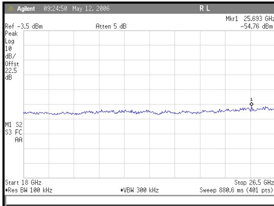
Plot 11. Hi Channel Conducted Emissions 18 – 26.5 GHz
