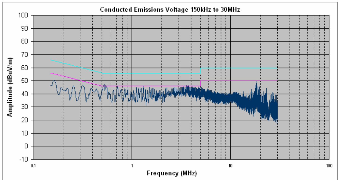
Conducted Emissions Test Results, Phase Line
