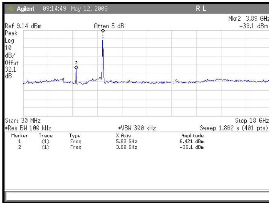
Plot 10. Hi Channel Conducted Emissions 30 MHz- 18GHz
