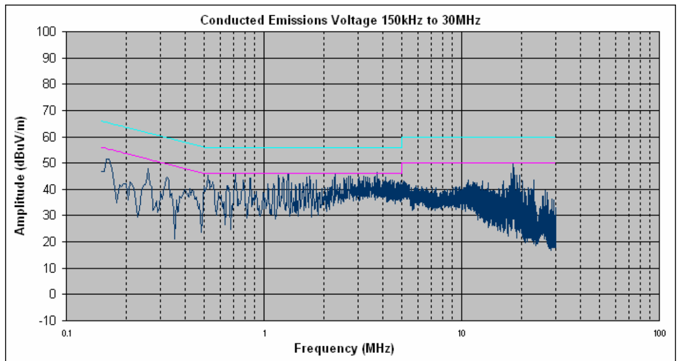
Conducted Emissions Test Results, Neutral Line
