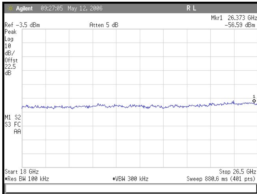
Plot 5. Low Channel Conducted Emissions 18 – 26.5 GHz
