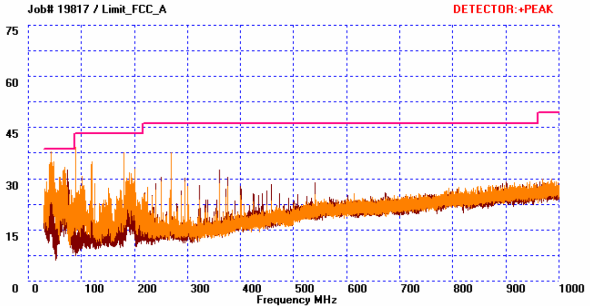
Radiated Emissions Limits, Test Results, 30 MHz to 1 GHz
