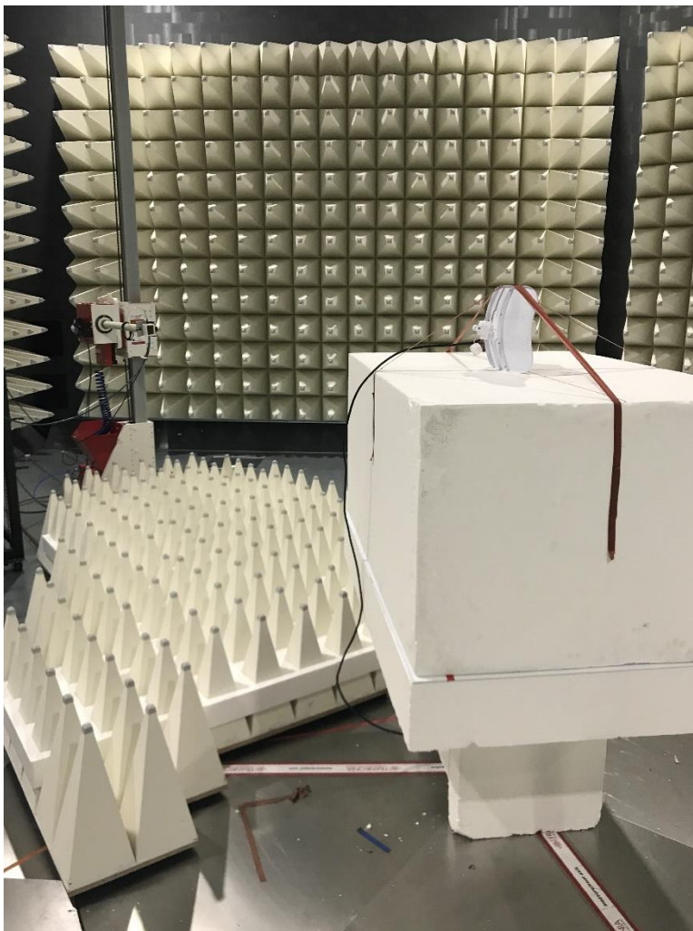
Photograph 3: View Test Set Up Radiated Emissions 17 – 40 GHz
