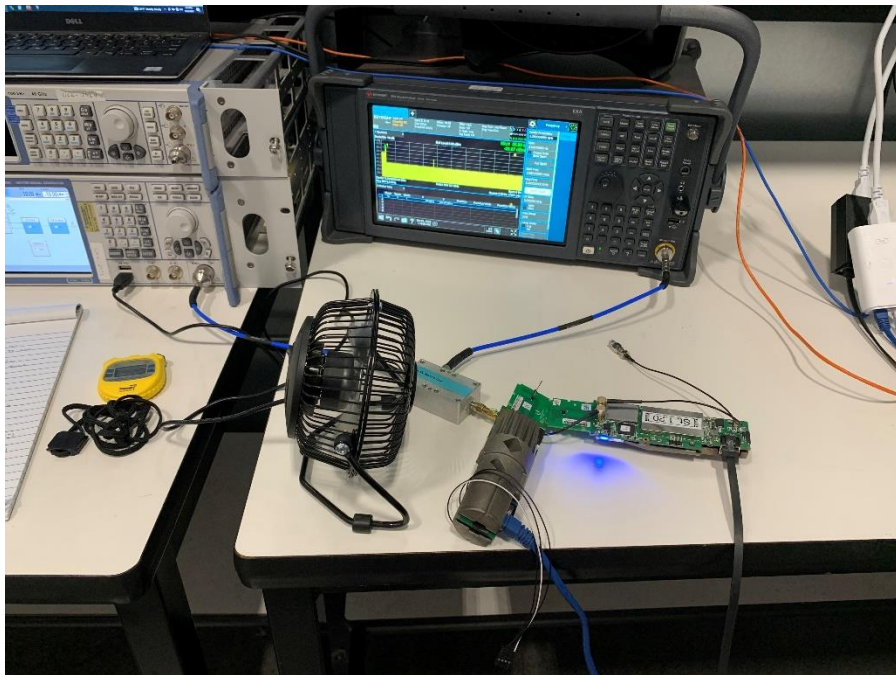
Photograph 5: DFS Test Setup
