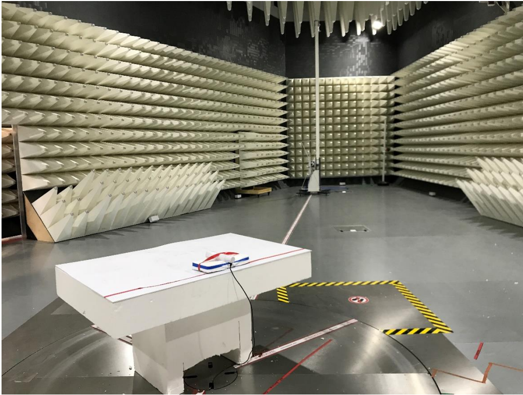
Photograph 1: View Test Set Up Radiated Emissions 30 – 1000 MHz
