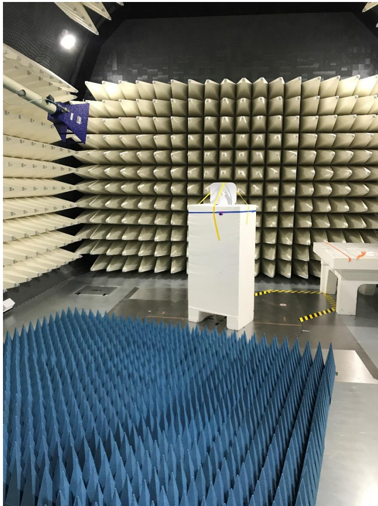
Photograph 2: View Test Set Up Radiated Emissions 1 – 17 GHz
