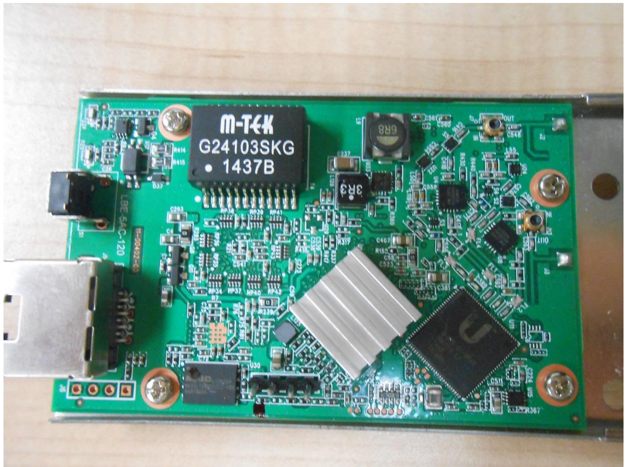
Internal Photos SWX-LBE5AC120-U
