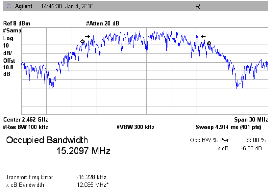
Plot 10. Occupied Band Width, 802.11b Mode, High Channel, FCC, 6 dB
