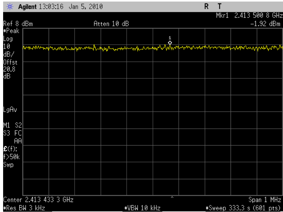
Plot 64. Power Spectral Density 2412MHz Low Channel 802.11b
