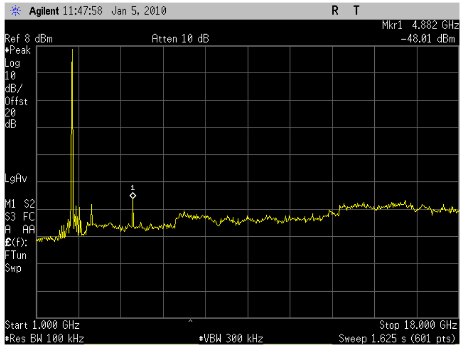
Plot 46. Conducted Spurious 2437MHz Mid Channel 802.11b (1-18GHz)
