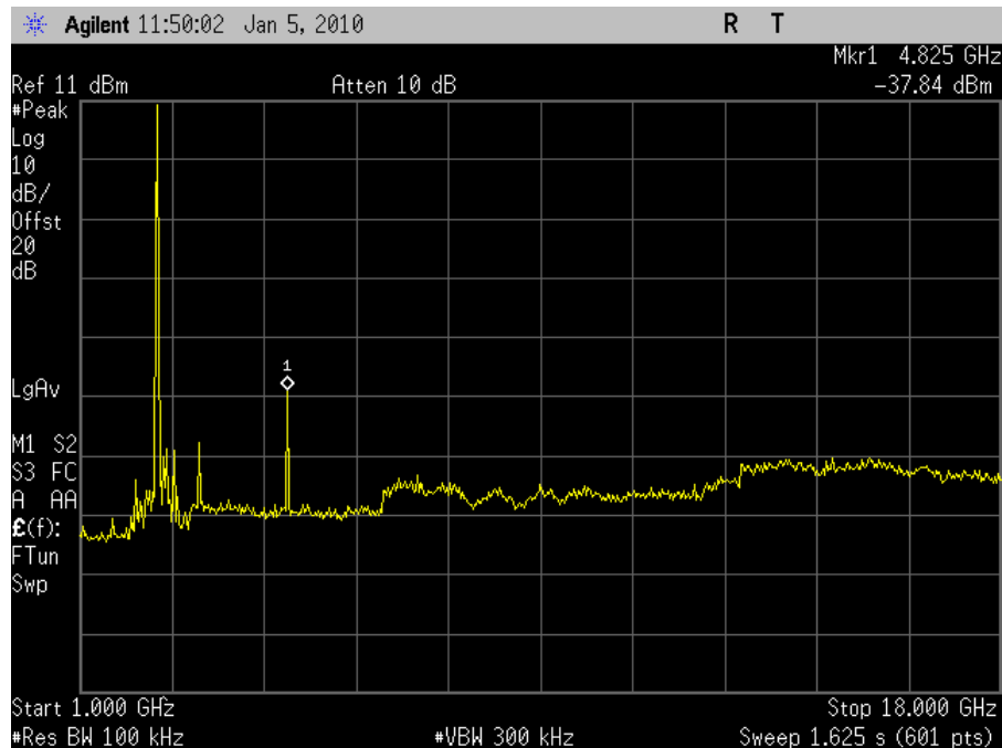
Plot 43. Conducted Spurious 2412MHz Low Channel 802.11b (1-18GHz)
