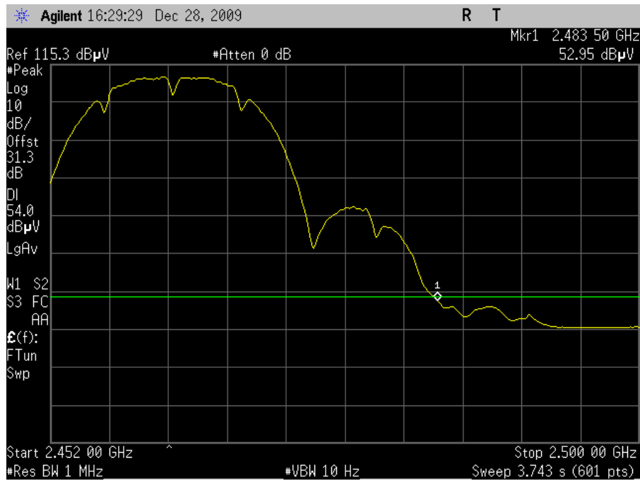
Plot 34. Restricted Band, 802.11b, Channel 11 (2462MHz), 8dBi Integrated Antenna, Average
