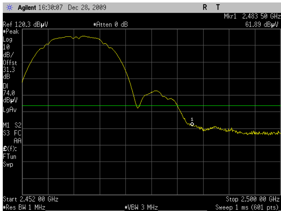
Plot 35. Restricted Band, 802.11b, Channel 11 (2462MHz), 8dBi Integrated Antenna, Peak
