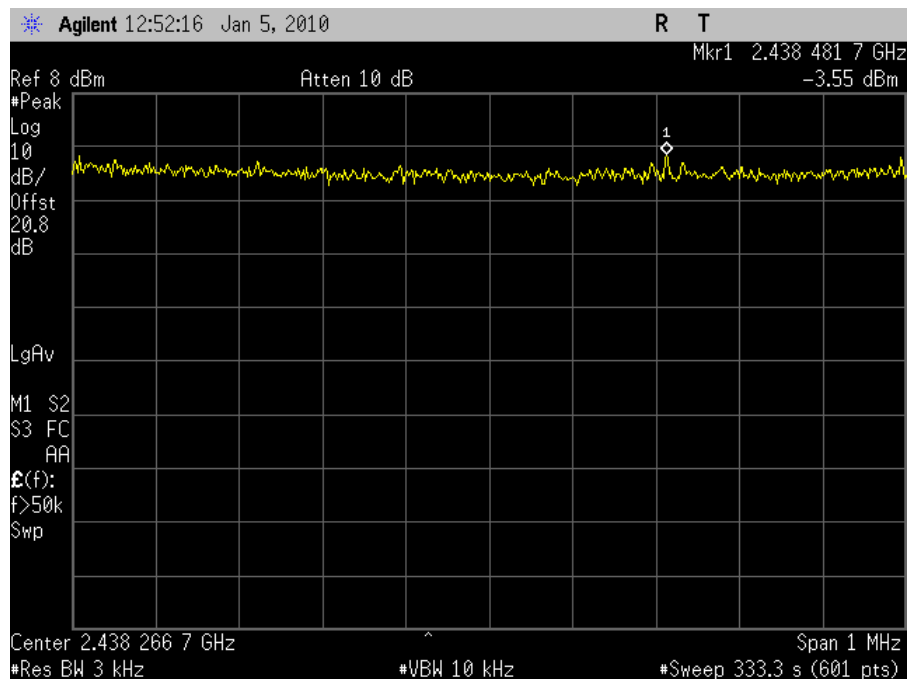
Plot 65. Power Spectral Density 2437MHz Mid Channel 802.11b
