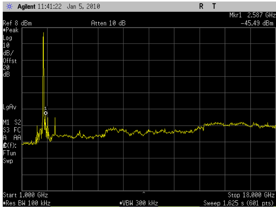
Plot 55. Conducted Spurious 2437MHz Mid Channel 802.11g (1-18GHz)
