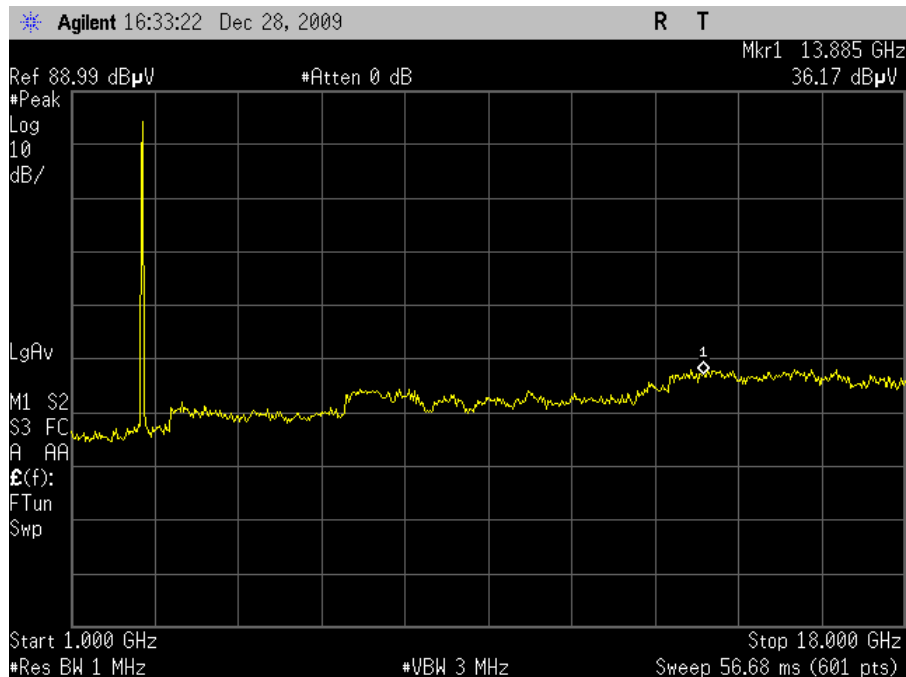
Plot 27. Radiated Spurious Emissions, 802.11b Mode Mid Channel
