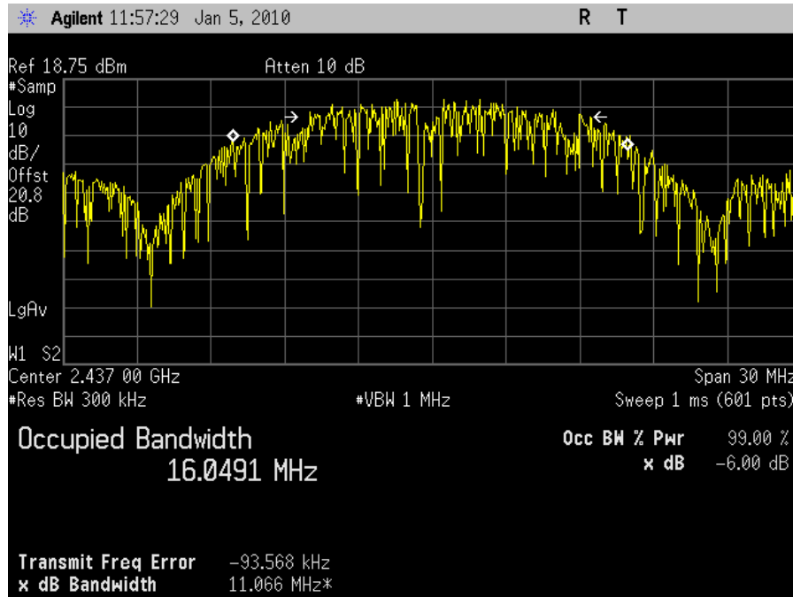
Plot 12. Occupied Band Width, 802.11b Mode, Mid Channel, 99% OBW
