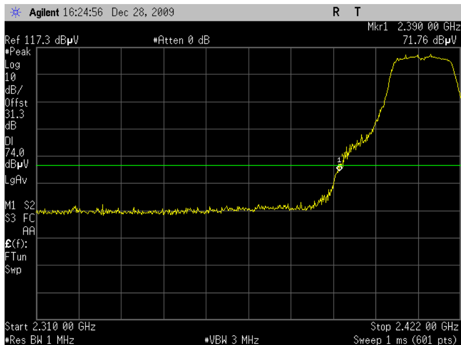
Plot 37. Restricted Band, 802.11g, Channel 1 (2412MHz), 8dBi Integrated Antenna, Peak
