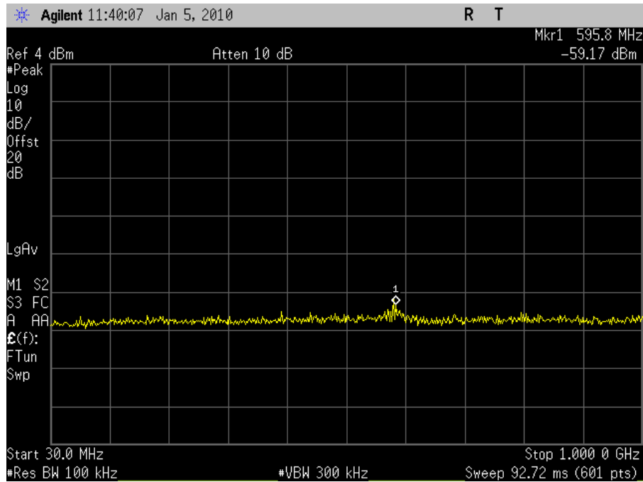
Plot 51. Conducted Spurious 2412MHz Low Channel 802.11g (30MHz-1GHz)
