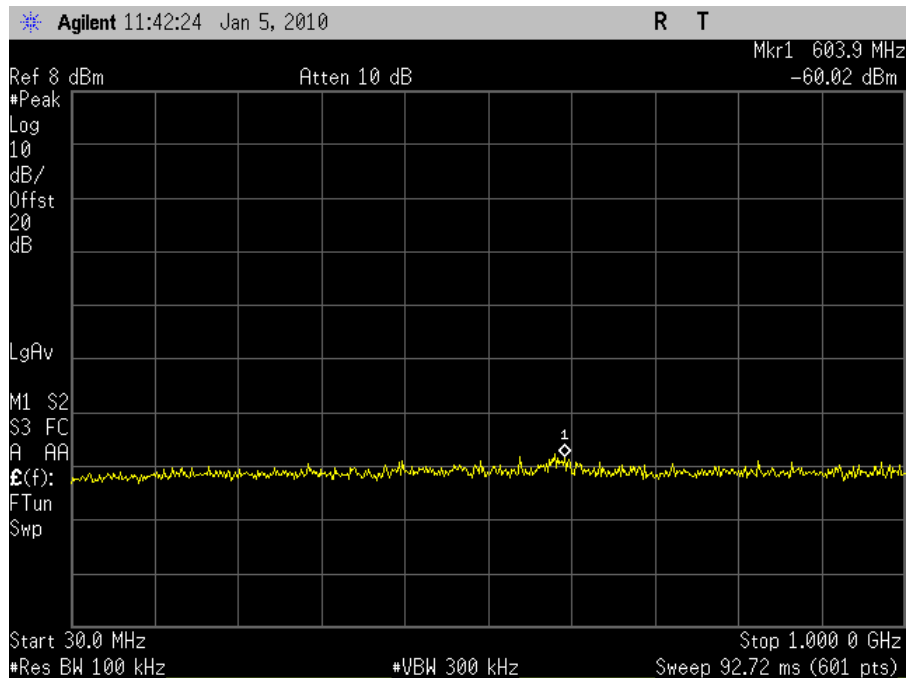
Plot 54. Conducted Spurious 2437MHz Mid Channel 802.11g (30MHz-1GHz)
