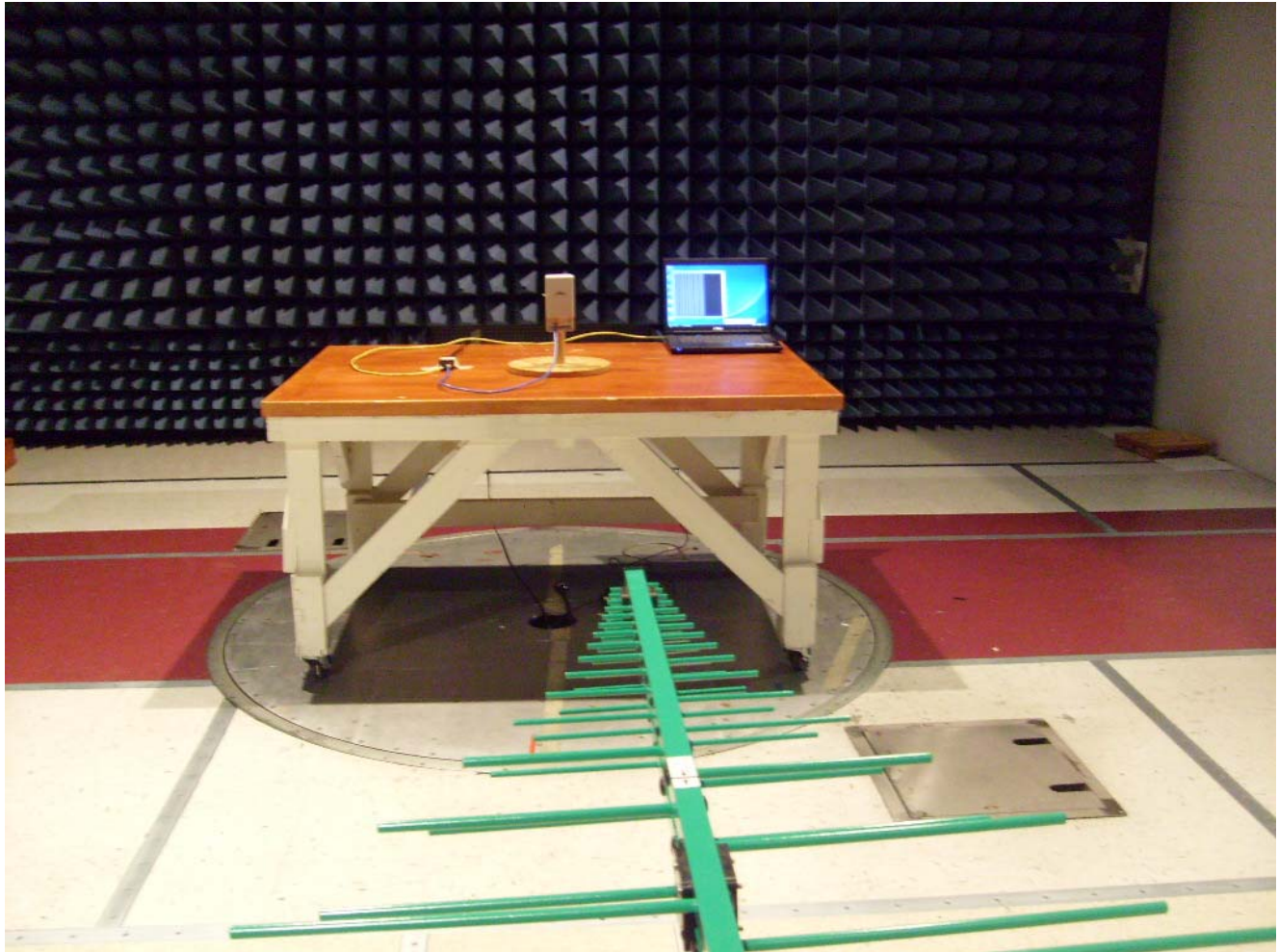
Photograph 2. Radiated Emission, 30MHz – 1GHz Test Setup
