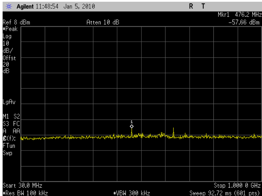
Plot 45. Conducted Spurious 2437MHz Mid Channel 802.11b (30MHz-1GHz)
