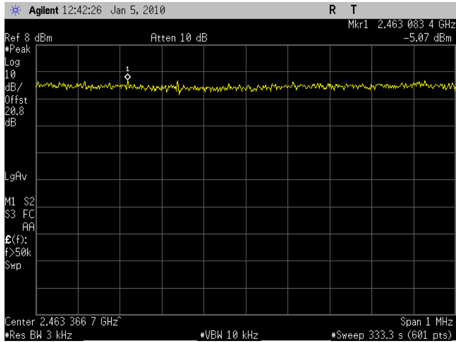
Plot 66. Power Spectral Density 2462MHz High Channel 802.11b
