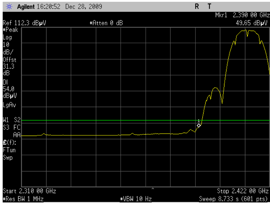
Plot 32. Restricted Band, 802.11b, Channel 1 (2412MHz), 8dBi Integrated Antenna, Average
