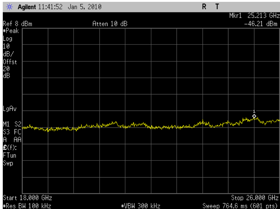
Plot 56. Conducted Spurious 2437MHz Mid Channel 802.11g (18-26GHz)
