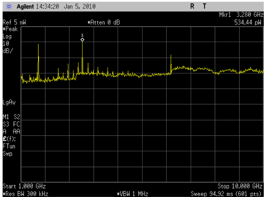
Plot 41. Conducted Receiver Spurious Emission, 1 GHz – 10 GHz
