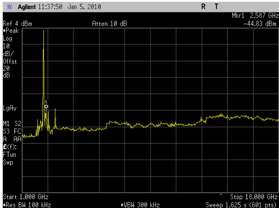
Plot 52. Conducted Spurious 2412MHz Low Channel 802.11g (1-18GHz)
