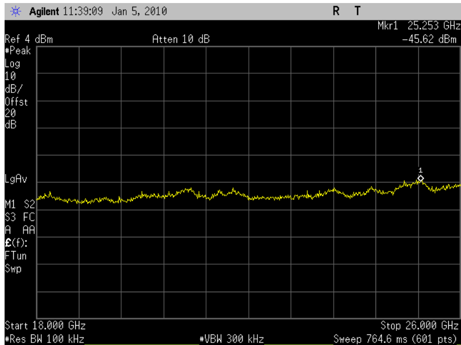
Plot 53. Conducted Spurious 2412MHz Low Channel 802.11g (18-26GHz)
