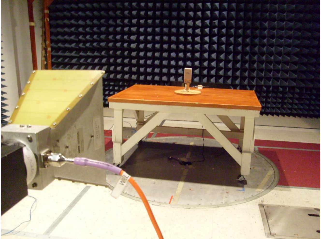
Photograph 5. Radiated Spurious Emission, Test Setup
