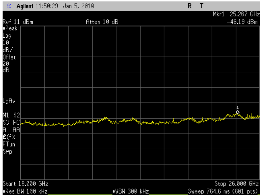
Plot 44. Conducted Spurious 2412MHz Low Channel 802.11b (18-26GHz)
