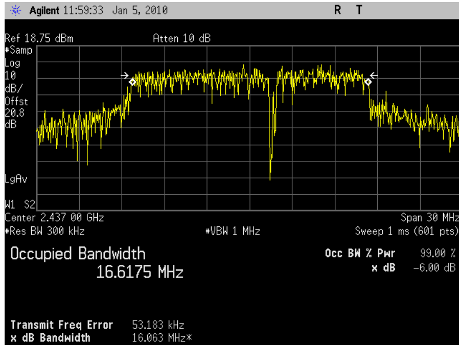
Plot 18. Occupied Band Width, 802.11g Mode, Mid Channel, 99% OBW
