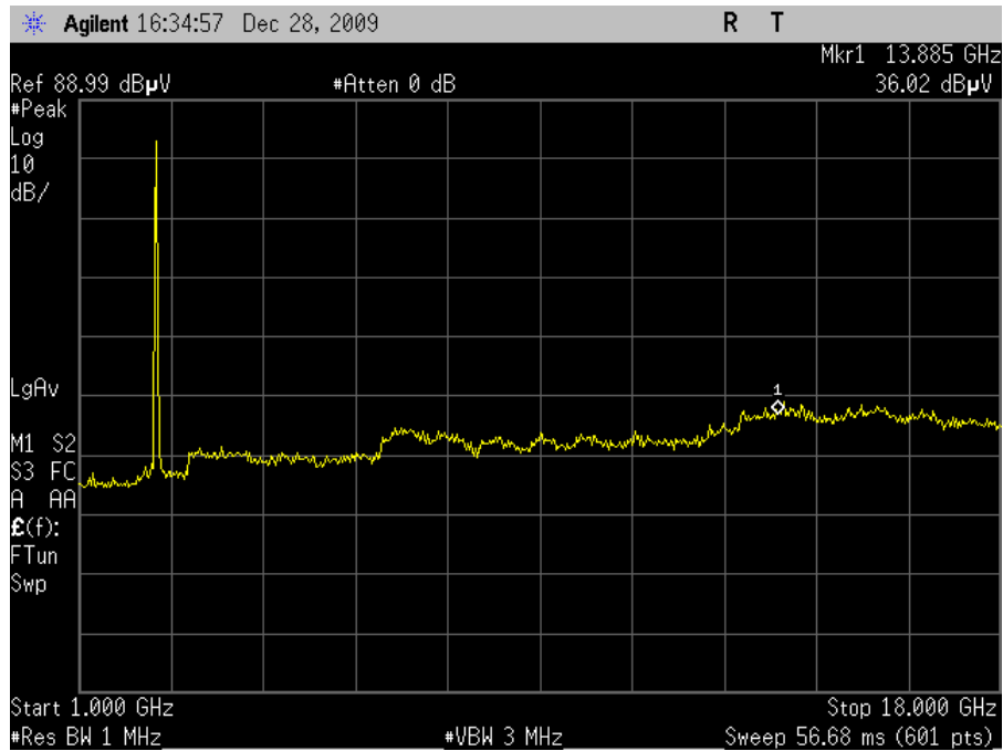
Plot 29. Radiated Spurious Emissions, 802.11g Mode Low Channel
