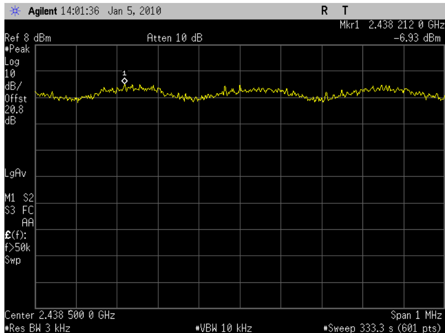
Plot 68. Power Spectral Density 2437MHz Mid Channel 802.11g
