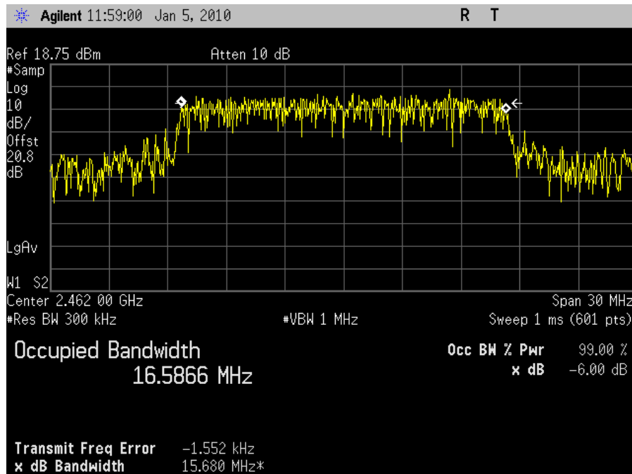
Plot 19. Occupied Band Width, 802.11g Mode, High Channel, 99 % OBW
