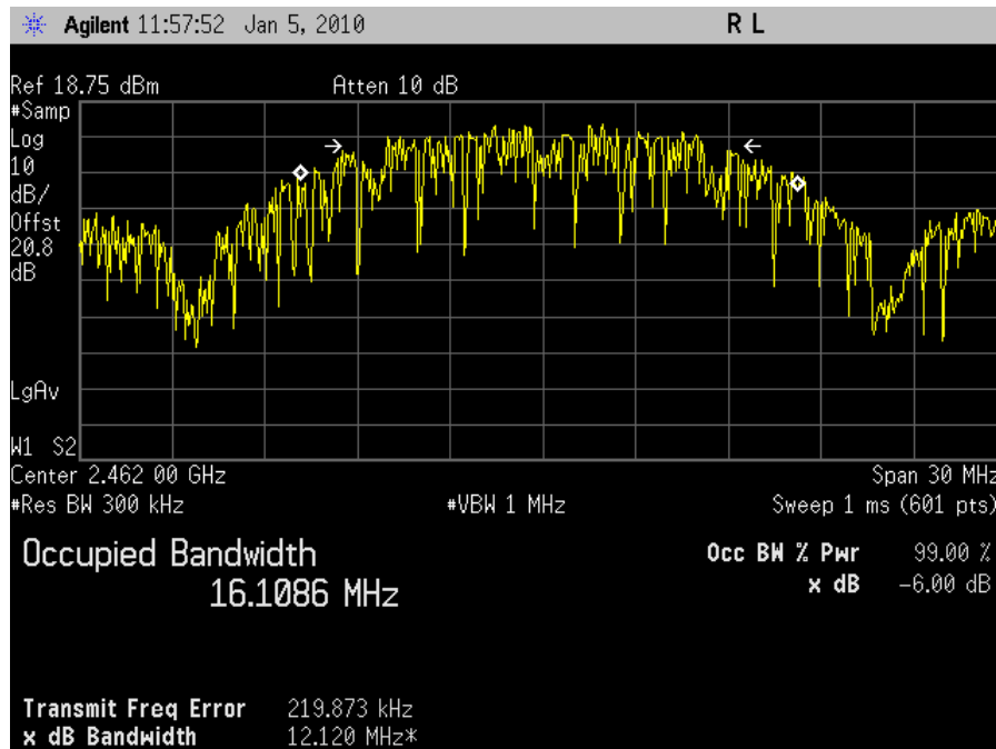
Plot 13. Occupied Band Width, 802.11b Mode, High Channel, 99 % OBW
