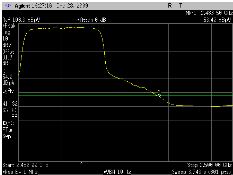
Plot 38. Restricted Band, 802.11g, Channel 11 (2462MHz), 8dBi Integrated Antenna, Average
