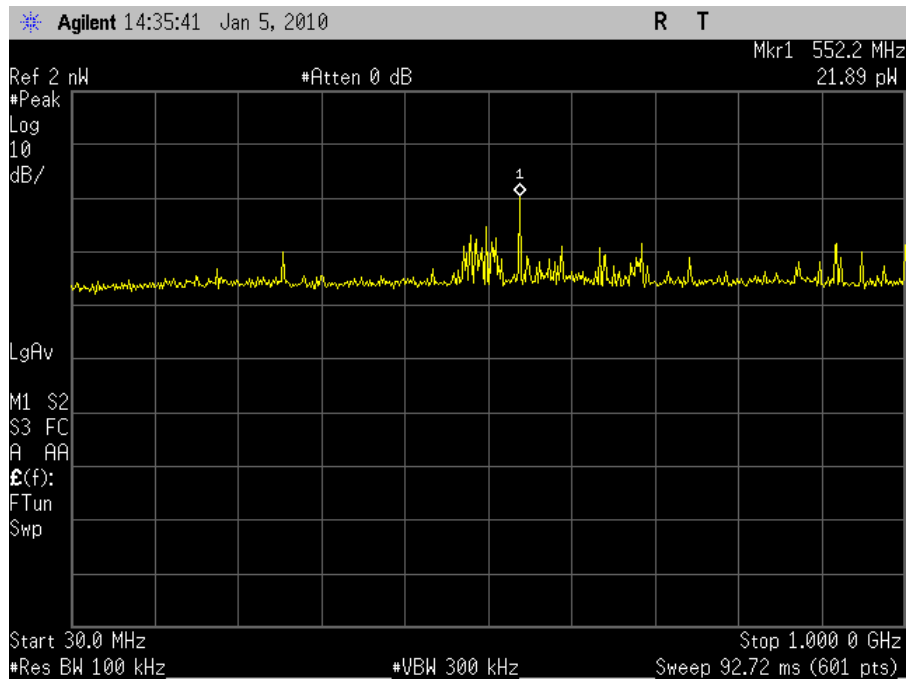
Plot 40. Conducted Receiver Spurious Emission, 30MHz – 1GHz
