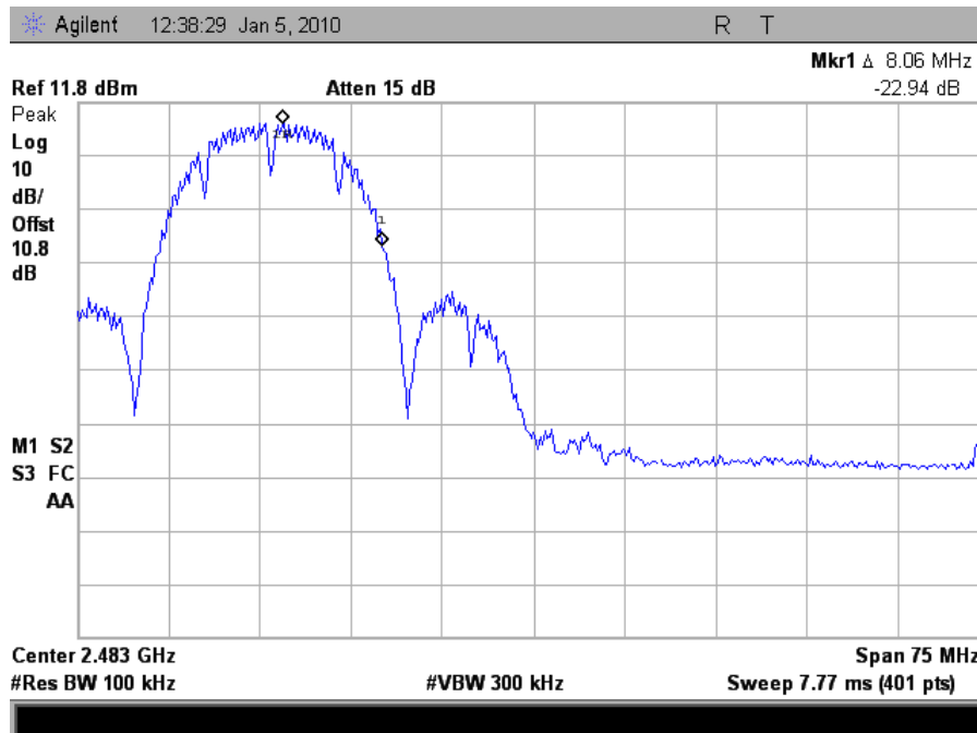
Plot 61. Conducted Band Edge, 802.11b Mode, High
