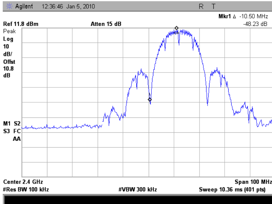
Plot 60. Conducted Band Edge, 802.11b Mode, Low
