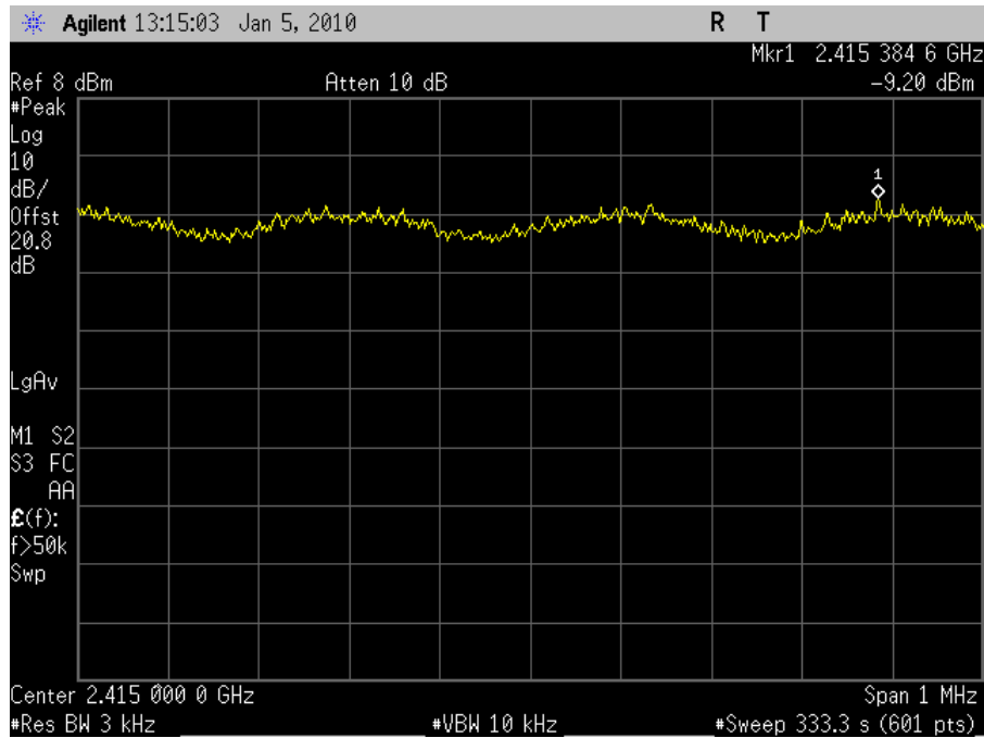
Plot 67. Power Spectral Density 2412MHz Low Channel 802.11g
