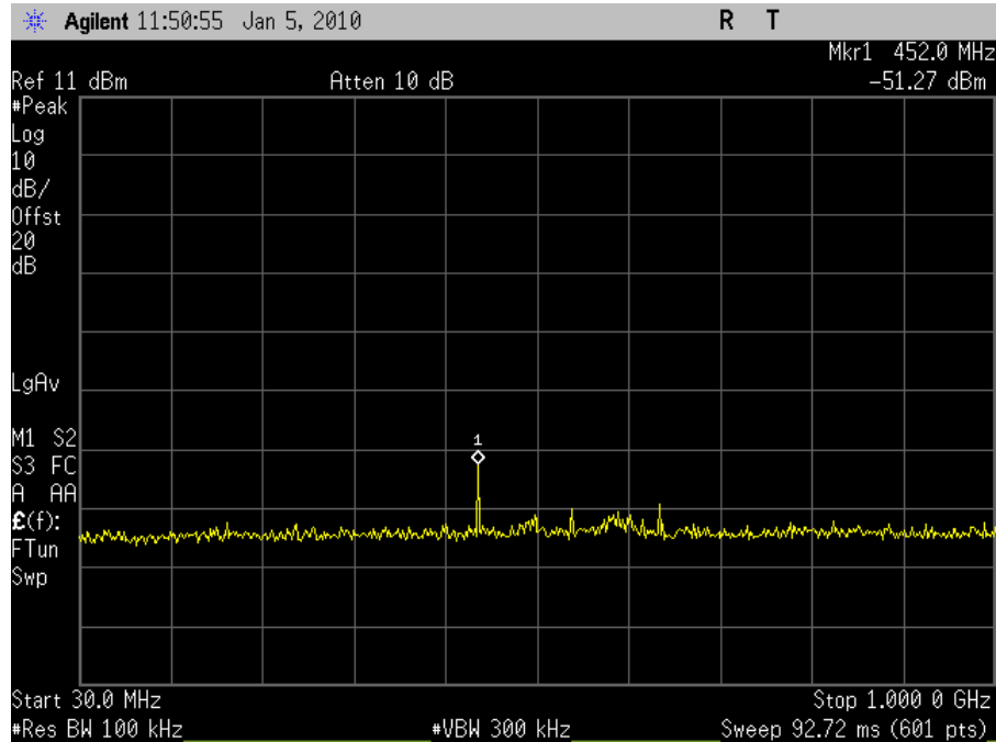
Plot 42. Conducted Spurious 2412MHz Low Channel 802.11b (30MHz-1GHz)
