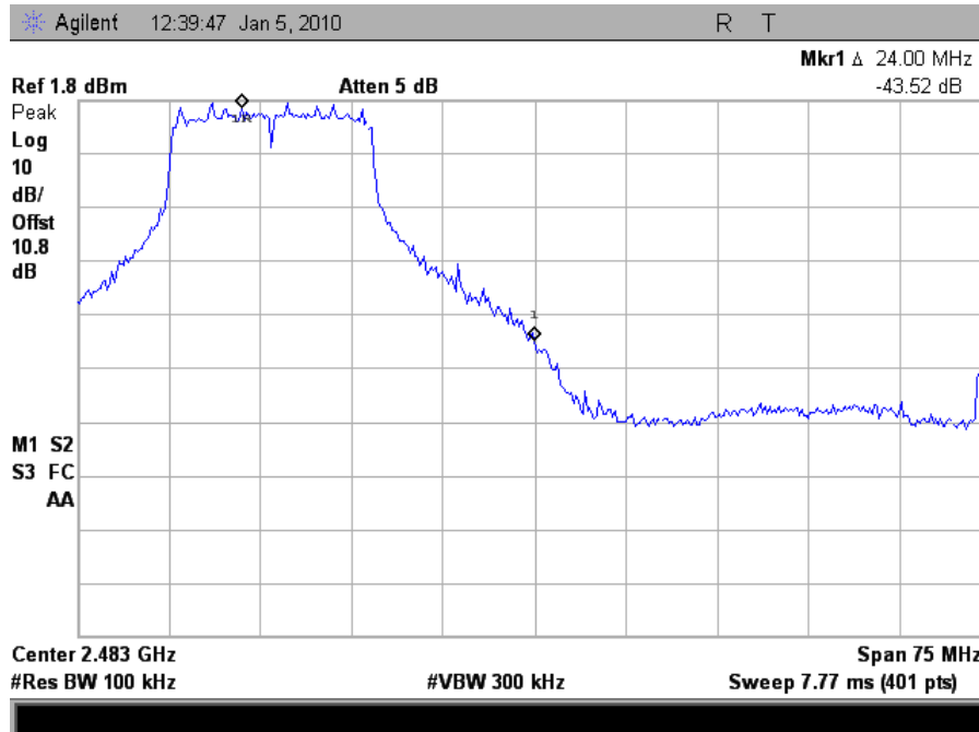
Plot 63. Conducted Band Edge, 802.11g Mode, High
