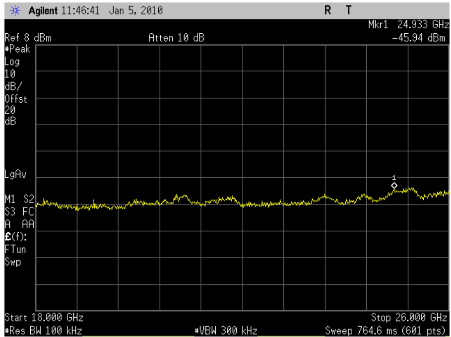
Plot 50. Conducted Spurious 2462MHz High Channel 802.11b (18-26GHz)
