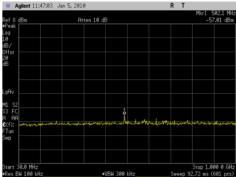
Plot 48. Conducted Spurious 2462MHz High Channel 802.11b (30MHz-1GHz)
