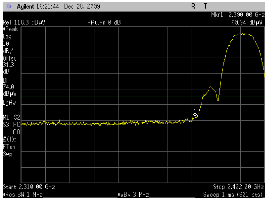
Plot 33. Restricted Band, 802.11b, Channel 1 (2412MHz), 8dBi Integrated Antenna, Peak
