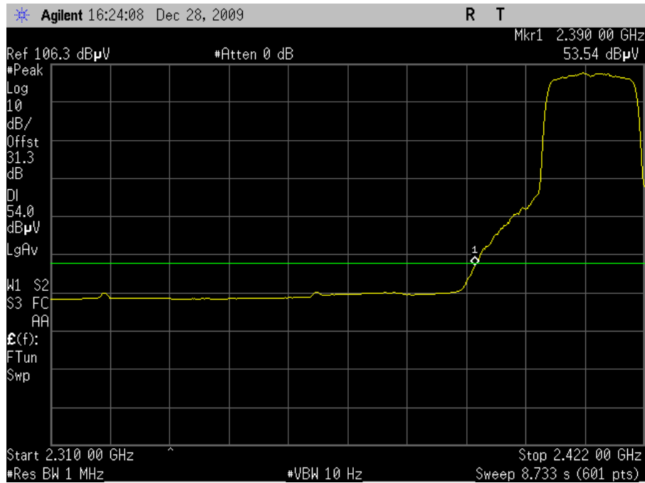
Plot 36. Restricted Band, 802.11g, Channel 1 (2412MHz), 8dBi Integrated Antenna, Average
