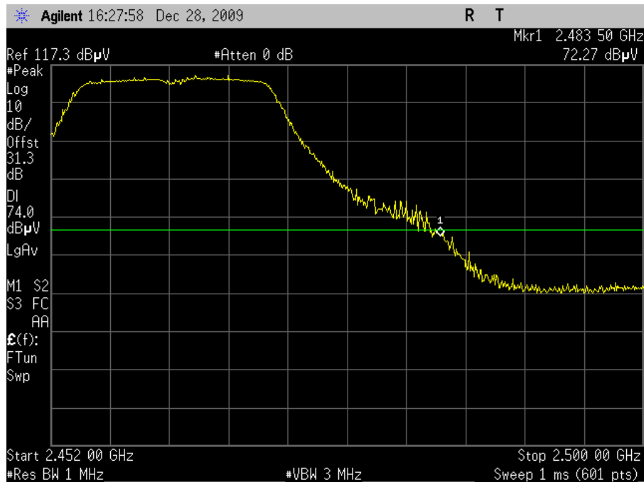
Plot 39. Restricted Band, 802.11g, Channel 11 (2462MHz), 8dBi Integrated Antenna, Peak
