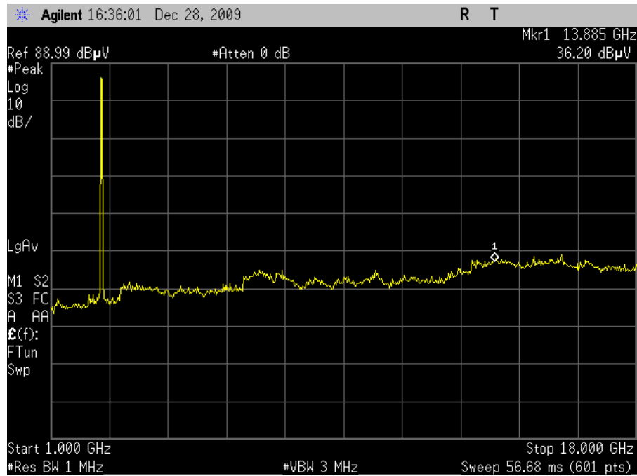
Plot 31. Radiated Spurious Emissions, 802.11g Mode High Channel
