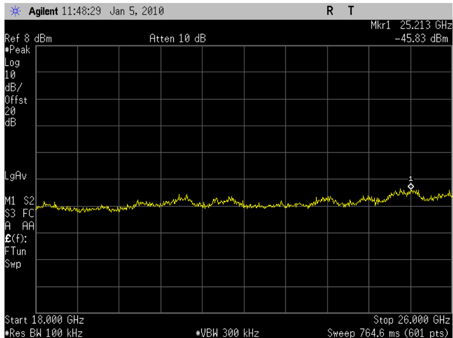
Plot 47. Conducted Spurious 2437MHz Mid Channel 802.11b (18-26GHz)
