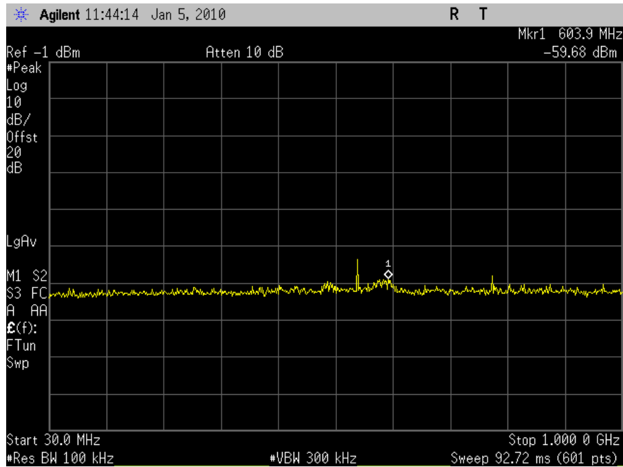
Plot 57. Conducted Spurious 2462MHz High Channel 802.11g (30MHz-1GHz)
