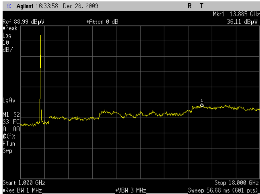
Plot 26. Radiated Spurious Emissions, 802.11b Mode Low Channel
