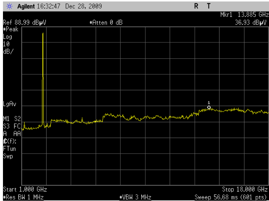
Plot 28. Radiated Spurious Emissions, 802.11b Mode High Channel
