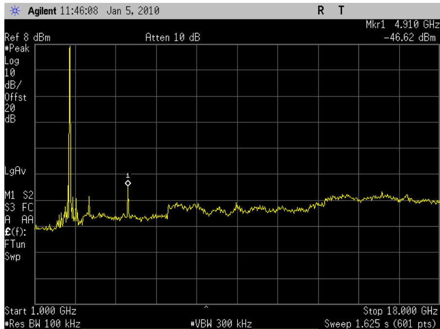
Plot 49. Conducted Spurious 2462MHz High Channel 802.11b (1-18GHz)
