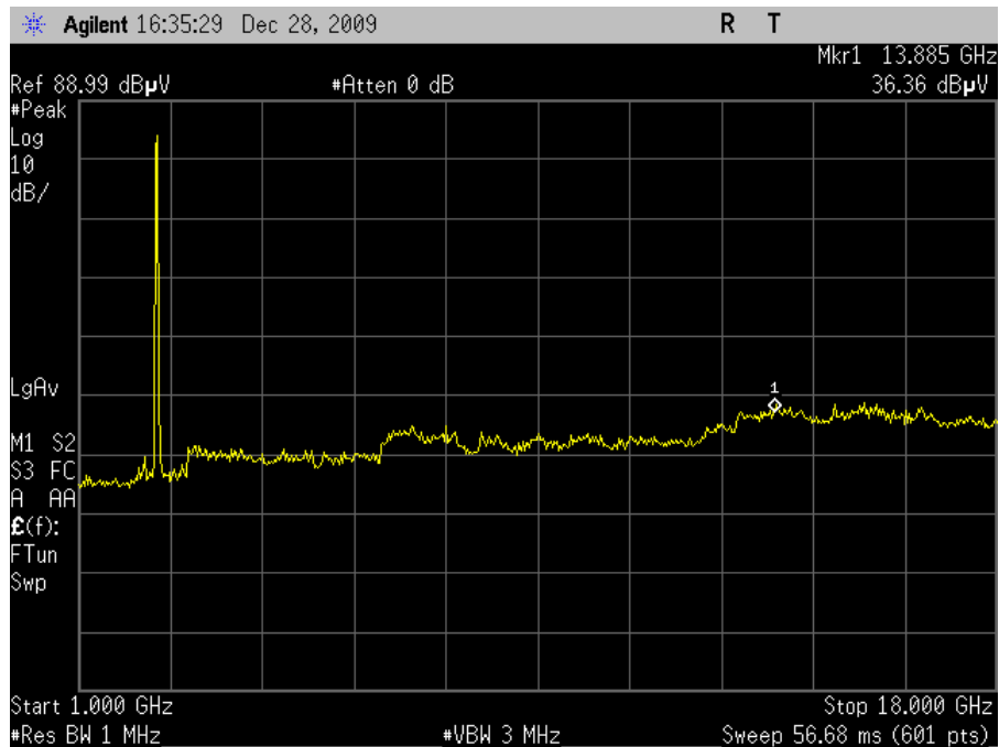
Plot 30. Radiated Spurious Emissions, 802.11g Mode Mid Channel
