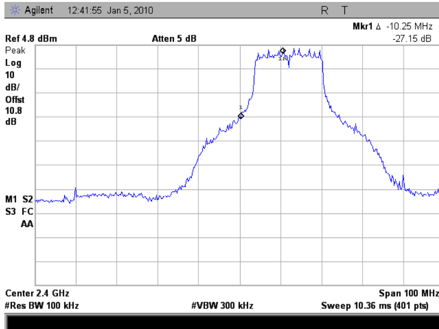
Plot 62. Conducted Band Edge, 802.11g Mode, Low
