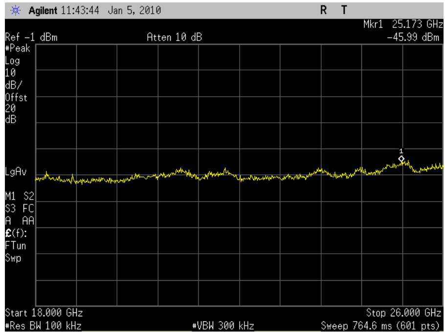
Plot 59. Conducted Spurious 2462MHz High Channel 802.11g (18-26GHz)
