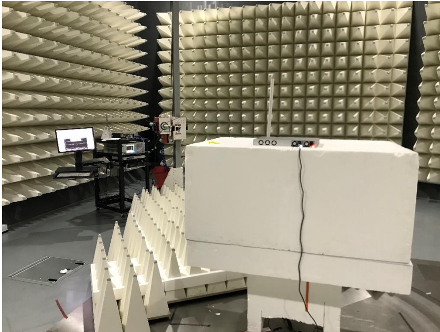
Photograph 5: View Test Set Up Radiated Emissions 17 - 26 GHz
