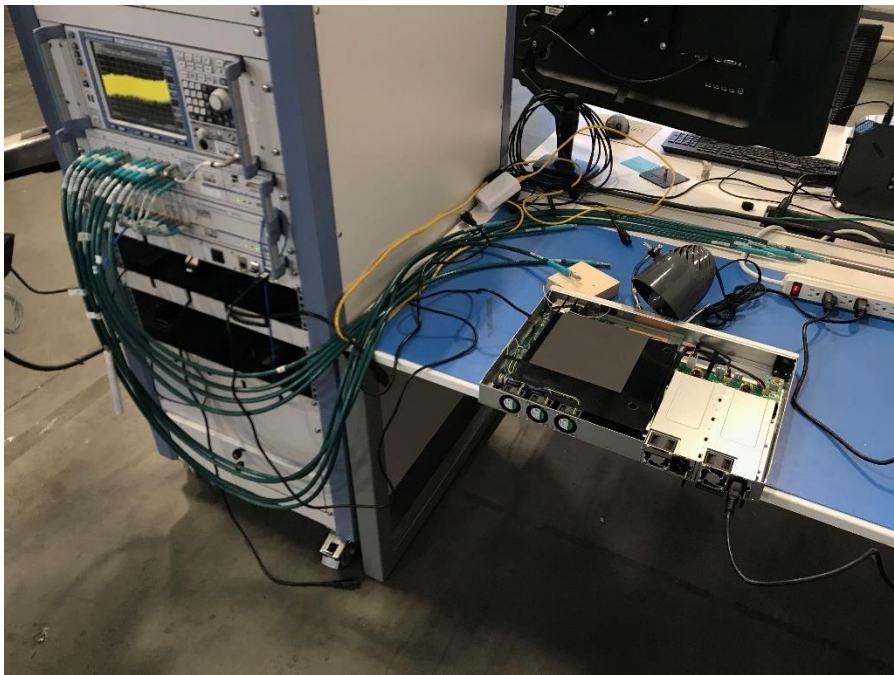
Photograph 6: View Test Set Up RF Conducted
