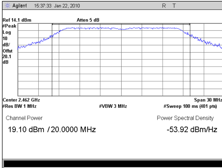
Plot 36. Peak Power Output, 802.11n, High Channel
