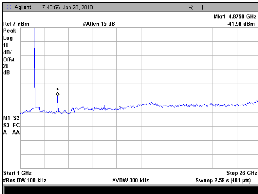
Plot 73. Conducted Spurious, Mid Channel, 802.11b (1 GHz - 26 GHz)
