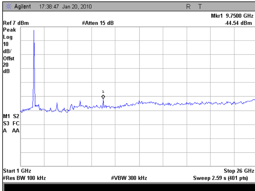
Plot 85. Conducted Spurious, Mid Channel, 802.11n (1 GHz - 26 GHz)
