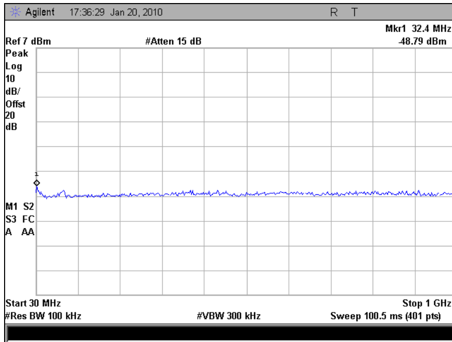
Plot 82. Conducted Spurious, Low Channel, 802.11n (30 MHz - 1 GHz)
