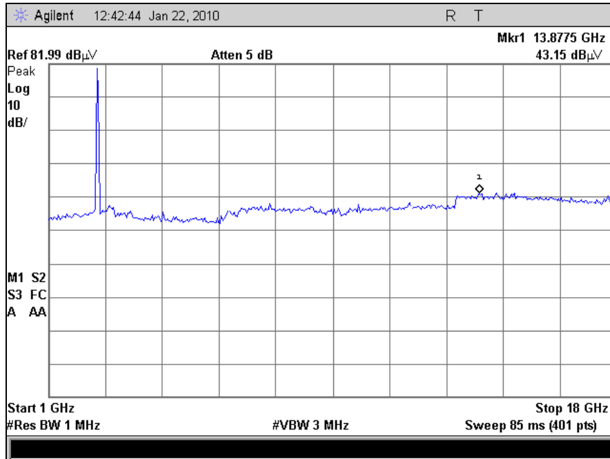
Plot 43. Radiated Spurious Emissions, 802.11g, Mid Channel
