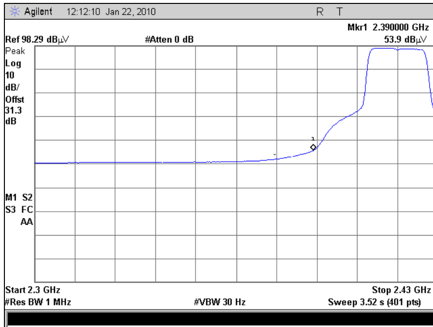
Plot 62. Radiated Band Edge, 802.11n, Channel 2 (Average)
