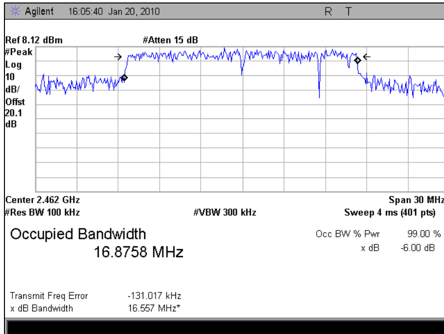
Plot 19. Occupied Bandwidth High Channel, 802.11g (FCC)
