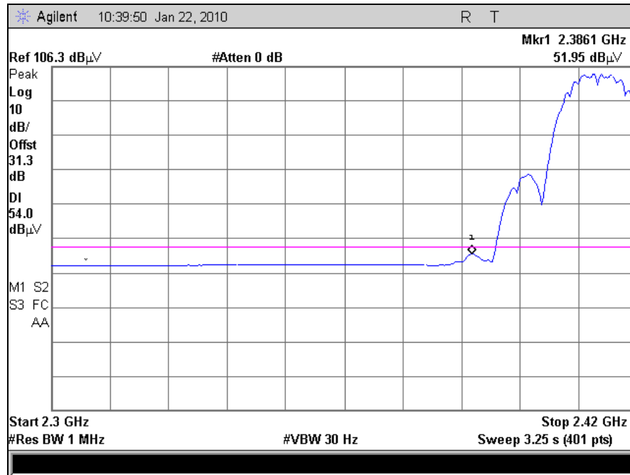
Plot 48. Radiated Band Edge, 802.11b, Channel 1 (Average)
