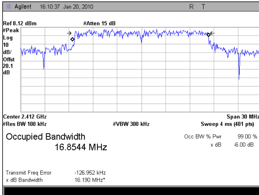
Plot 15. Occupied Bandwidth Low Channel, 802.11g (FCC)
