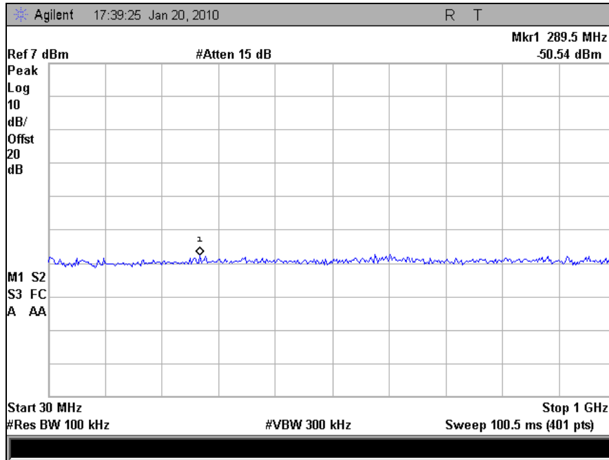
Plot 84. Conducted Spurious, Mid Channel, 802.11n (30 MHz - 1 GHz)
