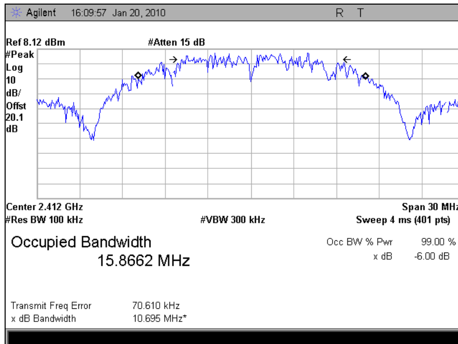
Plot 9. Occupied Bandwidth Low Channel, 802.11b (FCC)
