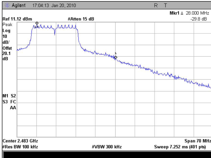
Plot 91. Conducted Band Edge, High Channel, 802.11g 20MHz
