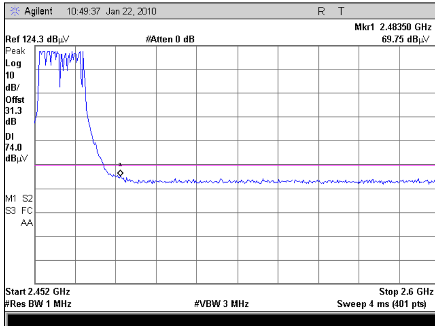
Plot 67. Radiated Band Edge, 802.11n, Channel 11 (Peak)
