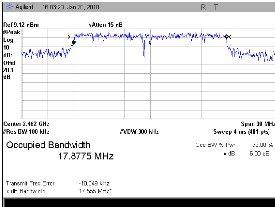
Plot 25. Occupied Bandwidth High Channel, 802.11n (FCC)
