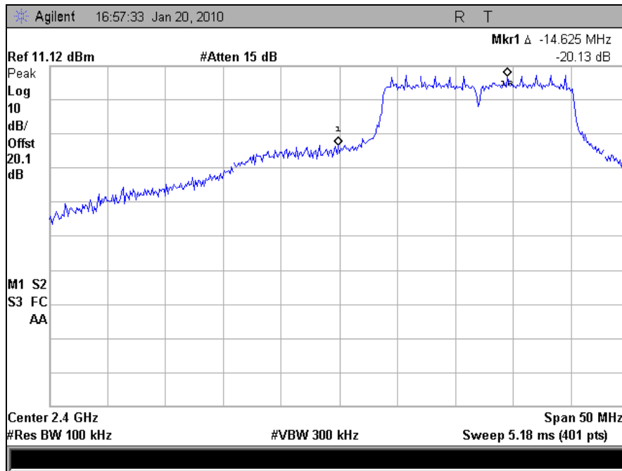
Plot 90. Conducted Band Edge, Low Channel, 802.11g 20MHz
