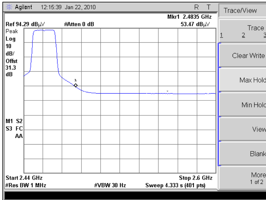
Plot 64. Radiated Band Edge, 802.11n, Channel 10 (Average)
