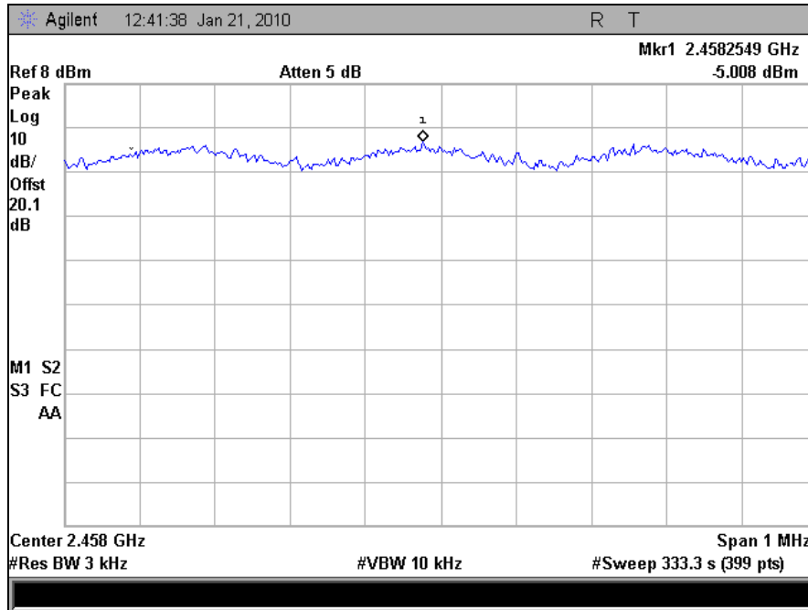
Plot 102. Peak Spectral Density, High Channel, 802.11n
