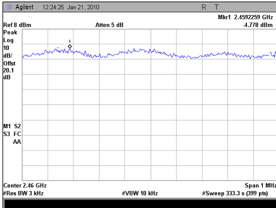
Plot 99. Peak Spectral Density, High Channel, 802.11g
