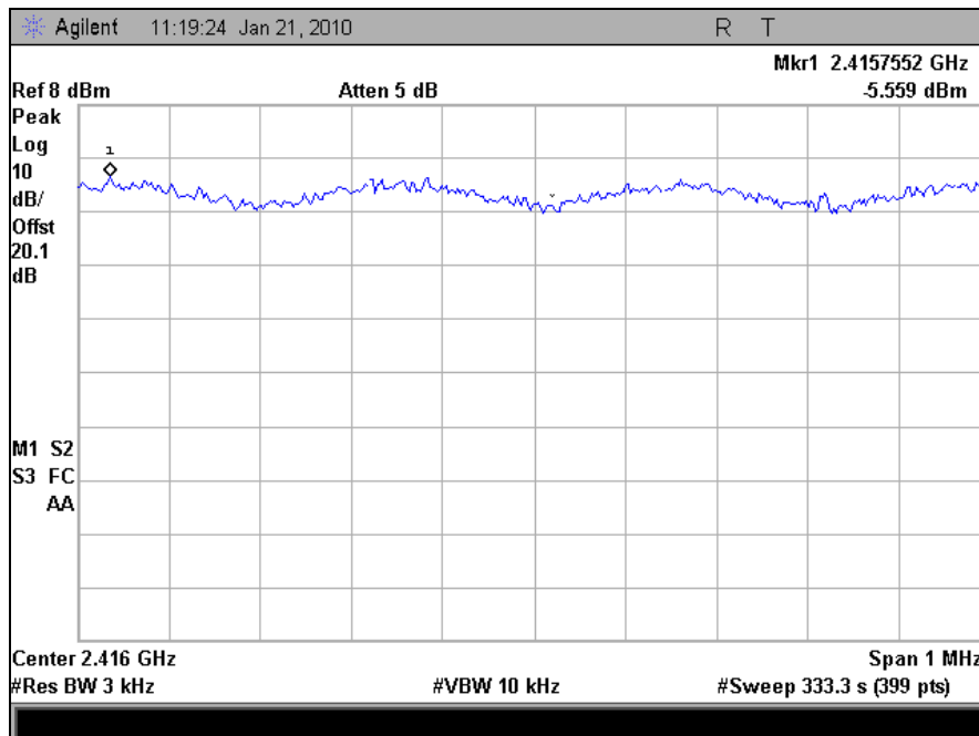
Plot 97. Peak Spectral Density, Low Channel, 802.11g
