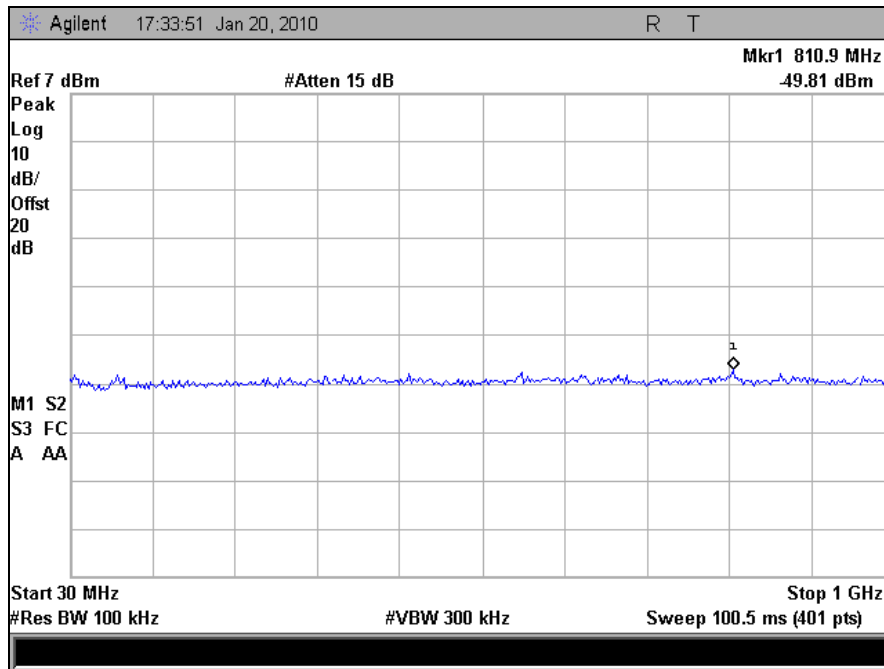
Plot 76. Conducted Spurious, Low Channel, 802.11g (30 MHz - 1 GHz)
