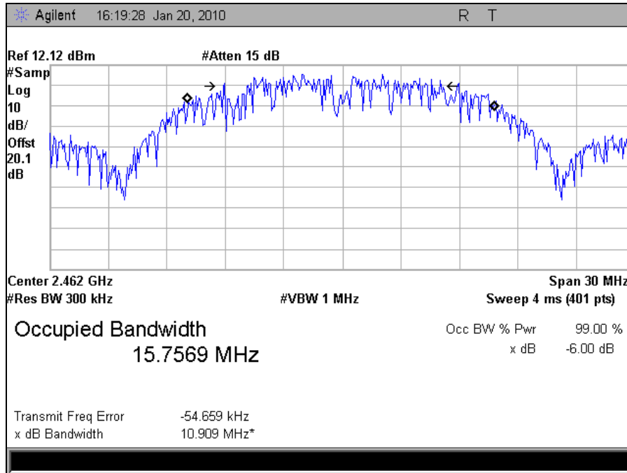
Plot 12. Occupied Bandwidth High Channel, 802.11b (99%)
