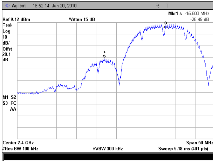
Plot 88. Conducted Band Edge, Low Channel, 802.11b 20MHz
