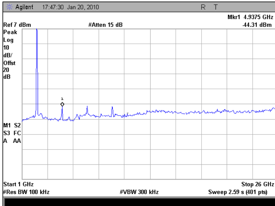
Plot 87. Conducted Spurious, High Channel, 802.11n (1 GHz - 26 GHz)
