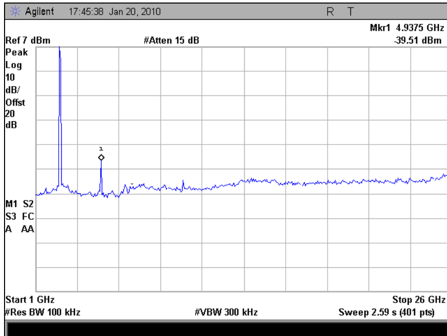
Plot 75. Conducted Spurious, High Channel, 802.11b (1 GHz - 26 GHz)
