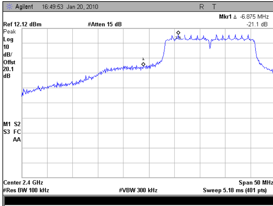
Plot 92. Conducted Band Edge, Low Channel, 802.11n 20MHz
