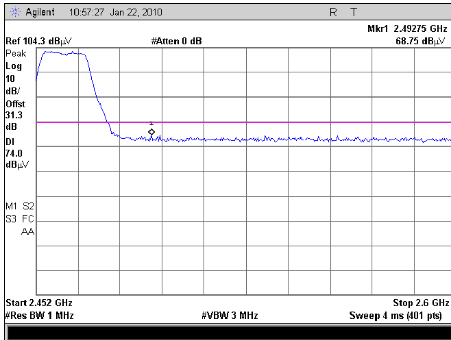
Plot 59. Radiated Band Edge, 802.11g, Channel 11 (Peak)
