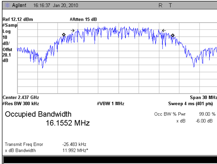
Plot 10. Occupied Bandwidth Mid Channel, 802.11b (99%)
