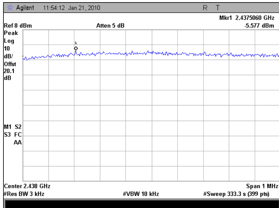
Plot 95. Peak Spectral Density, Mid Channel, 802.11b
