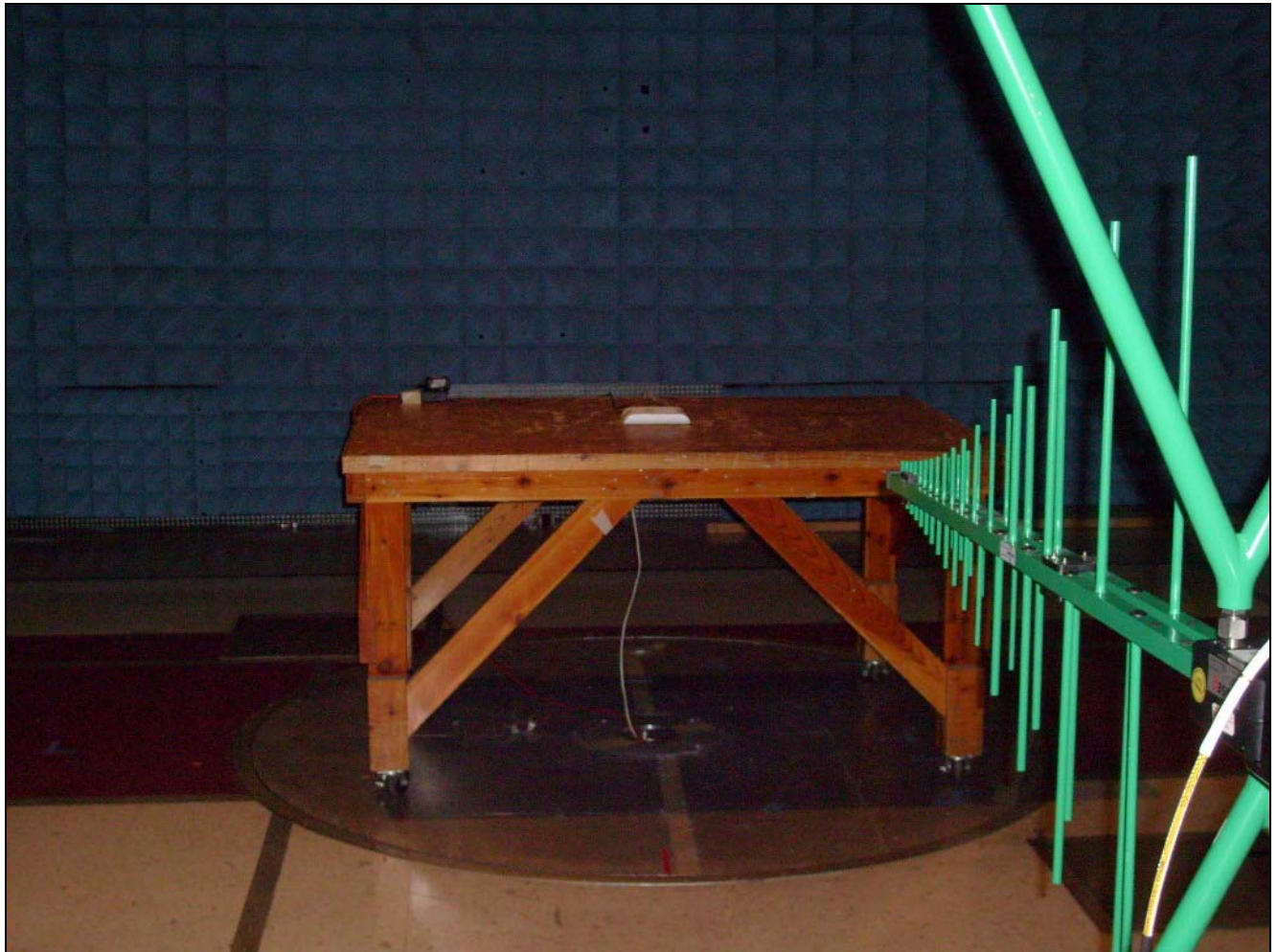
Photograph 4. Radiated Emissions, Test Setup
