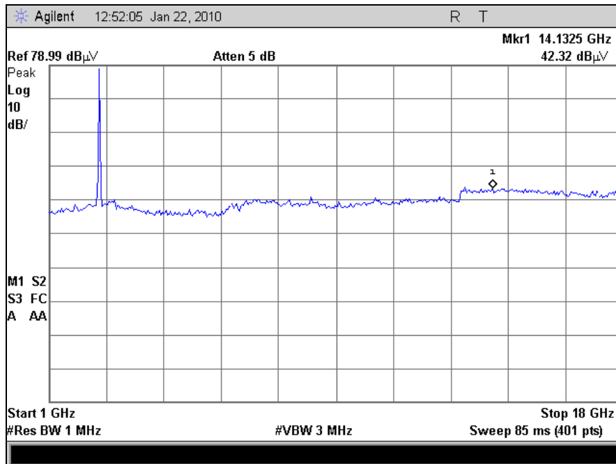
Plot 44. Radiated Spurious Emissions, 802.11g, High Channel
