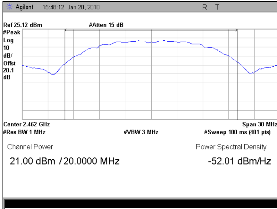
Plot 28. Peak Power Output, 802.11b, High Channel
