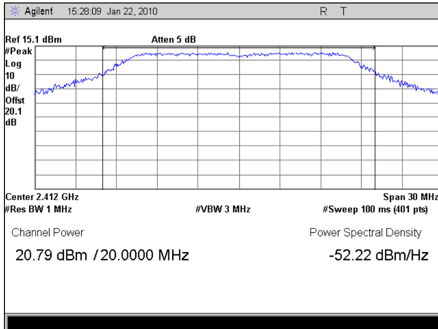
Plot 29. Peak Power Output, 802.11g, Low Channel
