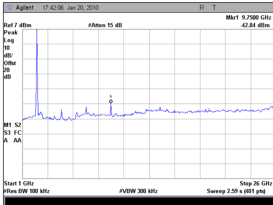
Plot 79. Conducted Spurious, Mid Channel, 802.11g (1 GHz - 26 GHz)
