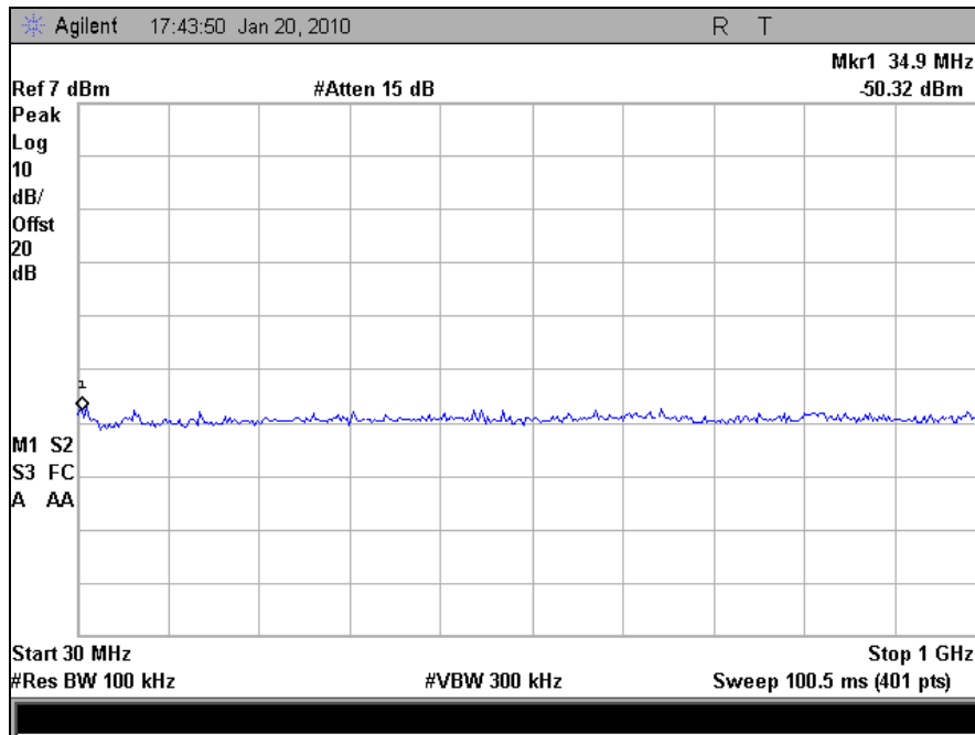
Plot 80. Conducted Spurious, High Channel, 802.11g (30 MHz - 1 GHz)
