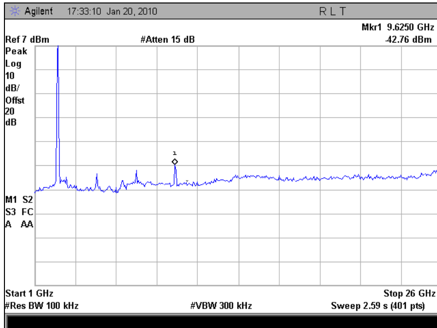
Plot 77. Conducted Spurious, Low Channel, 802.11g (1 GHz - 26 GHz)
