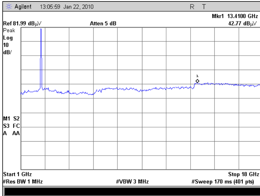
Plot 45. Radiated Spurious Emissions, 802.11n, Low Channel
