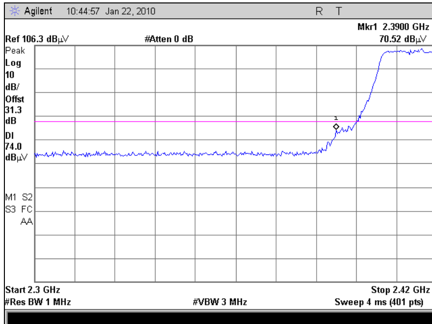
Plot 61. Radiated Band Edge, 802.11n, Channel 1 (Peak)
