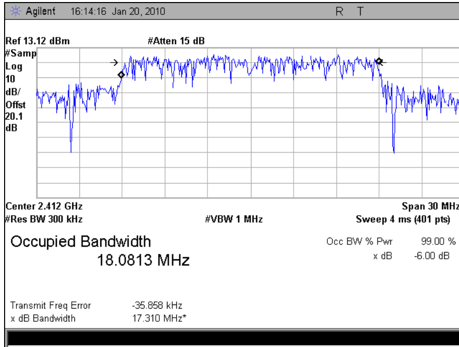
Plot 20. Occupied Bandwidth Low Channel, 802.11n (99%)
