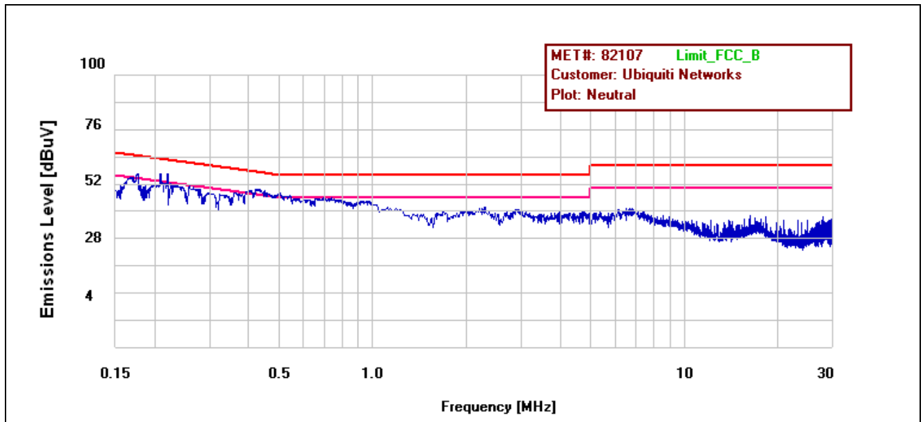
Plot 7. Conducted Emissions, Neutral Line Plot
