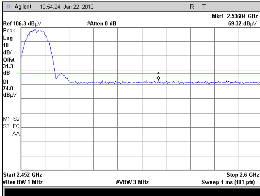
Plot 51. Radiated Band Edge, 802.11b, Channel 11 (Peak)
