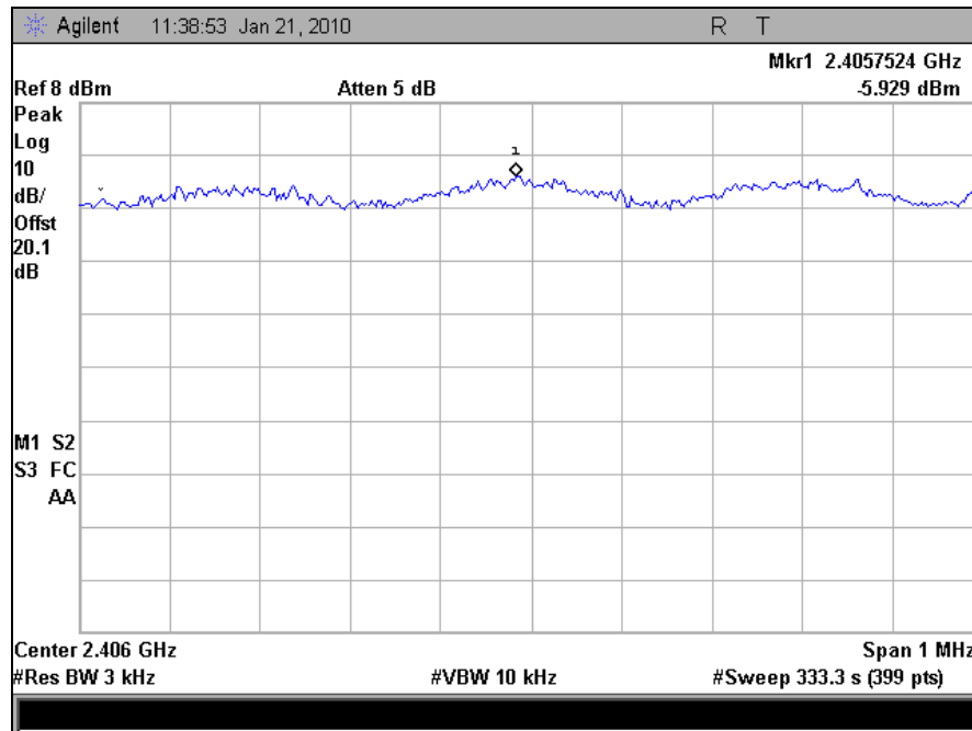
Plot 100. Peak Spectral Density, Low Channel, 802.11n
