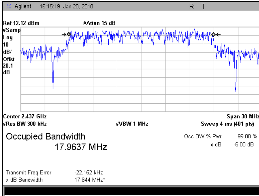
Plot 22. Occupied Bandwidth Mid Channel, 802.11n (99%)
