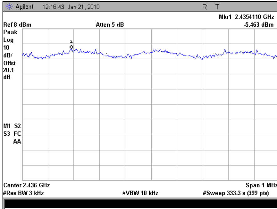
Plot 98. Peak Spectral Density, Mid Channel, 802.11g
