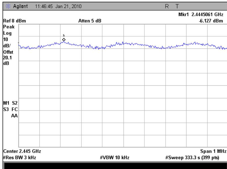
Plot 101. Peak Spectral Density, Mid Channel, 802.11n
