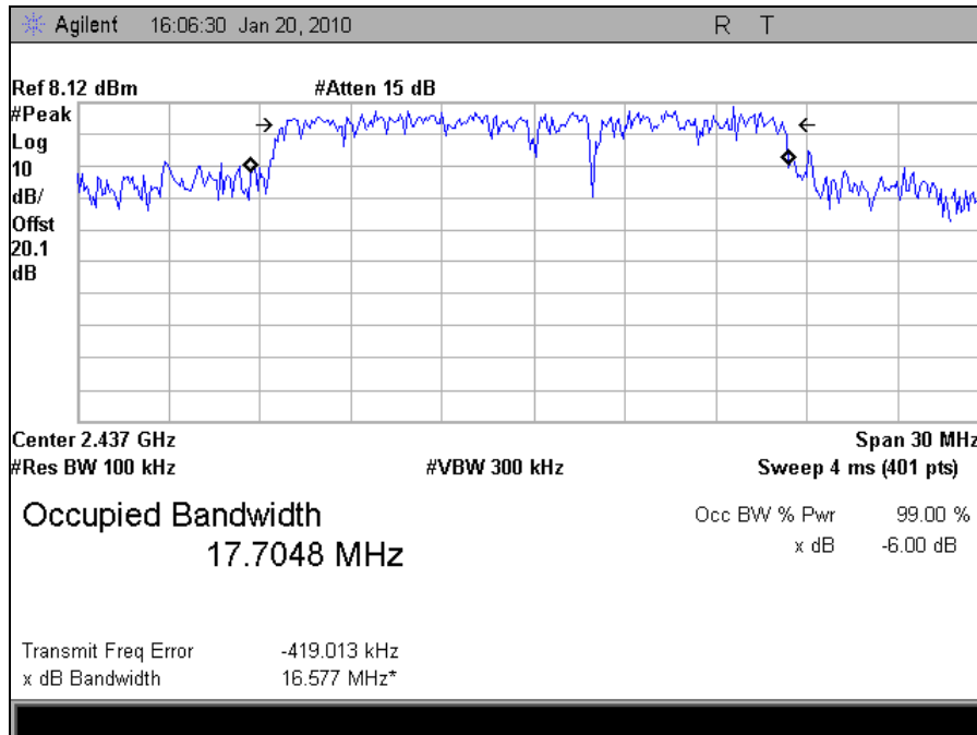
Plot 17. Occupied Bandwidth Mid Channel, 802.11g (FCC)
