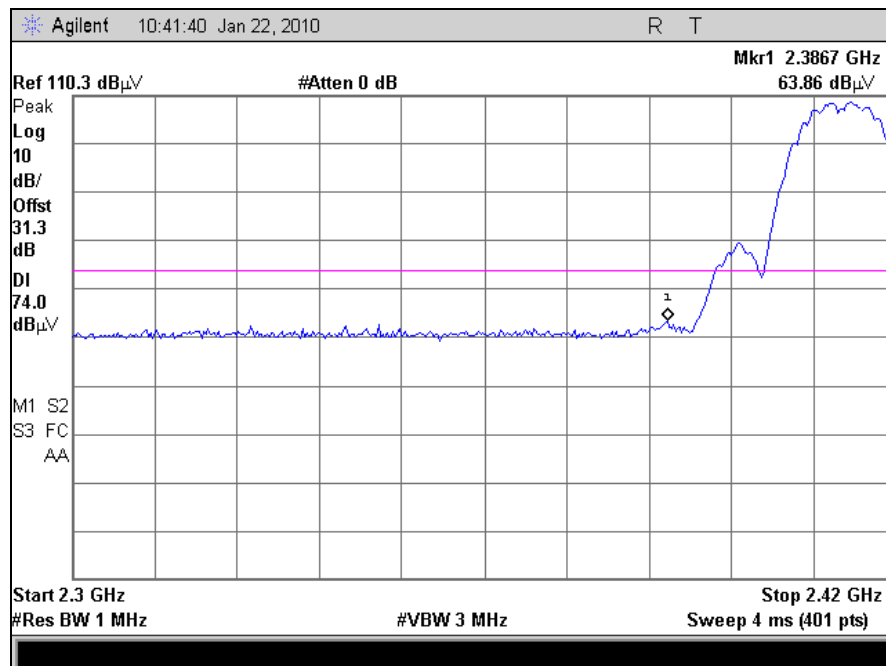
Plot 49. Radiated Band Edge, 802.11b, Channel 1 (Peak)
