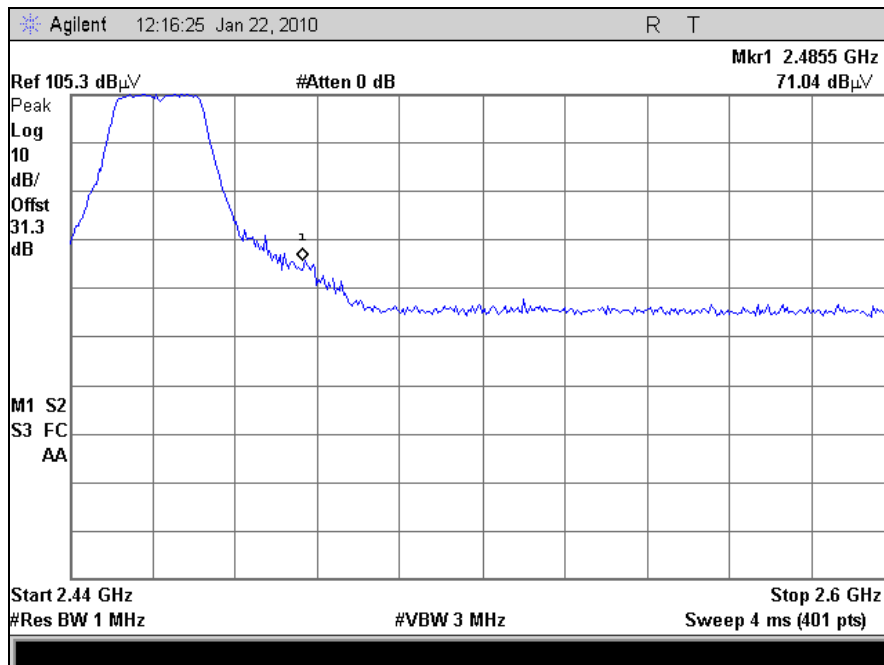
Plot 65. Radiated Band Edge, 802.11n, Channel 10 (Peak)
