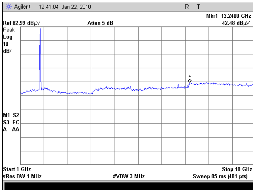
Plot 42. Radiated Spurious Emissions, 802.11g, Low Channel
