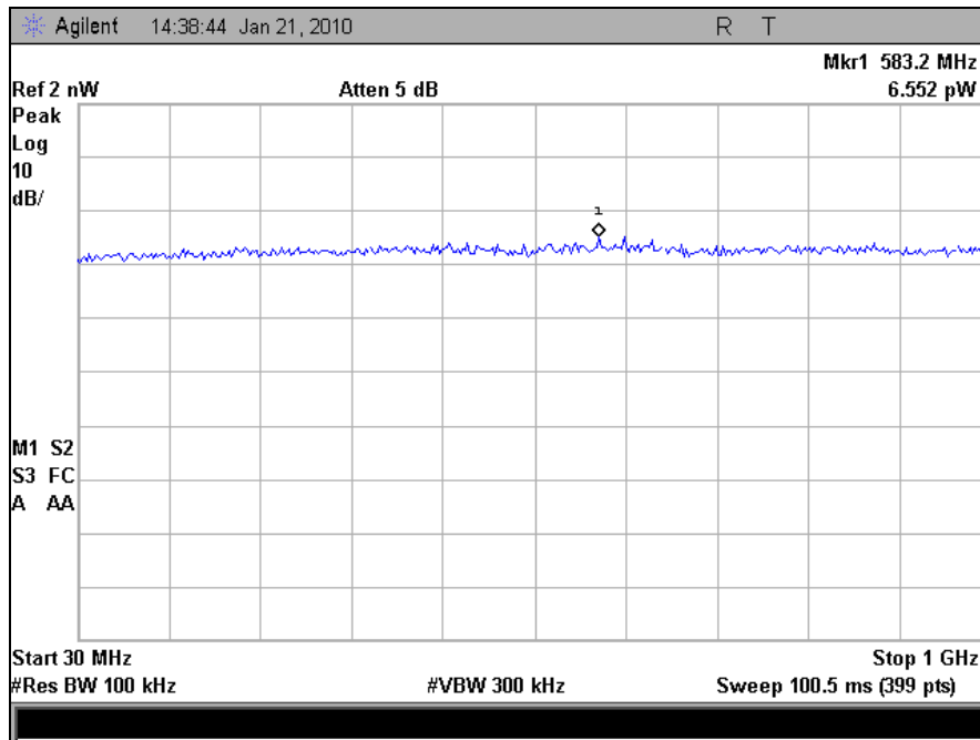
Plot 68. Receiver Spurious Emission, 30 MHz – 1 GHz, Horizontal
