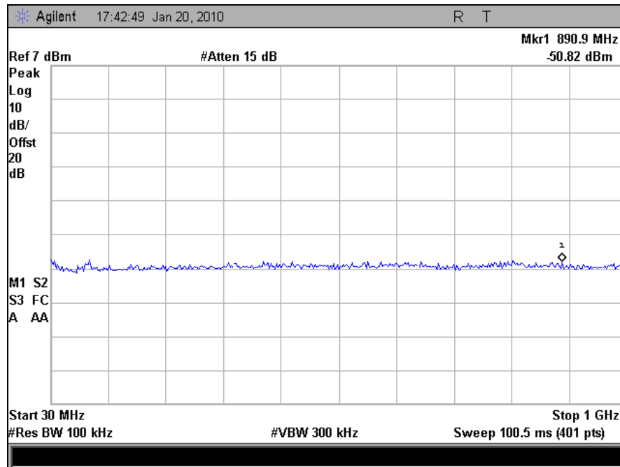
Plot 78. Conducted Spurious, Mid Channel, 802.11g (30 MHz - 1 GHz)
