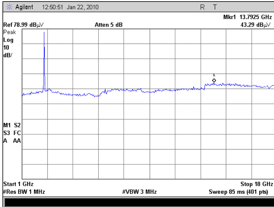
Plot 41. Radiated Spurious Emissions, 802.11b, High Channel
