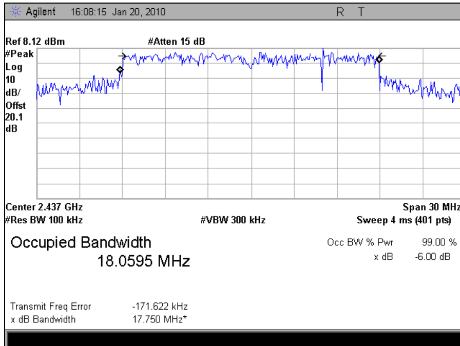
Plot 23. Occupied Bandwidth Mid Channel, 802.11n (FCC)
