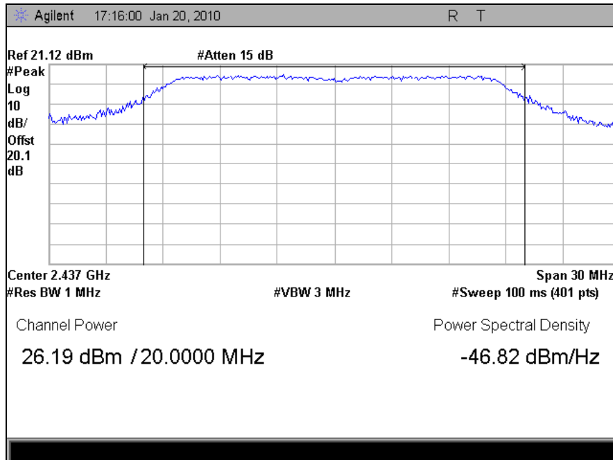
Plot 35. Peak Power Output, 802.11n, Mid Channel
