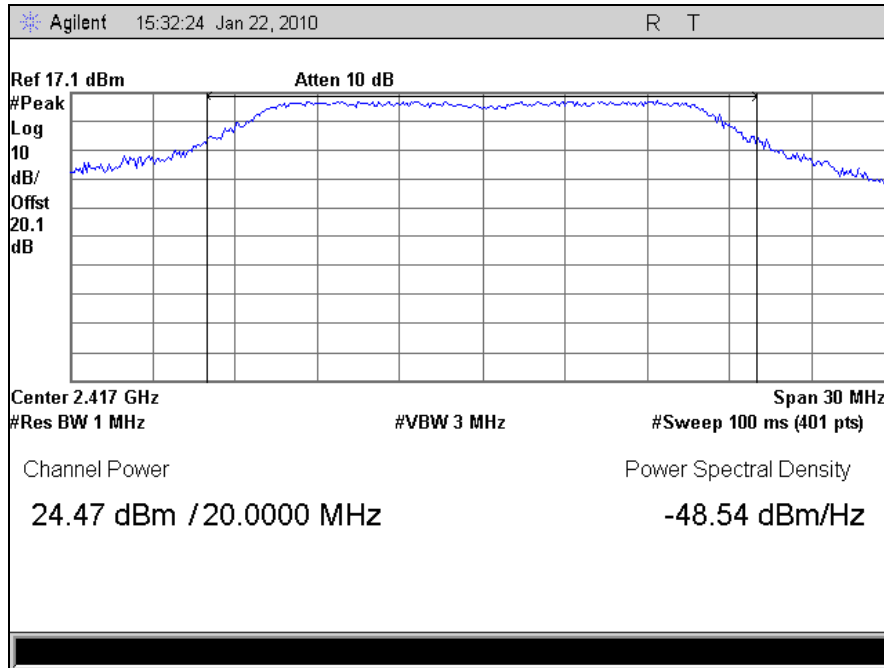
Plot 32. Peak Power Output, Channel 2, 802.11g
