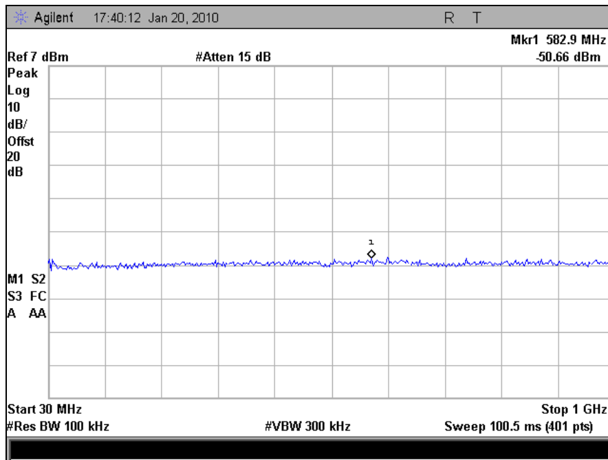
Plot 72. Conducted Spurious, Mid Channel, 802.11b (30 MHz - 1 GHz)
