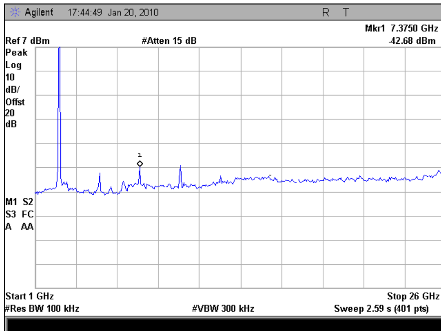
Plot 81. Conducted Spurious, High Channel, 802.11g (1 GHz - 26 GHz)
