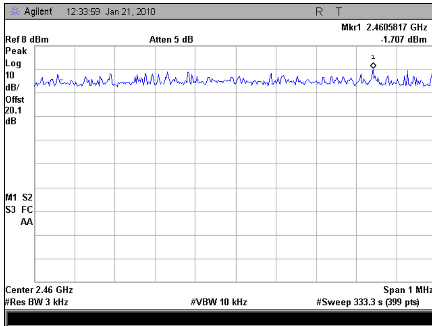
Plot 96. Peak Spectral Density, High Channel, 802.11b
