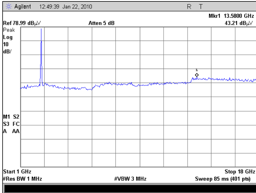
Plot 47. Radiated Spurious Emissions, 802.11n, High Channel
