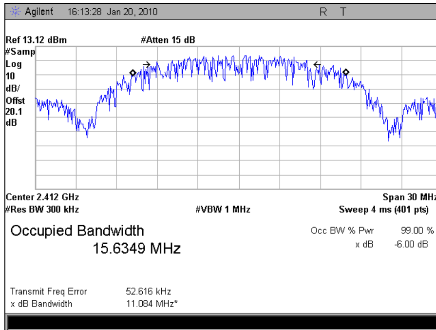
Plot 8. Occupied Bandwidth Low Channel, 802.11b (99%)
