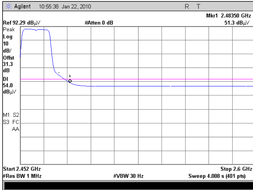
Plot 58. Radiated Band Edge, 802.11g, Channel 11 (Average)
