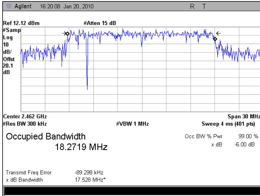
Plot 24. Occupied Bandwidth High Channel, 802.11n (99%)
