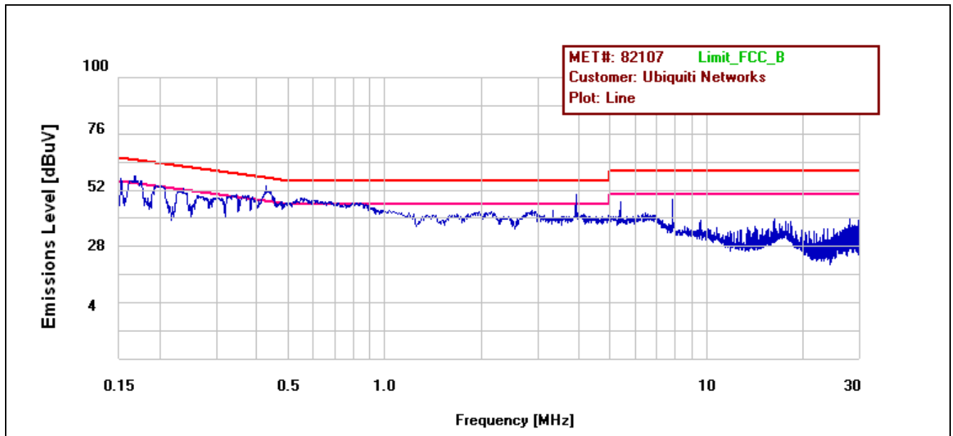
Plot 6. Conducted Emissions, Phase Line Plot
