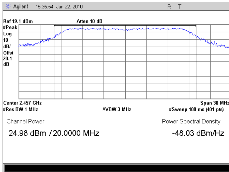
Plot 38. Peak Power Output, 802.11n, Channel 10
