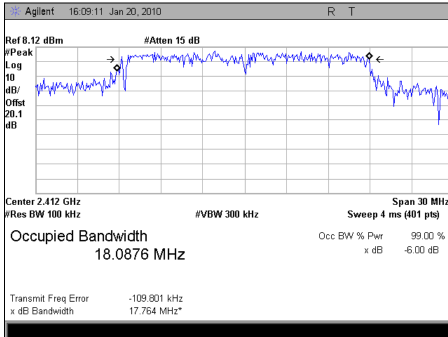
Plot 21. Occupied Bandwidth Low Channel, 802.11n (FCC)
