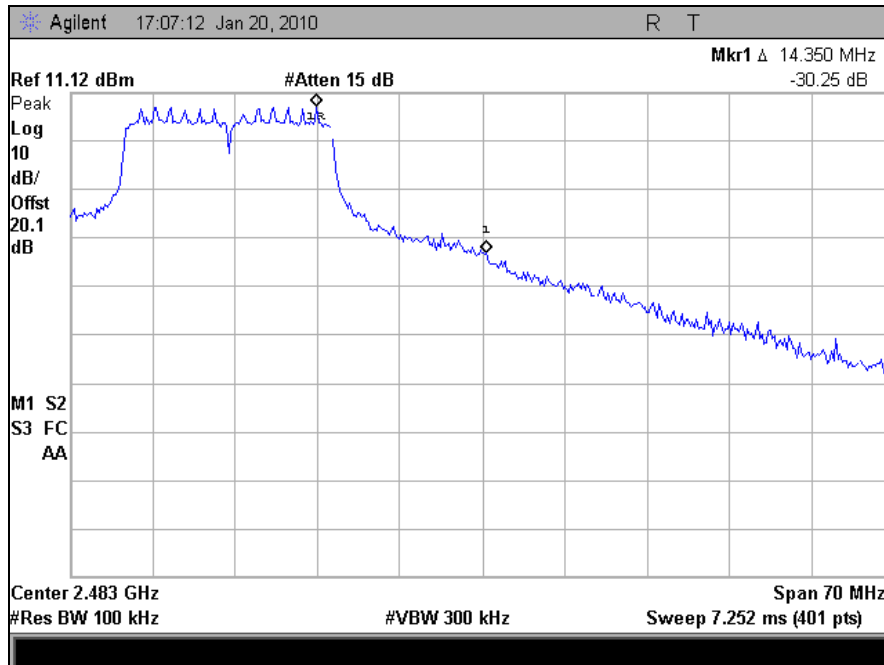
Plot 93. Conducted Band Edge, High Channel, 802.11n 20MHz
