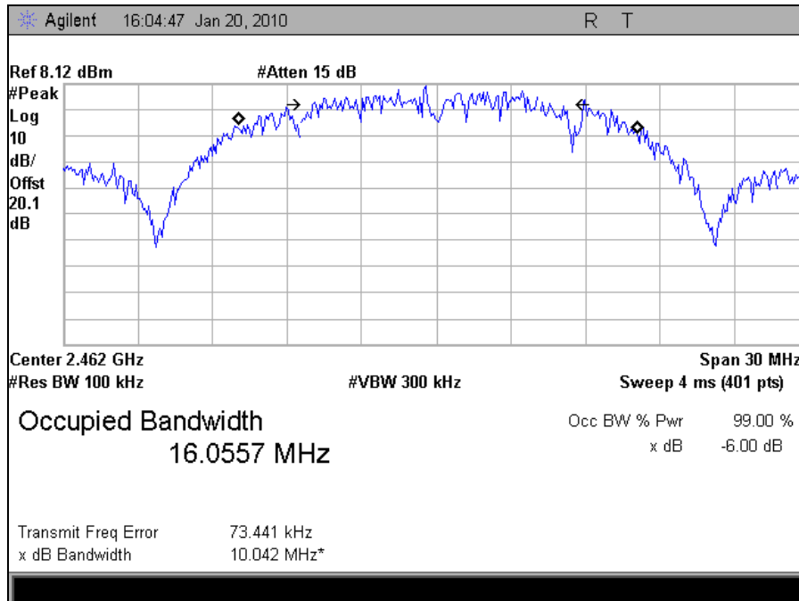
Plot 13. Occupied Bandwidth High Channel, 802.11b (FCC)
