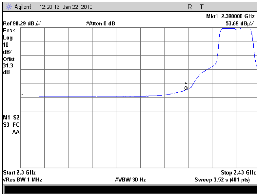
Plot 54. Radiated Band Edge, 802.11g, Channel 2 (Average)
