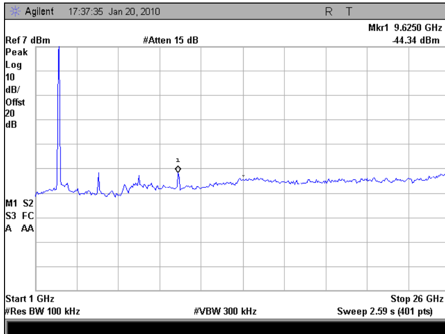
Plot 83. Conducted Spurious, Low Channel, 802.11n (1 GHz - 26 GHz)
