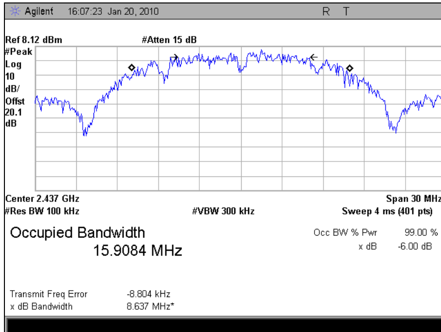
Plot 11. Occupied Bandwidth Mid Channel, 802.11b (FCC)
