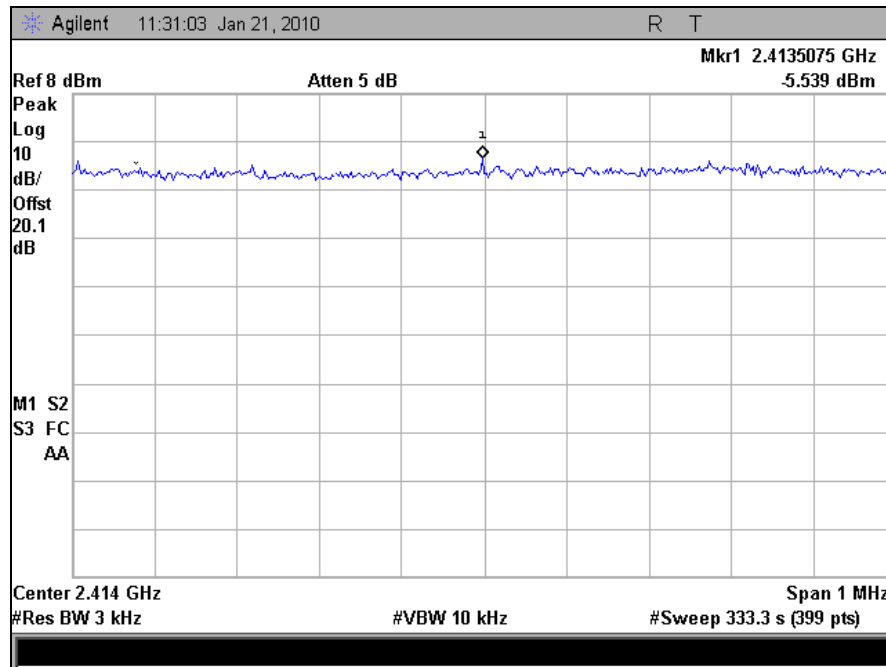
Plot 94. Peak Spectral Density, Low Channel, 802.11b
