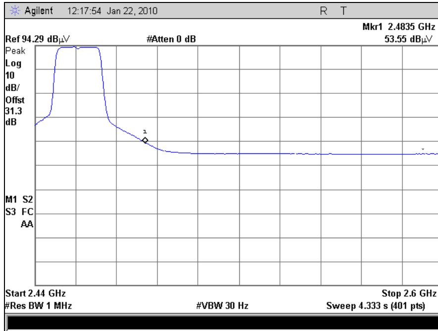
Plot 56. Radiated Band Edge, 802.11g, Channel 10 (Average)
