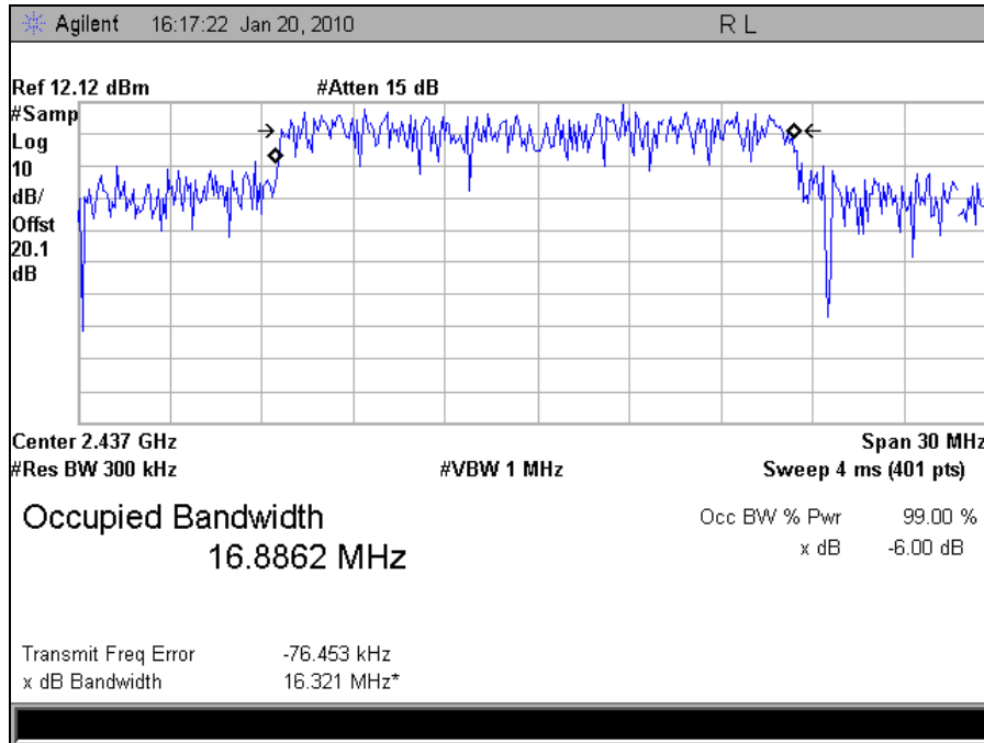
Plot 16. Occupied Bandwidth Mid Channel, 802.11g (99%)
