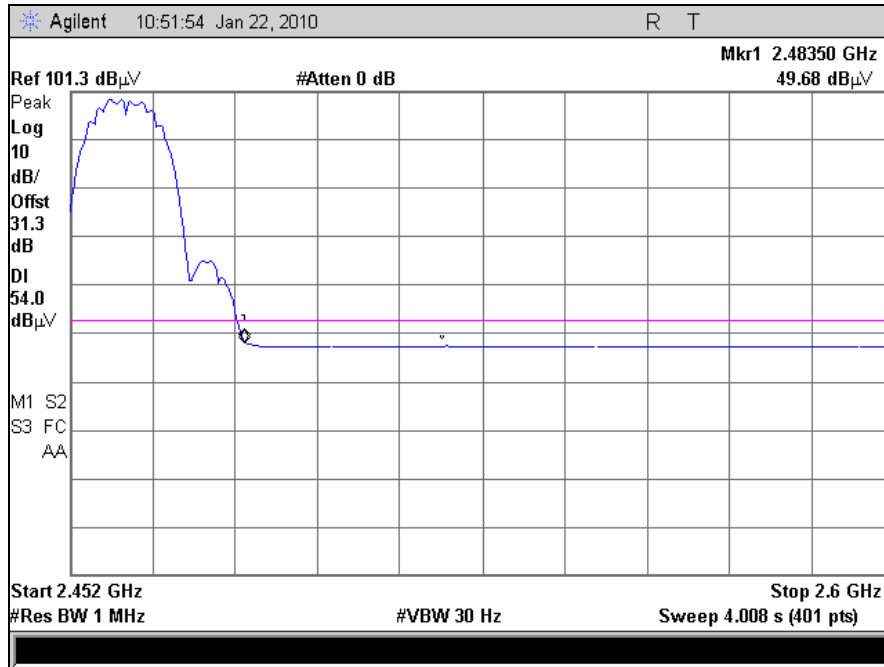
Plot 50. Radiated Band Edge, 802.11b, Channel 11 (Average)
