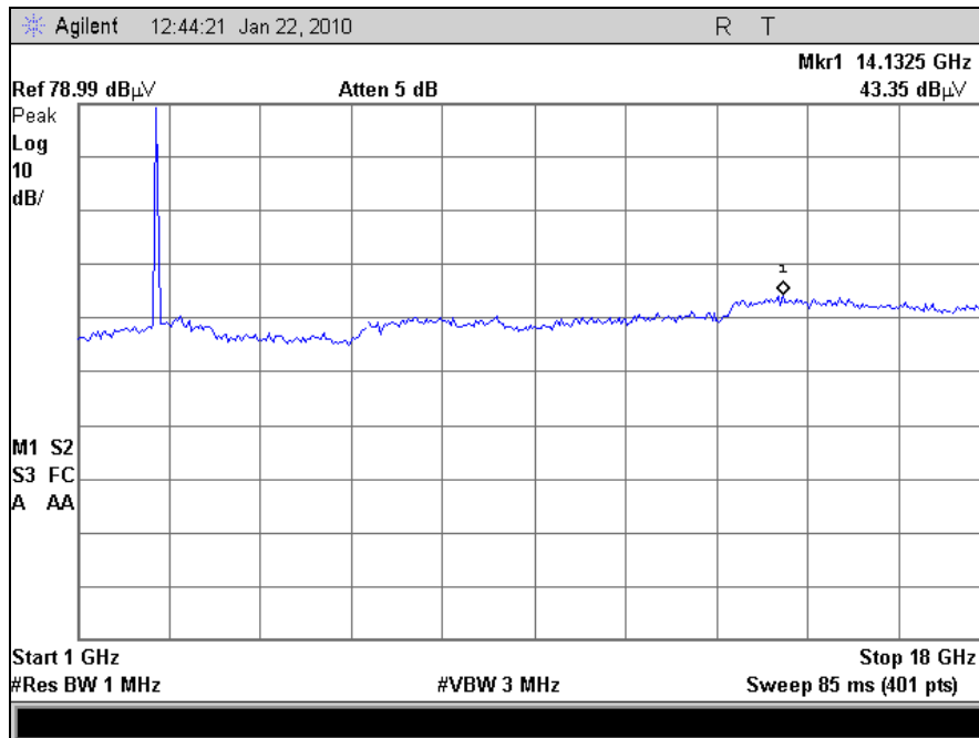
Plot 40. Radiated Spurious Emissions, 802.11b, Mid Channel
