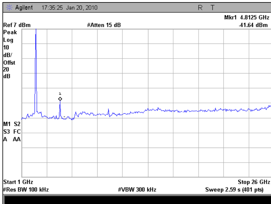
Plot 71. Conducted Spurious, Low Channel, 802.11b (1 GHz - 26 GHz)
