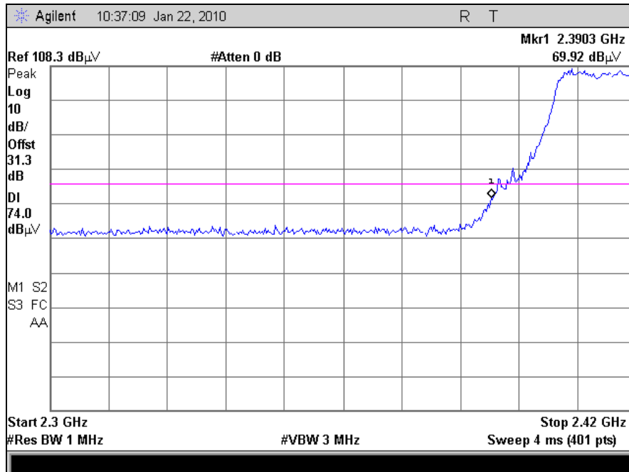
Plot 53. Radiated Band Edge, 802.11g, Channel 1(Peak)
