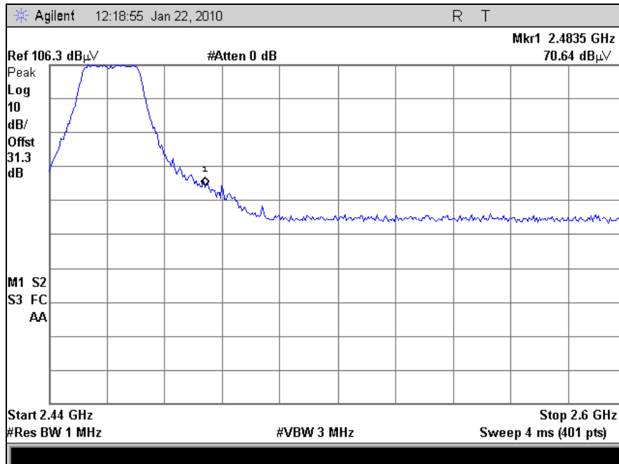
Plot 57. Radiated Band Edge, 802.11g, Channel 10 (Peak)
