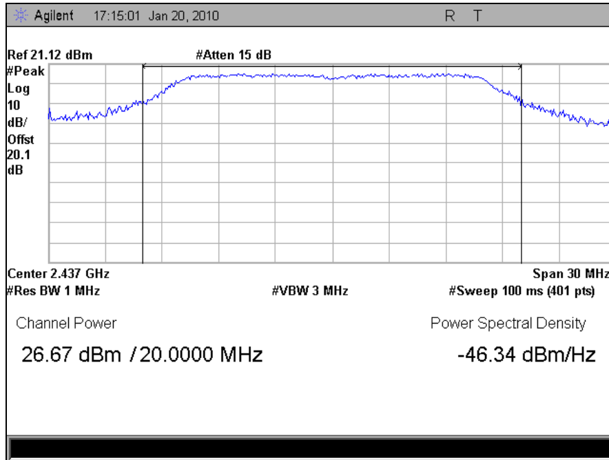
Plot 30. Peak Power Output, 802.11g, Mid Channel
