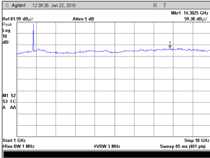
Plot 39. Radiated Spurious Emissions, 802.11b, Low Channel
