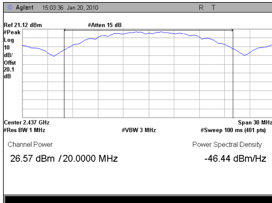
Plot 27. Peak Power Output, 802.11b, Mid Channel
