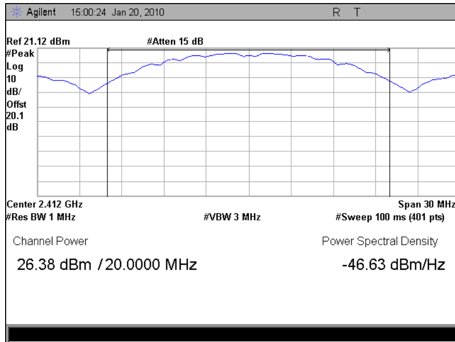
Plot 26. Peak Power Output, 802.11b, Low Channel
