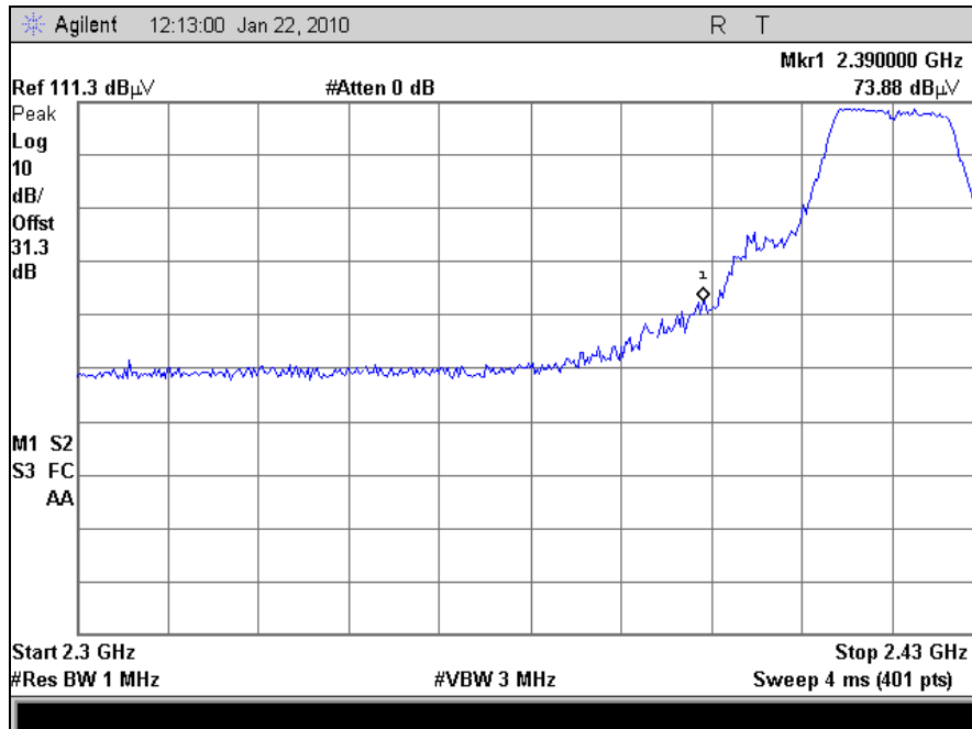
Plot 63. Radiated Band Edge, 802.11n, Channel 2 (Peak)
