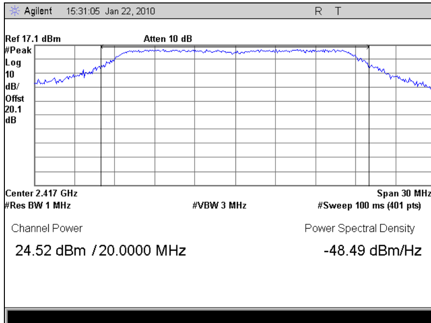
Plot 37. Peak Power Output, 802.11n, Channel 2
