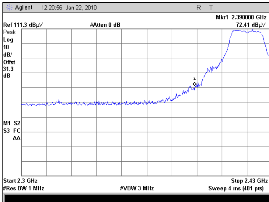
Plot 55. Radiated Band Edge, 802.11g, Channel 2 (Peak)
