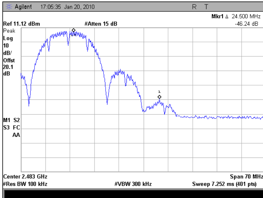
Plot 89. Conducted Band Edge, High Channel, 802.11b 20MHz
