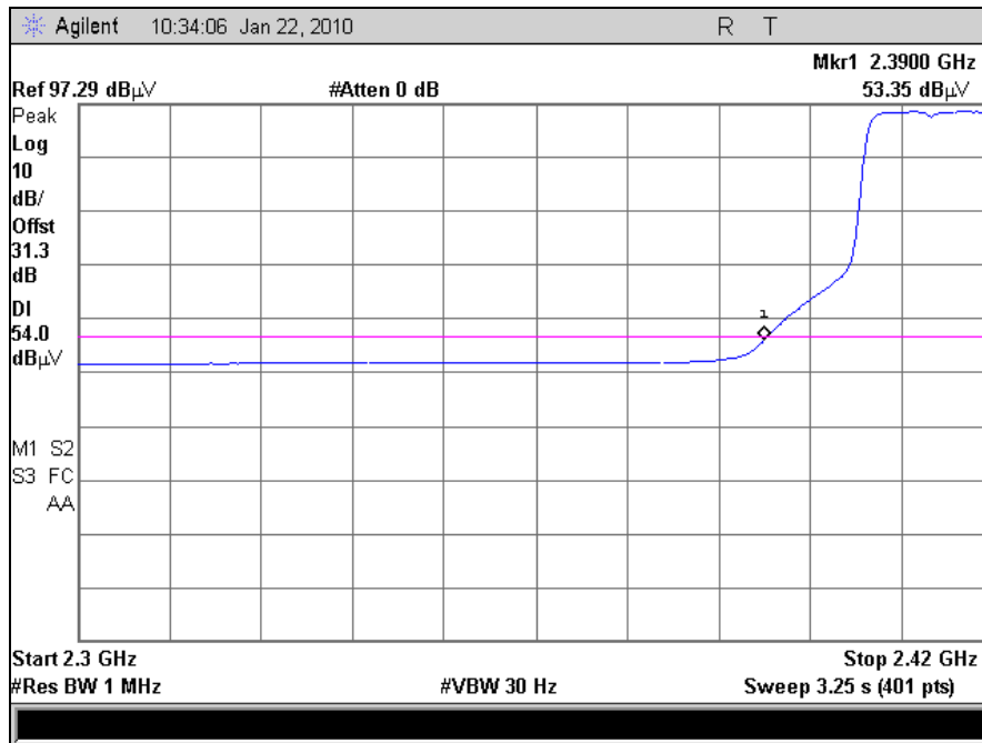
Plot 52. Radiated Band Edge, 802.11g, Channel 1 (Average)
