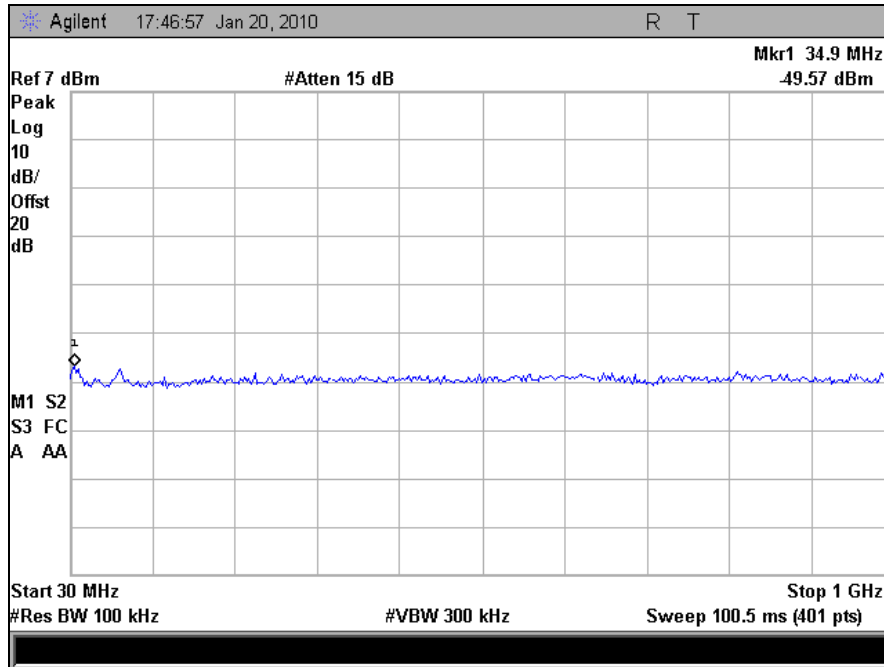
Plot 86. Conducted Spurious, High Channel, 802.11n (30 MHz - 1 GHz)
