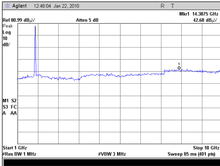
Plot 46. Radiated Spurious Emissions, 802.11n, Mid Channel
