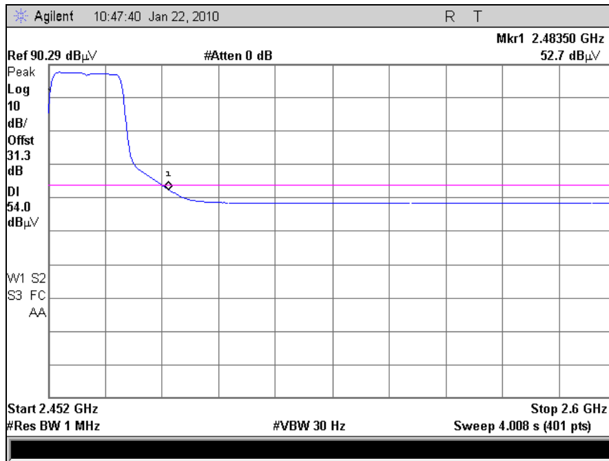
Plot 66. Radiated Band Edge, 802.11n, Channel 11 (Average)
