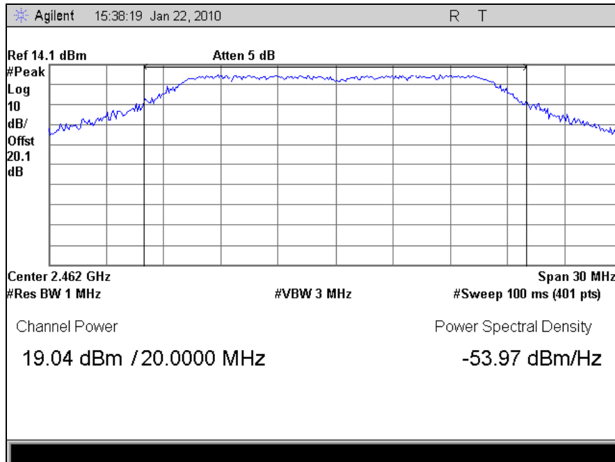
Plot 31. Peak Power Output, 802.11g, High Channel
