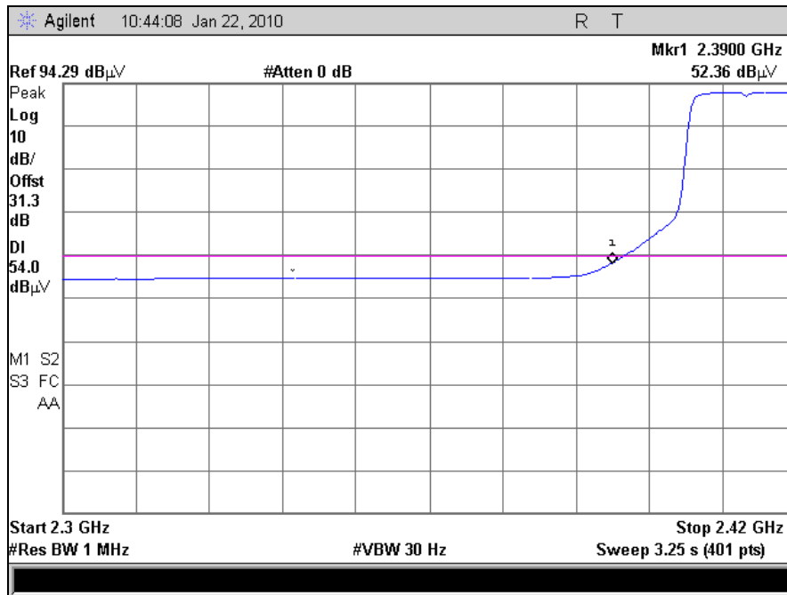
Plot 60. Radiated Band Edge, 802.11n, Channel 1 (Average)
