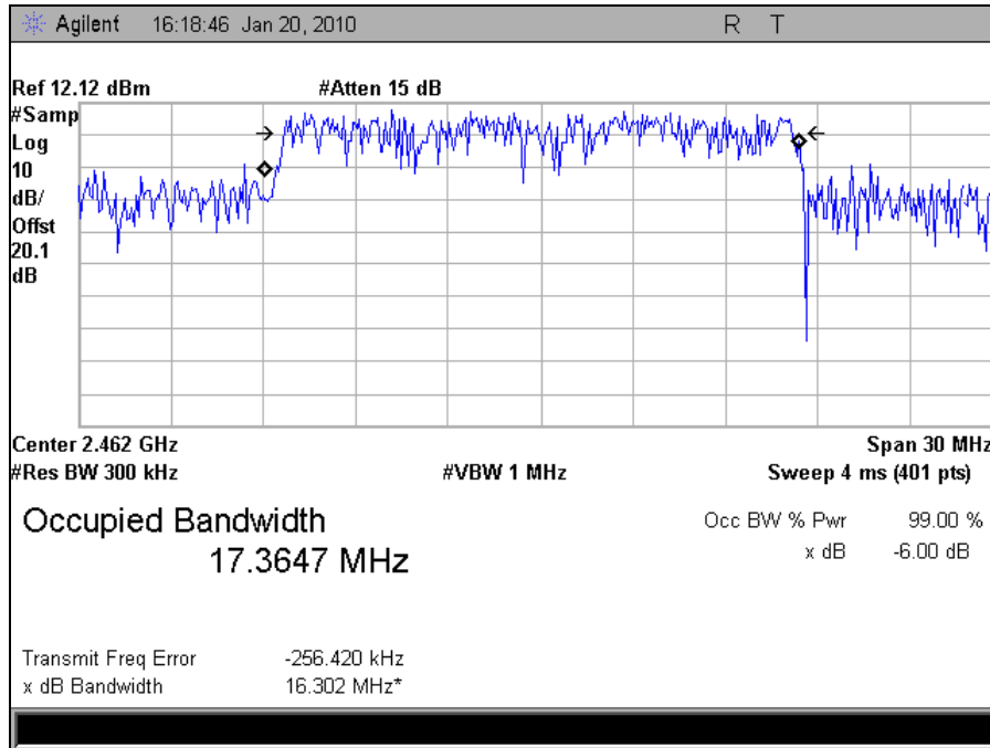
Plot 18. Occupied Bandwidth High Channel, 802.11g (99%)
