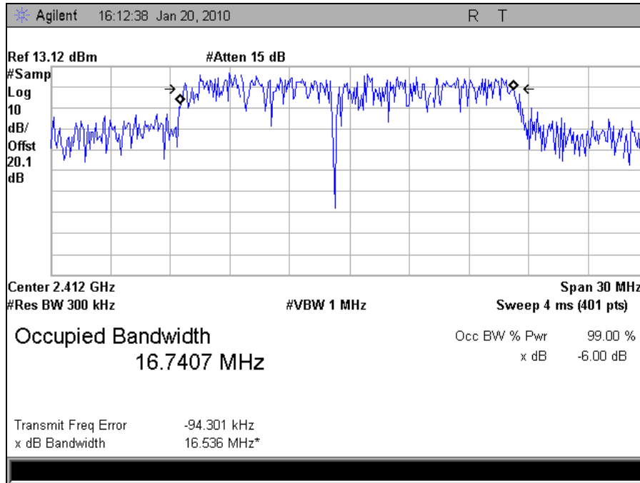
Plot 14. Occupied Bandwidth Low Channel, 802.11g (99%)
