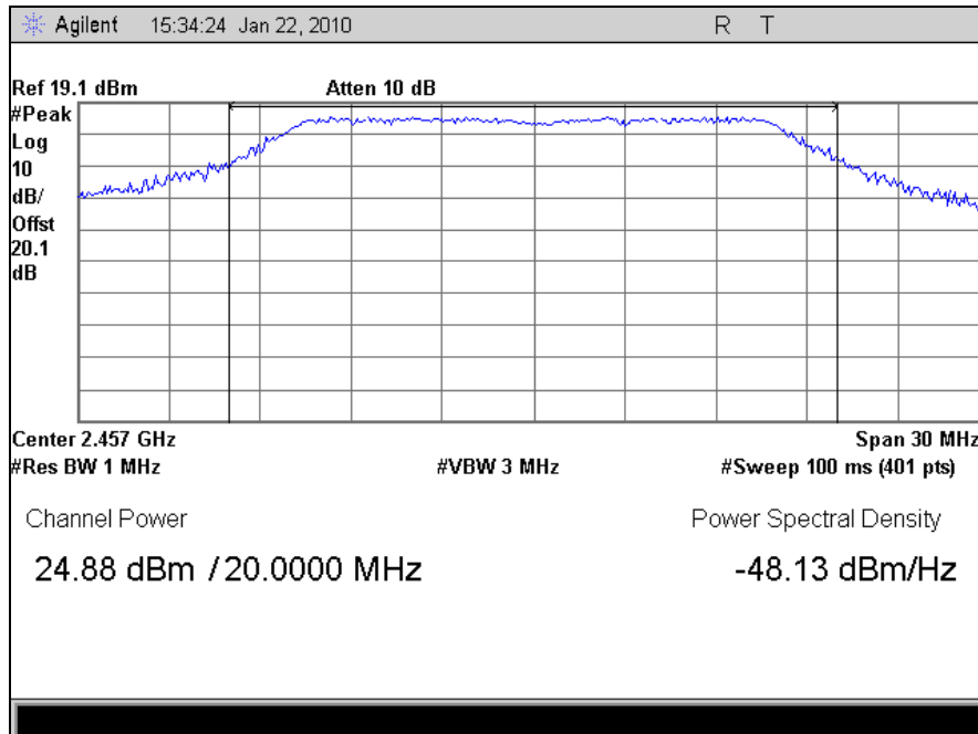
Plot 33. Peak Power Output, Channel 10, 802.11g
