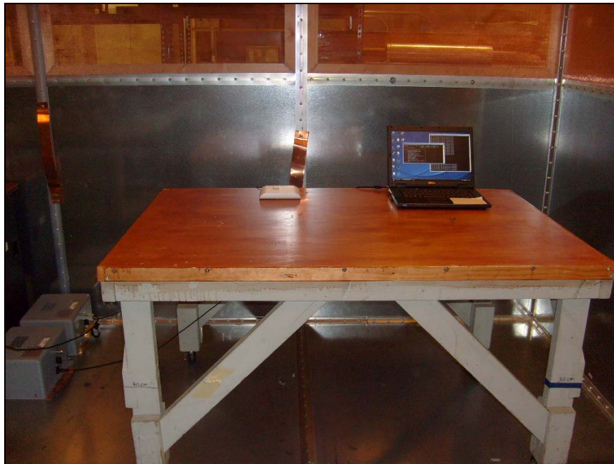
Photograph 5. Conducted Emissions, 15.207, Test Setup
