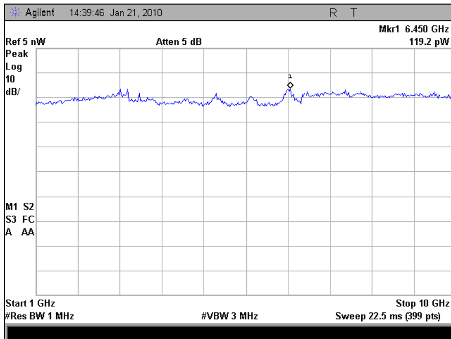
Plot 69. Receiver Spurious Emission, 1 GHz – 10 GHz, Vertical
