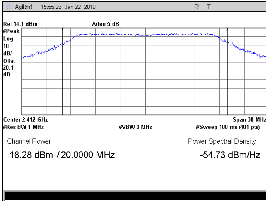
Plot 34. Peak Power Output, 802.11n, Low Channel
