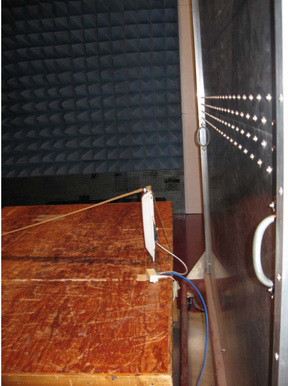
Photograph 5. Conducted Emissions Test Setup
