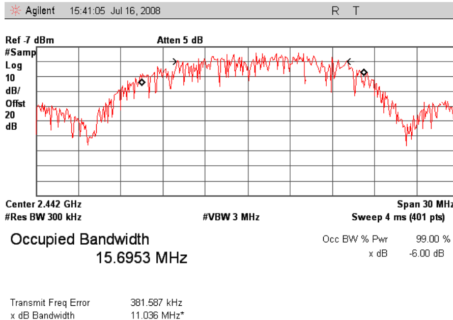
Plot 3. 802.11/b Mid Ch Occupied Band Width
