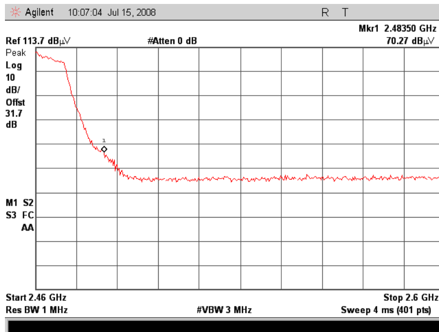
Plot 15. Radiated Band Edge High Channel, Peak
