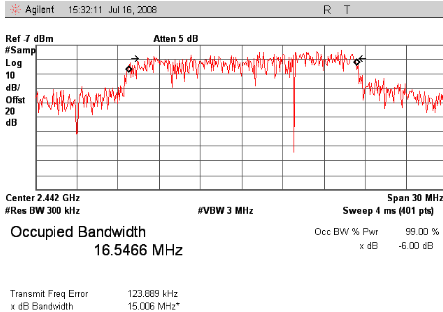
Plot 6. 802.11/g Mid Ch Occupied Band Width
