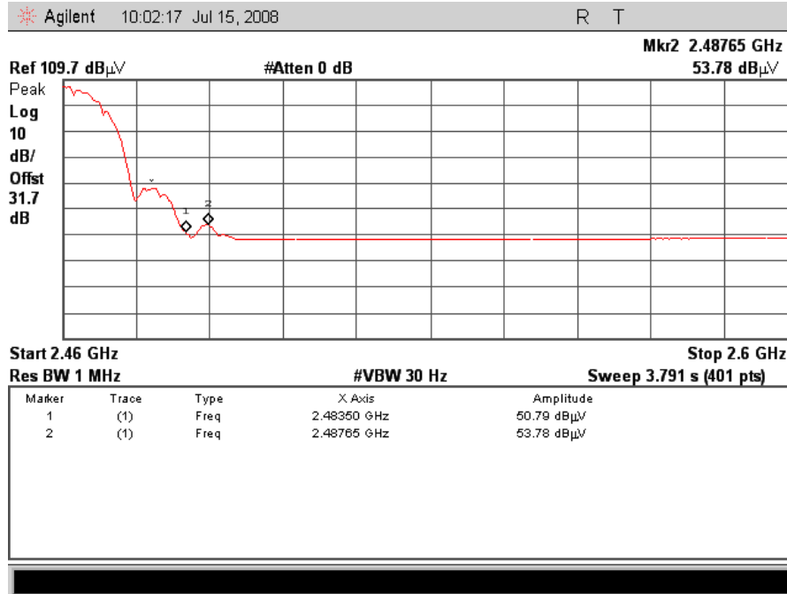
Plot 10. Radiated Band Edge High Channel, Avg
