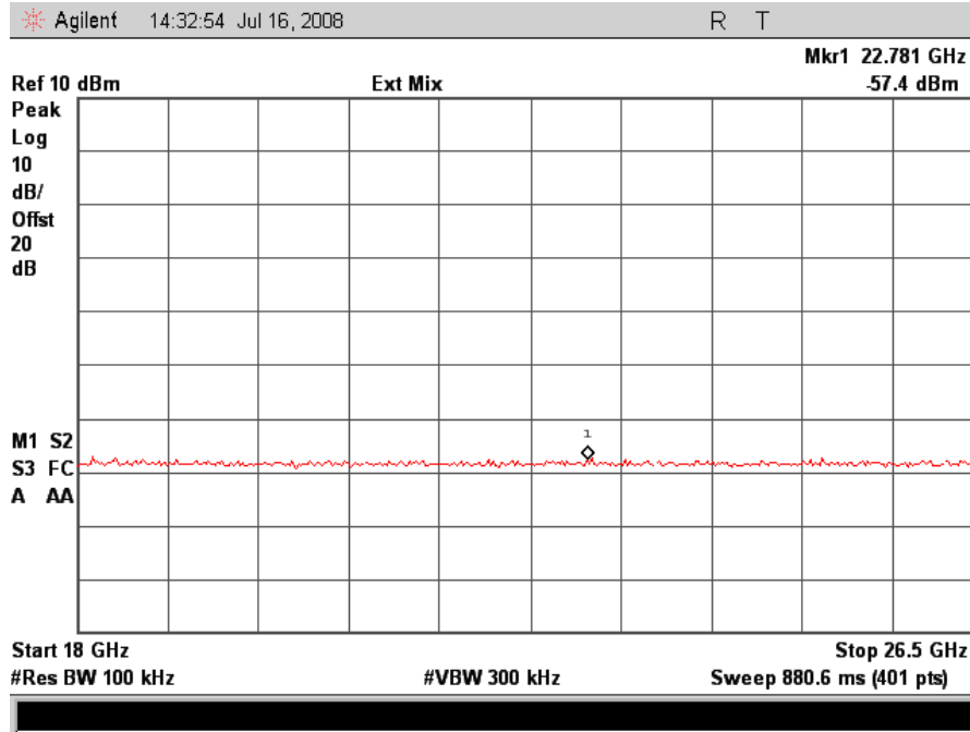
802.11/g – High Channel Conducted Emissions 18GHz – 26GHz
