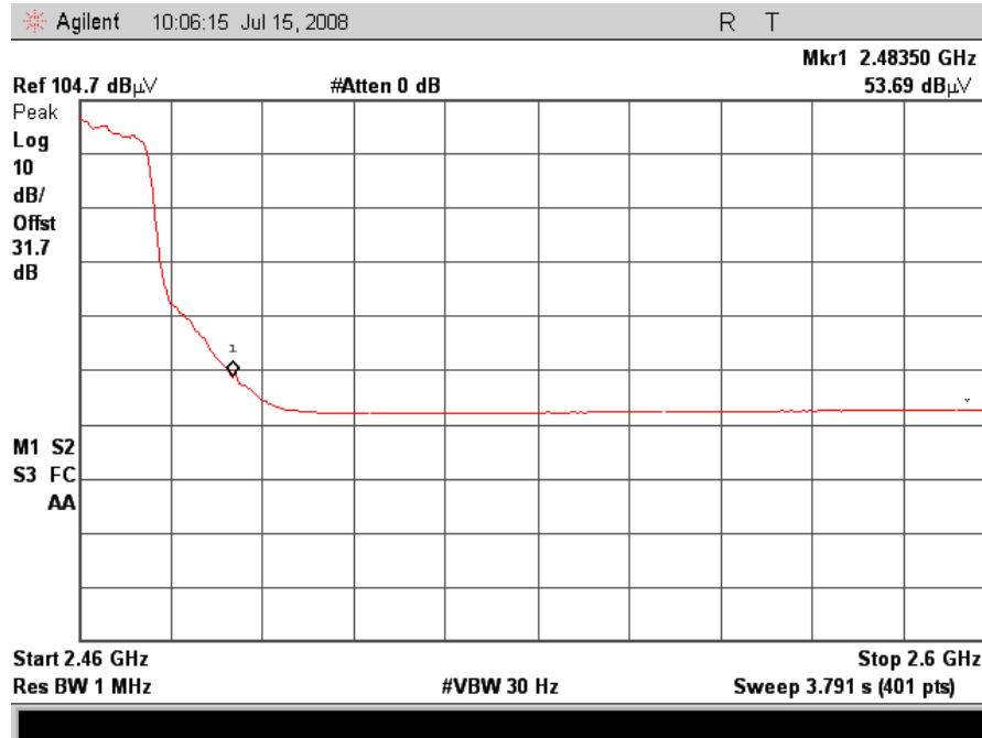
Plot 14. Radiated Band Edge High Channel, Avg
