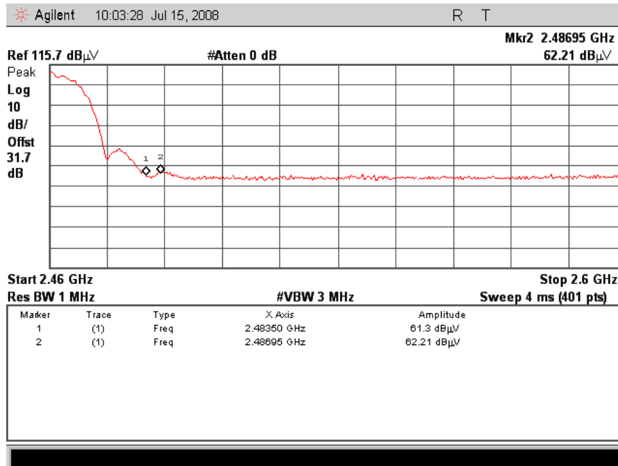
Plot 11. Radiated Band Edge High Channel, Peak
