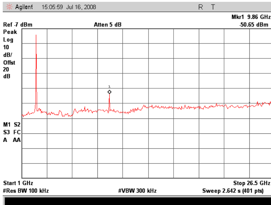
802.11/b – High Channel Conducted Emissions 1-26GHz
