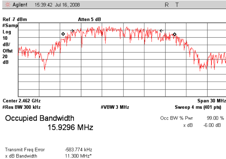
Plot 4. 802.11/b High Ch Occupied Band Width
