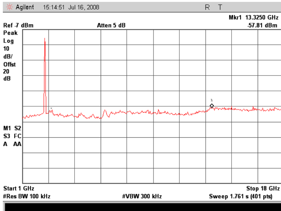
802.11/g – High Channel Conducted Emissions 1-18GHz
