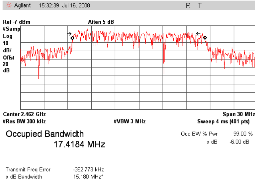
Plot 7. 802.11/g High Ch Occupied Band Width
