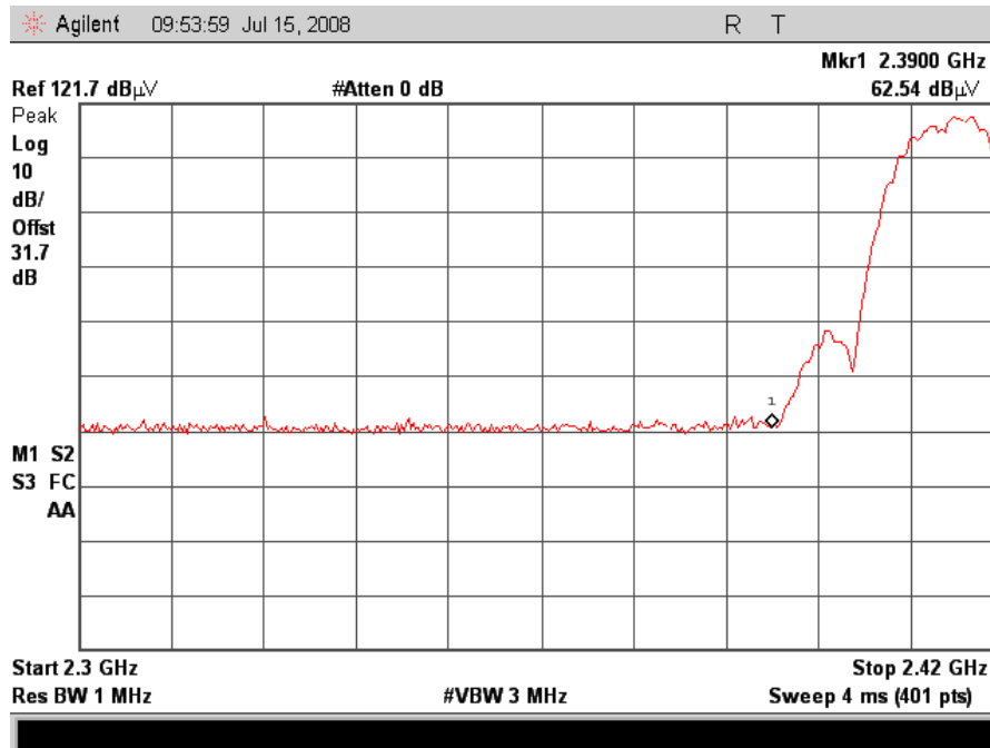
Plot 9. Radiated Band Edge Low Channel, Peak
