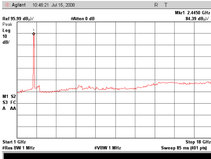
Plot 21. Radiated Spurious, High Channel, 1-18GHz
