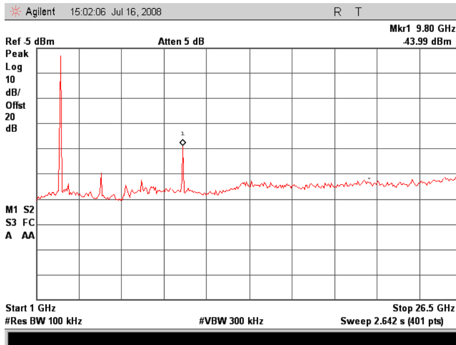
802.11/b – Mid Channel Conducted Emissions 1-26GHz
