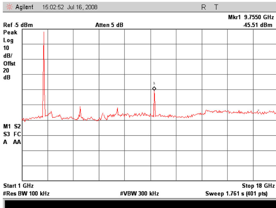
802.11/b – Mid Channel Conducted Emissions 1 - 18GHz
