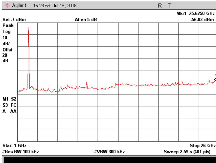
802.11/g – Low Channel Conducted Emissions 1-26GHz
