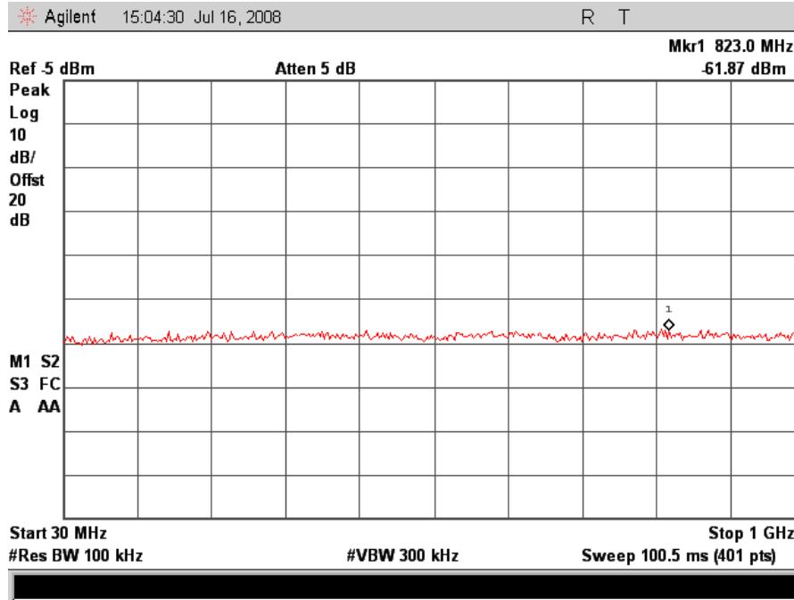
802.11/b – High Channel Conducted Emissions 30MHz- 1GHz
