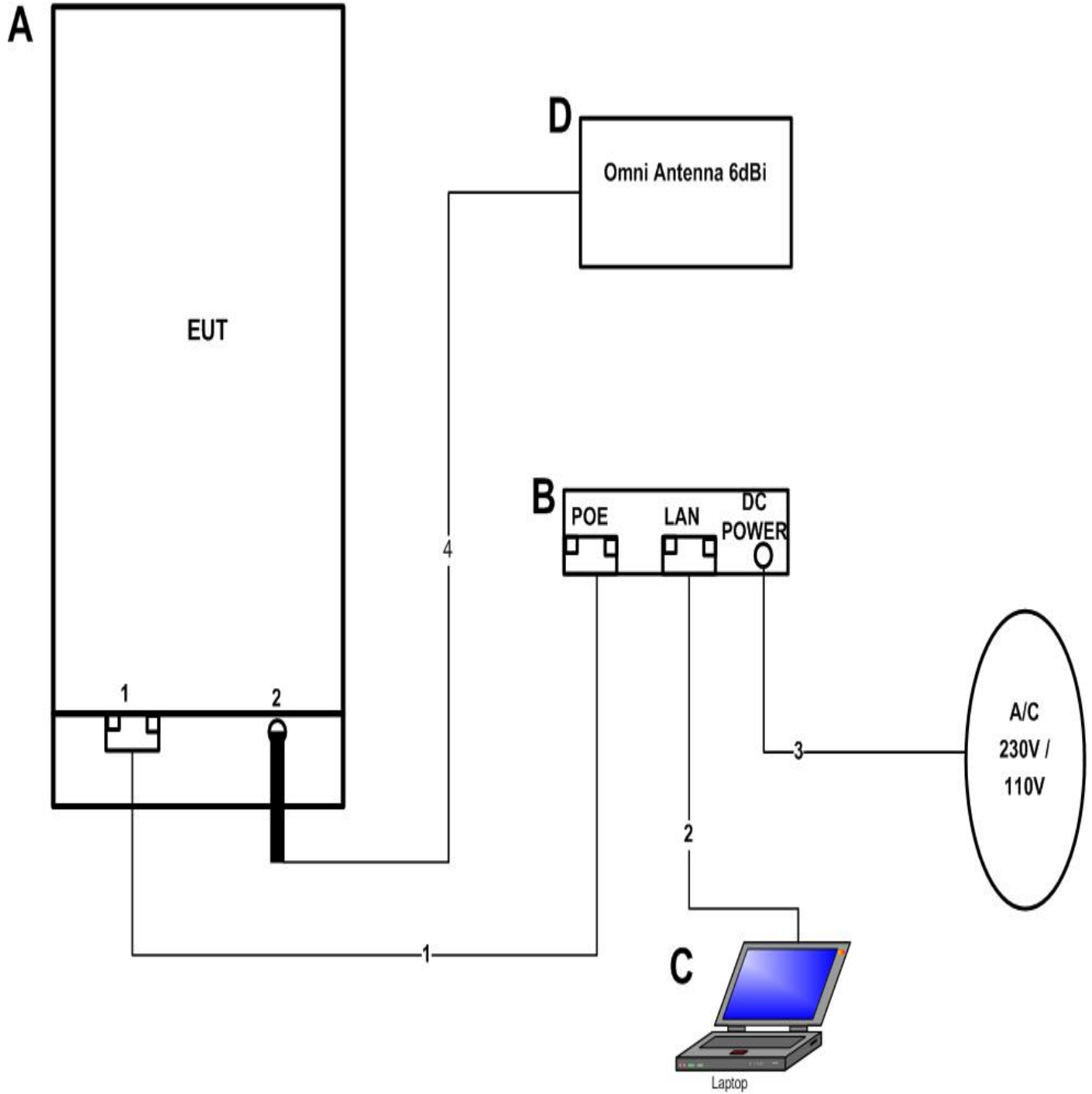
Figure 1. Block Diagram of Test Configuration (Radiated Emissions)
