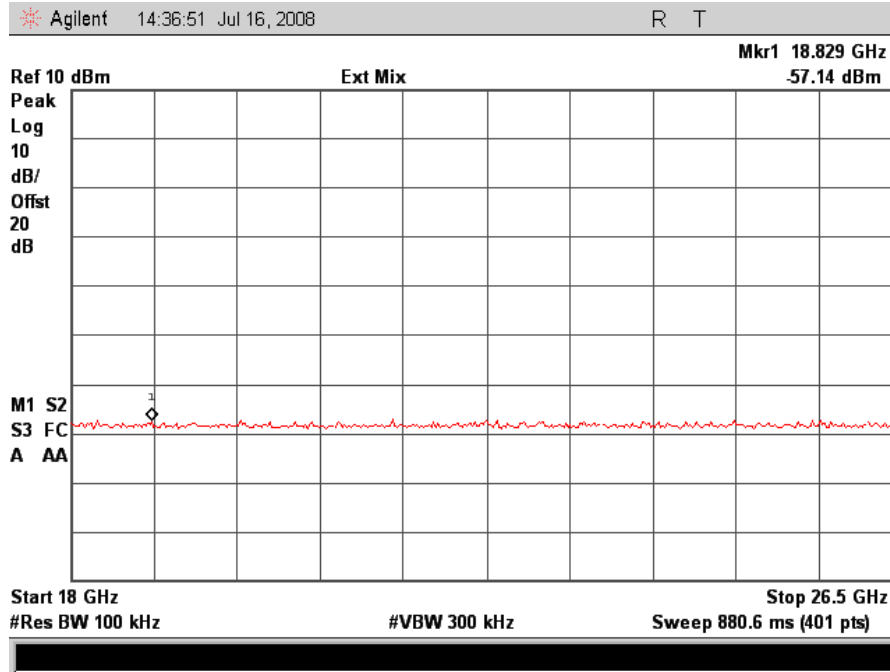
802.11/b – Low Channel Conducted Emissions 18-26GHz
