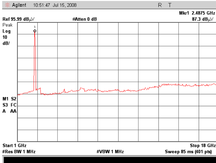
Plot 18. Radiated Spurious, High Channel, 1-18GHz
