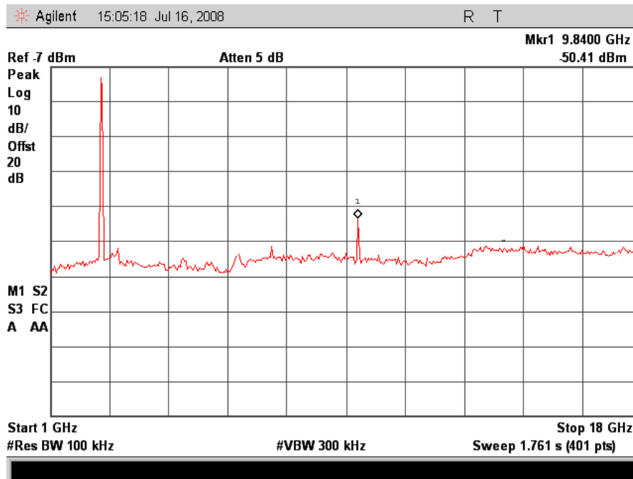
802.11/b – High Channel Conducted Emissions 1-18GHz
