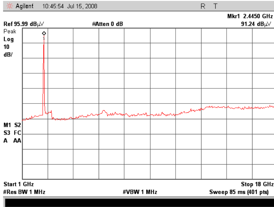
Plot 19. Radiated Spurious, Low Channel, 1-18GHz
