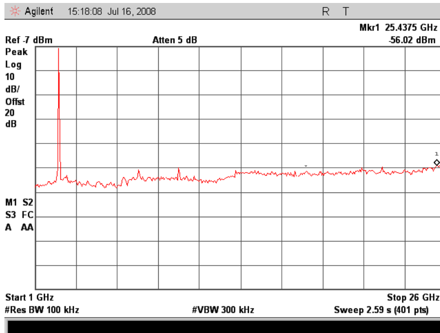
802.11/g – Mid Channel Conducted Emissions 1-26GHz
