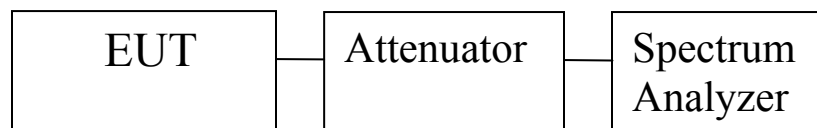
Block Diagram 4. Peak Power Spectral Density Test Setup
