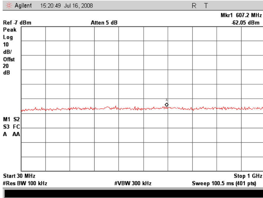
802.11/g – Mid Channel Conducted Emissions 30MHz – 1GHz
