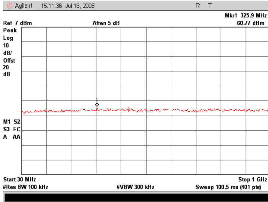
802.11/g – High Channel Conducted Emissions 30MHz – 1GHz
