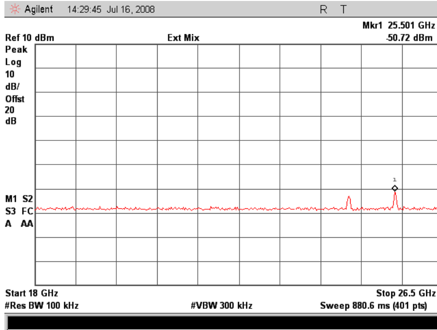
802.11/g – Low Channel Conducted Emissions 18GHz – 26GHz
