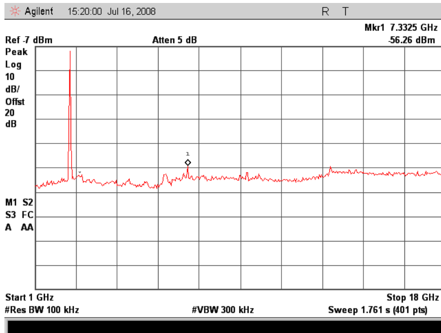
802.11/g – Mid Channel Conducted Emissions 1-18GHz
