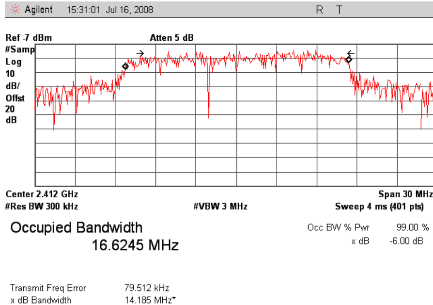
Plot 5. 802.11/g Low Ch Occupied Band Width
