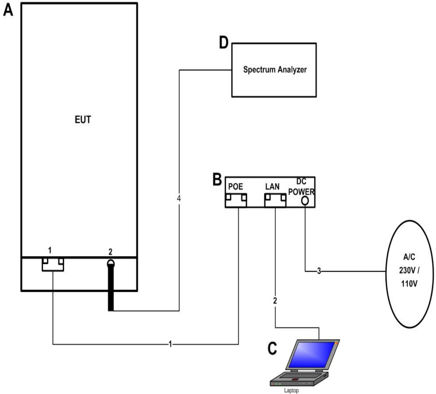
Figure 2. Block Diagram of Test Configuration (Conducted Measurement)
