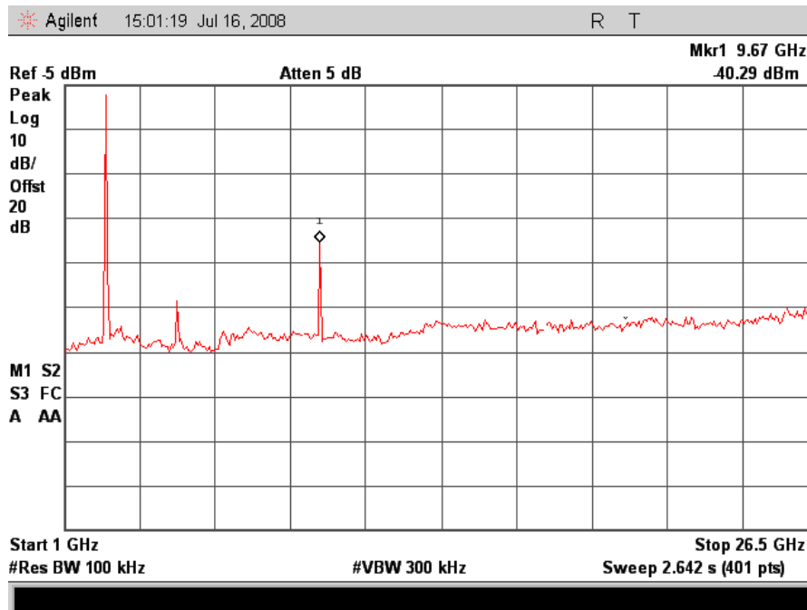
802.11/b – Low Channel Conducted Emissions 1-26GHz
