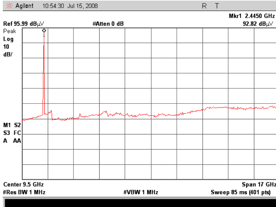
Plot 16. Radiated Spurious, Low Channel, 1-18GHz
