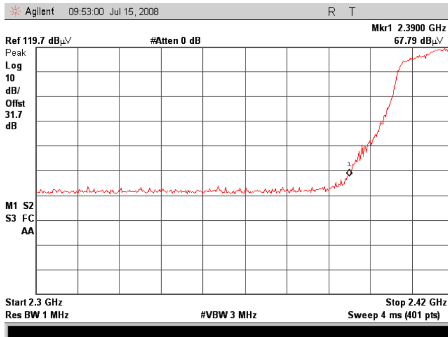
Plot 13. Radiated Band Edge Low Channel, Peak
