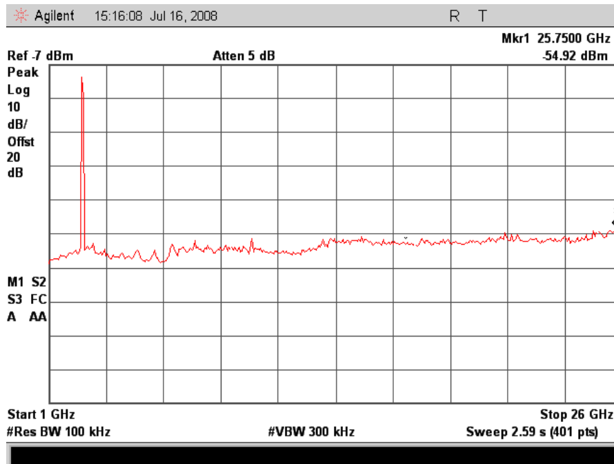
802.11/g – High Channel Conducted Emissions 1-26GHz
