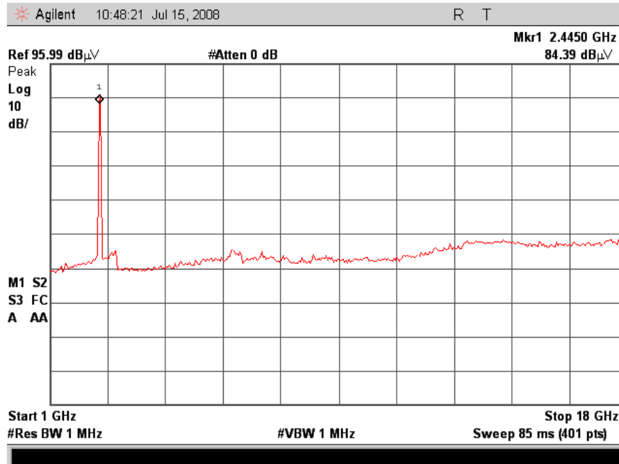
Plot 20. Radiated Spurious, Mid Channel, 1-18GHz
