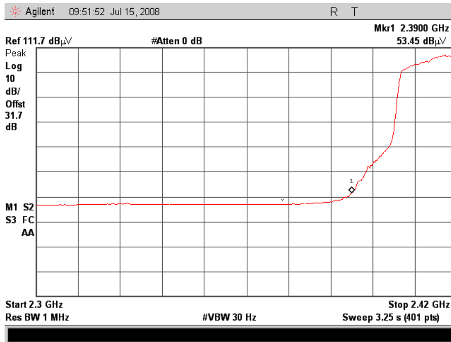
Plot 12. Radiated Band Edge Low Channel, Avg
