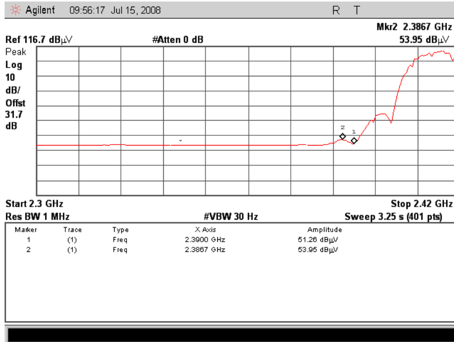
Plot 8. Radiated Band Edge Low Channel, Avg
