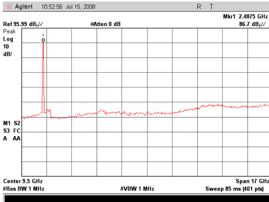
Plot 17. Radiated Spurious, Mid Channel, 1-18GHz
