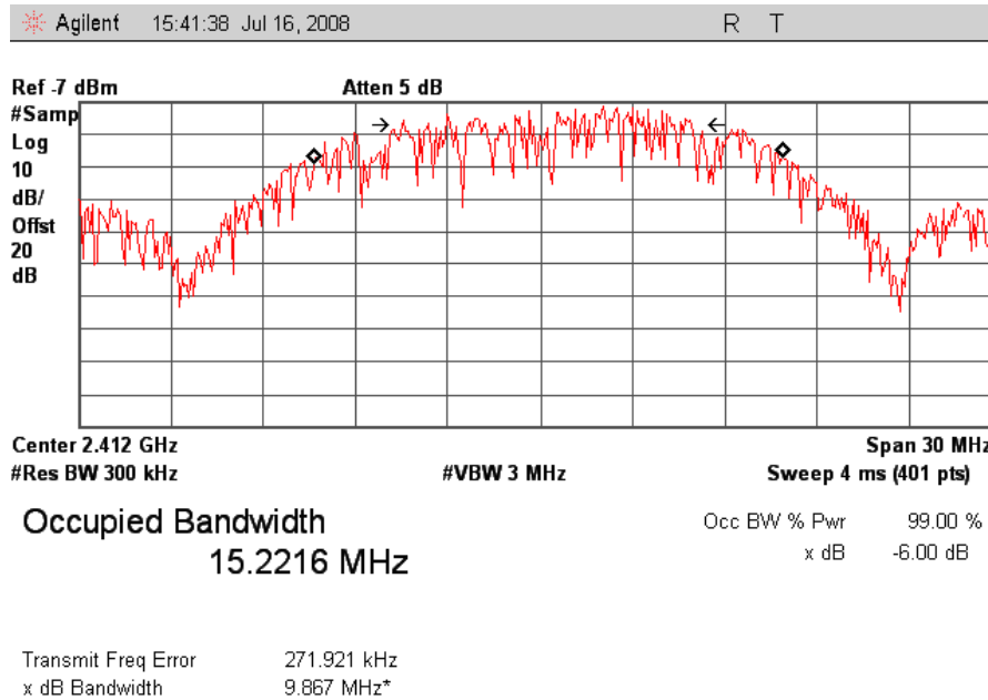
Plot 2. 802.11/b Low Ch Occupied Band Width.
