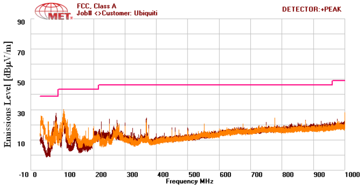
Plot 1. Radiated Emissions 30MHz – 1GHz Plot
