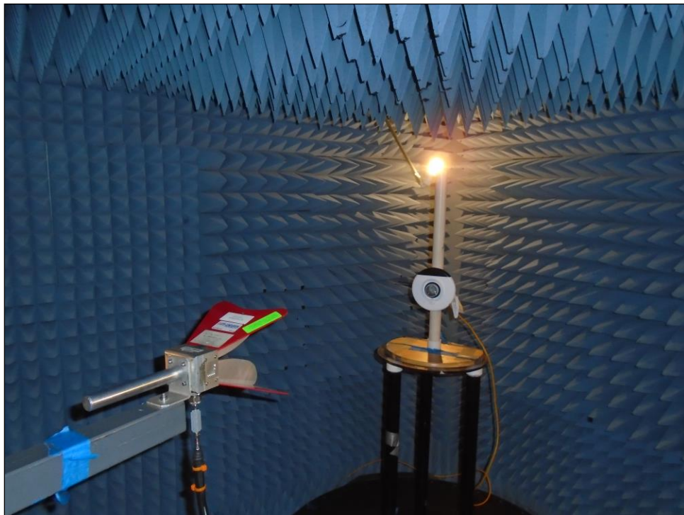
Photograph 3. Radiated Spurious Emissions, Test Setup, Above 1 GHz
