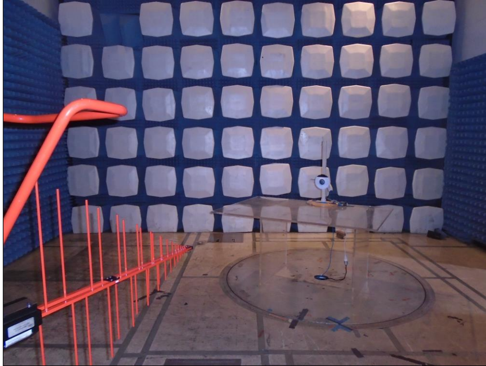
Photograph 2. Radiated Spurious Emissions, Test Setup, Up to 1 GHz
