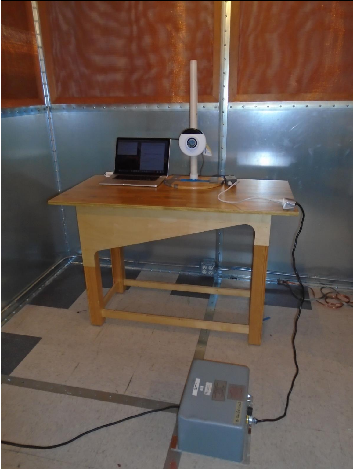
Photograph 1. Conducted Emissions, 15.207(a), Test Setup
