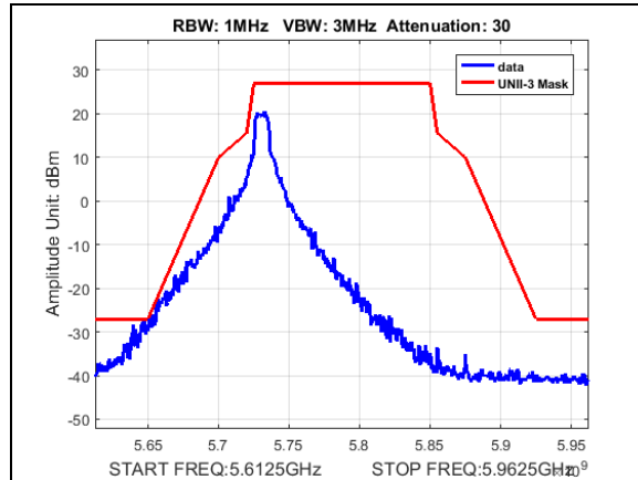
Plot 168. Undesirable Emissions, UNII3, emission mask, BW 10M, CF 5730M, 19dBm
