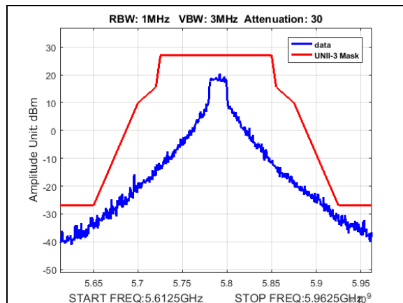
Plot 179. Undesirable Emissions, UNII3, emission mask, BW 20M, CF 5790M, 13dBm
