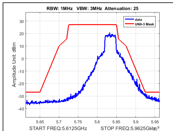
Plot 193. Undesirable Emissions, UNII3, emission mask, BW 30M, CF 5835M, 27dBm
