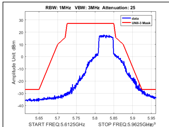
Plot 202. Undesirable Emissions, UNII3, emission mask, BW 40M, CF 5830M, 27dBm
