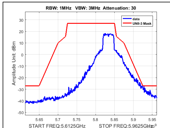
Plot 191. Undesirable Emissions, UNII3, emission mask, BW 30M, CF 5835M, 13dBm
