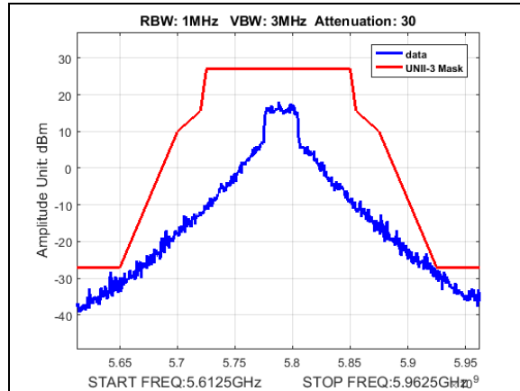
Plot 189. Undesirable Emissions, UNII3, emission mask, BW 30M, CF 5790M, 19dBm
