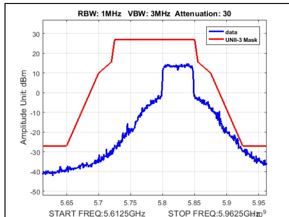
Plot 209. Undesirable Emissions, UNII3, emission mask, BW 50M, CF 5825M, 13dBm
