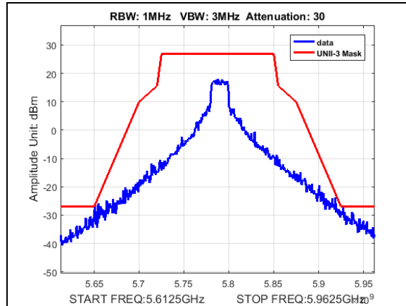
Plot 180. Undesirable Emissions, UNII3, emission mask, BW 20M, CF 5790M, 19dB
