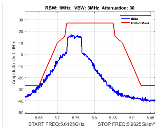
Plot 194. Undesirable Emissions, UNII3, emission mask, BW 40M, CF 5745M, 13dBm
