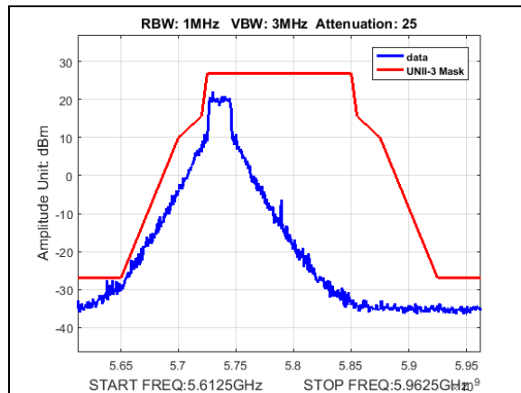
Plot 178. Undesirable Emissions, UNII3, emission mask, BW 20M, CF 5735M, 27dBm
