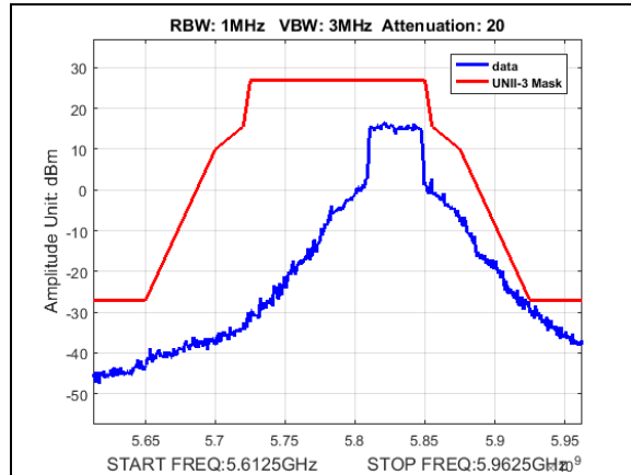
Plot 201. Undesirable Emissions, UNII3, emission mask, BW 40M, CF 5830M, 19dBm
