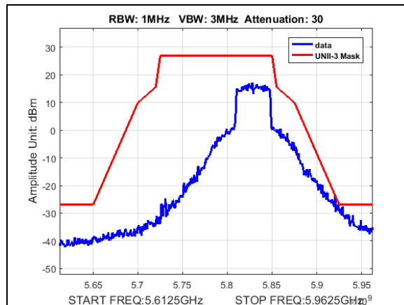
Plot 200. Undesirable Emissions, UNII3, emission mask, BW 40M, CF 5830M, 13dBm
