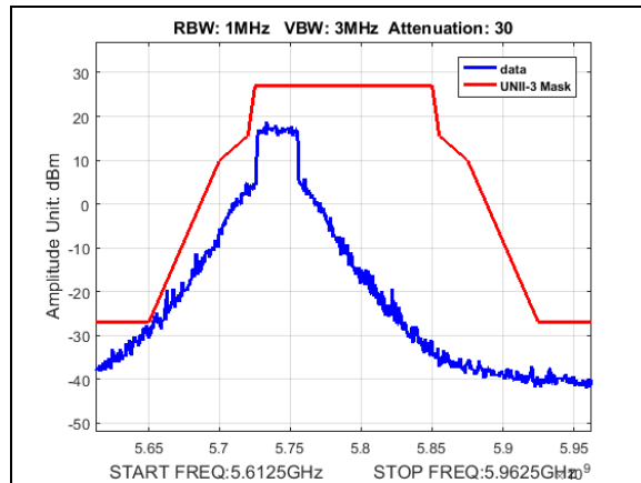
Plot 185. Undesirable Emissions, UNII3, emission mask, BW 30M, CF 5740M, 13dBm
