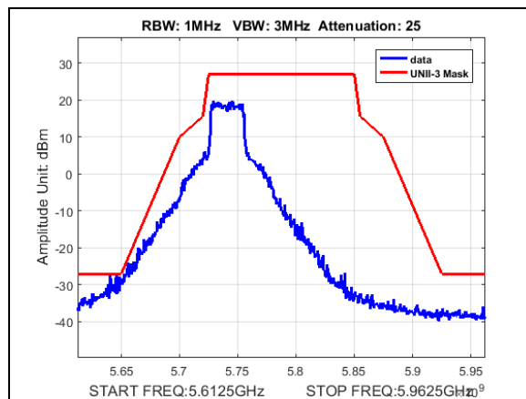
Plot 187. Undesirable Emissions, UNII3, emission mask, BW 30M, CF 5740M, 27dBm
