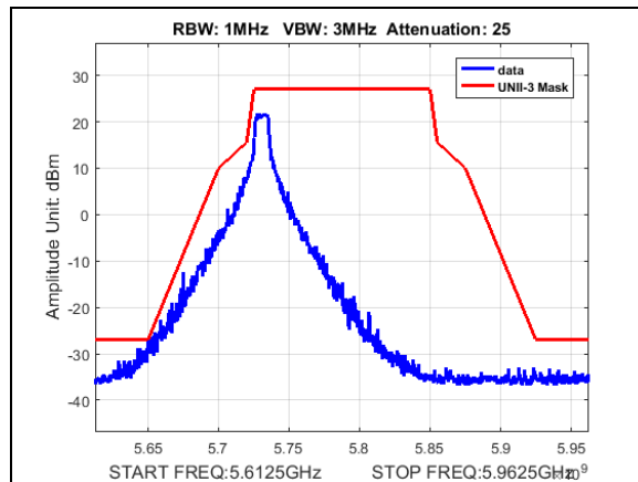
Plot 169. Undesirable Emissions, UNII3, emission mask, BW 10M, CF 5730M, 27dBm
