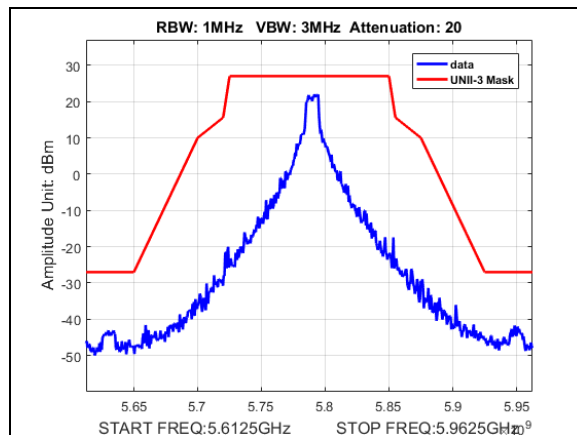
Plot 170. Undesirable Emissions, UNII3, emission mask, BW 10M, CF 5790M, 13dBm
