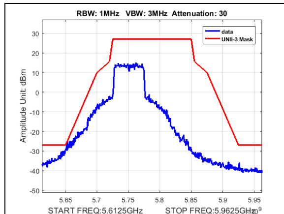
Plot 203. Undesirable Emissions, UNII3, emission mask, BW 50M, CF 5750M, 13dBm
