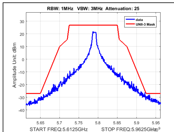
Plot 172. Undesirable Emissions, UNII3, emission mask, BW 10M, CF 5790M, 27dBm
