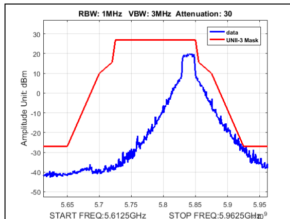
Plot 182. Undesirable Emissions, UNII3, emission mask, BW 20M, CF 5840M, 13dB
