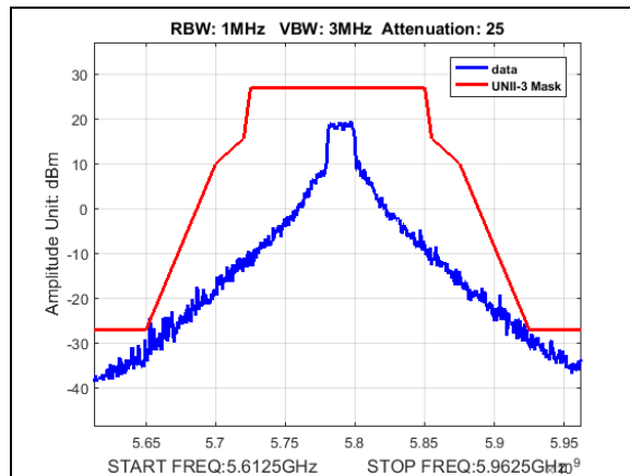
Plot 181. Undesirable Emissions, UNII3, emission mask, BW 20M, CF 5790M, 27dB
