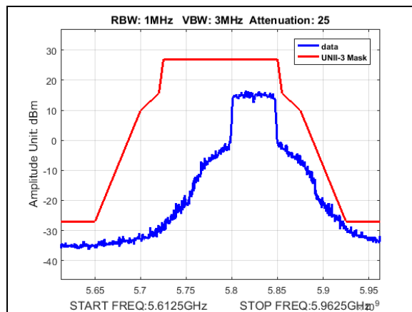
Plot 211. Undesirable Emissions, UNII3, emission mask, BW 50M, CF 5825M, 27dBi
