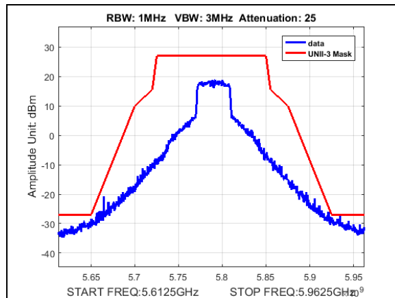
Plot 199. Undesirable Emissions, UNII3, emission mask, BW 40M, CF 5790M, 27dBm
