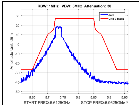
Plot 177. Undesirable Emissions, UNII3, emission mask, BW 20M, CF 5735M, 19dBm
