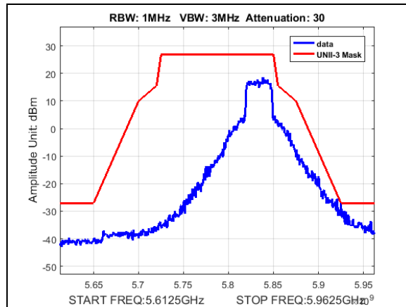
Plot 192. Undesirable Emissions, UNII3, emission mask, BW 30M, CF 5835M, 19dBm
