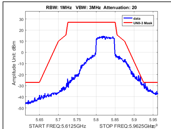
Plot 210. Undesirable Emissions, UNII3, emission mask, BW 50M, CF 5825M, 19dBi
