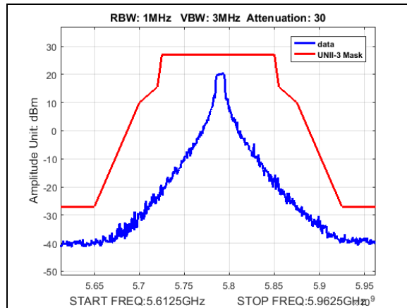
Plot 171. Undesirable Emissions, UNII3, emission mask, BW 10M, CF 5790M, 19dBm
