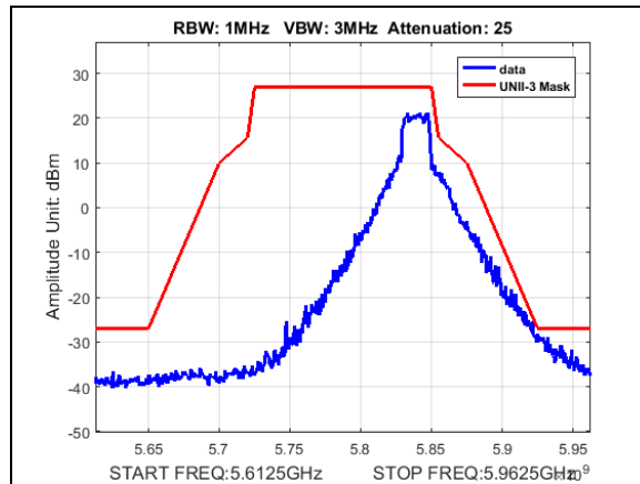
Plot 184. Undesirable Emissions, UNII3, emission mask, BW 20M, CF 5840M, 27dBm
