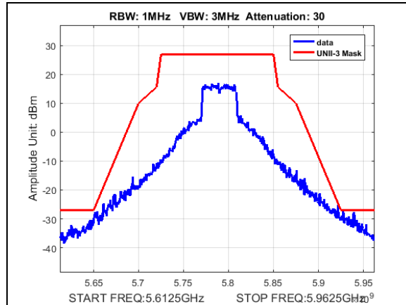
Plot 198. Undesirable Emissions, UNII3, emission mask, BW 40M, CF 5790M, 19dBm
