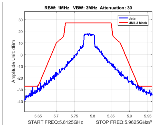
Plot 188. Undesirable Emissions, UNII3, emission mask, BW 30M, CF 5790M, 13dBm
