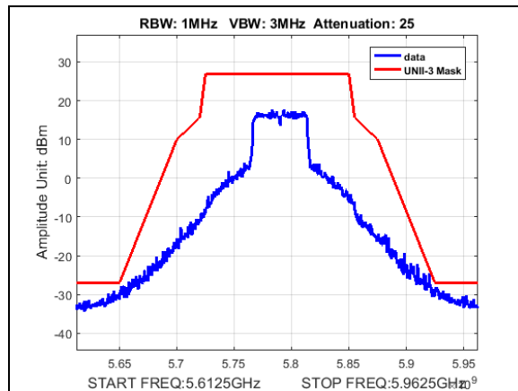
Plot 208. Undesirable Emissions, UNII3, emission mask, BW 50M, CF 5790M, 27dBm
