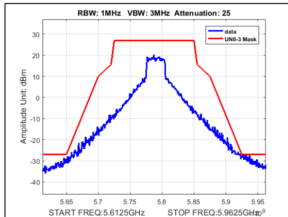
Plot 190. Undesirable Emissions, UNII3, emission mask, BW 30M, CF 5790M, 27dBm
