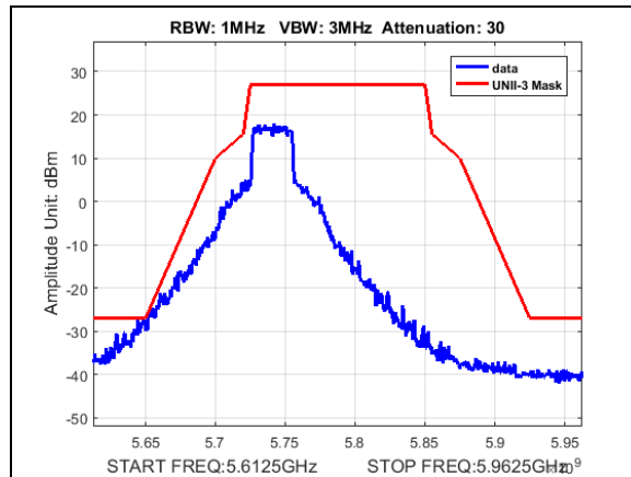
Plot 186. Undesirable Emissions, UNII3, emission mask, BW 30M, CF 5740M, 19dBm
