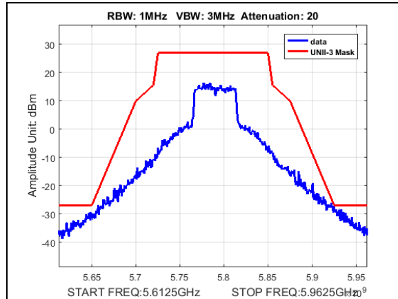
Plot 207. Undesirable Emissions, UNII3, emission mask, BW 50M, CF 5790M, 19dBm
