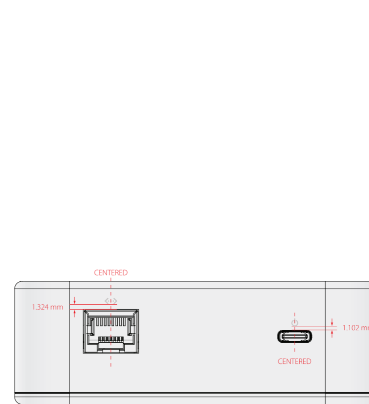
Back View
