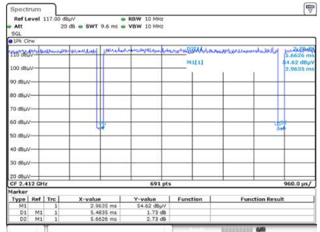
Modulation Type: 802.11ax HE20 (7.3Mbps)
