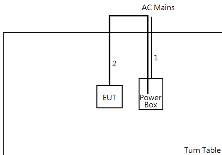
Test Setup Diagram - Radiated Test (Below 1G)
