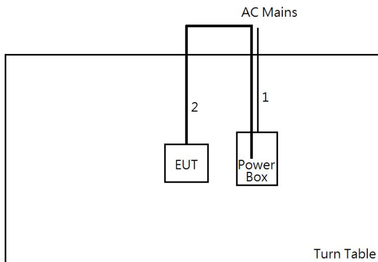
Test Setup Diagram - Radiated Test (Above 1G)
