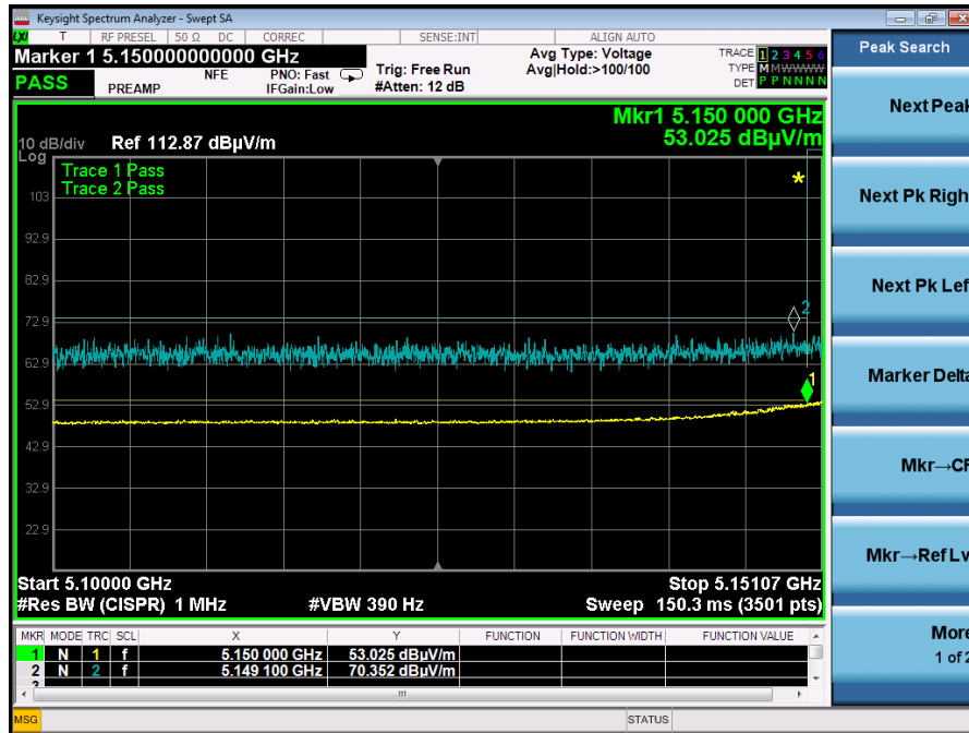
Graph 10: Band Edge ac Mode 80 MHz - 5210 MHz
