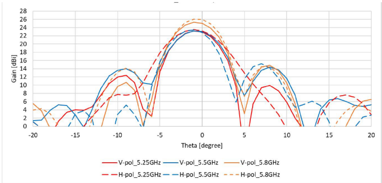
Graph 5: Elevation Plot (showing worse case)
