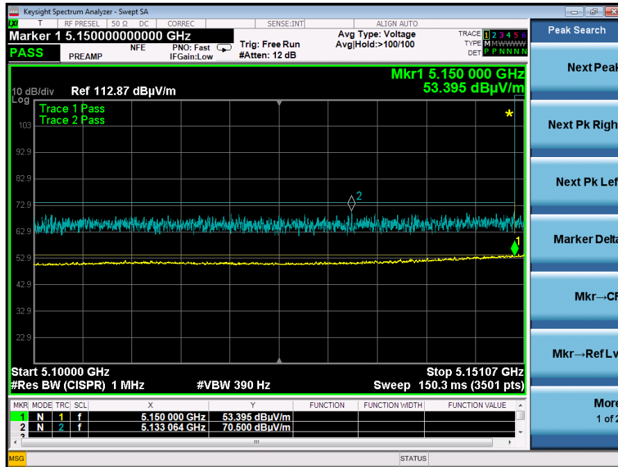
Graph 6: Band Edge ac Mode 20 MHz – 5180 MHz
