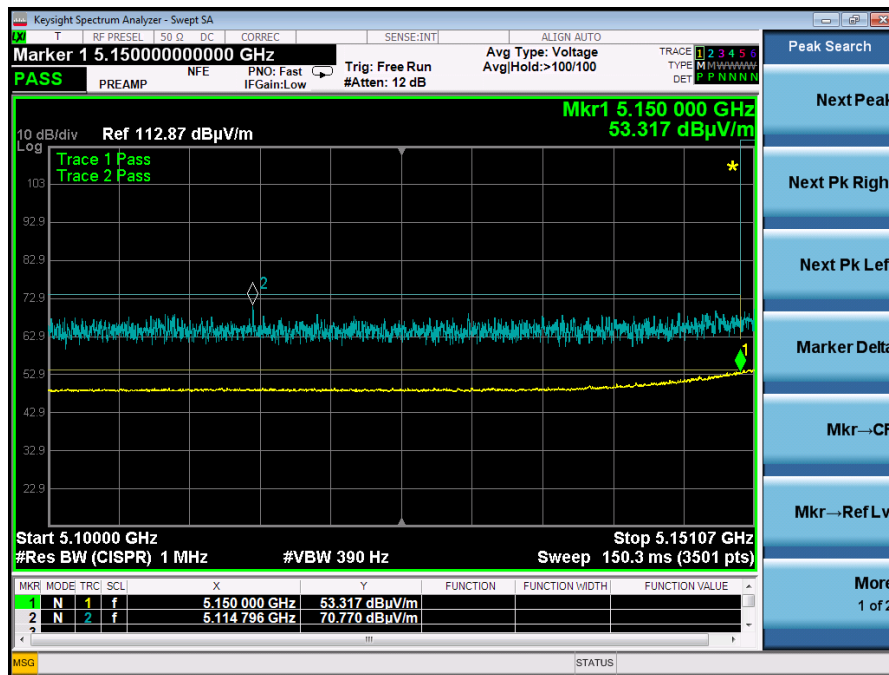
Graph 8: Band Edge ac Mode 40 MHz - 5190 MHz
