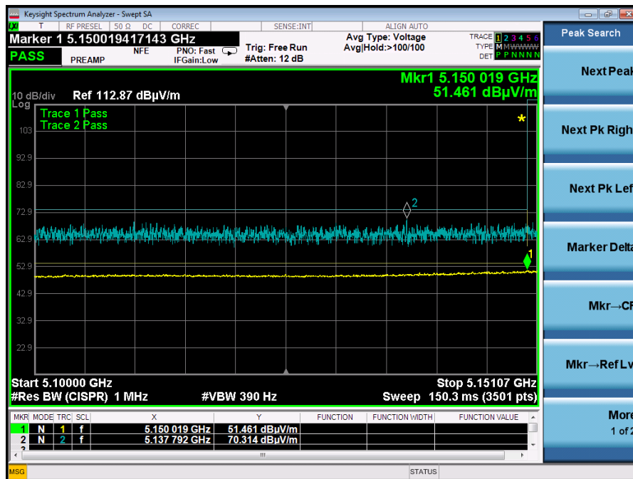
Graph 9: Band Edge ac Mode 40 MHz - 5230 MHz
