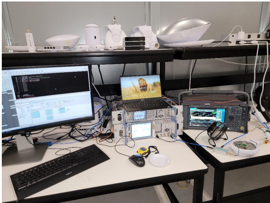
Photograph 6: DFS Test Setup
