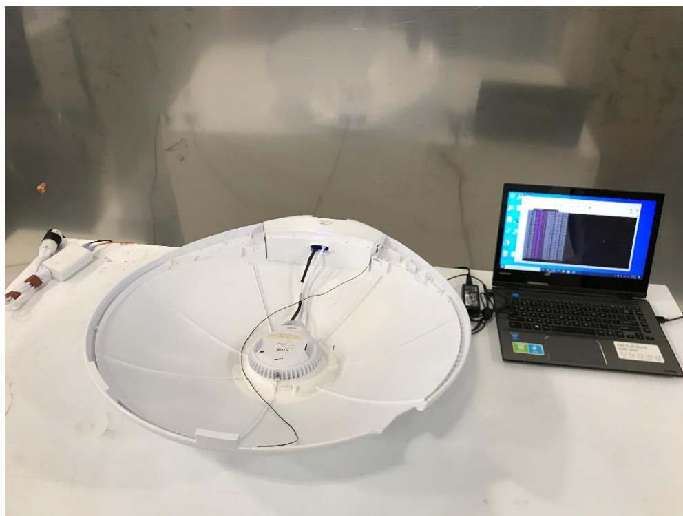
Photograph 4: Front View Test Set Up Conducted Emissions
