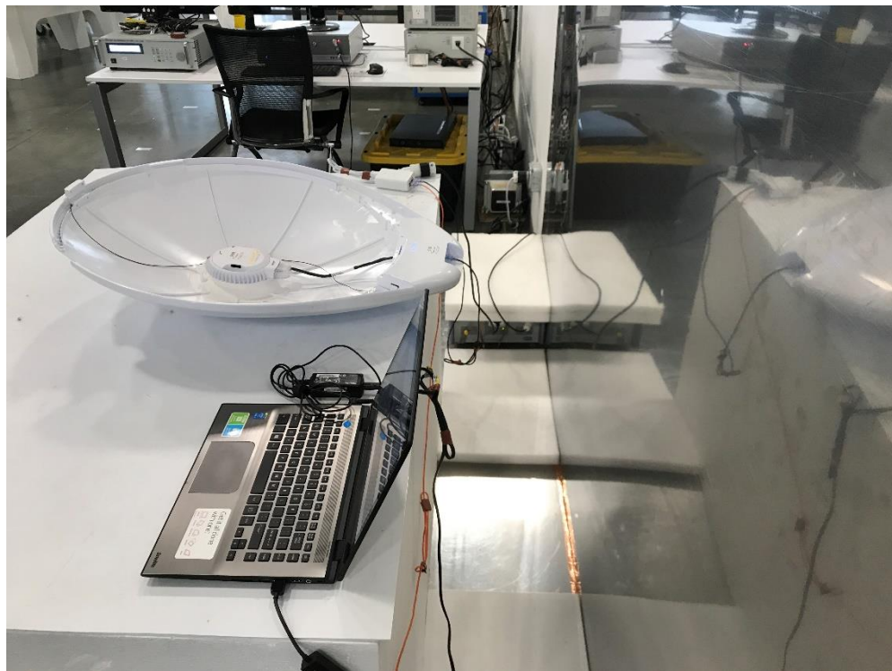
Photograph 5: Back View Test Set Up Conducted Emissions
