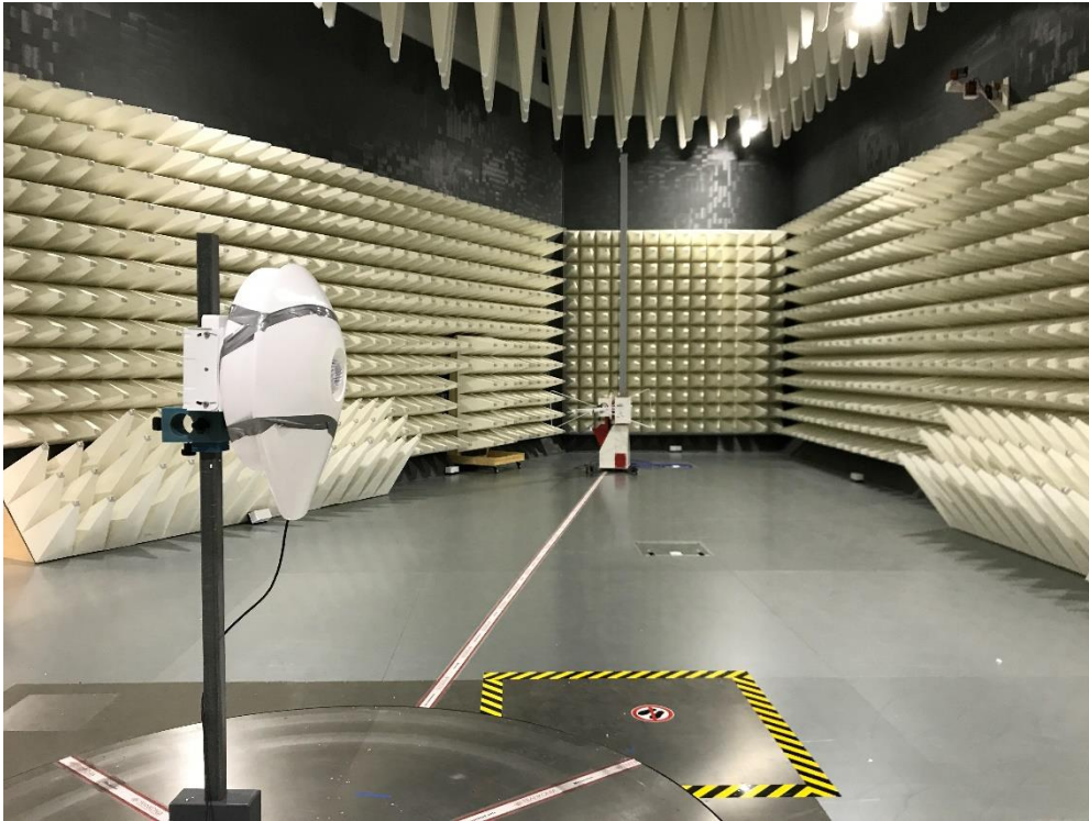
Photograph 1: Test Set Up Radiated Emissions 30 – 1000 MHz
