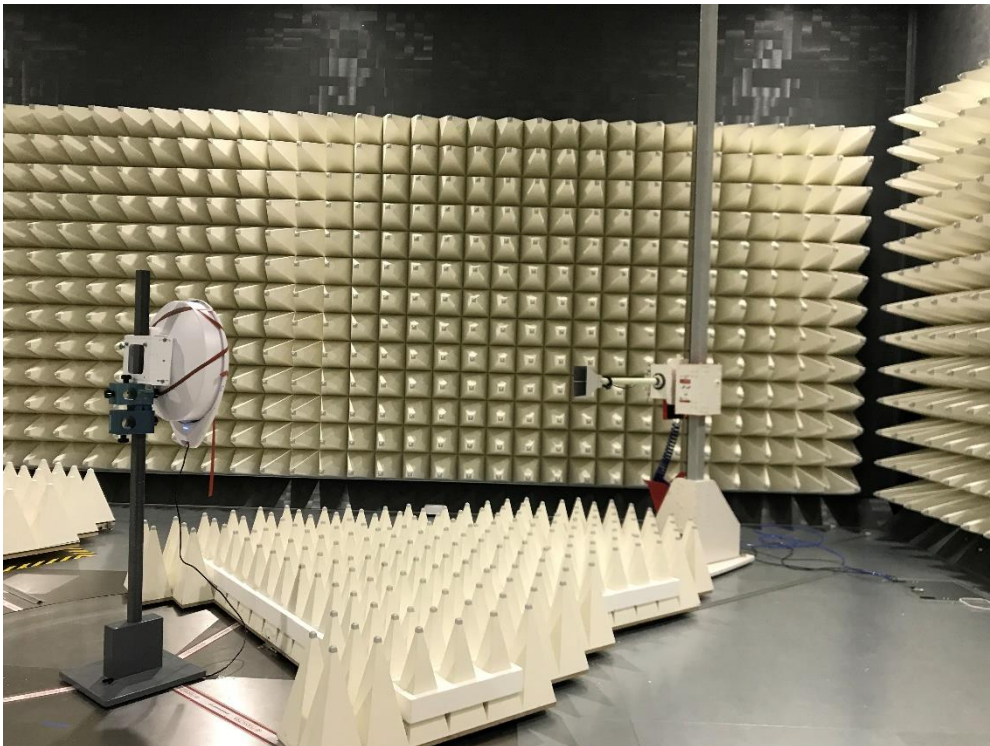
Photograph 2: Test Set Up Radiated Emissions 1 – 17 GHz
