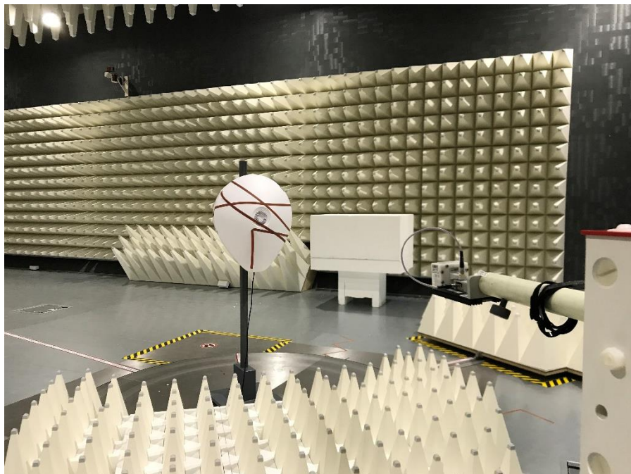
Photograph 3: Test Set Up Radiated Emissions 17 – 40 GHz
