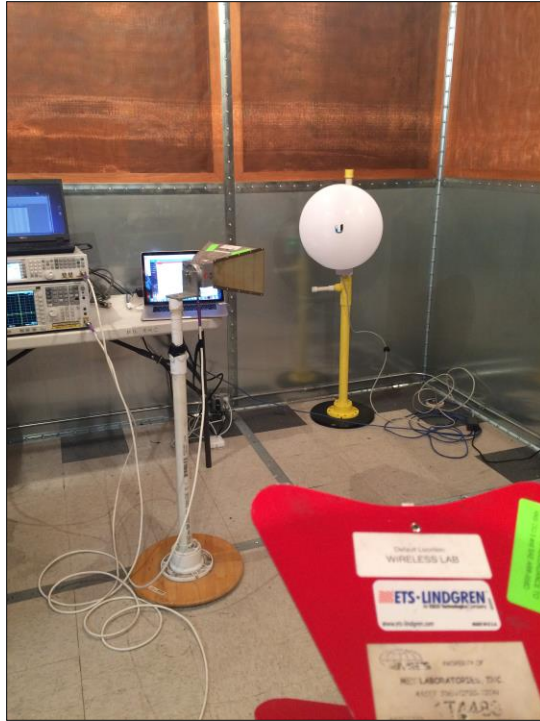
Photograph 1. DFS Setup for CACT and channel move and close time
