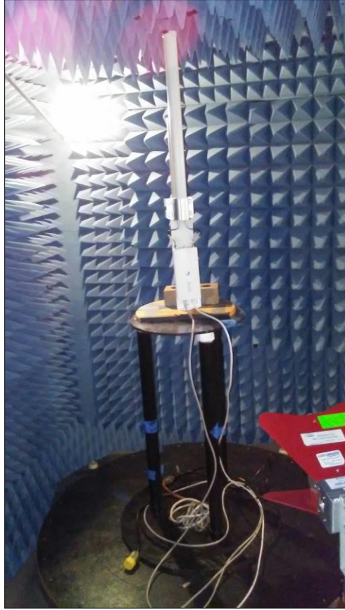
Photograph 6. Test Setup, Radiated Emissions Above 1GHz, 13dBi antenna
