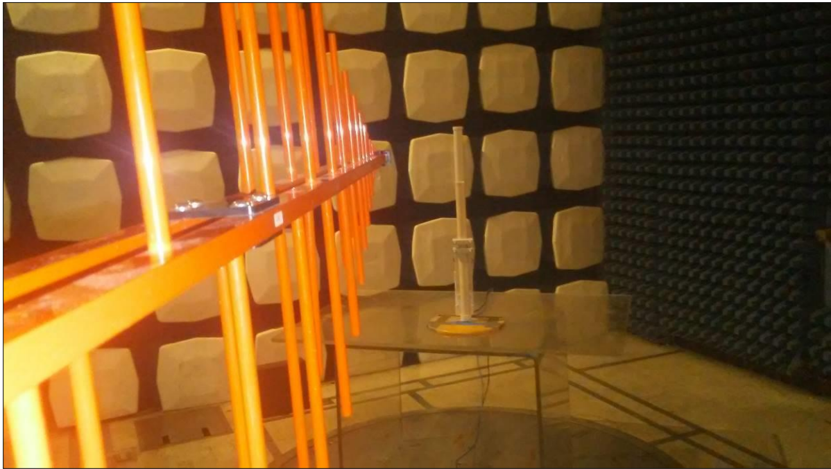
Photograph 5. Test Setup, Radiated Emissions Below 1GHz, 13dBi antenna
