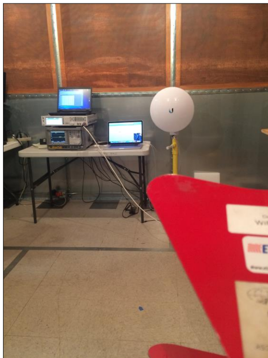
Photograph 2. DFS Setup for Detection Bandwidth and Statistical Analysis
